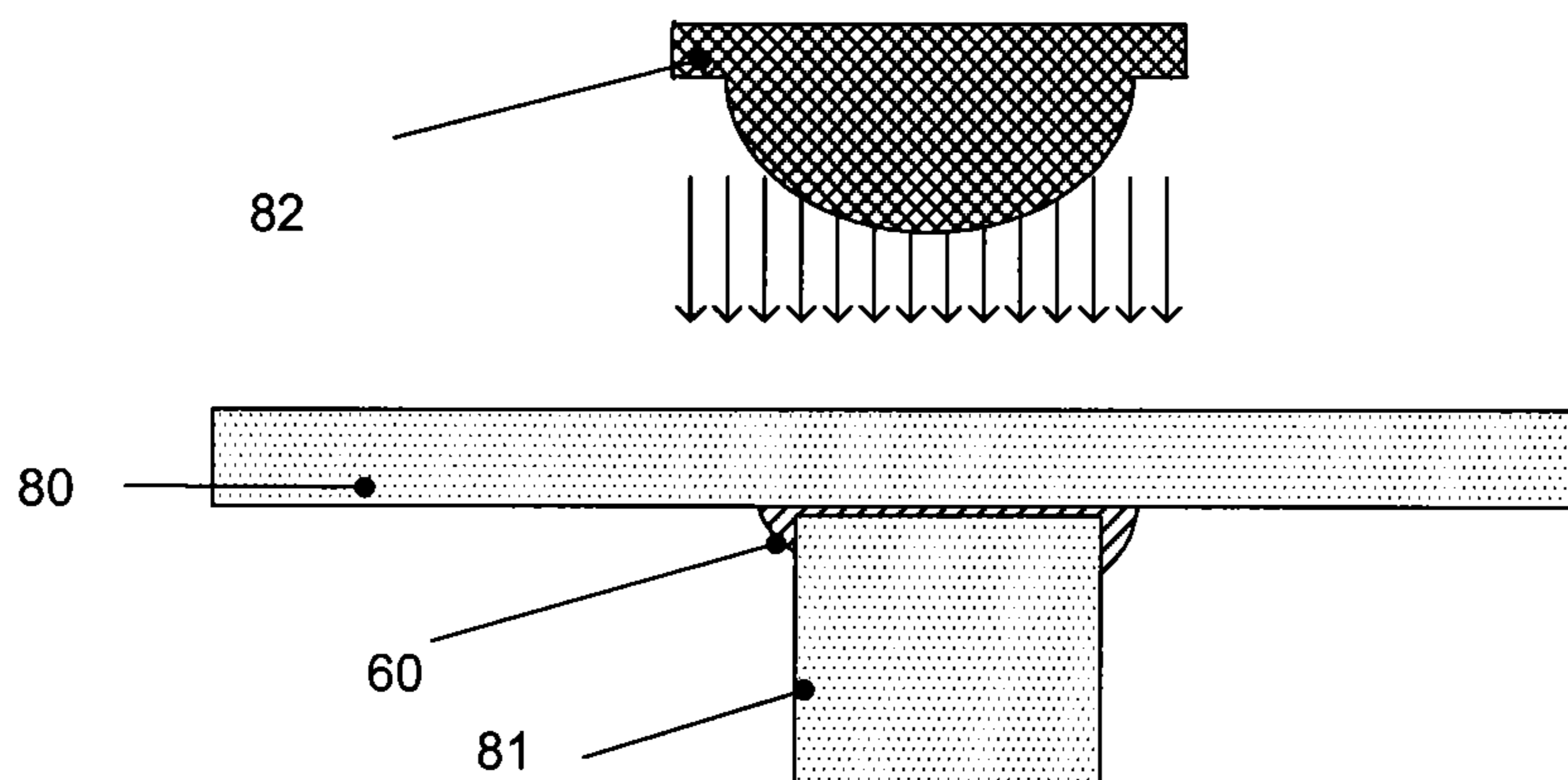
FIG. 31C - The assembly was turned upside down and cured under X-ray at 32-Kvp and 20mA. The X-ray target was Tungsten.
