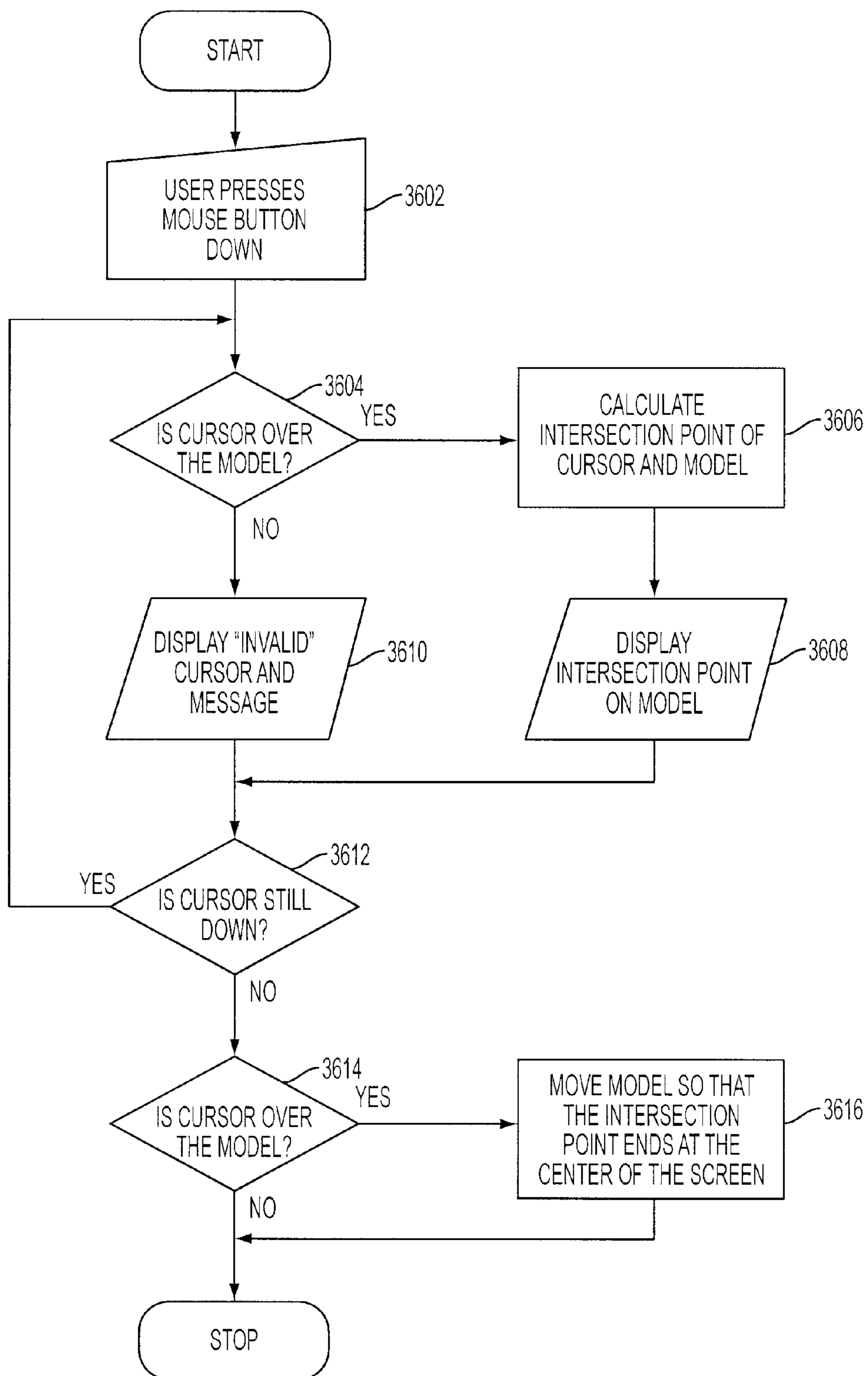
FLOWCHART OF CENTER TOOL
