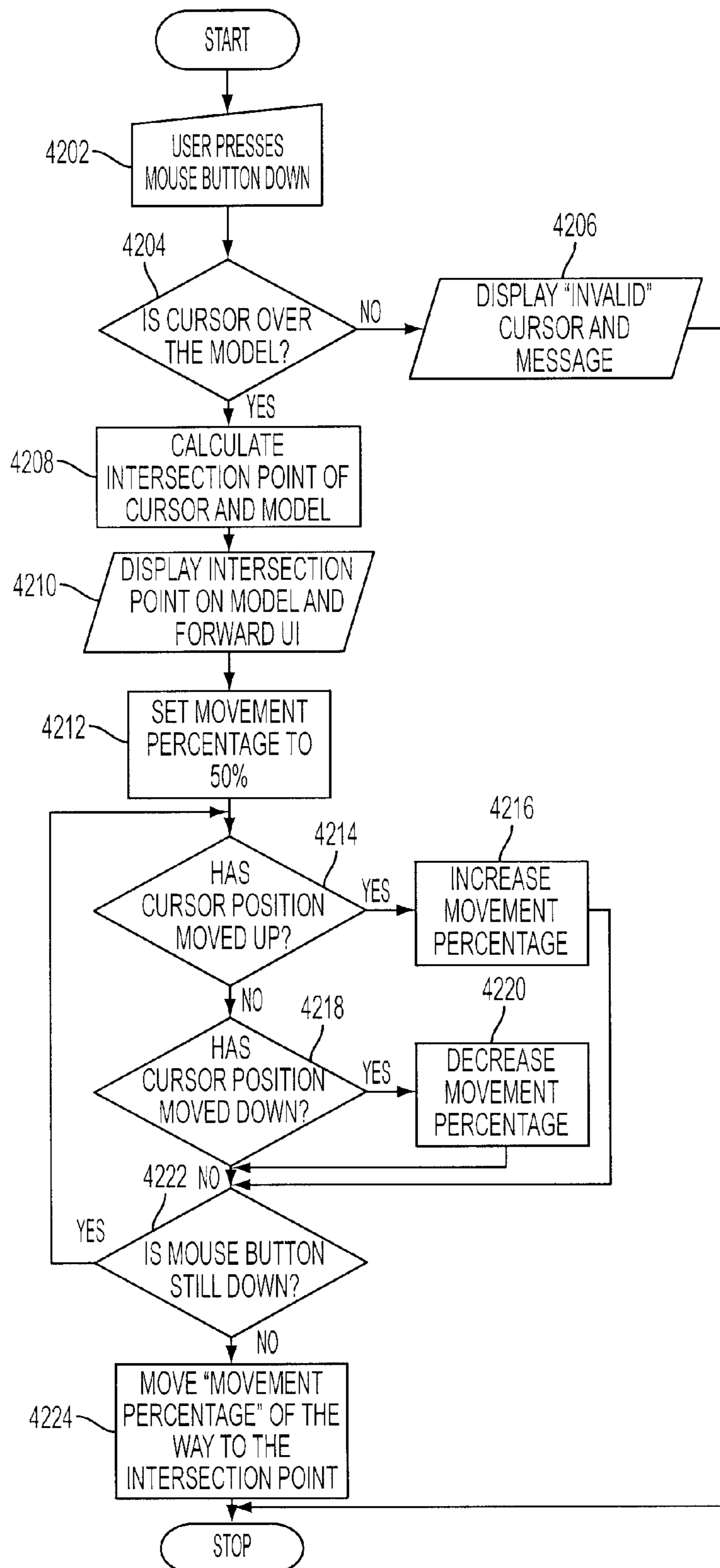
FLOWCHART OF FORWARD TOOL
