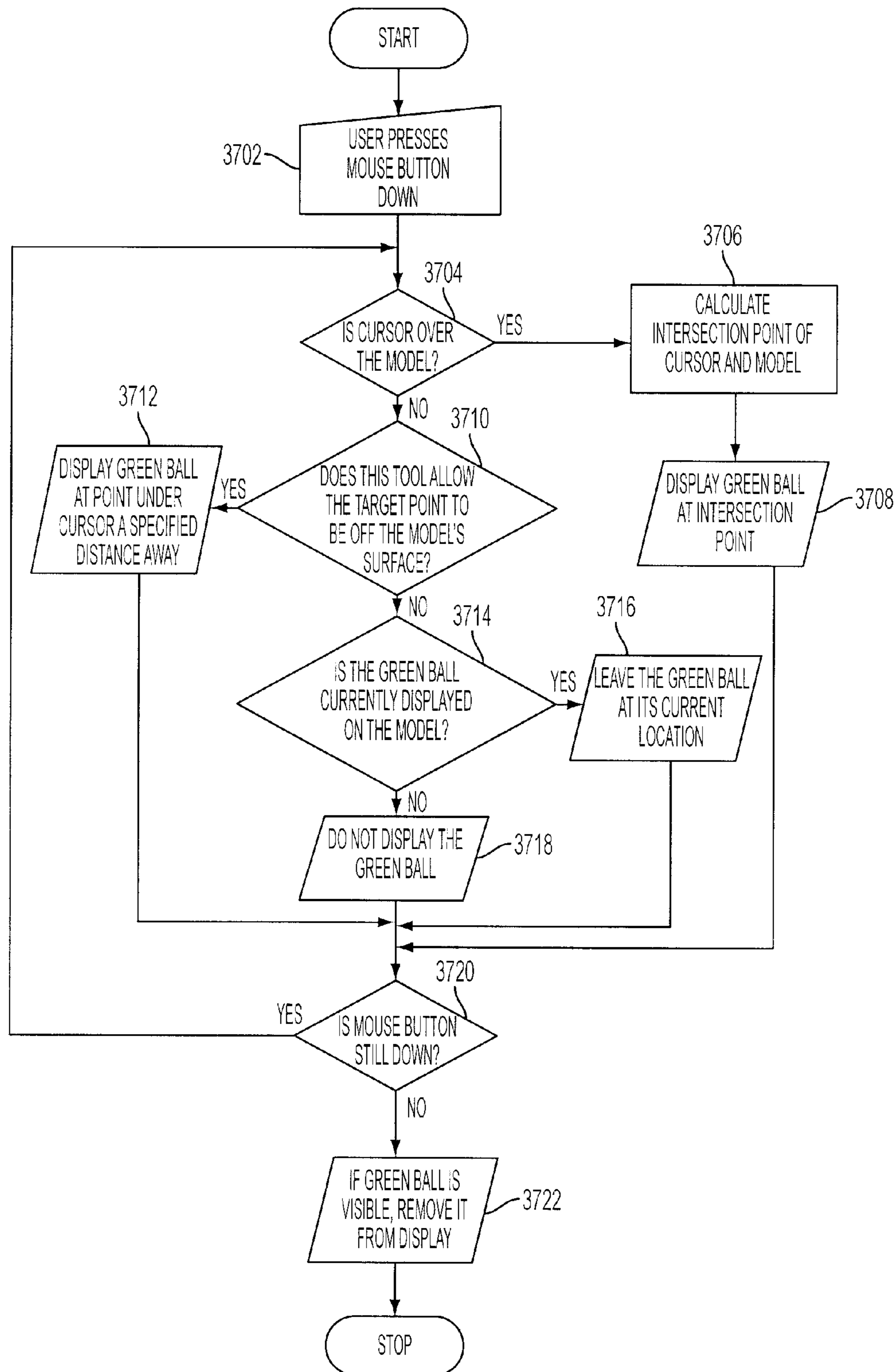
FLOWCHART OF GREEN BALL DISPLAYING
