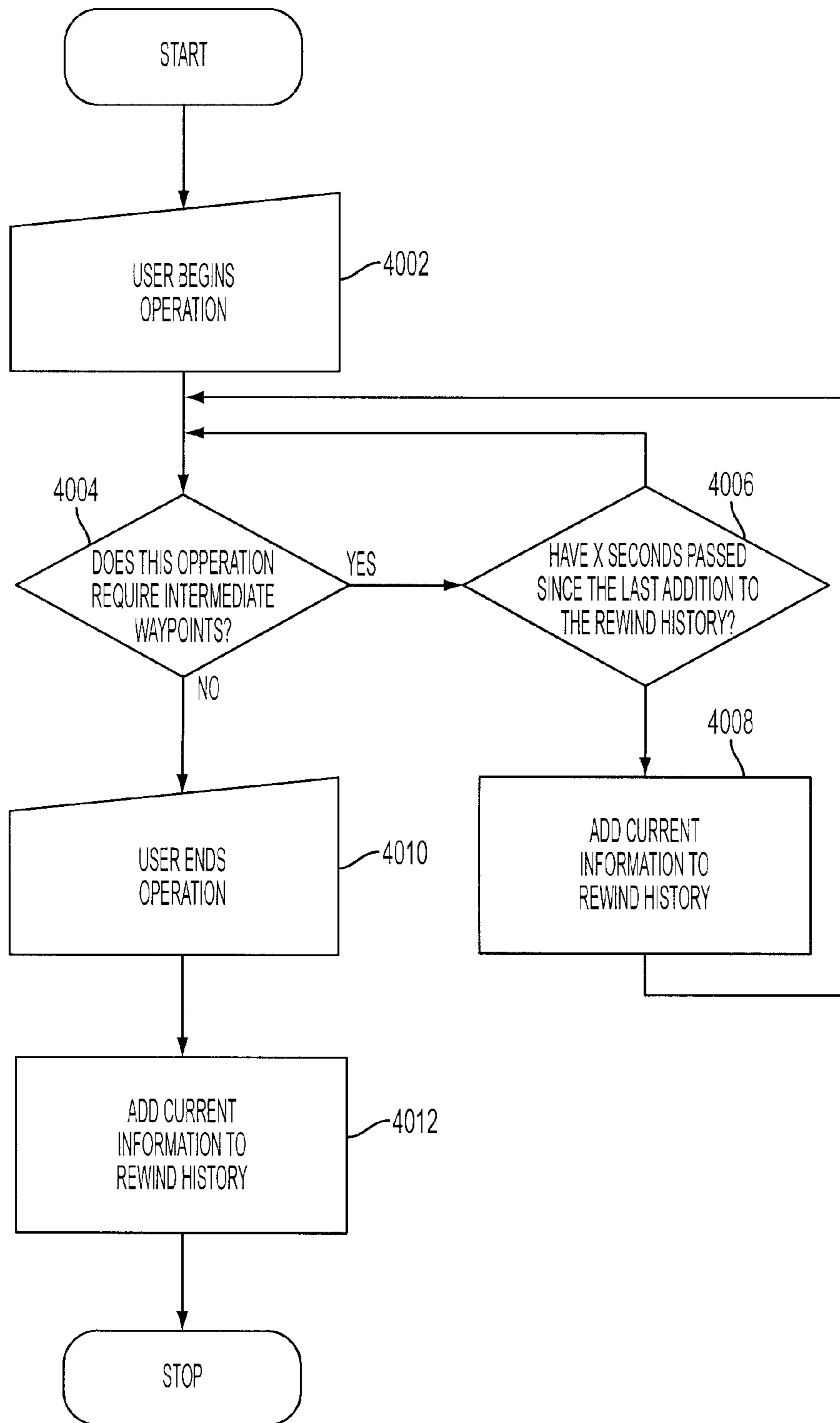
FLOWCHART OF REWIND HISTORY ADDITIONS
