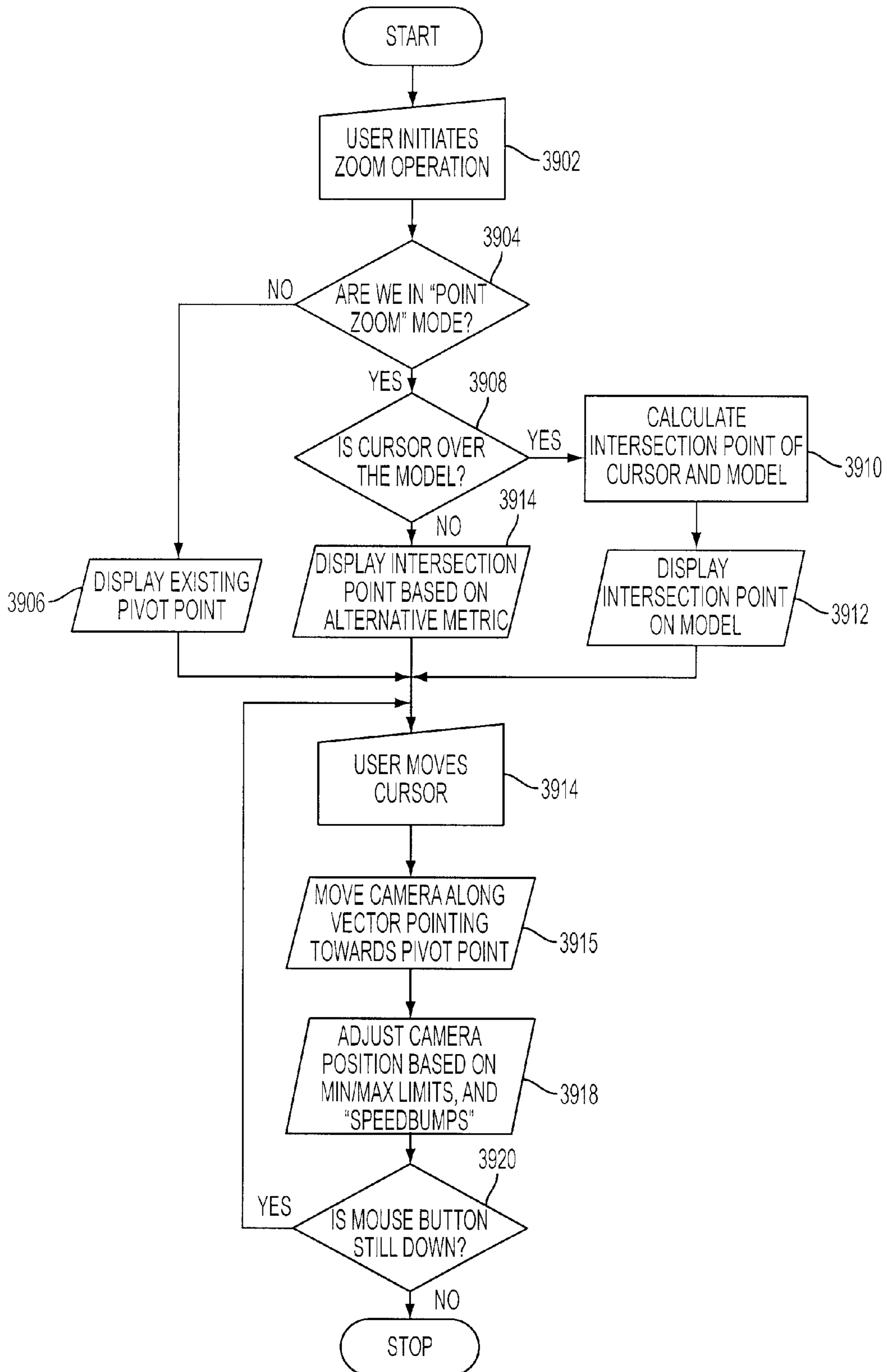
FLOWCHART OF ZOOM TOOL
