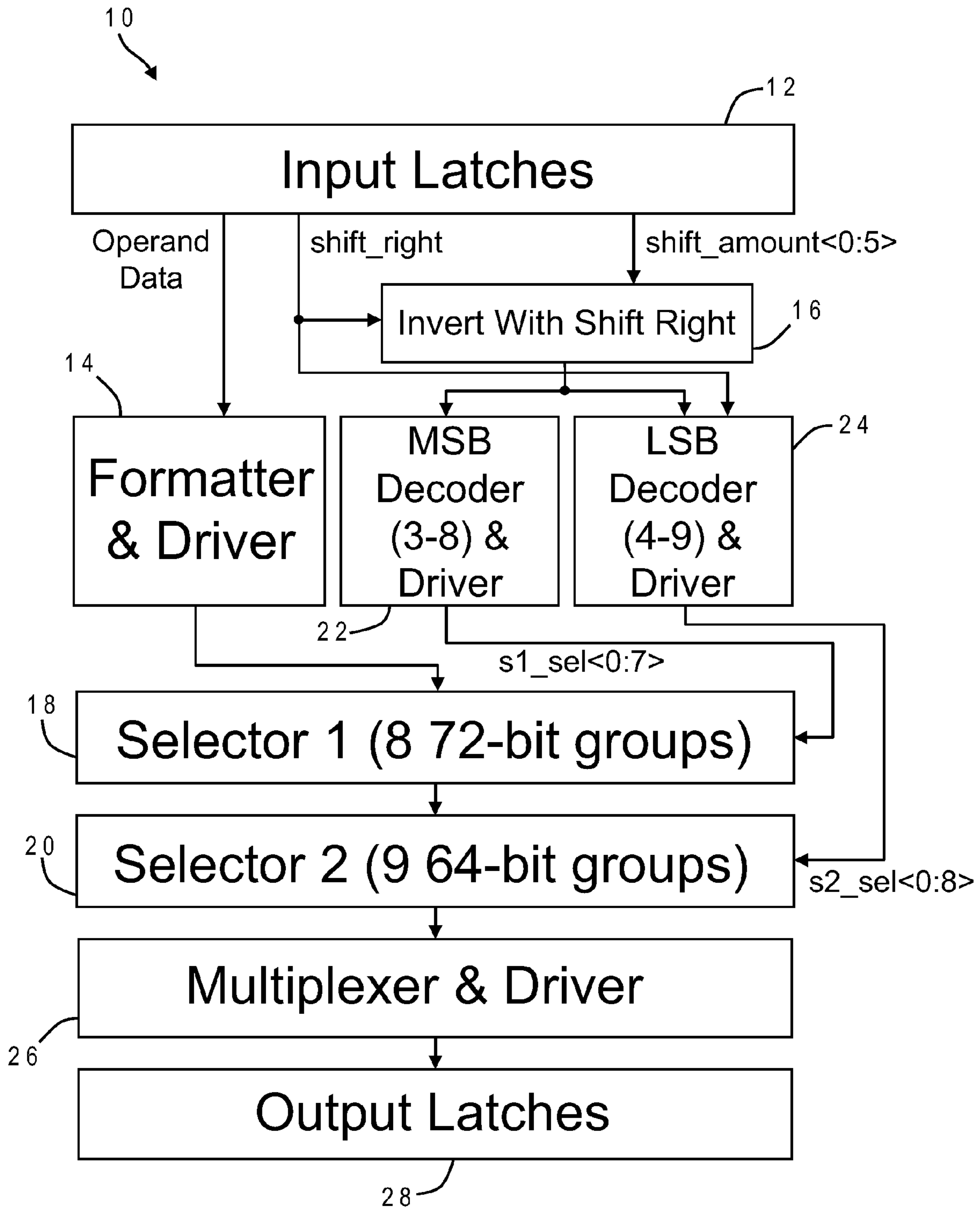
FIG. 1 Prior Art
