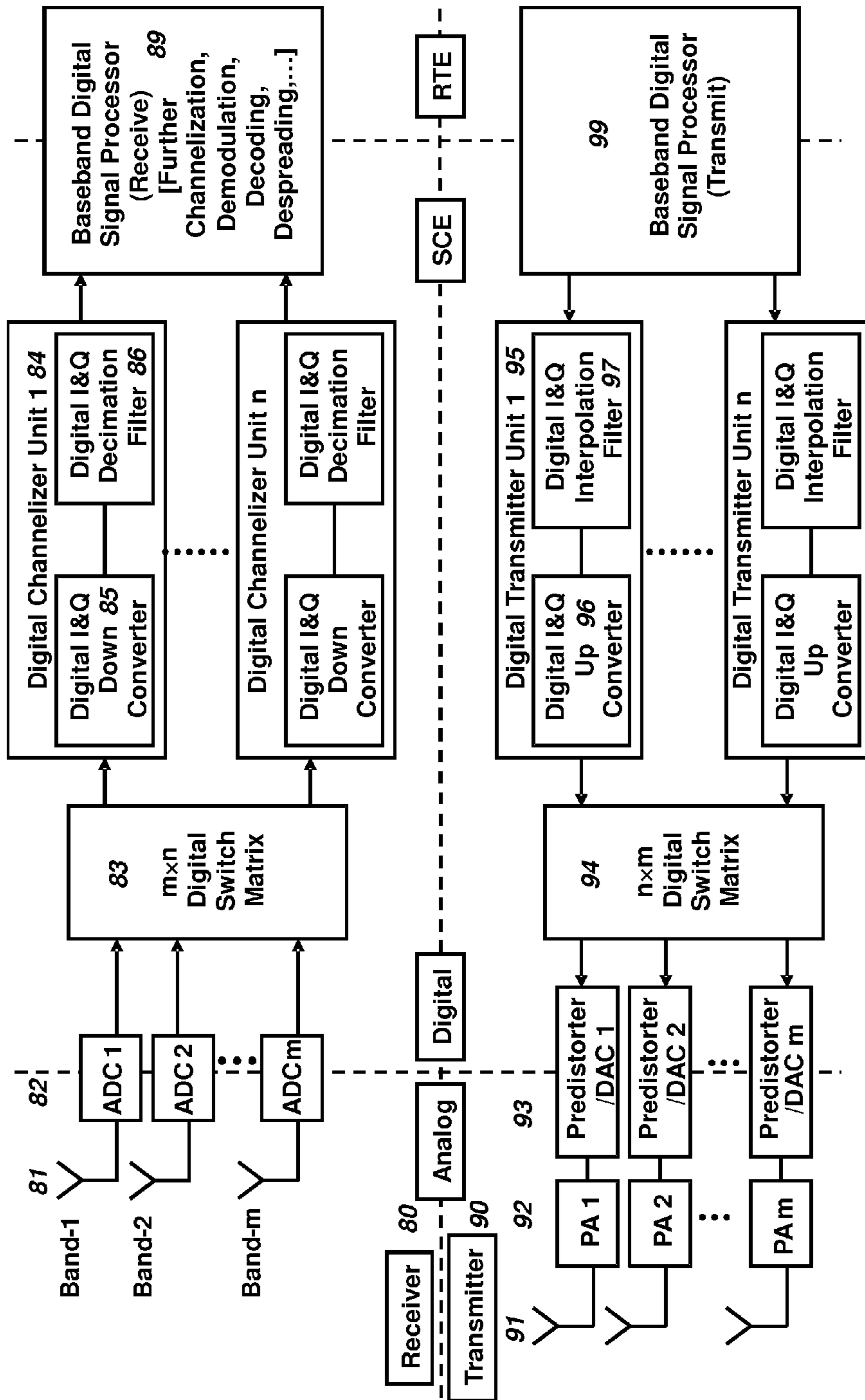
FIG. 4. Digital-RF™ Multichannel Transceiver
