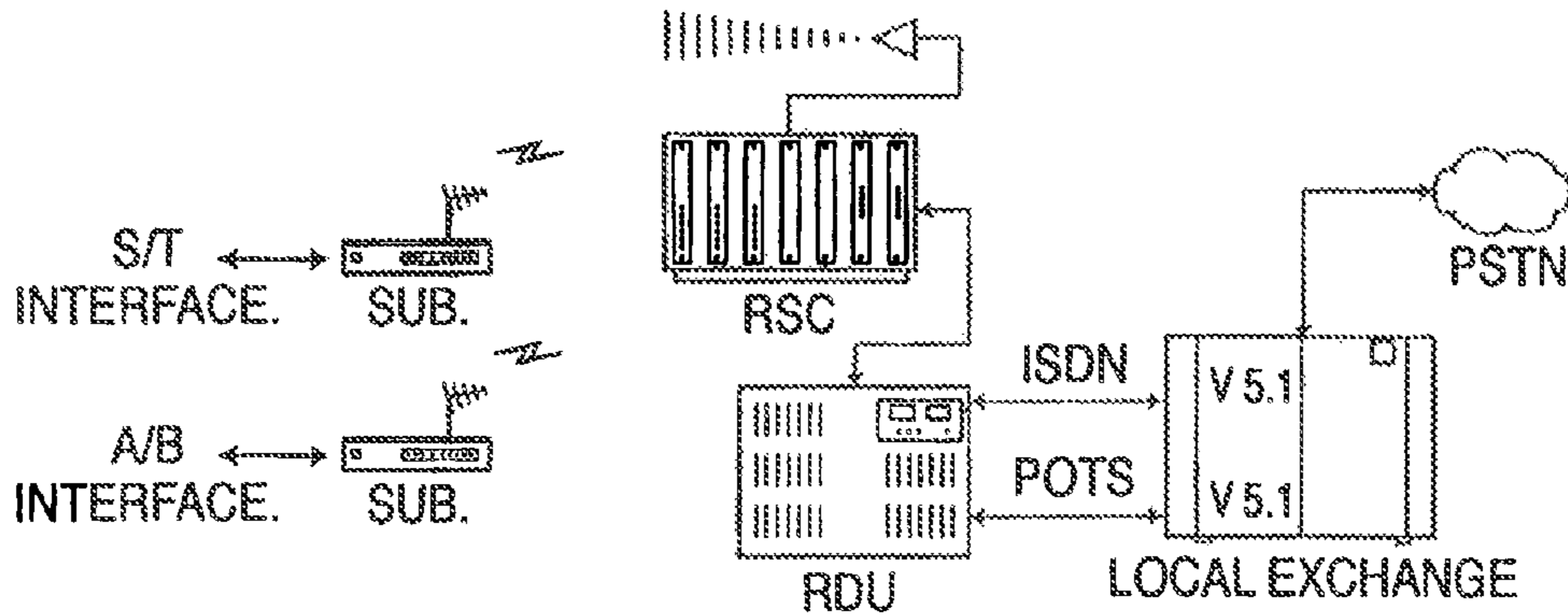
ISDN AND POTS NETWORK INTERFACE
