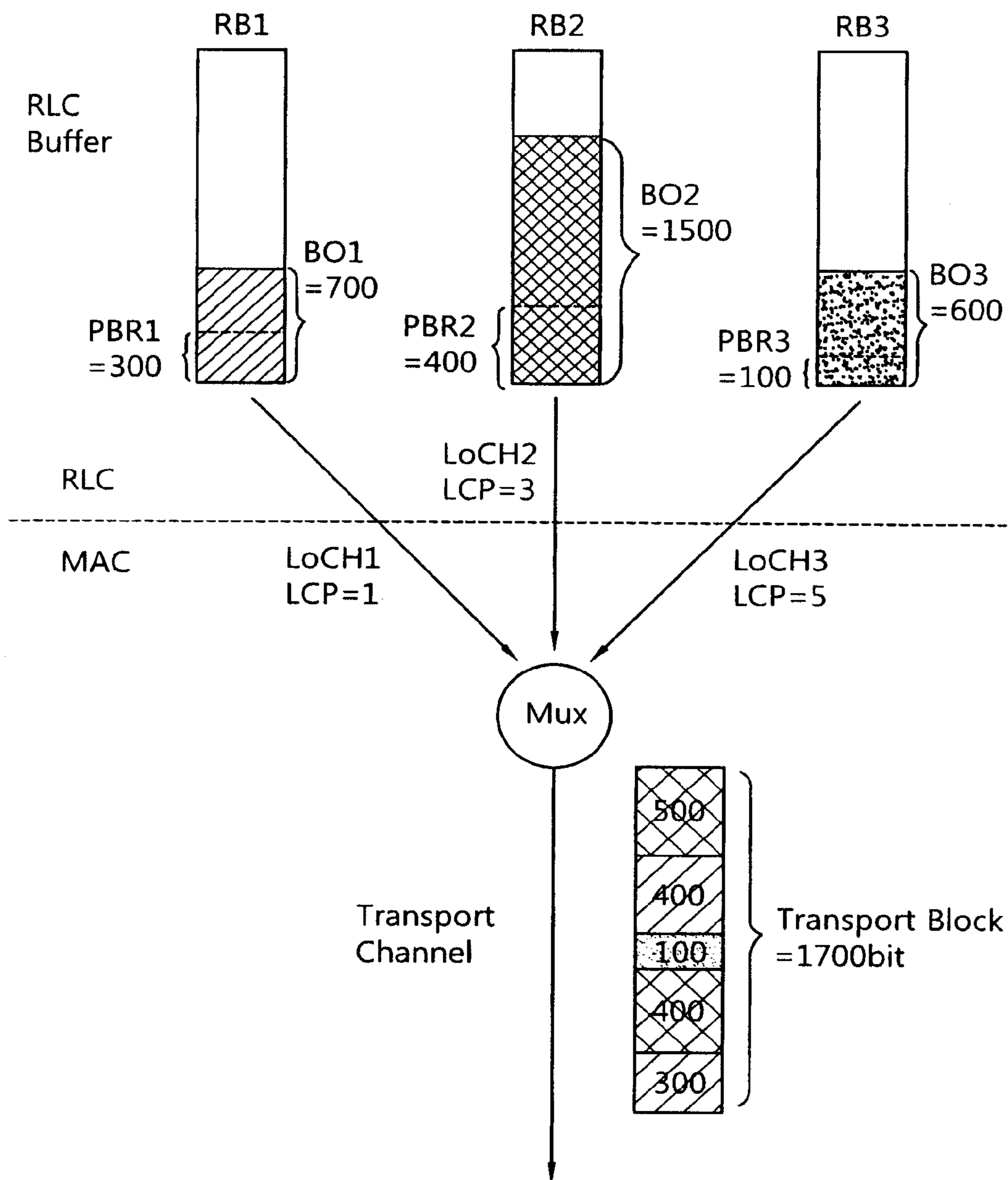
FIG. 7 (PRIOR ART)
