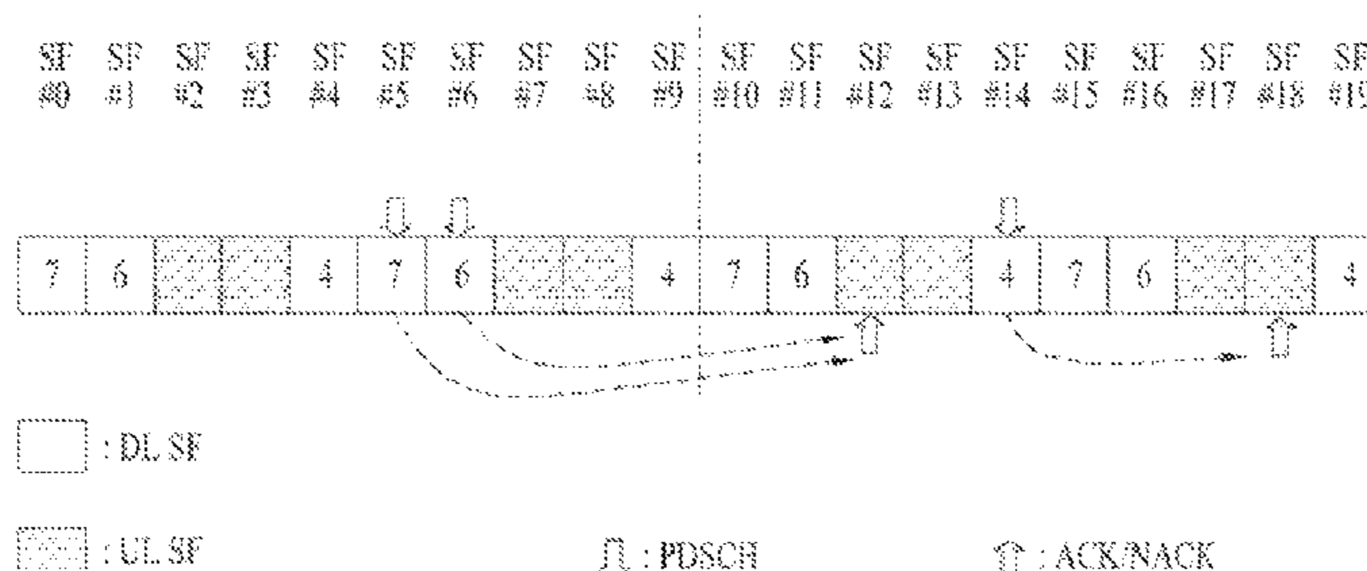
PDSCH-ACK/NACK timing (UL-DL configuration #1)
