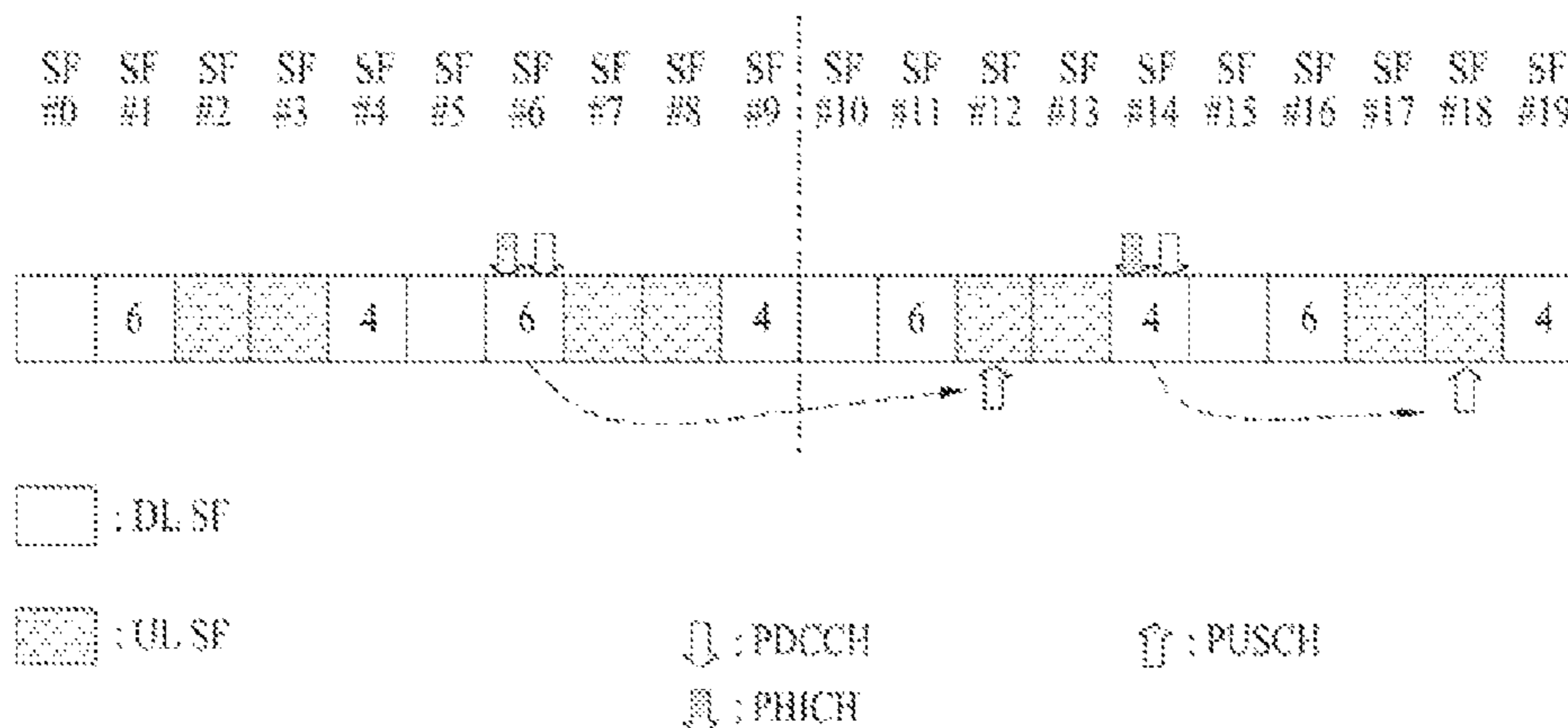
PHICH/UL grant-PUSCH timing (UL-DL configuration #1)
