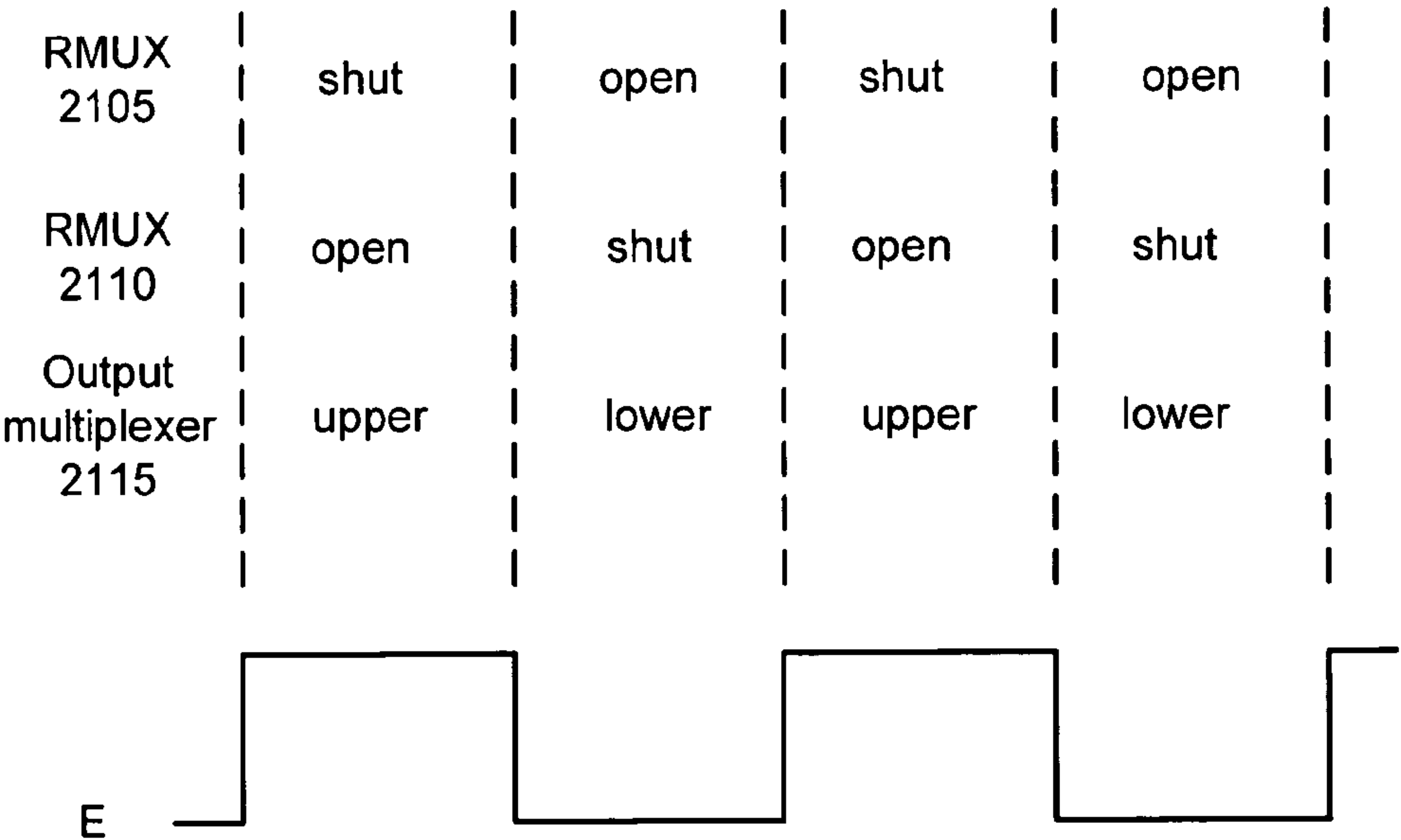
FIGURE 22 Timing diagram of the double-edge triggered register
