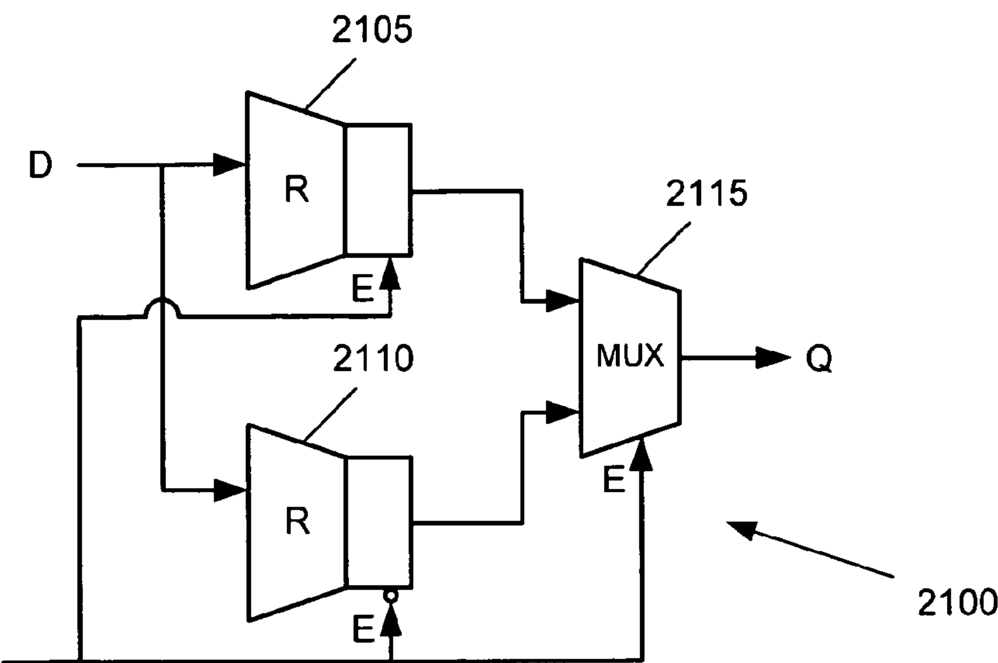
FIGURE 21 Double-edge triggered register
