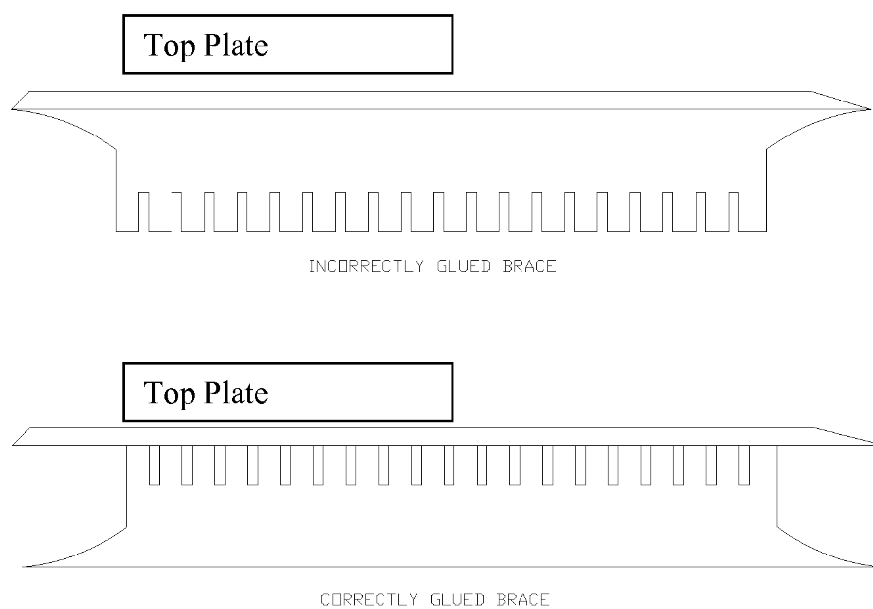
Figure 1. Incorrectly (top) and correctly (bottom) glued braces to the top plate
