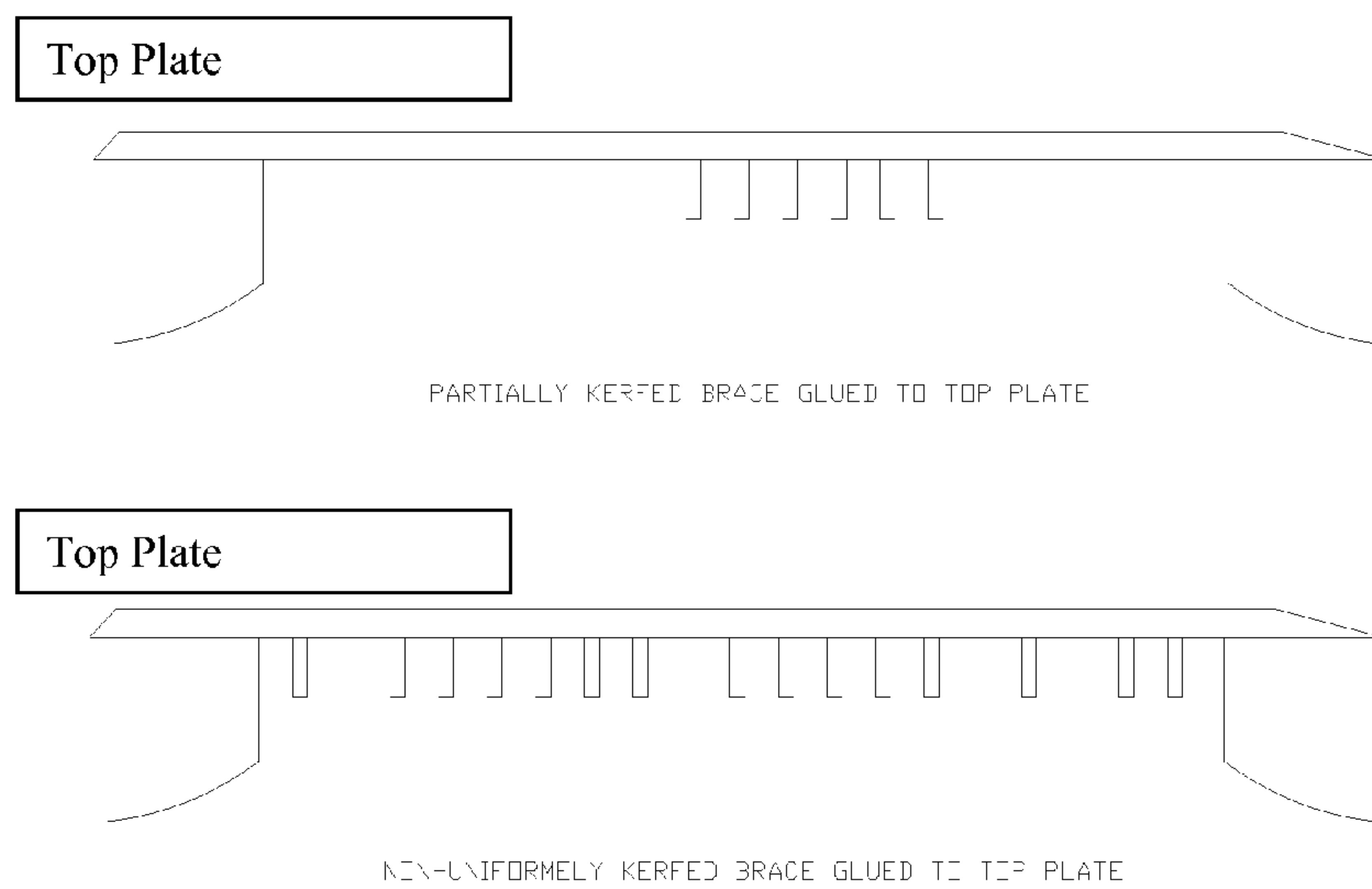
Figure 2. Partially kerfed (top) and non-uniformly kerfed braces glued to the top plate
