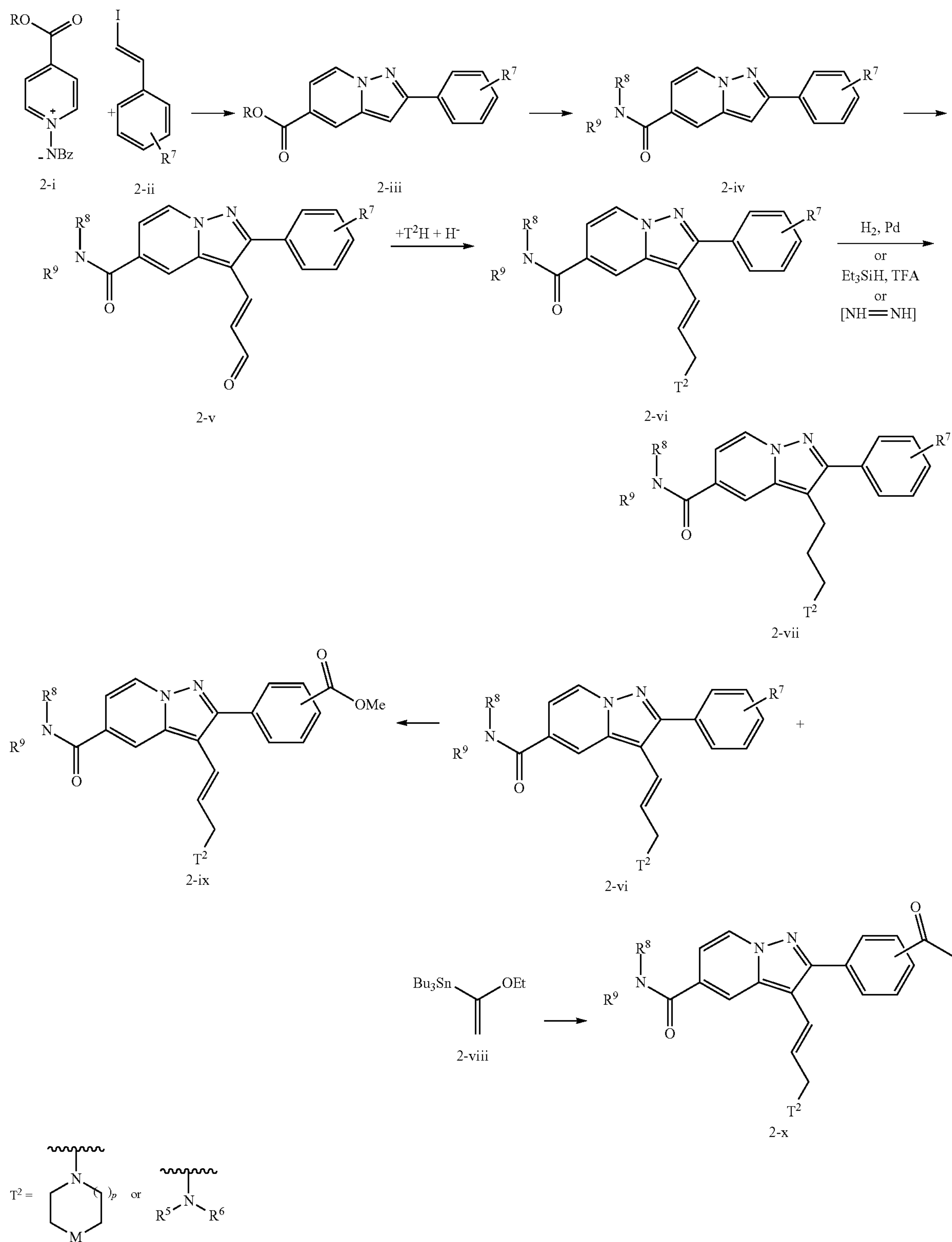
Scheme 2
