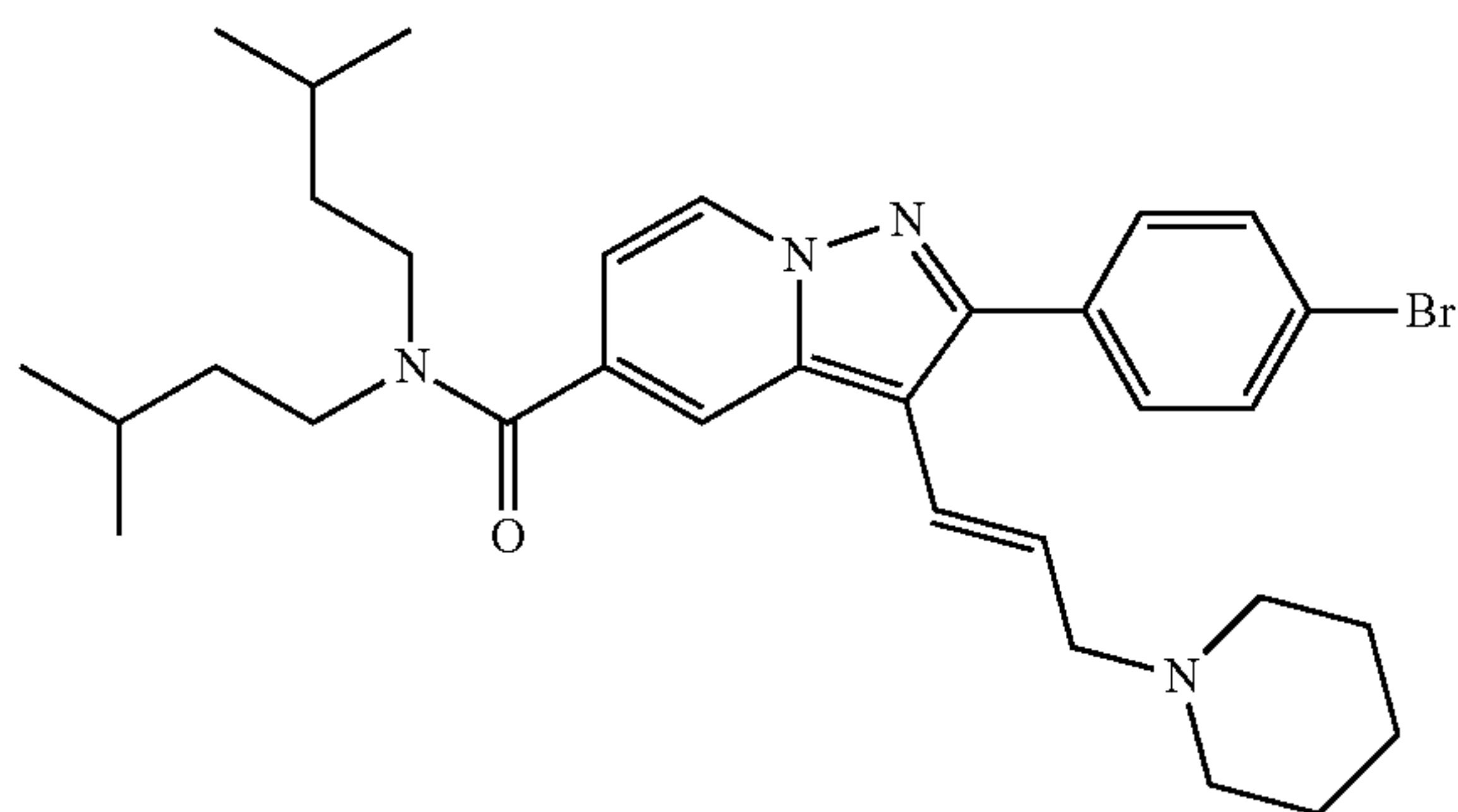
(E)-2-(4-Bromophenyl)-N,N-diisopentyl-3-(3-(piperidin-1-yl)prop-1-en-1-yl)pyrazolo[1,5-a]pyridine-5-carboxamide
