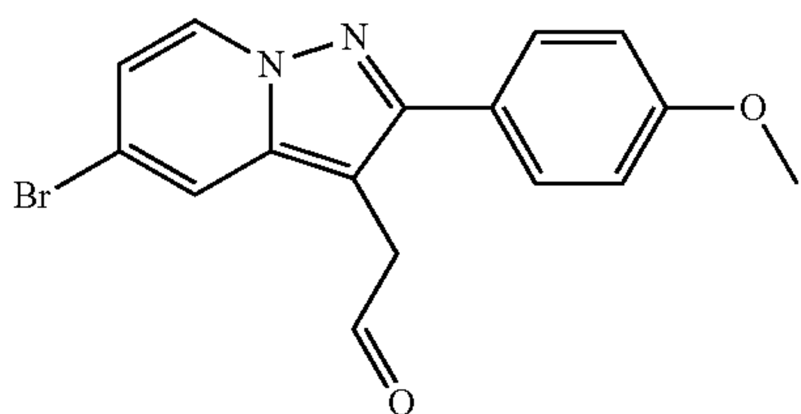
2-(5-bromo-2-(4-methoxyphenyl)pyrazolo[1,5-a]pyridin-3-yl)acetaldehyde
