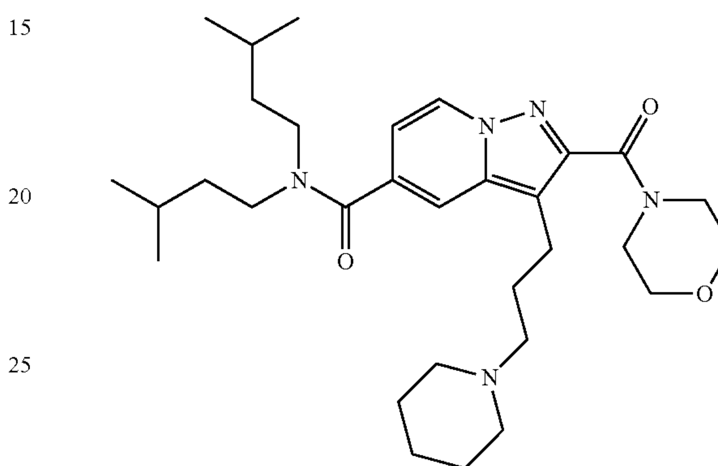
N,N-diisopentyl-2-(morpholine-4-carbonyl)-3-(3-(piperidin-1-yl)propyl)pyrazolo[1,5-a]pyridine-5-carboxamide
