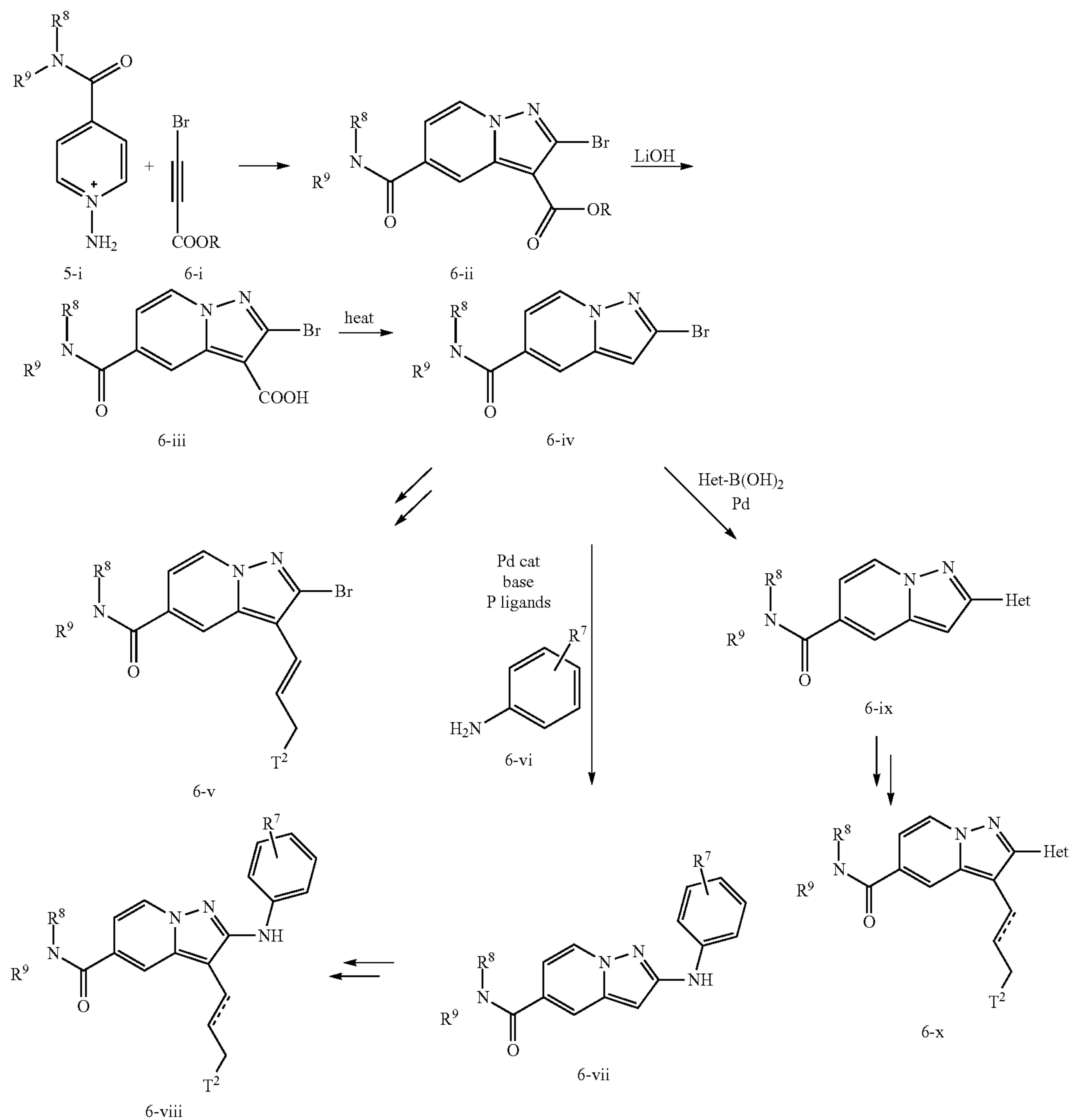
Scheme 6
