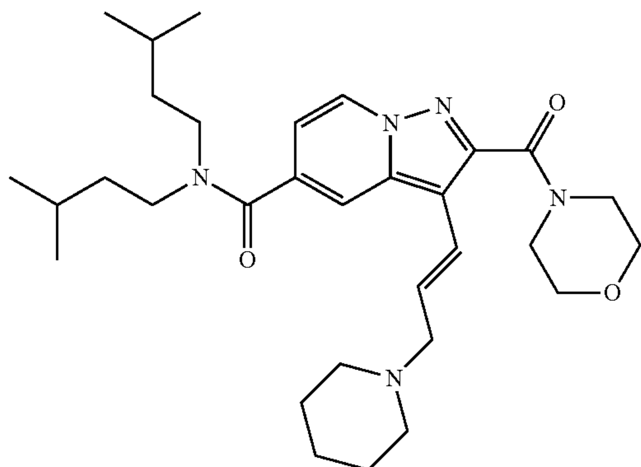
(E)-N,N-diisopentyl-2-(morpholine-4-carbonyl)-3-(3-(piperidin-1-yl)prop-1-en-1-yl)pyrazolo[1,5-a]pyridine-5-carboxamide
