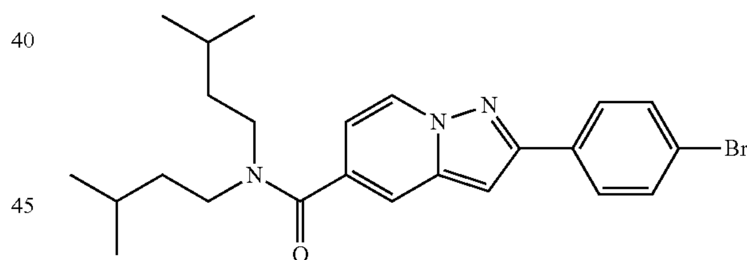
2-(p-Bromophenyl)pyrazolo[1,5-a]pyridine-5-carboxylic diisopentylamide
