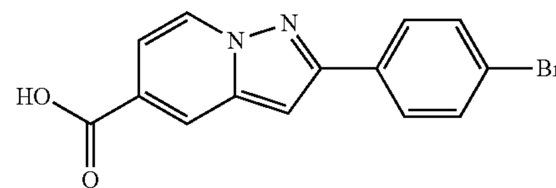
2-(4-Bromophenyl)pyrazolo[1,5-a]pyridine-5-carboxylic acid
