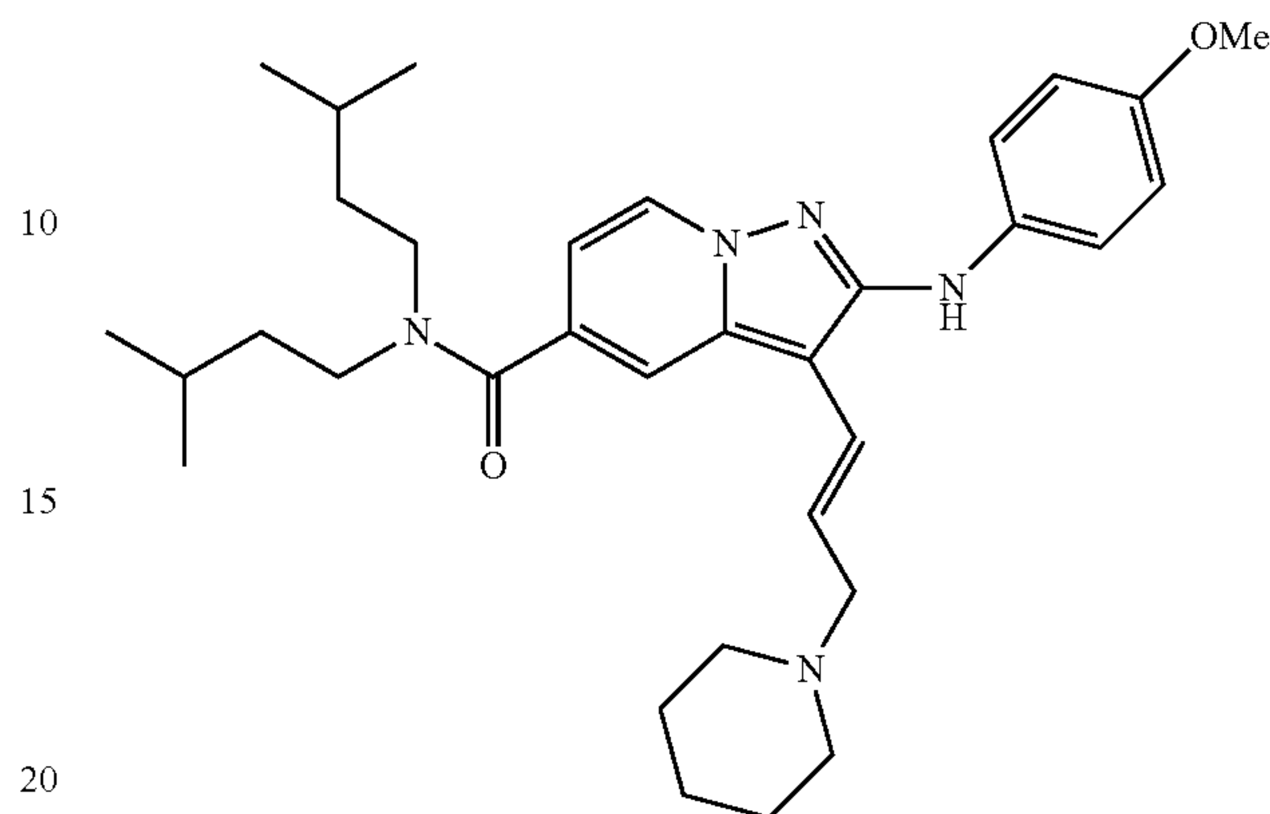
(E)-N,N-diisopentyl-2-((4-methoxyphenyl)amino)-3- (3-(piperidin-1-yl)prop-1-en-1-yl)pyrazolo[1,5-a] pyridine-5-carboxamide
