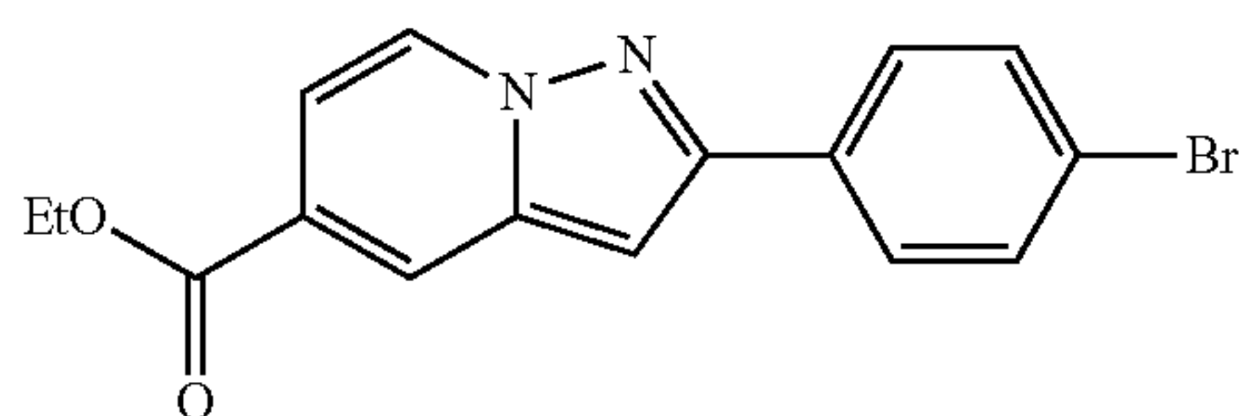
Ethyl 2-(4-bromophenyl)pyrazolo[1,5-a]pyridine-5-carboxylate
