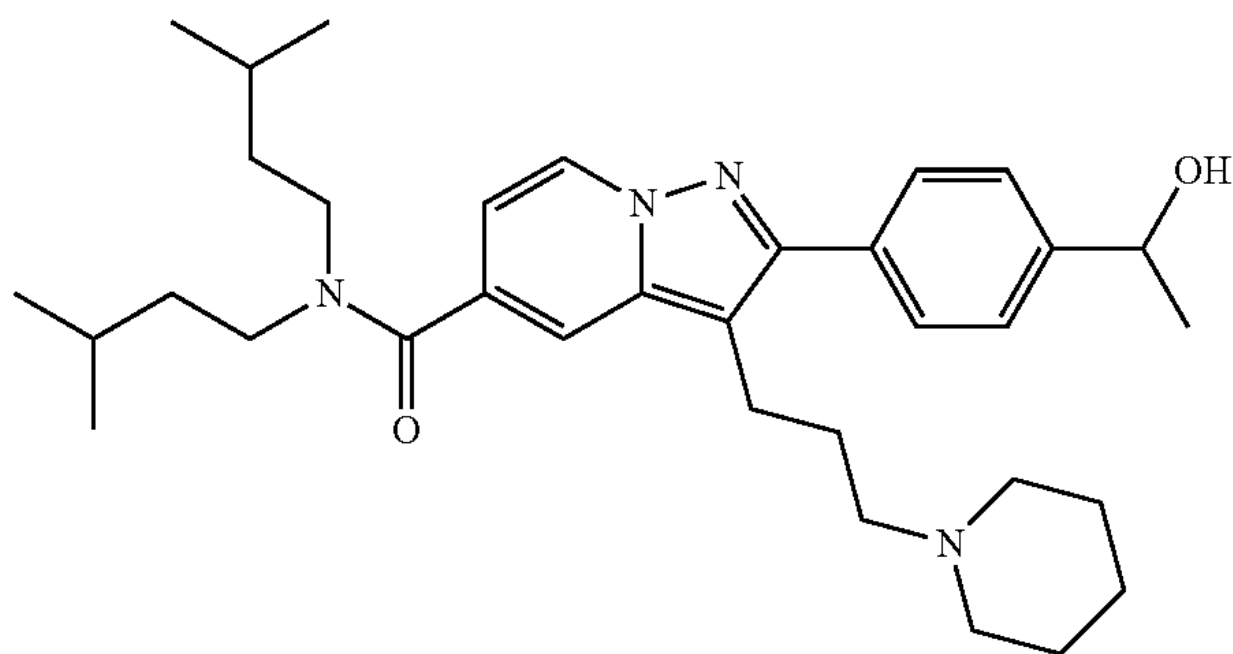
2-(4-(1-Hydroxyethyl)phenyl)-N,N-diisopentyl-3-(3-(piperidin-1-yl)propyl)pyrazolo[1,5-a]pyridine-5-carboxamide
