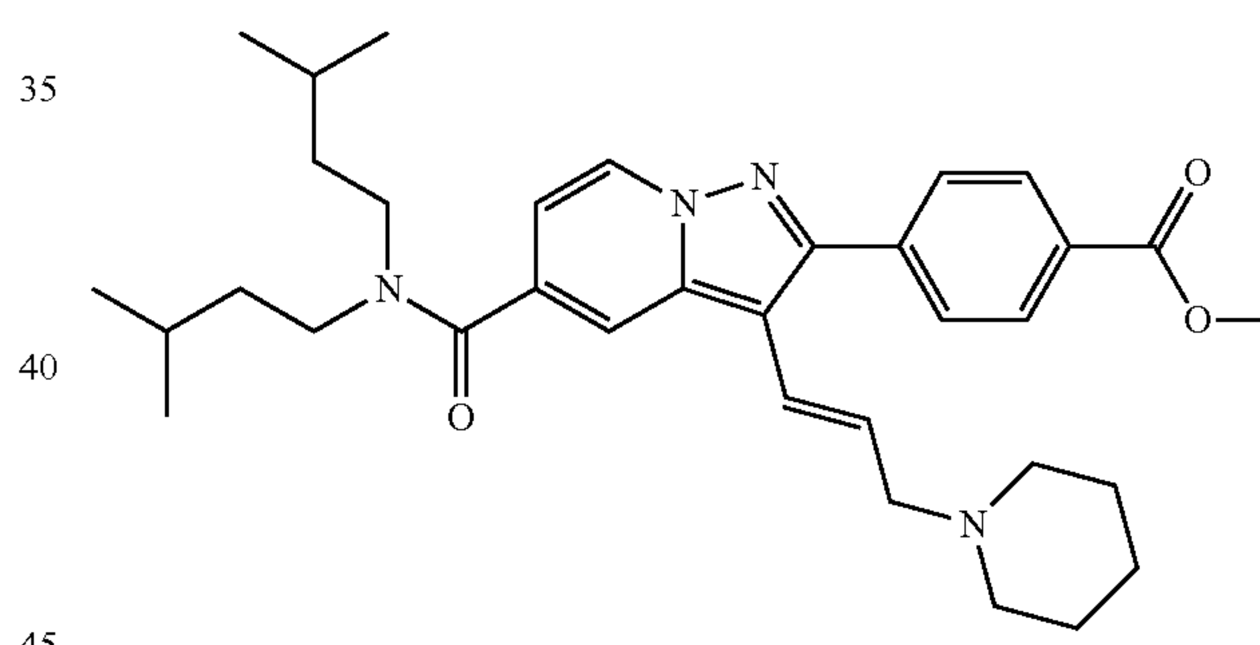
(E)-Methyl 4-(5-(diisopentylcarbamoyl)-3-(3-(piperidin-1-yl)prop-1-en-1-yl)pyrazolo[1,5-a]pyridin-2-yl)benzoate
