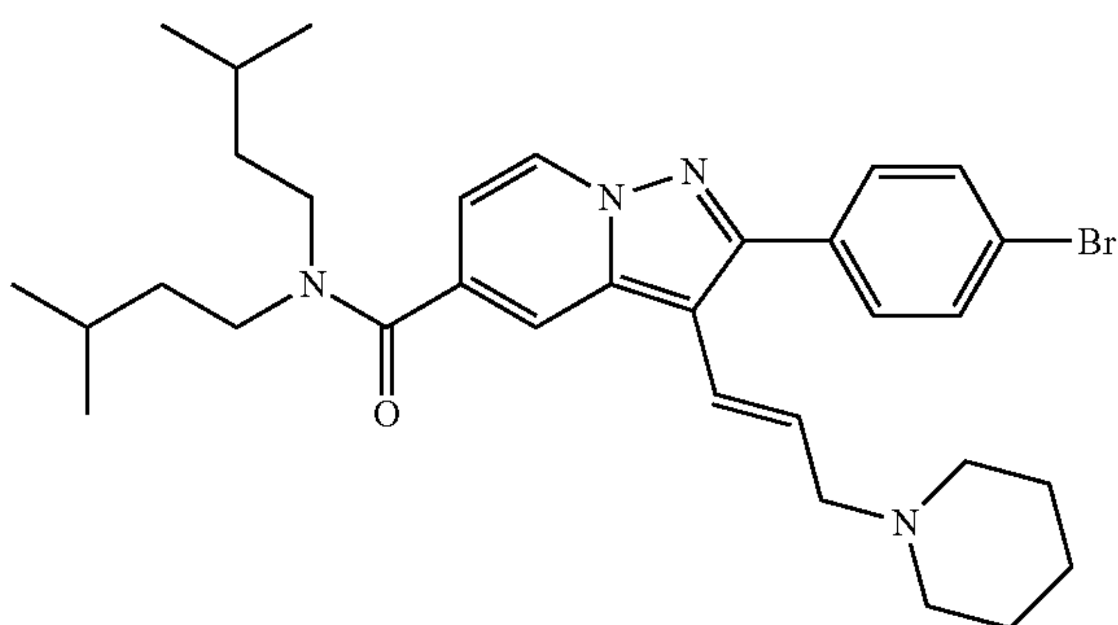
(E)-2-(4-Bromophenyl)-N,N-diisopentyl-3-(3-(piperidin-1-yl)prop-1-en-1-yl)pyrazolo[1,5-a]pyridine-5-carboxamide
