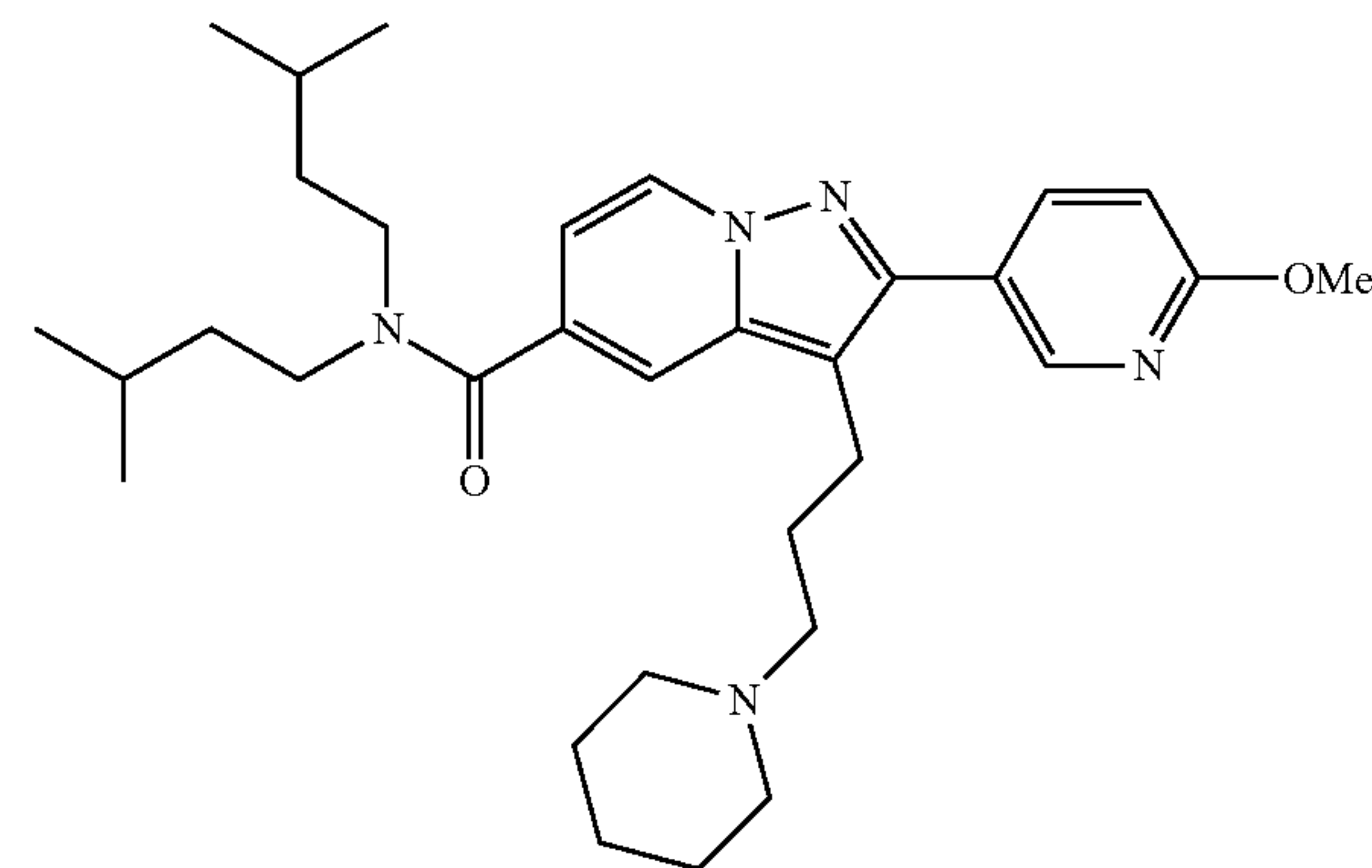
Example 164
