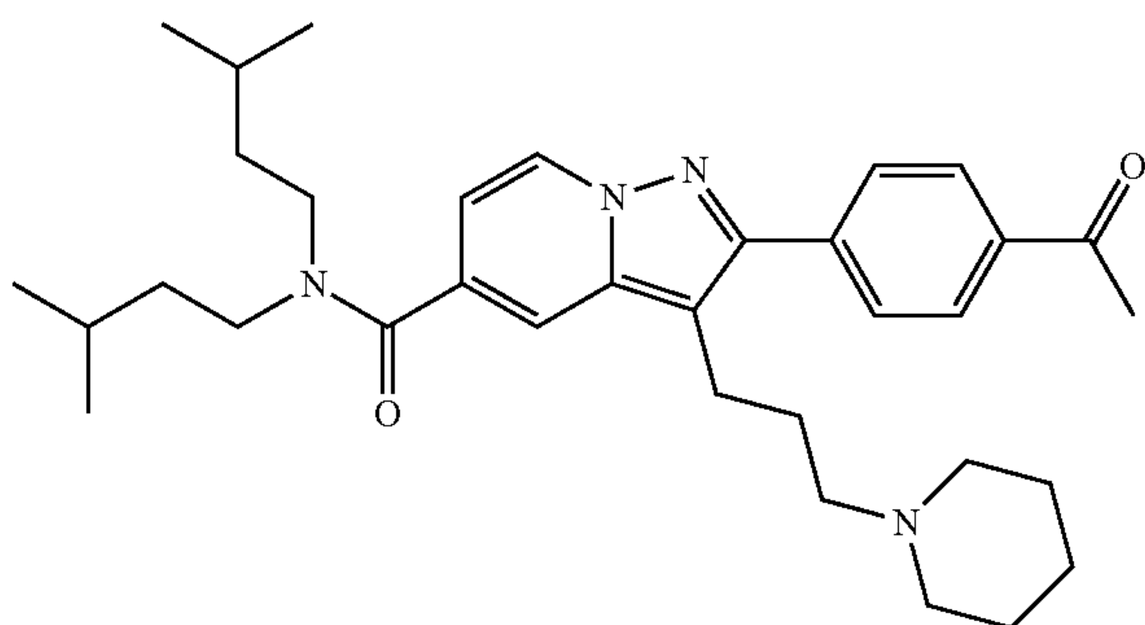
2-(4-Acetylphenyl)-N,N-diisopentyl-3-(3-(piperidin-1-yl)propyl)pyrazolo[1,5-a]pyridine-5-carboxamide
