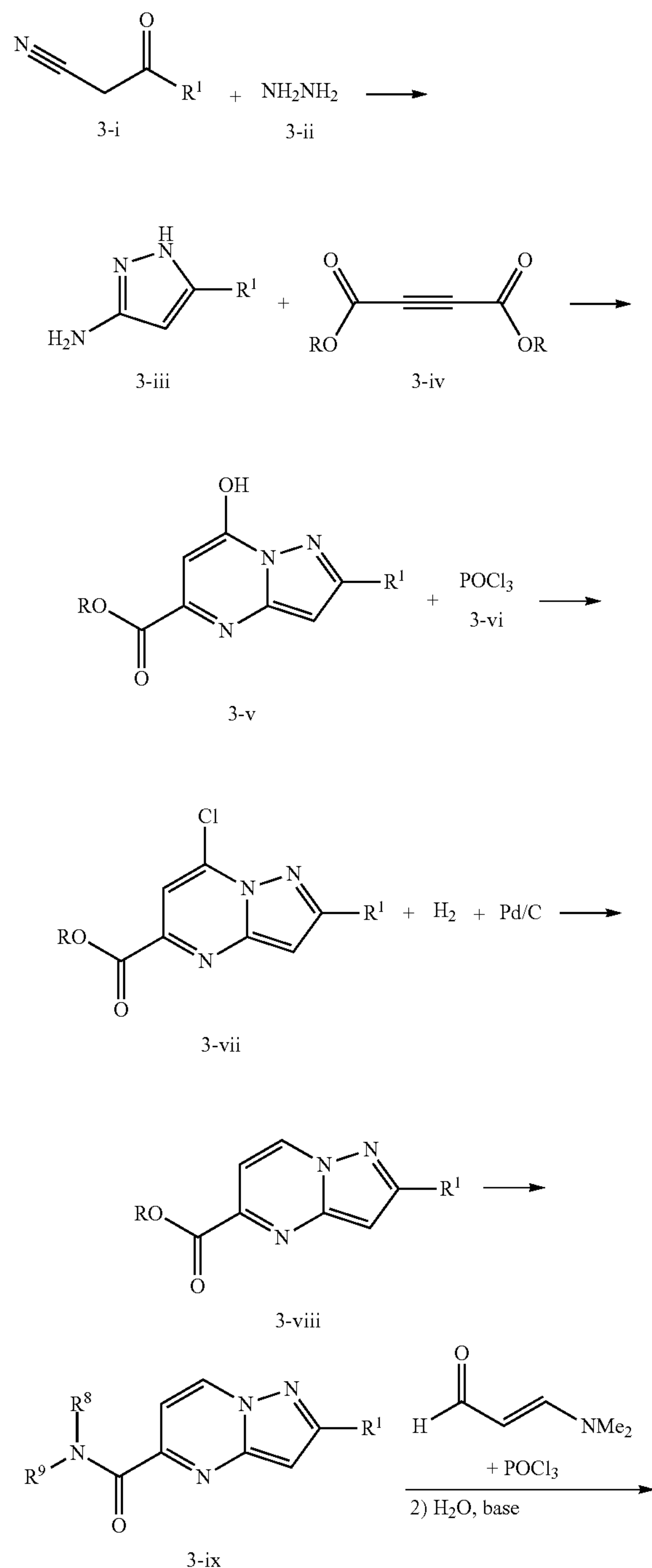
Scheme 3
