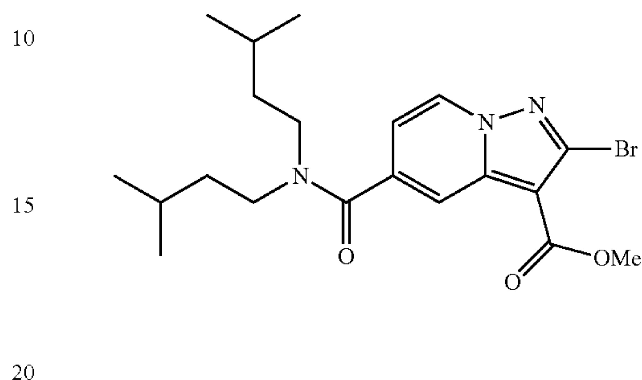
methyl 2-bromo-5-(diisopentylcarbamoyl)pyrazolo[1,5-a]pyridine-3-carboxylate
