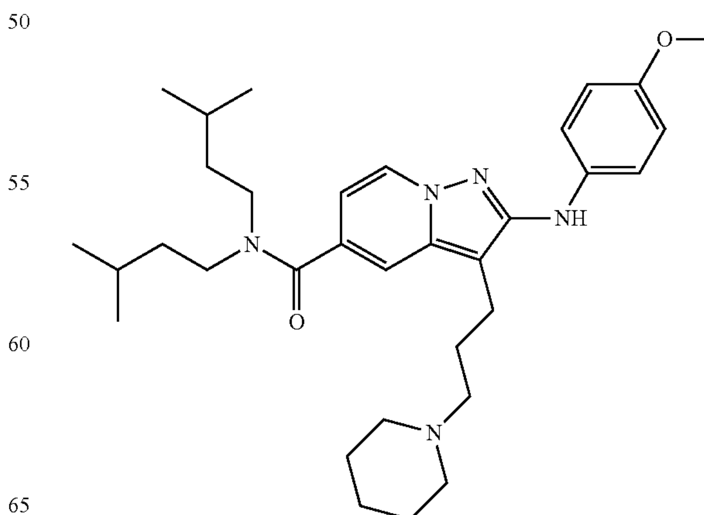
(E)-N,N-diisopentyl-2-(morpholine-4-carbonyl)-3-(3-(piperidin-1-yl)prop-1-en-1-yl)pyrazolo[1,5-a]pyridine-5-carboxamide
