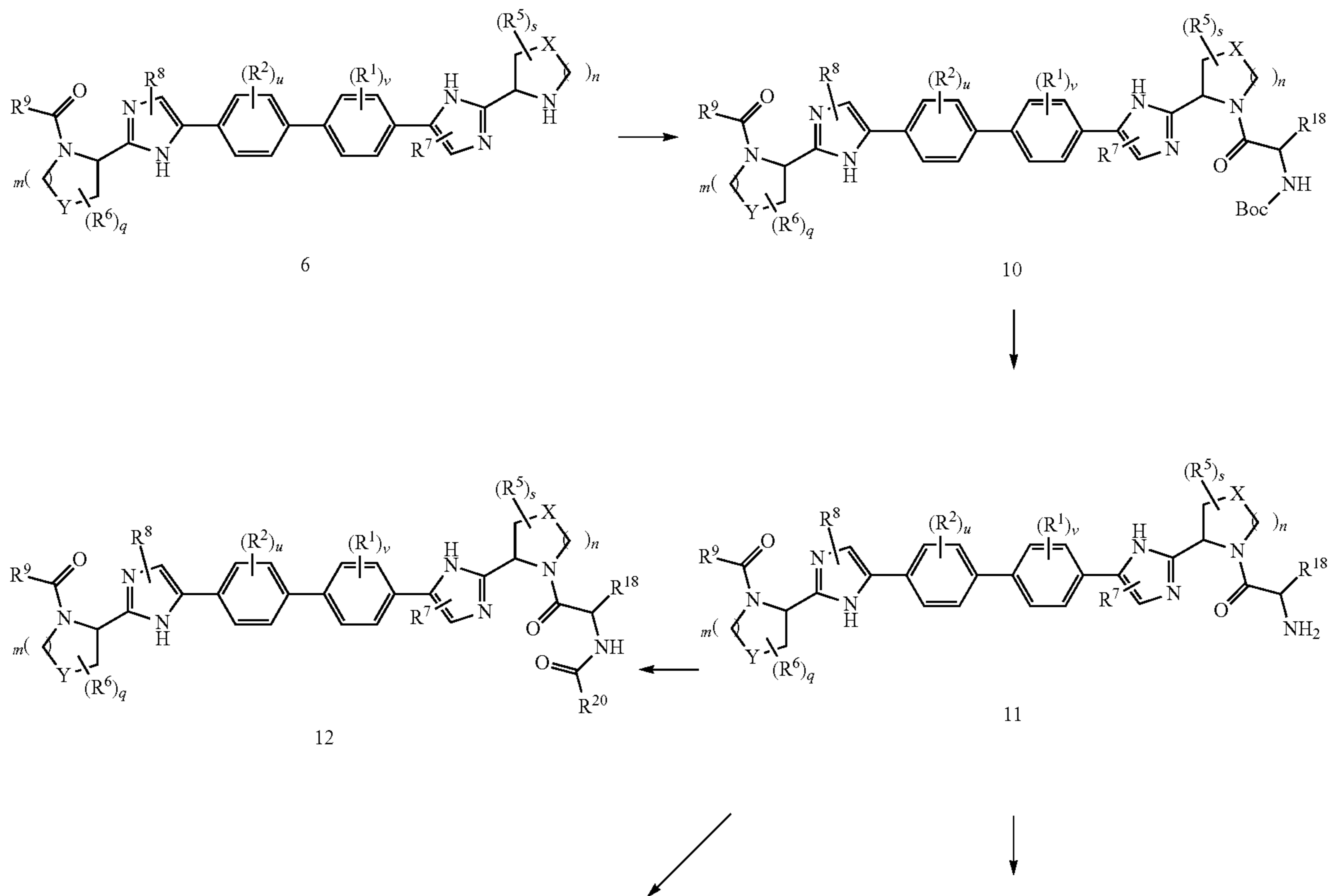
Scheme 3: Symmetric Cap Elaborated Biphenyls
