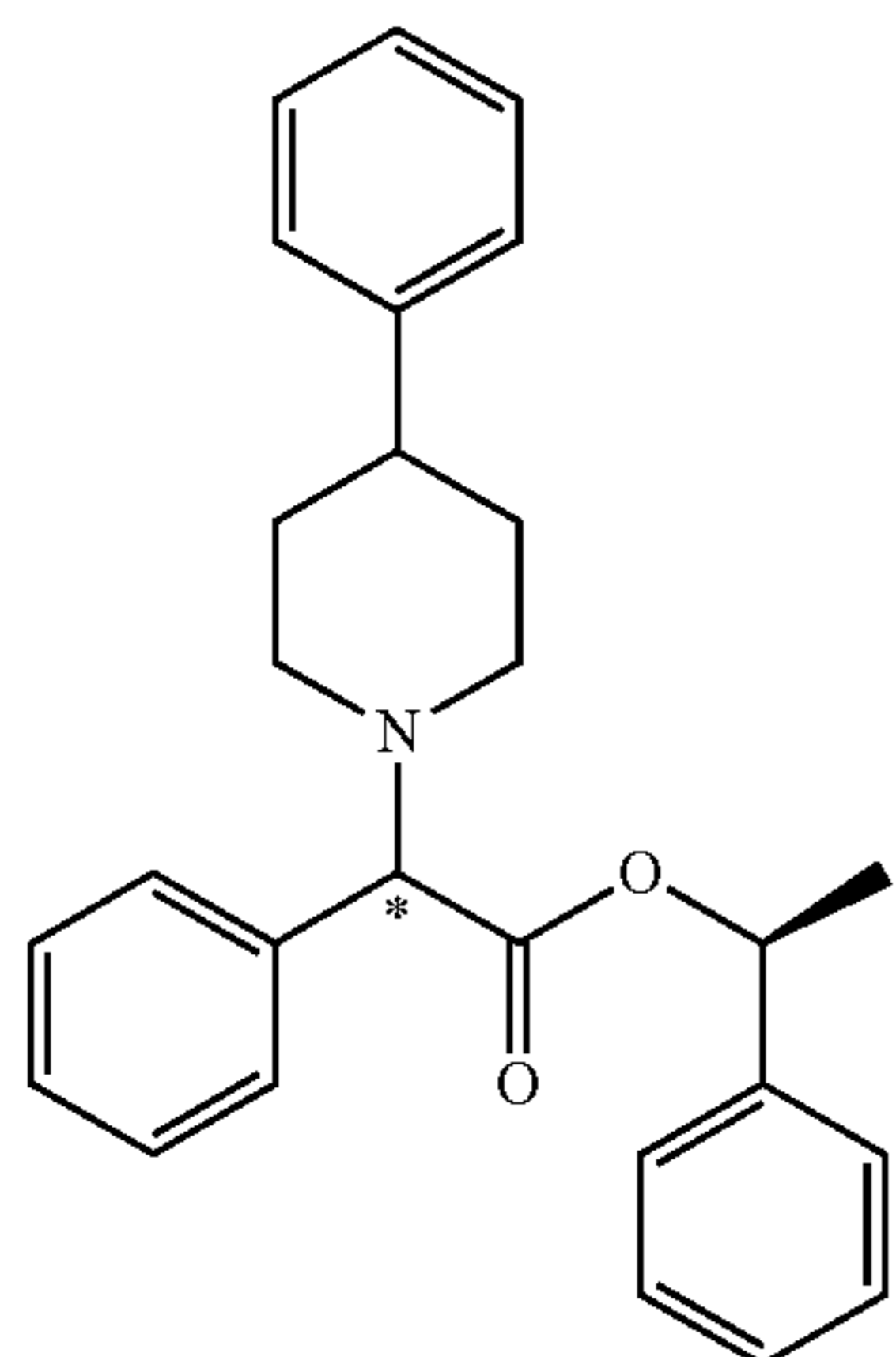
Intermediate-17d
