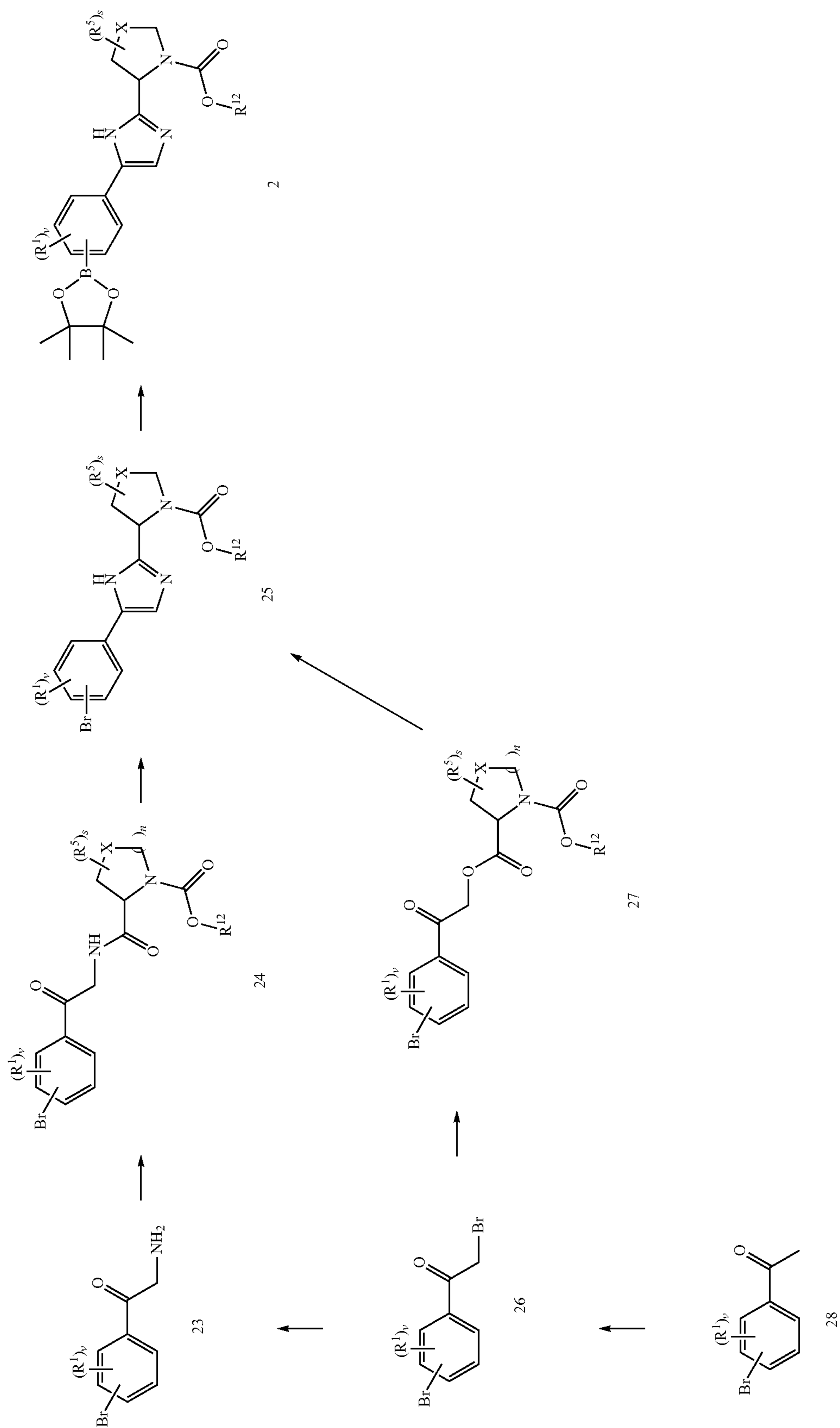
Scheme 6: Starting Material 31a
