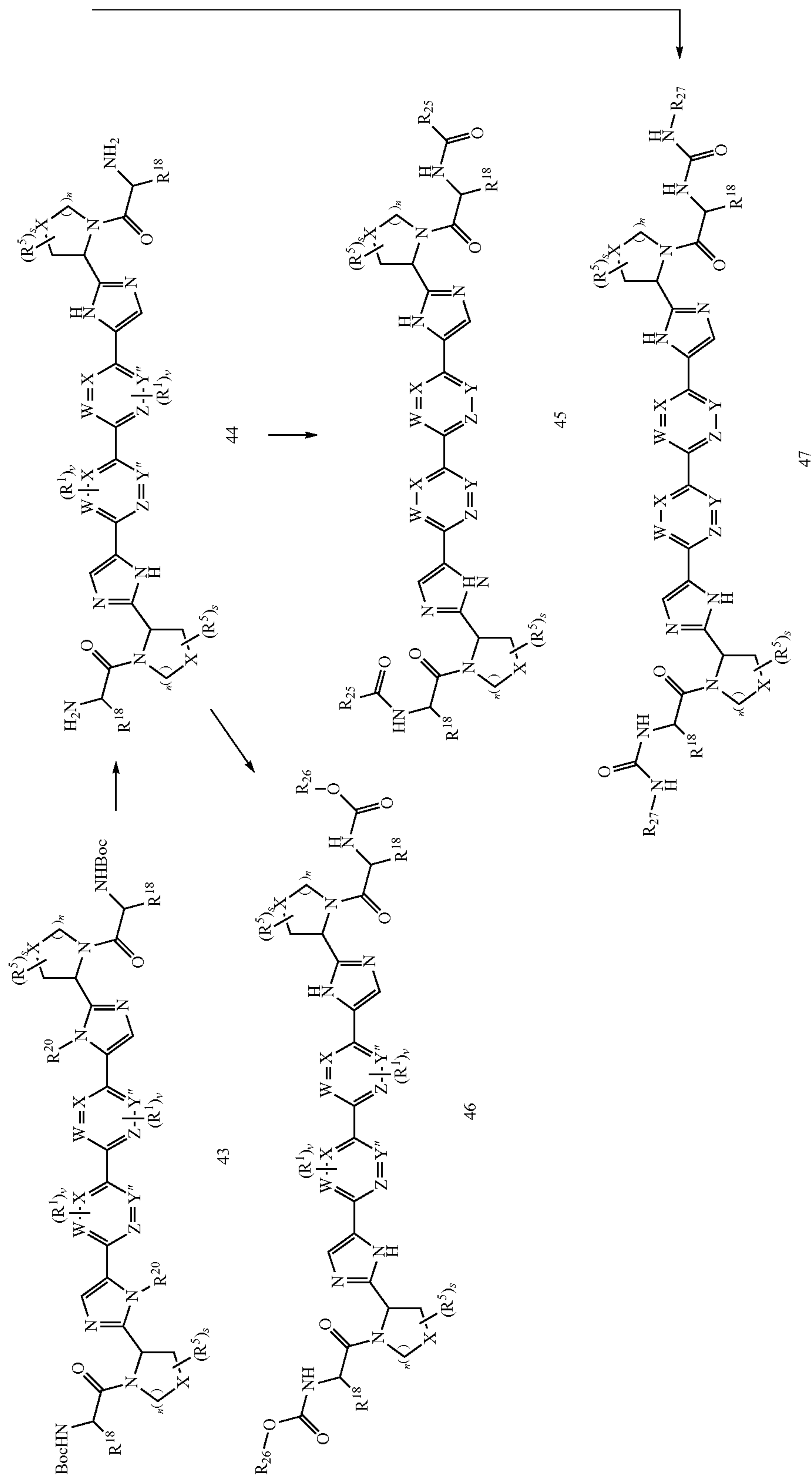
Scheme 10: Starting Material 29
