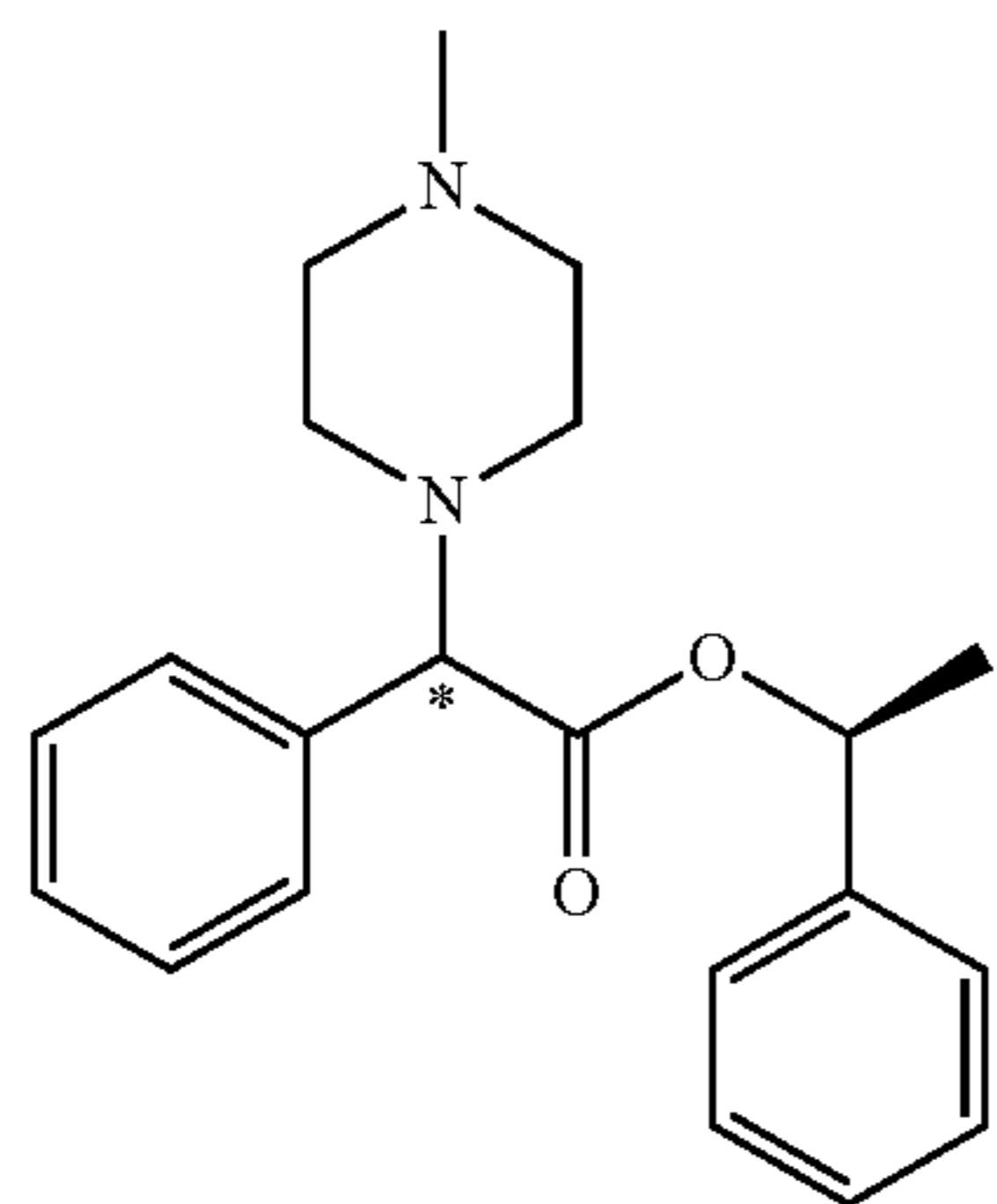
Intermediate-17c
