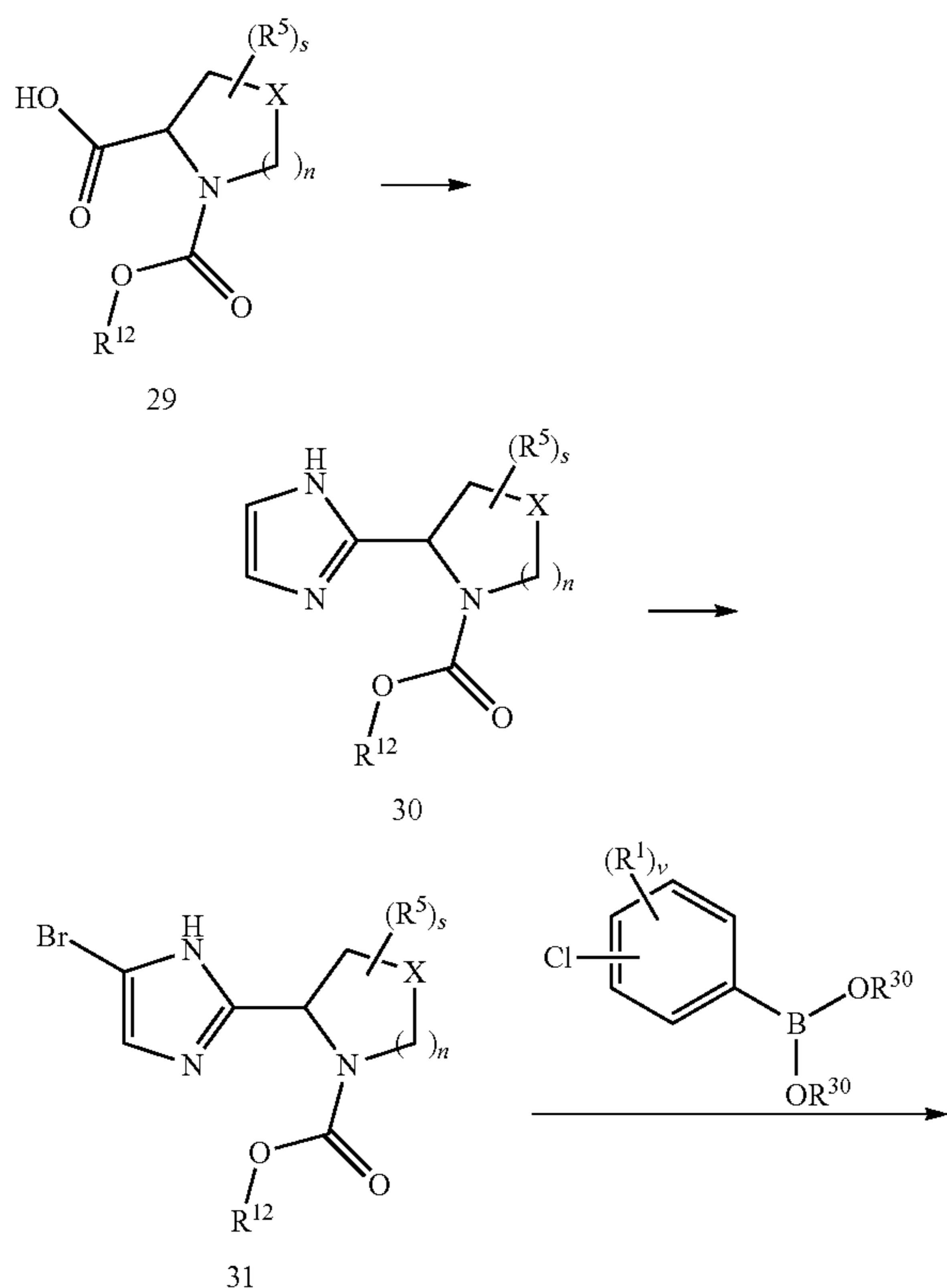
Scheme 7: Heteroaryls
