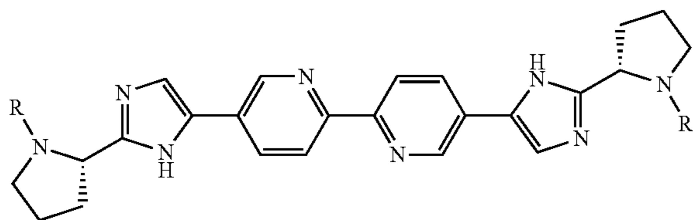
145a: R = Boc 145b: R = H
