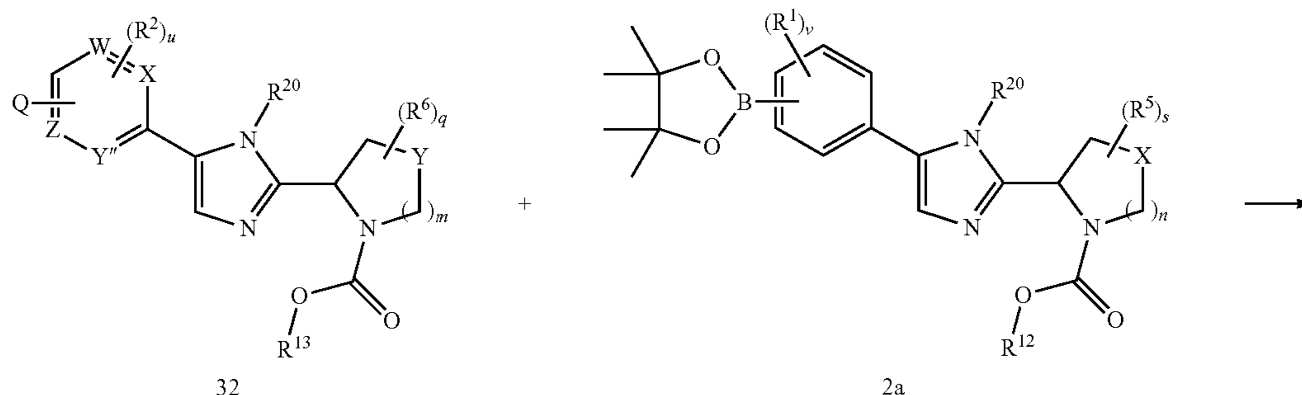
Scheme 8
