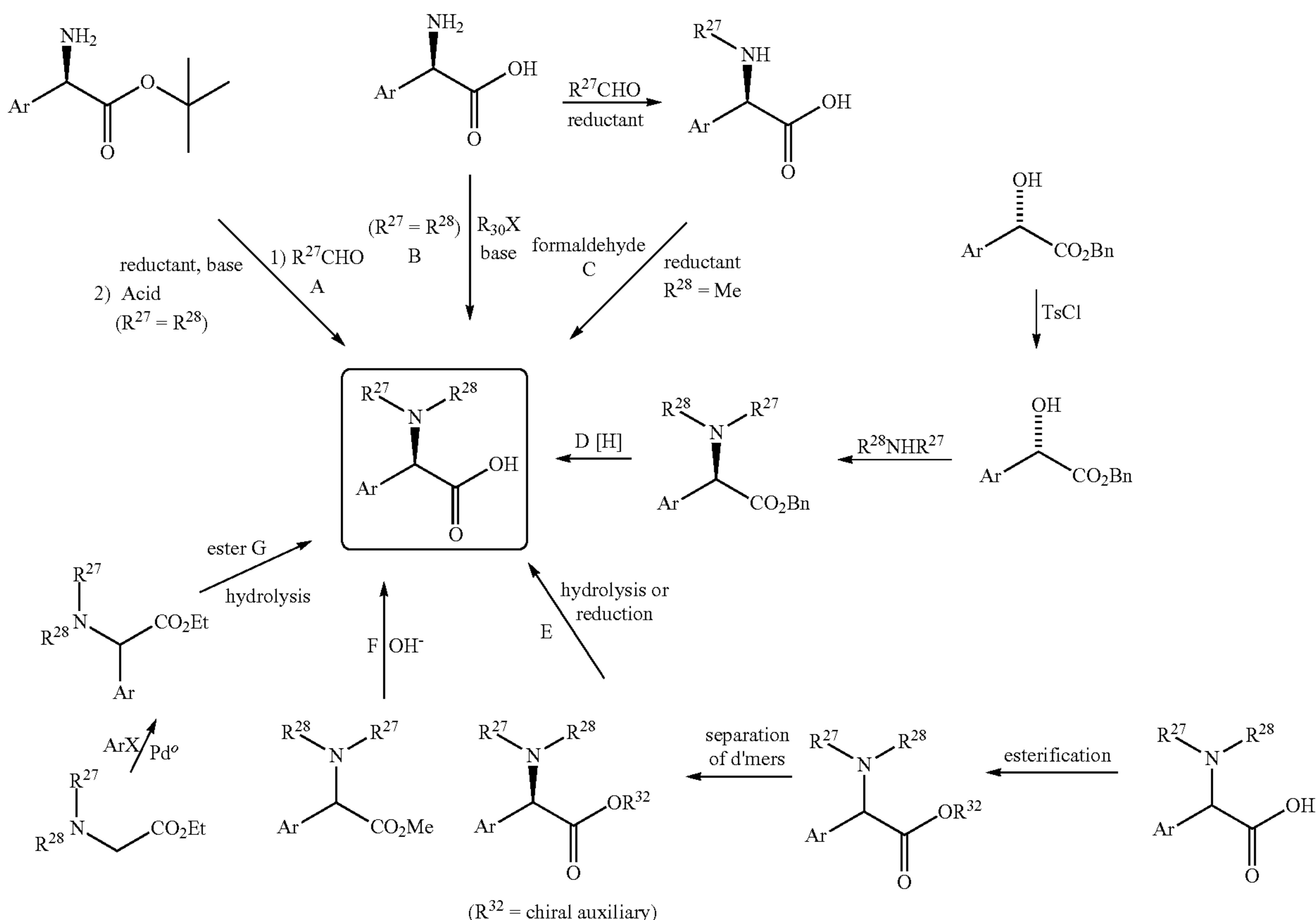
Scheme 12: Acylated Amino Acid Derivatives
