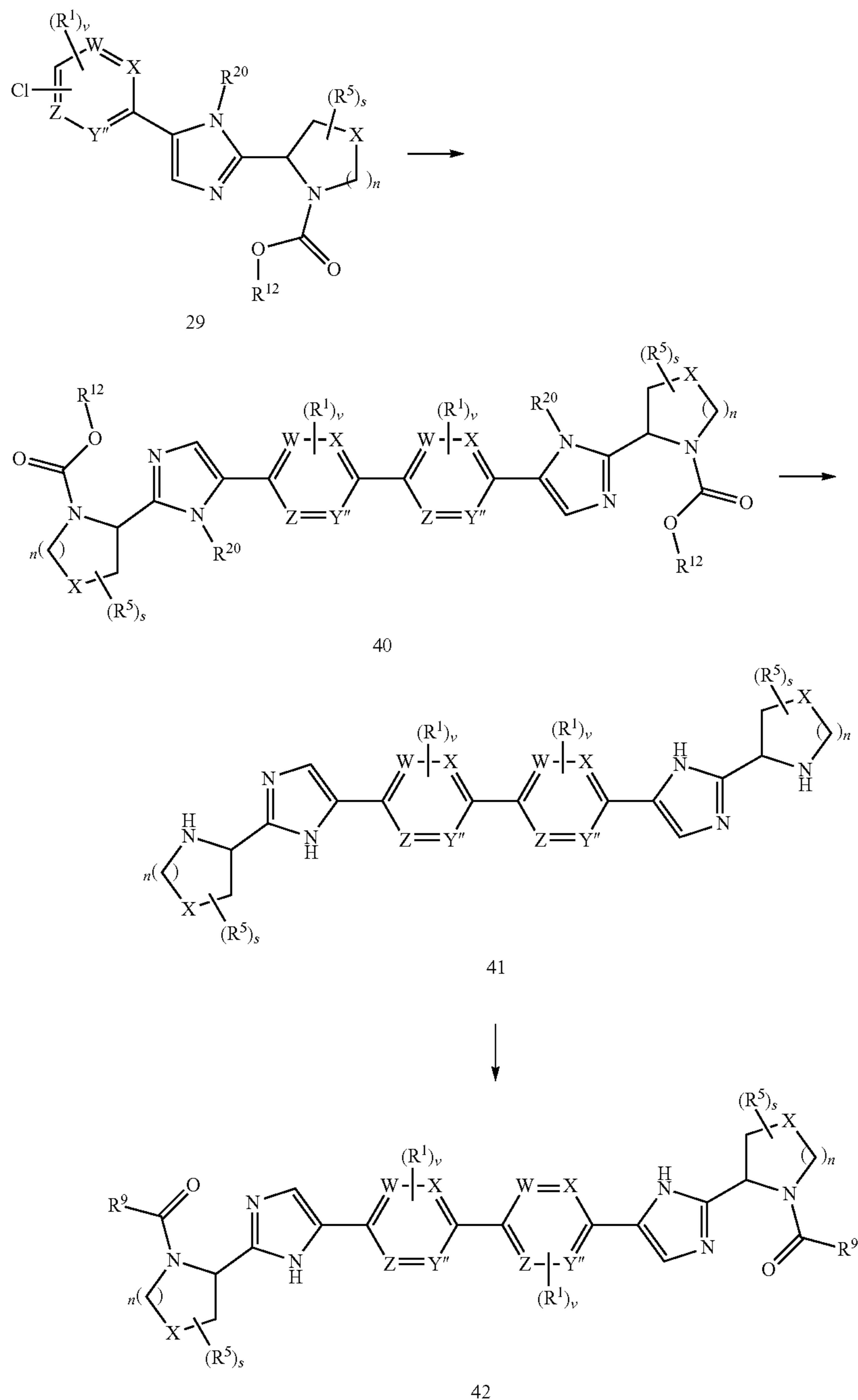
Scheme 9: Symmetric Cap Substituted Heteroaryls
