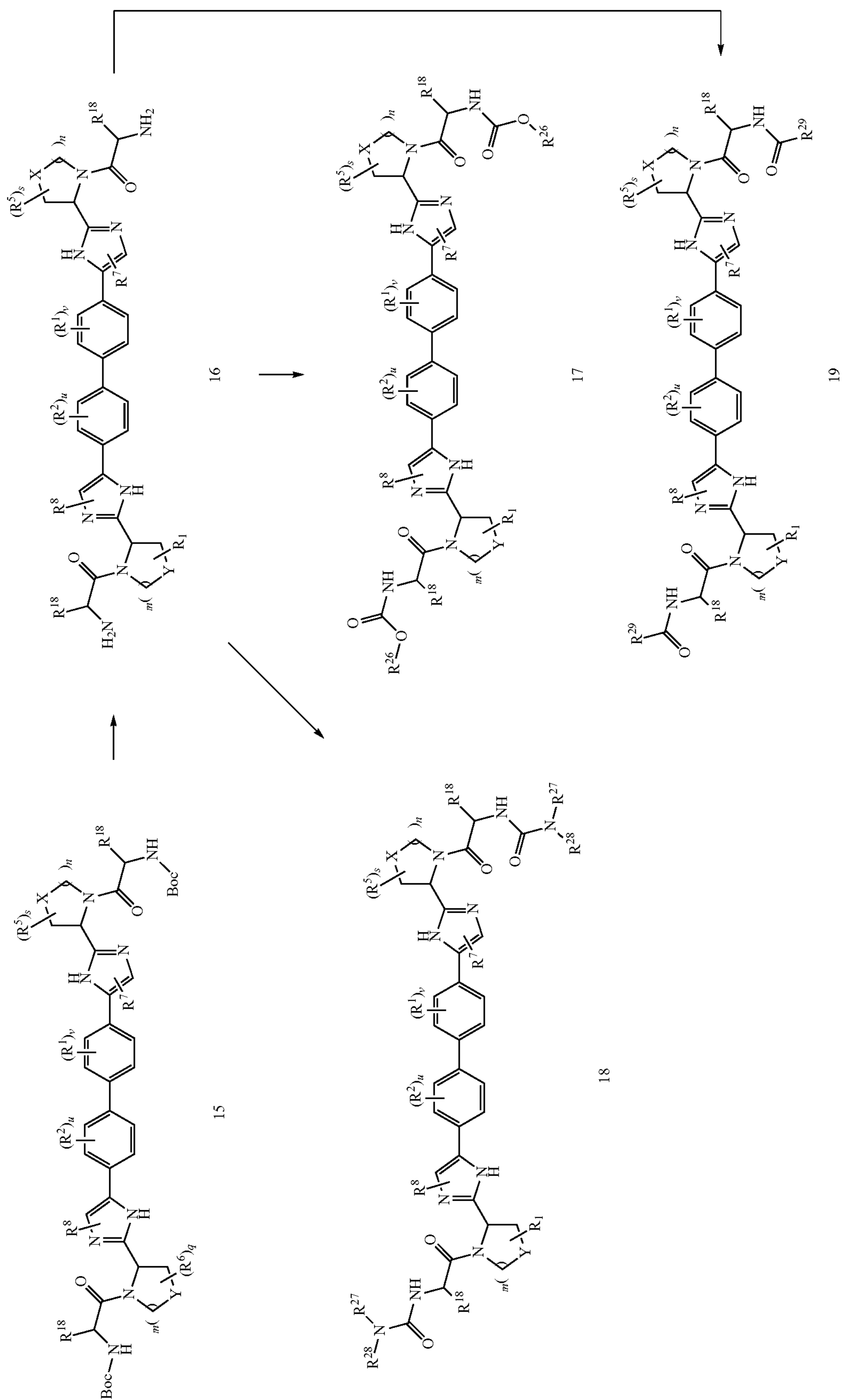
Scheme 4: Symmetric Biphenyls
