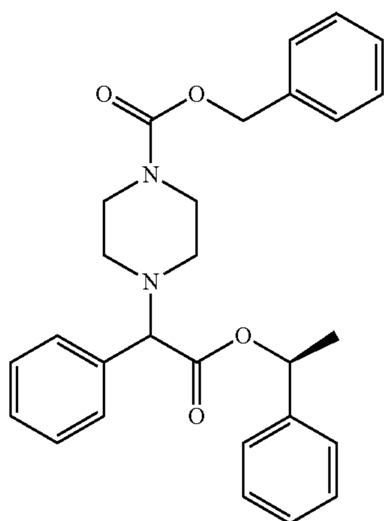
Intermediate-17a
