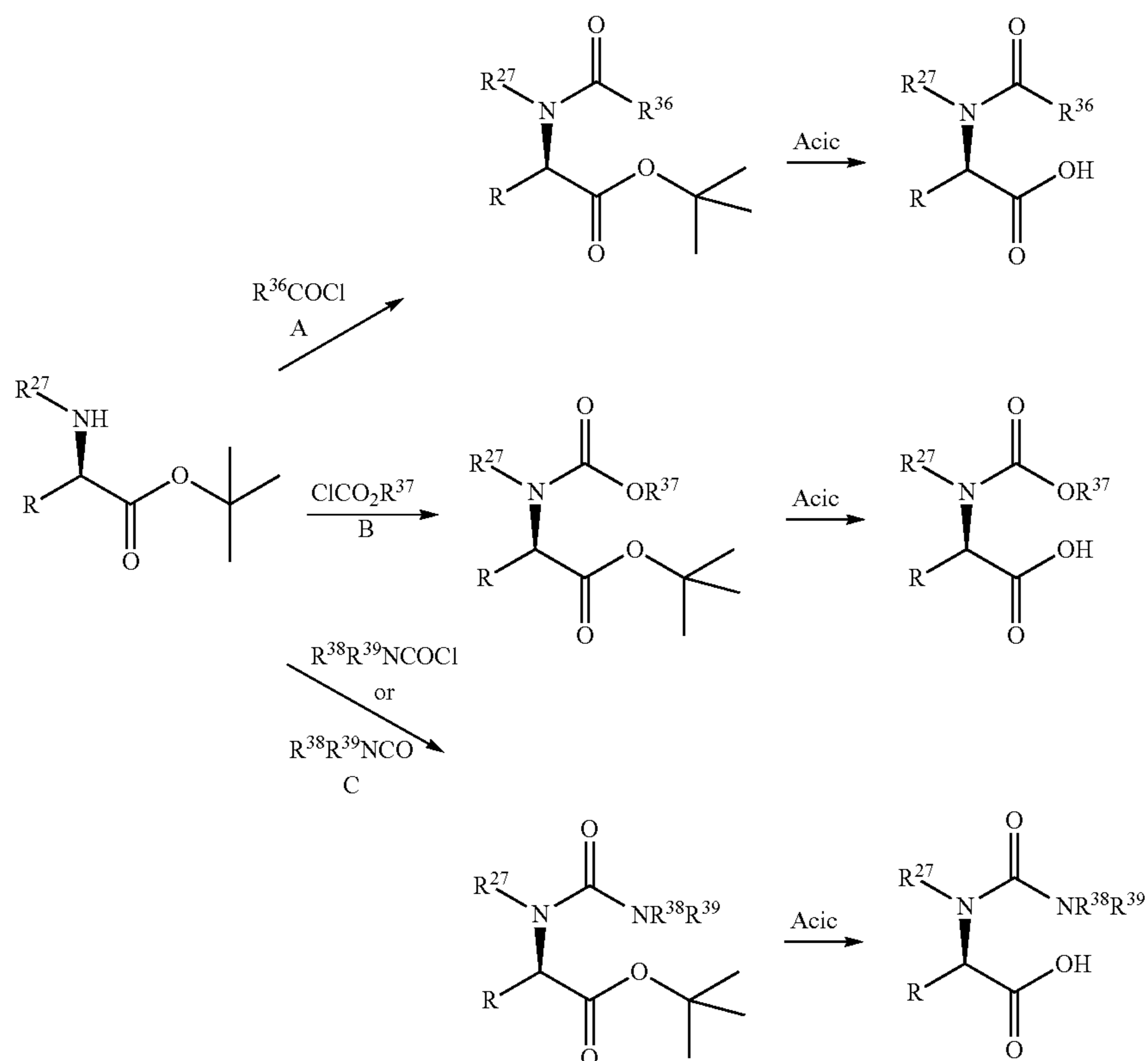
Scheme 13
