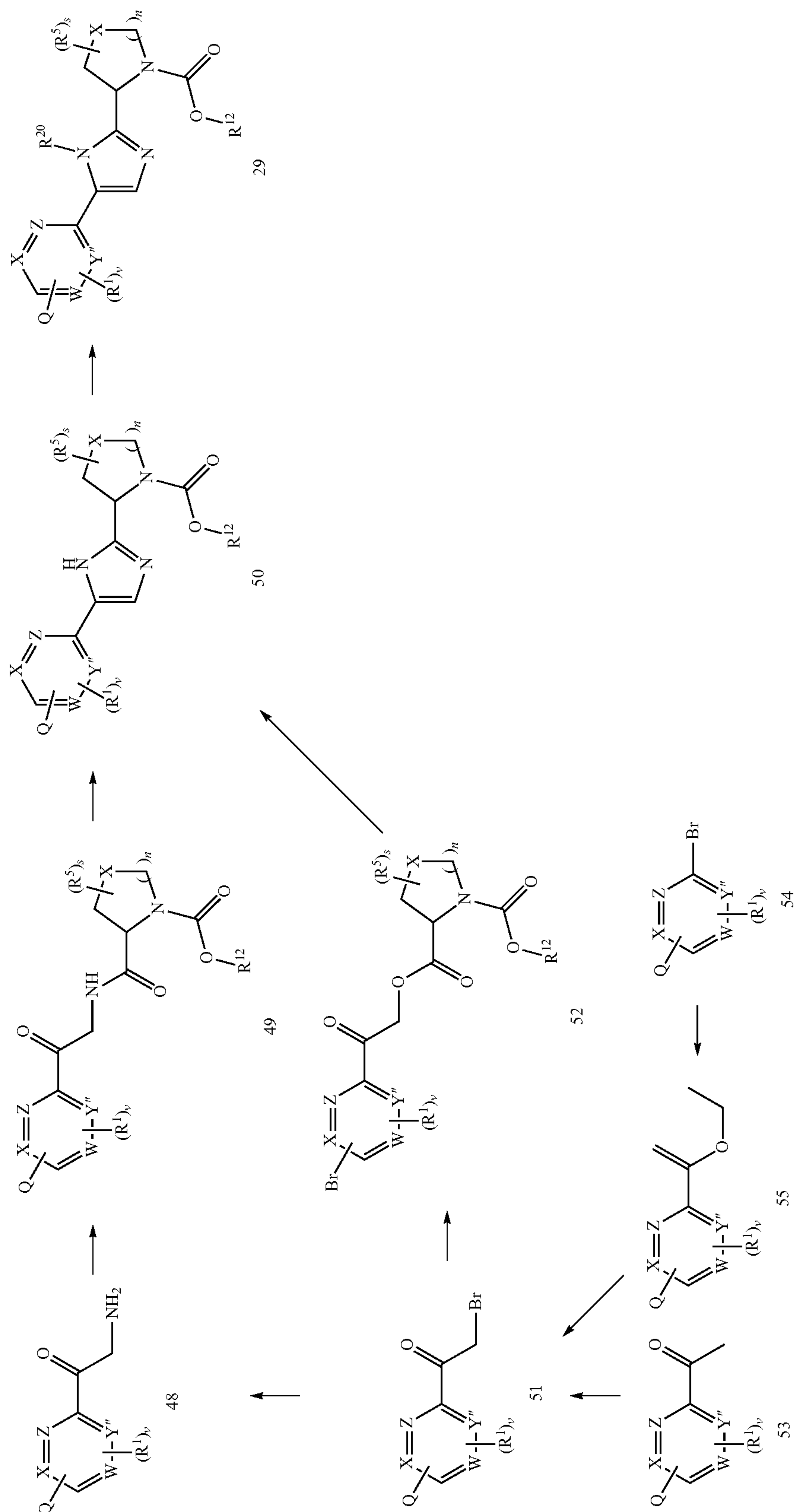
Scheme 11: Substituted Phenylglycine Derivatives
