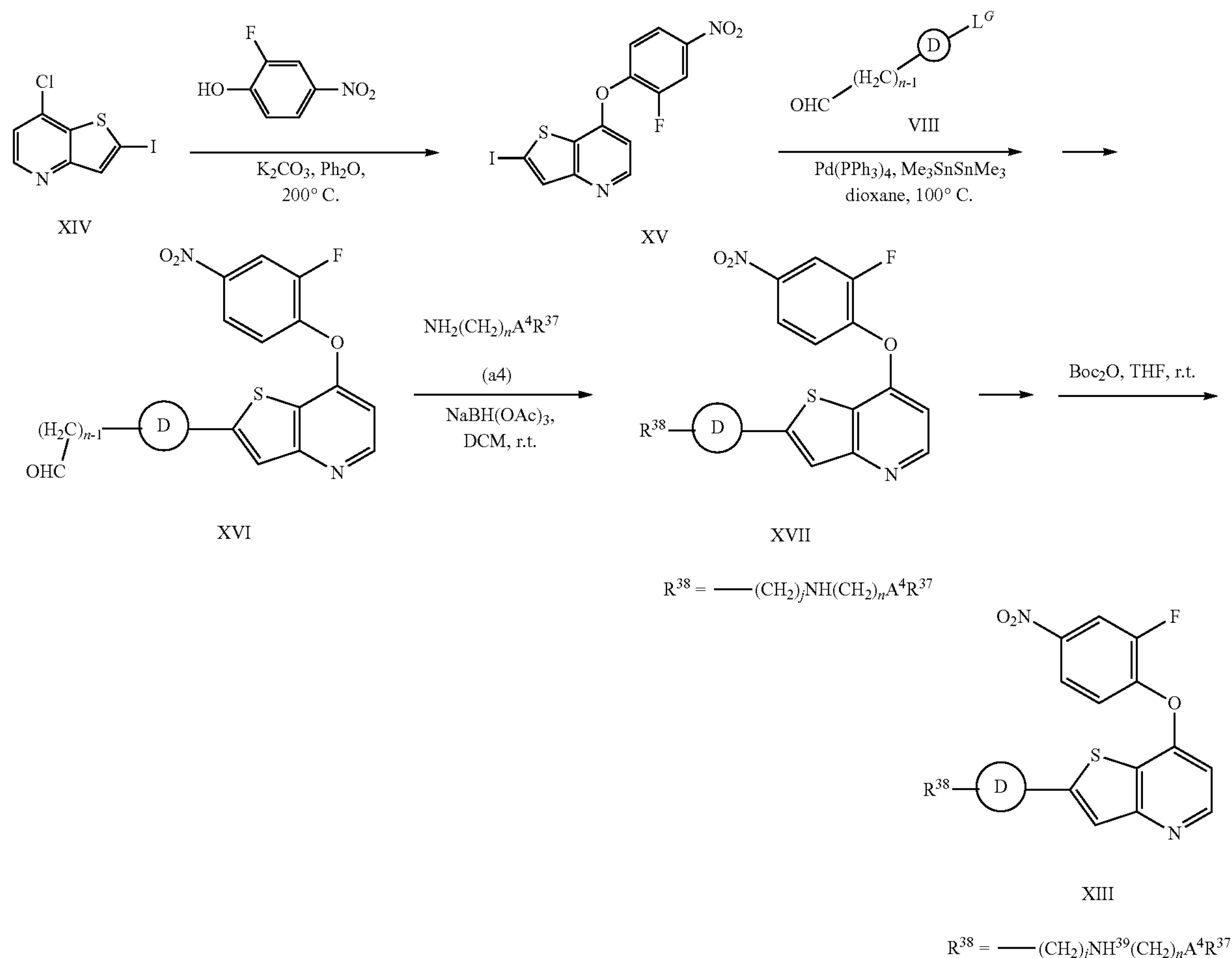
Scheme C
