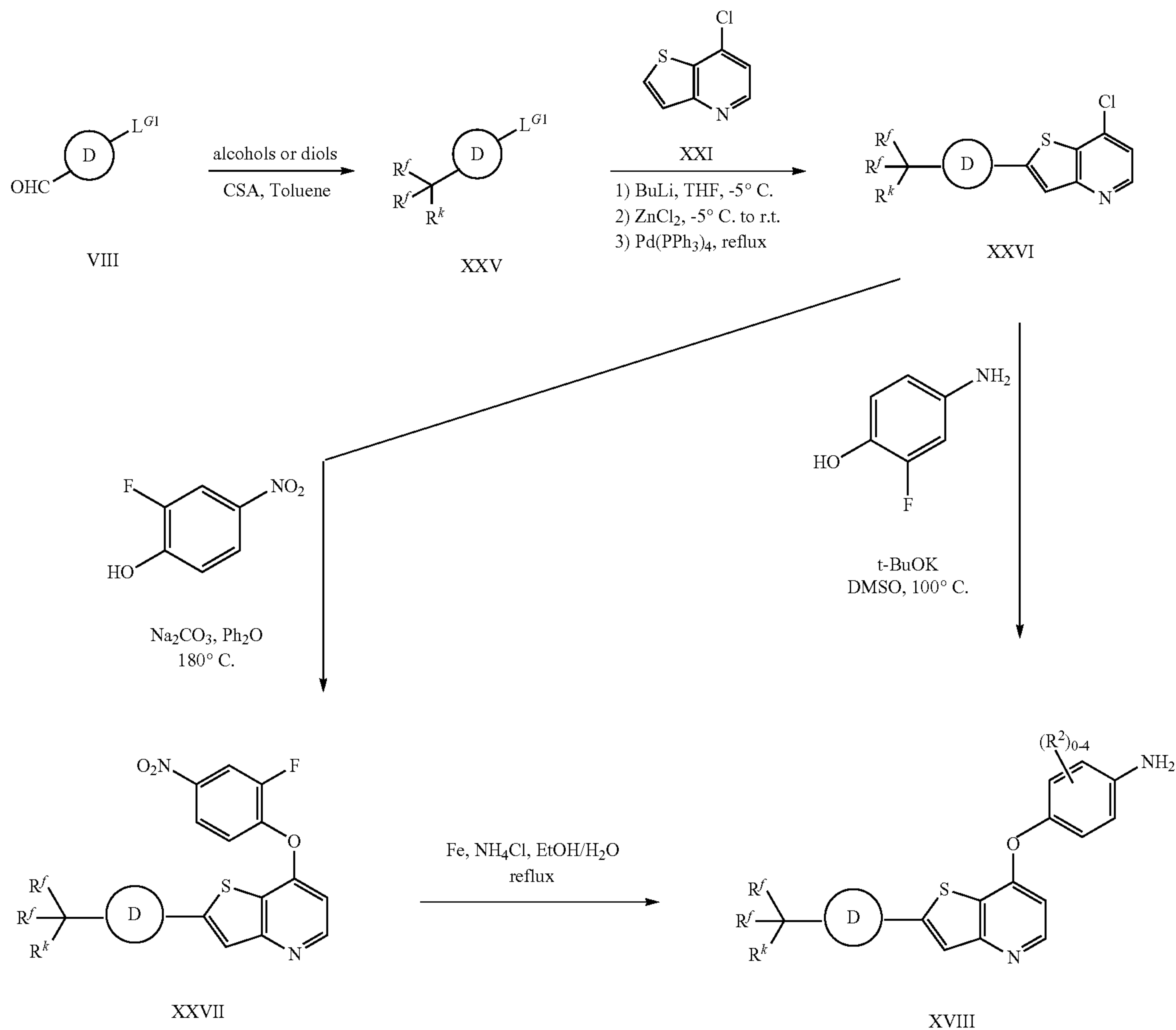
Scheme G
