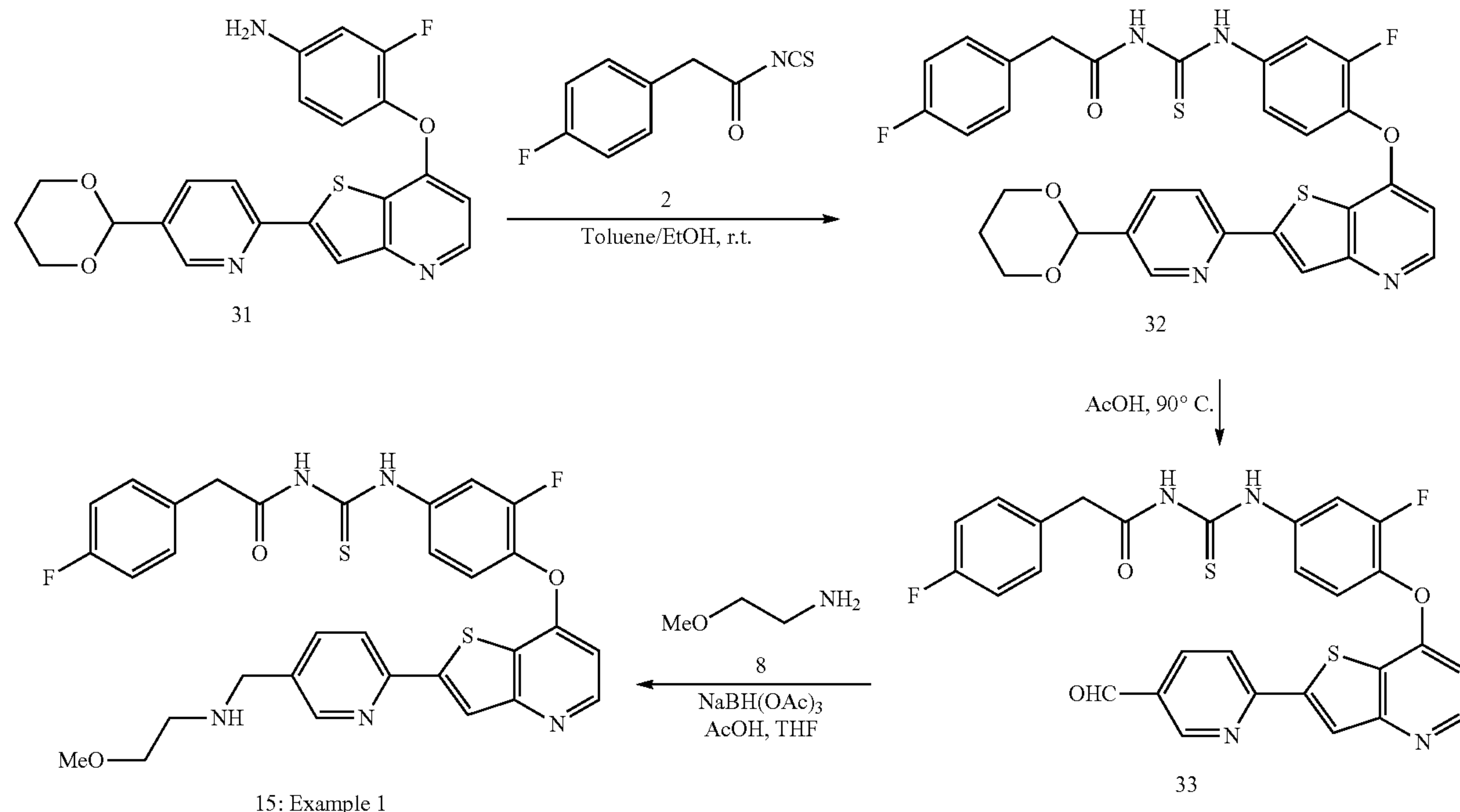
Scheme 9
