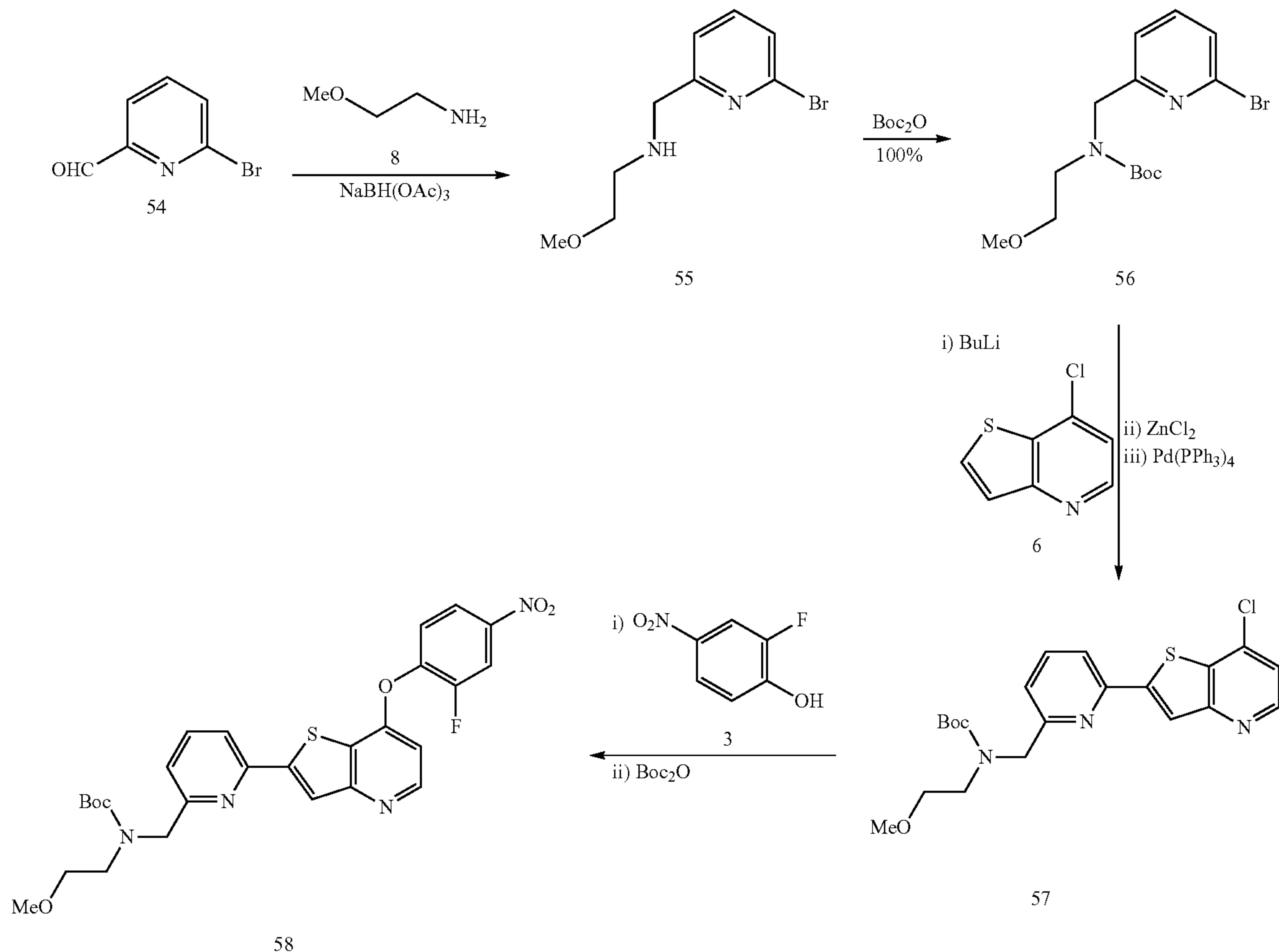
Scheme 15
