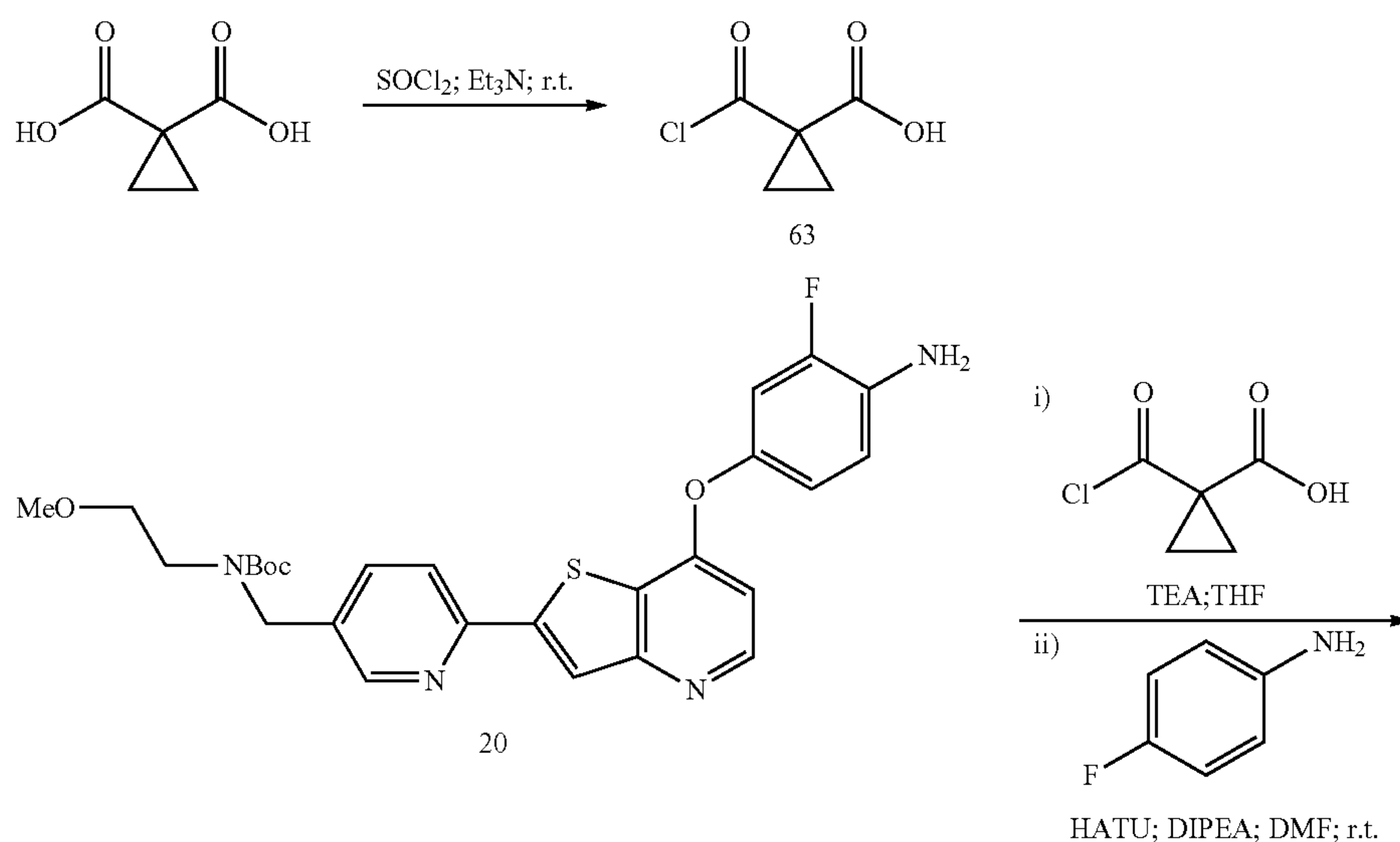
Scheme 17
