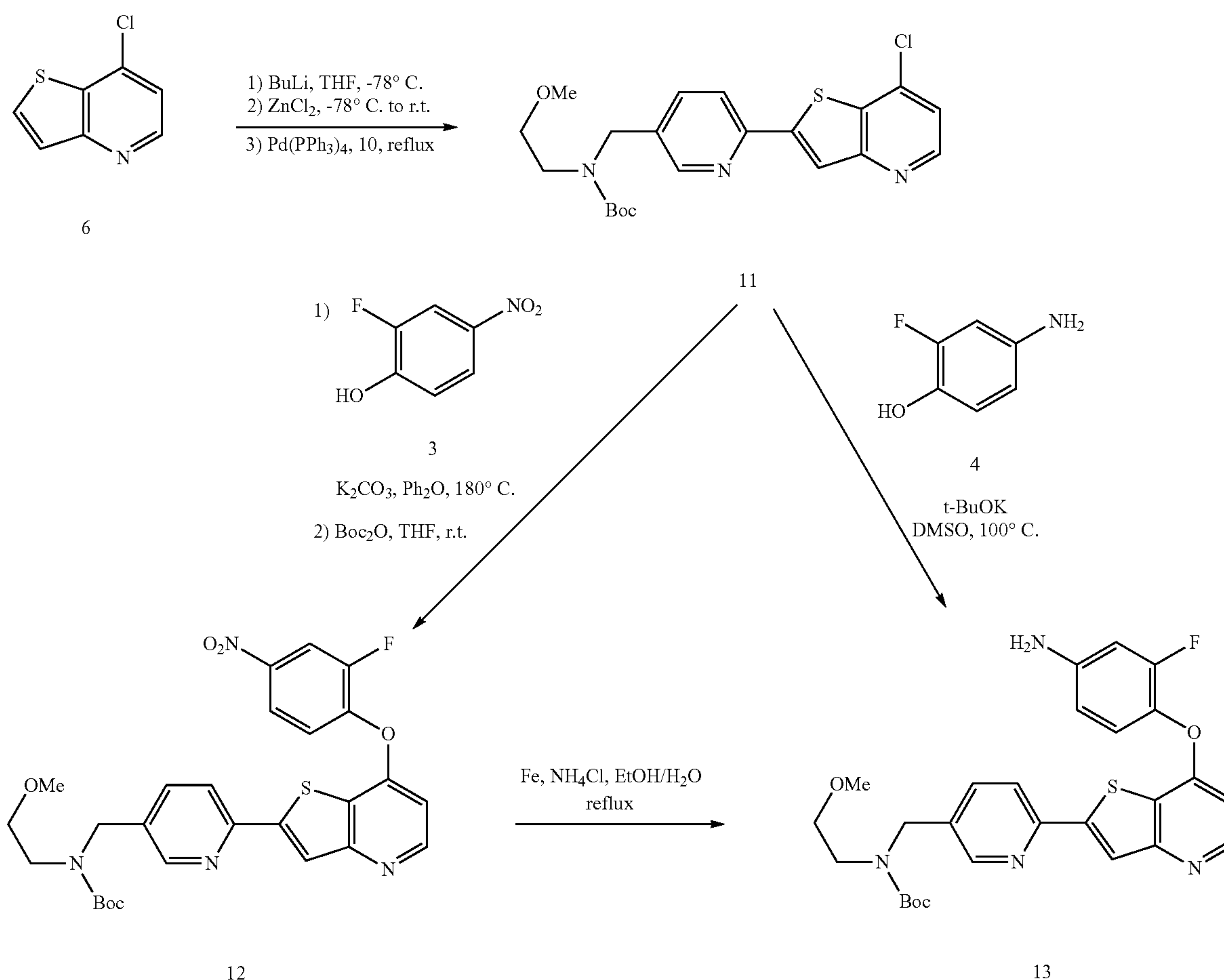
Scheme 3
