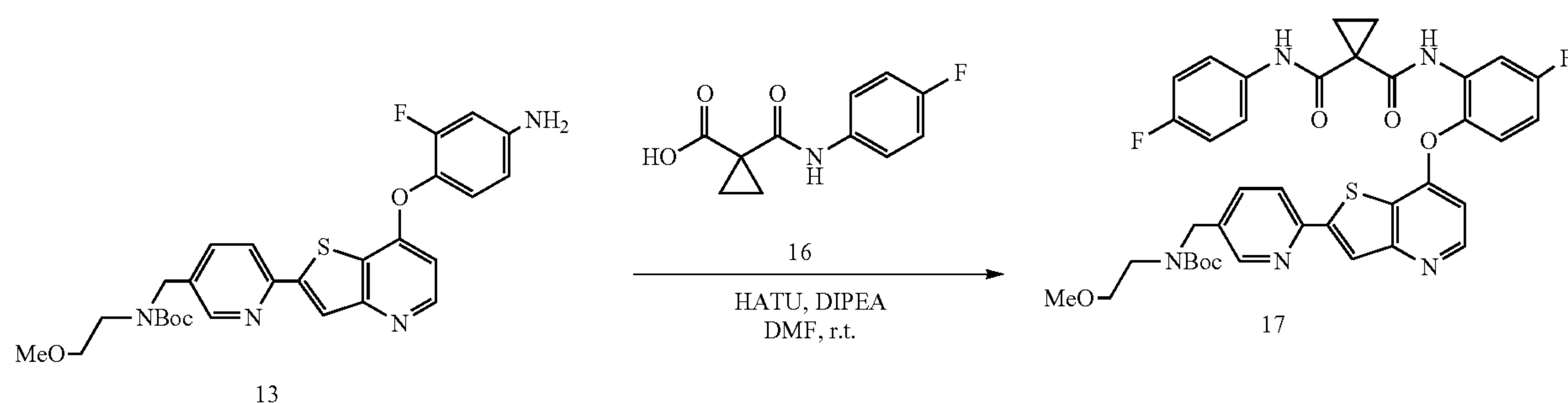
Scheme 5
