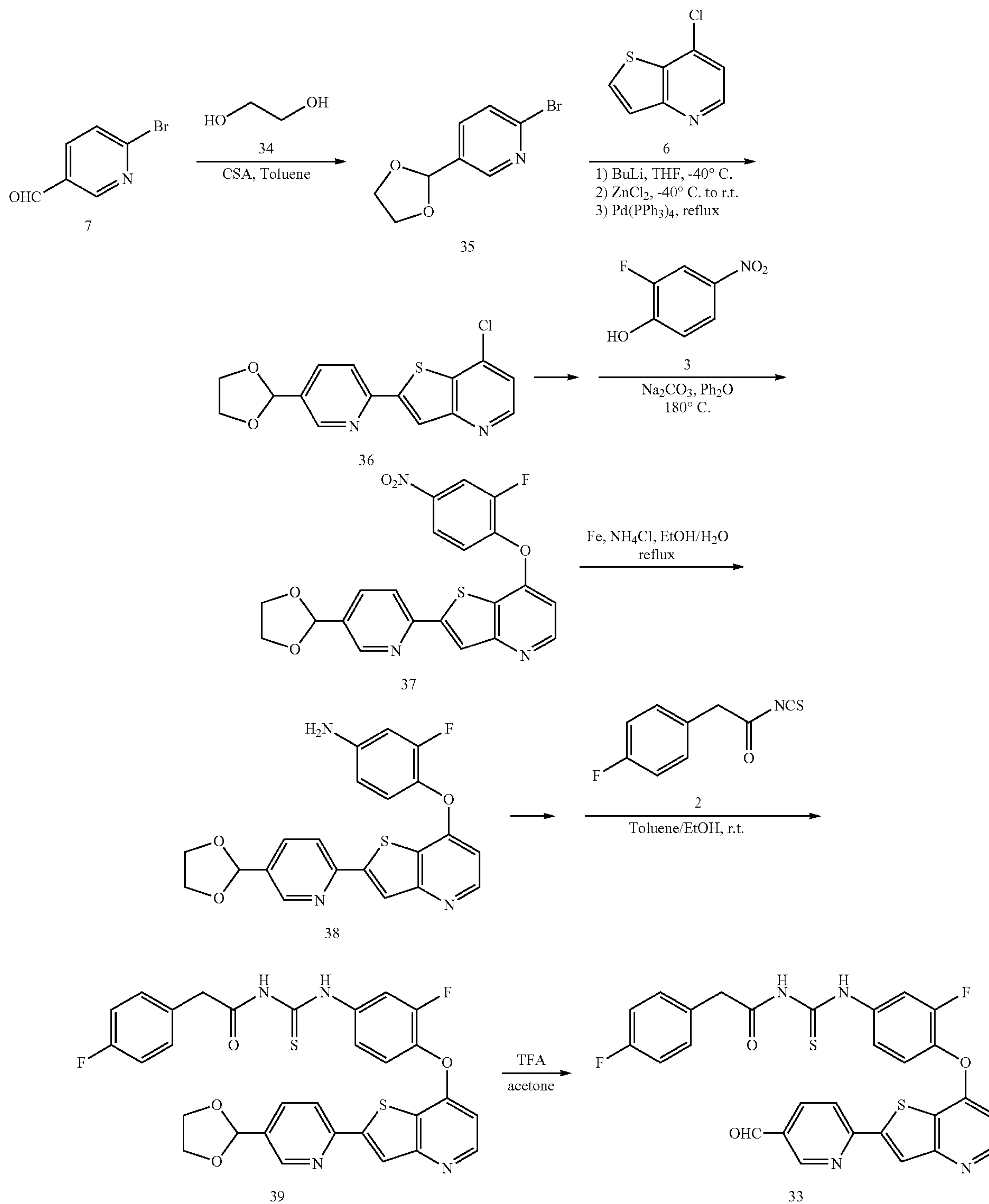
Scheme 10
