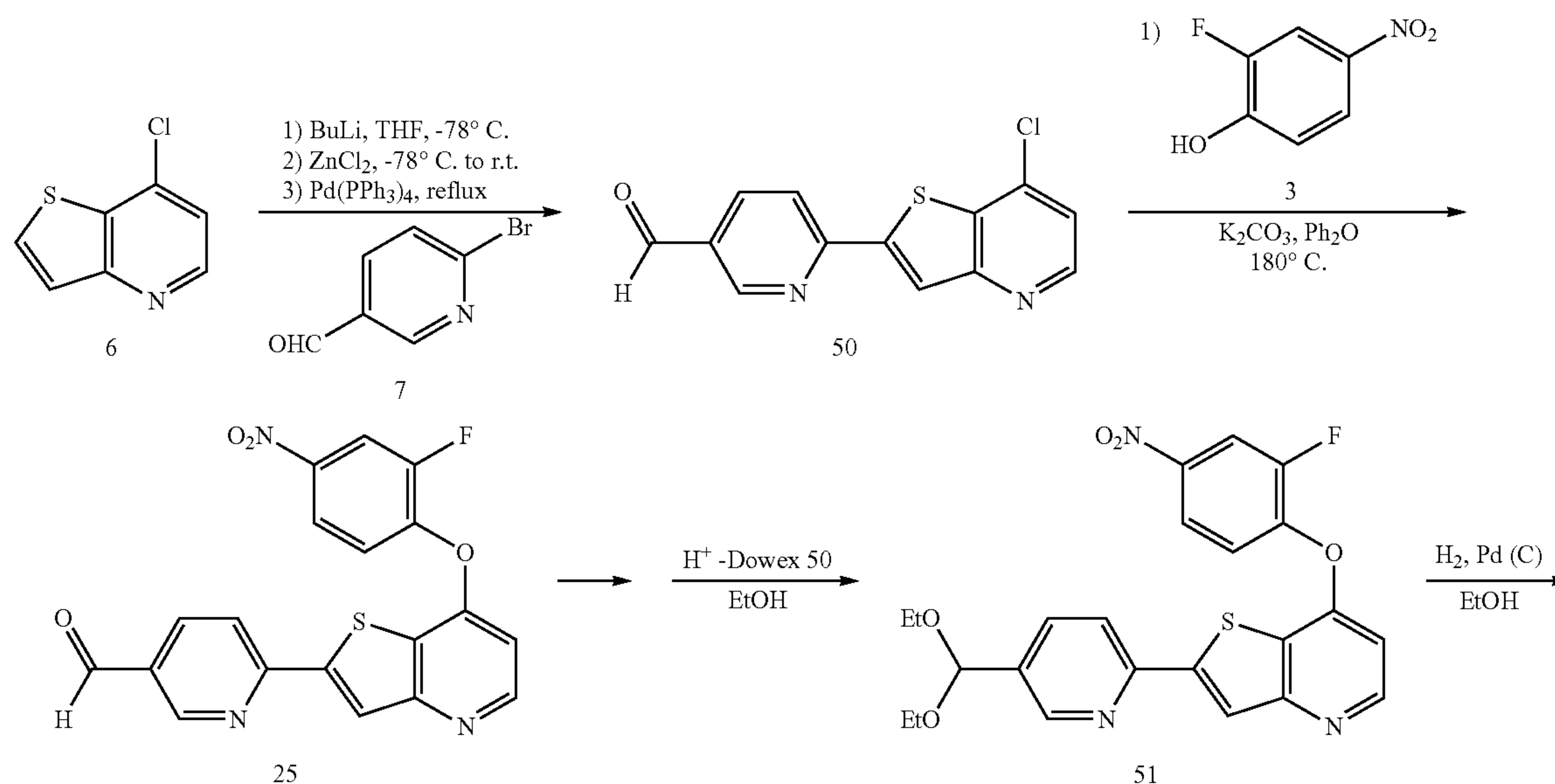
Scheme 14
