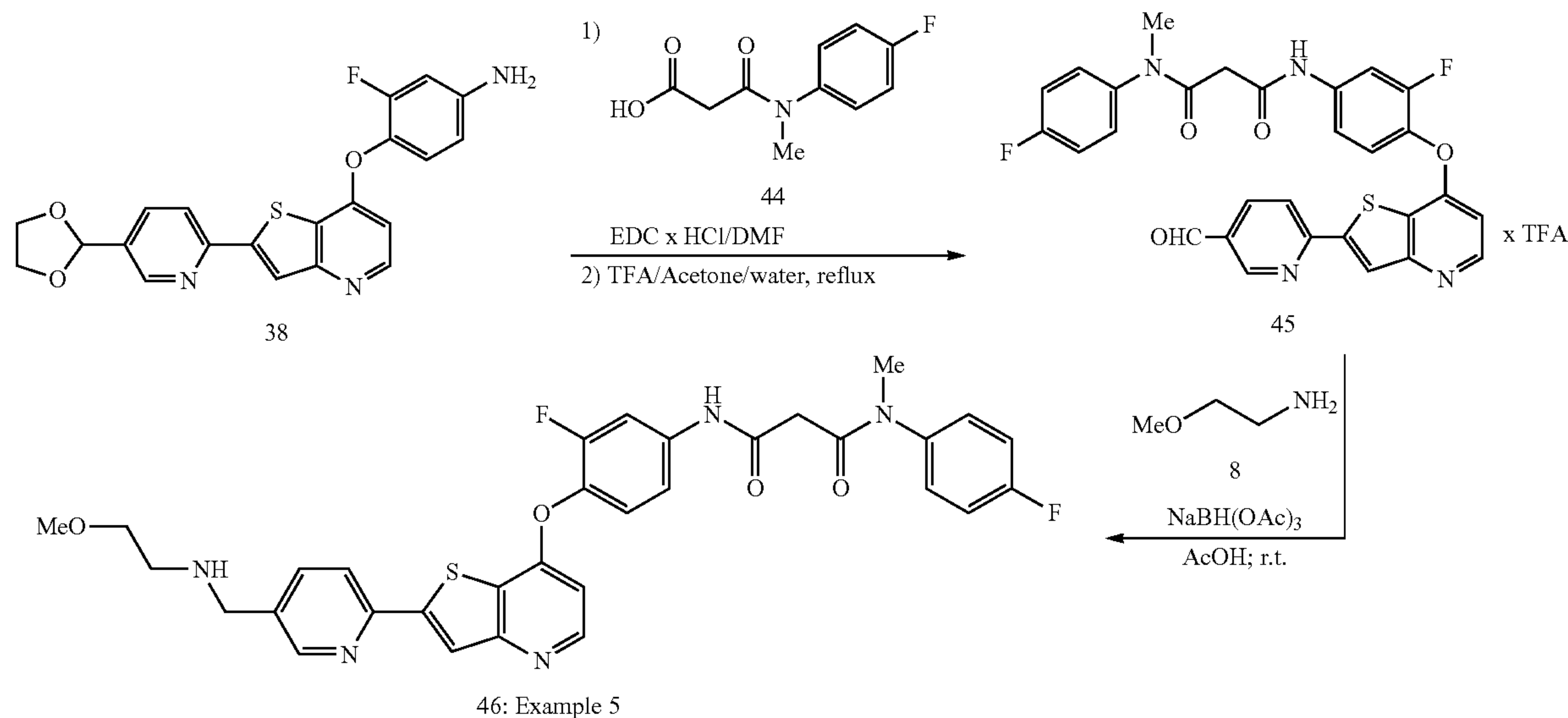
Scheme 12
