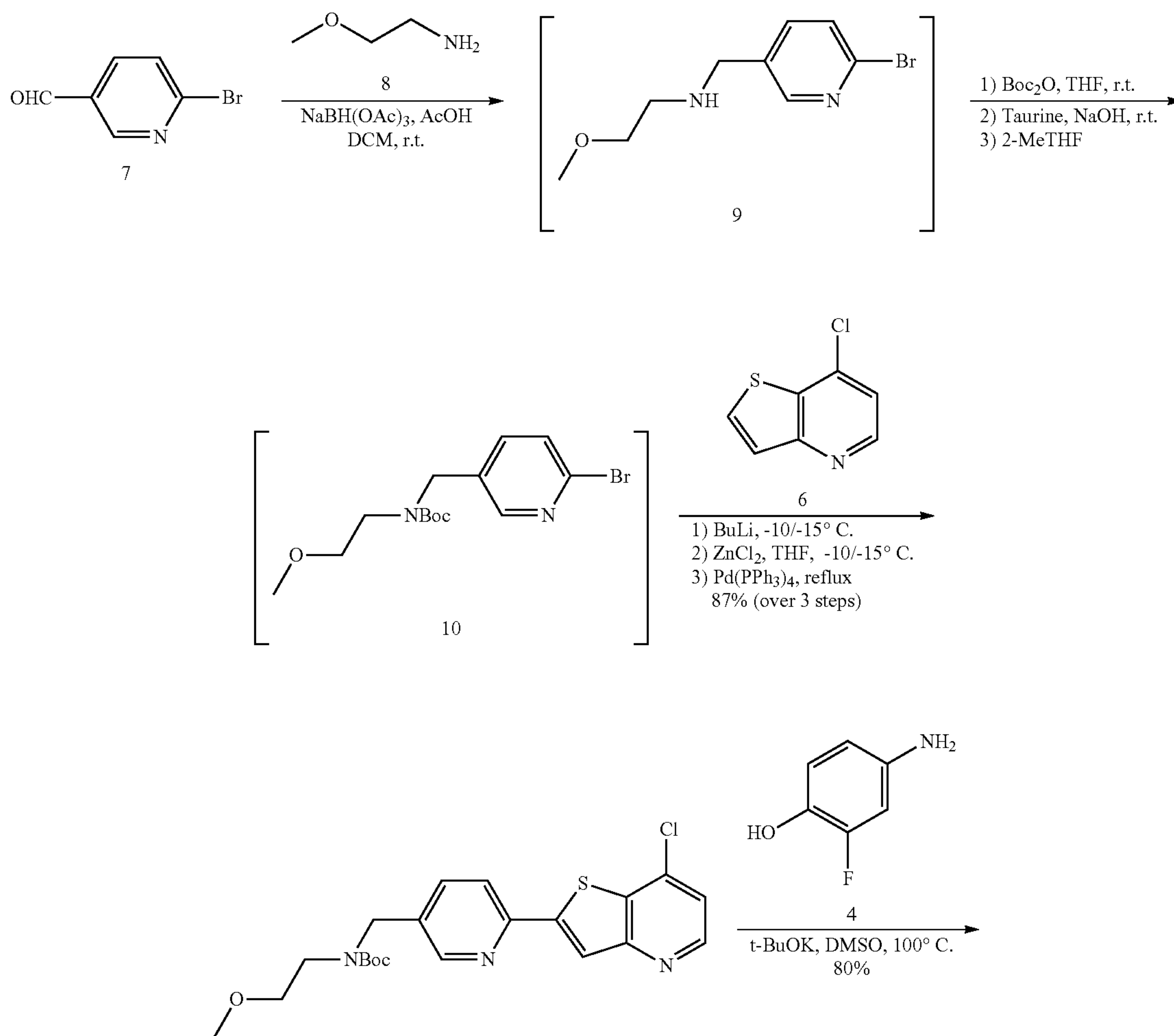
Scheme 20
