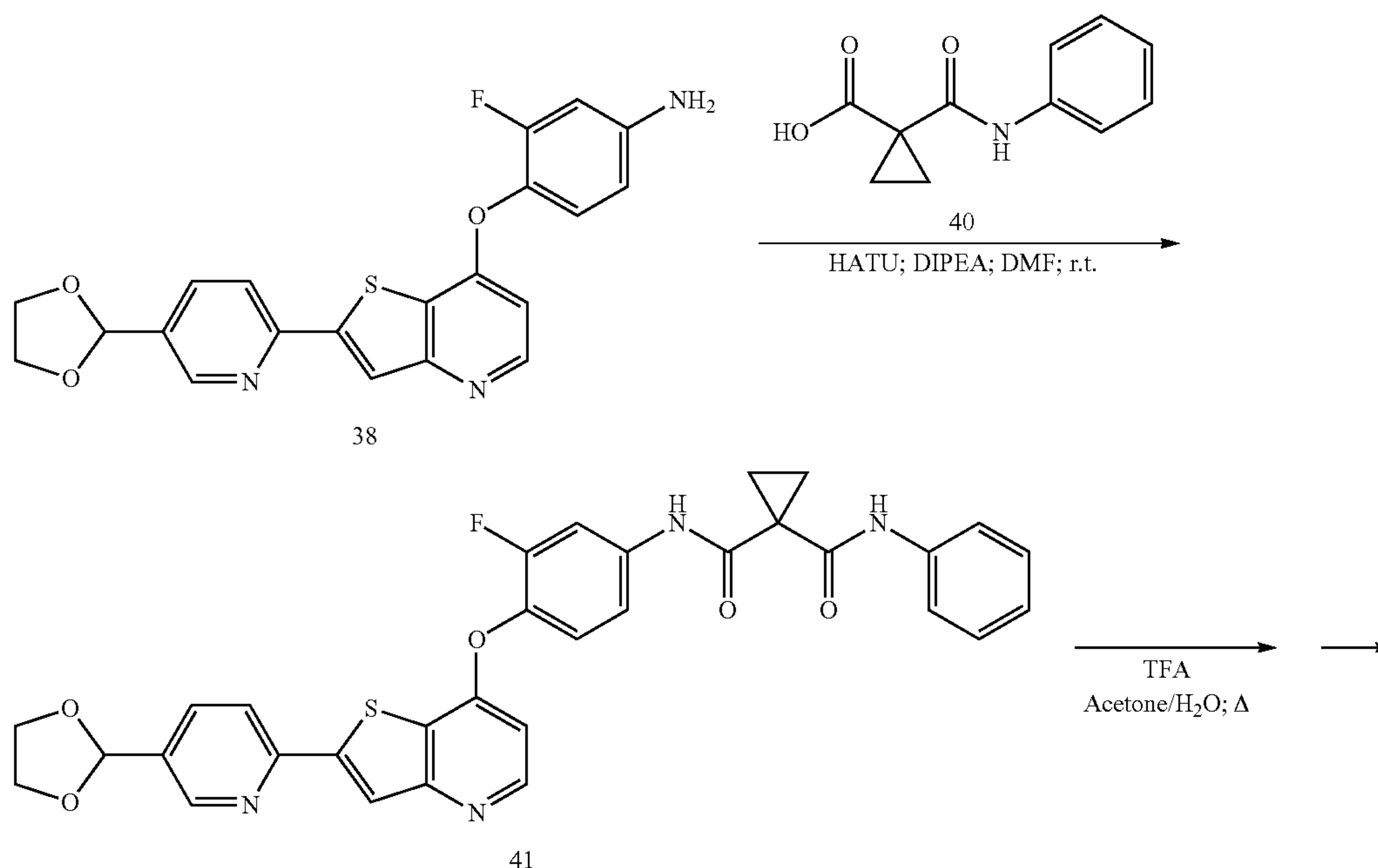
Scheme 11
