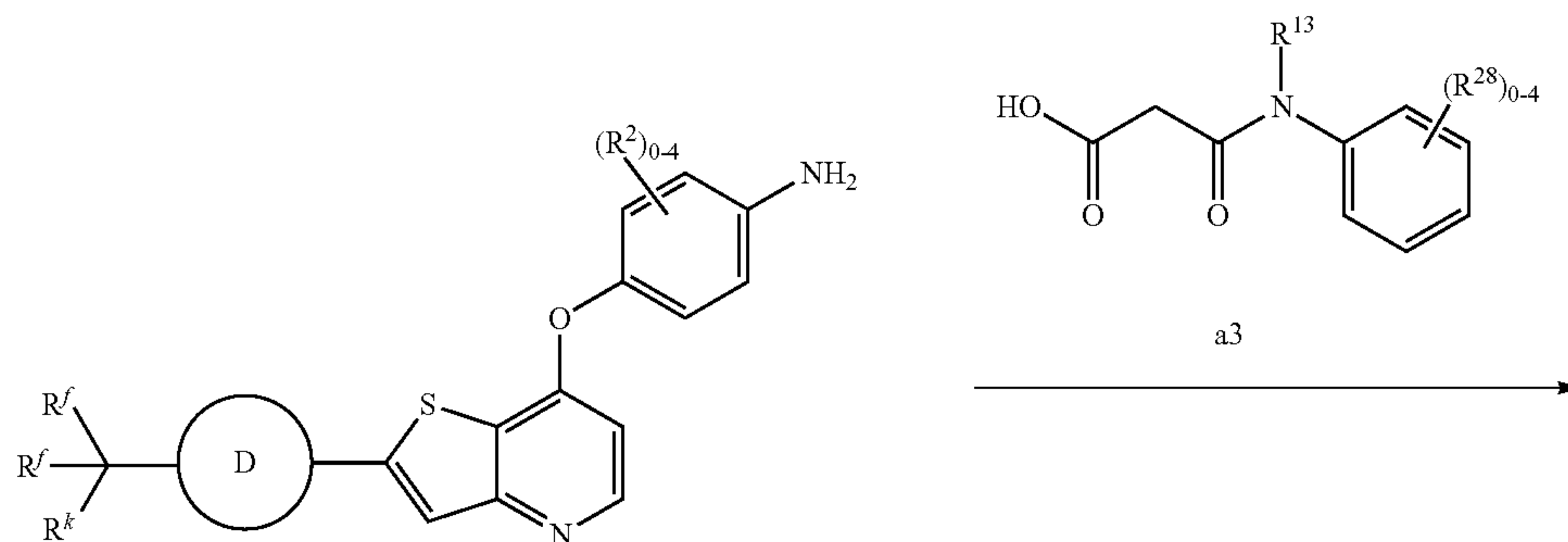
Scheme F
