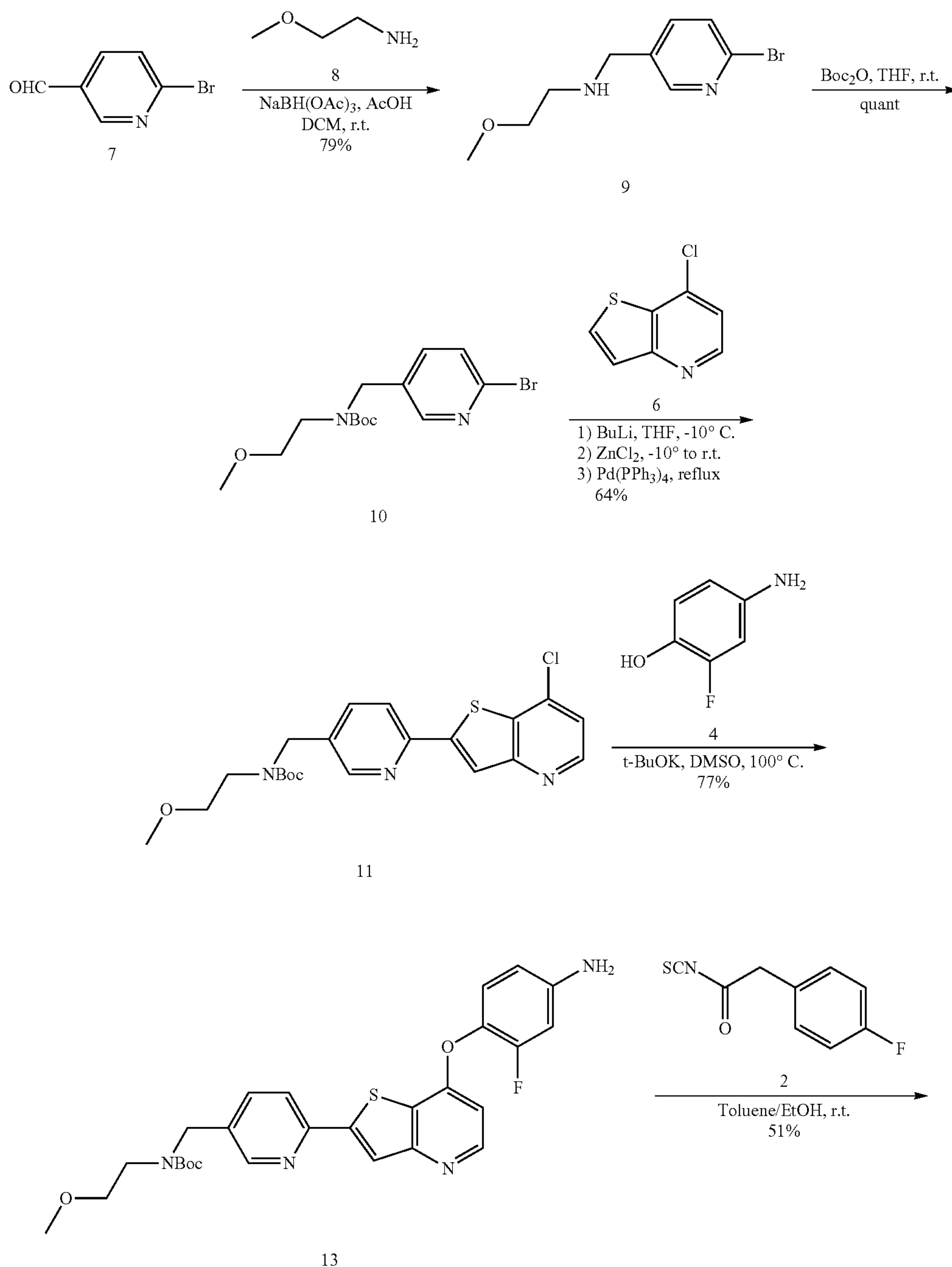
Scheme 19
