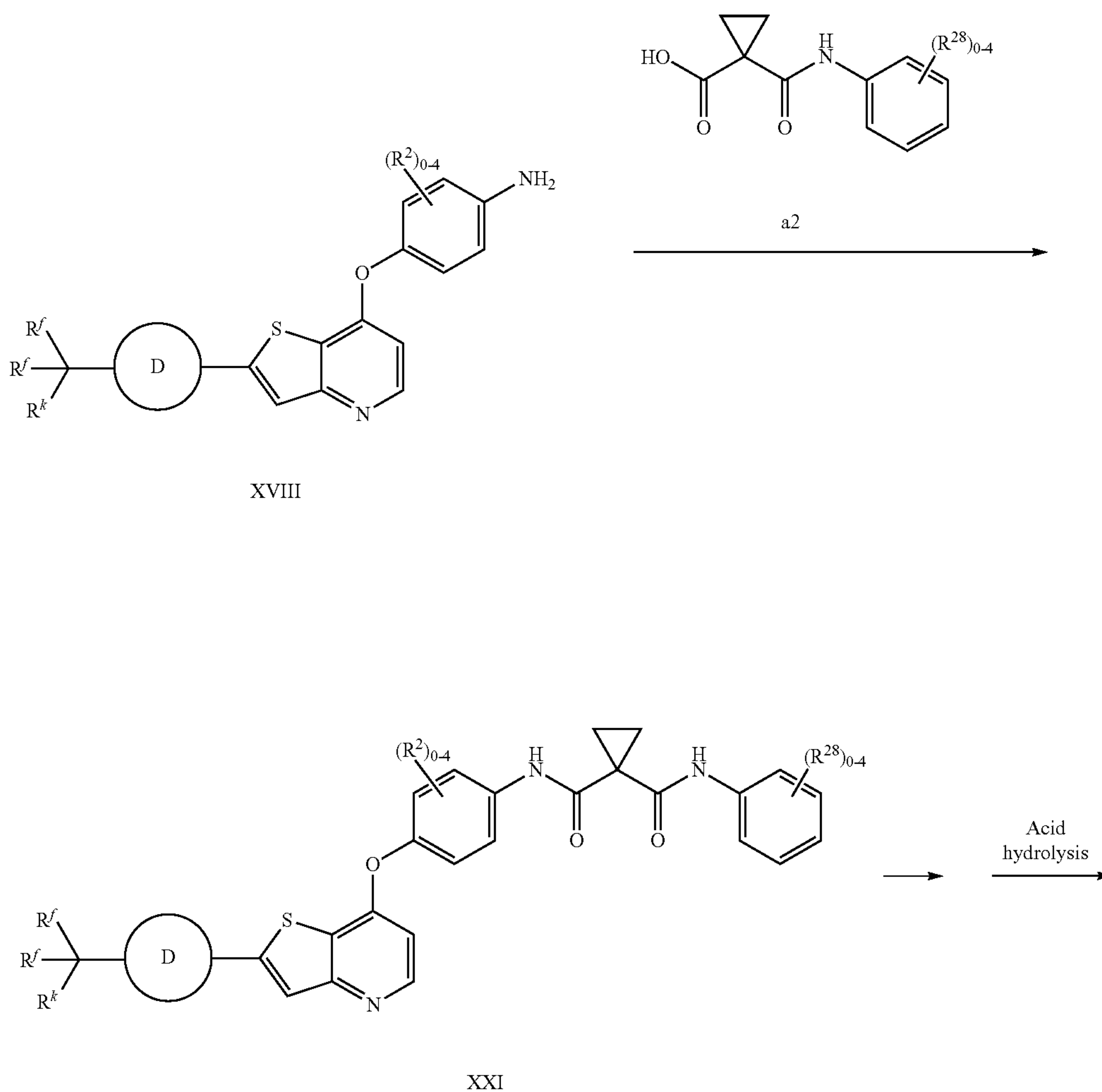
Scheme E
