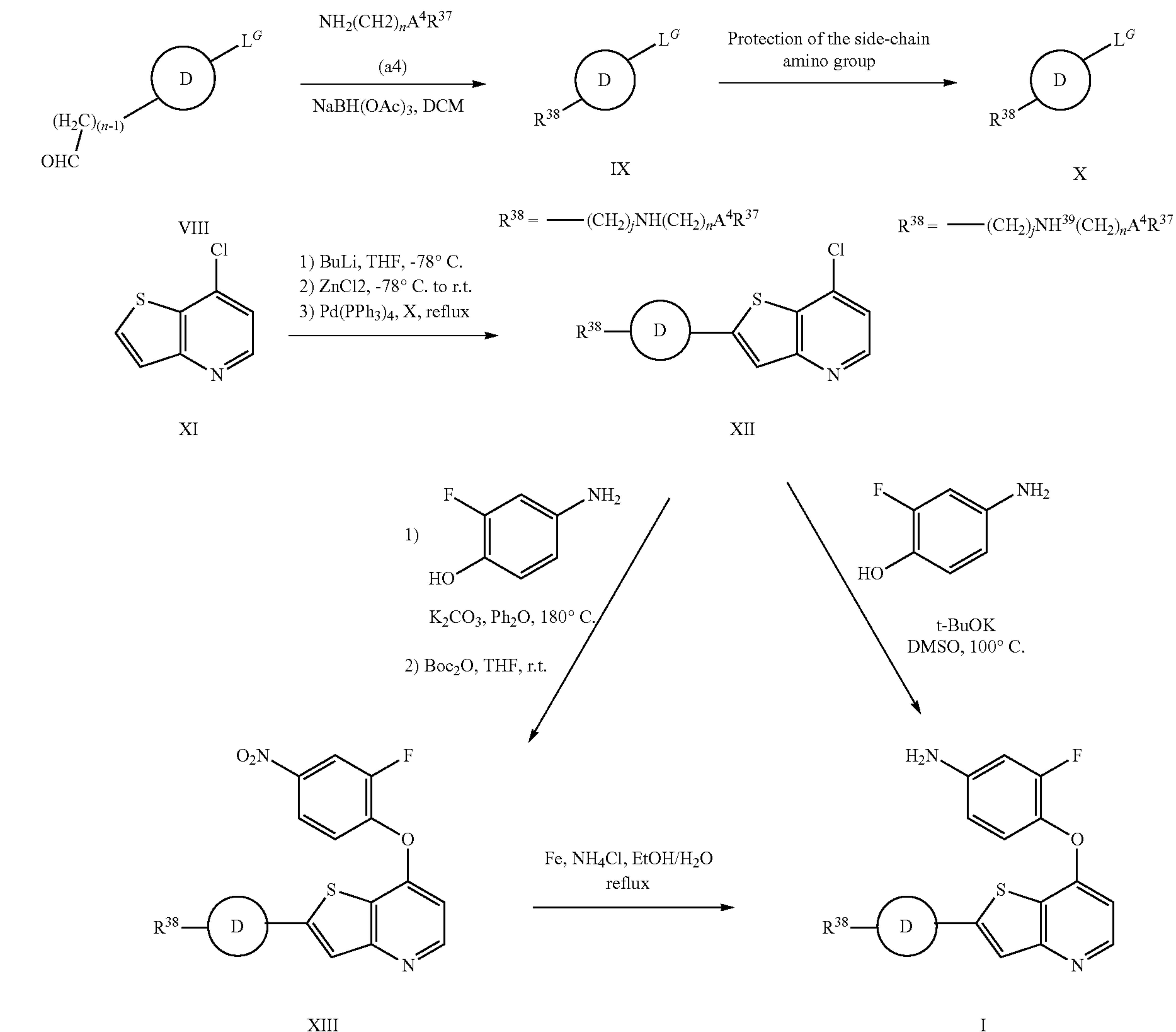
Scheme B
