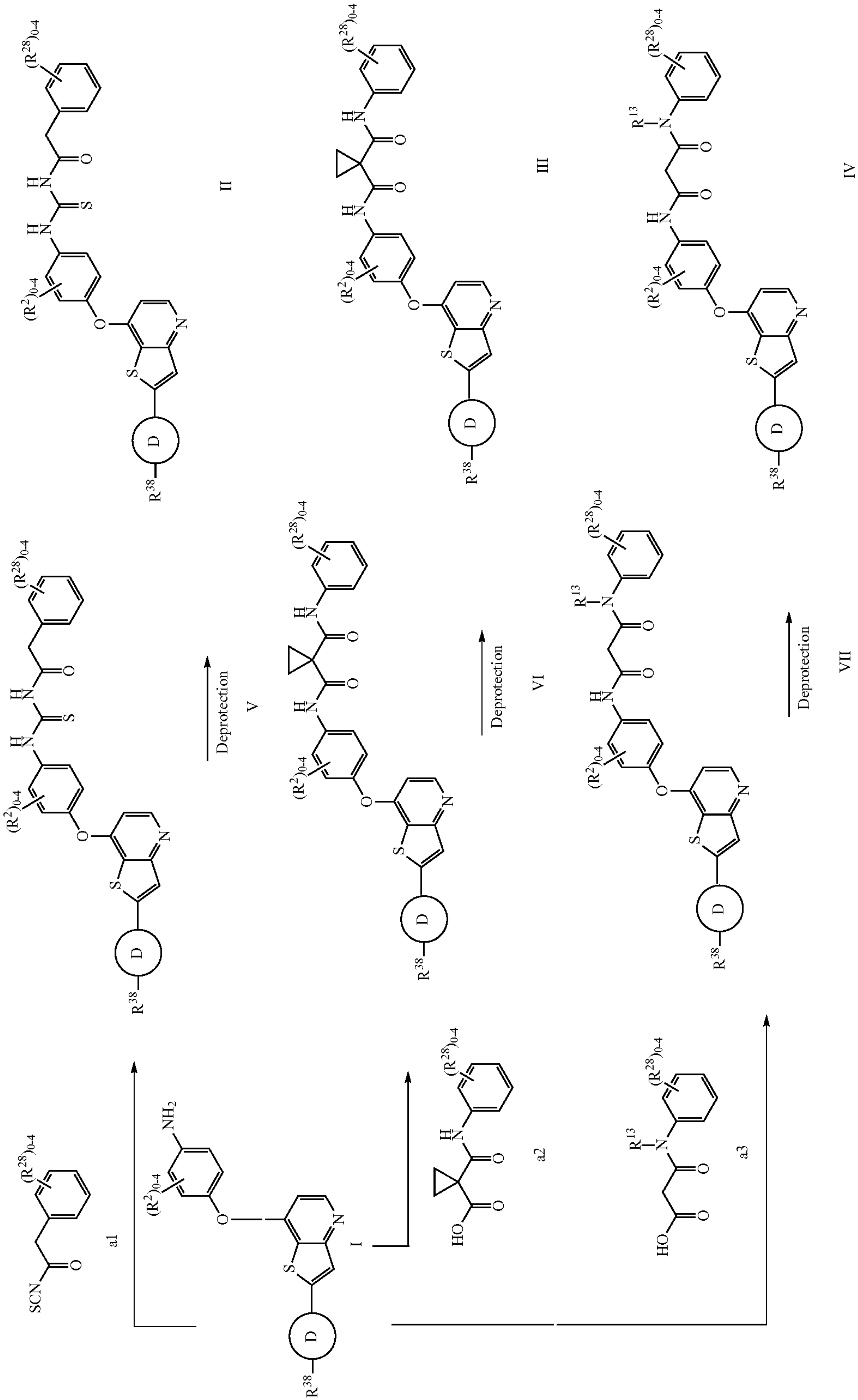
Scheme A
