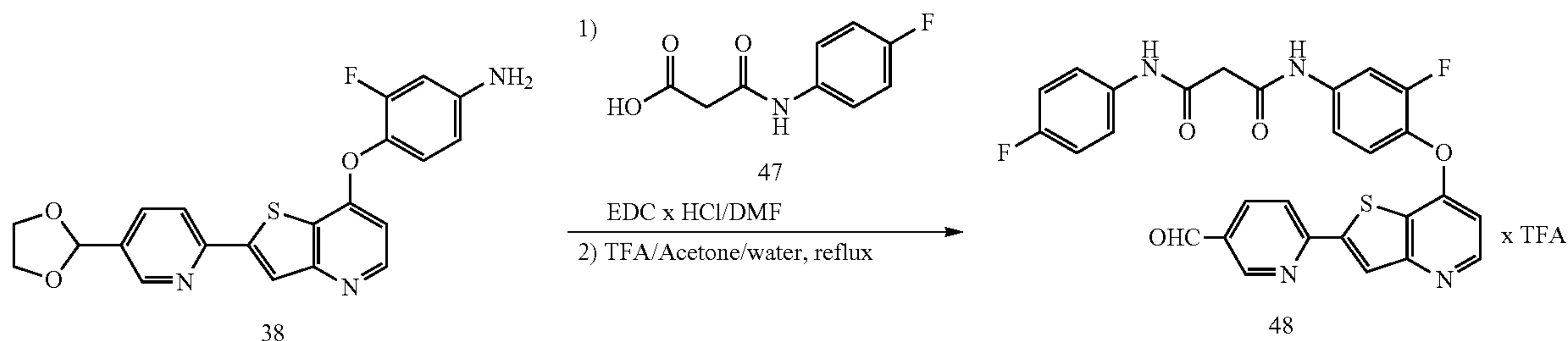
Scheme 13
