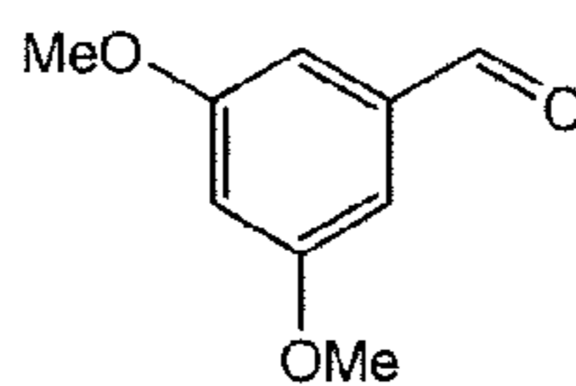
3,5-dimethoxybenzaldehyde
