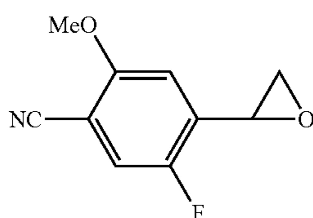
5-Fluoro-2-methoxy-4-oxiran-2-ylbenzotrile
