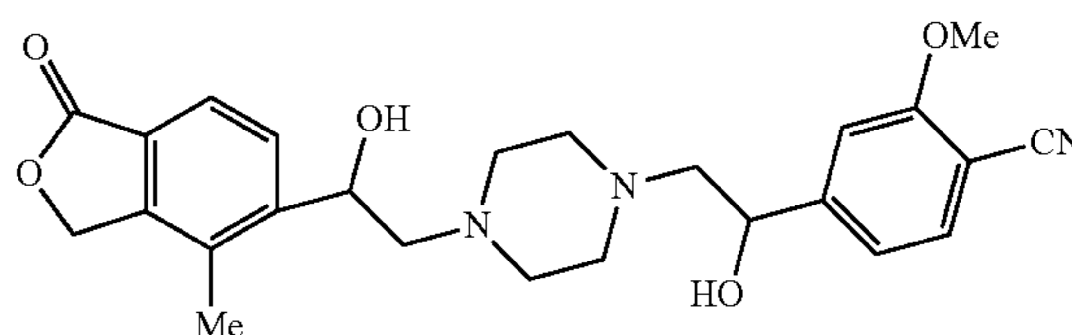
4-(1-hydroxy-2-{4-[2-hydroxy-2-(4-methyl-1-oxo-1,3-dihydro-2-benzofuran-5-yl)ethyl]piperazin-1-yl}ethyl)-2-(methoxy)benzonitrile
