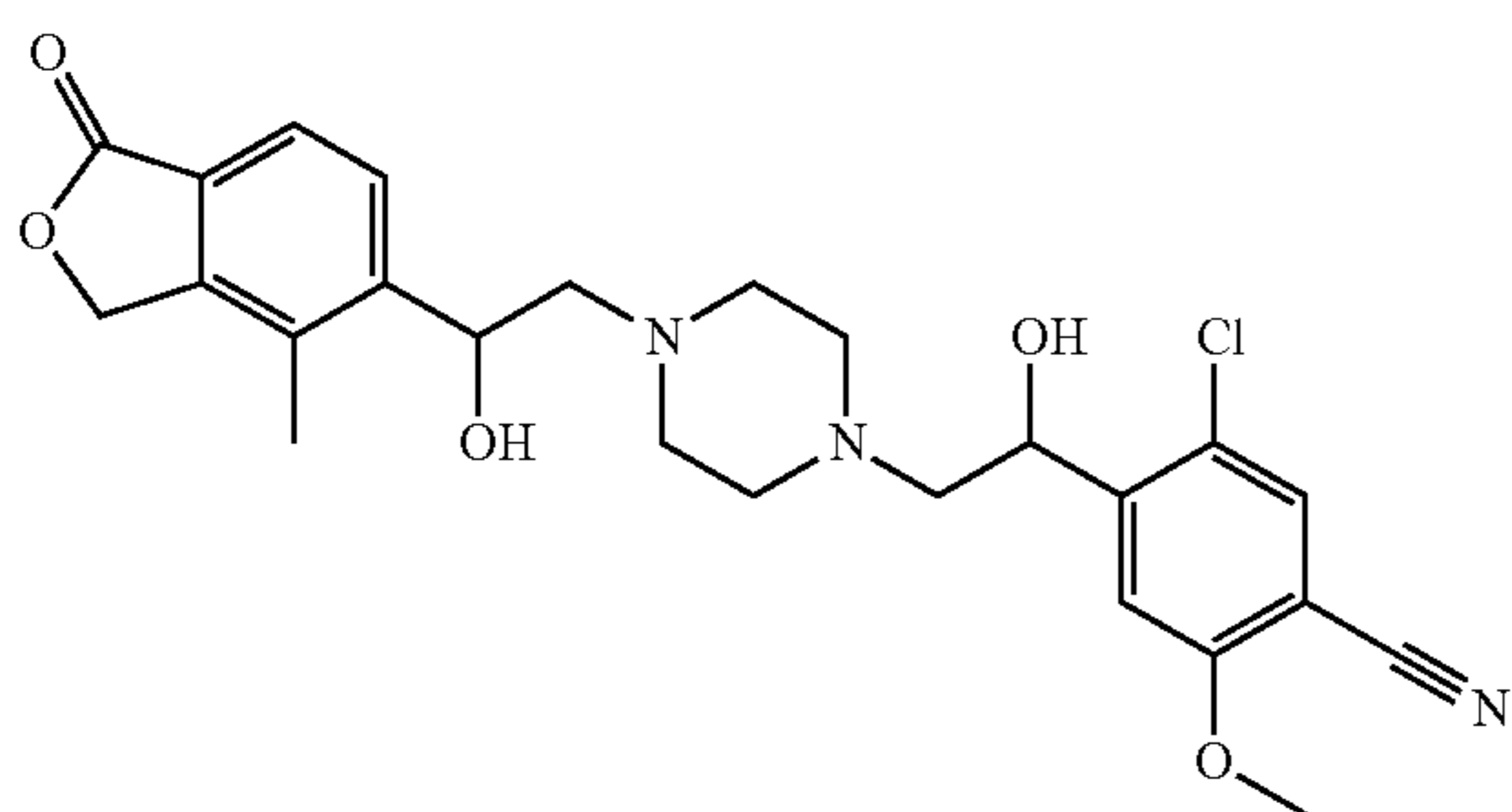
5-chloro-4-(1-hydroxy-2-{4-[2-hydroxy-2-(4-methyl-1-oxo-1,3-dihydro-2-benzofuran-5-yl)ethyl]piperazin-1-yl}ethyl)-2-(methoxy)benzonitrile
