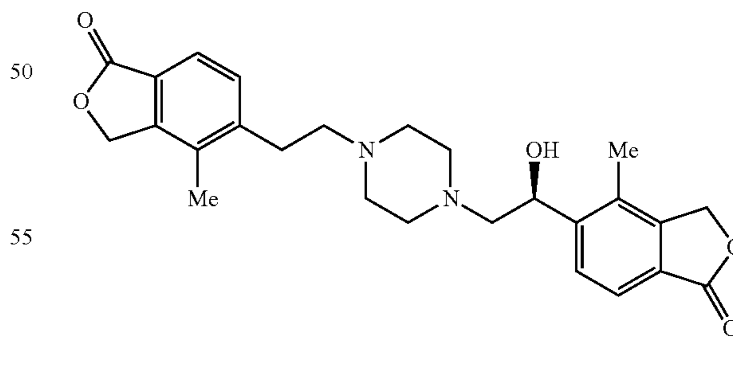
5-((1S)-1-hydroxy-2-{4-[2-(4-methyl-1-oxo-1,3-dihydro-2-benzofuran-5-yl)ethyl]piperazin-1-yl}ethyl)-4-methyl-2-benzofuran-1(3H)-one
