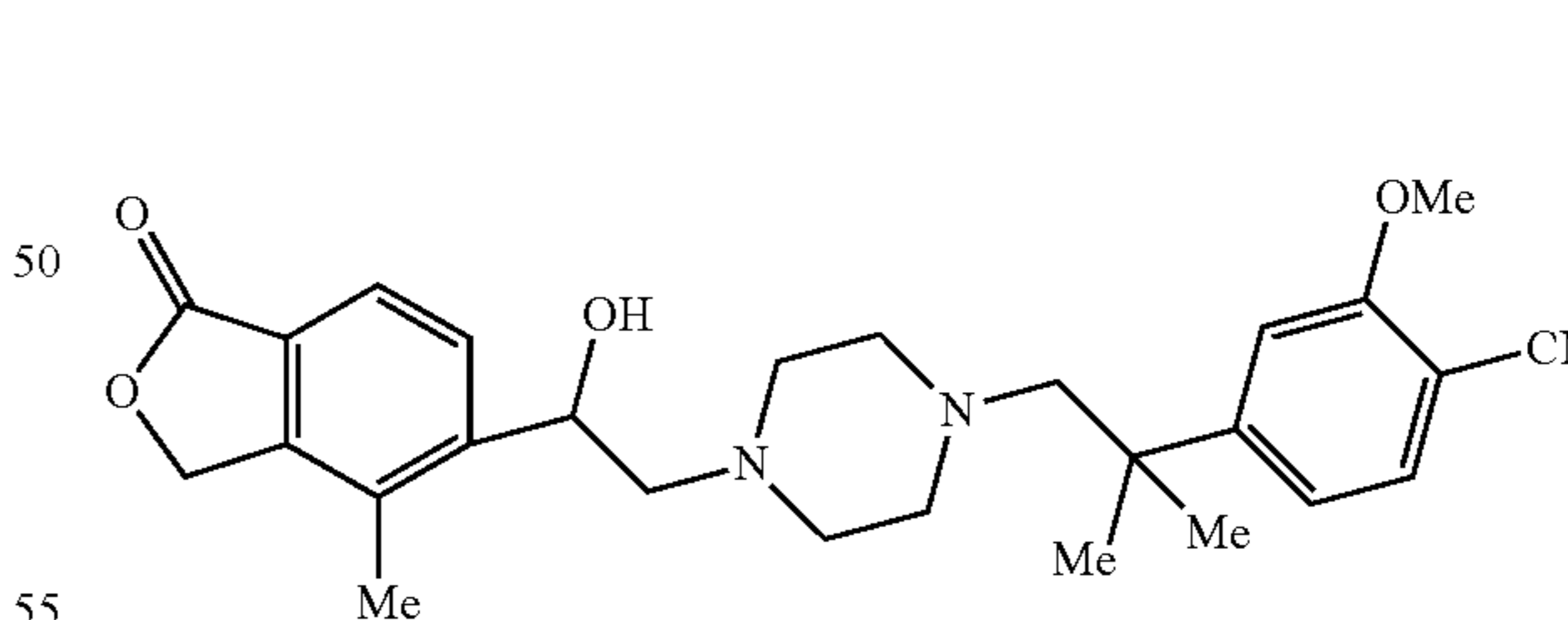
4-2-({4-[2-hydroxy-2-(4-methyl-1-oxo-1,3-dihydro-2-benzofuran-5-yl)ethyl]piperazin-1-yl}-1,1-dimethylethyl)-2-(methoxy)benzonitrile
