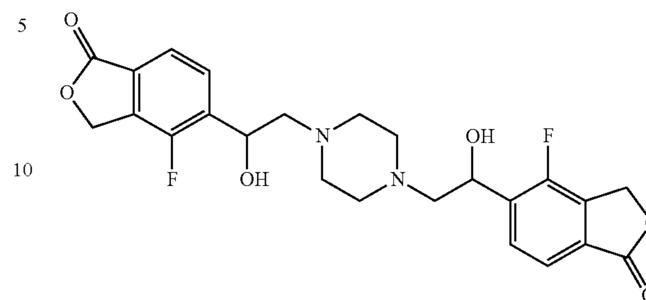
5,5'-[piperazine-1,4-diylbis(1-hydroxyethane-2,1-diyl)]bis(4-fluoro-2-benzofuran-1(3H)-one)
