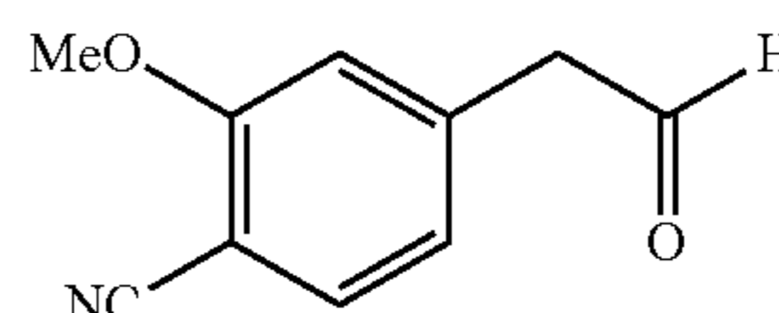
2-(methoxy)-4-(2-oxoethyl)benzonitrile
