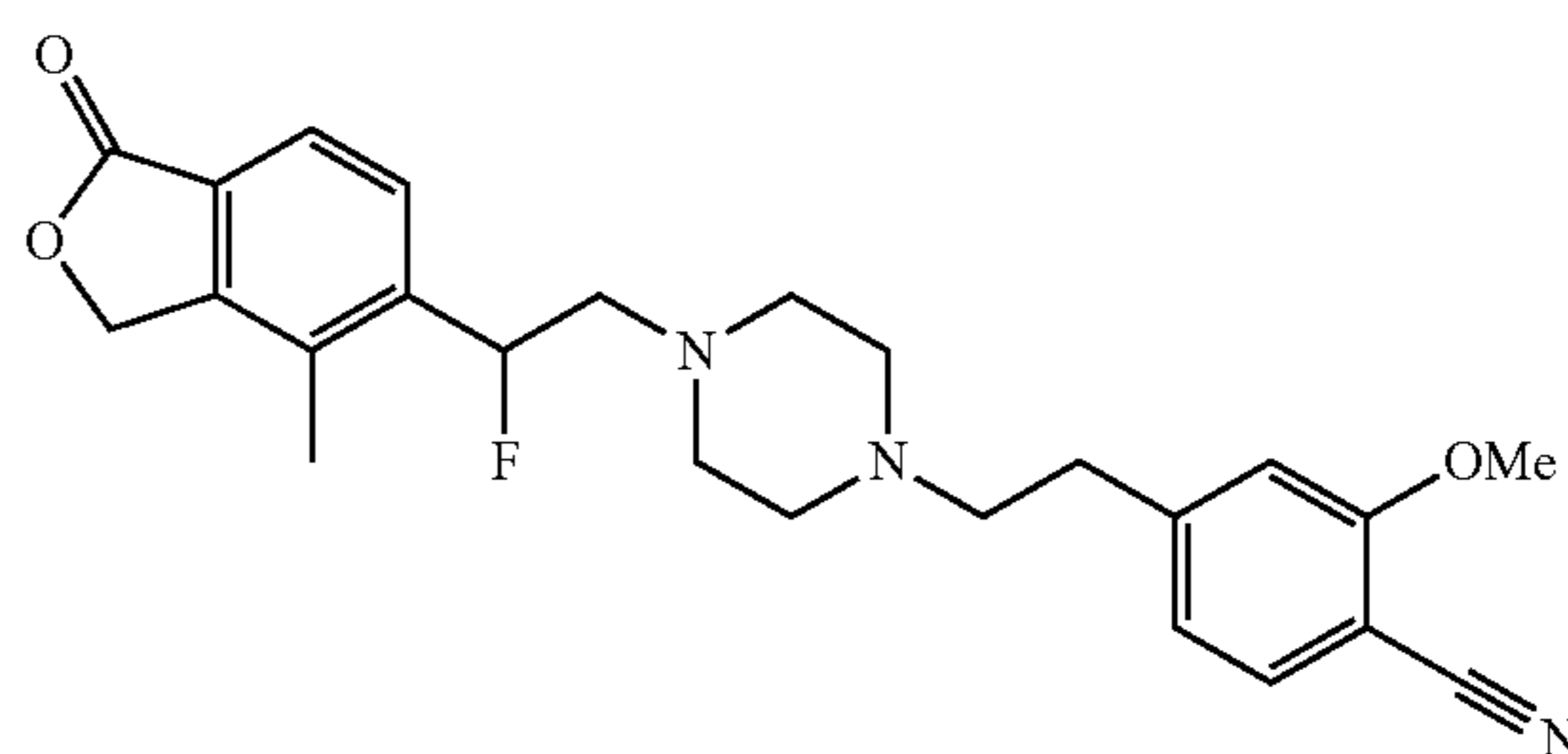
4-(2-{4-[2-fluoro-2-(4-methyl-1-oxo-1,3-dihydro-2-benzofuran-5-yl)ethyl]piperazin-1-yl}ethyl)-2-(methoxy)benzonitrile
