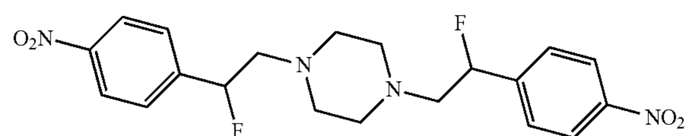
1,4-bis[2-fluoro-2-(4-nitrophenyl)ethyl]piperazine
