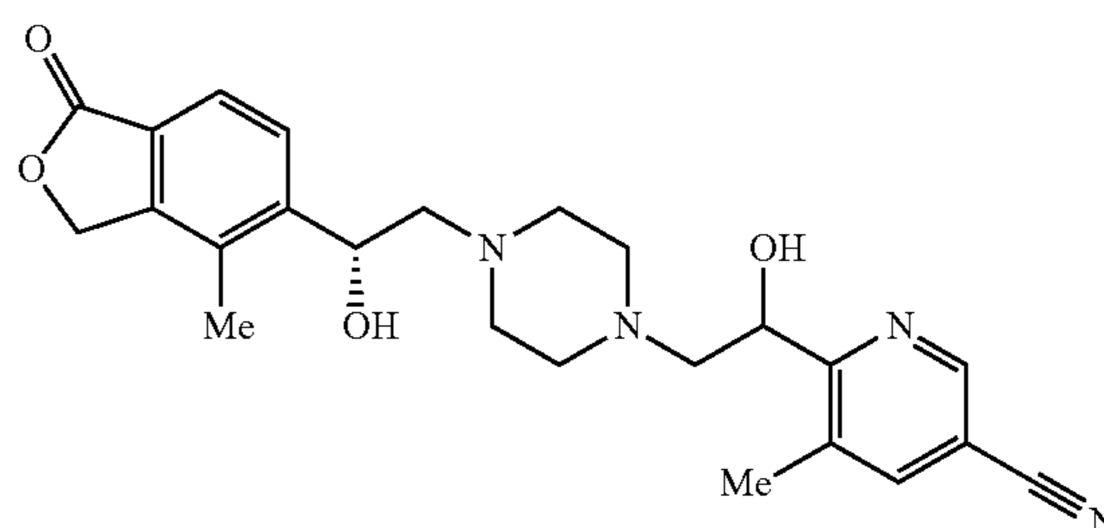
6-(1-Hydroxy-2-{4-[(2R)-2-hydroxy-2-(4-methyl-1-oxo-1,3-dihydro-2-benzofuran-5-yl)ethyl]piperazin-1-yl}ethyl)-5-methylpyridine-3-carbonitrile
