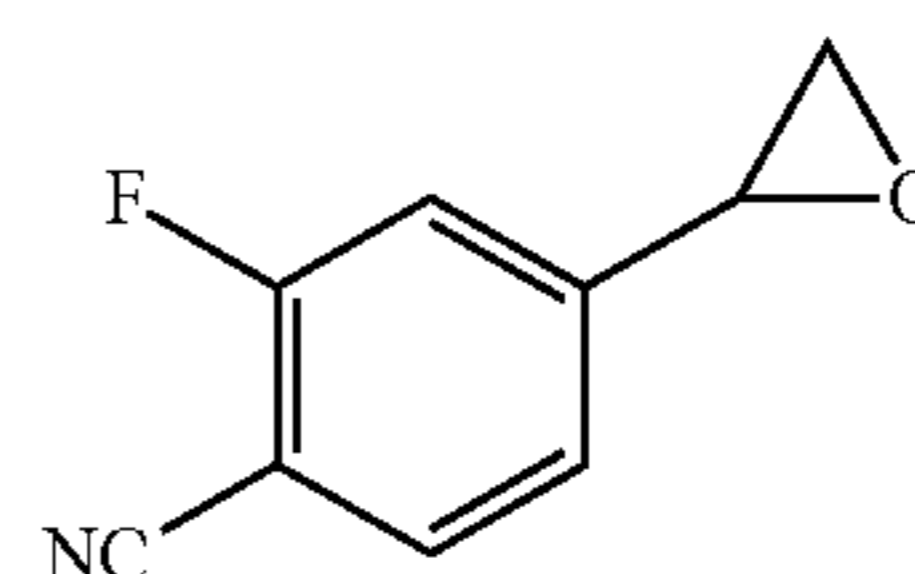
2-fluoro-4-(oxiran-2-yl)benzonitrile
