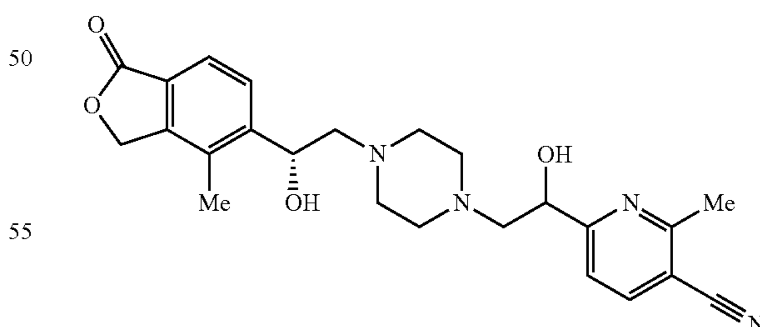
6-[1-Hydroxy-2-[4-[(2R)-2-hydroxy-2-(4-methyl-1-oxo-3H-isobenzofuran-5-yl)ethyl]piperazin-1-yl]ethyl]-2-methylpyridine-3-carbonitrile
