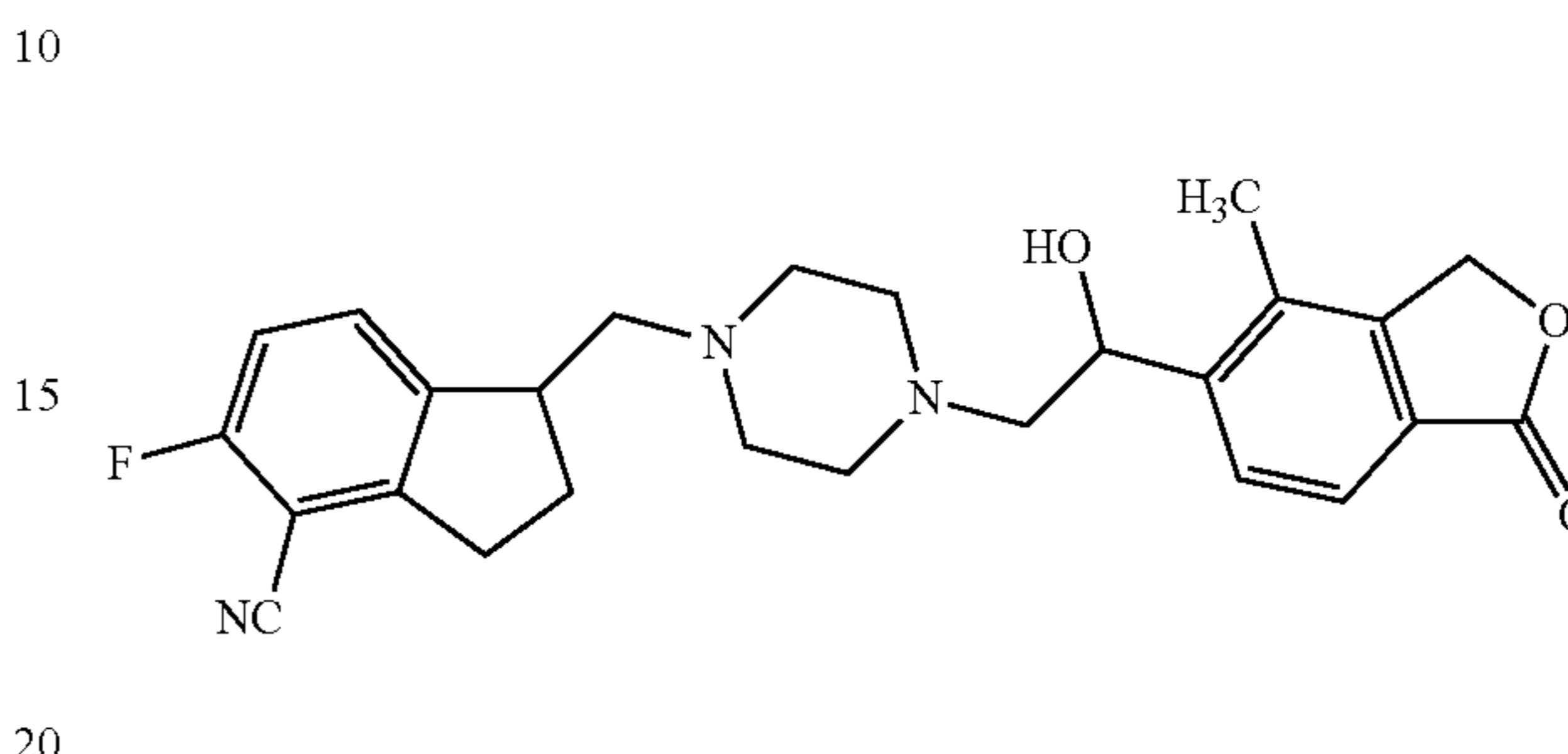
5-fluoro-1-({4-[2-hydroxy-2-(4-methyl-1-oxo-1,3-dihydro-2-benzofuran-5-yl)ethyl]piperazin-1-yl}methyl)-2,3-dihydro-1H-indene-4-carbonitrile
