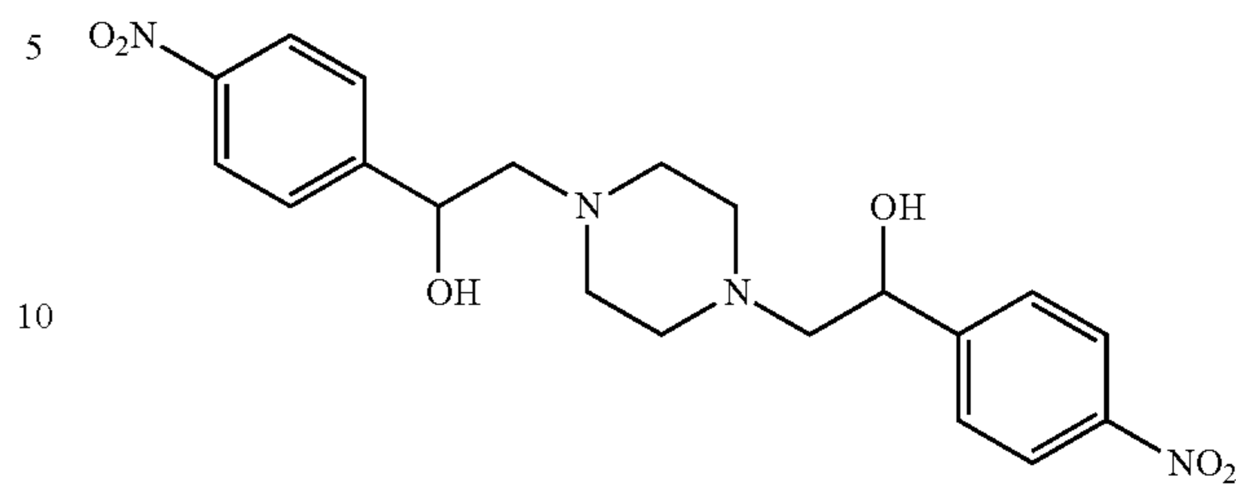
2,2'-piperazine-1,4-diylbis[1-(4-nitrophenyl)ethanol]
