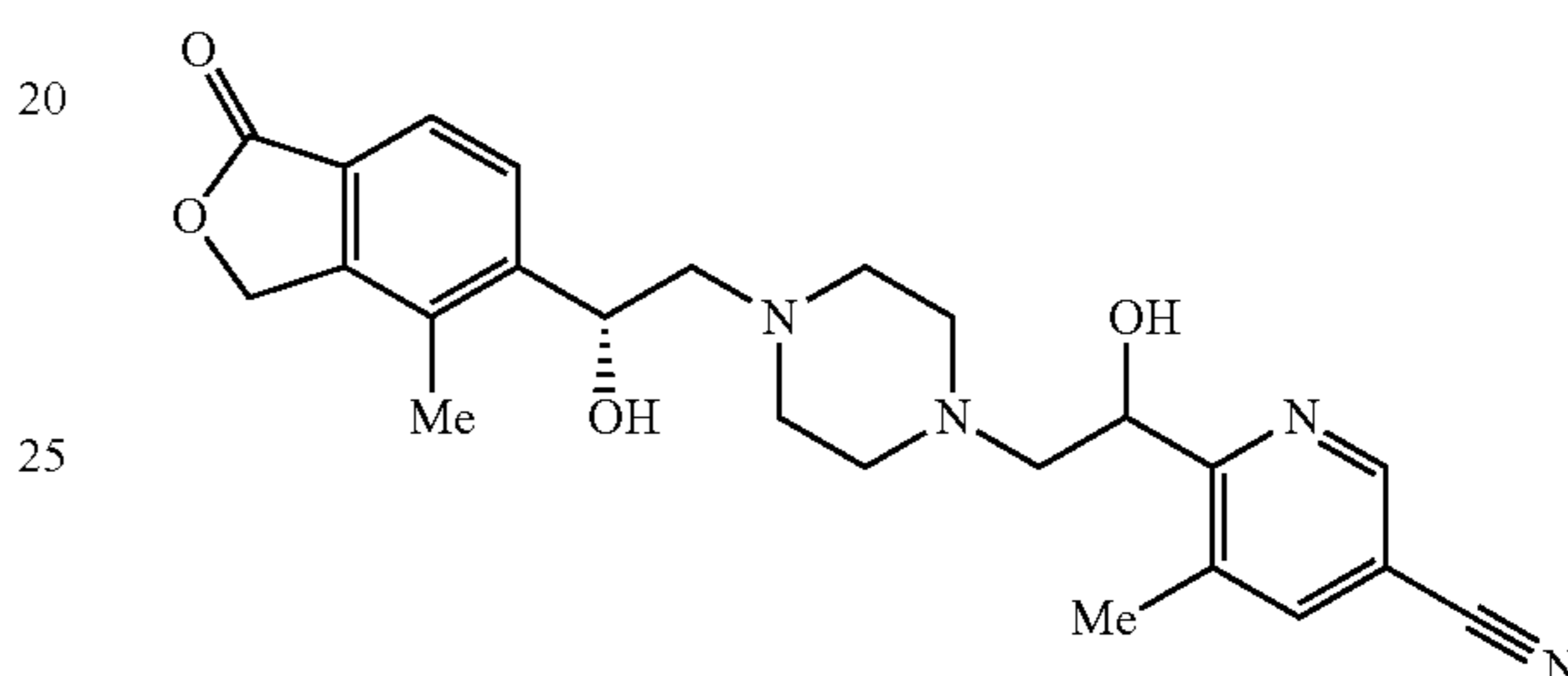
6-(1-Hydroxy-2-{4-[(2R)-2-hydroxy-2-(4-methyl-1-oxo-1,3-dihydro-2-benzofuran-5-yl)ethyl]piperazin-1-yl}ethyl)-5-methylpyridine-3-carbonitrile
