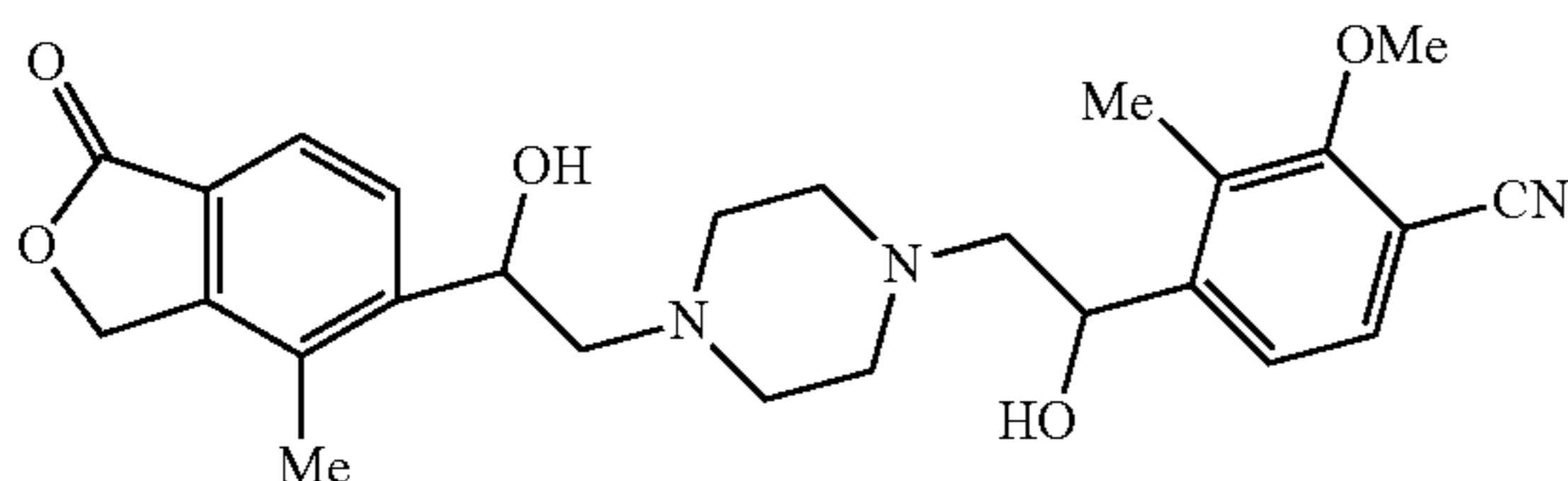
4-(1-hydroxy-2-{4-[2-hydroxy-2-(4-methyl-1-oxo-1,3-dihydro-2-benzofuran-5-yl)ethyl]piperazin-1-yl}ethyl)-3-methyl-2-(methoxy)benzonitrile
