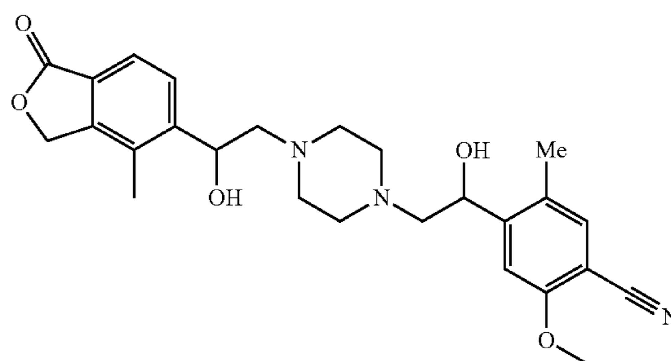
4-(1-hydroxy-2-{4-[2-hydroxy-2-(4-methyl-1-oxo-1,3-dihydro-2-benzofuran-5-yl)ethyl]piperazin-1-yl}ethyl)-5-methyl-2-(methoxy)benzonitrile
