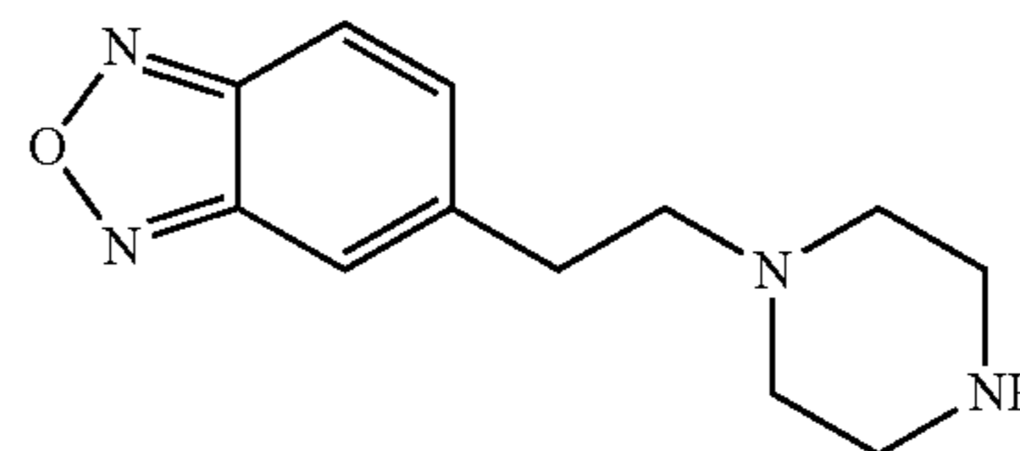
5-[2-(piperazin-1-yl)ethyl]-2,1,3-benzoxadiazole
