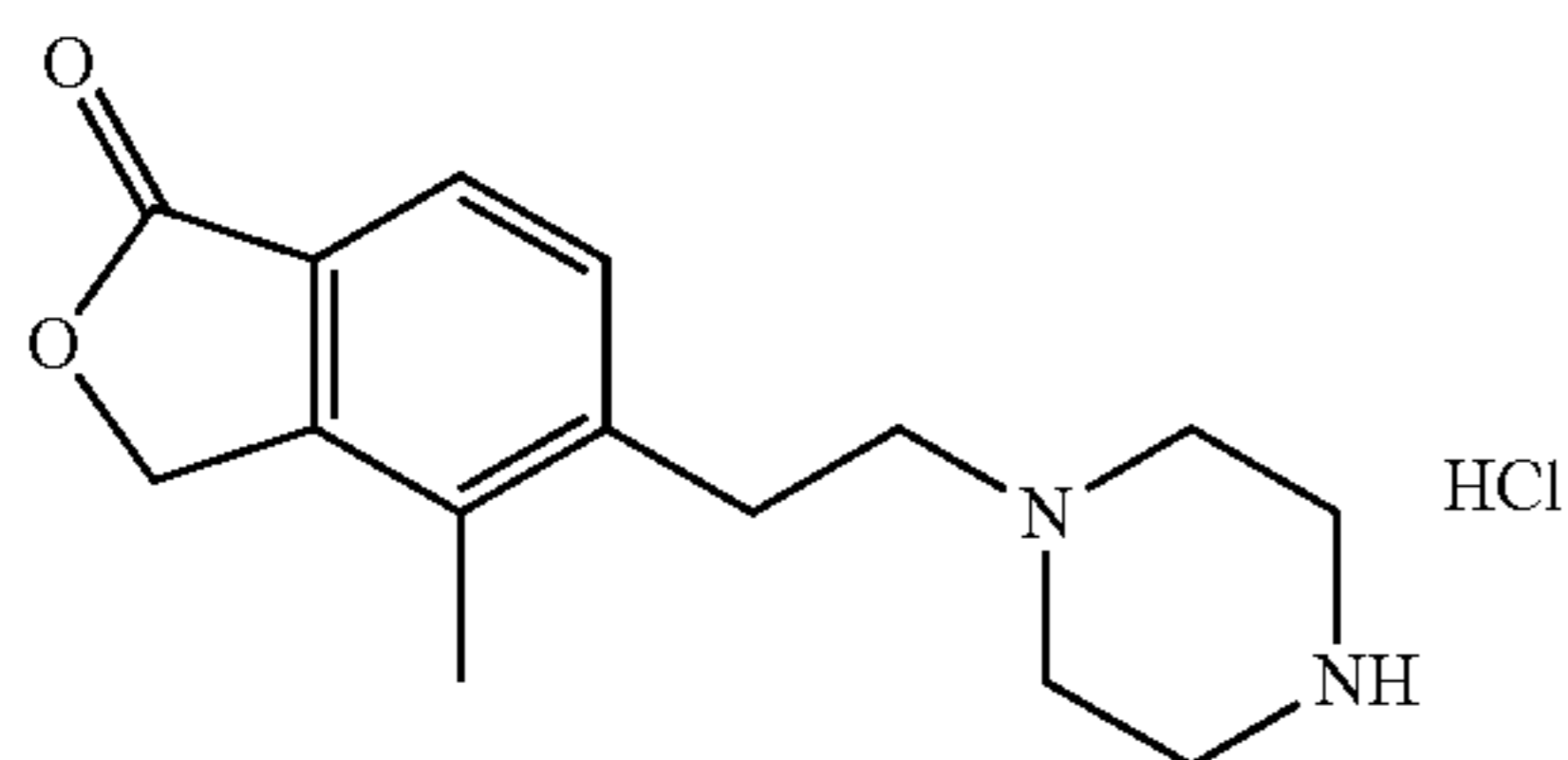
4-methyl-5-(2-piperazin-1-ylethyl)-2-benzofuran-1(3H)-one hydrochloride
