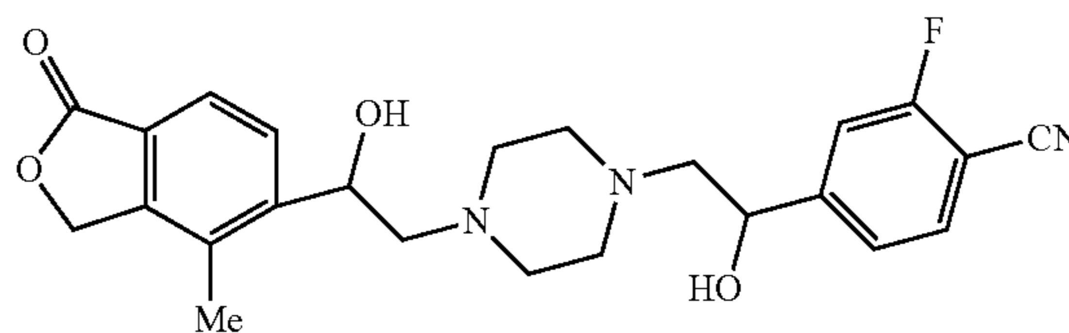
2-fluoro-4-(1-hydroxy-2-{4-[2-hydroxy-2-(4-methyl-1-oxo-1,3-dihydro-2-benzofuran-5-yl)ethyl]piperazin-1-yl}ethyl)benzonitrile
