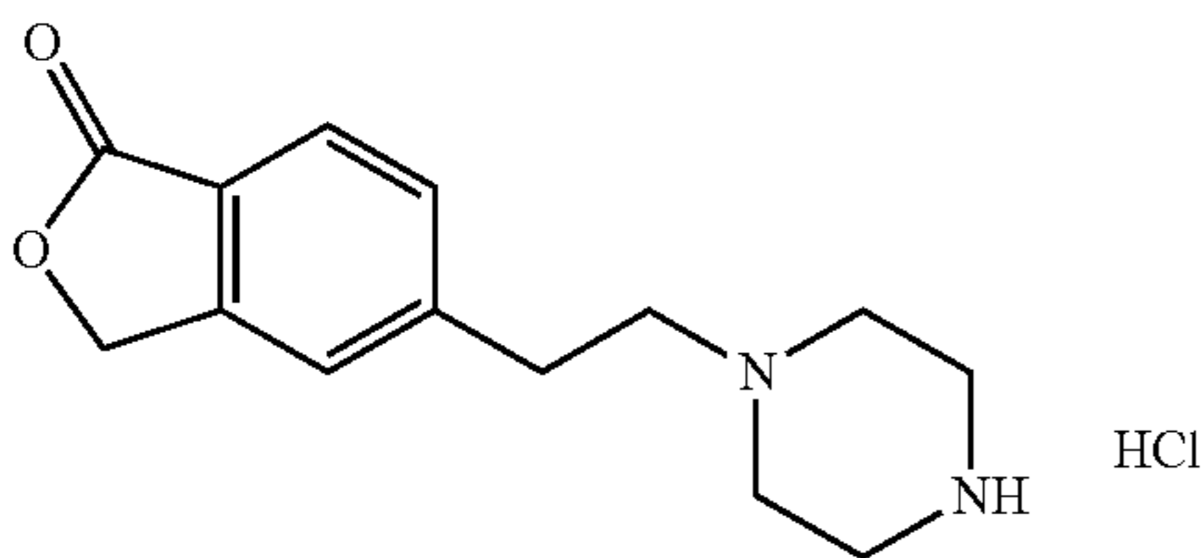
5-(2-piperazin-1-ylethyl)-2-benzofuran-1(3H)-one hydrochloride
