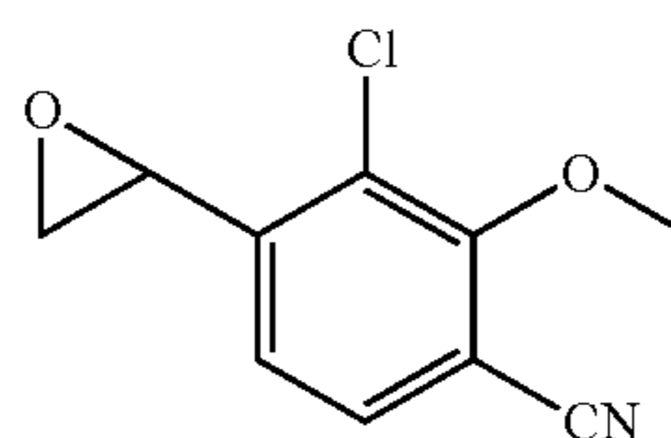
(2-Chloro-4-cyano-3-methoxyphenyl)ethylene oxide
