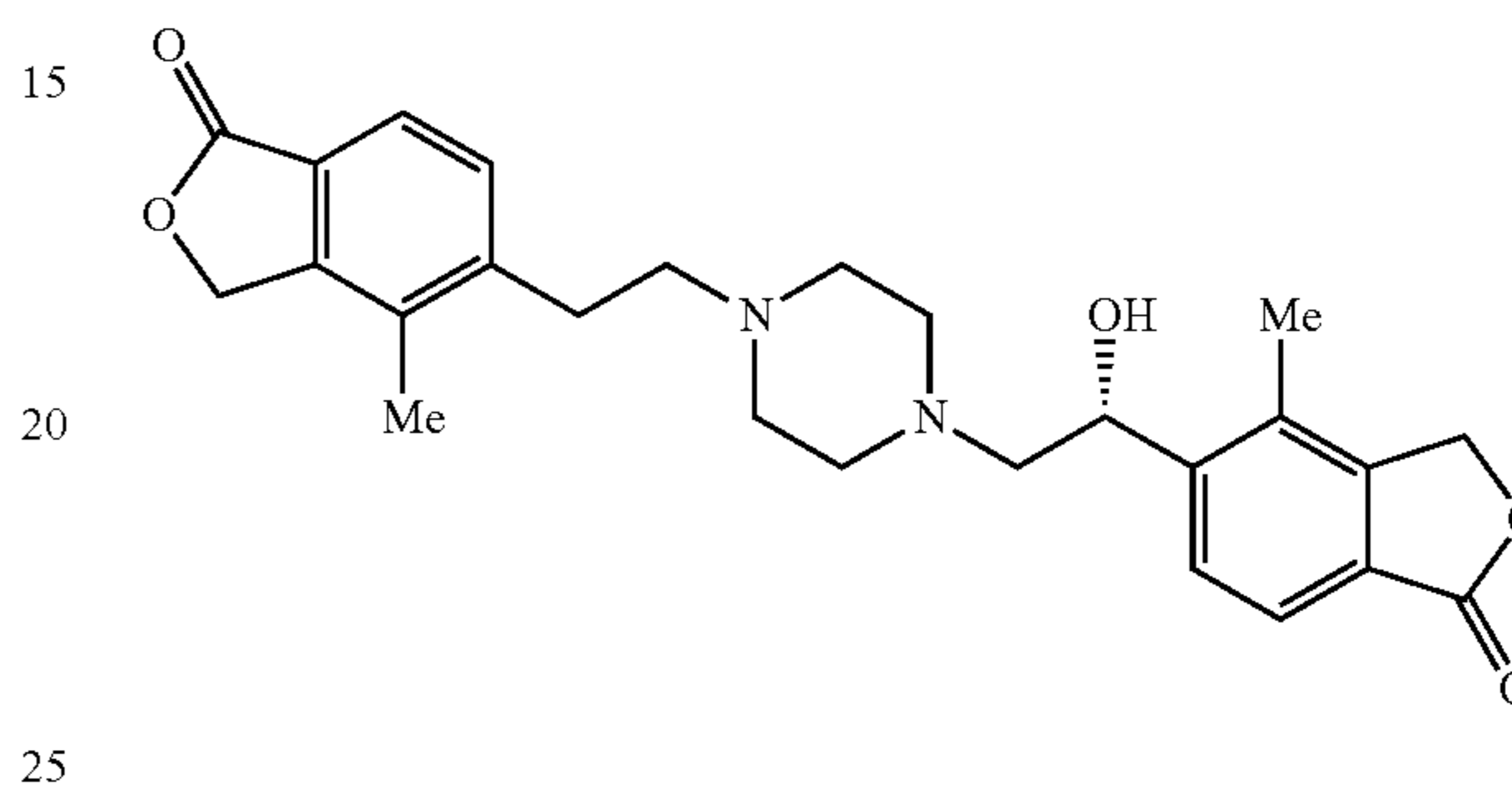
5-((1R)-1-hydroxy-2-{4-[2-(4-methyl-1-oxo-1,3-dihydro-2-benzofuran-5-yl)ethyl]piperazin-1-yl}ethyl)-4-methyl-2-benzofuran-1(3H)-one
