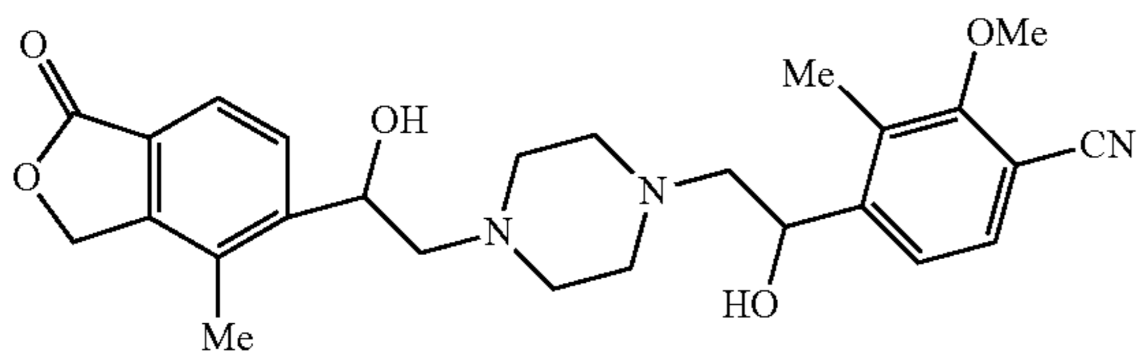
4-(1-hydroxy-2-{4-[2-hydroxy-2-(4-methyl-1-oxo-1,3-dihydro-2-benzofuran-5-yl)ethyl]piperazin-1-yl}ethyl)-3-methyl-2-(methoxy)benzonitrile
