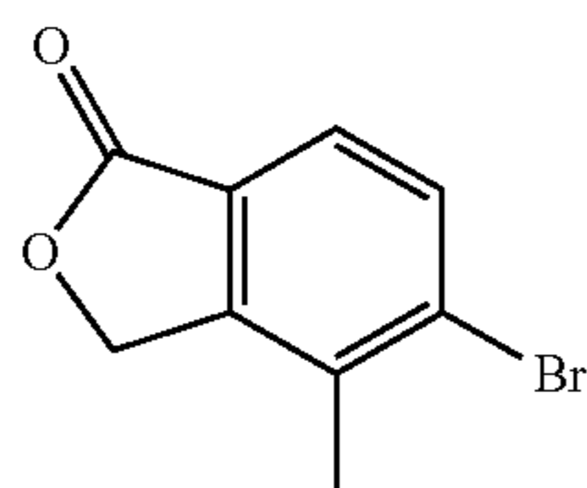
5-bromo-4-methyl-2-benzofuran-1(3H)-one
