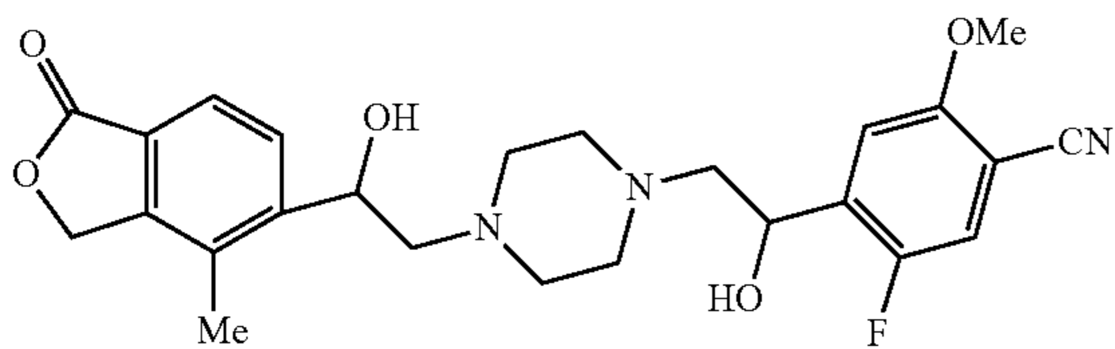
5-fluoro-4-(1-hydroxy-2-{4-[2-hydroxy-2-(4-methyl-1-oxo-1,3-dihydro-2-benzofuran-5-yl)ethyl]piperazin-1-yl}ethyl)-2-(methoxy)benzonitrile
