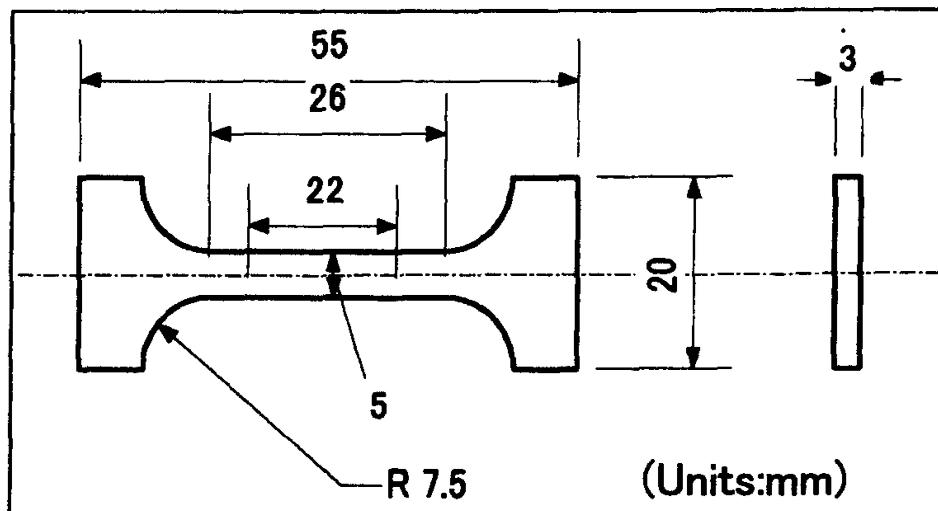
Configuration, Tensile Test Piece
