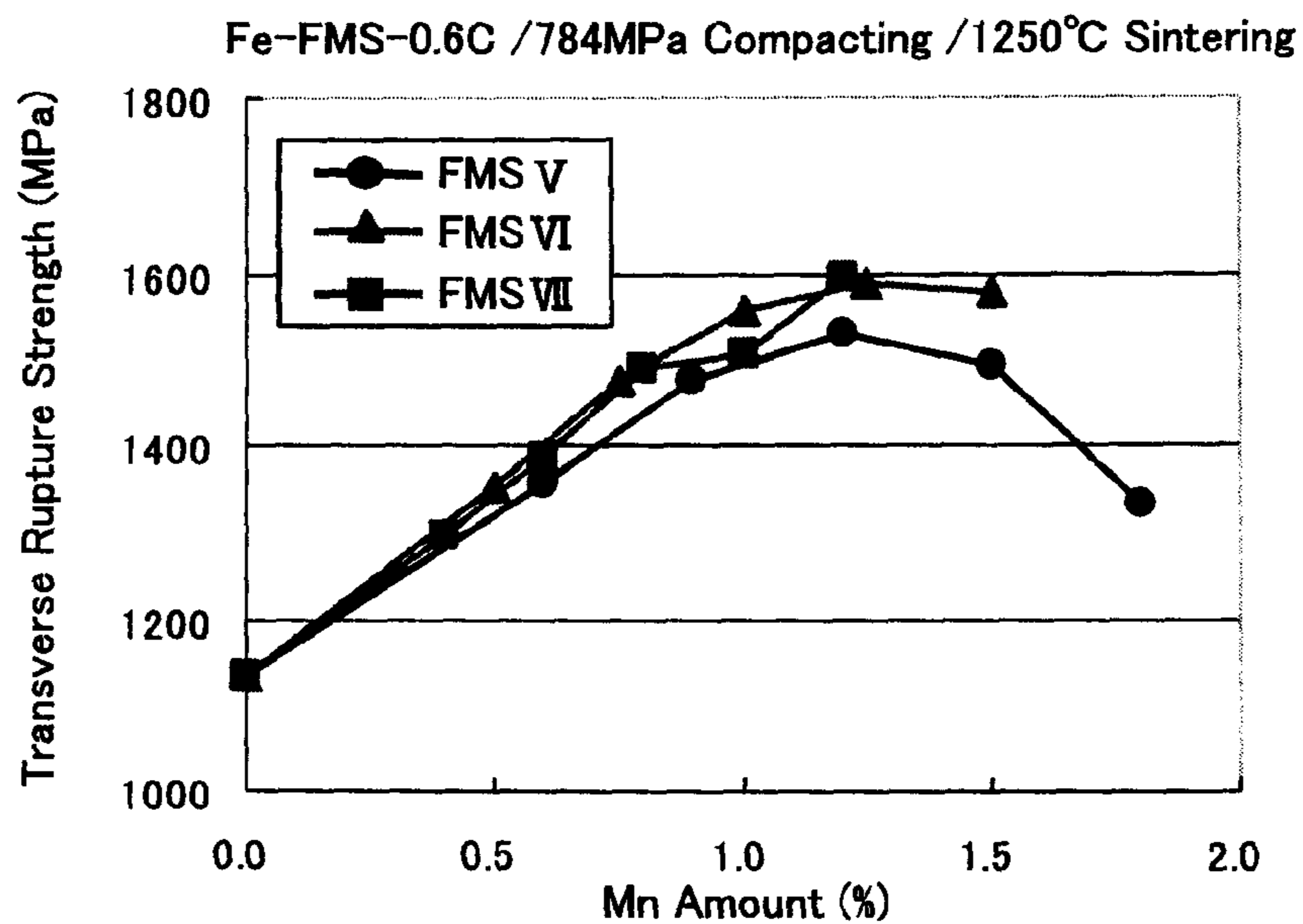
Influence of Mn Amount Exerted to Transverse Rupture Strength of 1250°C-Sintered Body
