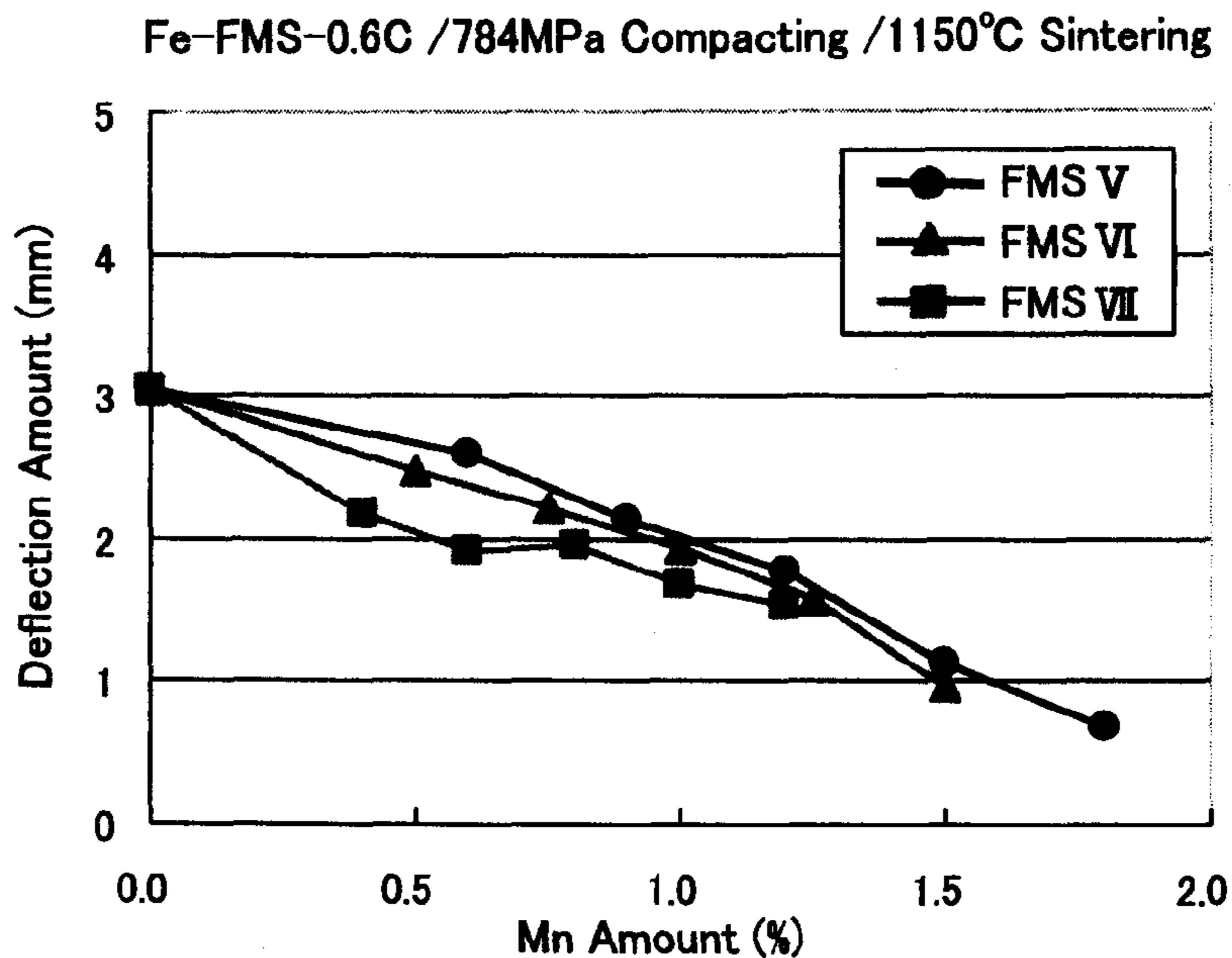
Influence of Mn Amount Exerted to Deflection Amount in Transverse Test to 1150°C-Sintered Body
