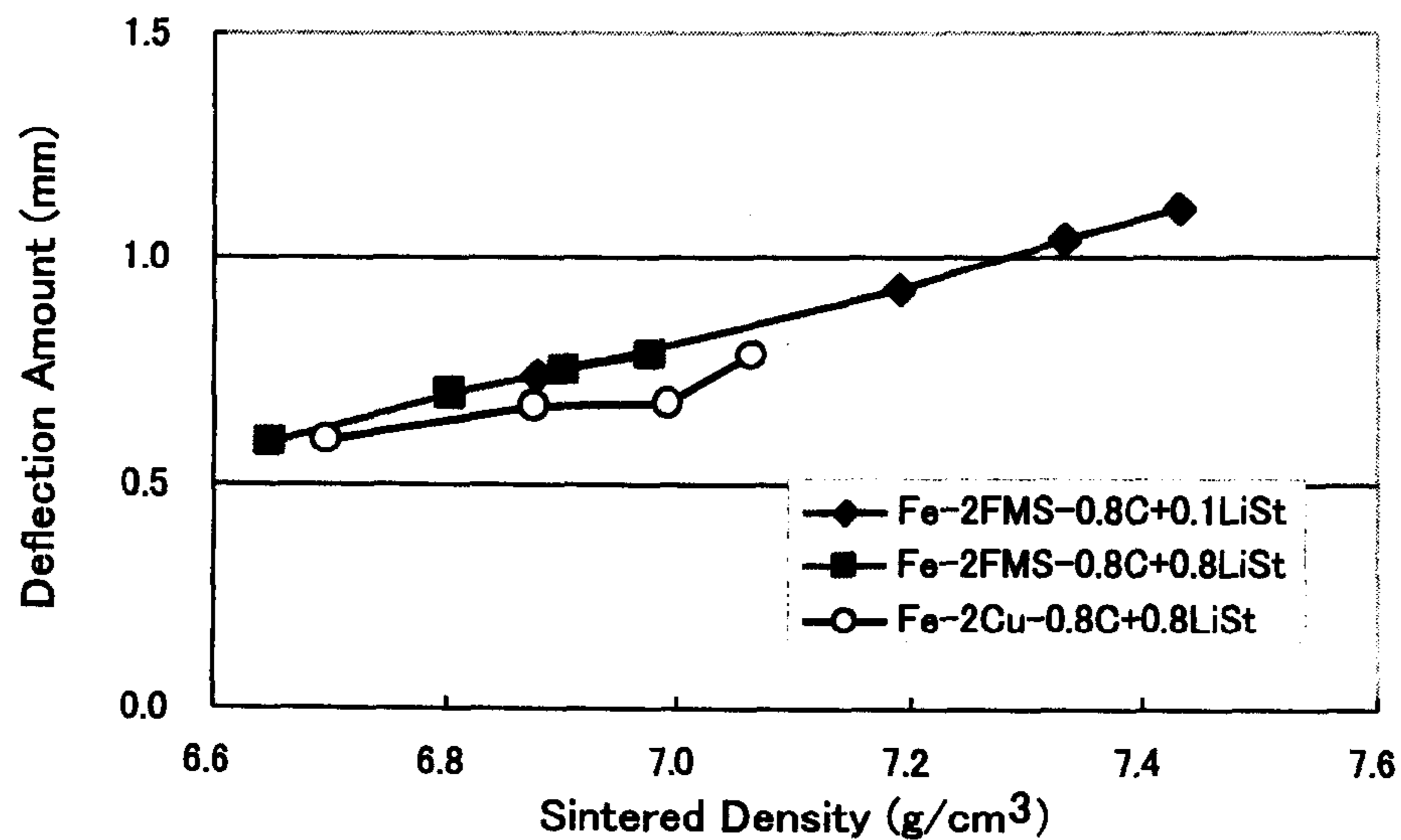
Relationship between Sintered Density and Deflection Amount
