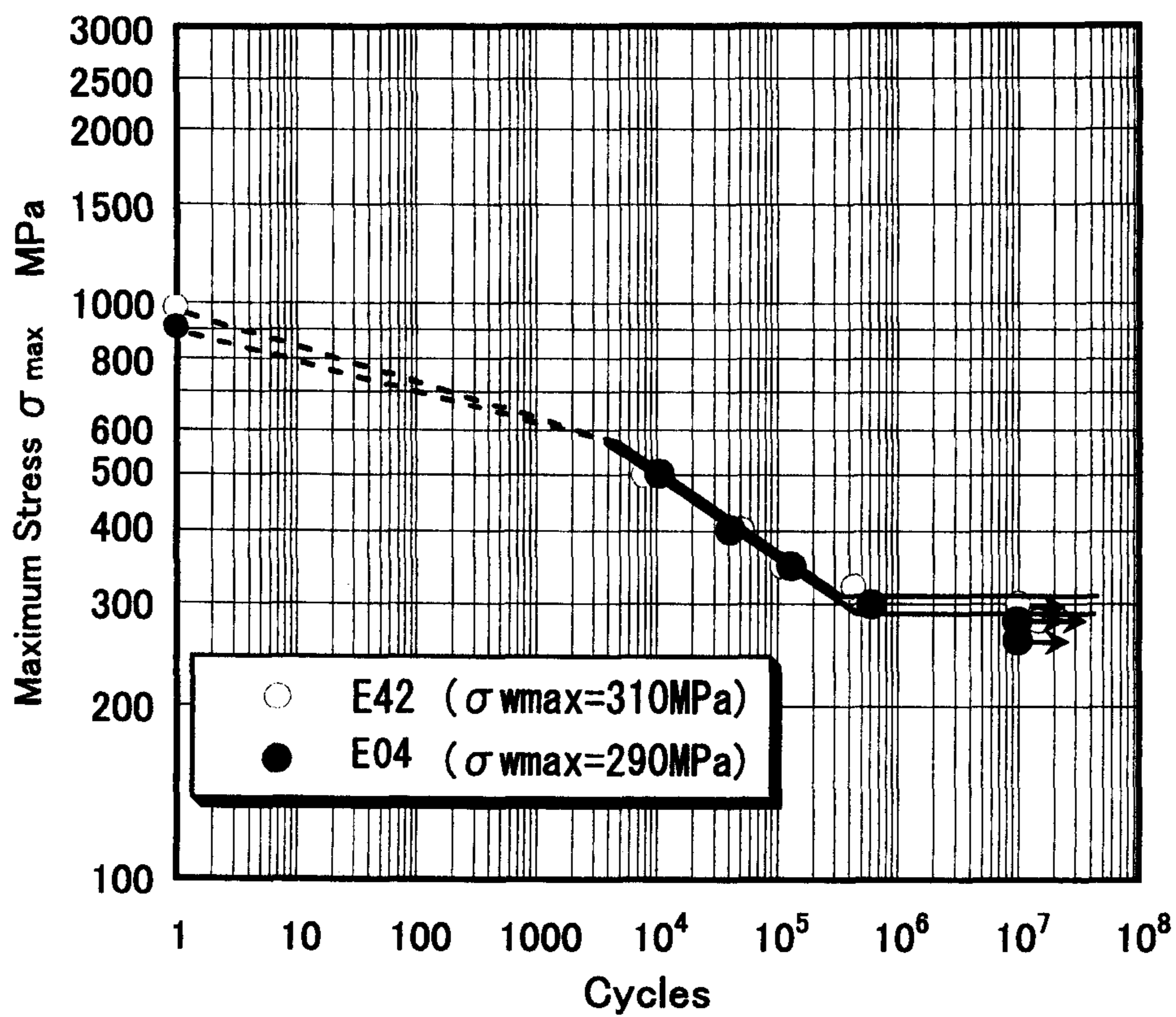
Three-point Bending Fatigue Test Result
