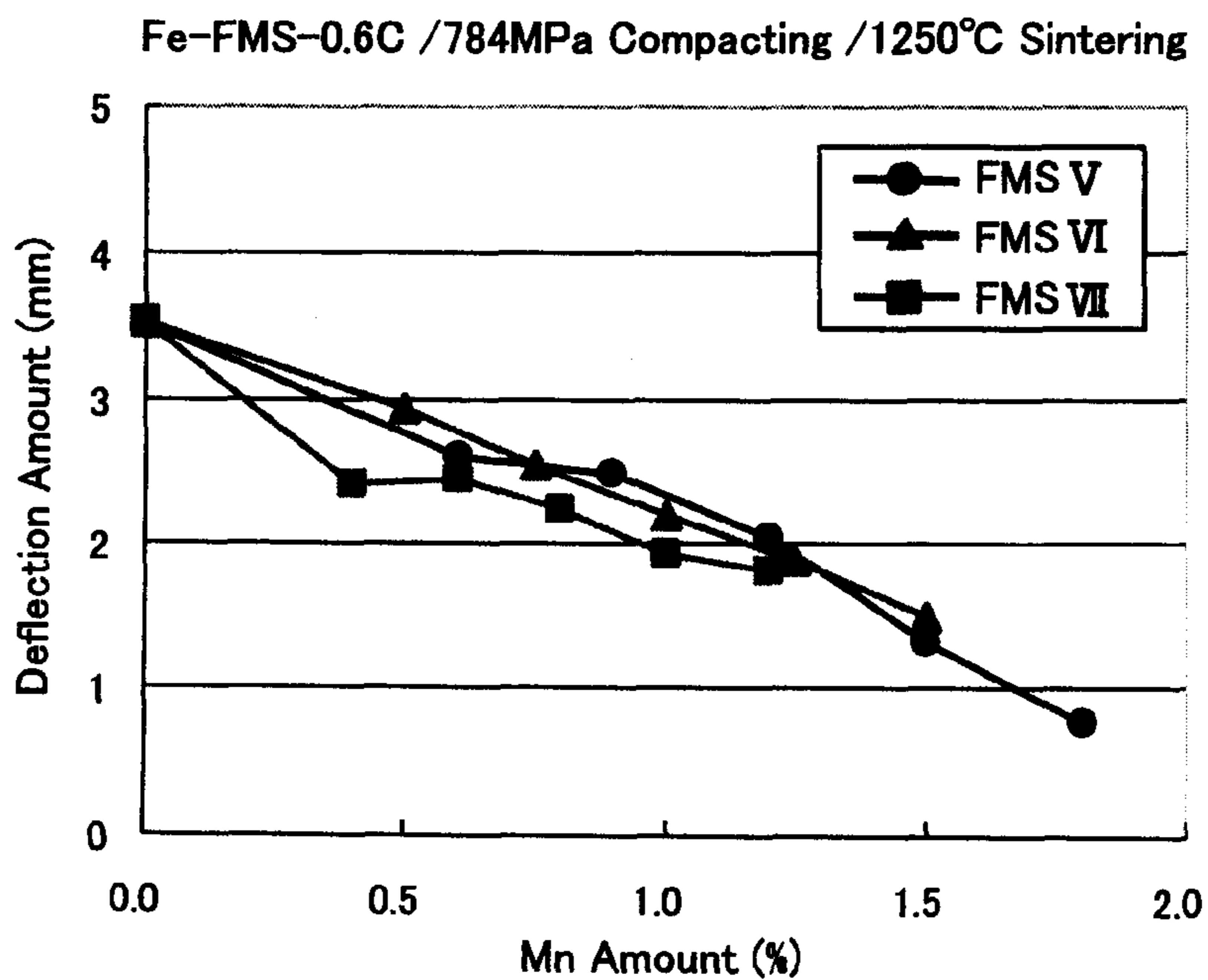
Influence of Mn Amount Exerted to Deflection Amount in Transverse Test to 1250°C-Sintered Body
