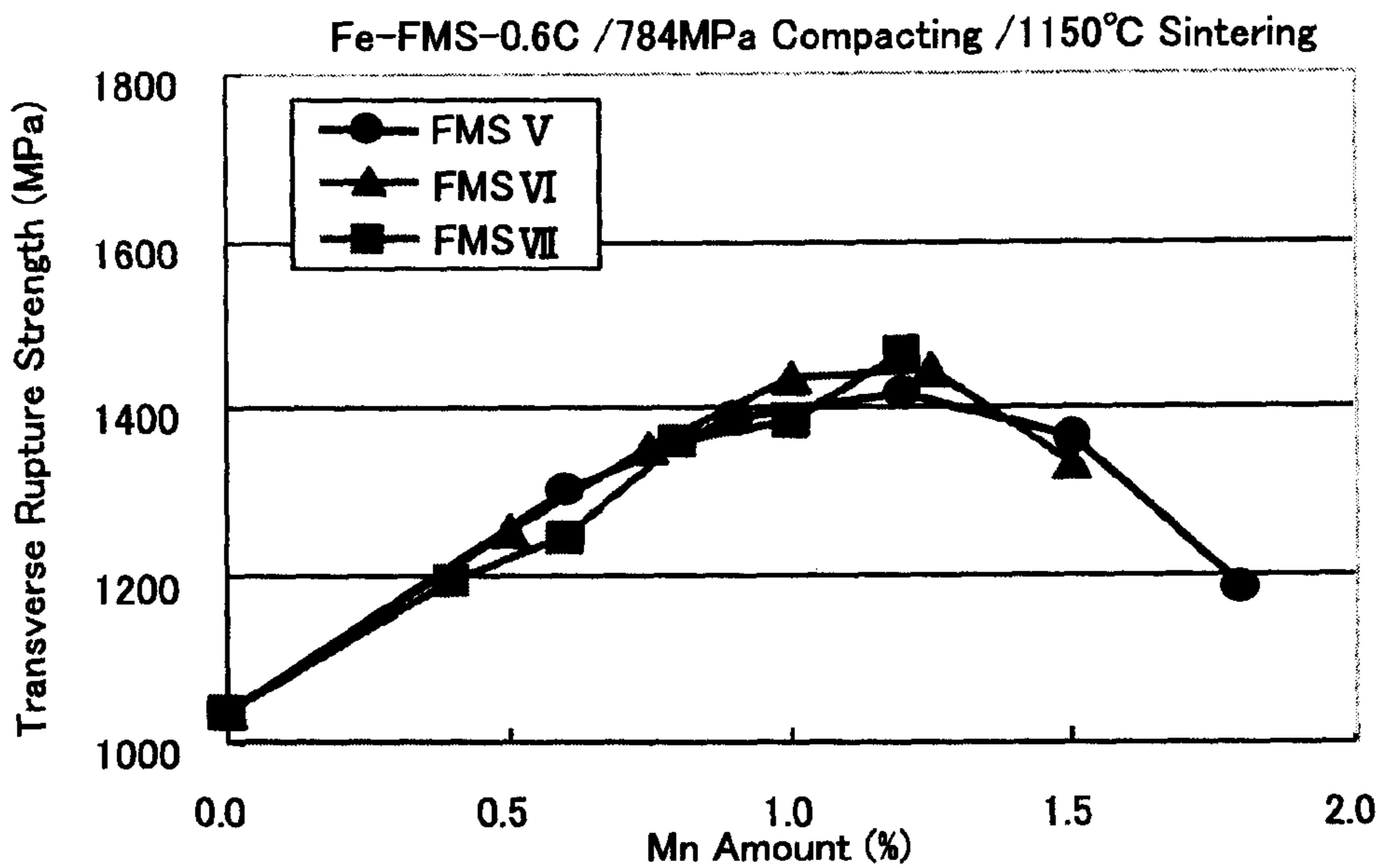
Influence of Mn Amount Exerted to Transverse Rupture Strength of 1150°C-Sintered Body
