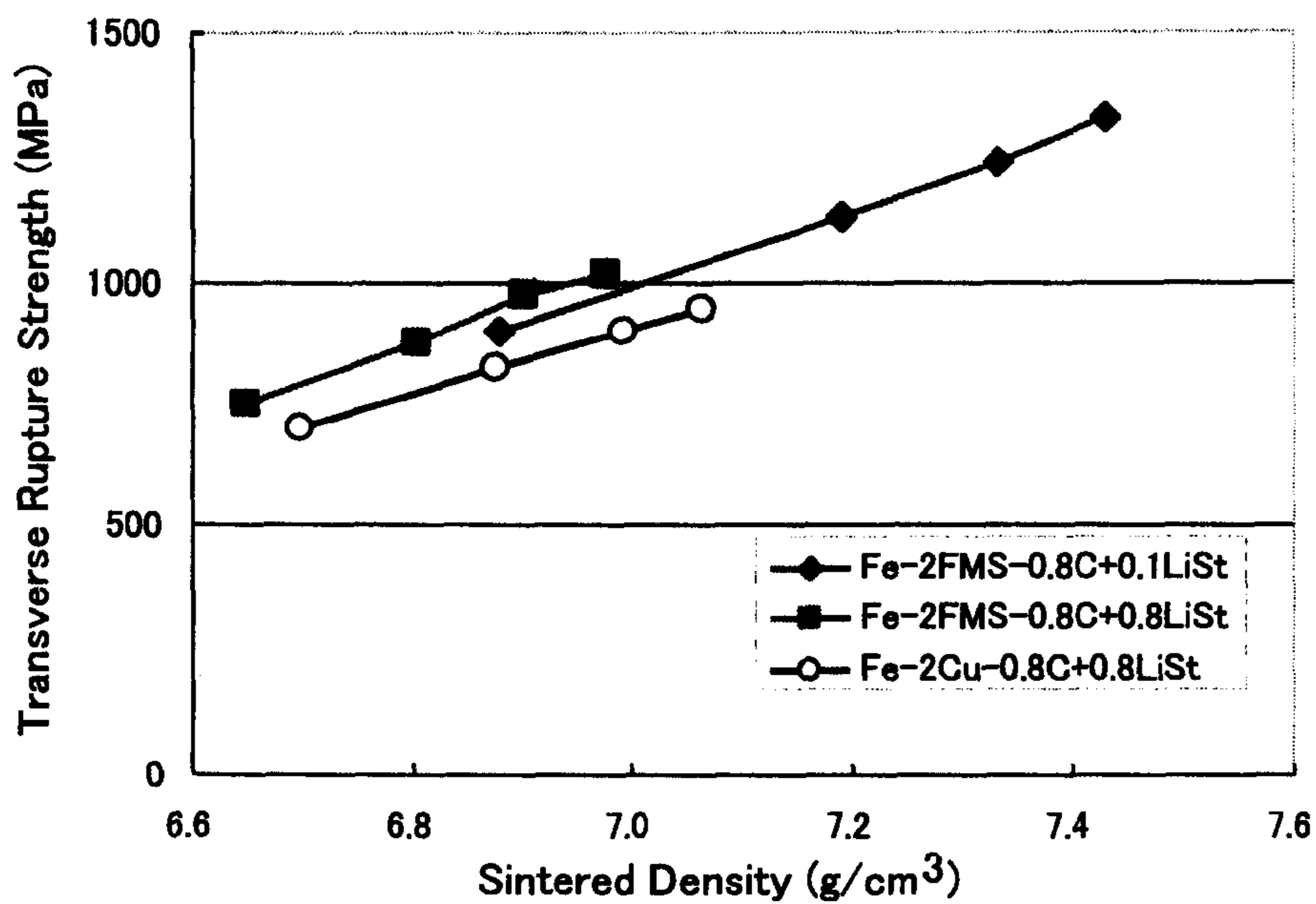
Relationship between Sintered Density and Traverse Rupture Strength
