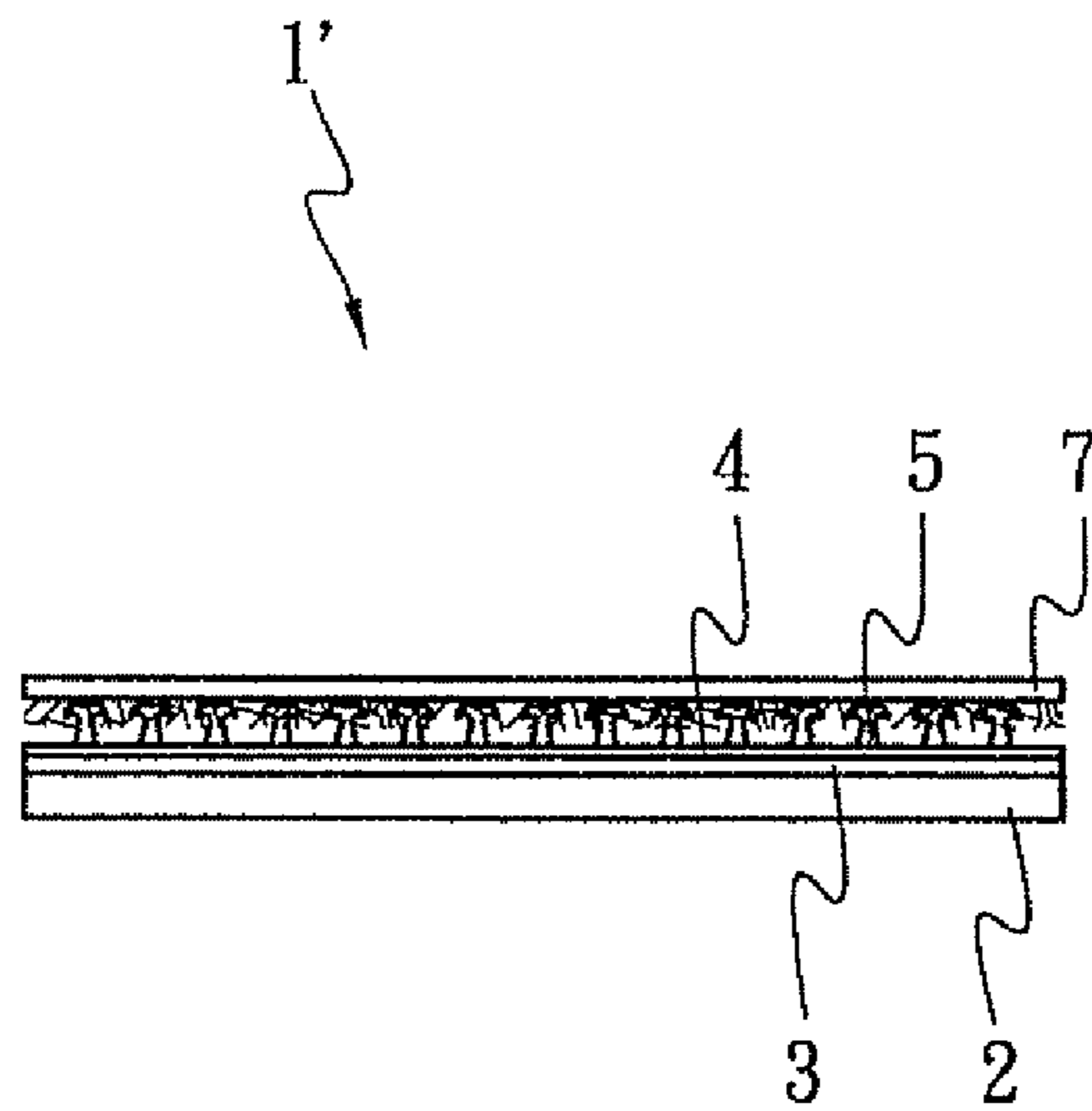
Fig. 2 (PRIOR ART)
