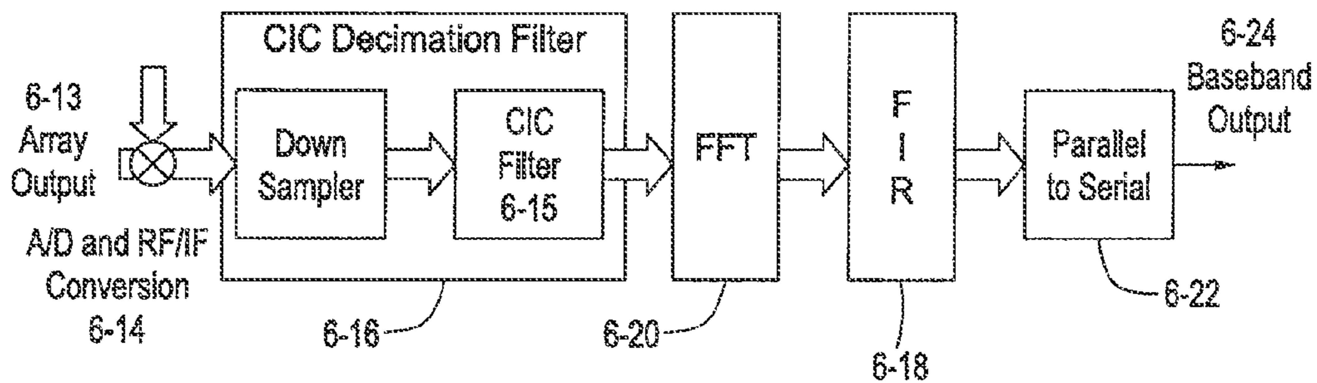
RX Configuration
