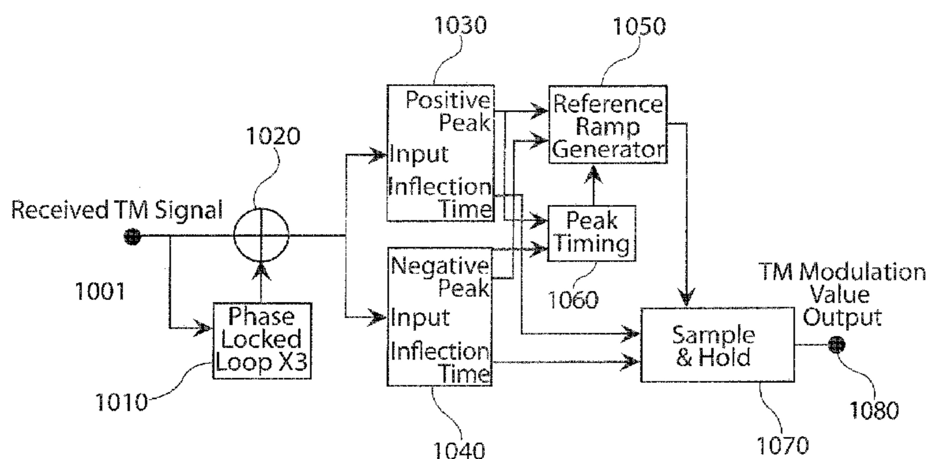
The Sub-Cycle Calibration method of TM demodulation.
