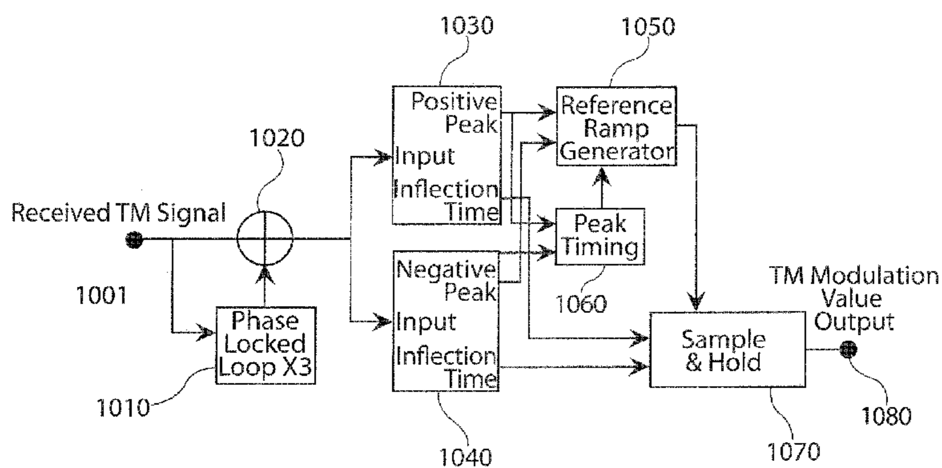
The Sub-Cycle Calibration method of TM demodulation.
