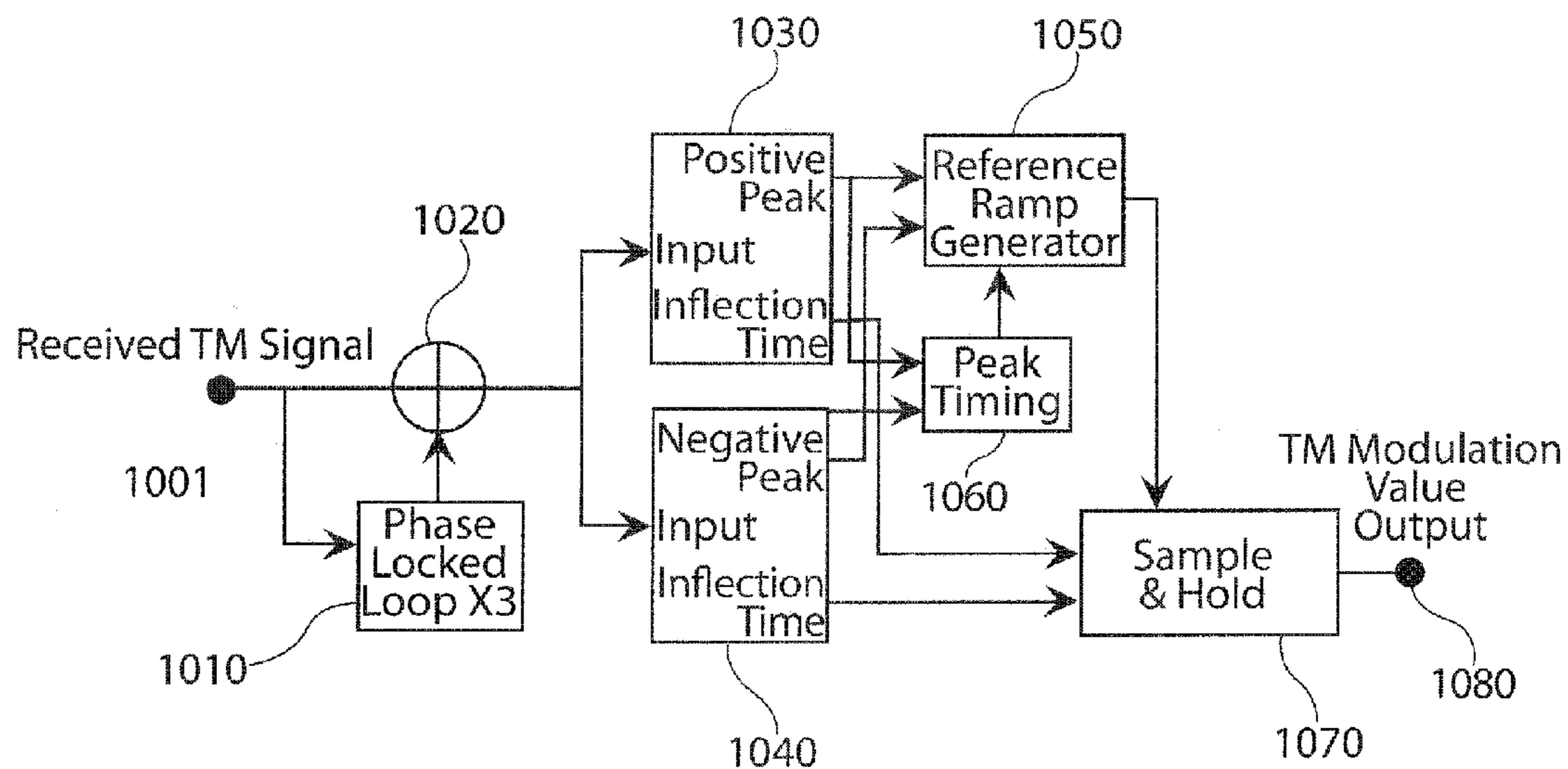
The Sub-Cycle Calibration method of TM demodulation.
