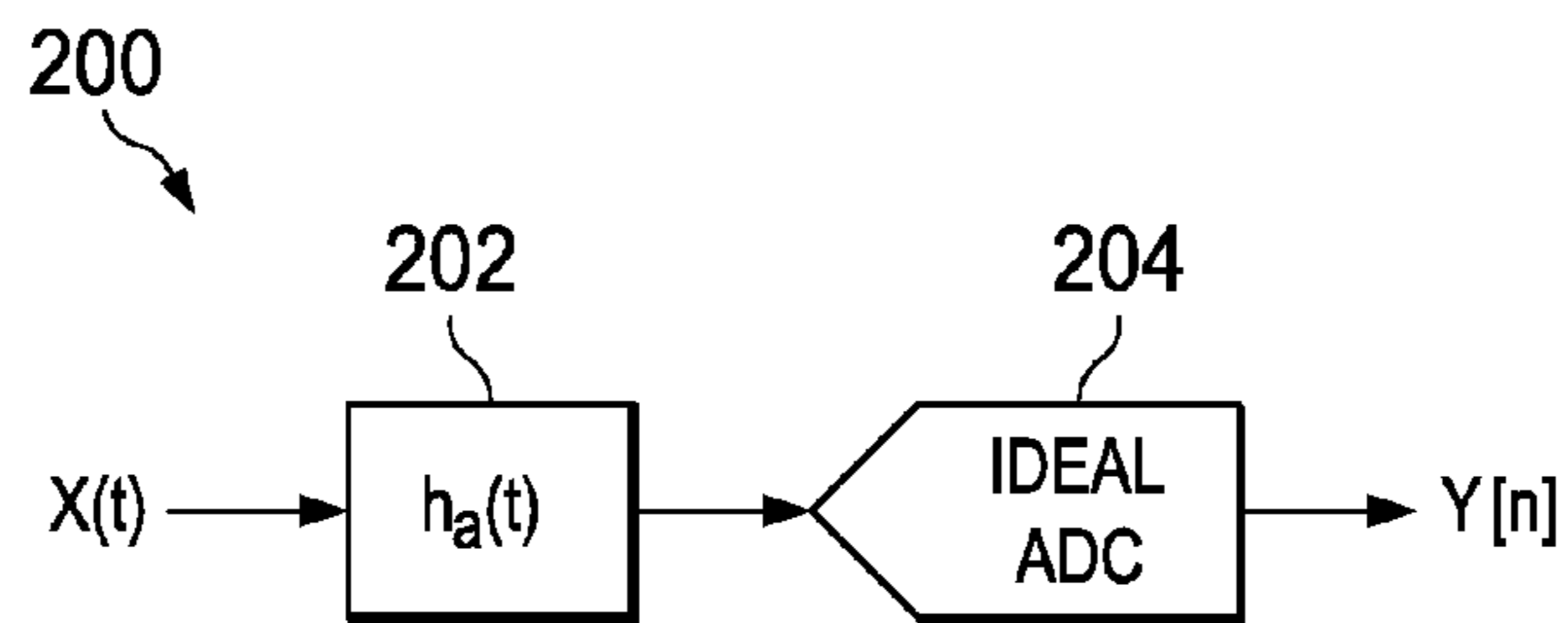
FIG. 2 (PRIOR ART)
