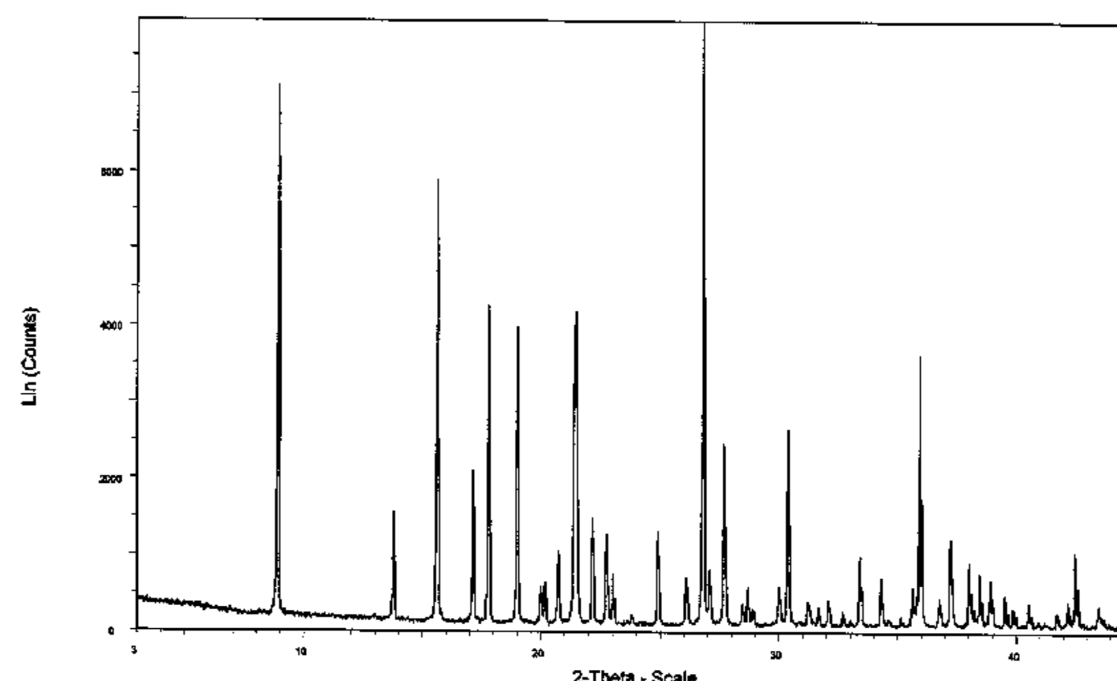
PXRD pattern of potassium 2,5-dihydroxybenzenesulfonic acid (Example 6)
