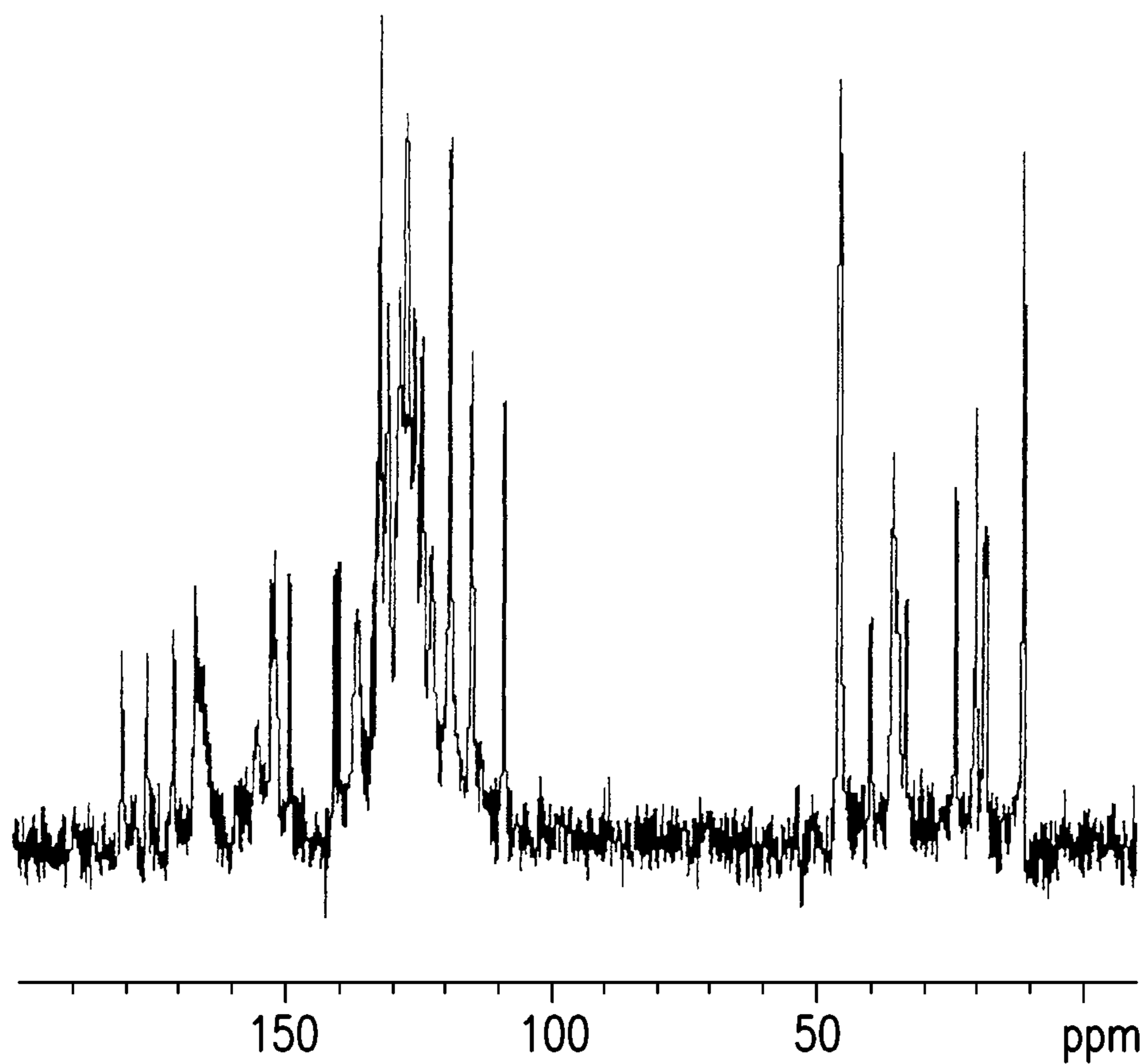
13C solid state NMR of free acid hydrate polymorphic Form I of Compound A.
