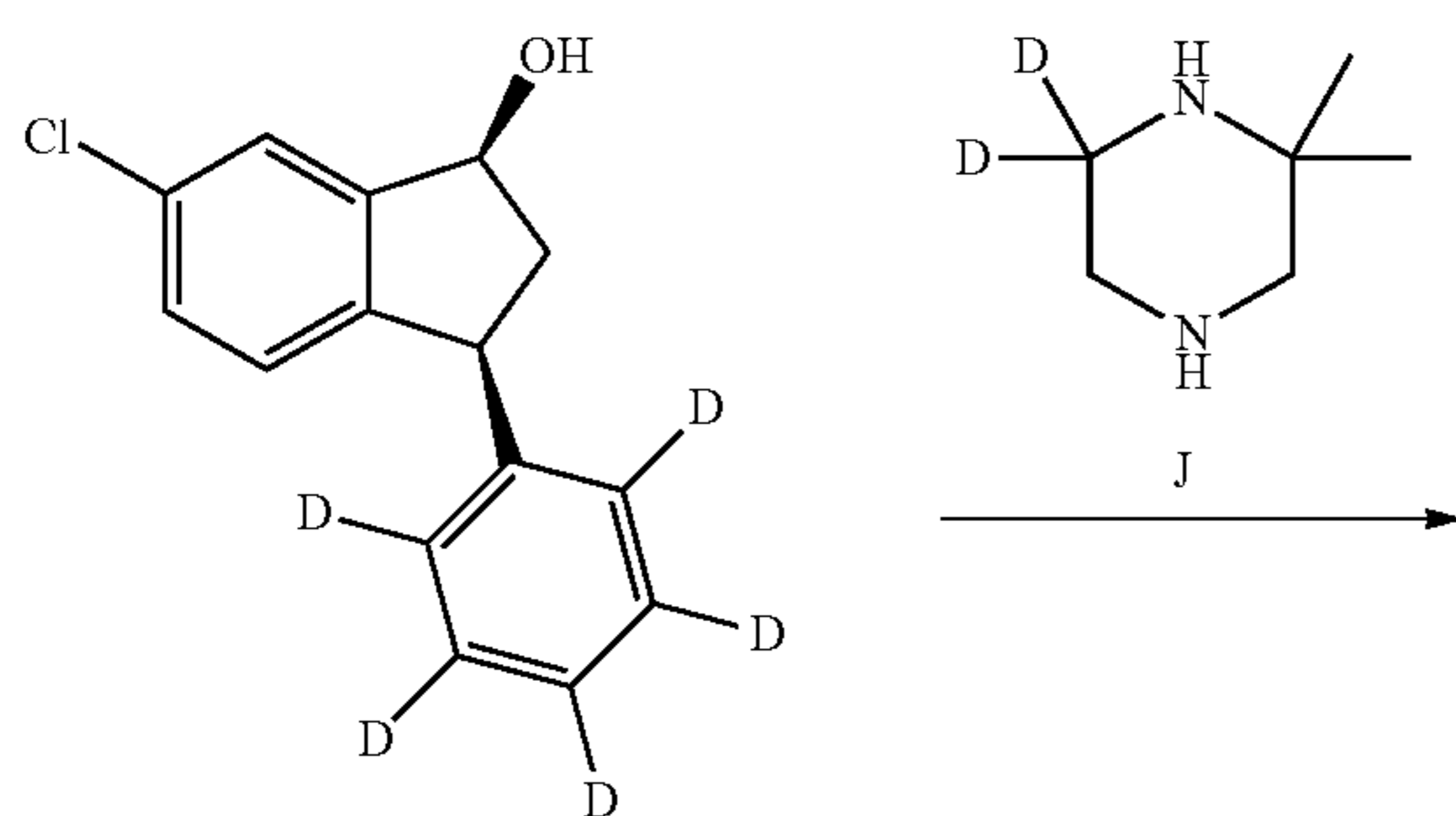
E ((1 S ,3 S )-enantiomer)
