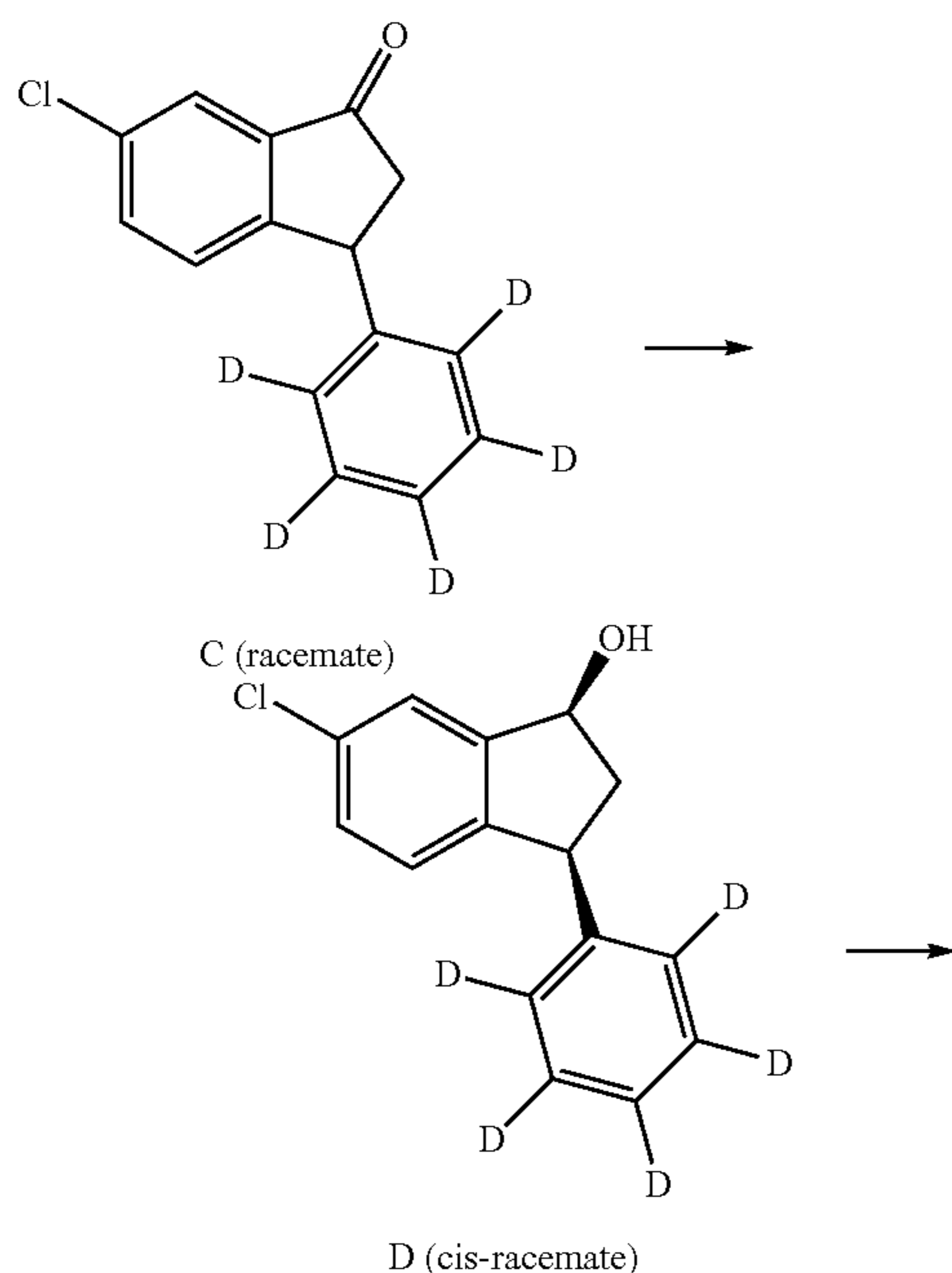
Scheme 10. Synthesis and resolution of Compound E.
