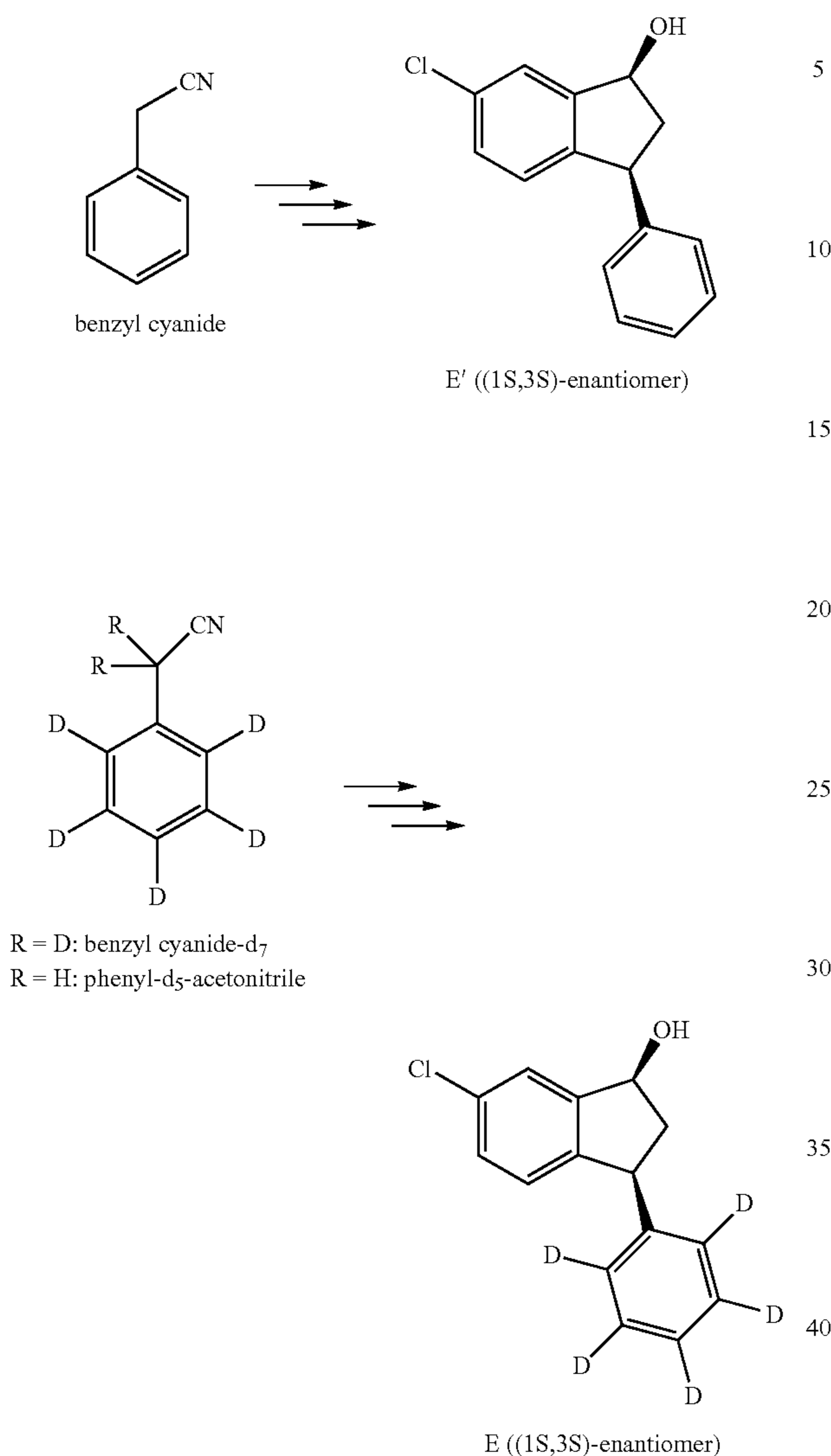
Scheme 4. Exemplary synthesis of intermediates E and E'.
