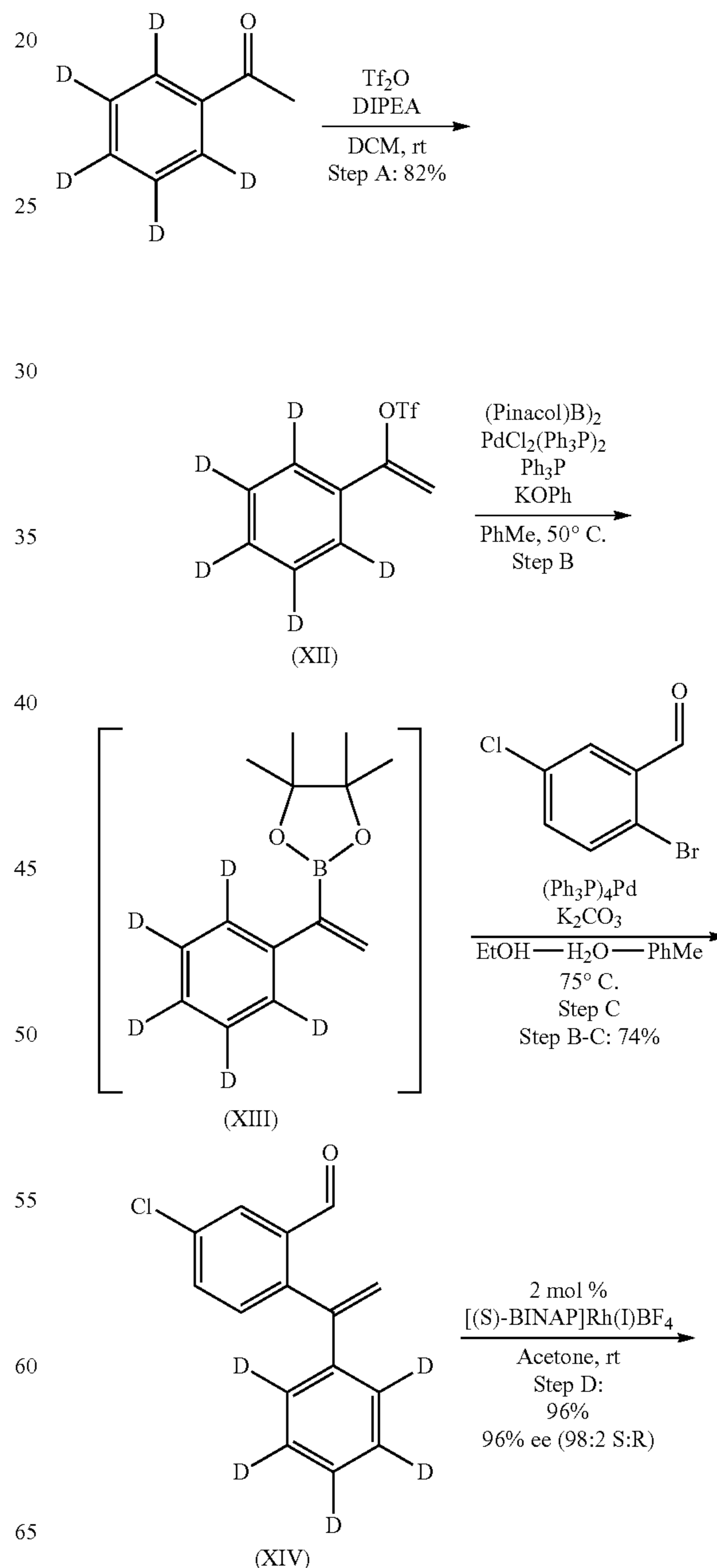
Scheme 14. Synthesis of Compound (XV)
