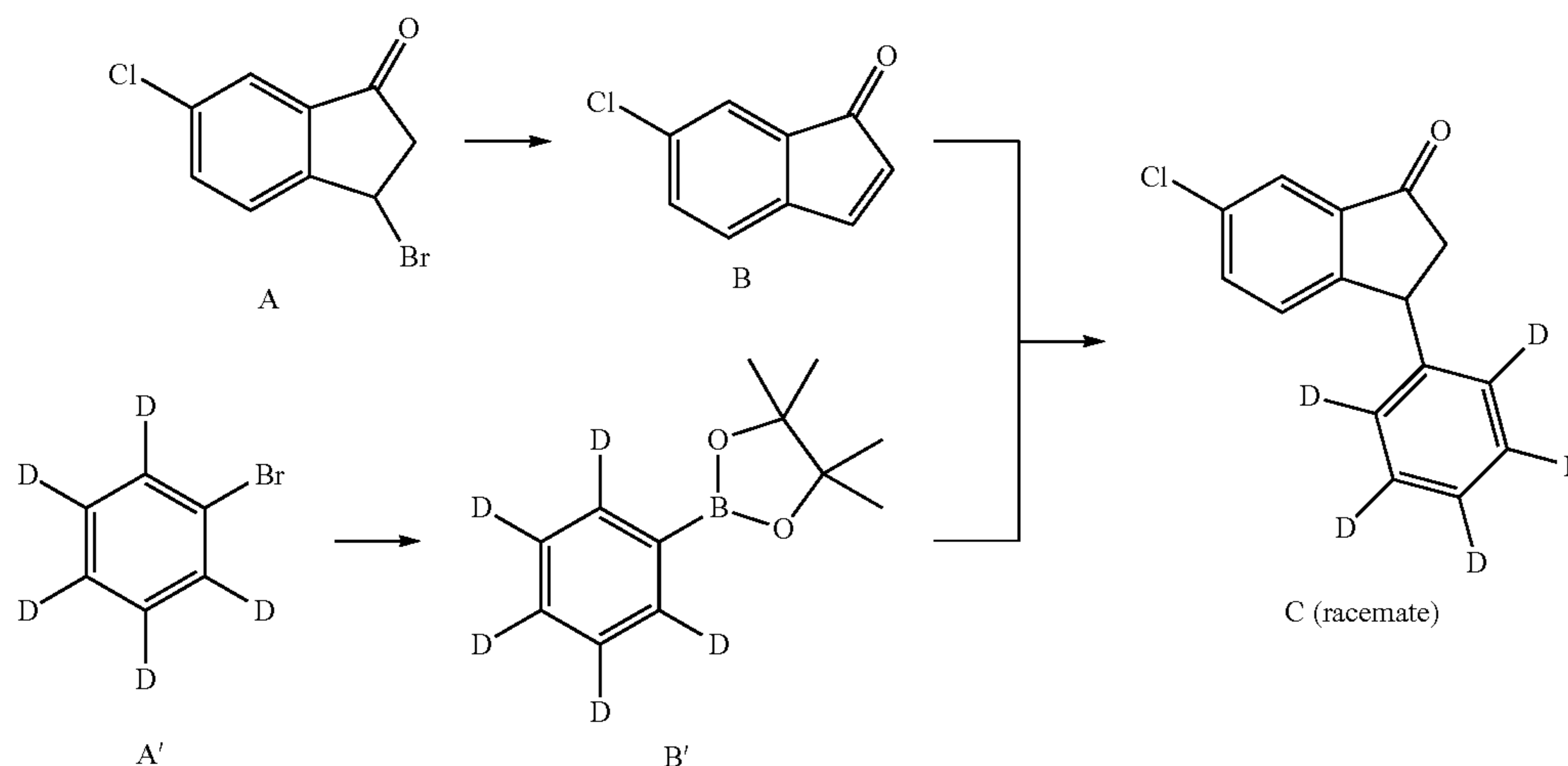
Scheme 9. Synthesis of Compound C.
