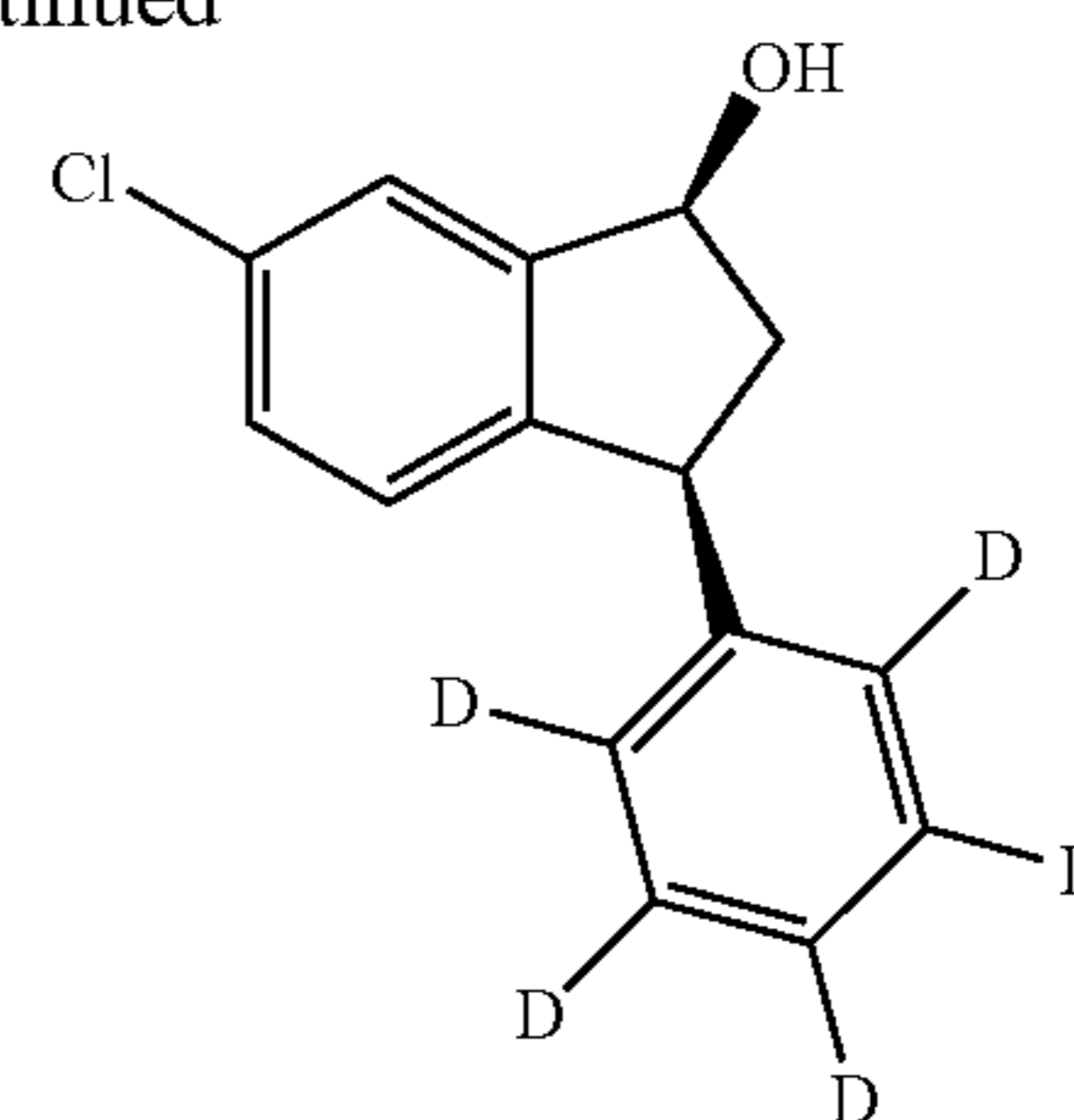
E ((1S,3S)-enantiomer)
