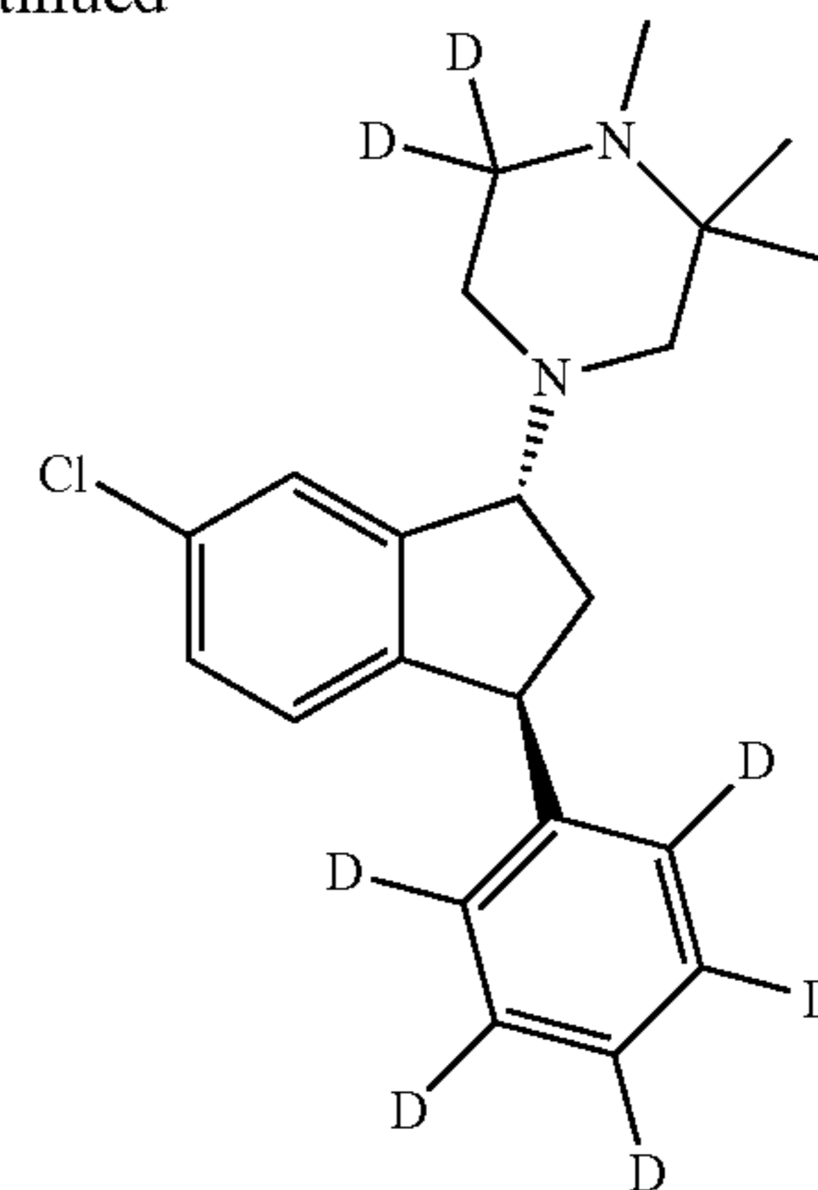
Compound (VII)
