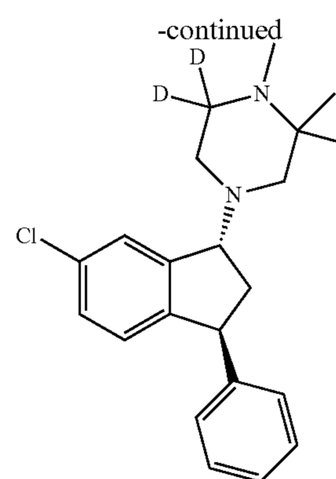
Compound (III)
