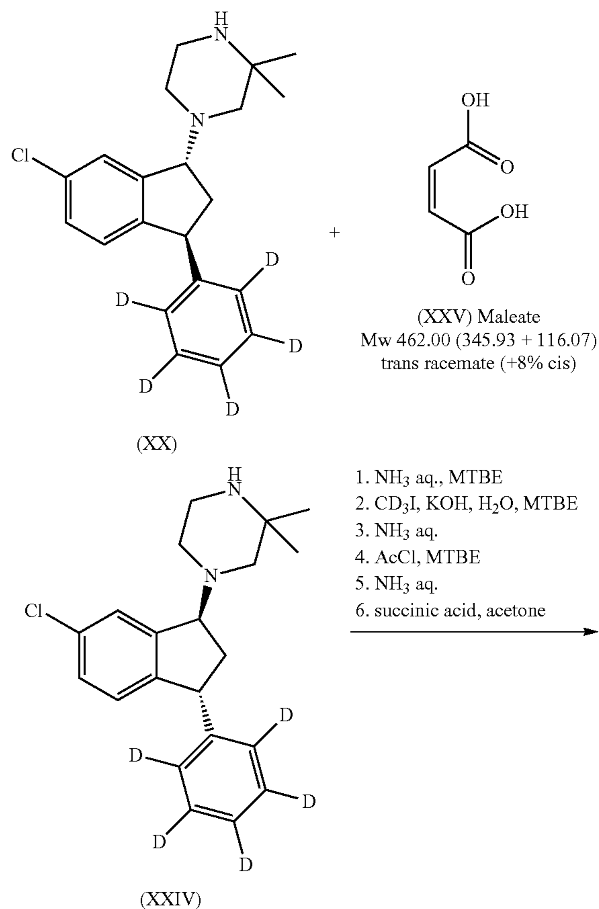
Scheme 17: Synthesis of rac-trans-1-(6-chloro-3-phenyl(d 3 )-indan-1-yl)-1(d 3 ), 2,2-trimethyl-piperazine succinate.
