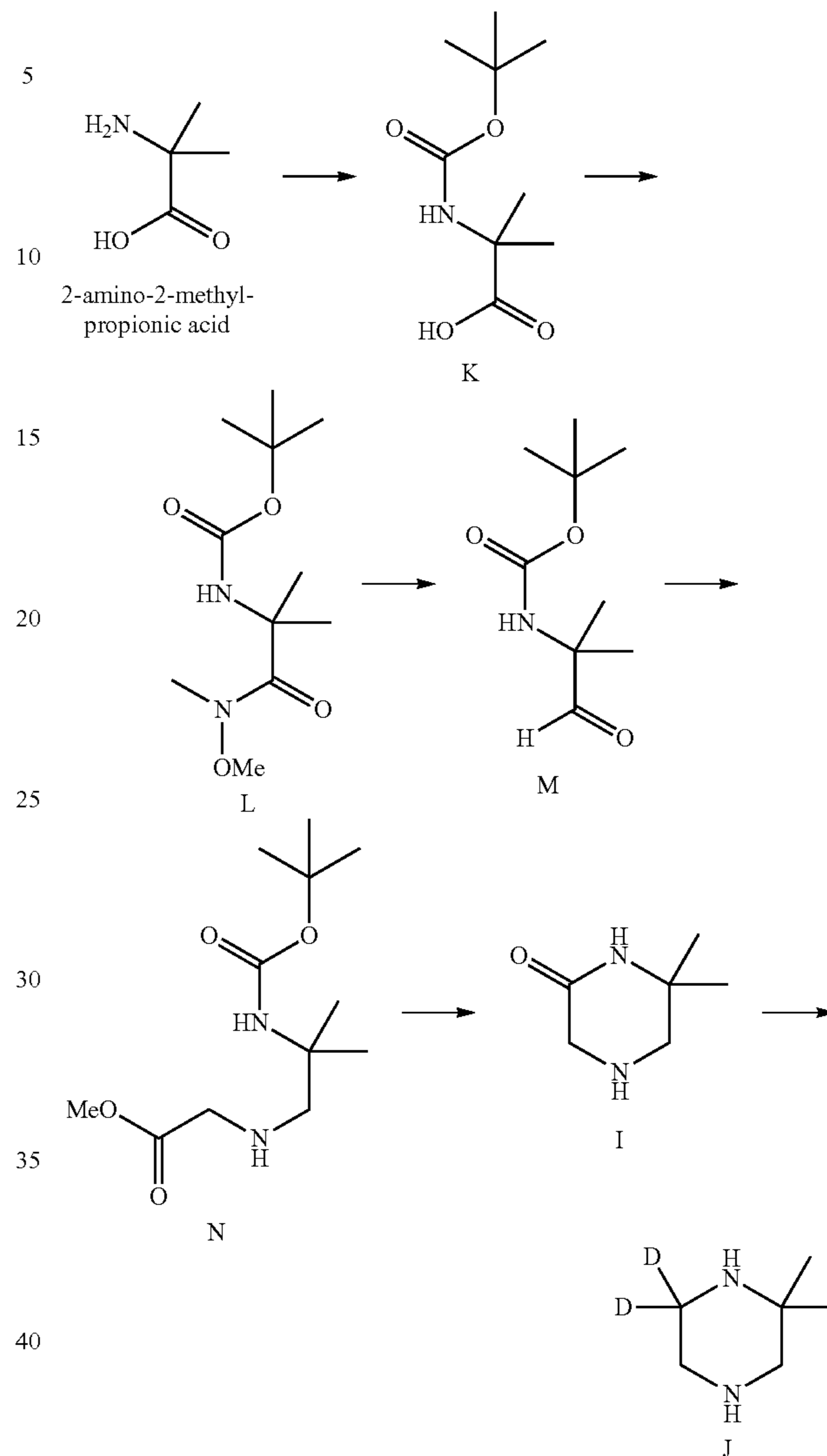
Scheme 7. Alternative exemplary synthesis of intermediate J.
