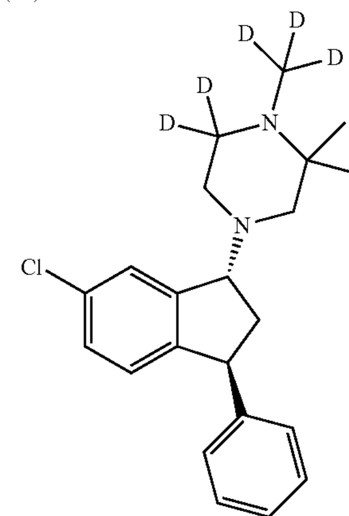
Compound (V)
