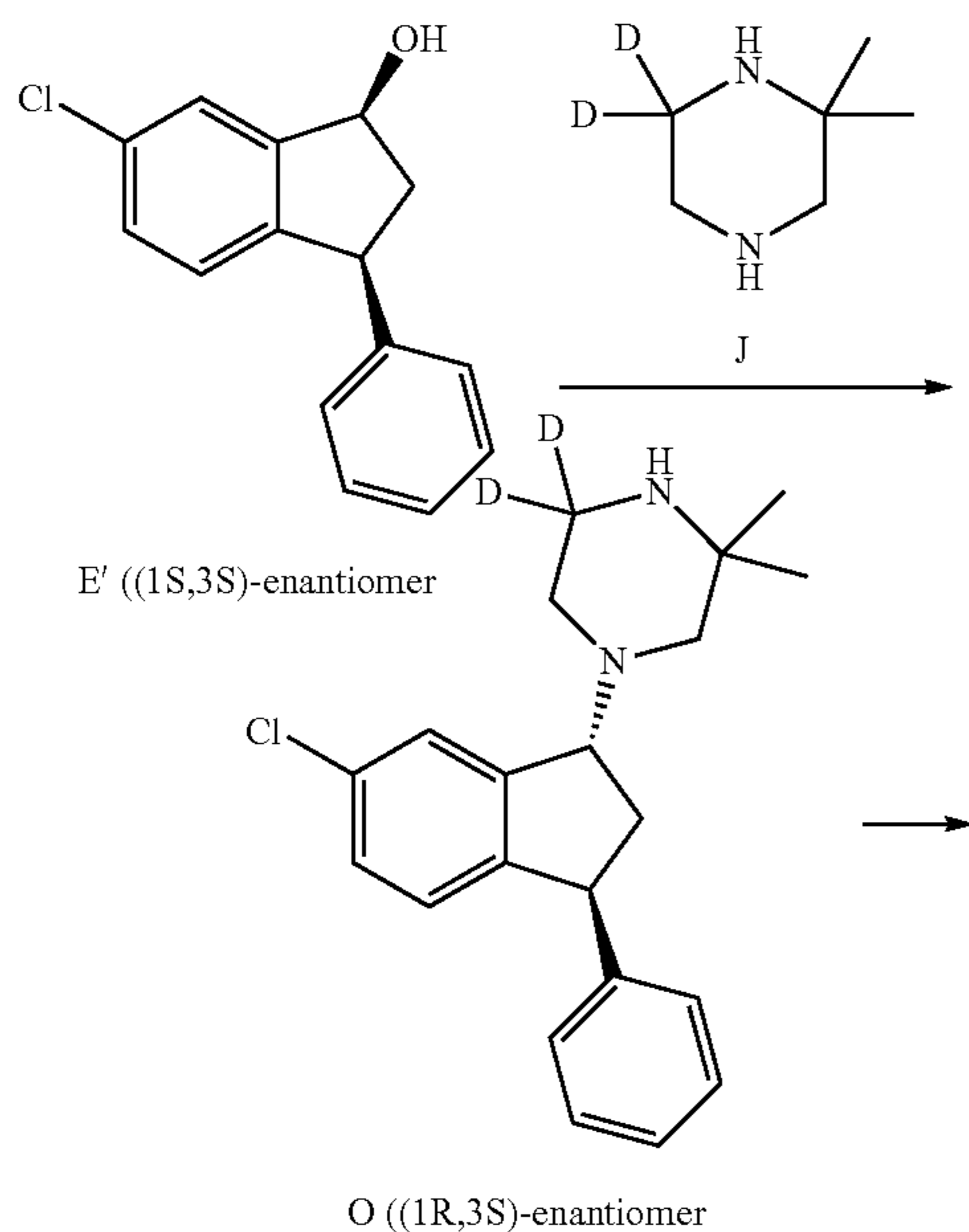
Scheme 12. Synthesis of Compound (III) and Compound (V).
