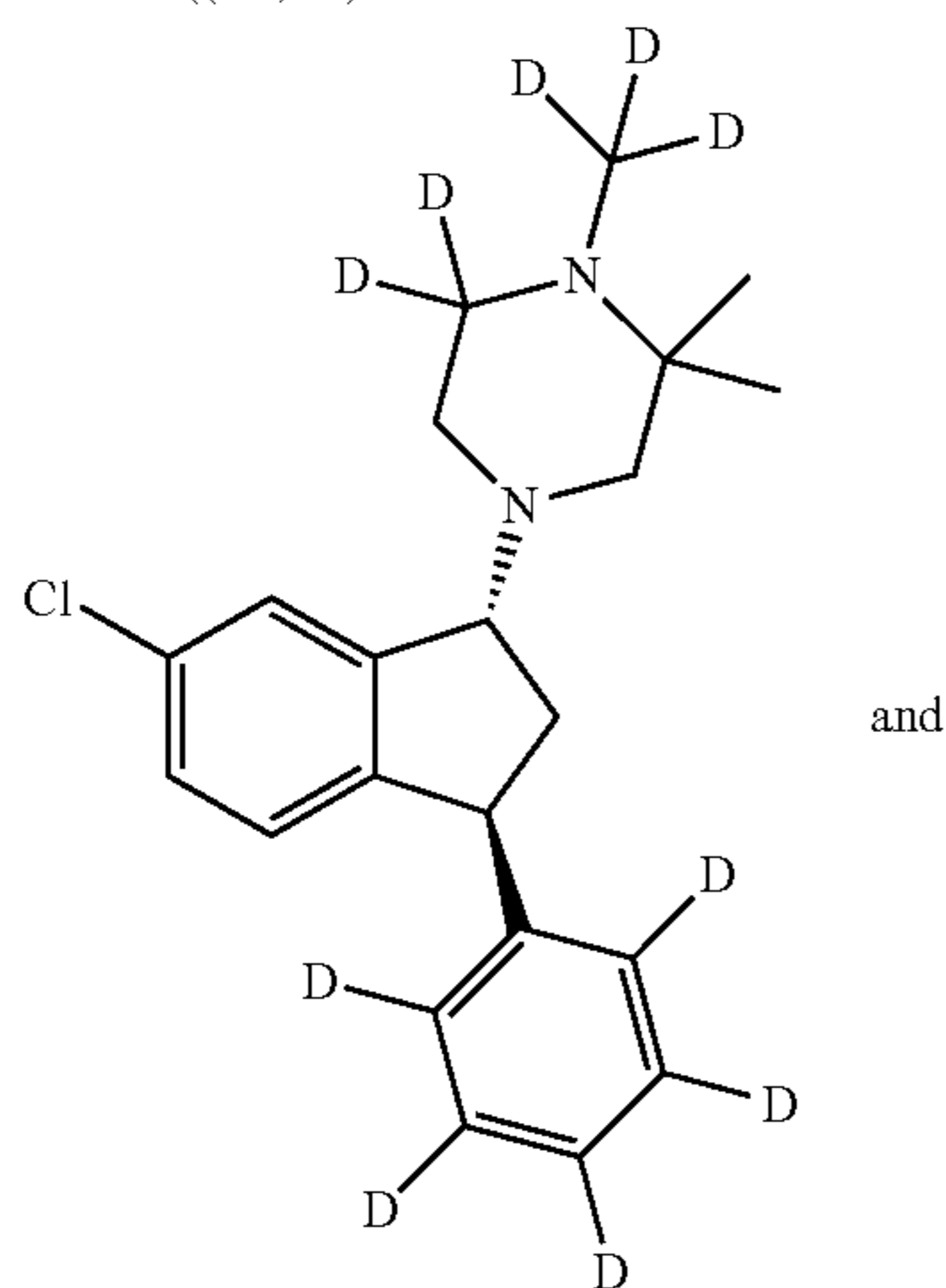
Compound (VI)
