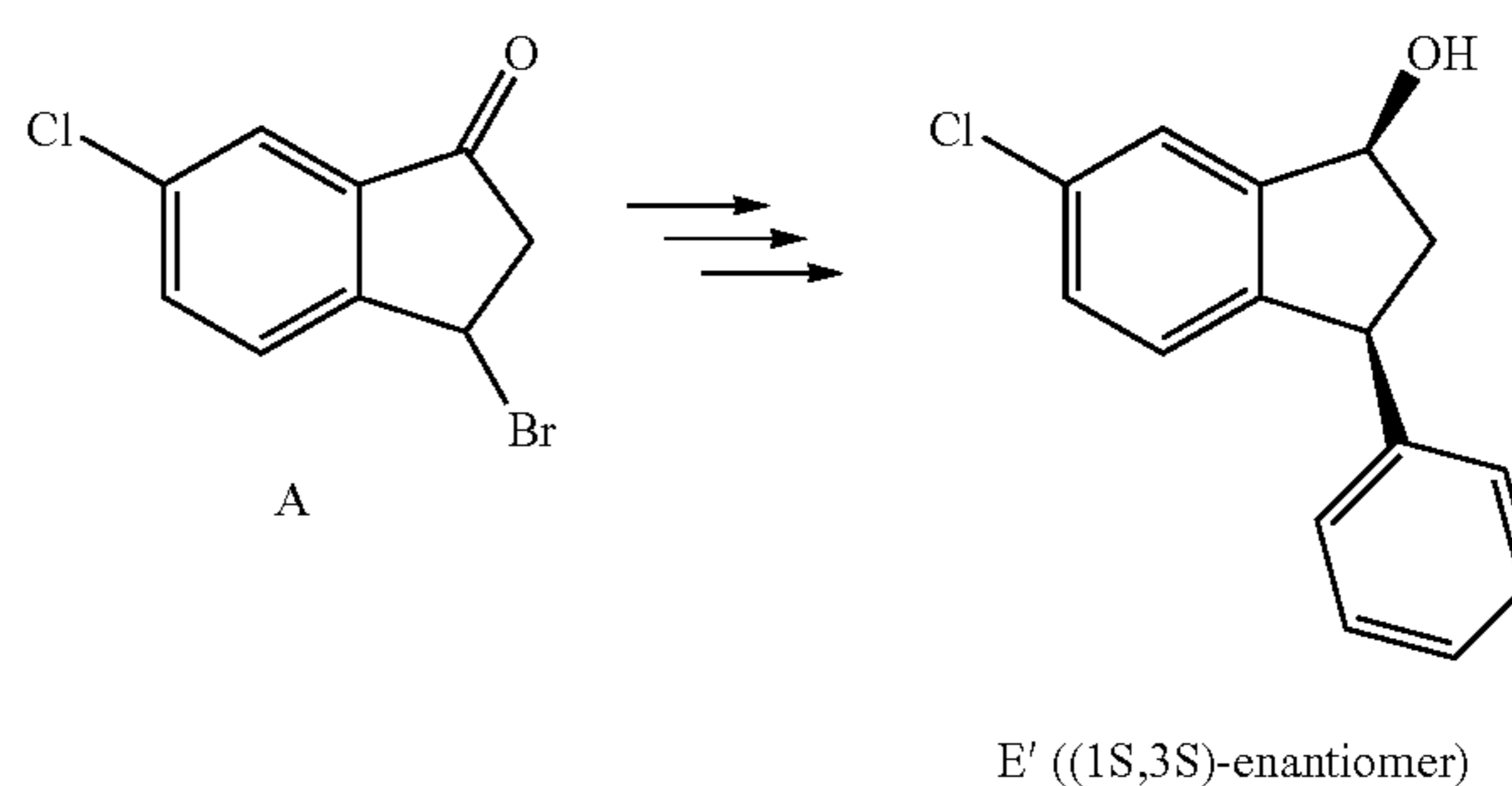
Scheme 3. Exemplary synthesis of intermediate E'.
