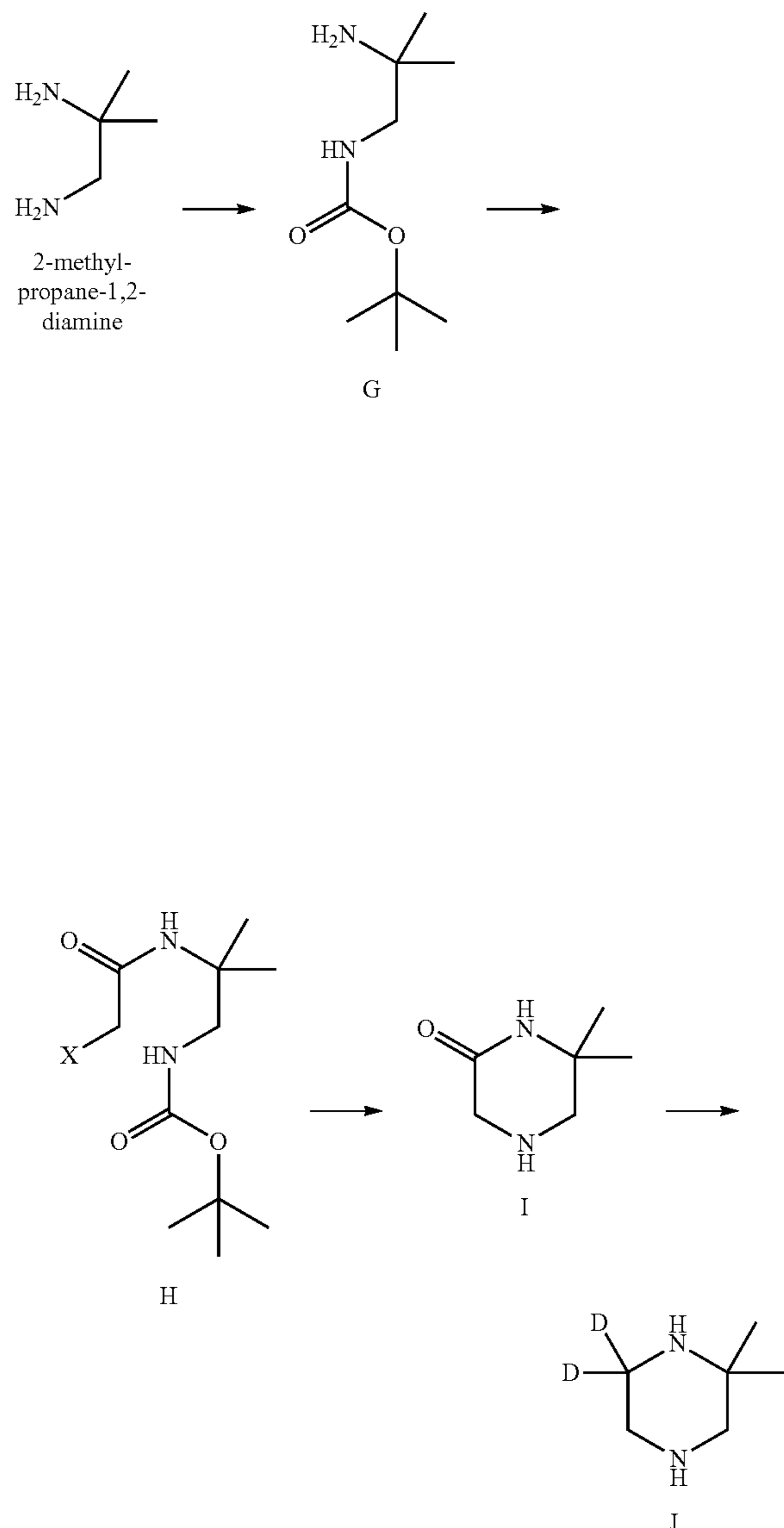
Scheme 6. Exemplary synthesis of intermediate J.
