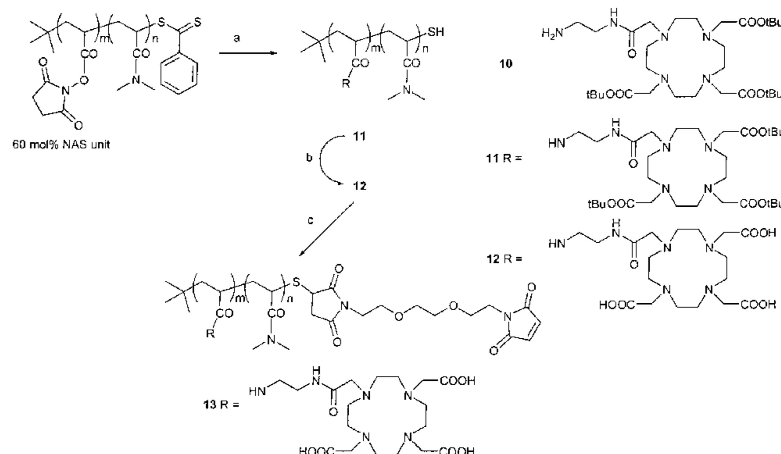
Scheme 12. Preparation of DOTA based ligand-polymer conjugate
