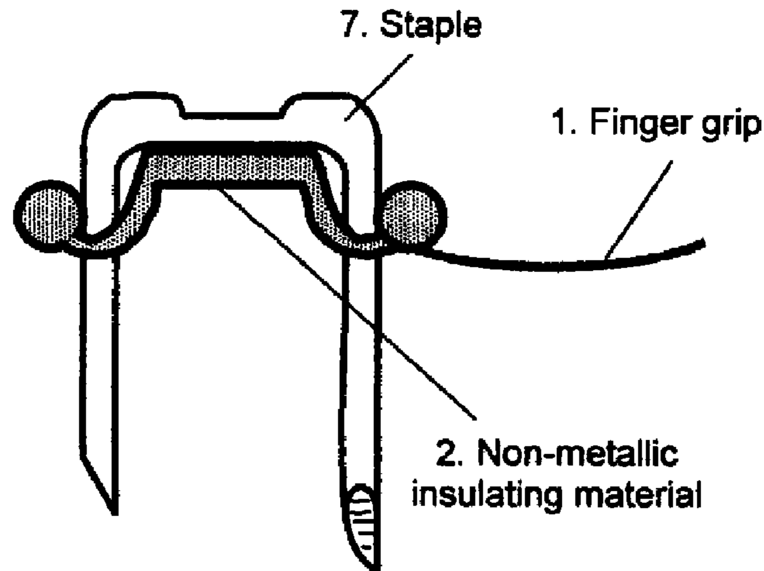
(Front elevation view)
