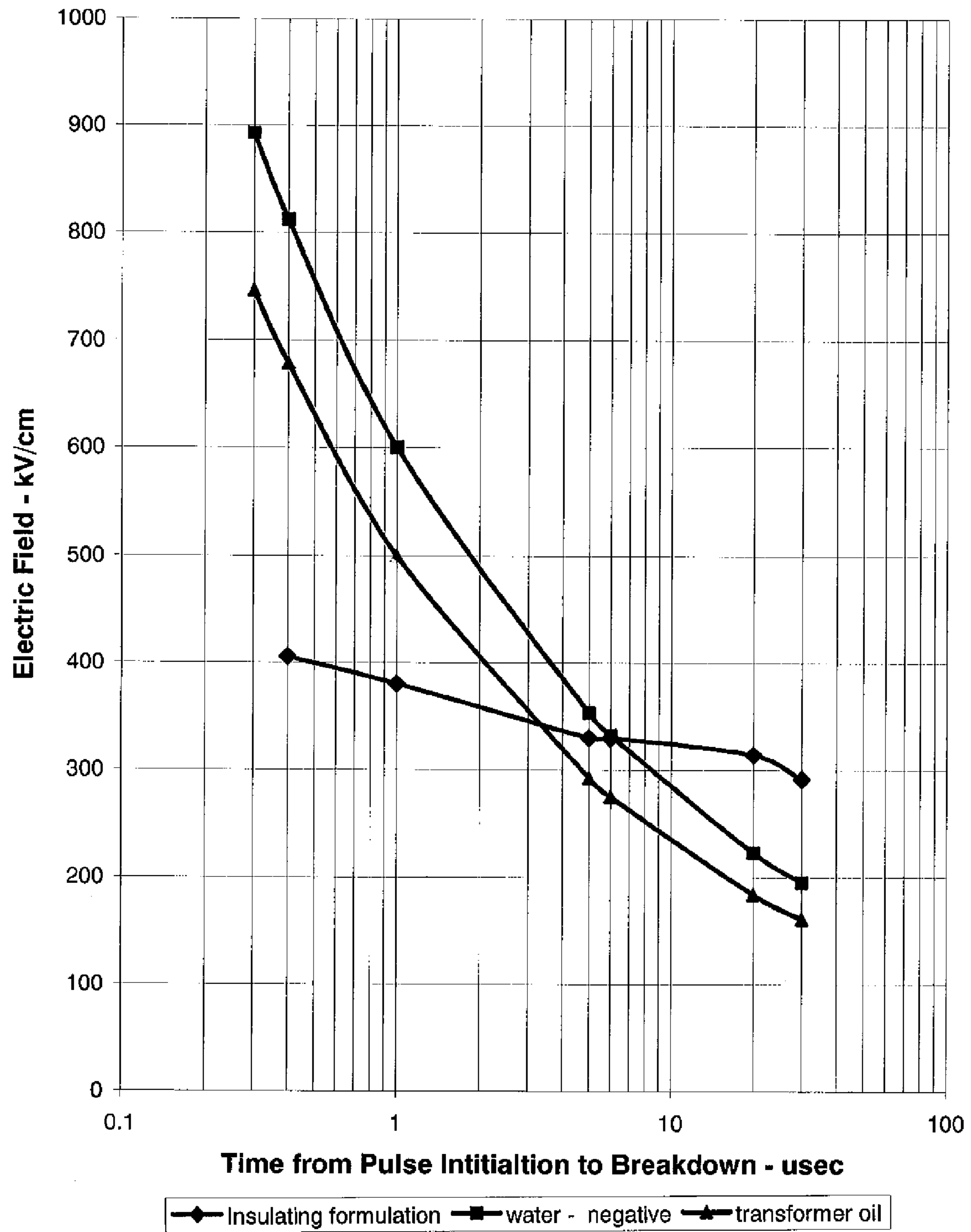
Dielectric Strength vs. Delay To Breakdown Figure 32
