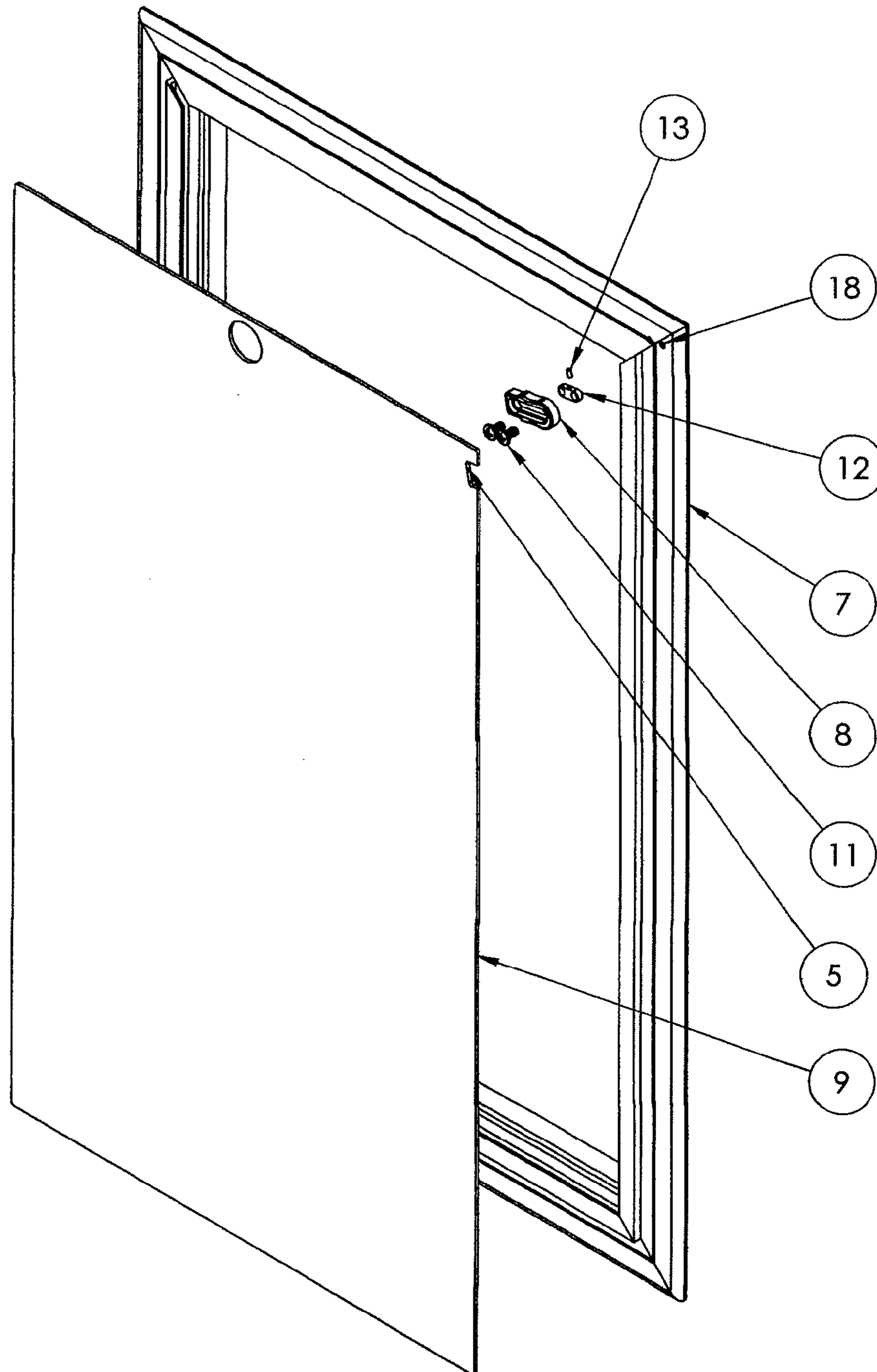
EXPLODED VIEW
