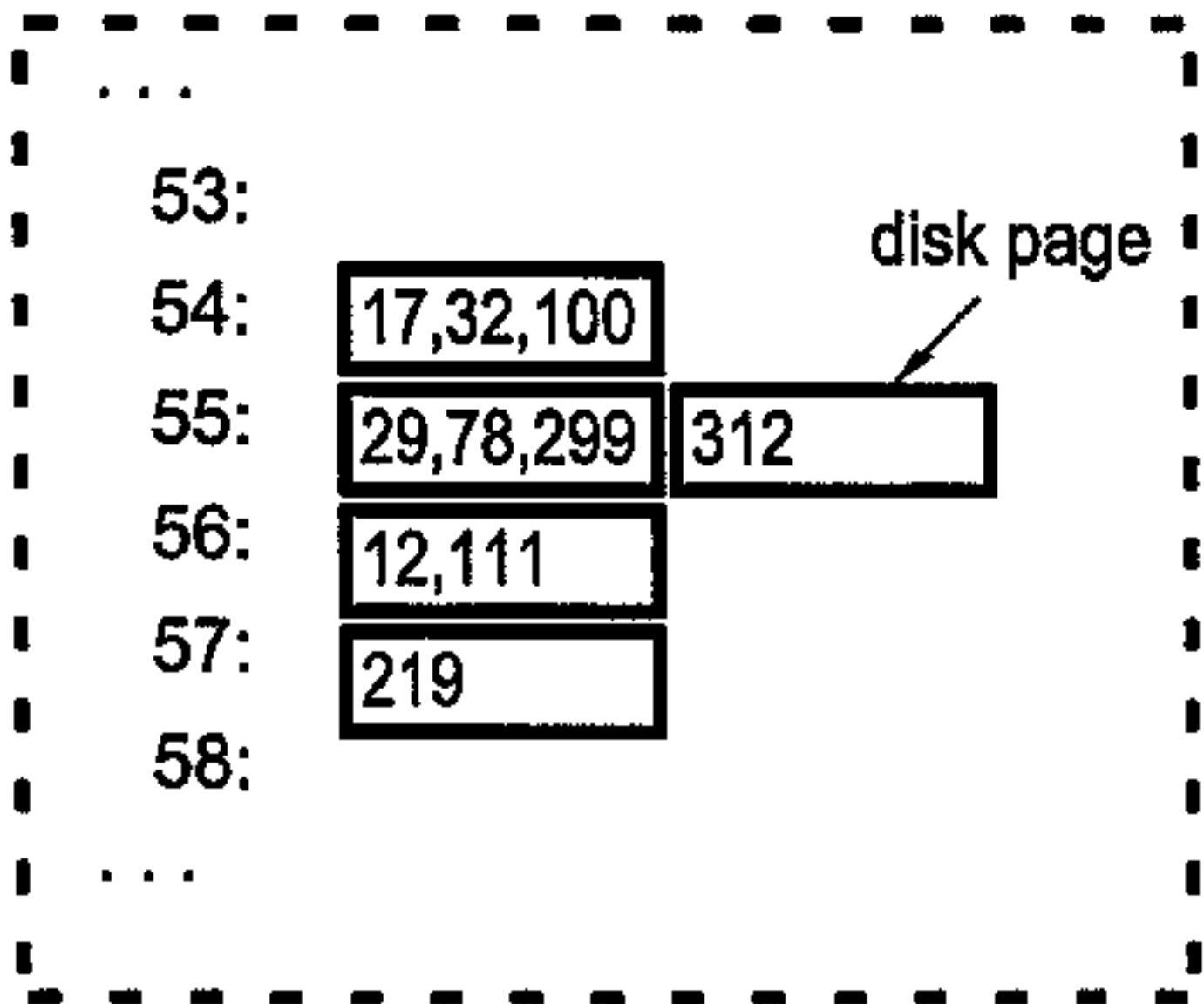
PART II: disk pages of offset lists
