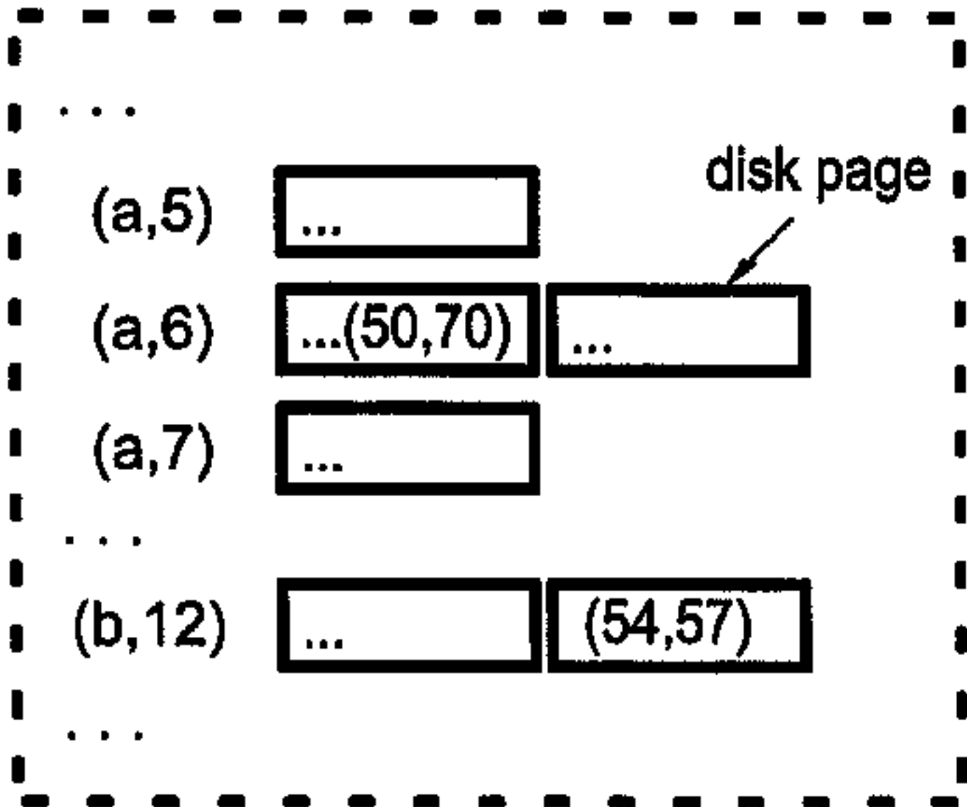
PART I: disk pages of iso-depth arrays
