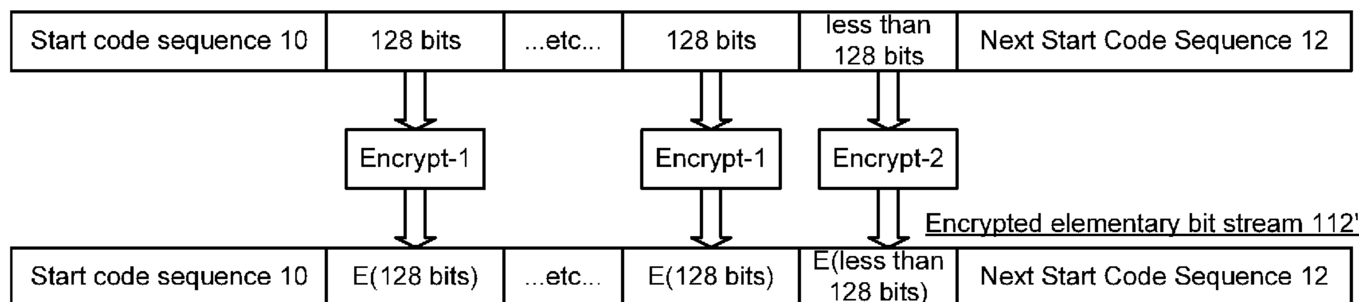
Elementary bit stream 110'
