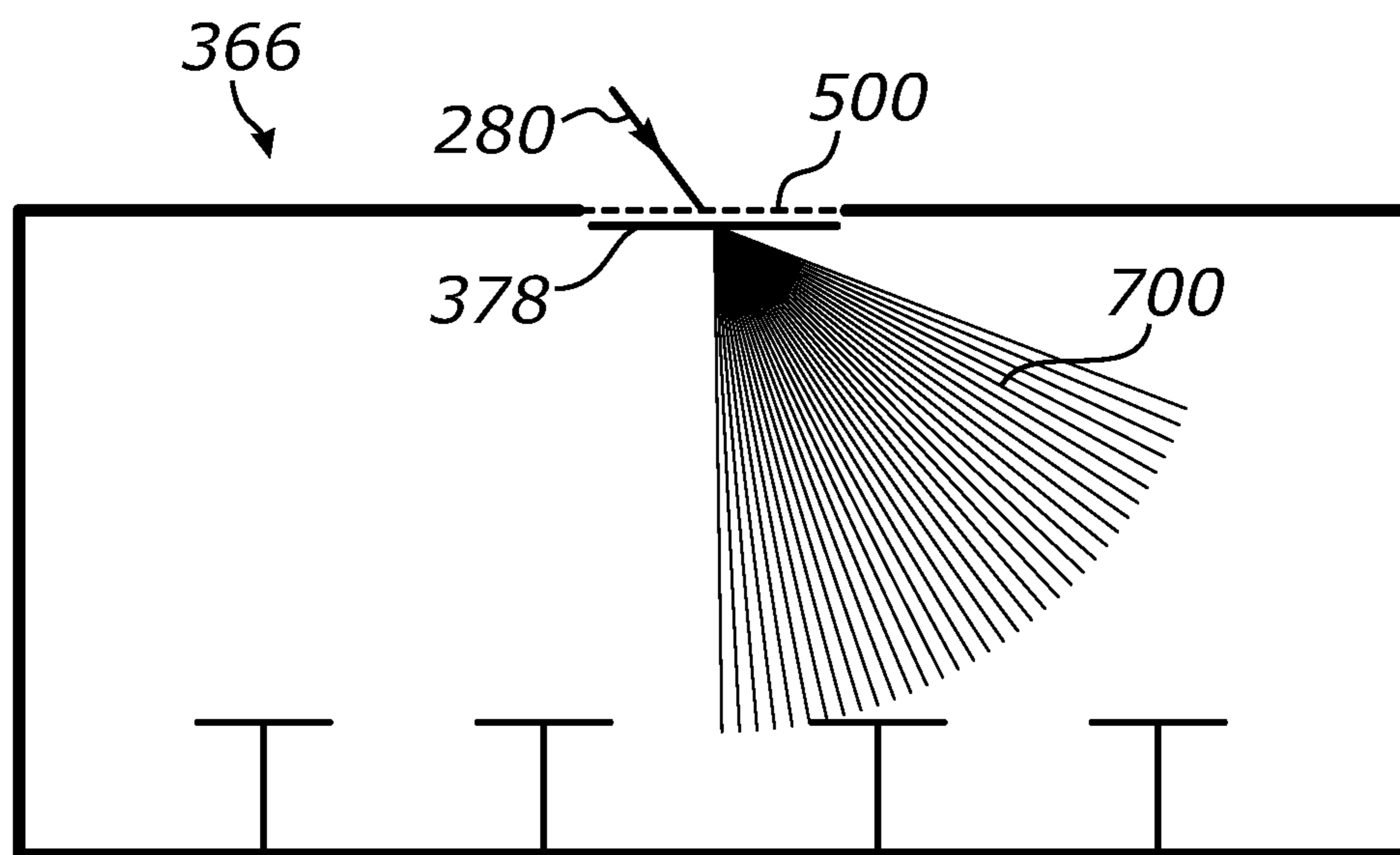
FIG. 30 (PRIOR ART)
