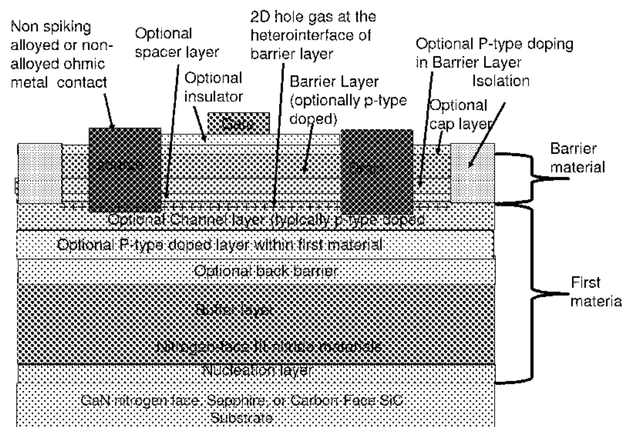
Non-Inverted P-Channel III-Nitride transistor with hole carriers in the channel with non-spiking ohmic contacts
