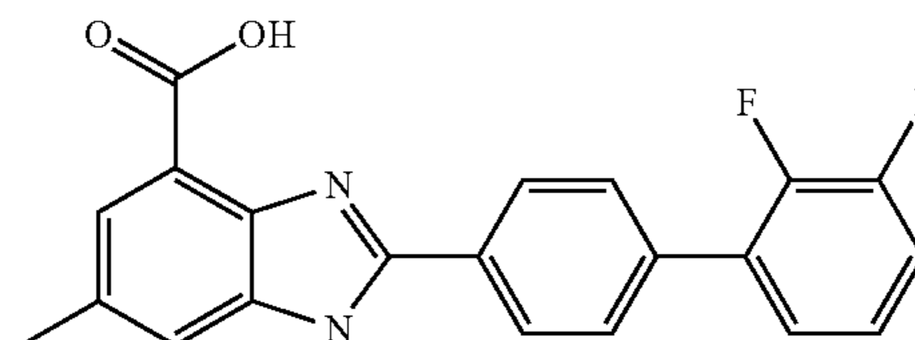
Step 3: 2-(2',3'-Difluoro-biphenyl-4-yl)-6-methyl-1H-benzimidazole-4-carboxylic acid
