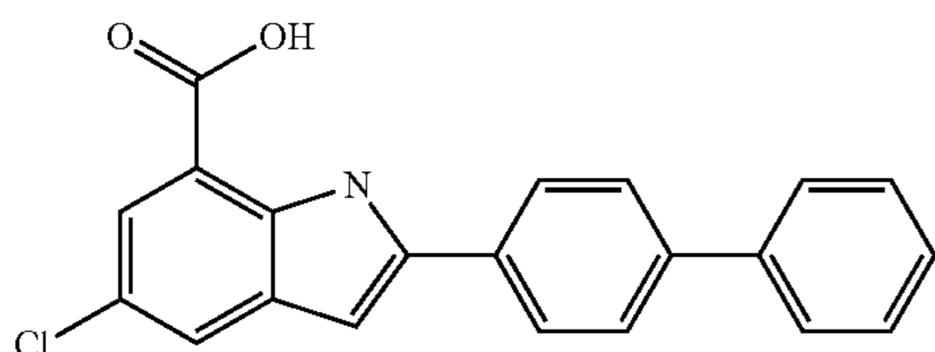
2-Biphenyl-4-yl-5-chloro-1H-indole-7-carboxylic acid
