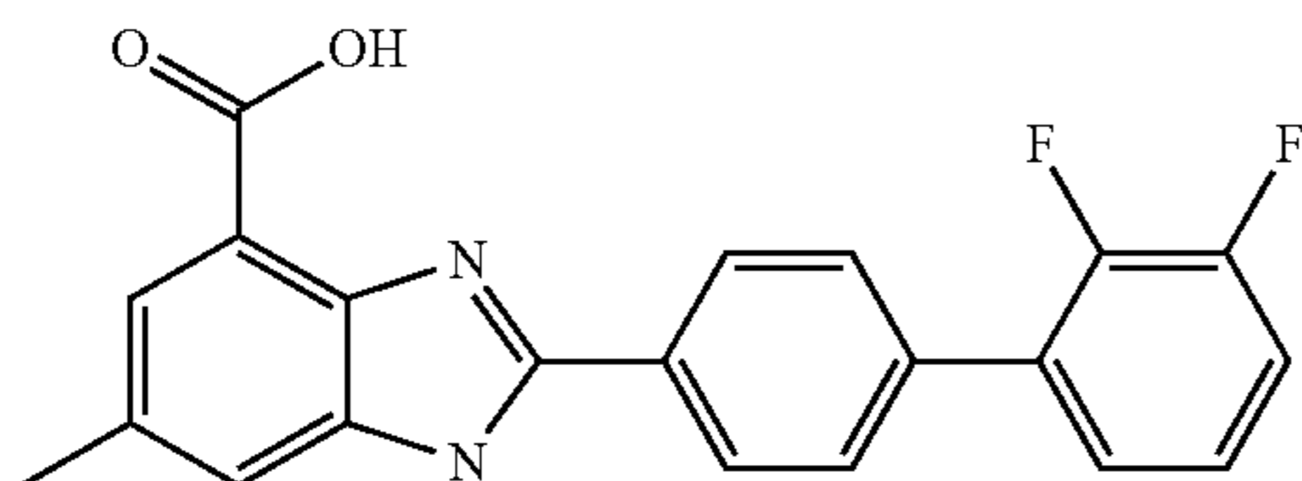
2-(2',3'-Difluoro-biphenyl-4-yl)-6-methyl-1H-benzimidazole-4-carboxylic acid
