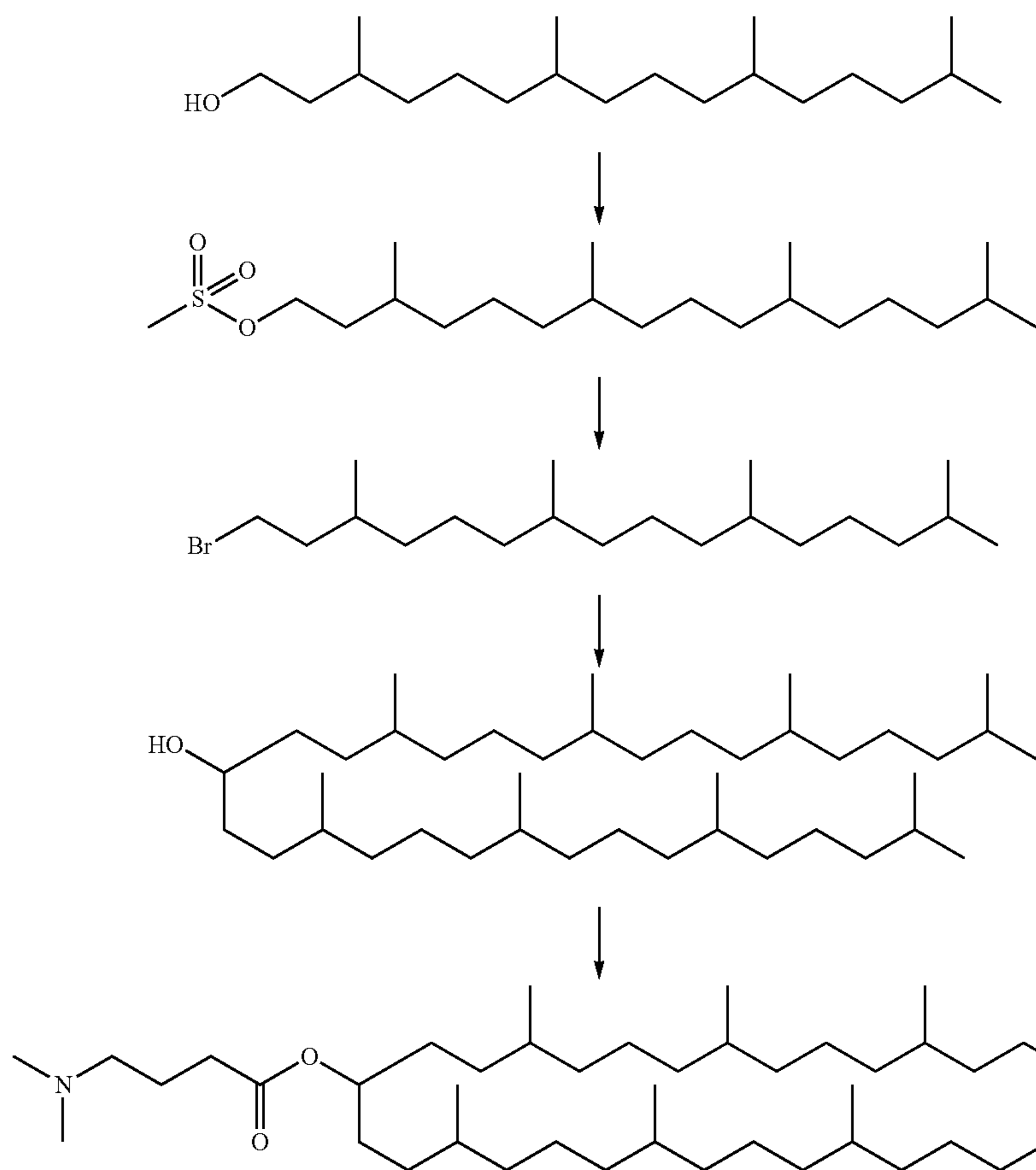
Scheme 12
