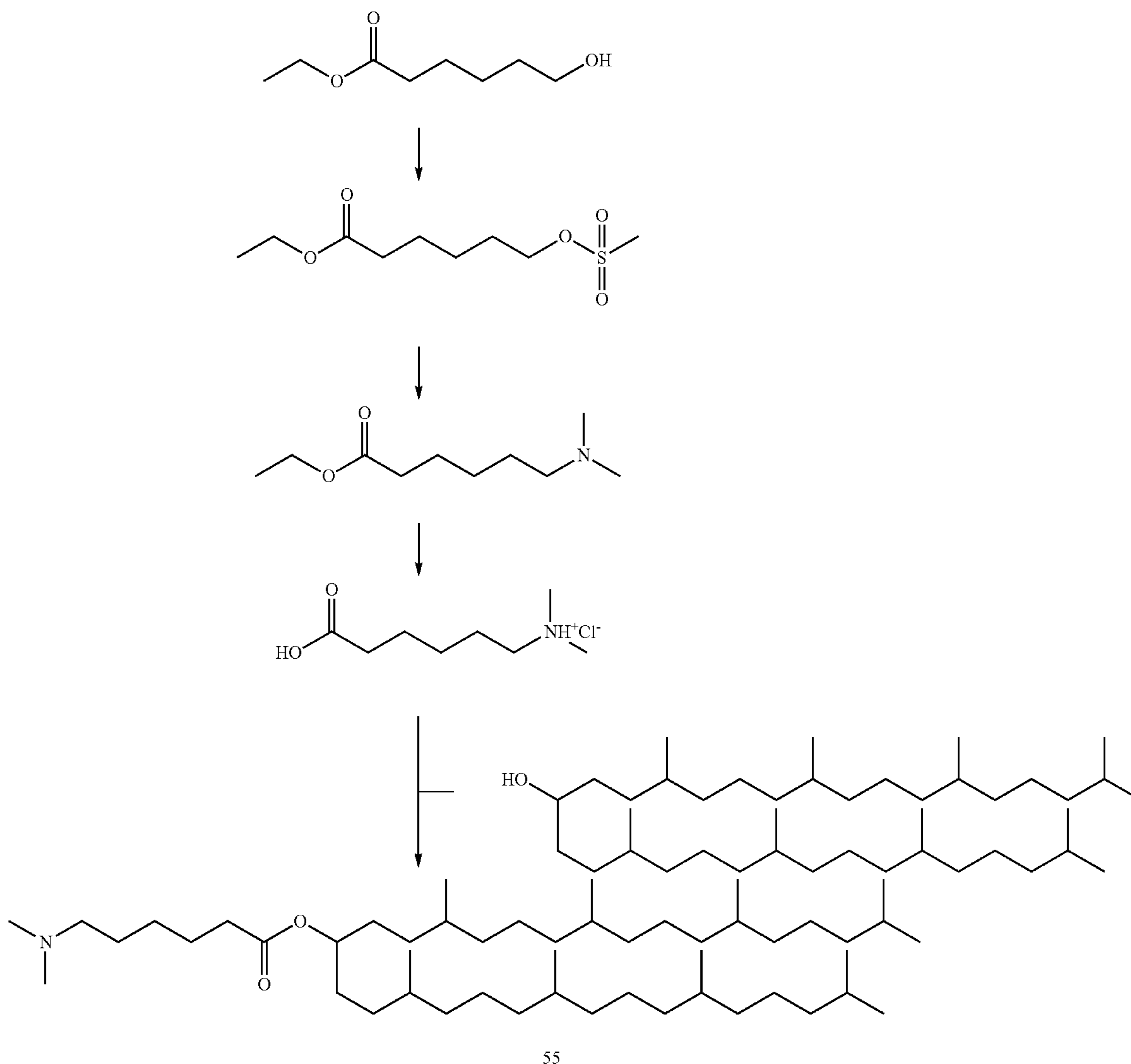
Scheme 14
