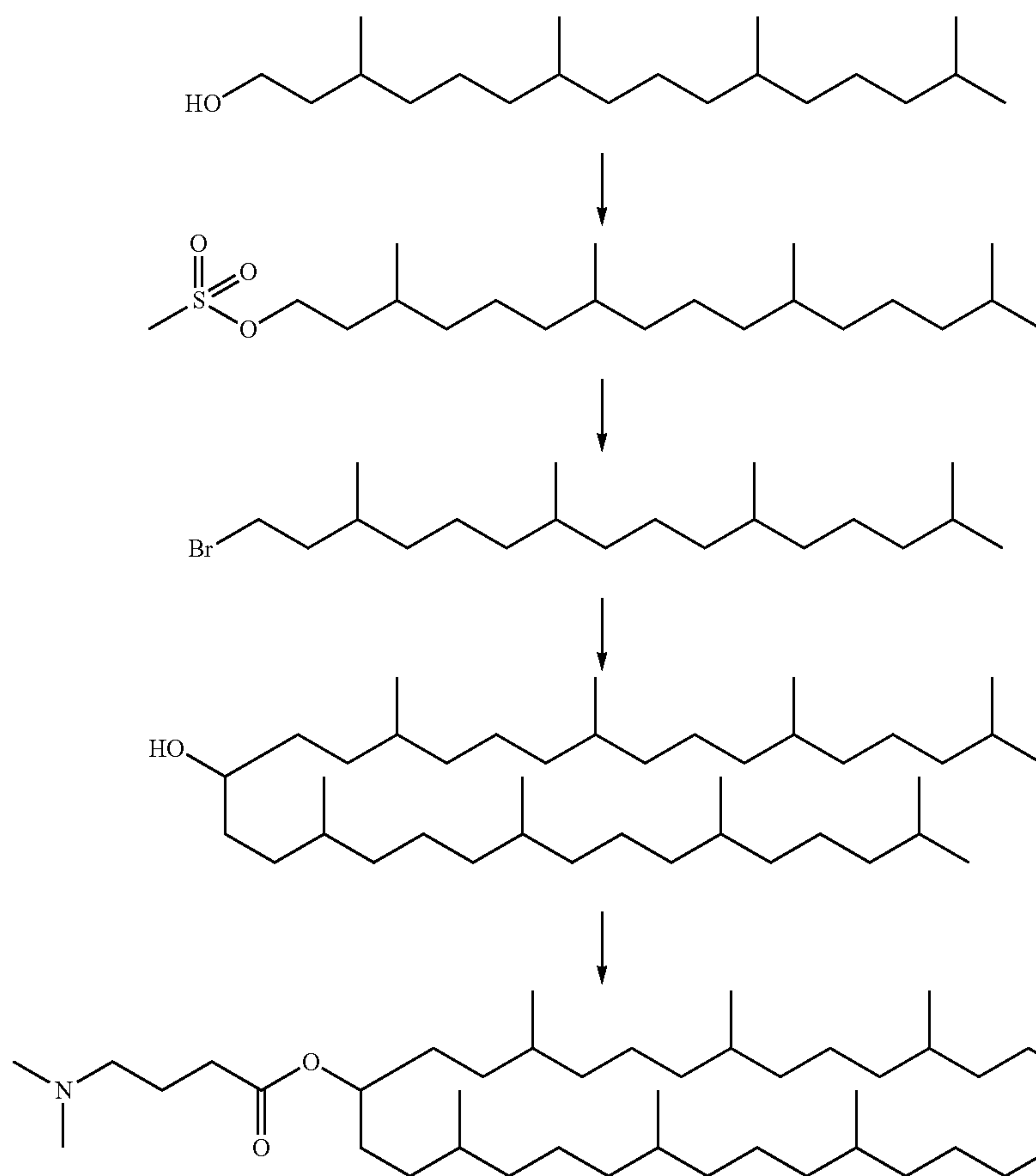
Scheme 12
