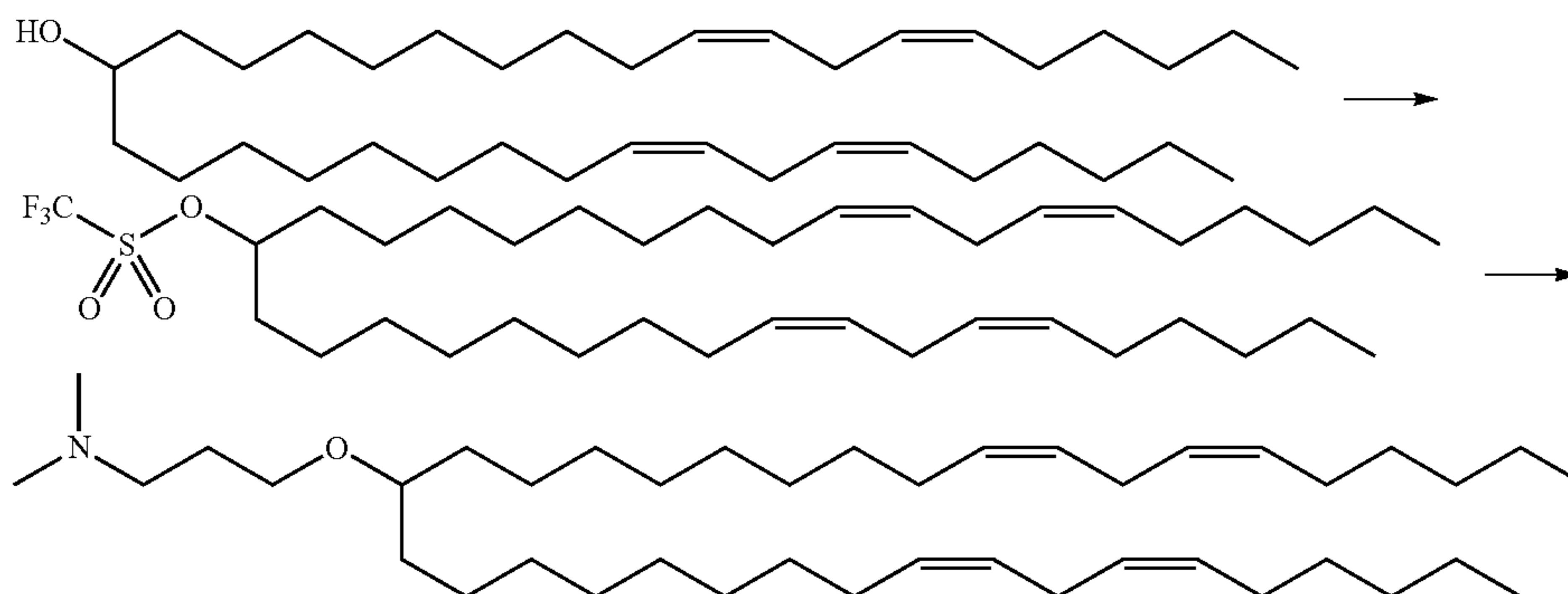
Scheme 8
