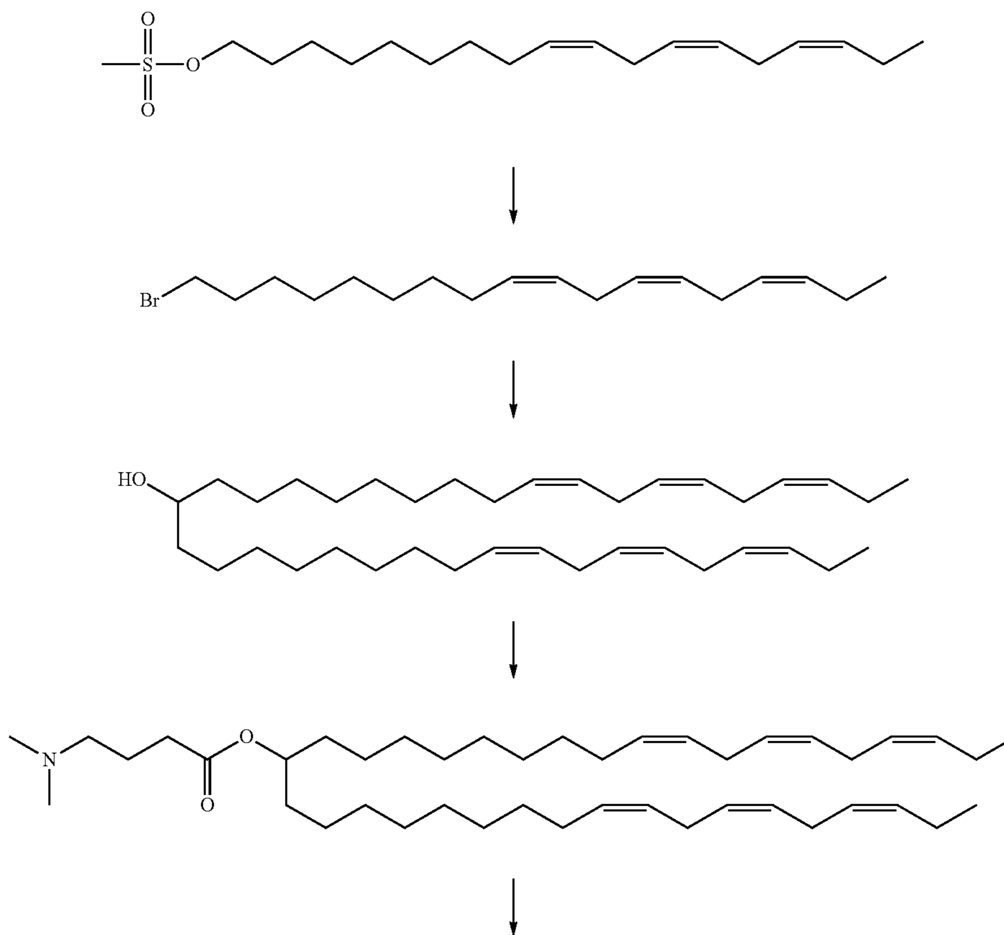
Scheme 2
