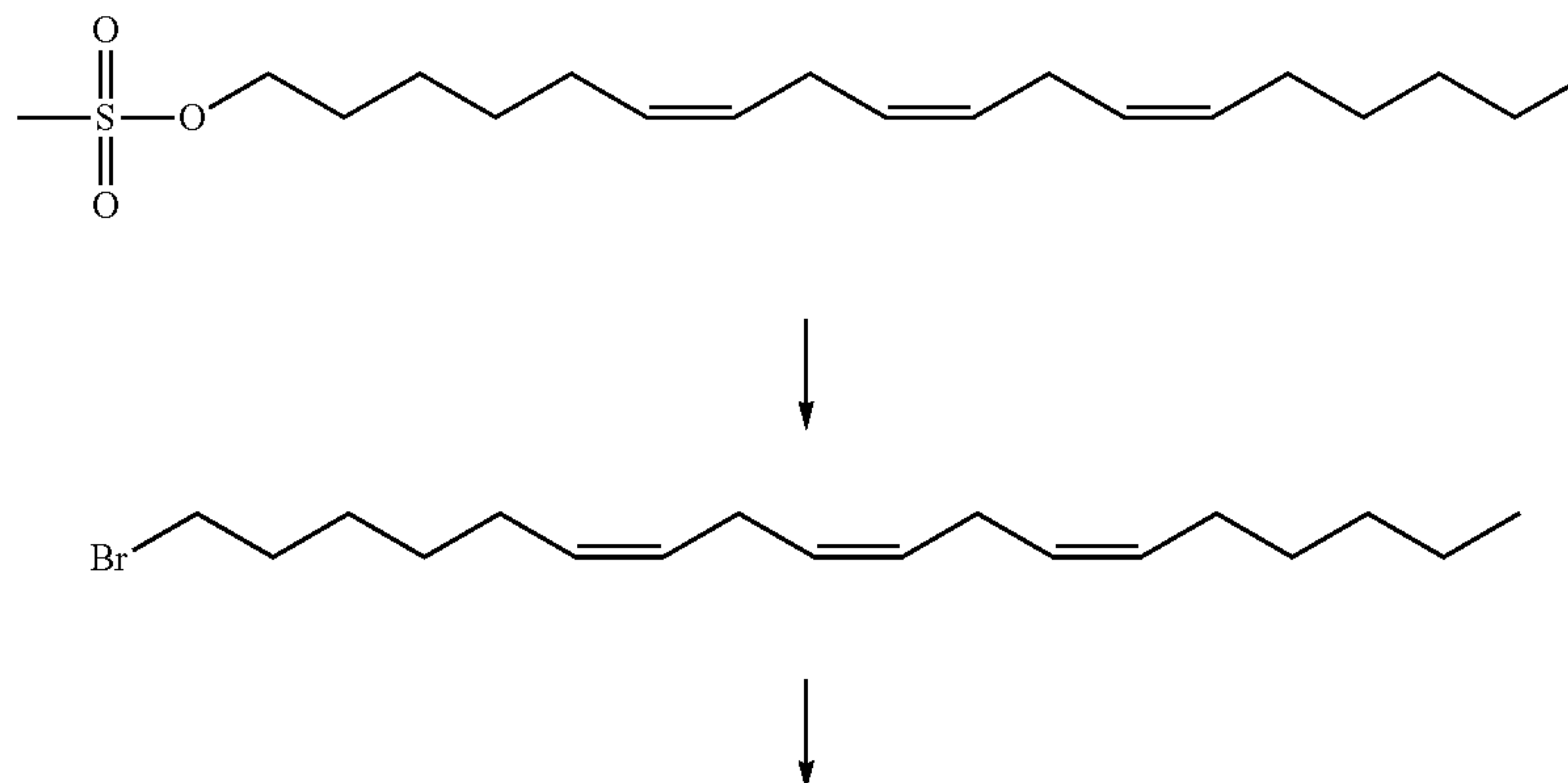
Scheme 3
