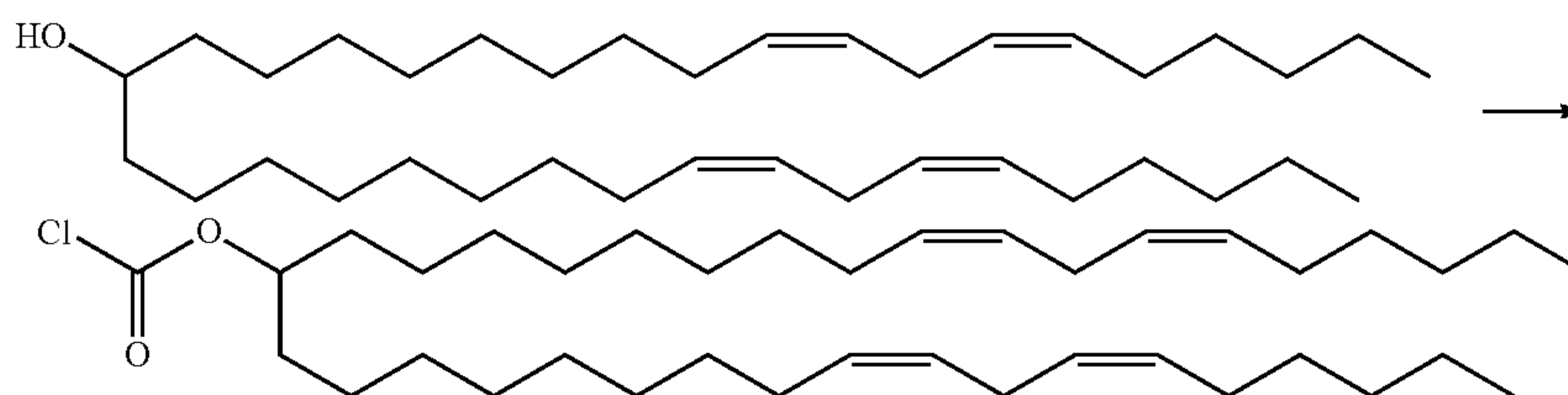
Scheme 4
