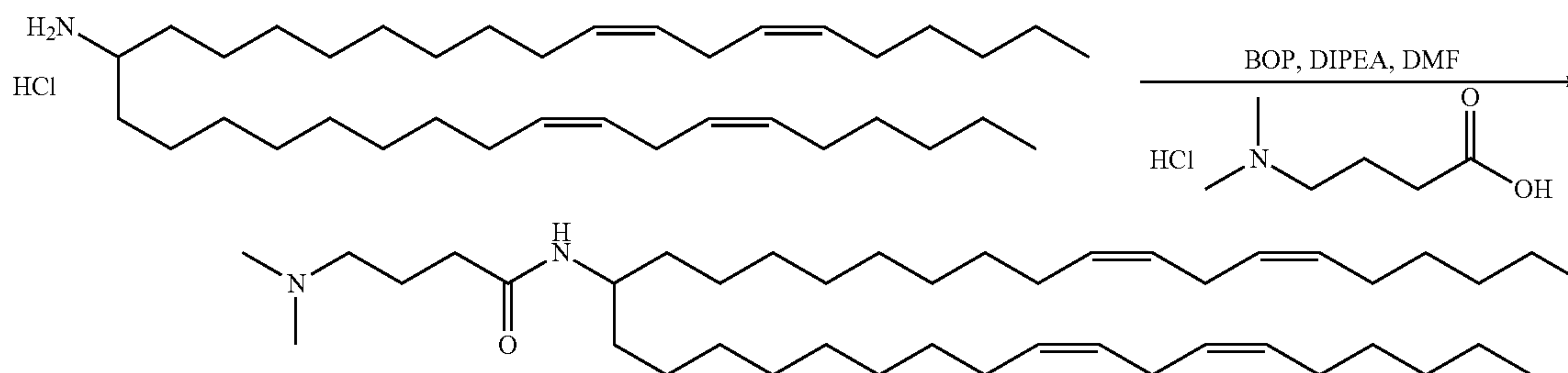
Scheme 11
