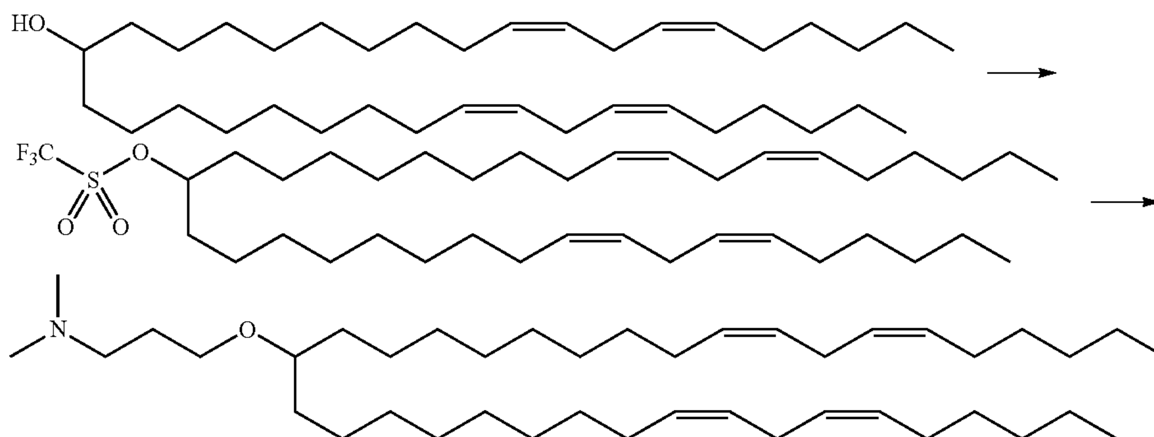
Scheme 8
