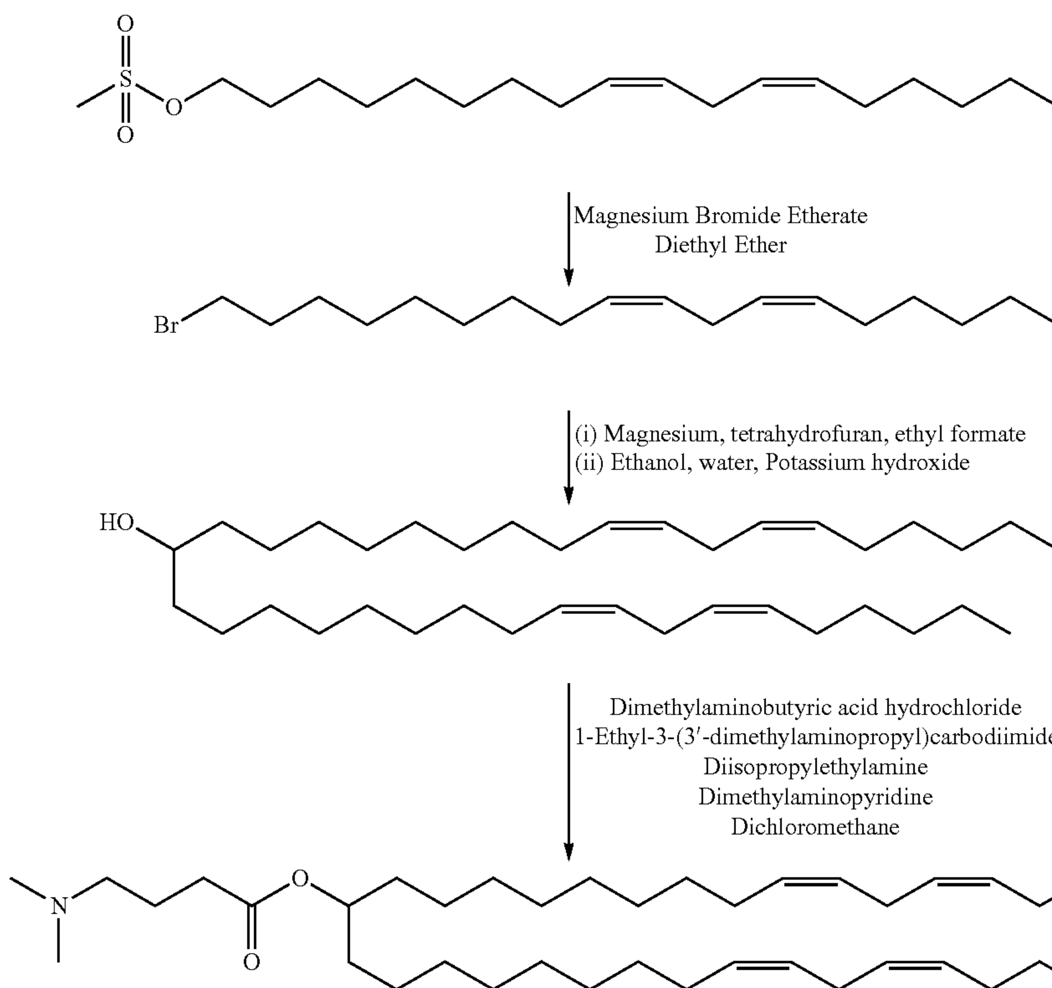
Scheme 1
