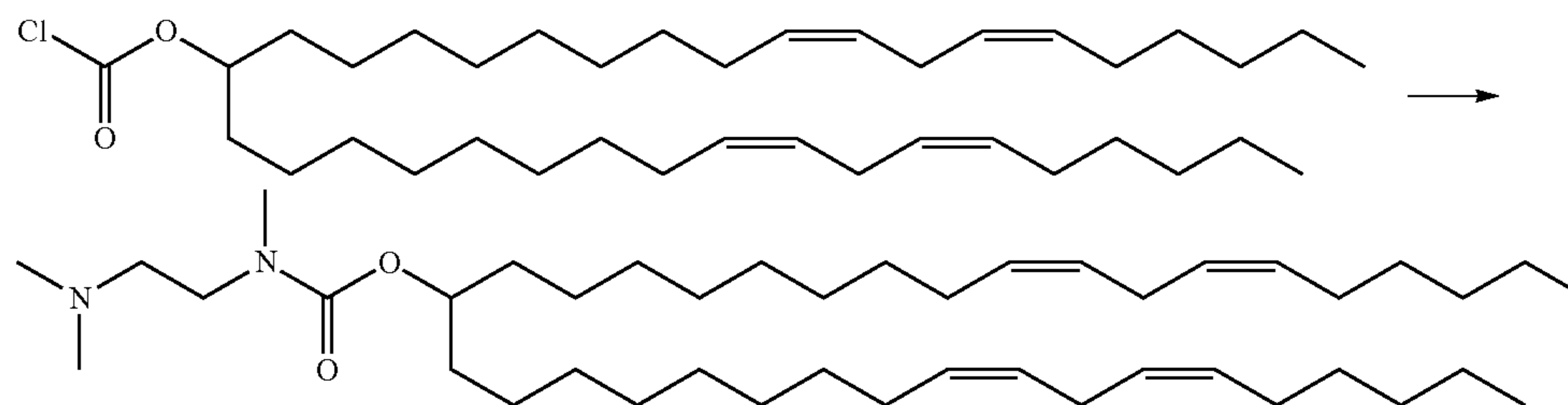
Scheme 6
