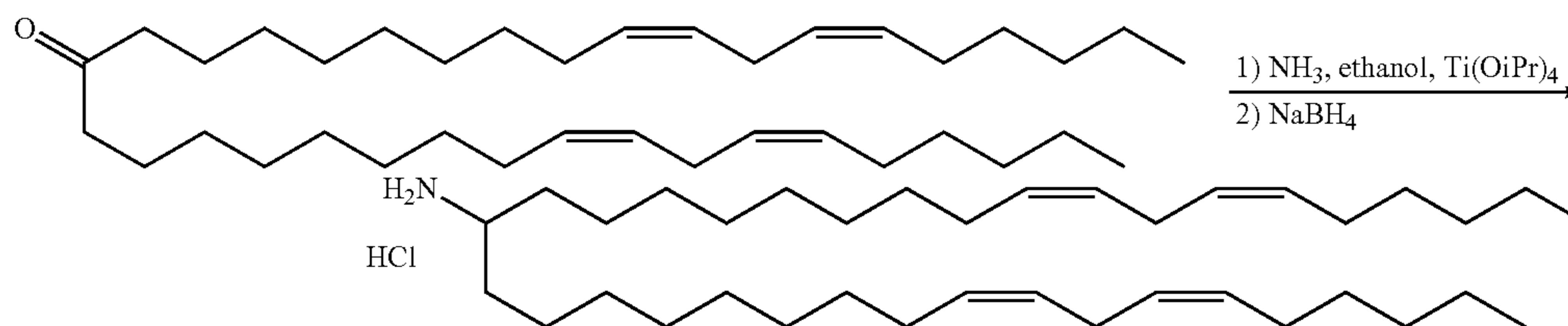
Scheme 10
