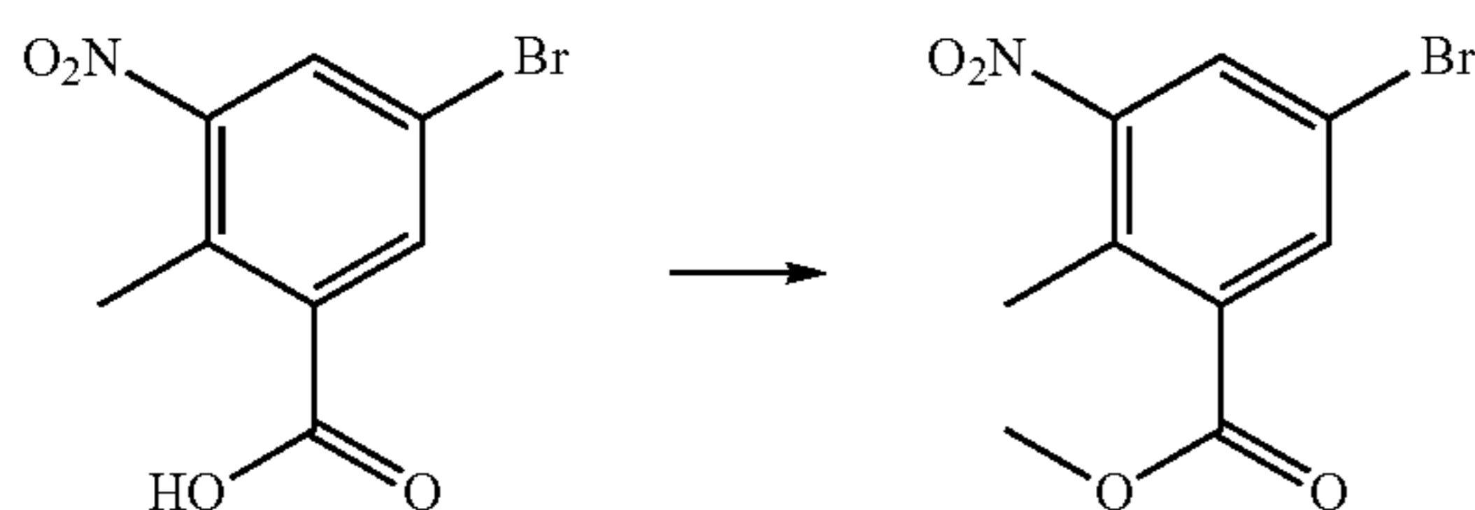
Methyl 5-bromo-2-methyl-3-nitrobenzoate
