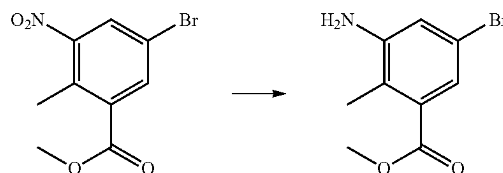
Methyl 3-amino-5-bromo-2-methylbenzoate
