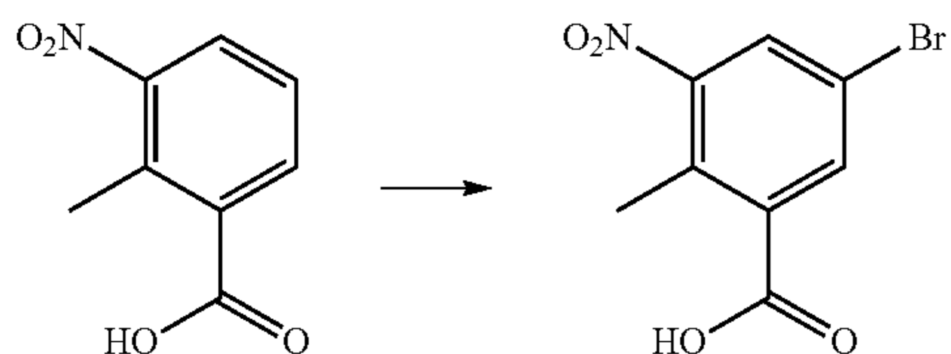
5-Bromo-2-methyl-3-nitrobenzoic acid
