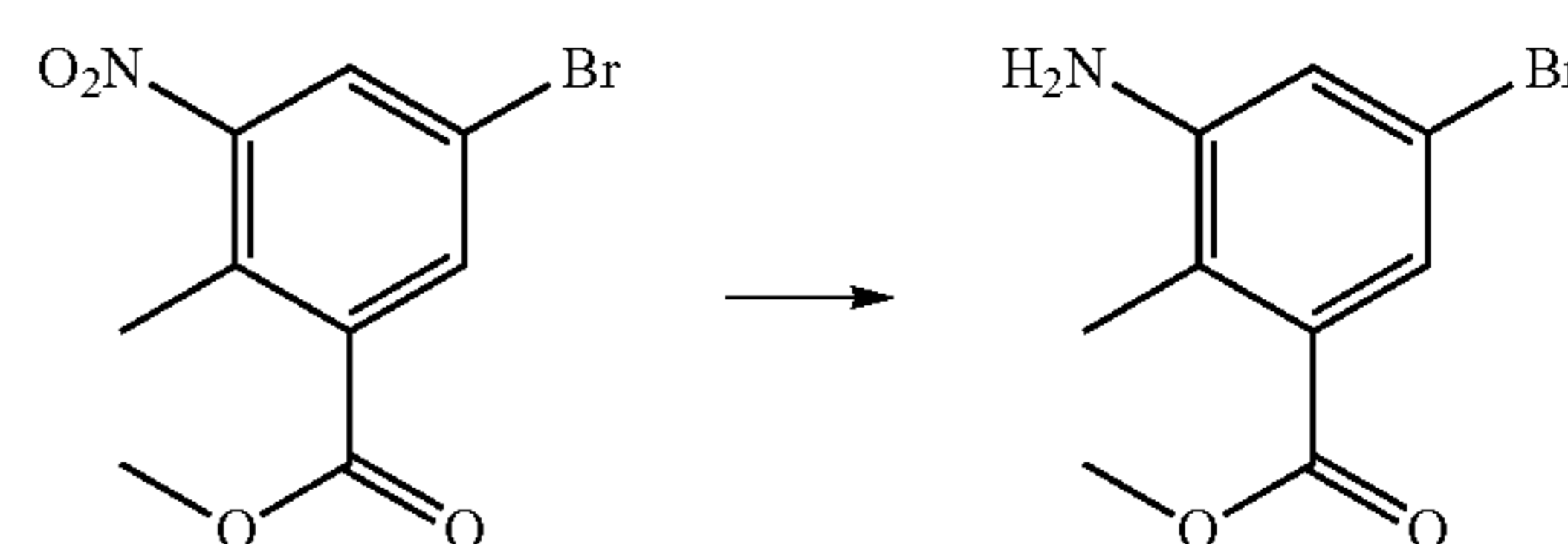
Methyl 3-amino-5-bromo-2-methylbenzoate
