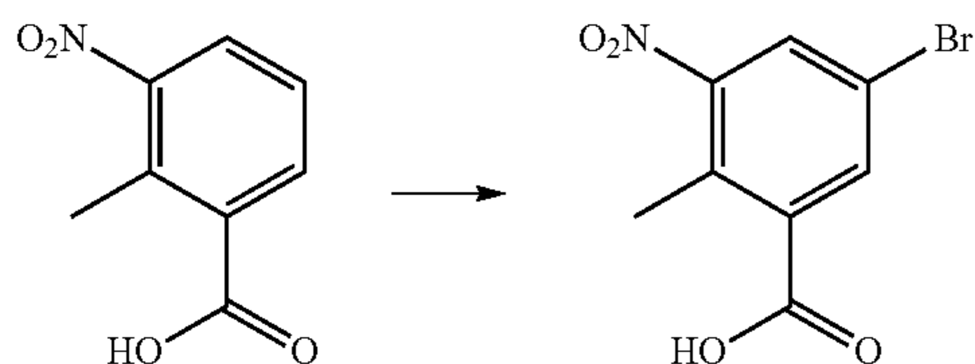
5-Bromo-2-methyl-3-nitrobenzoic acid
