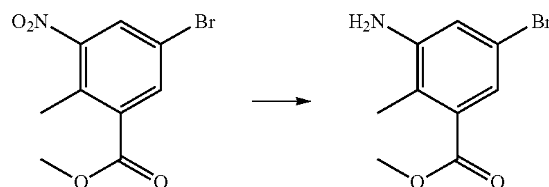
Methyl 3-amino-5-bromo-2-methylbenzoate
