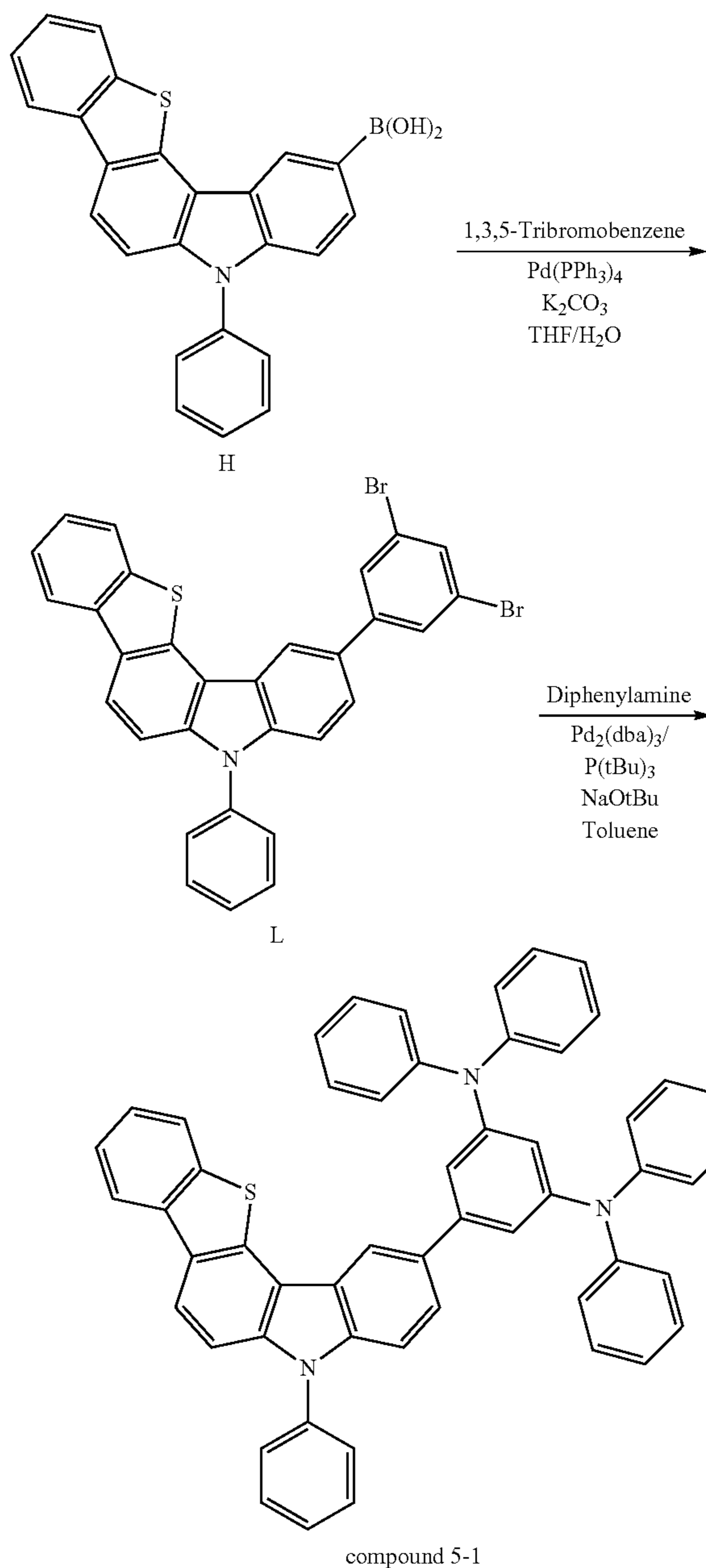
[Reaction Scheme 5]
