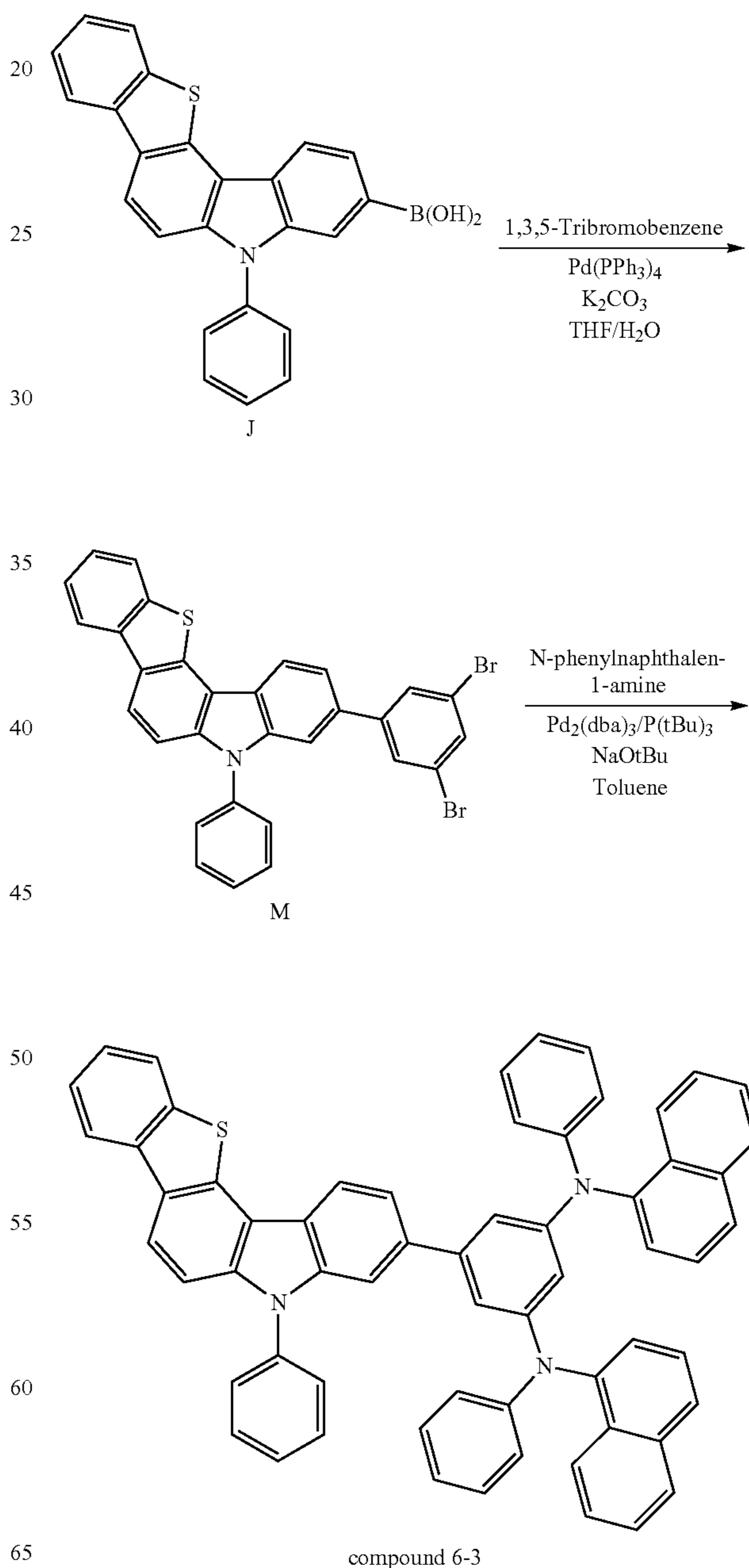
[Reaction Scheme 6]
