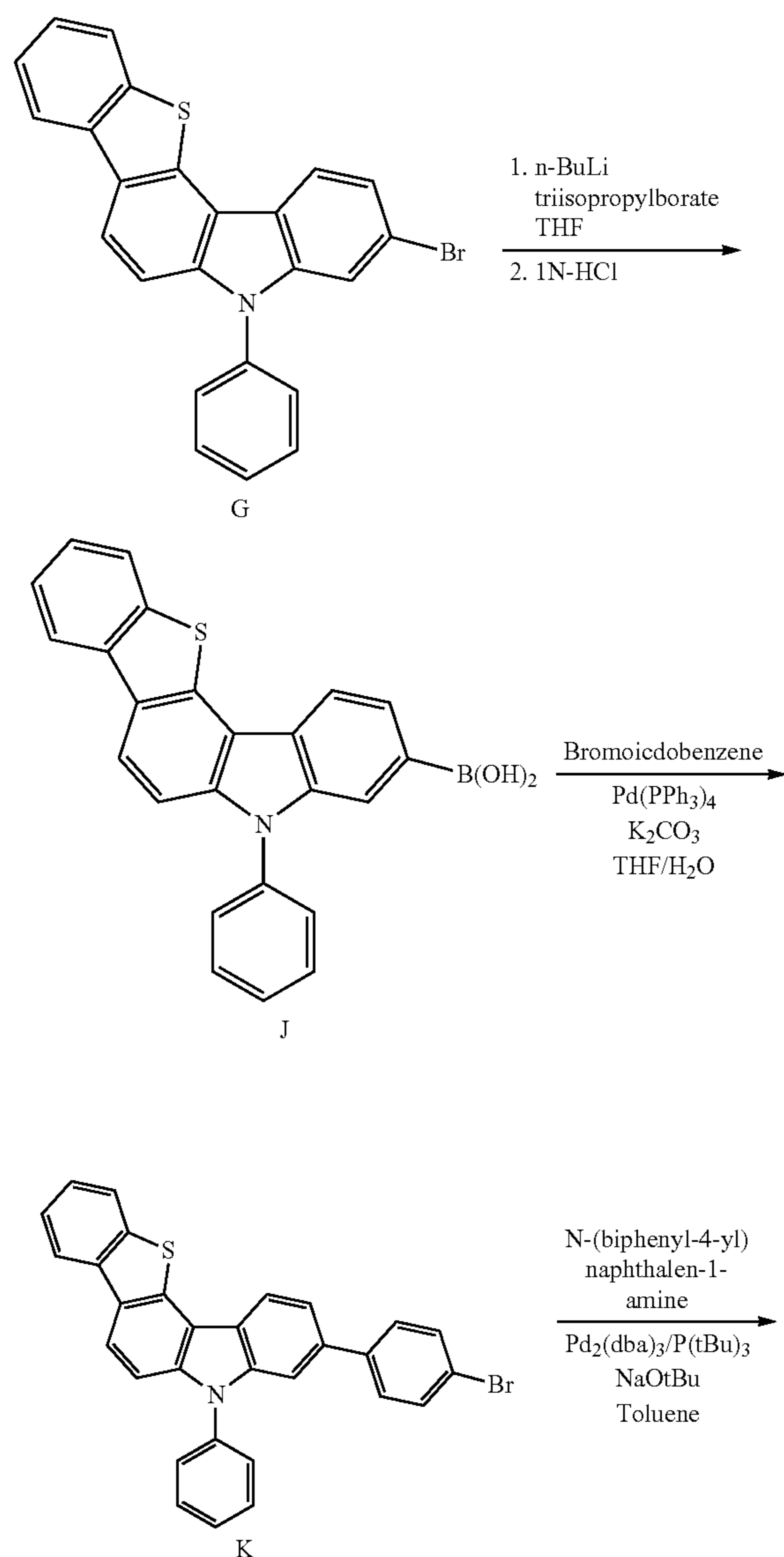
[Reaction Scheme 4]
