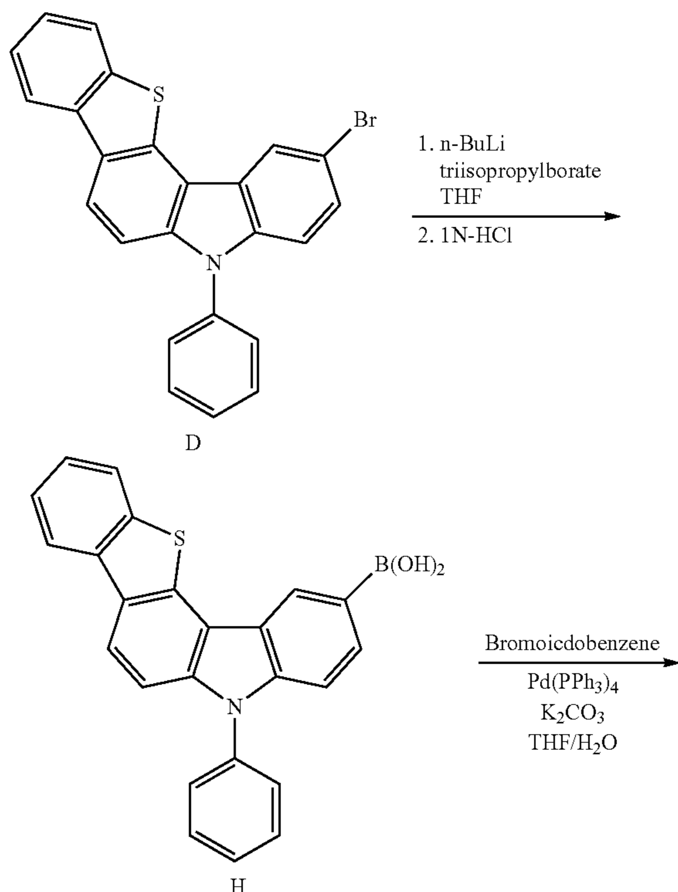
[Reaction Scheme 3]
