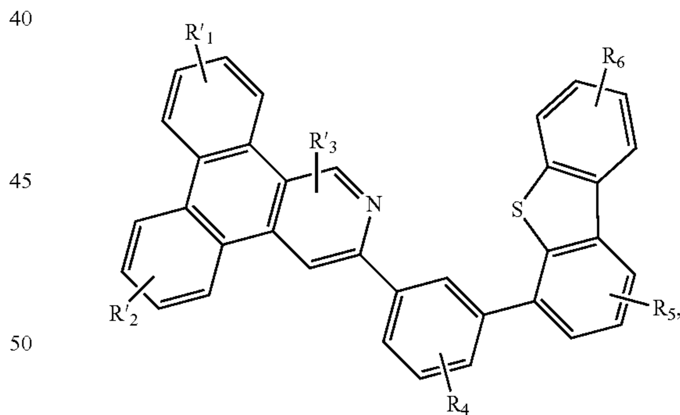
Compound 3G
