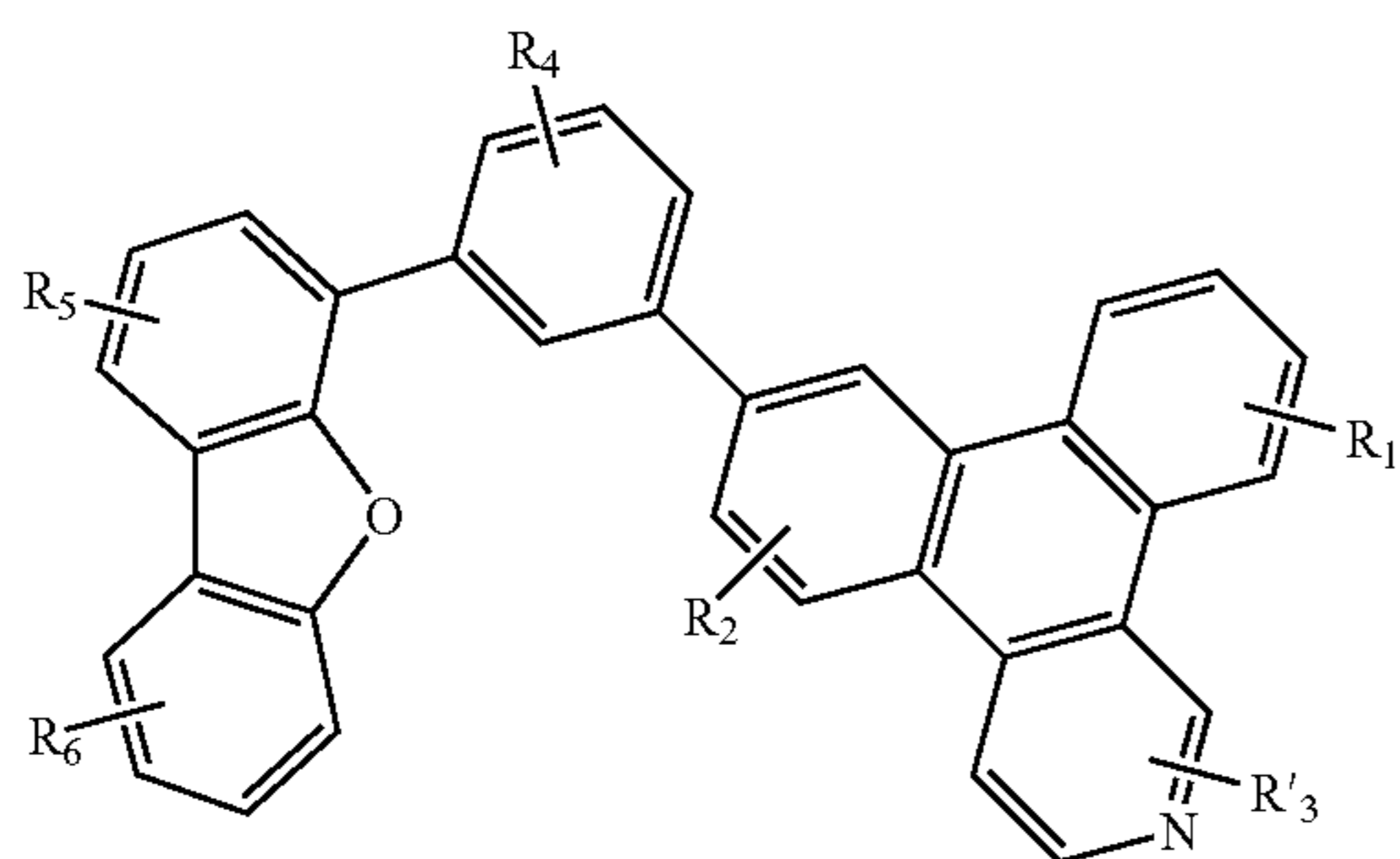
Compound 33G
