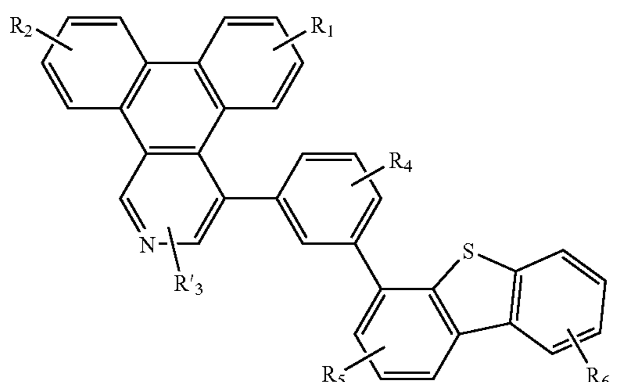
Compound 18G
