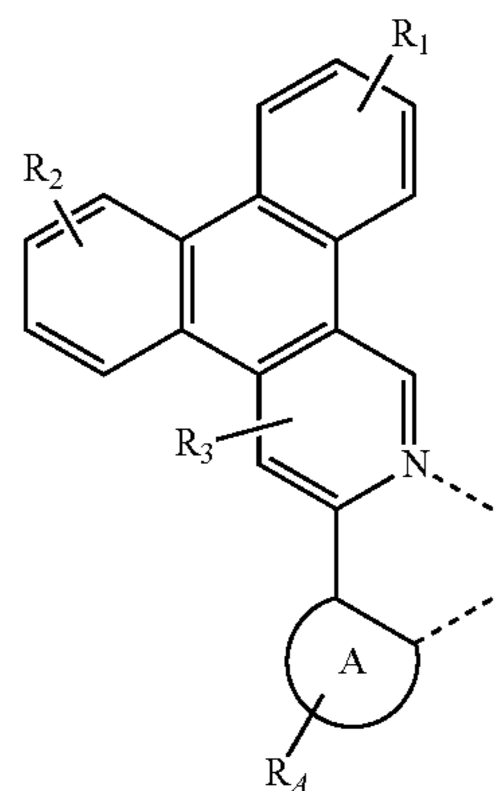
FORMULA I
