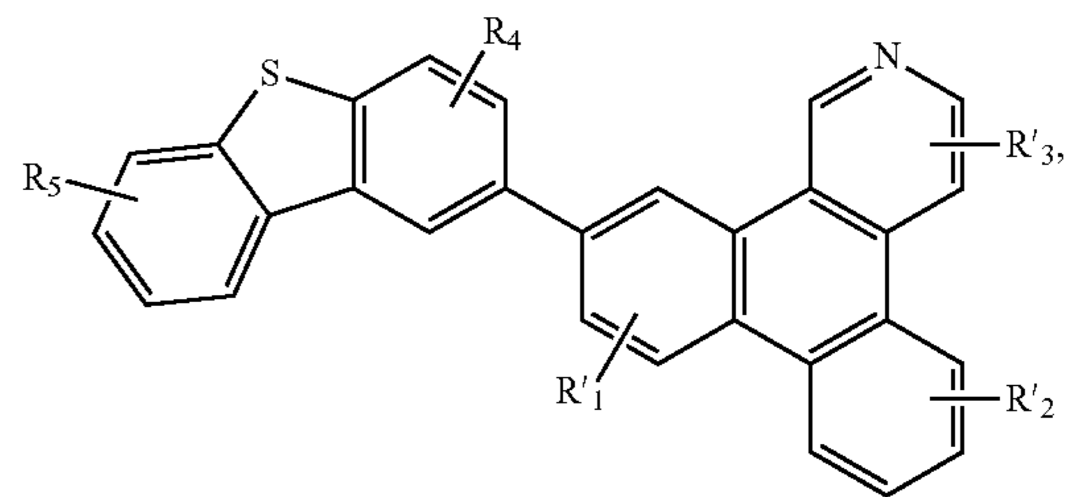
Compound 51G
