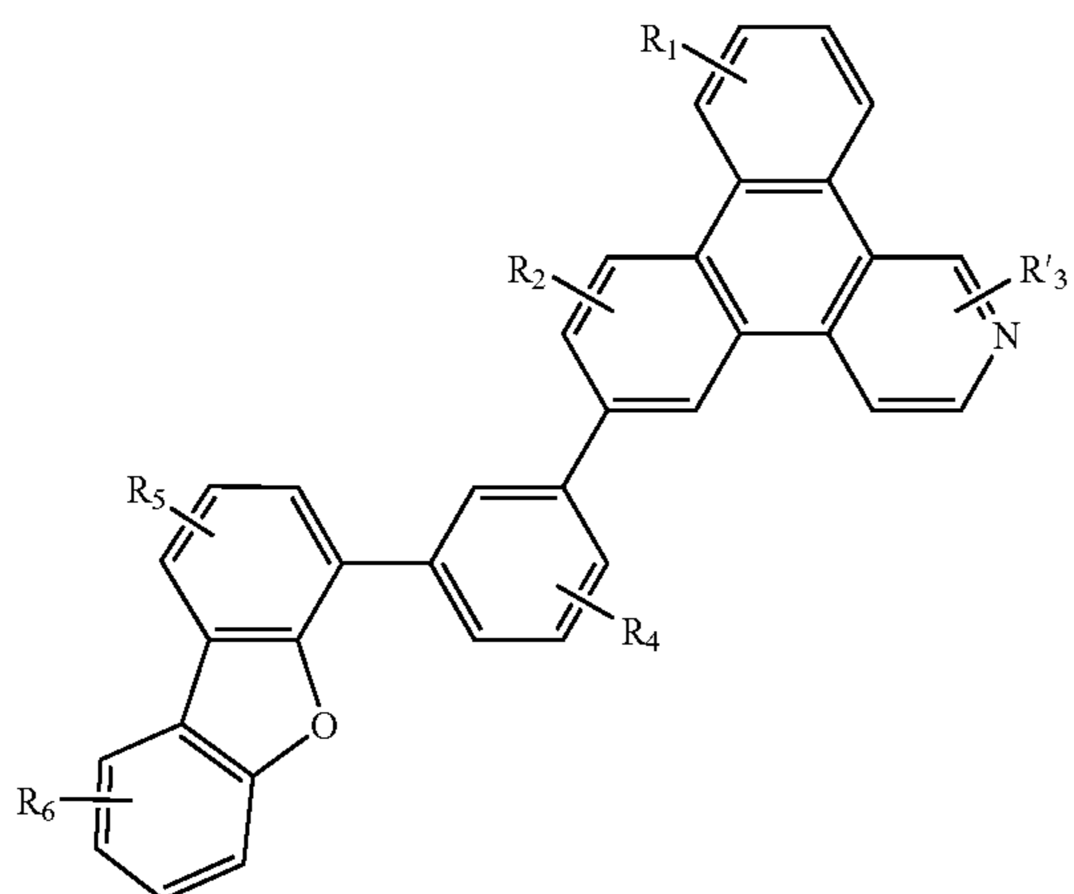
Compound 34G
