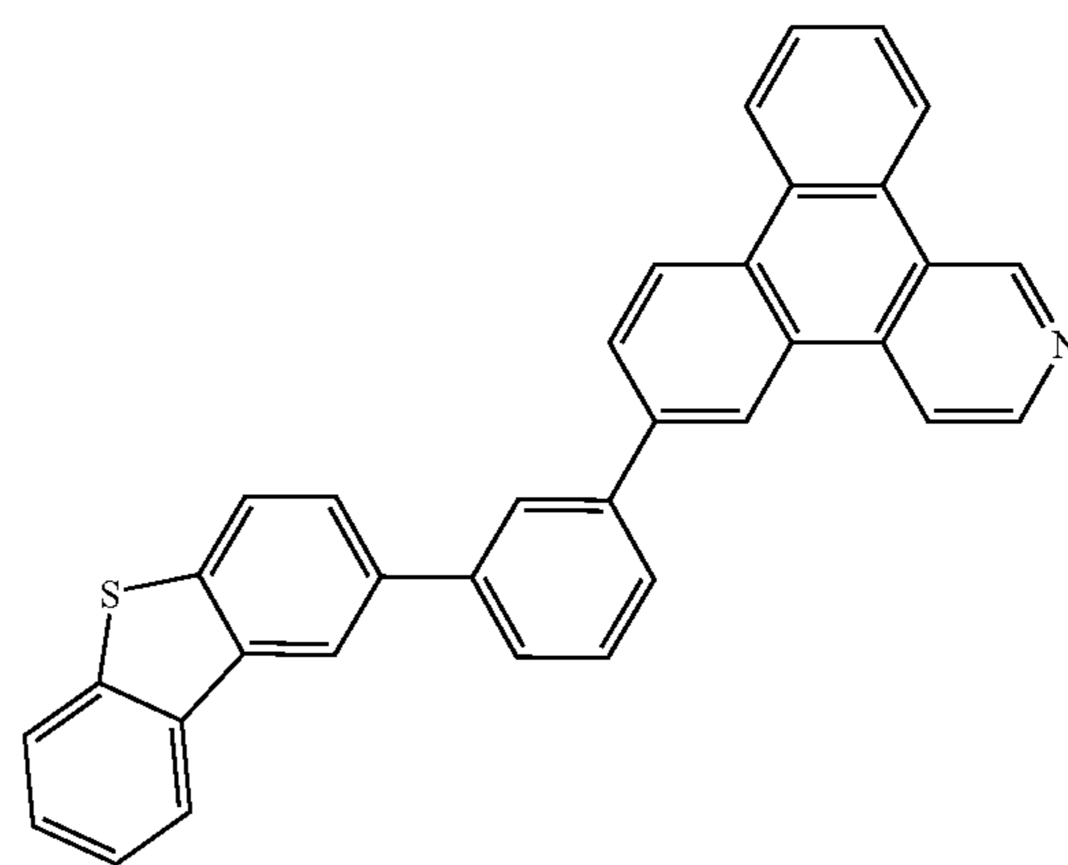
Compound 26
