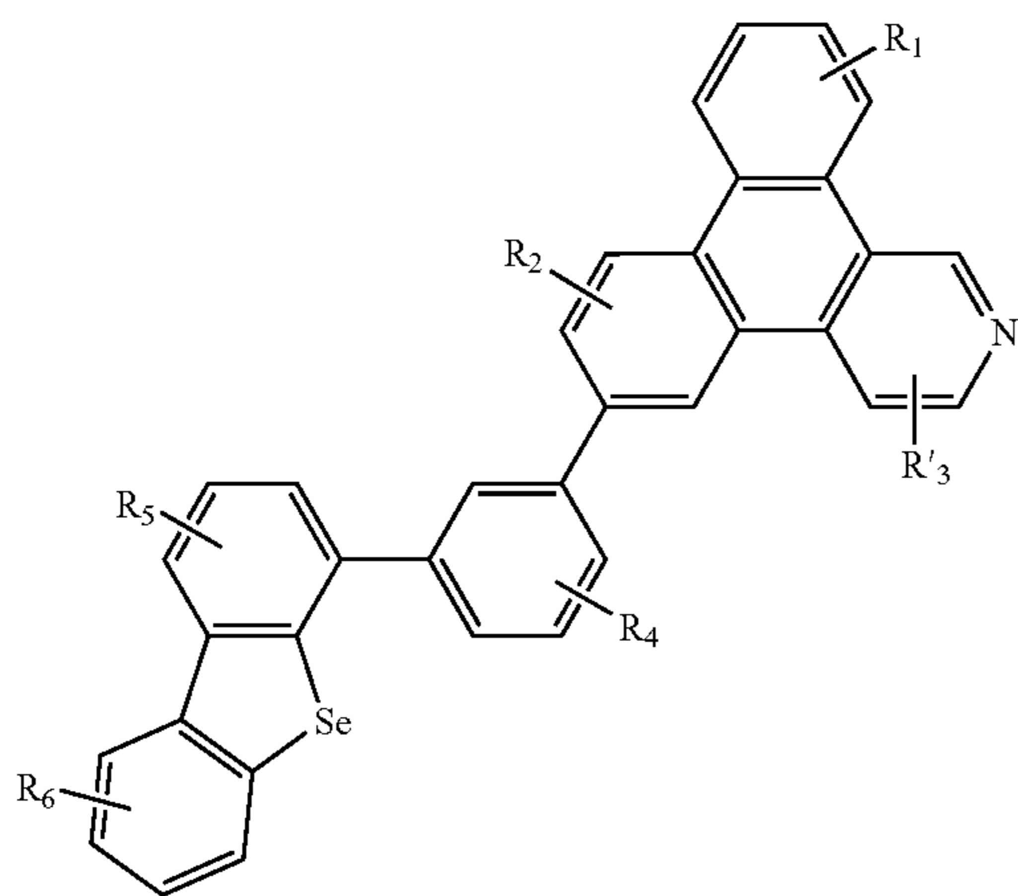
Compound 58G
