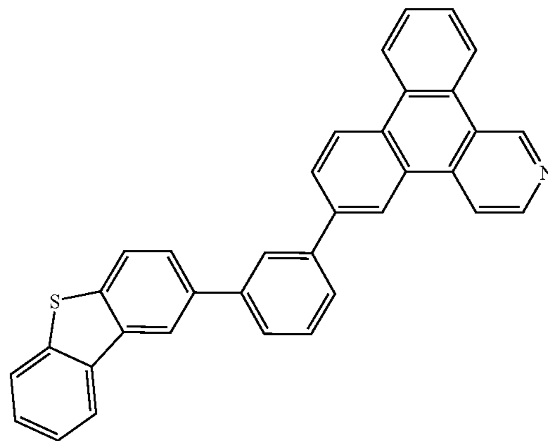
Compound 26
