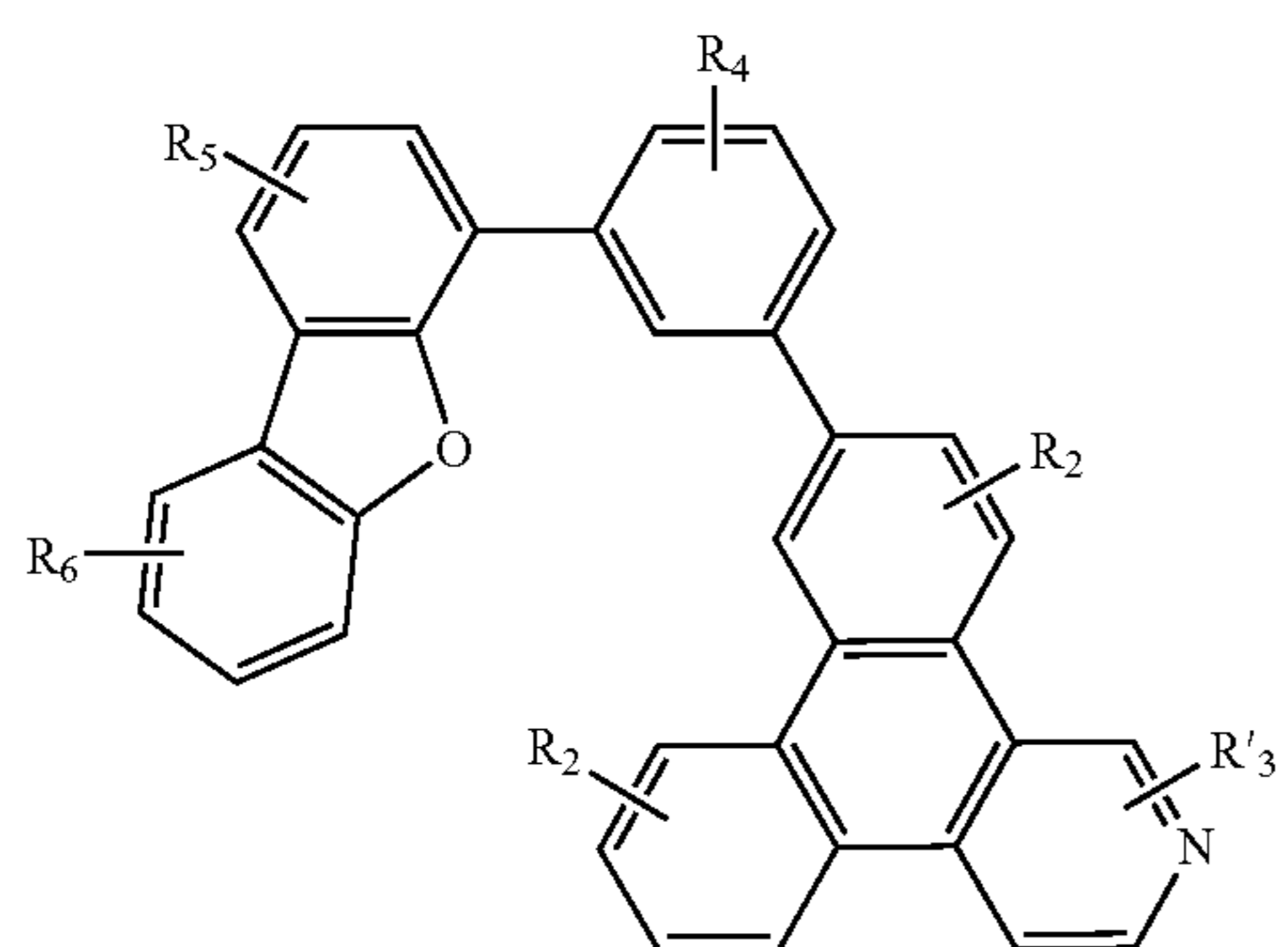
Compound 33G
