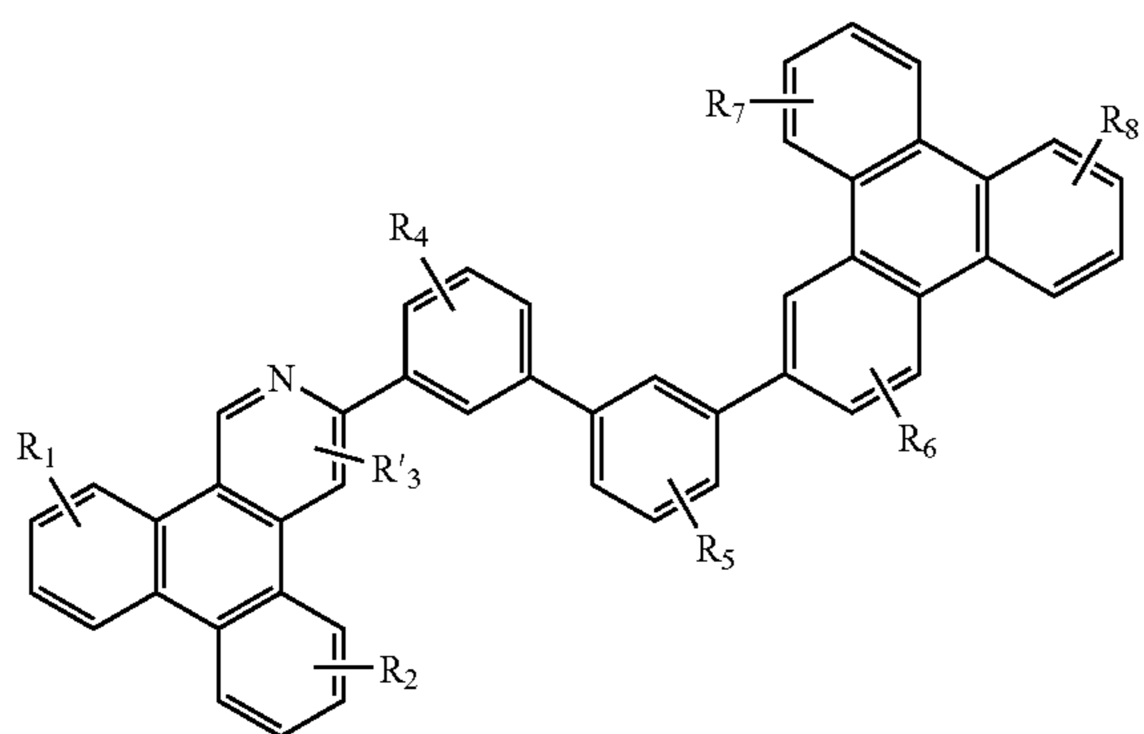
Compound 8G
