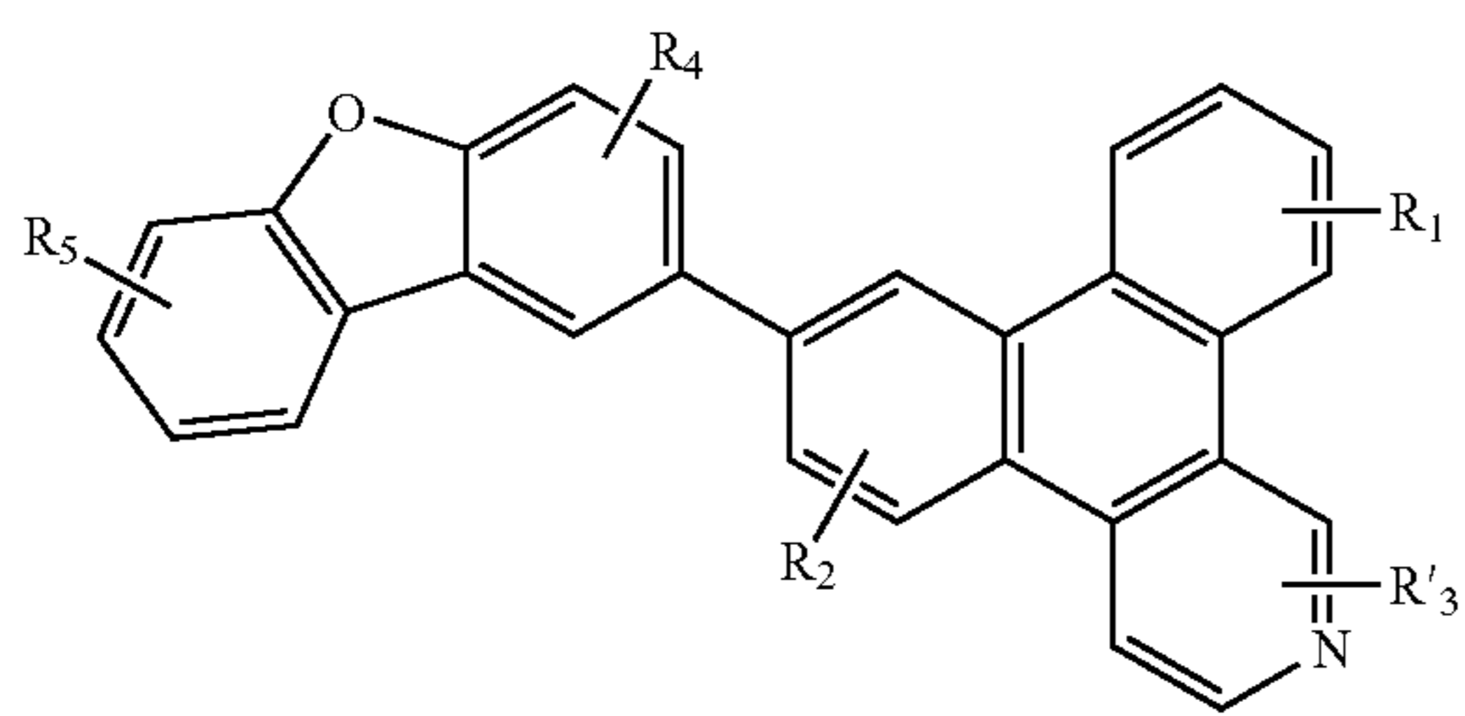
Compound 41G
