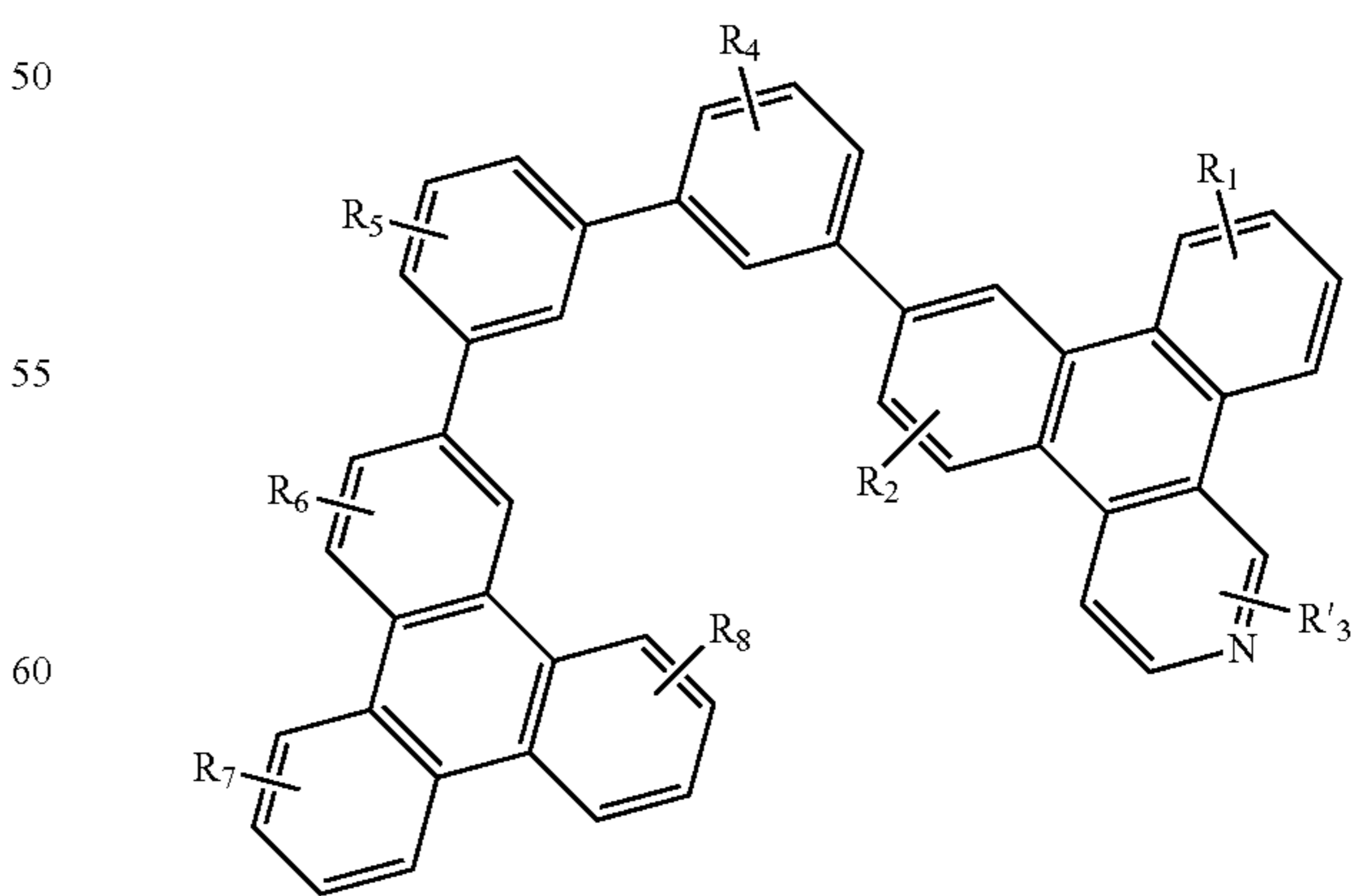
Compound 45G
