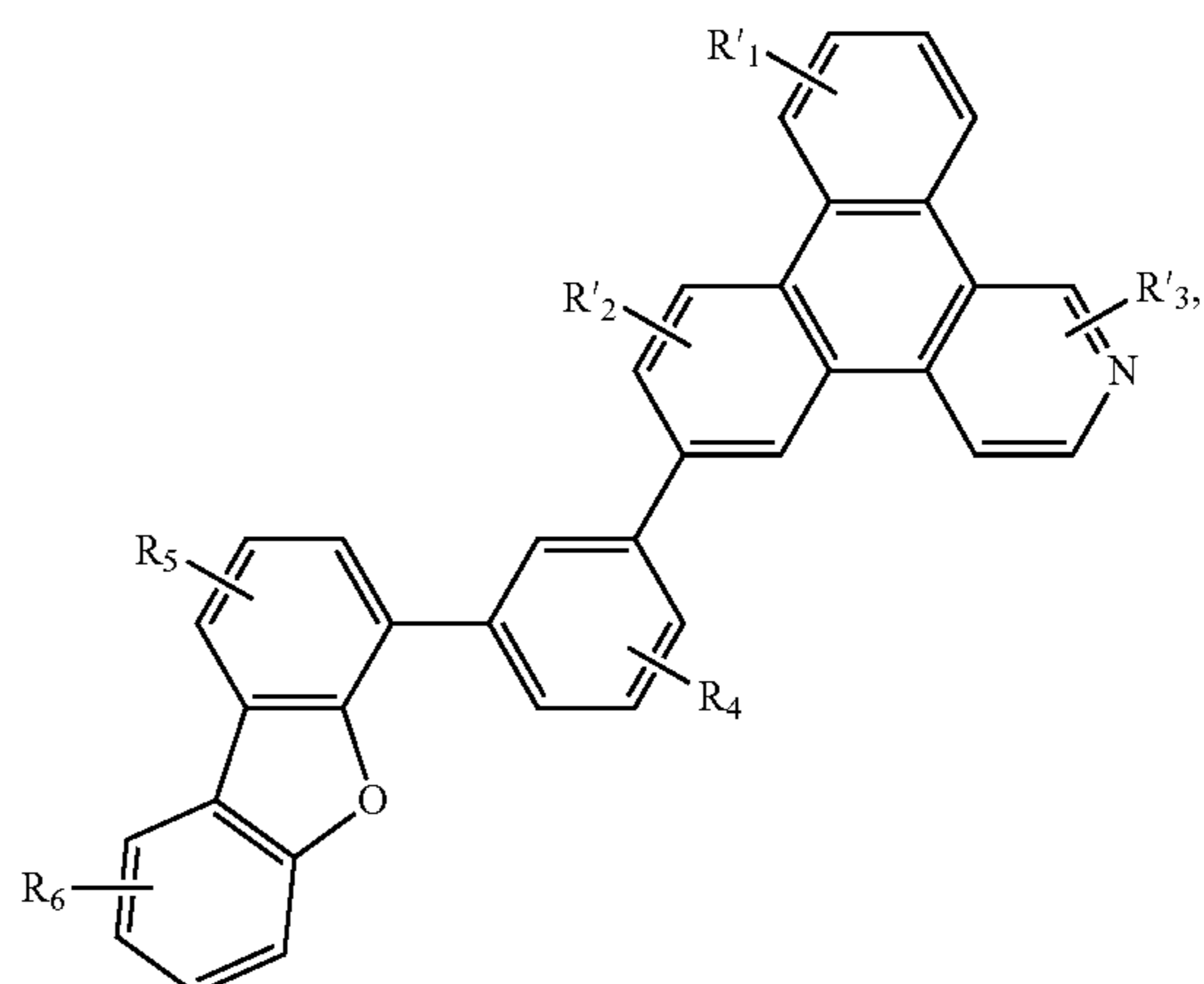
Compound 34G
