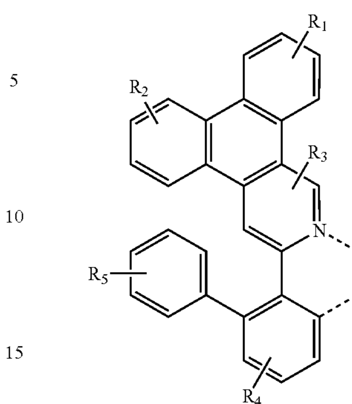
Compound 71G
