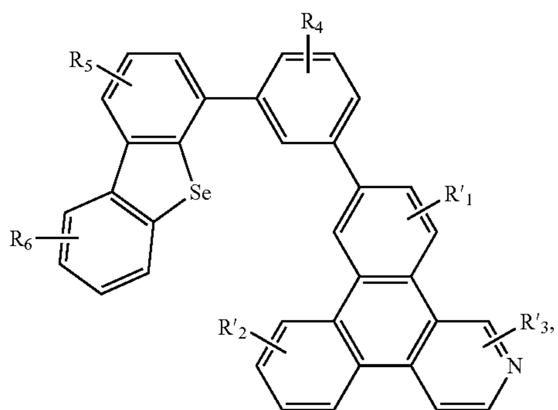
Compound 57G
