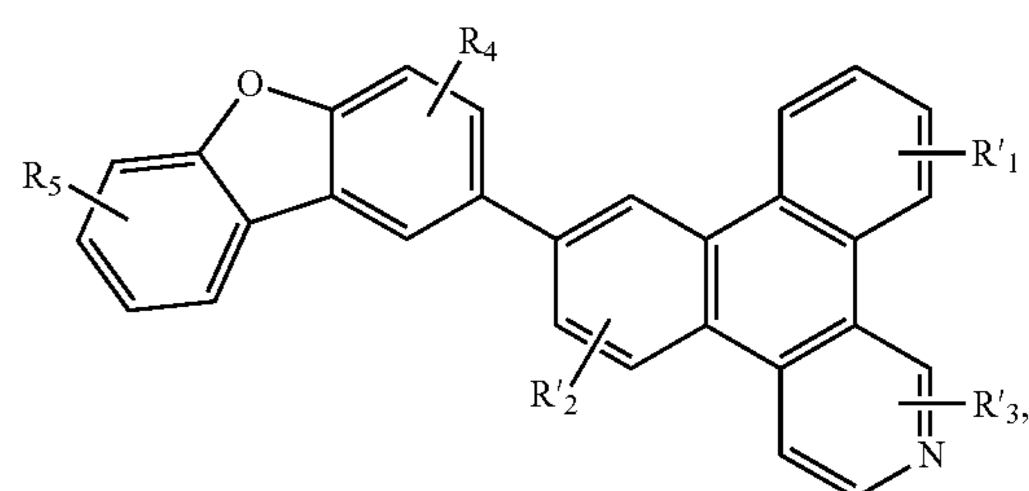
Compound 41G
