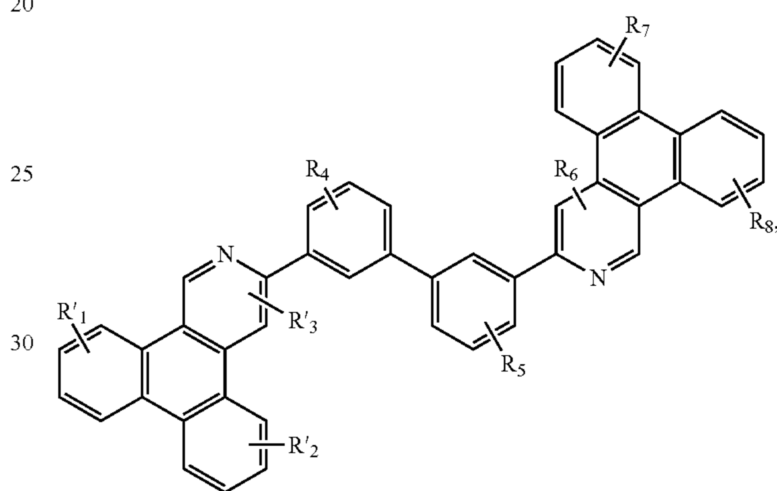
Compound 10G
