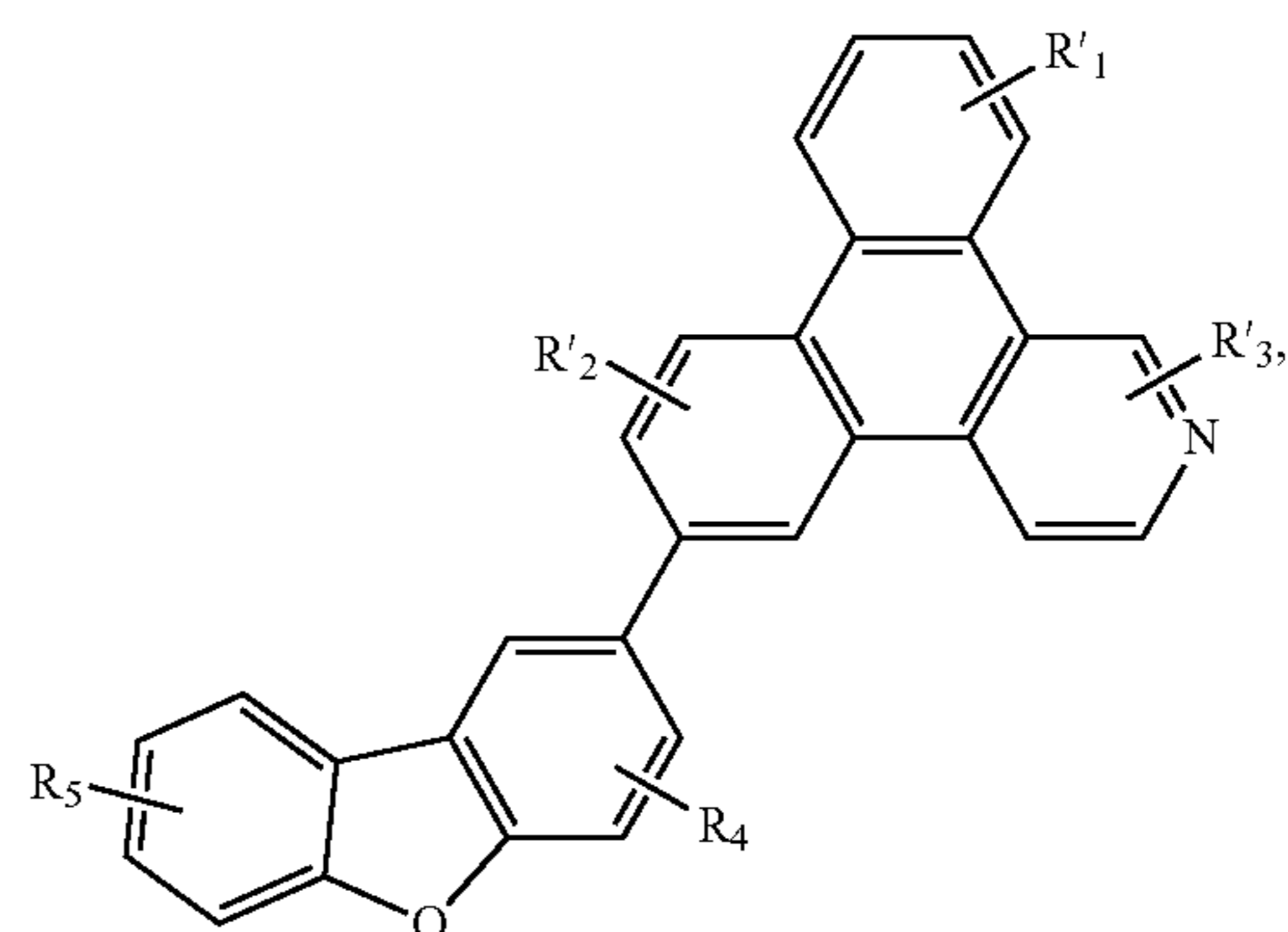
Compound 42G
