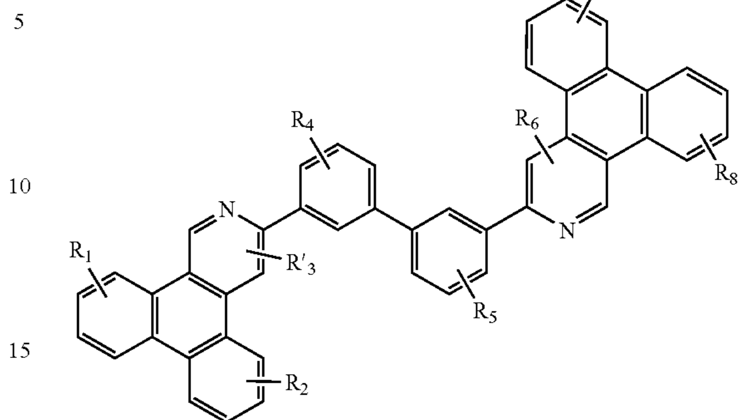
Compound 7G
