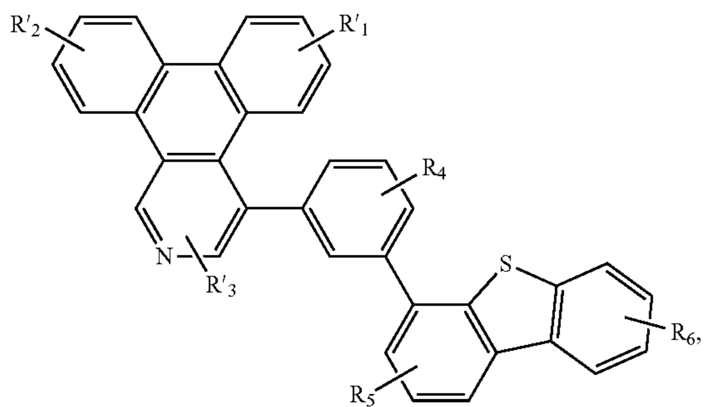
Compound 17G
