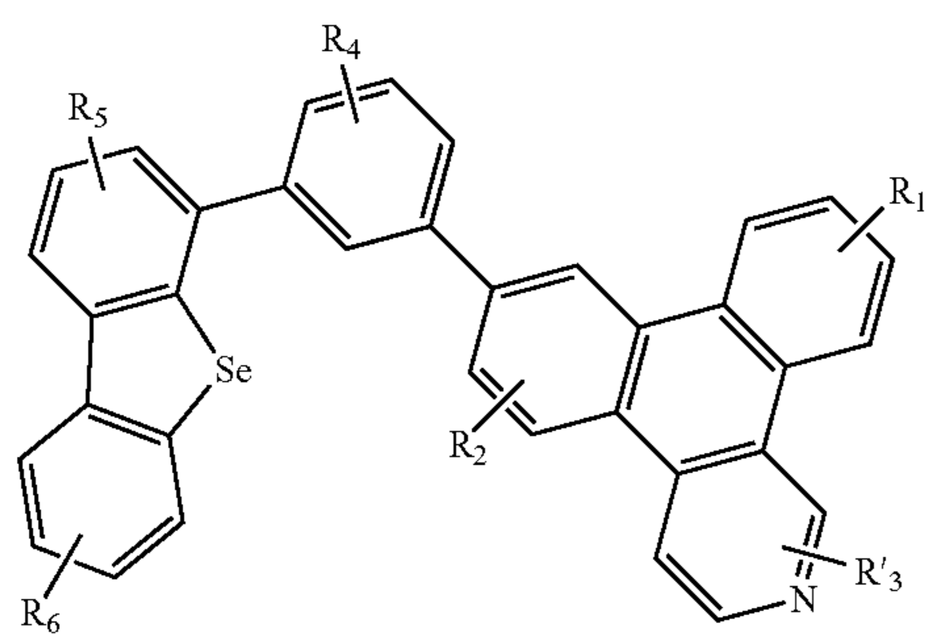
Compound 57G
