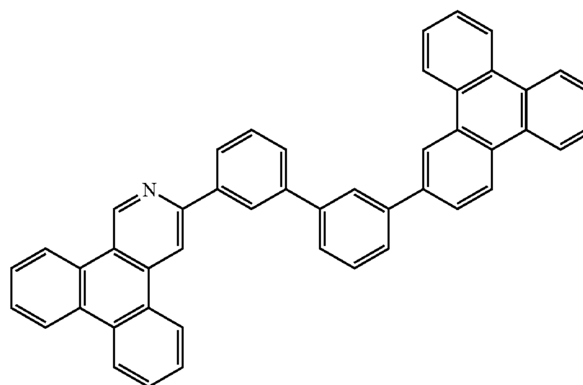
Compound 8
