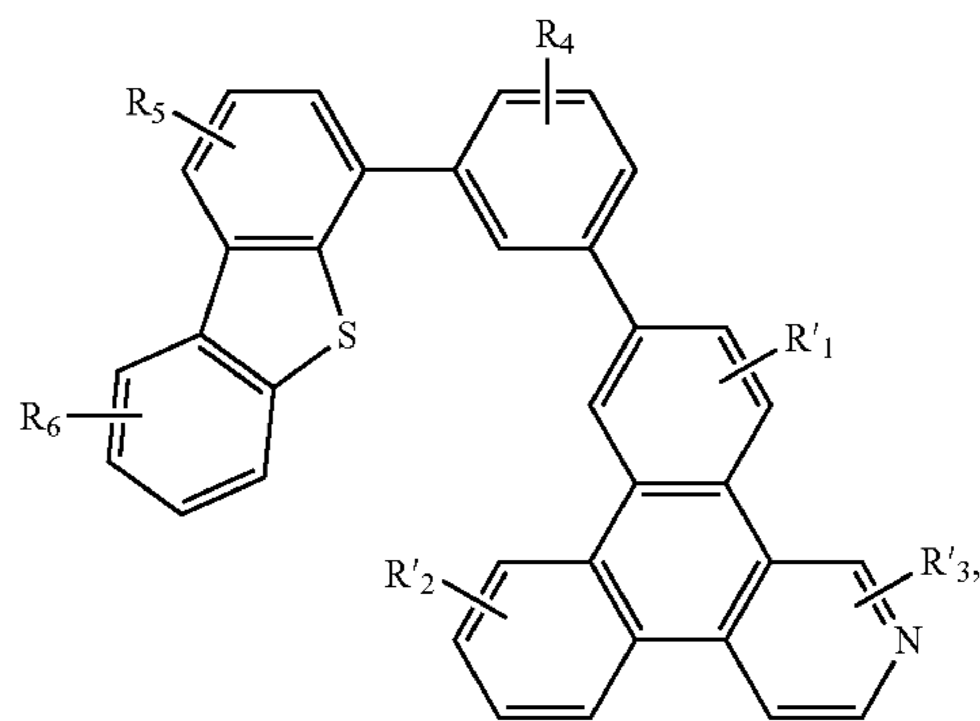
Compound 21G
