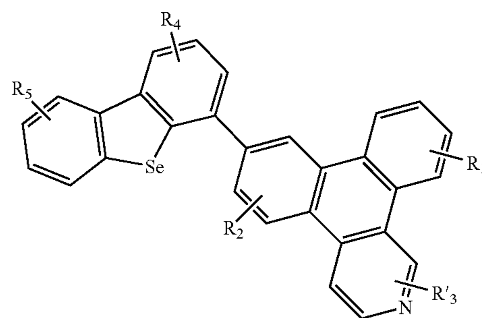
Compound 61G
