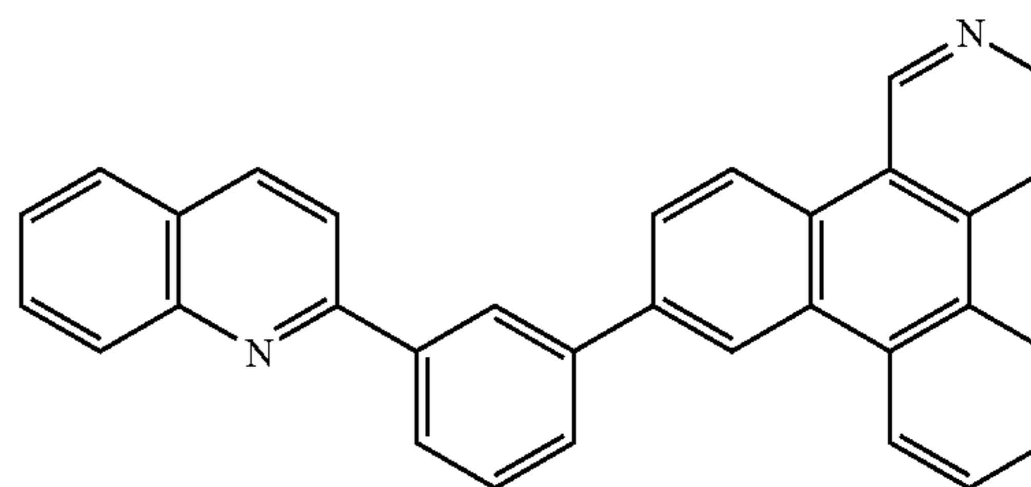
Compound 68
