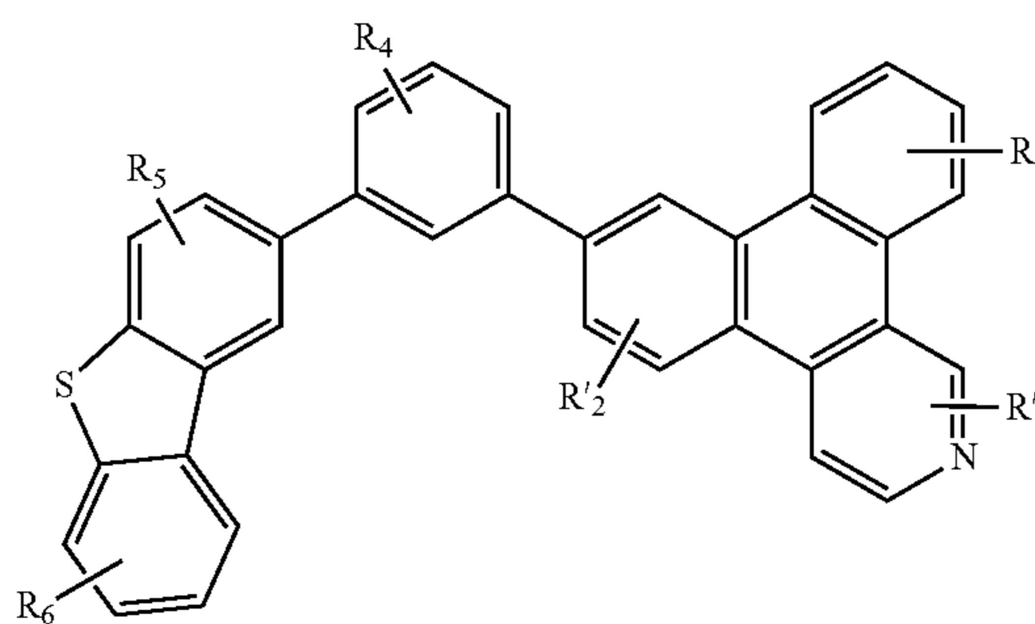
Compound 26G
