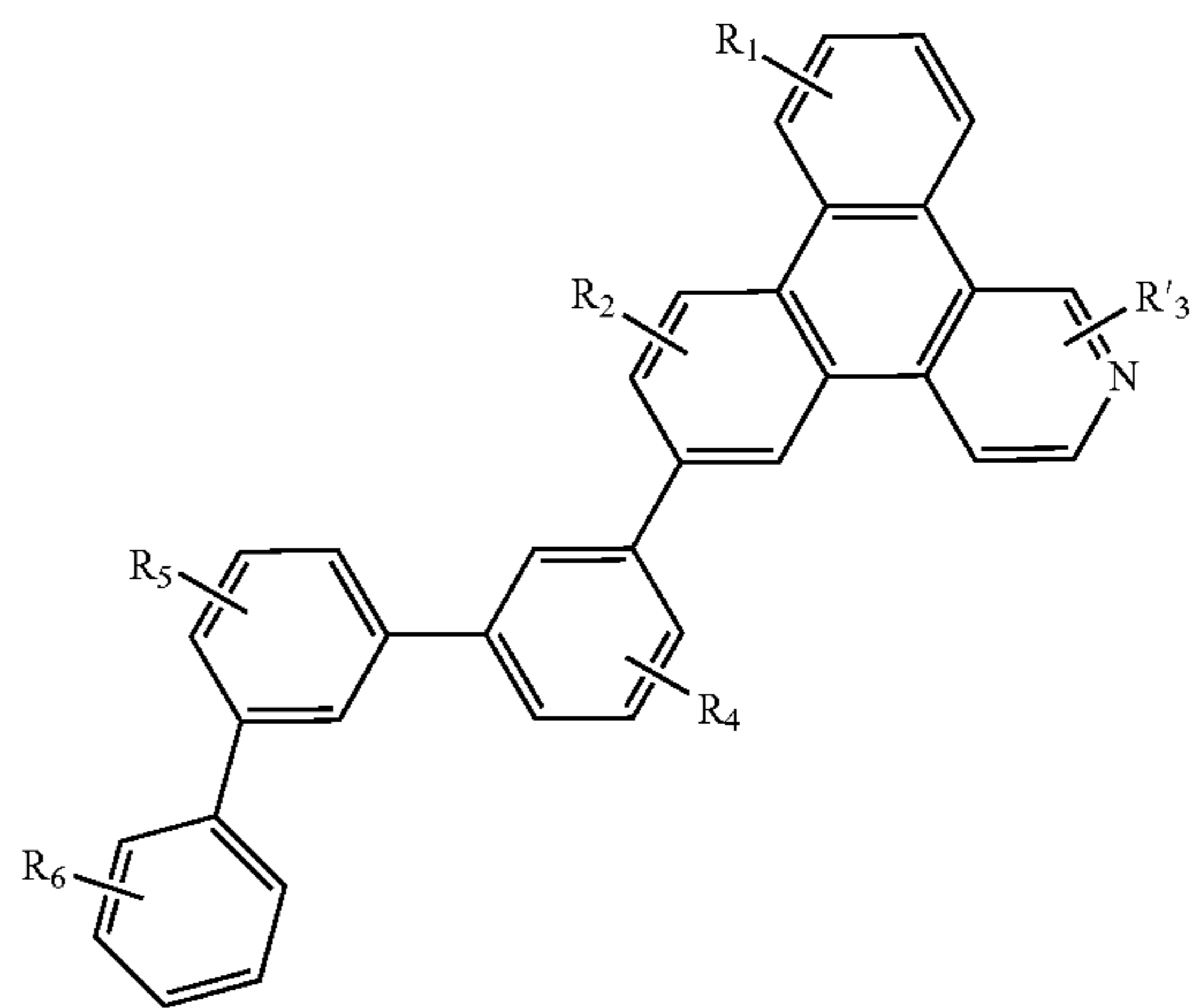
Compound 30G
