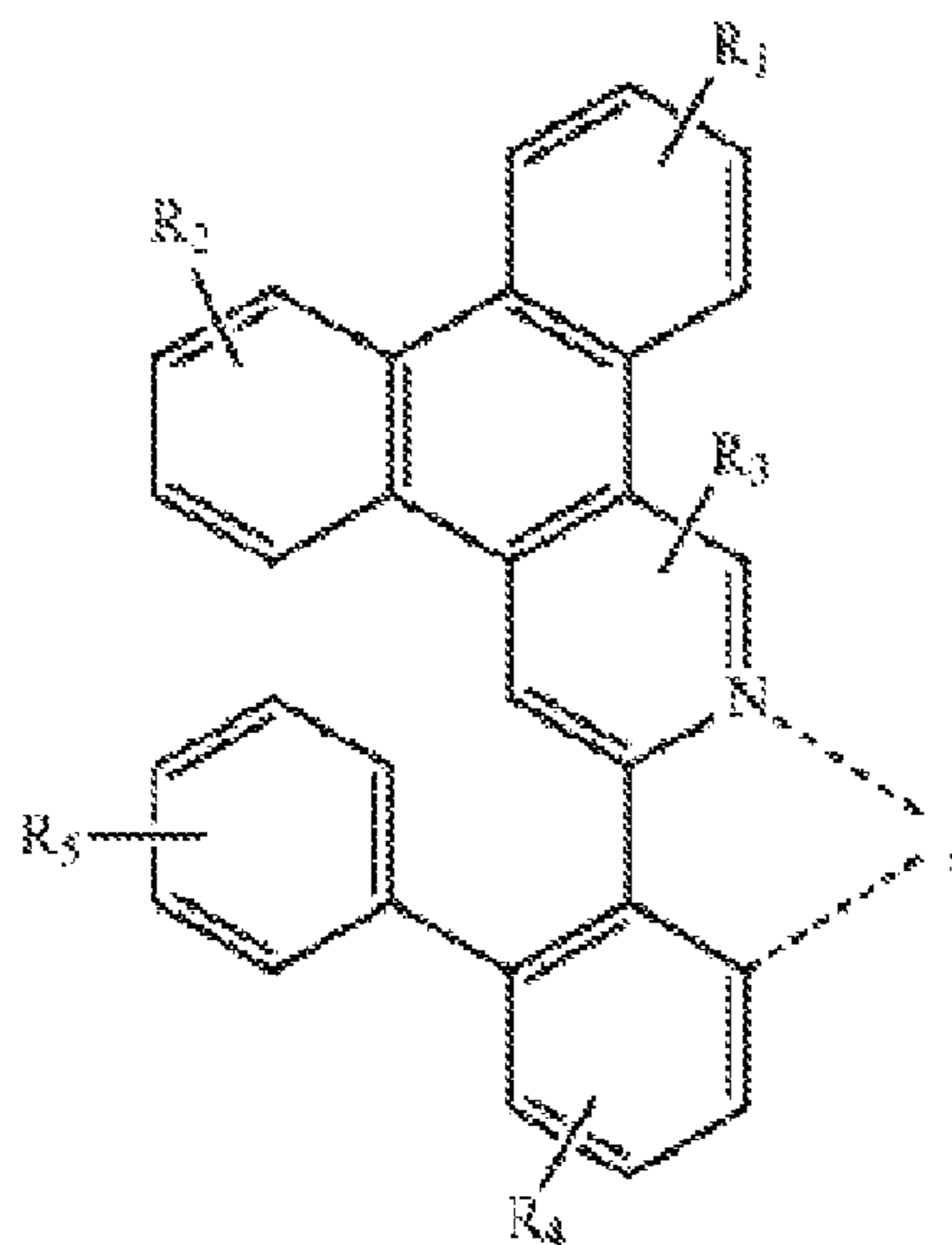
Compound 74G
