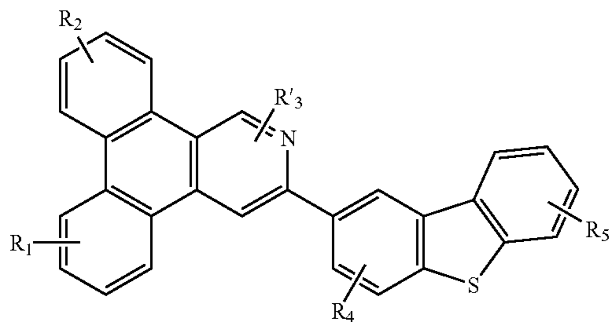
Compound 15G
