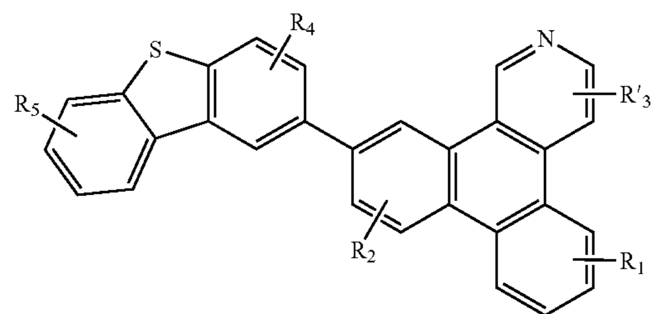
Compound 52G
