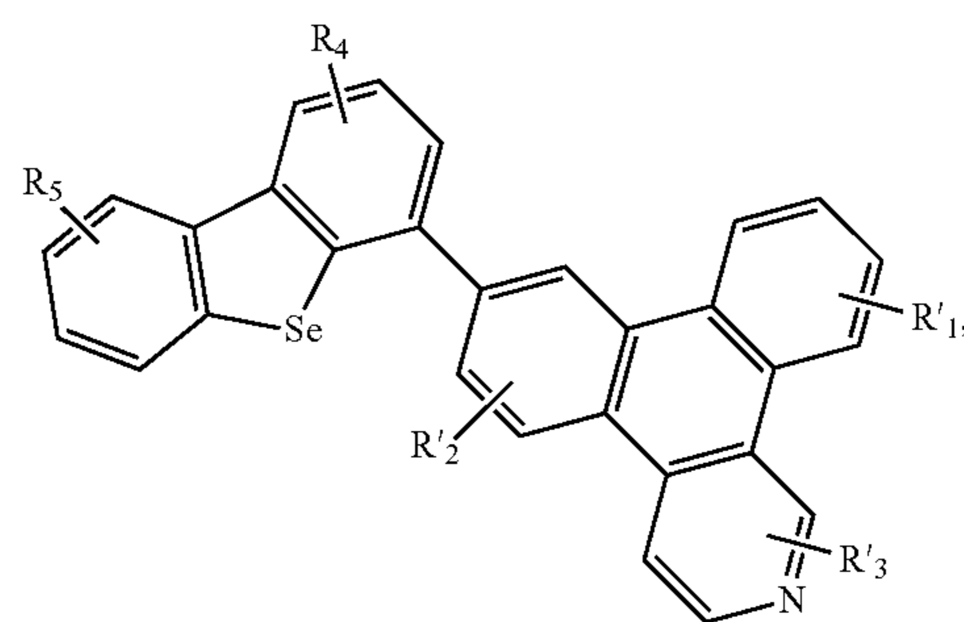
Compound 61G
