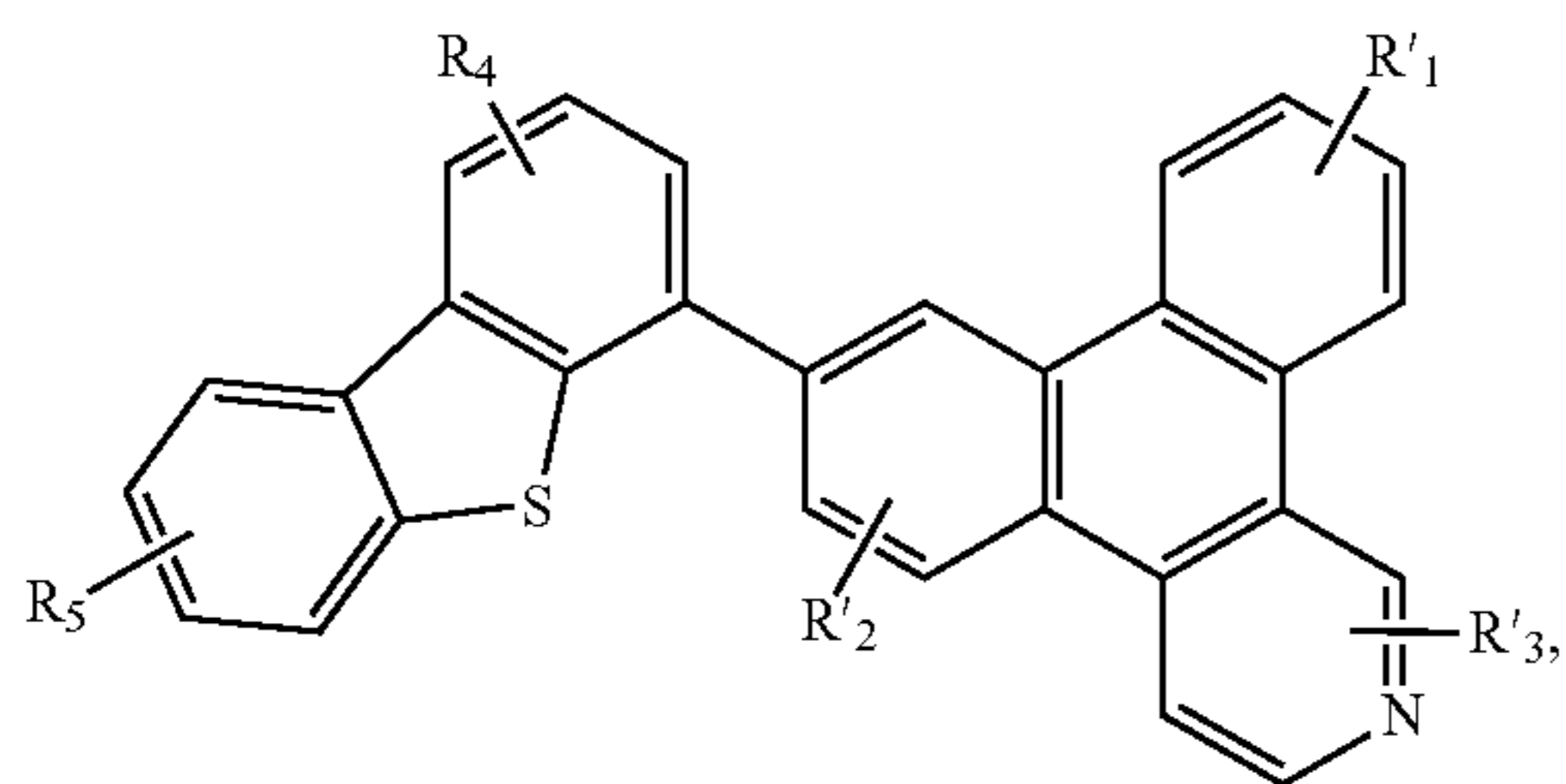
Compound 49G
