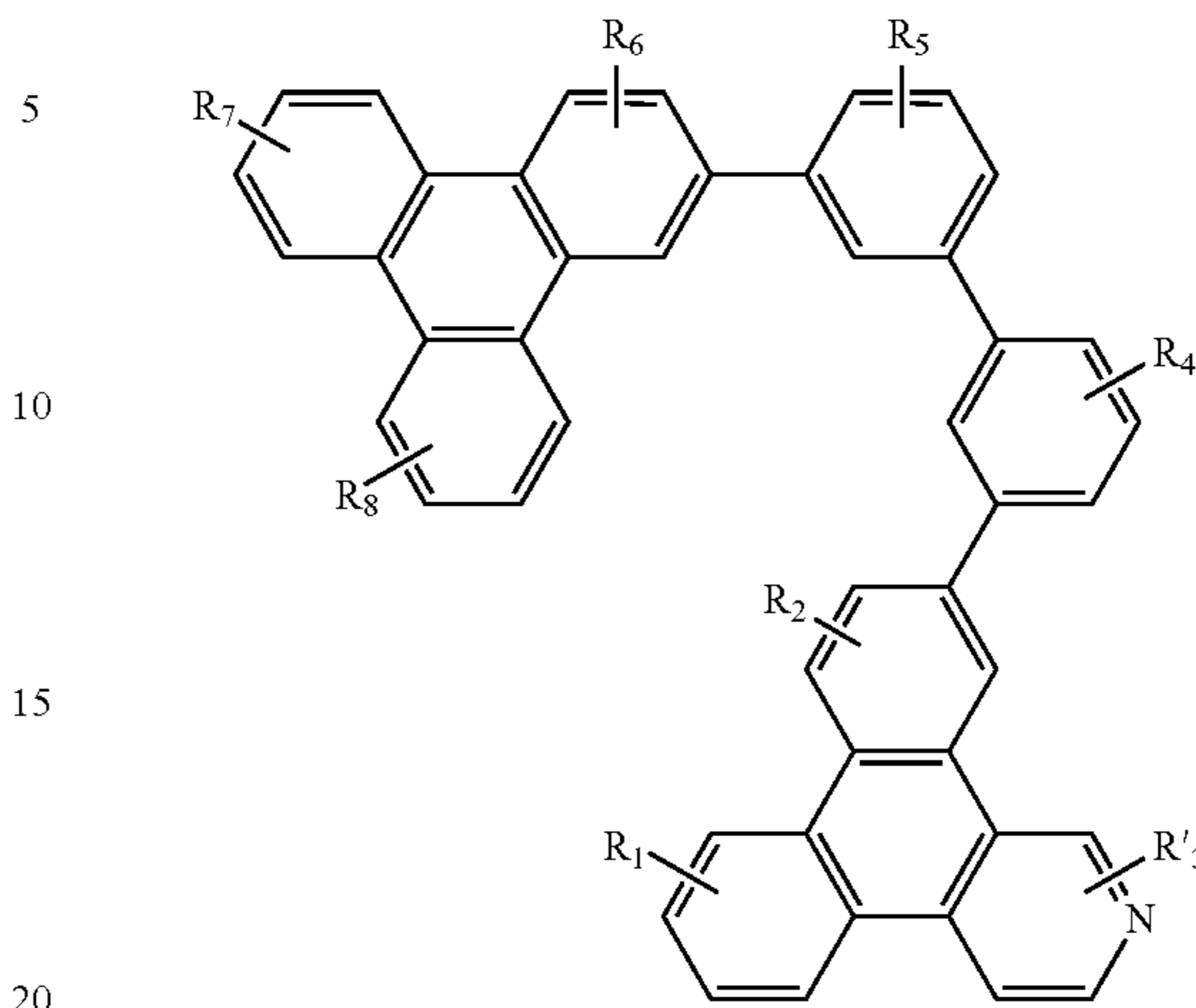
Compound 43G
