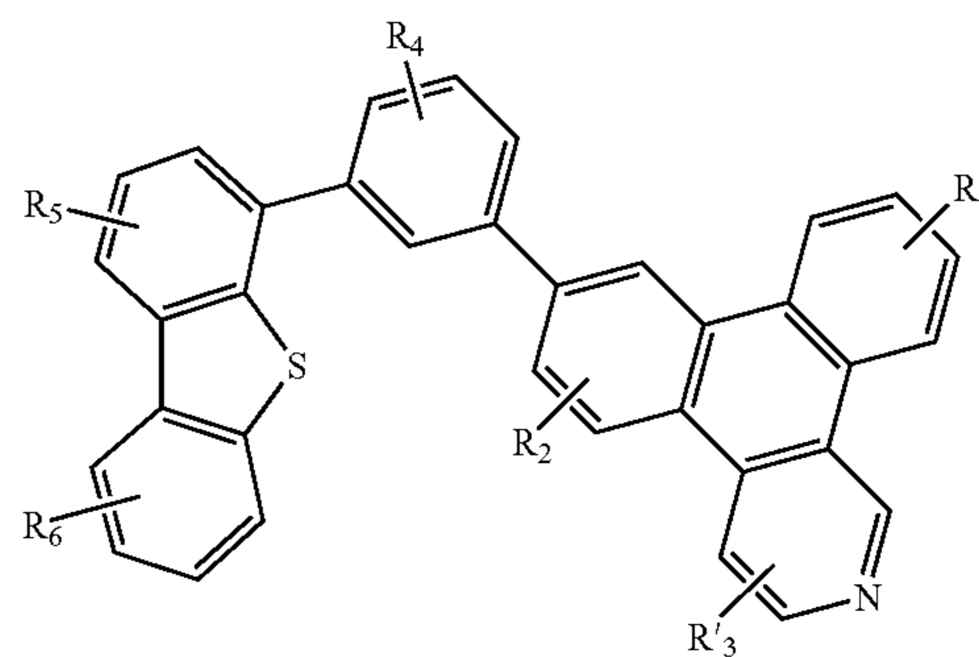
Compound 21G
