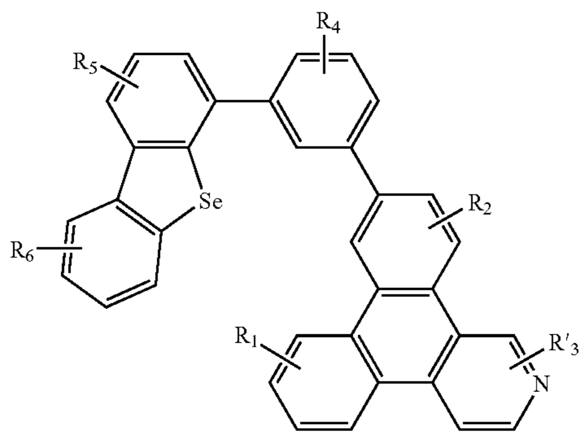
Compound 57G
