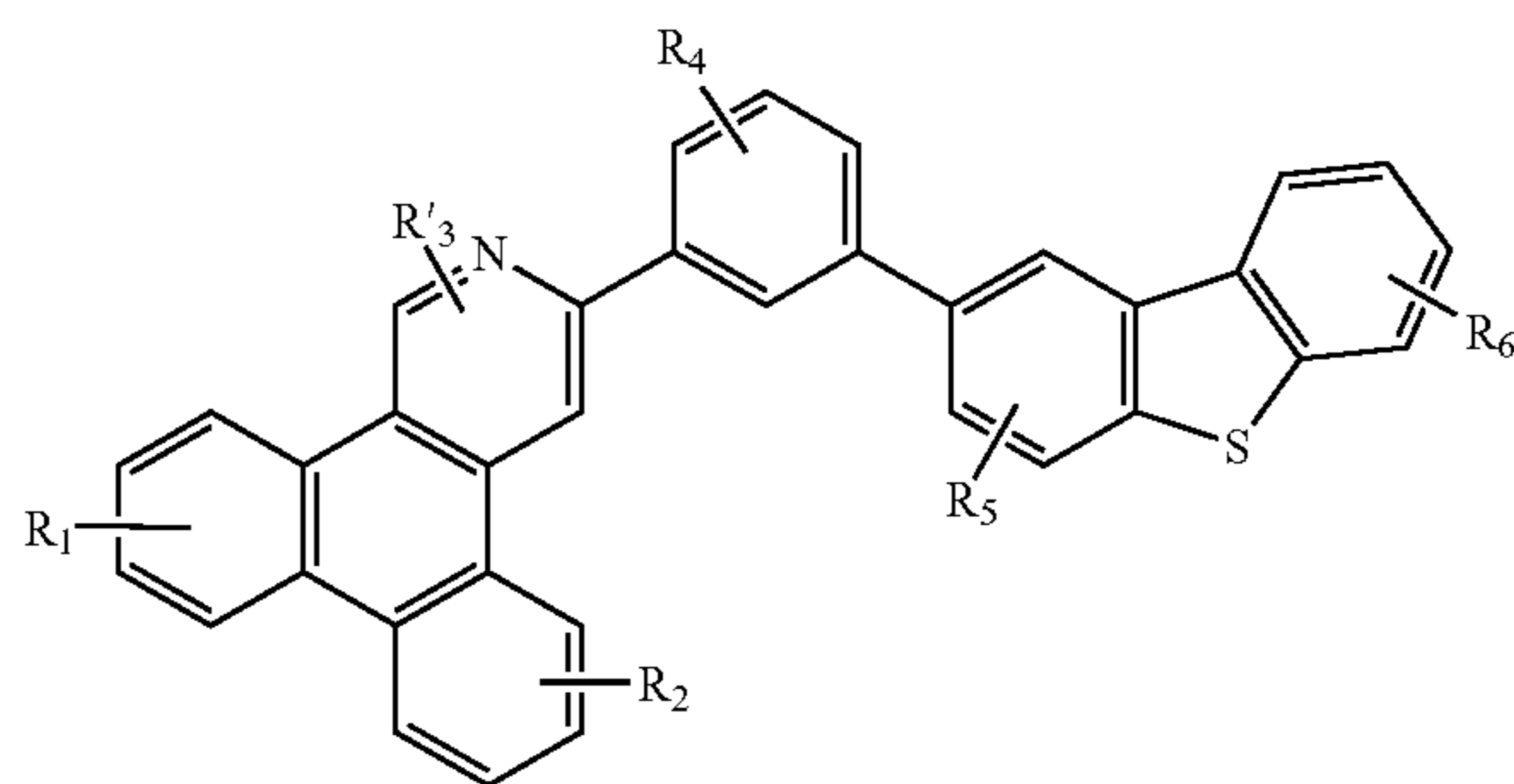
Compound 13G
