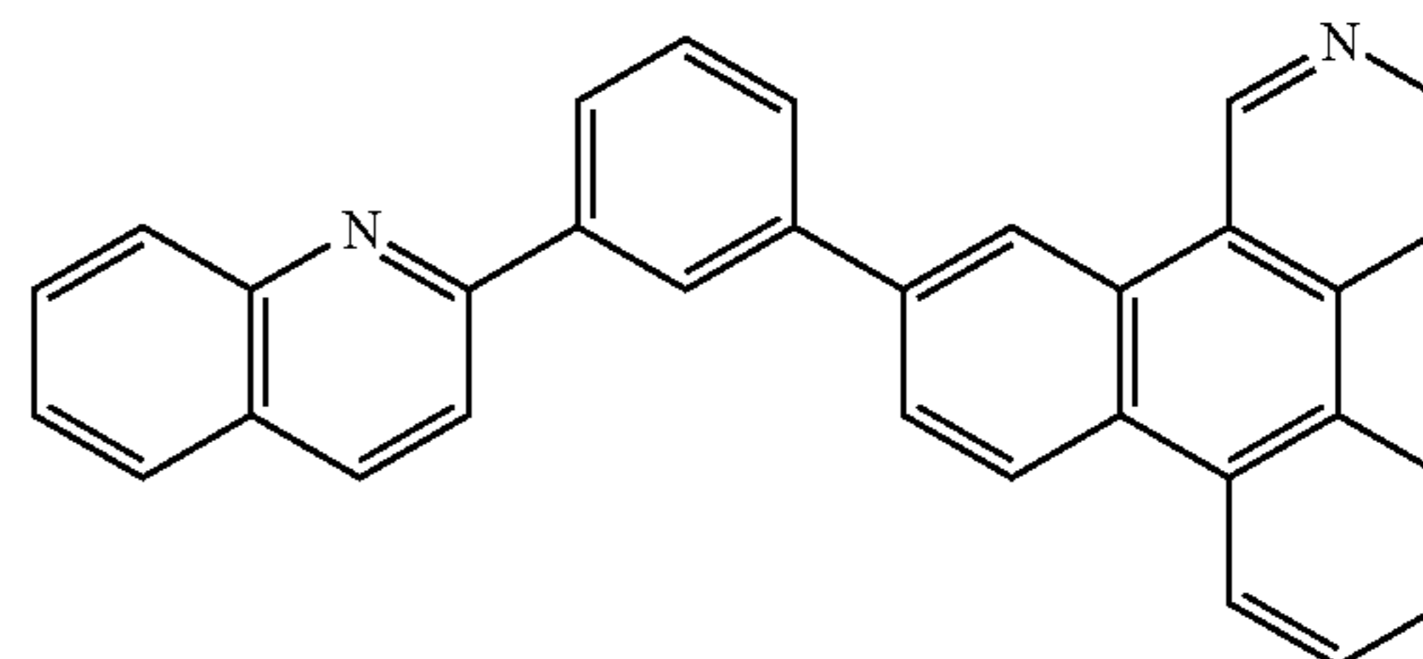
Compound 67
