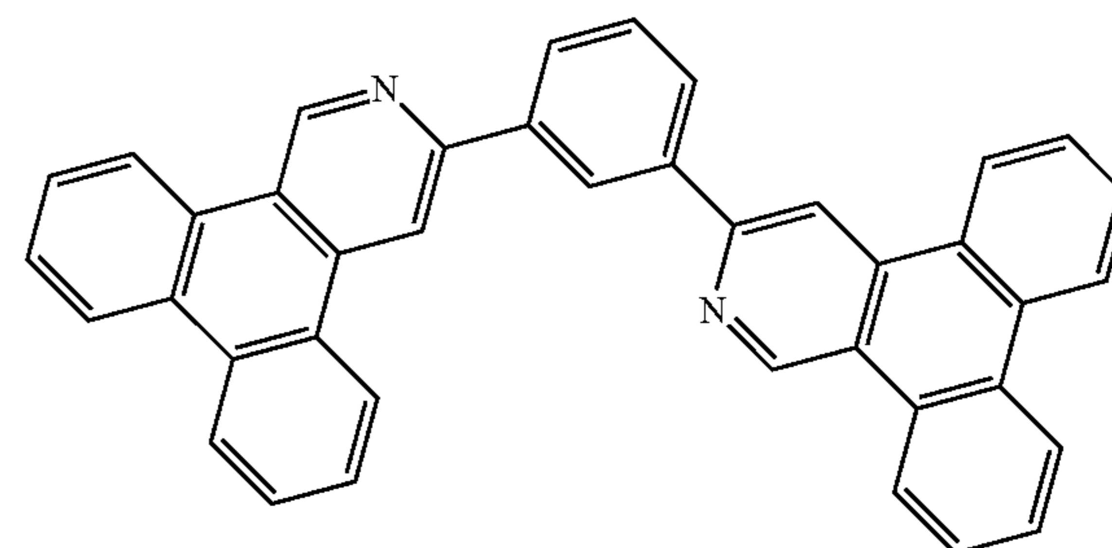
Compound 9
