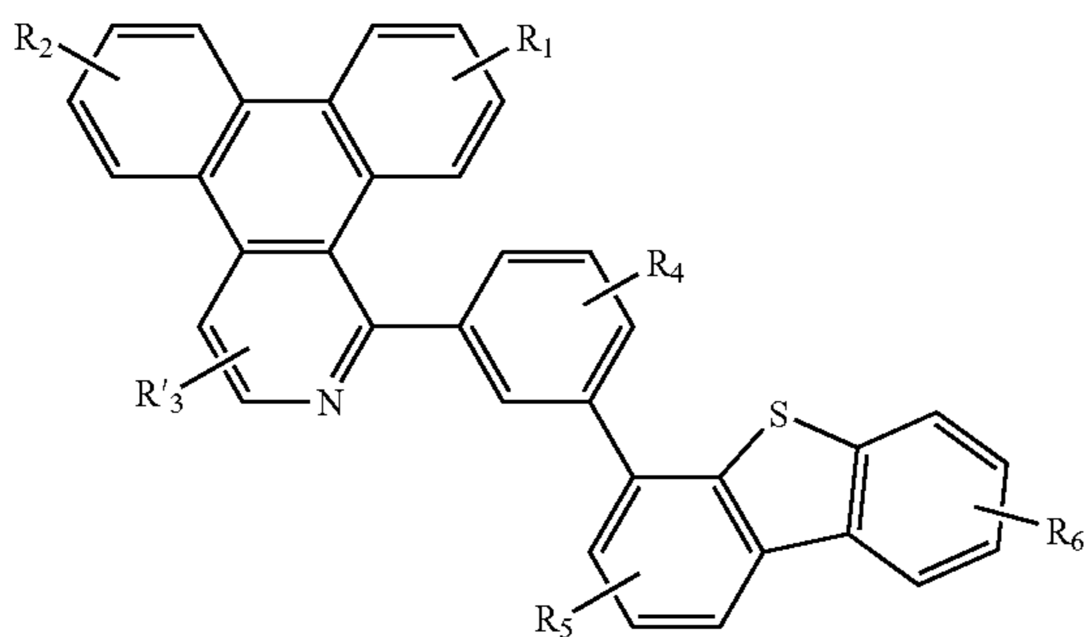
Compound 16G
