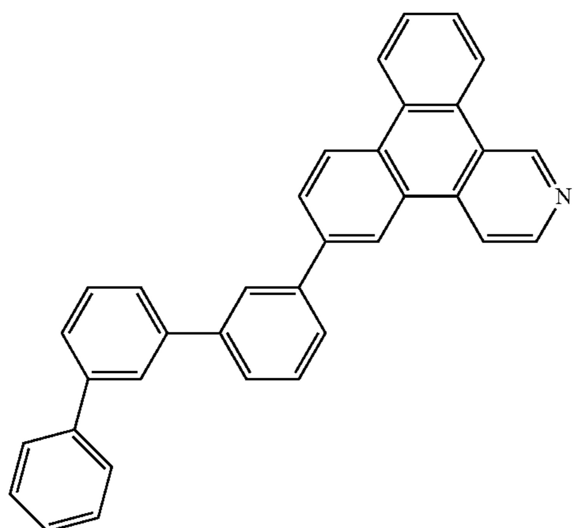
Compound 30
