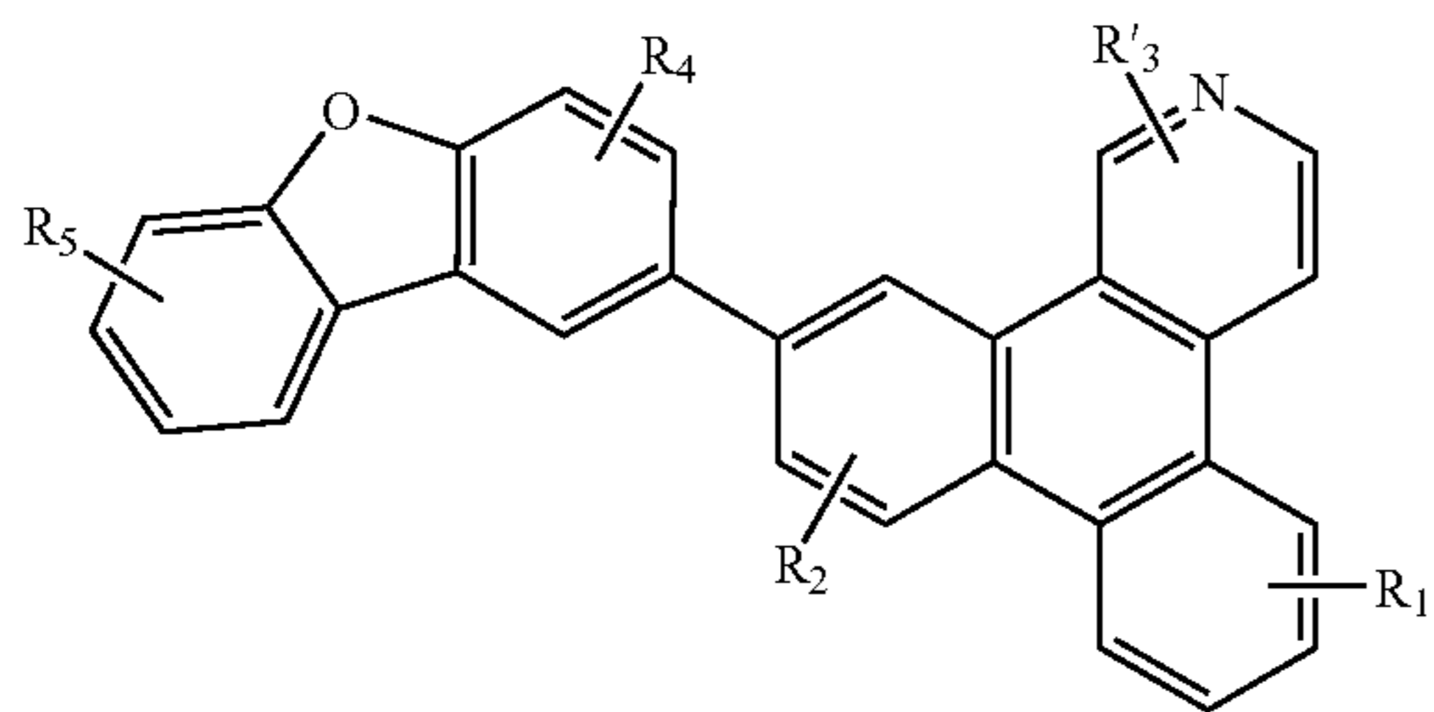
Compound 39G
