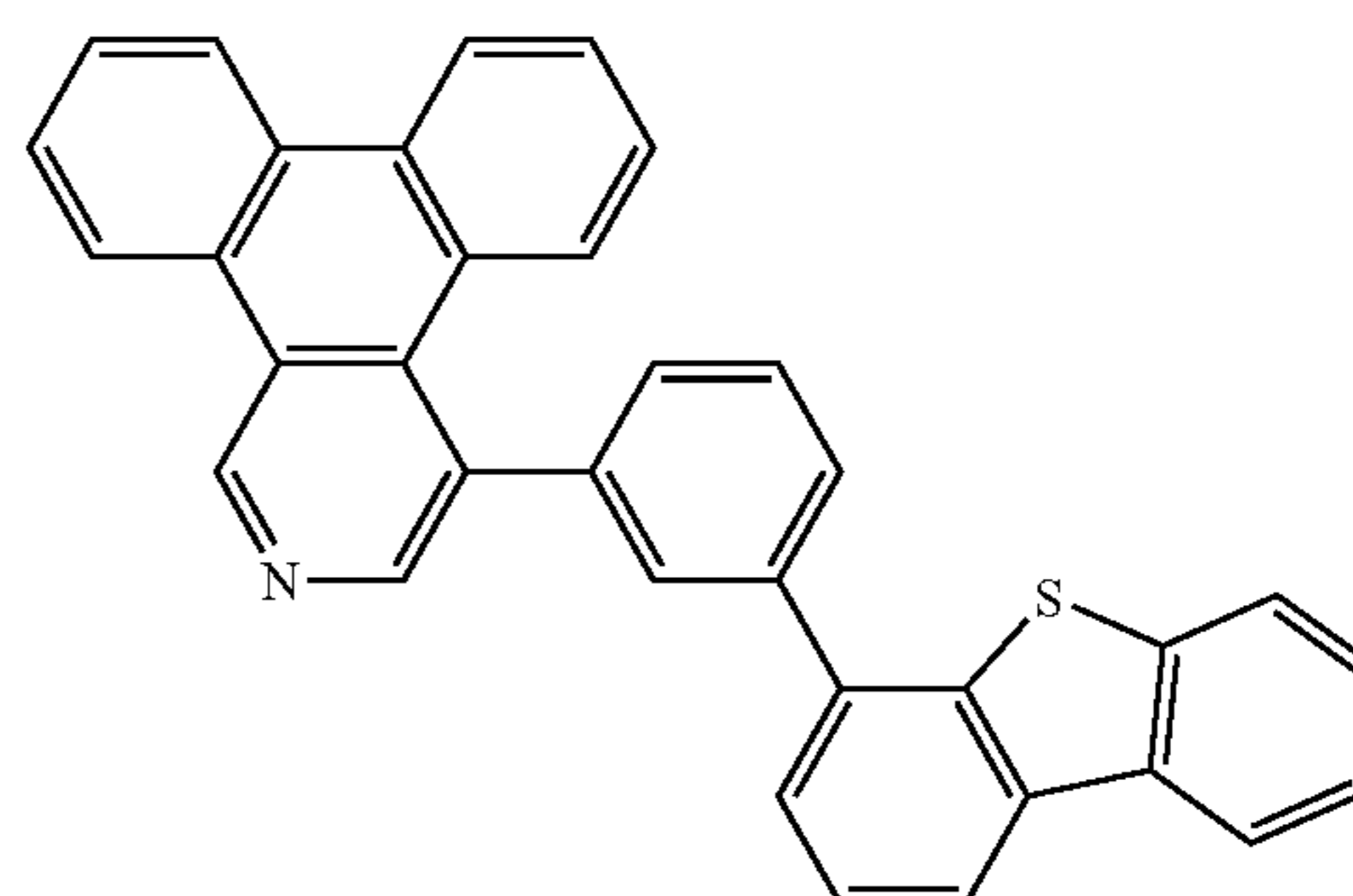
Compound 17
