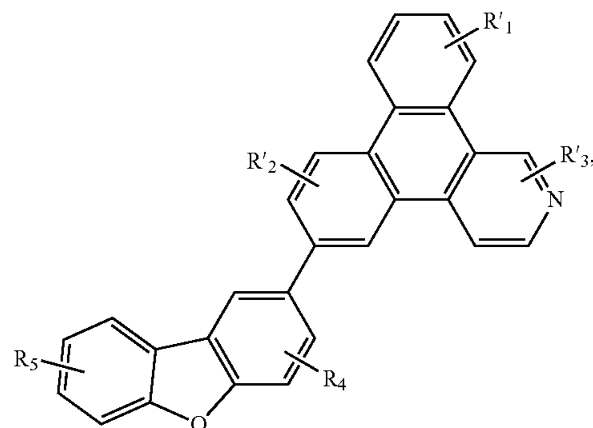
Compound 42G
