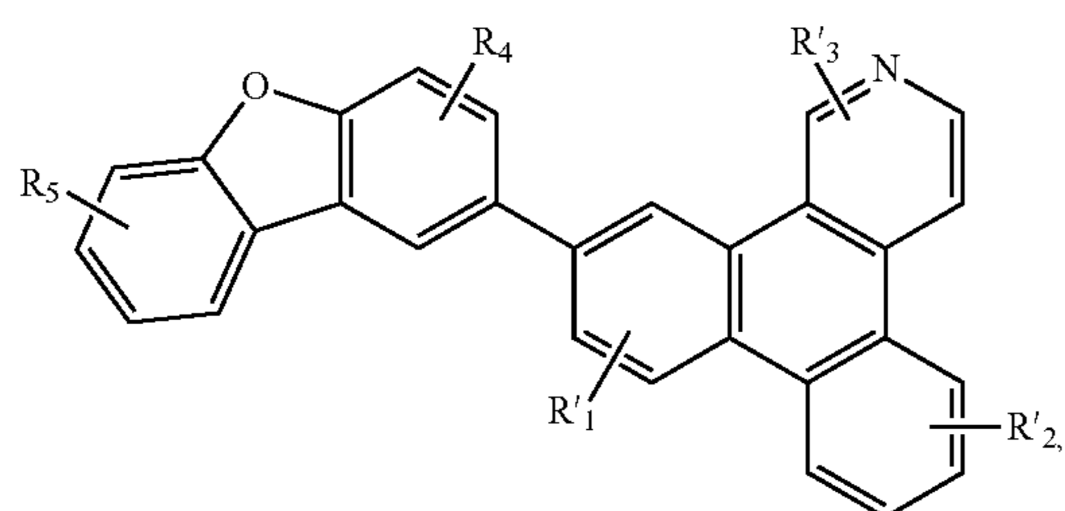
Compound 39G
