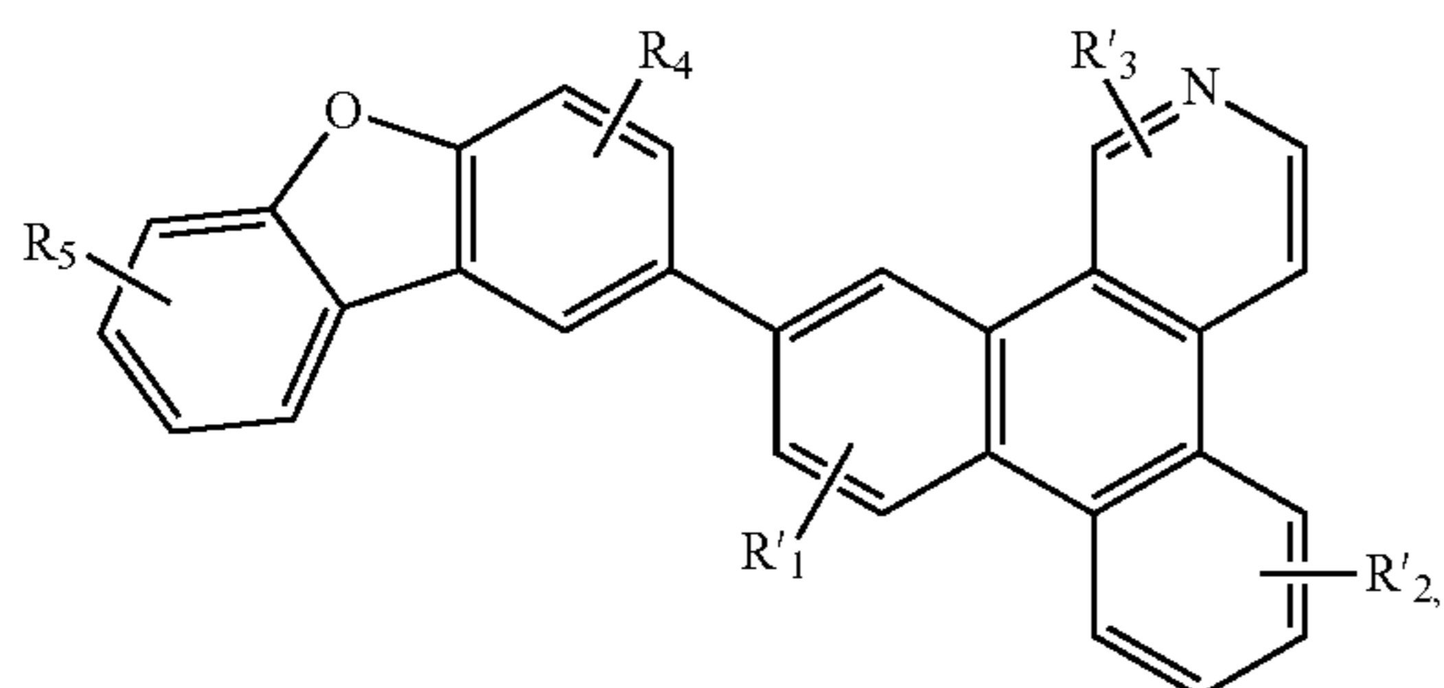
Compound 39G
