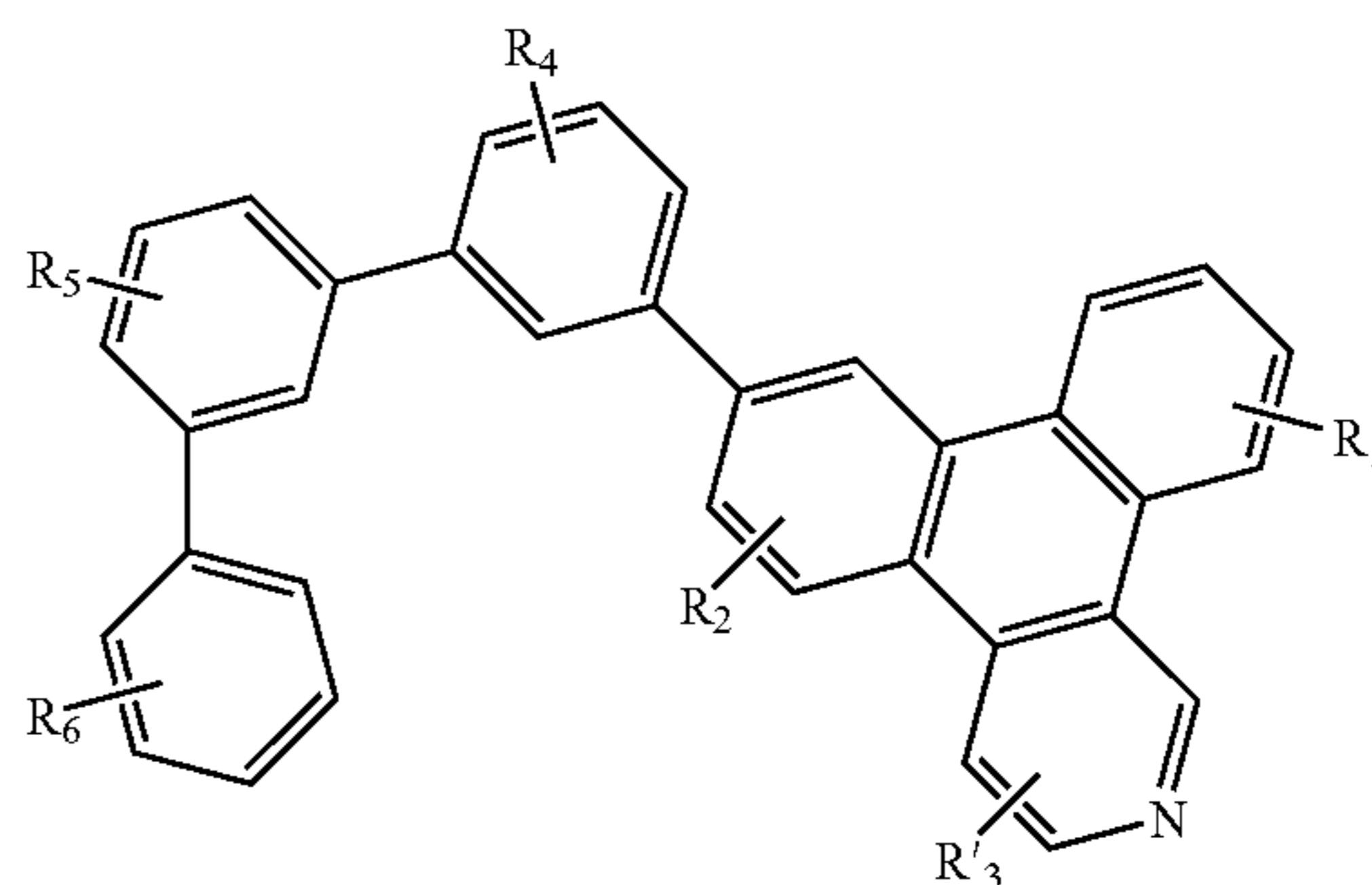
Compound 29G
