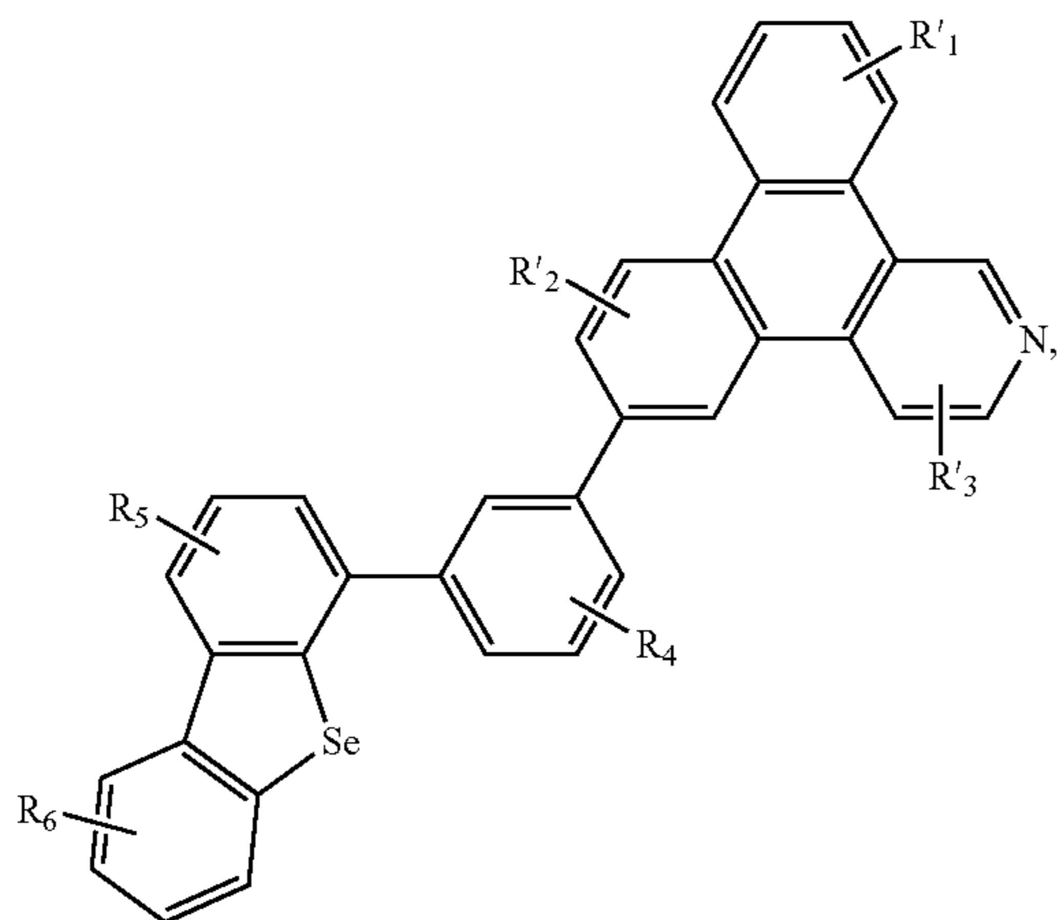
Compound 58G
