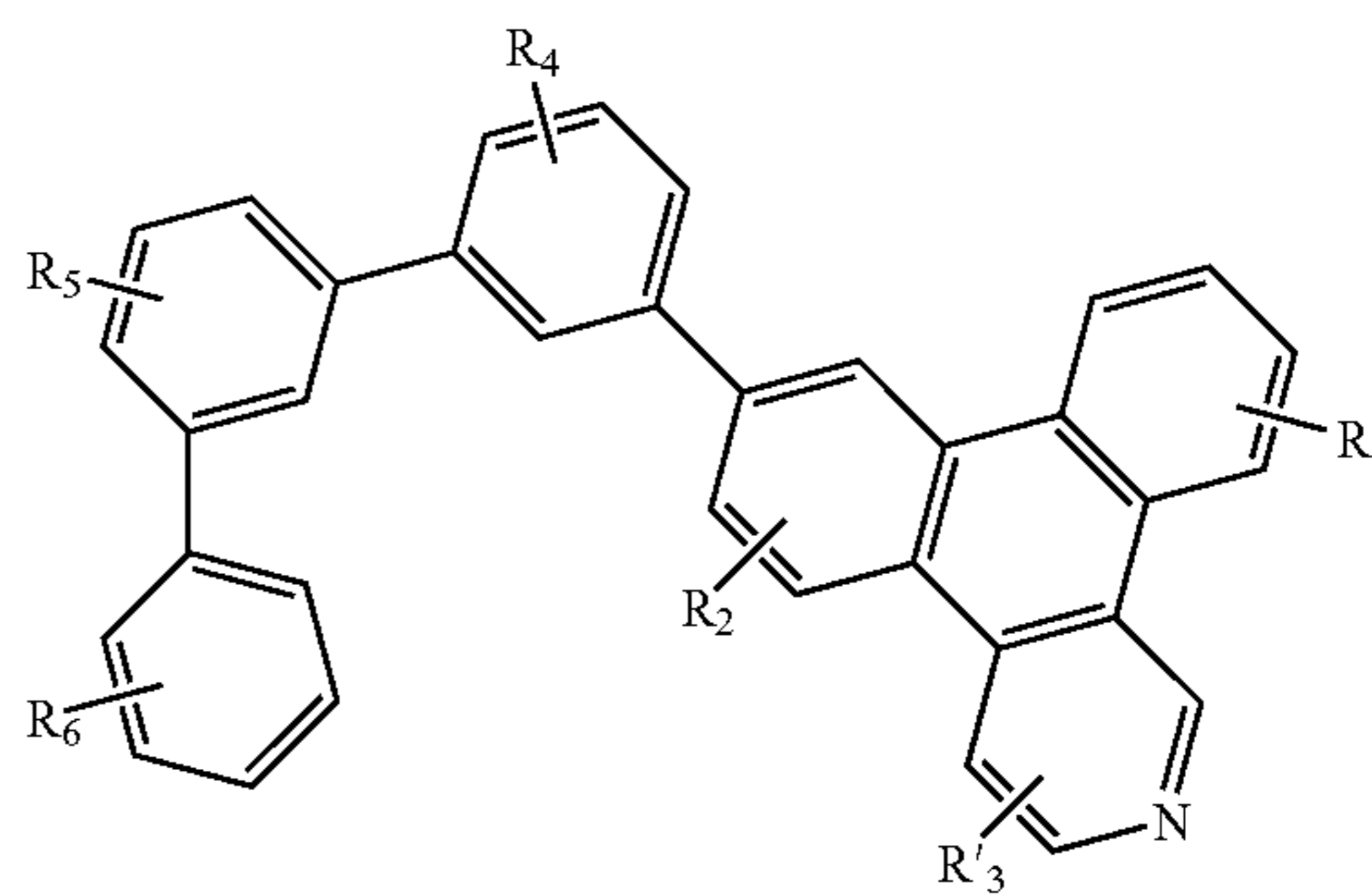
Compound 29G
