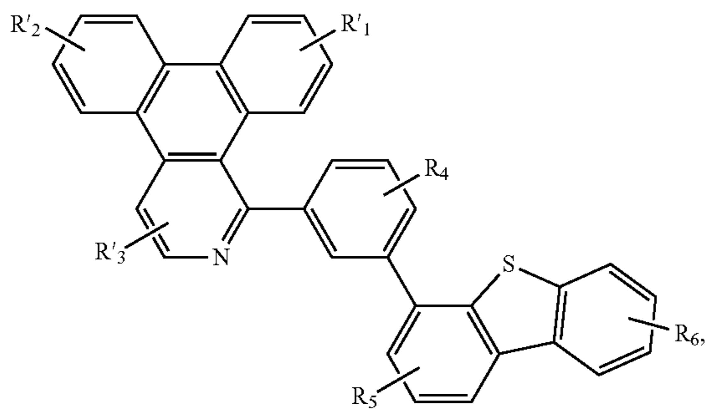
Compound 15G
