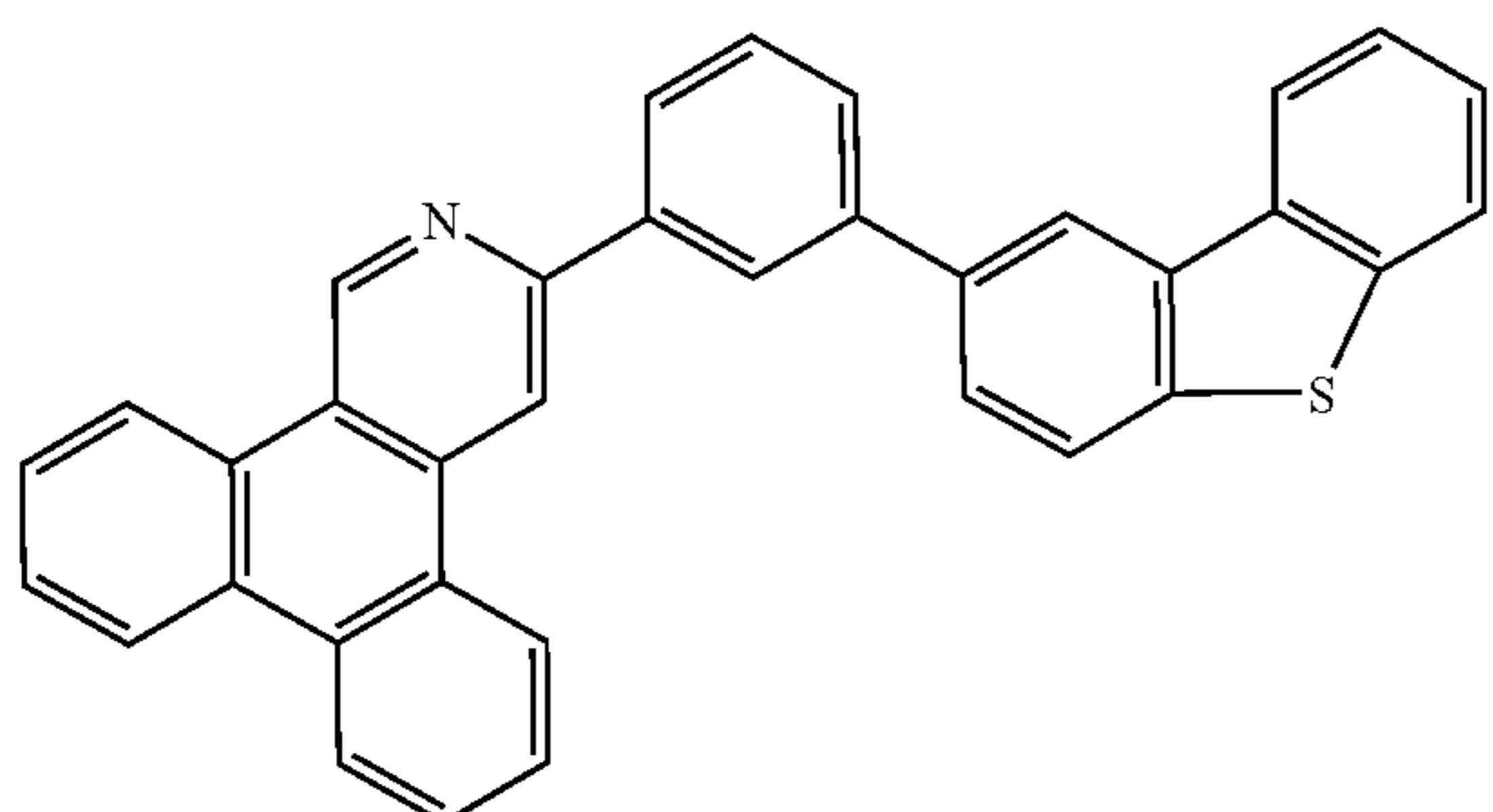
Compound 13
