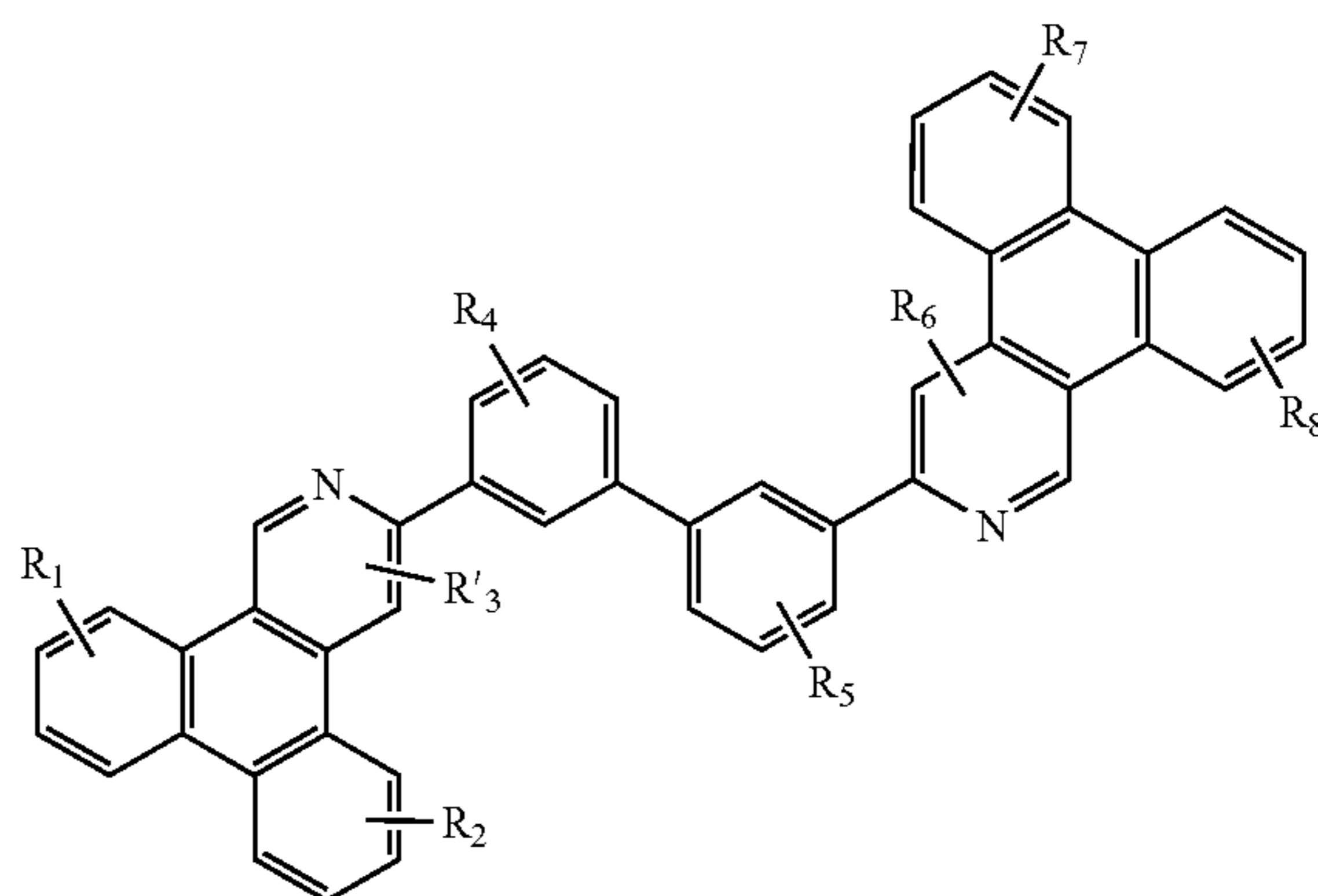
Compound 10G
