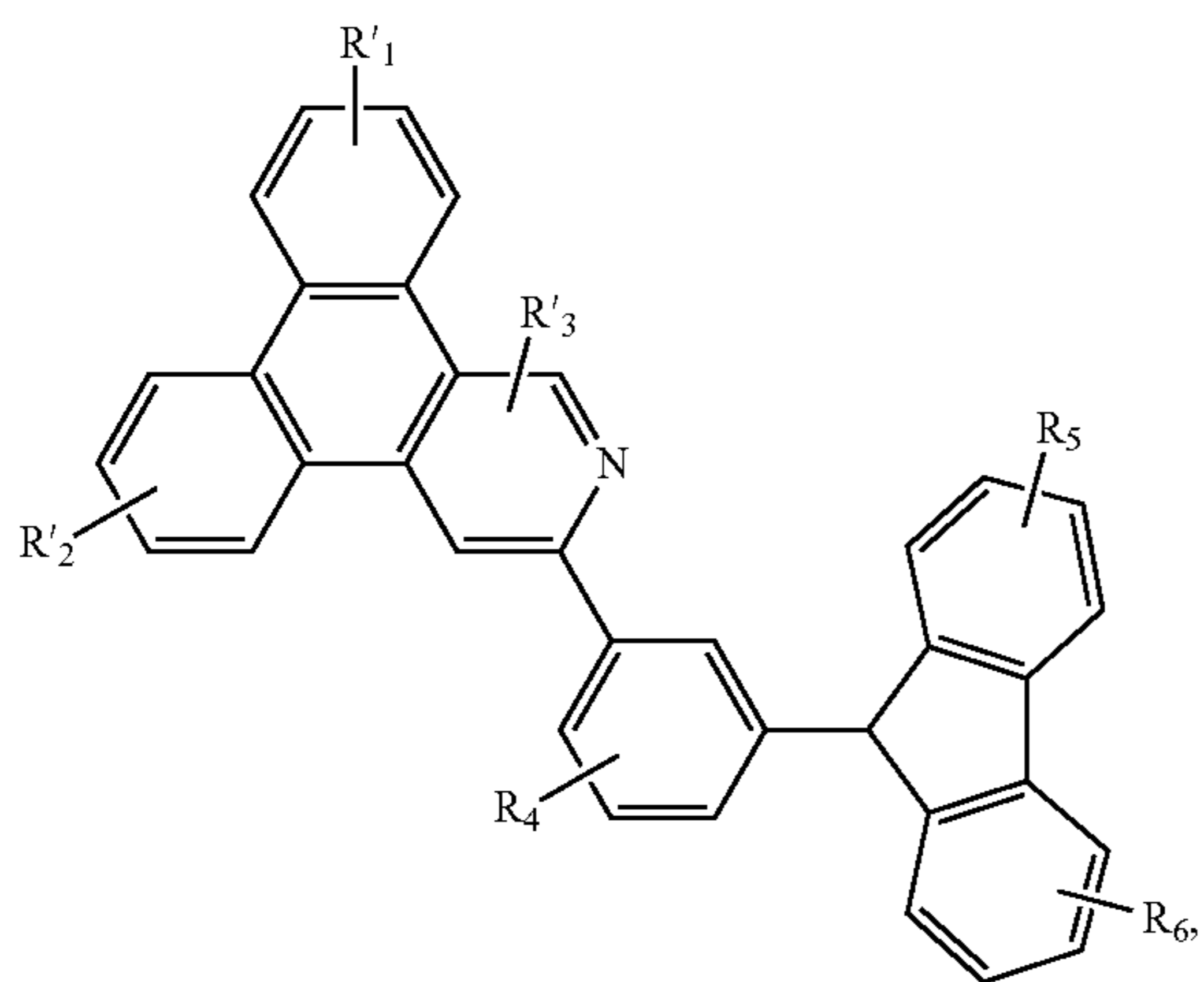
Compound 7G
