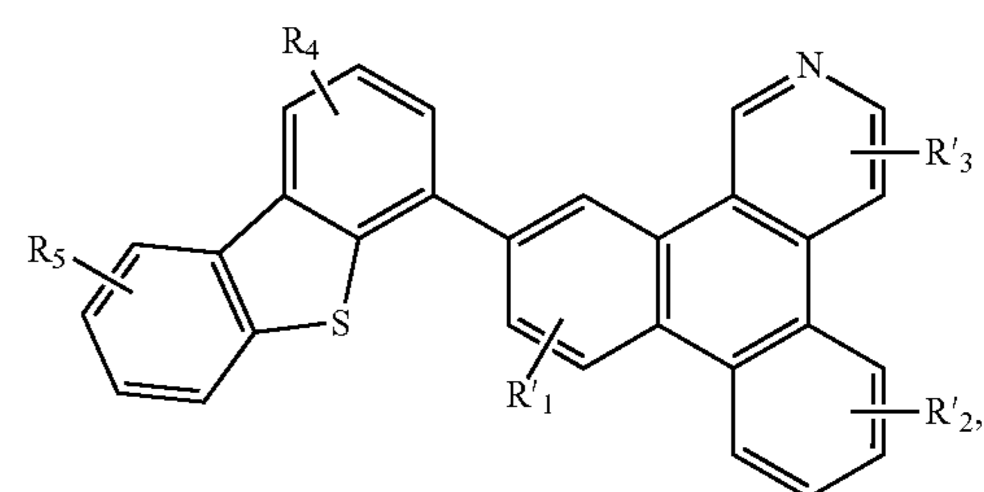
Compound 47G
