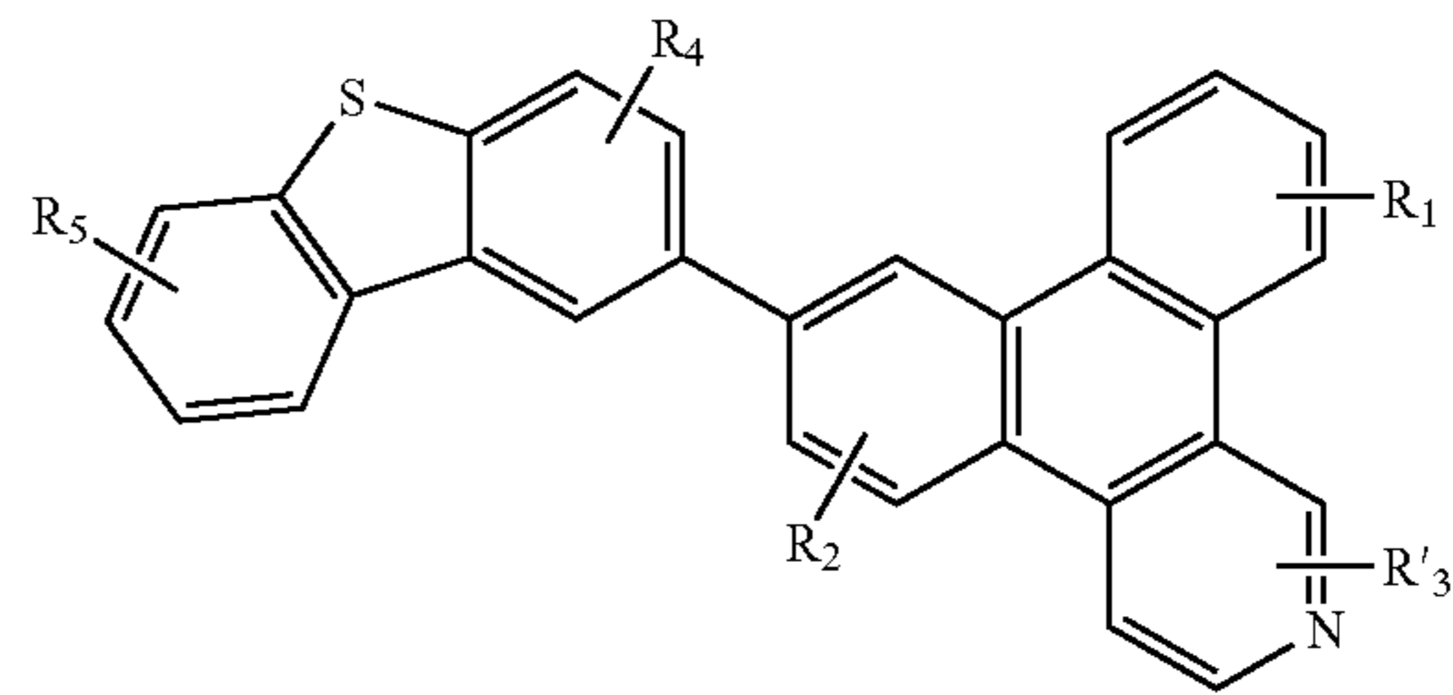
Compound 53G
