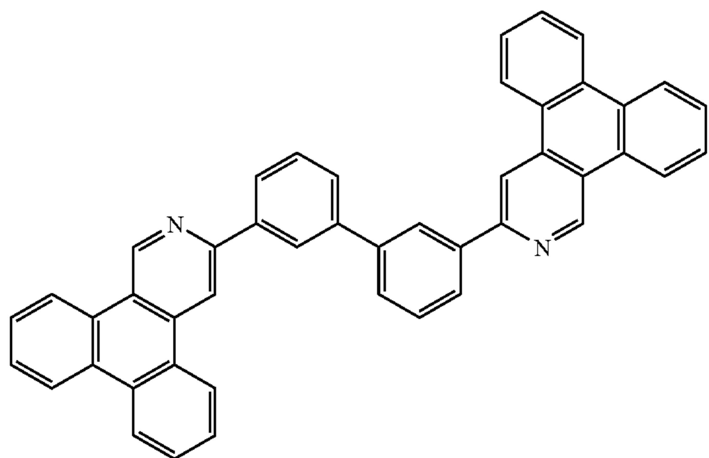
Compound 11
