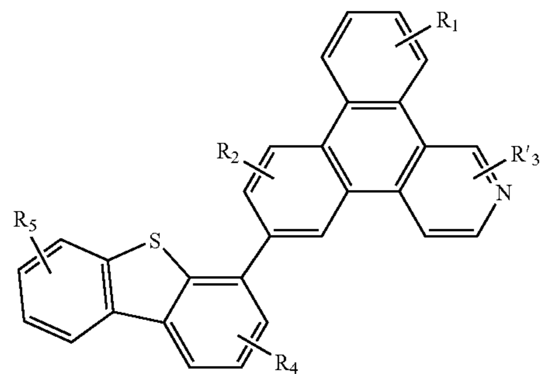
Compound 51G
