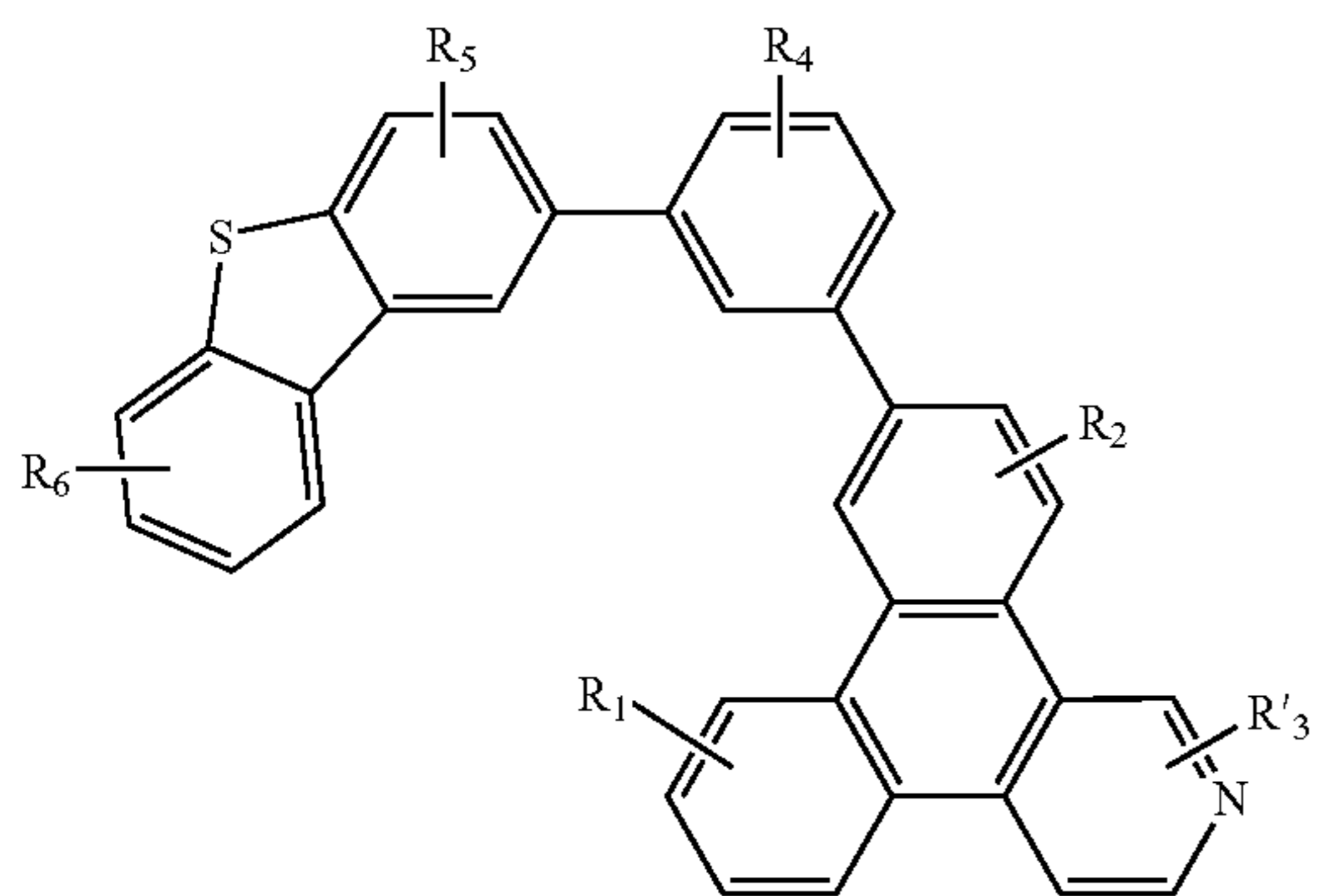
Compound 25G
