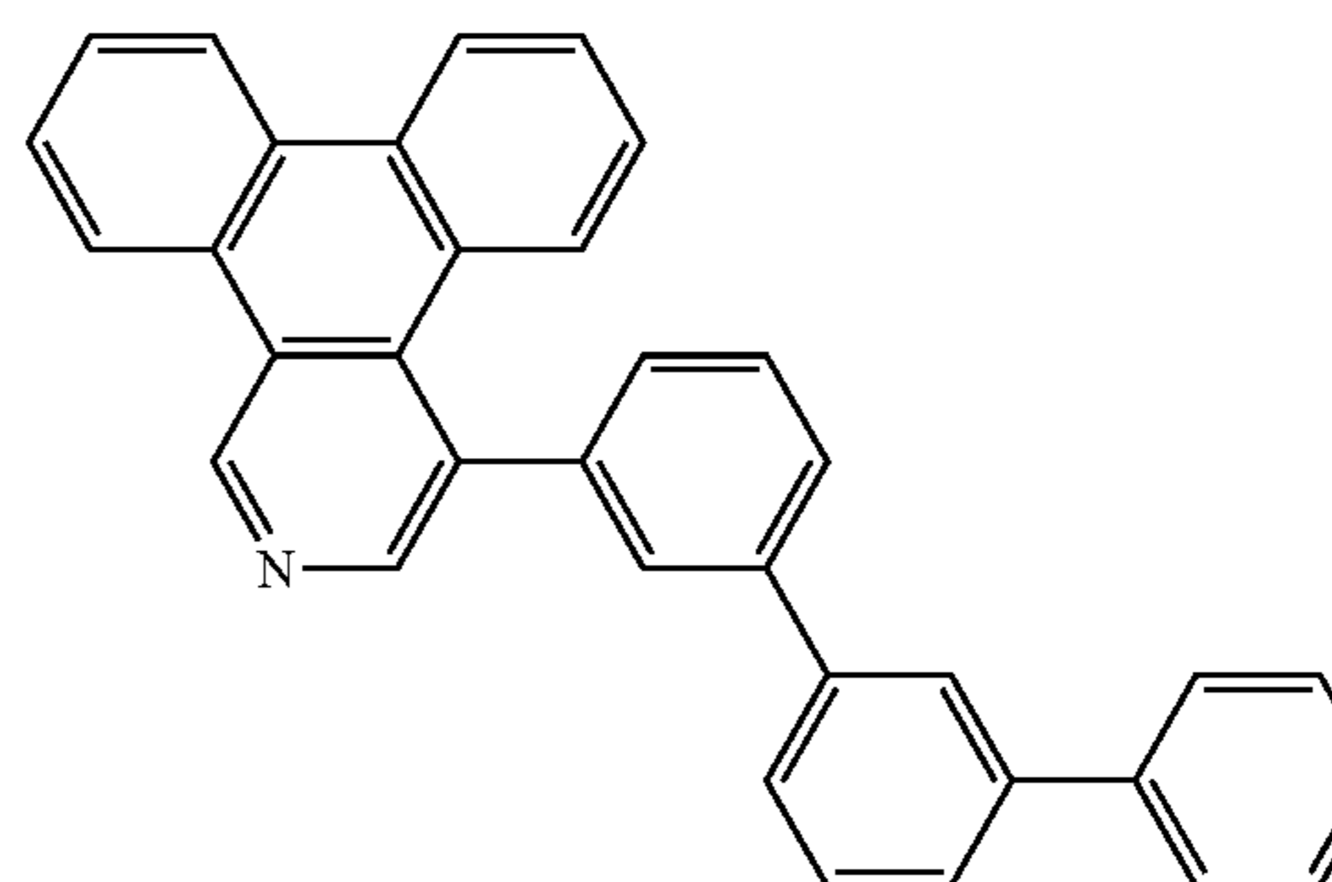
Compound 18
