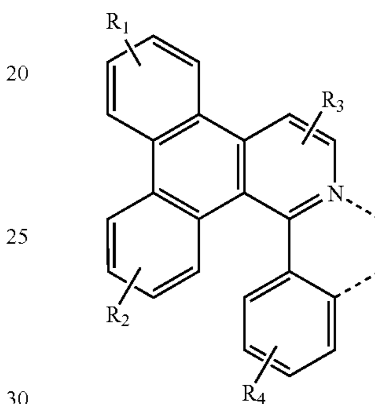
Compound 72G
