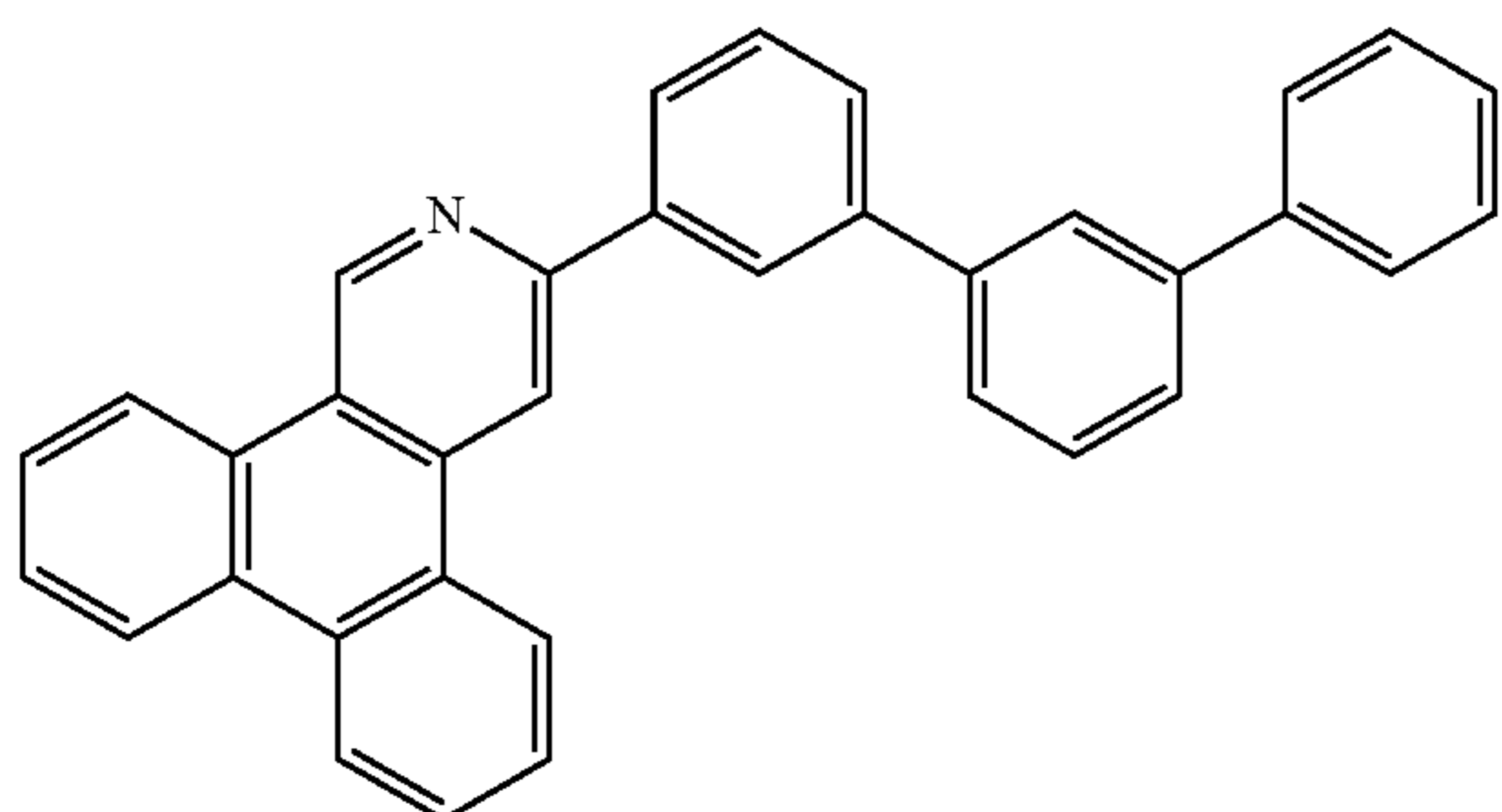
Compound 3
