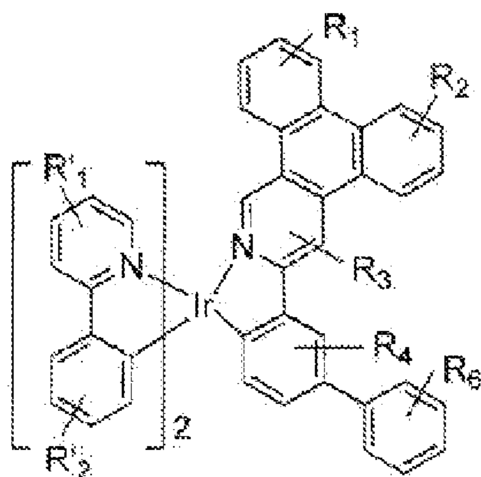
Compound 95
