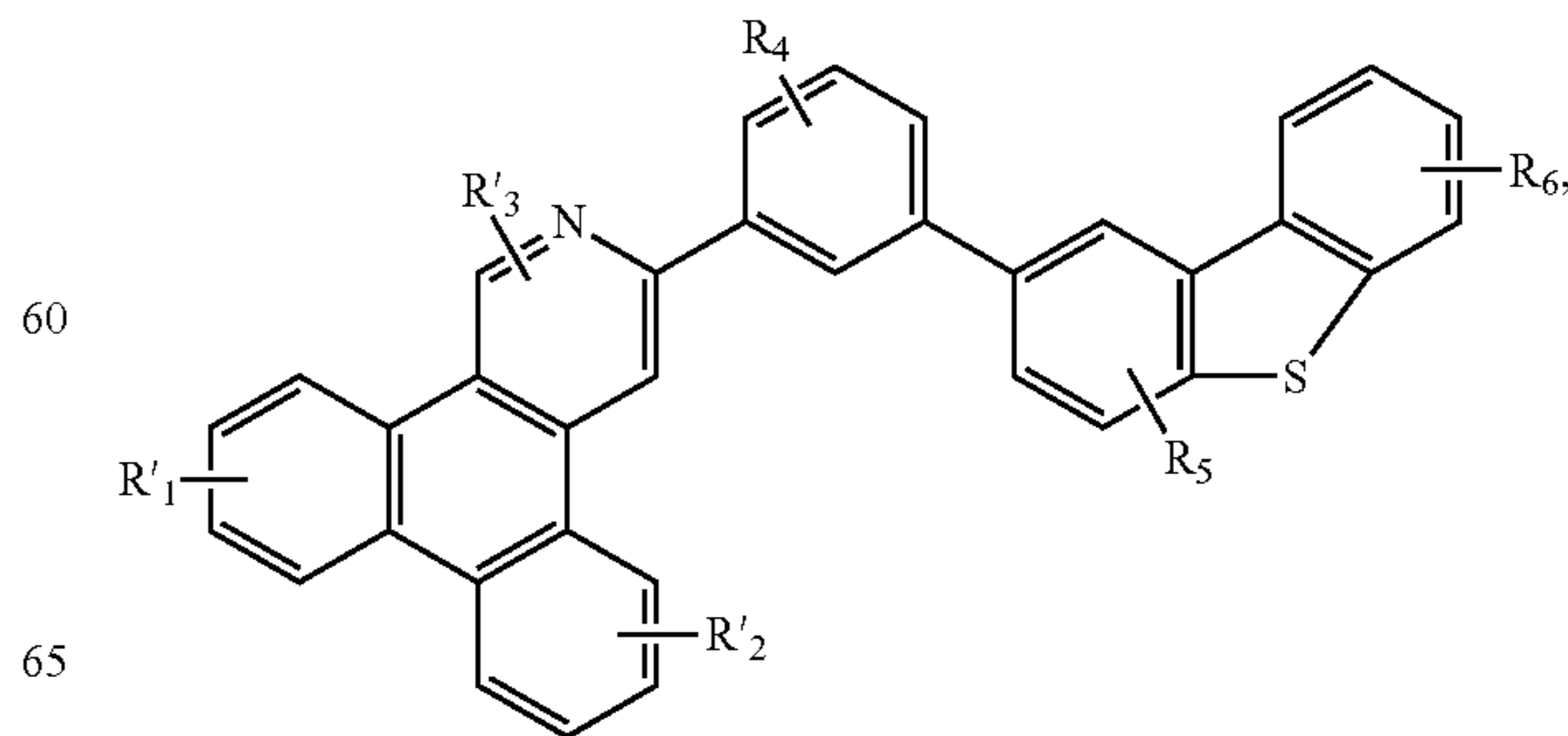
Compound 13G
