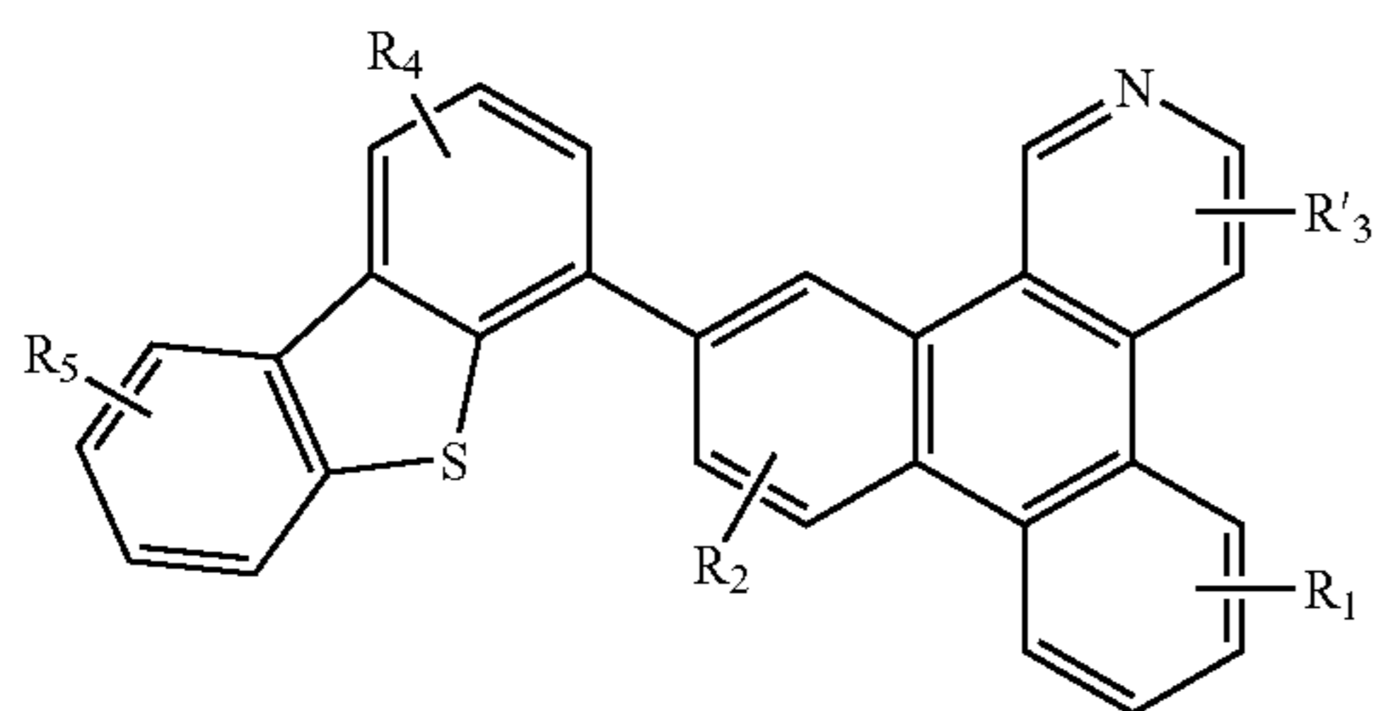
Compound 47G
