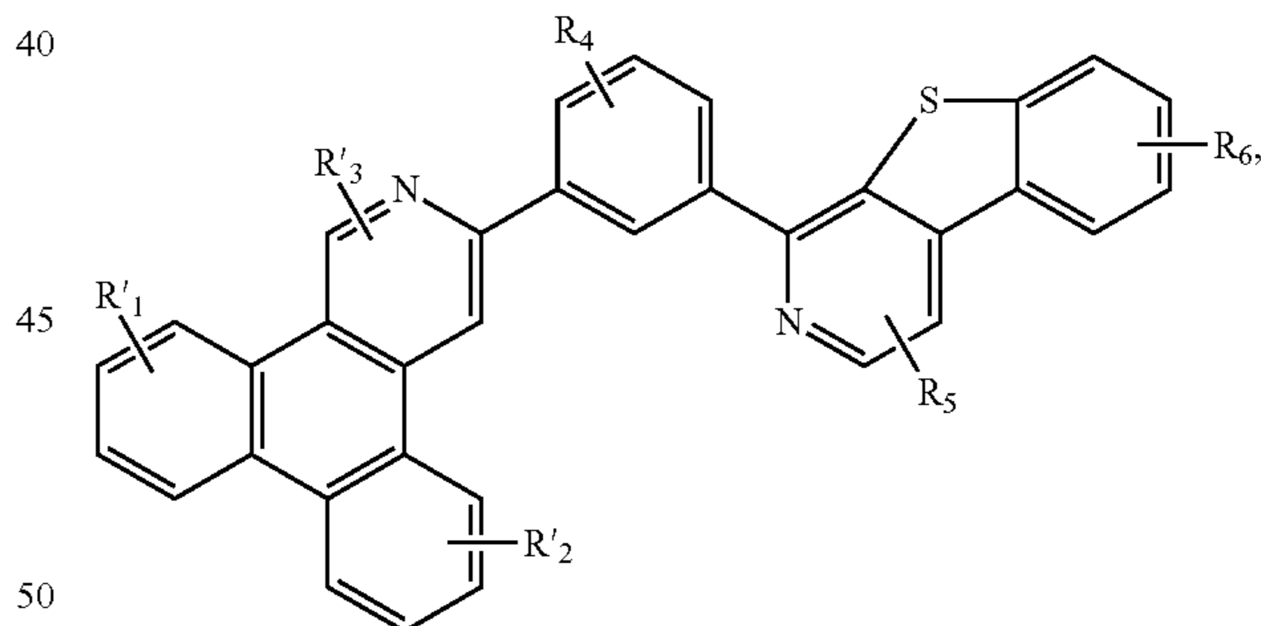
Compound 12G
