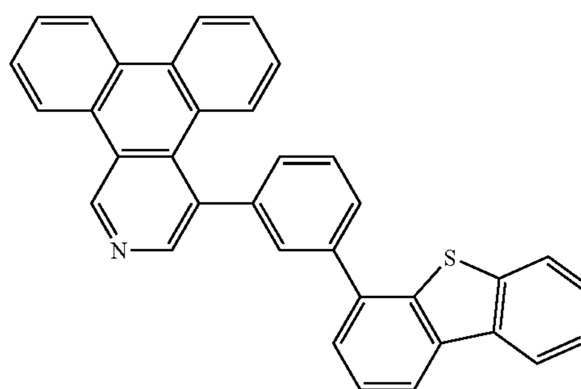
Compound 17
