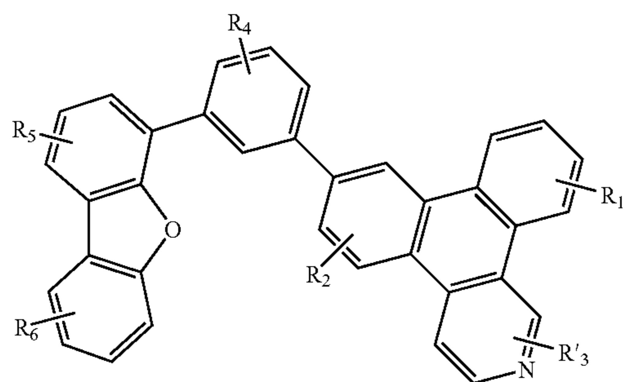
Compound 33G
