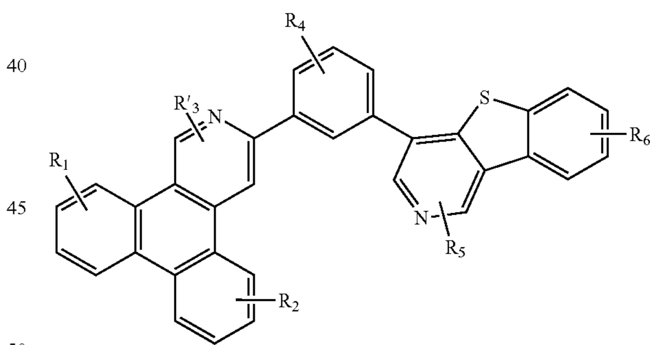
Compound 12G
