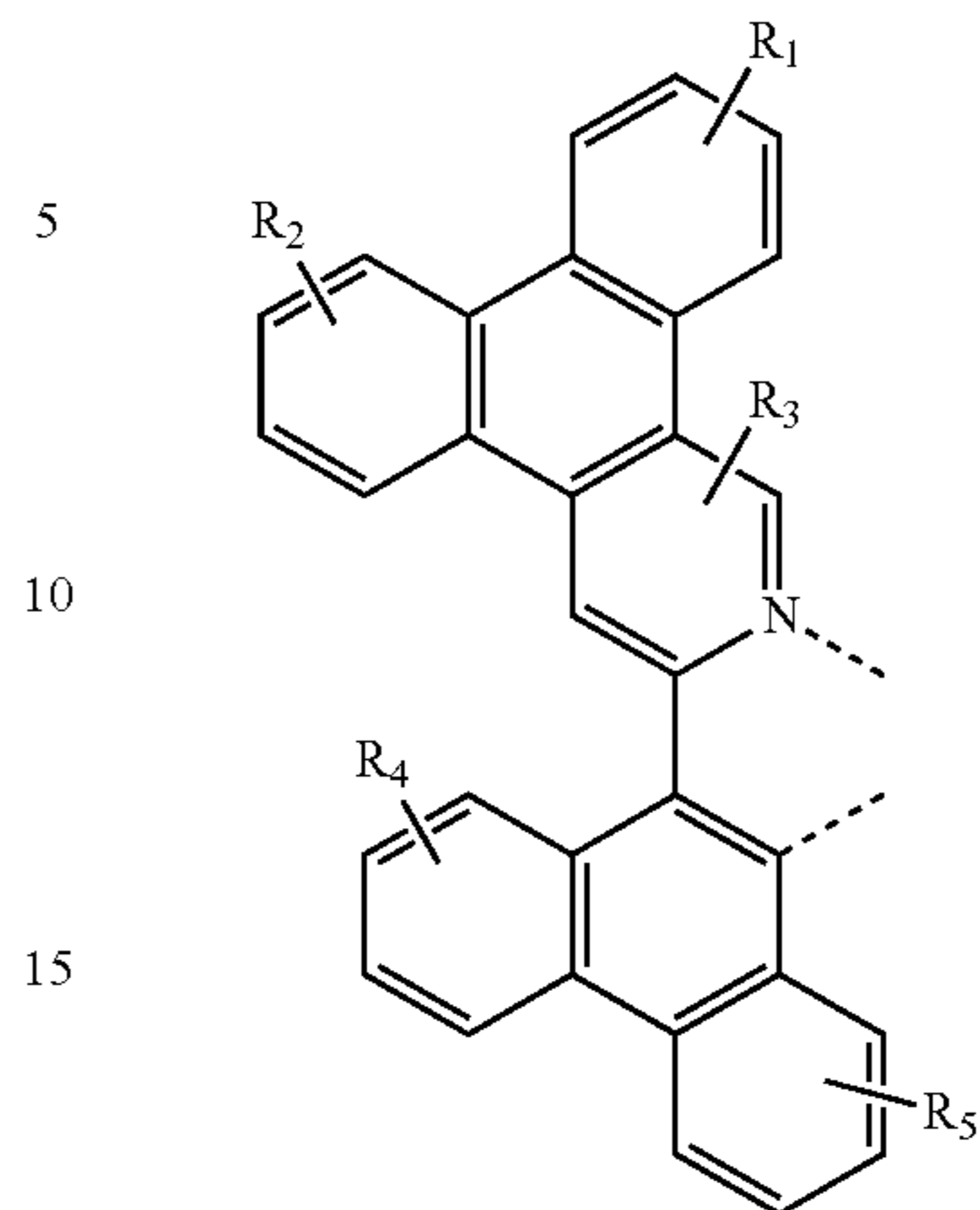
FORMULA II
