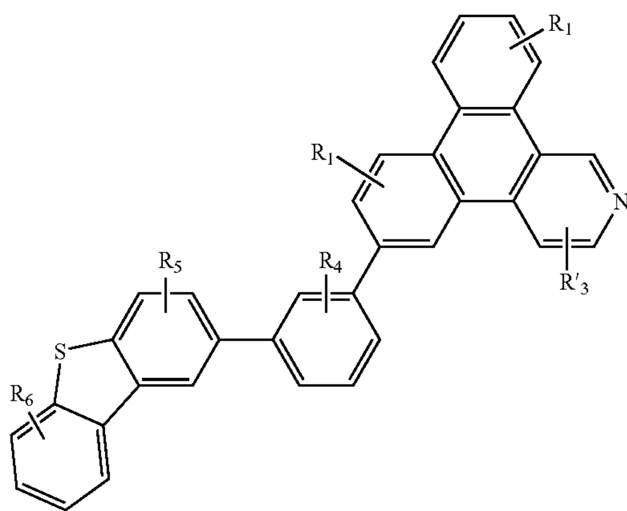
Compound 26G
