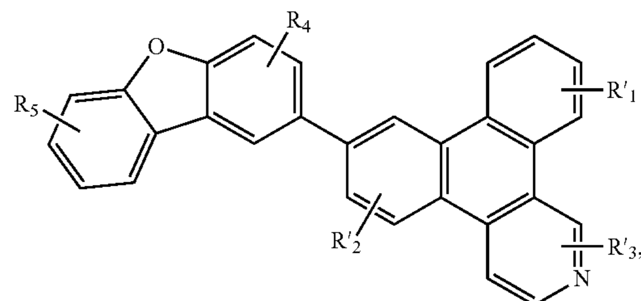
Compound 41G
