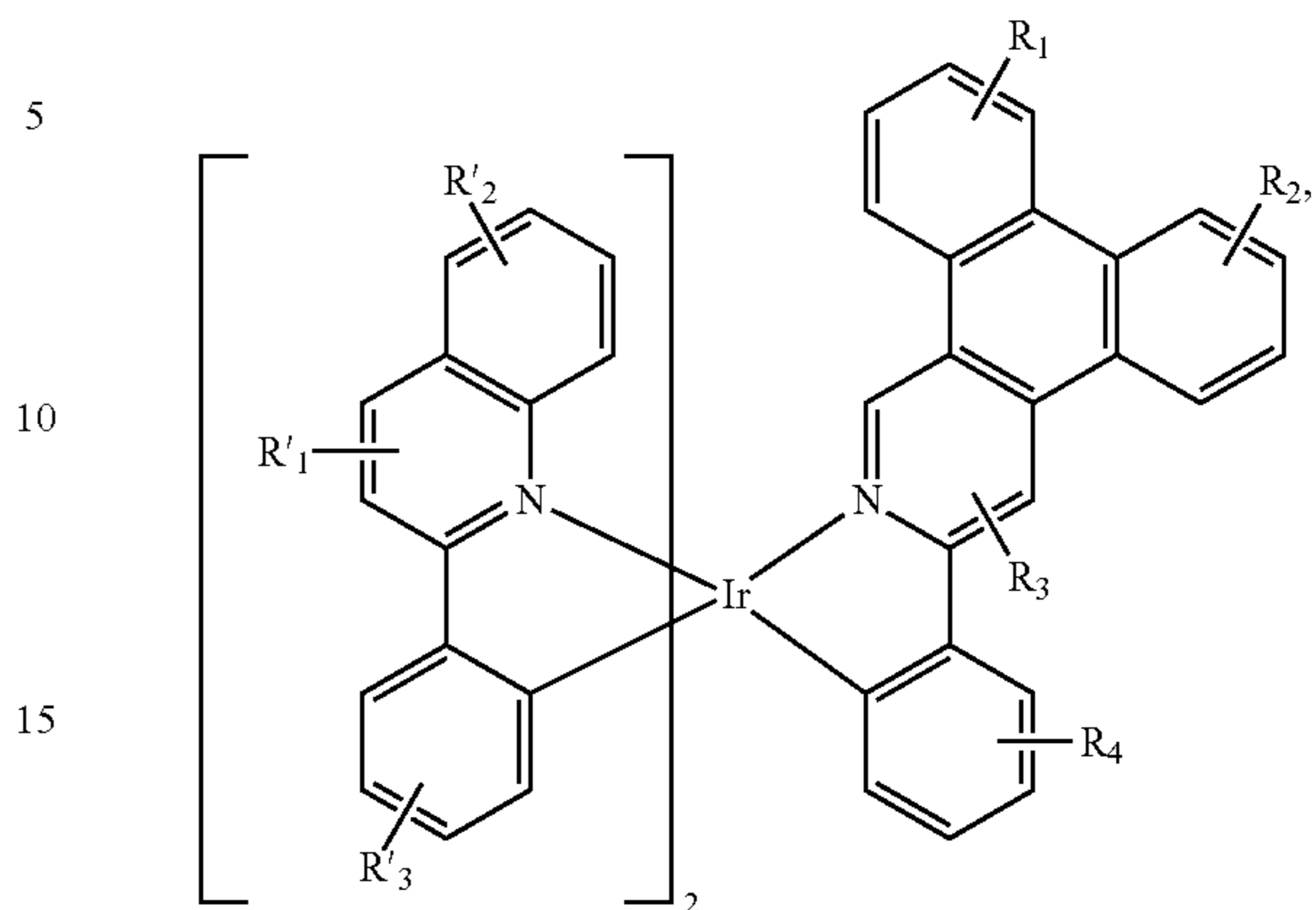
Compound 96
