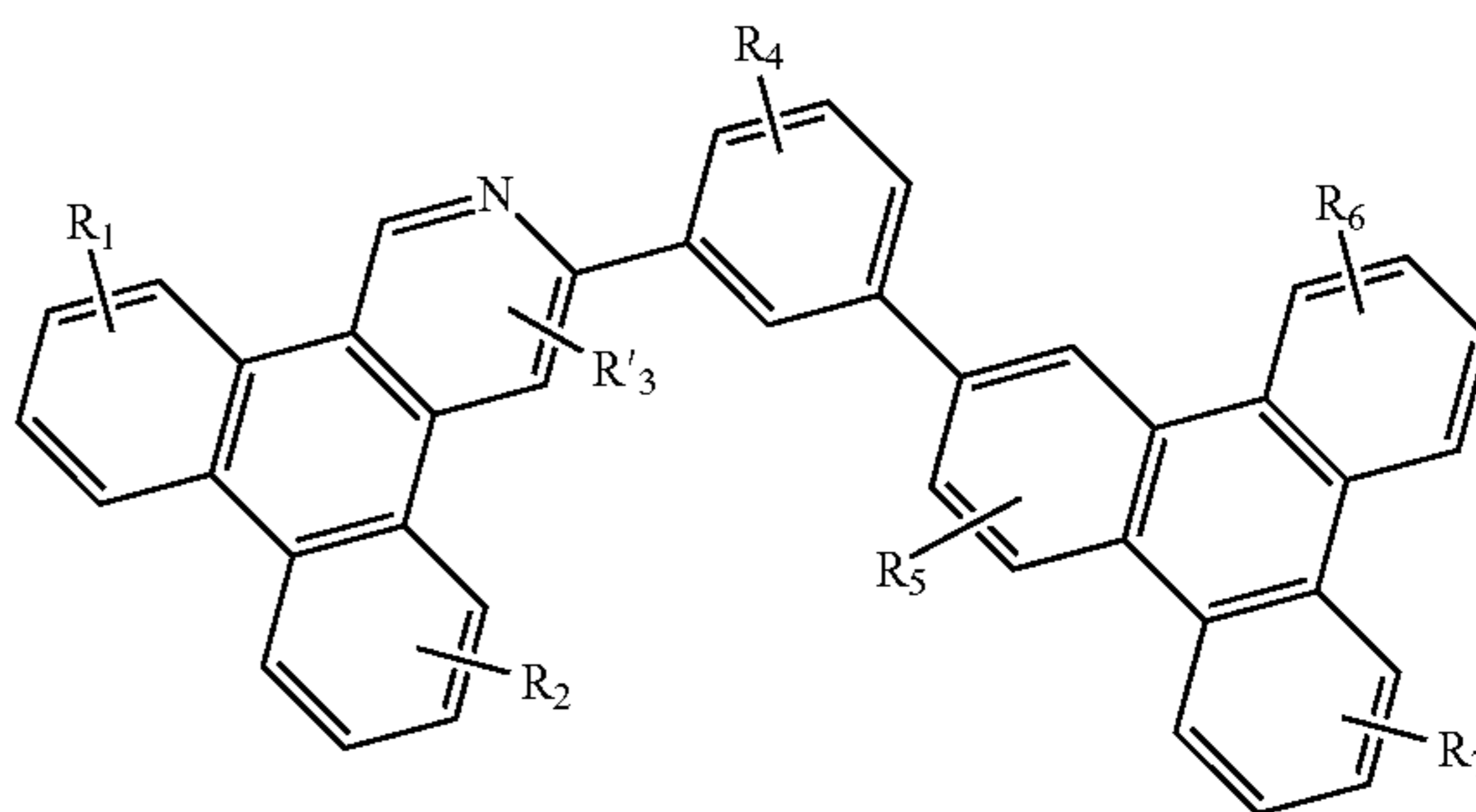
Compound 11G
