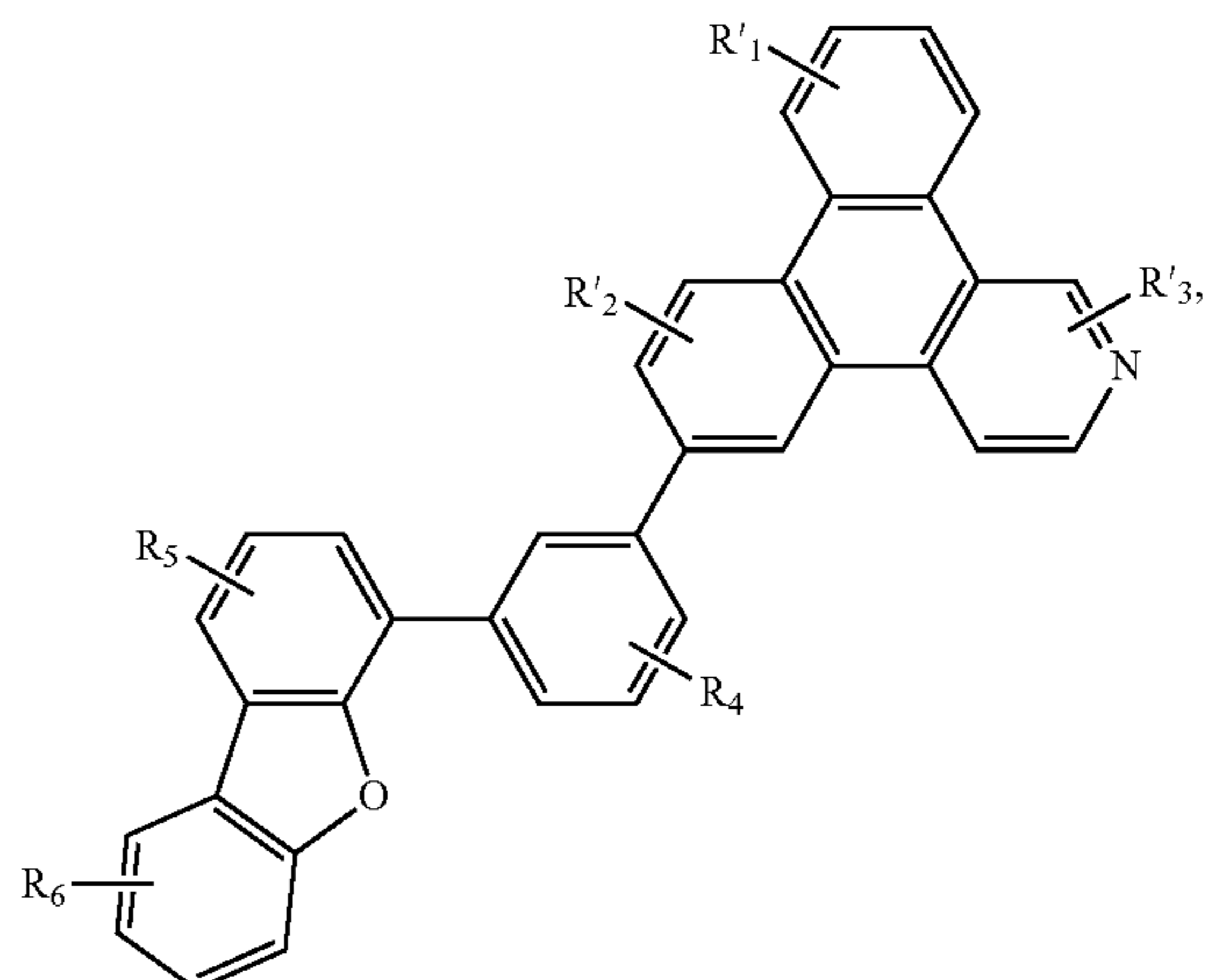
Compound 34G
