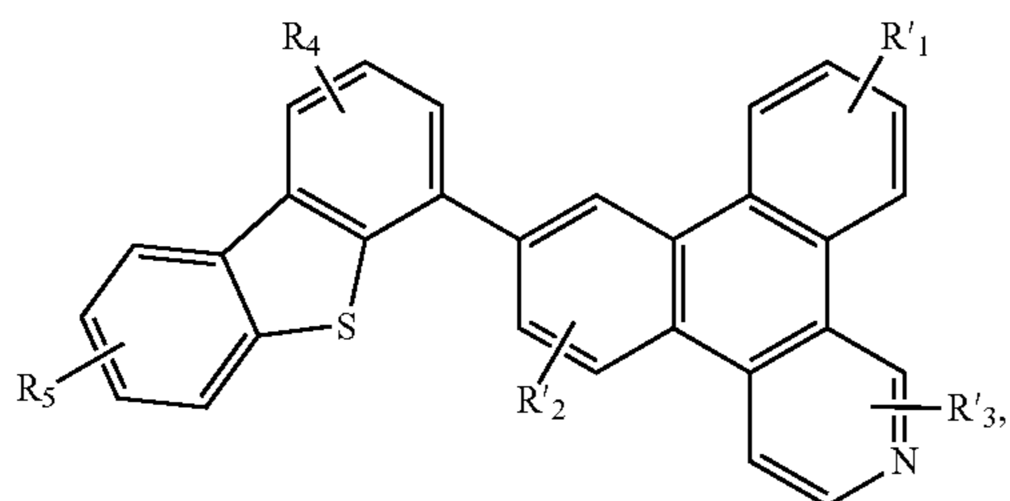
Compound 49G
