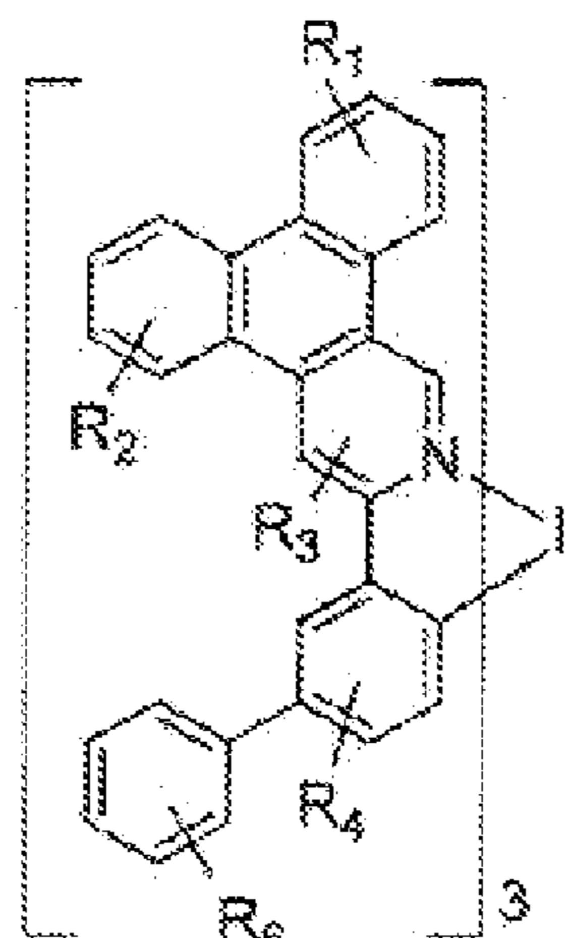
Compound 80
