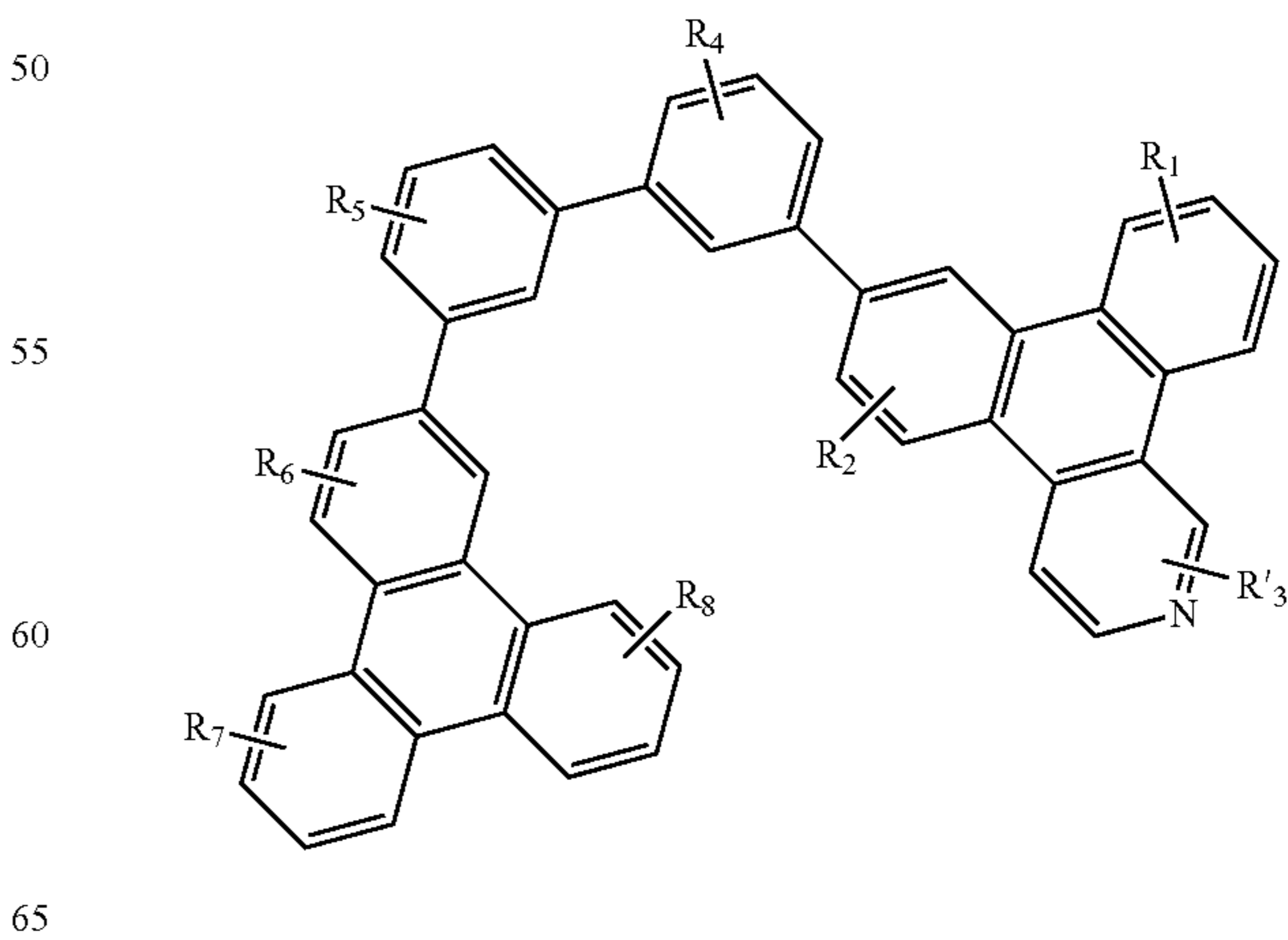
Compound 45G
