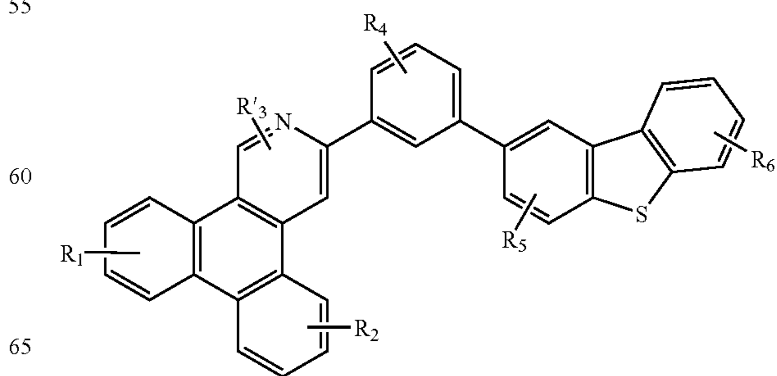
Compound 13G
