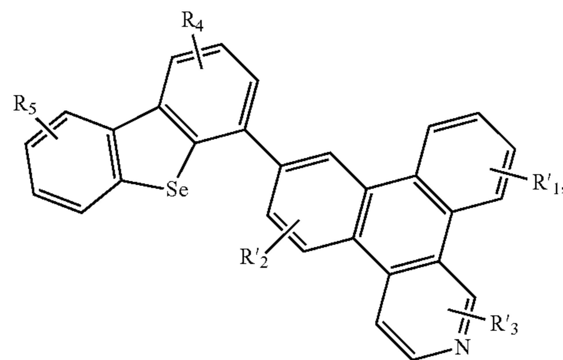
Compound 61G
