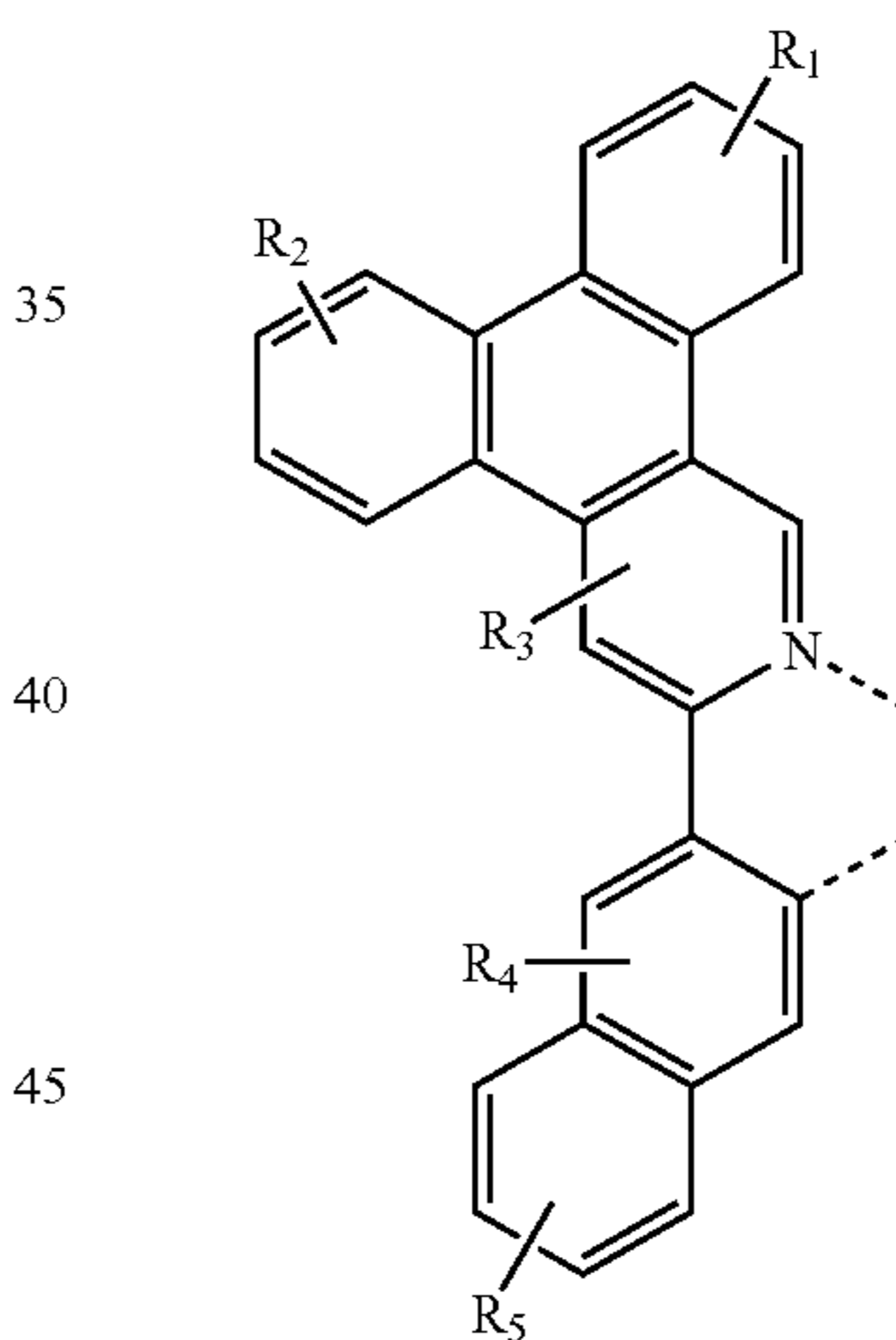
Compound 73G
