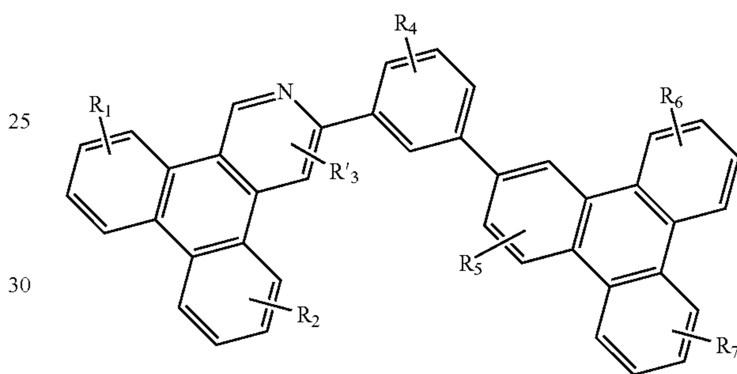
Compound 11G
