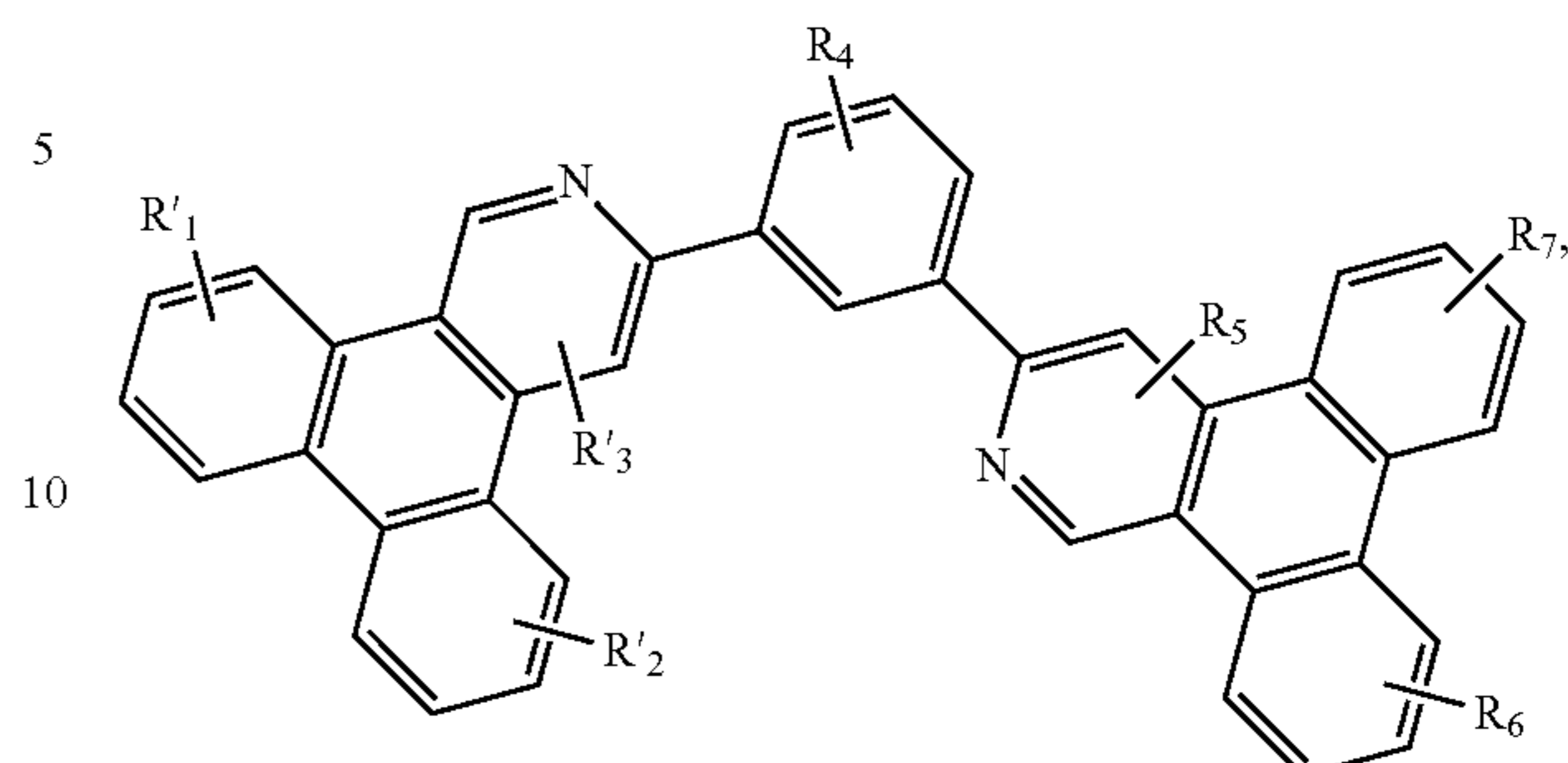
Compound 9G
