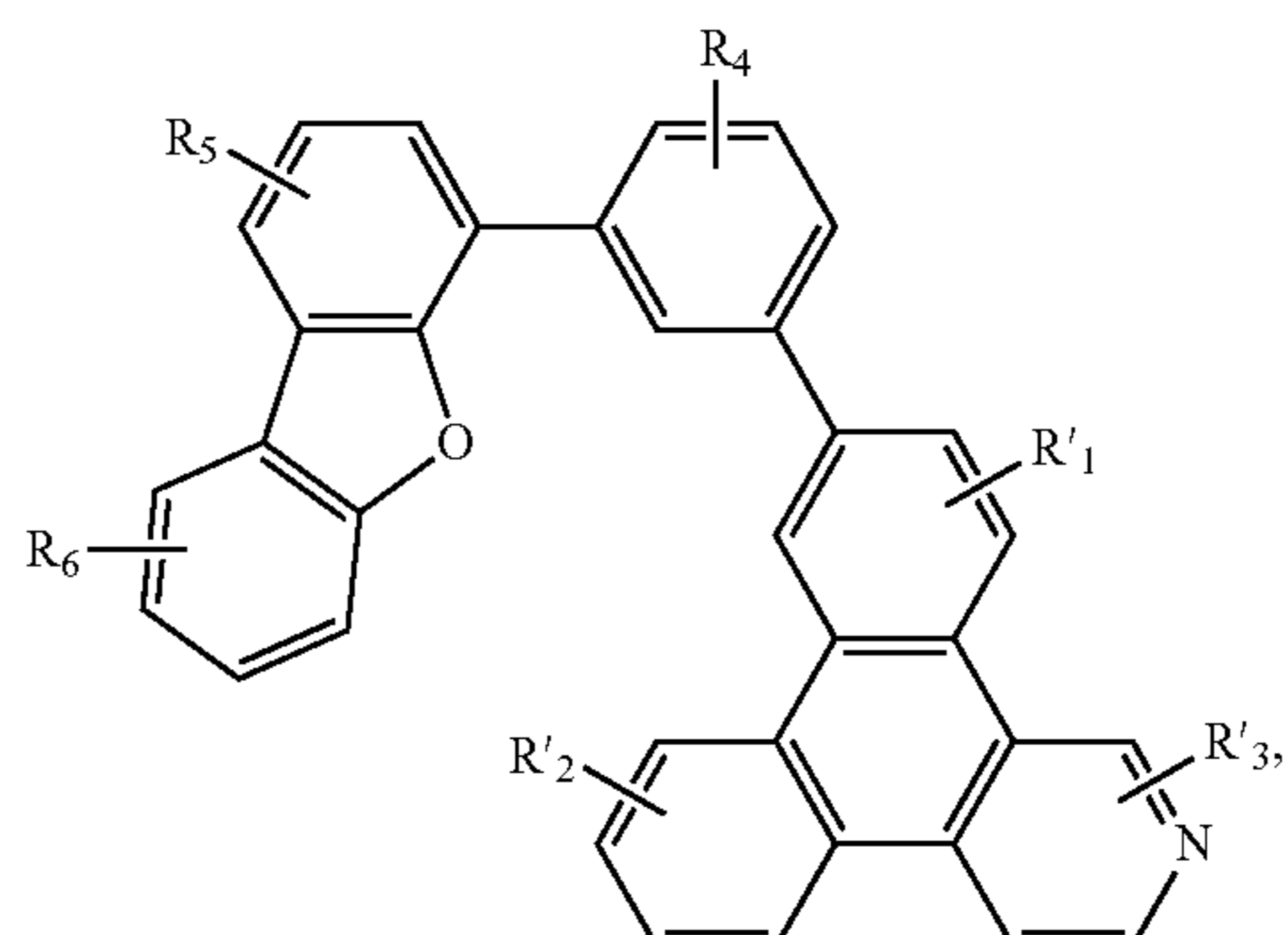
Compound 33G
