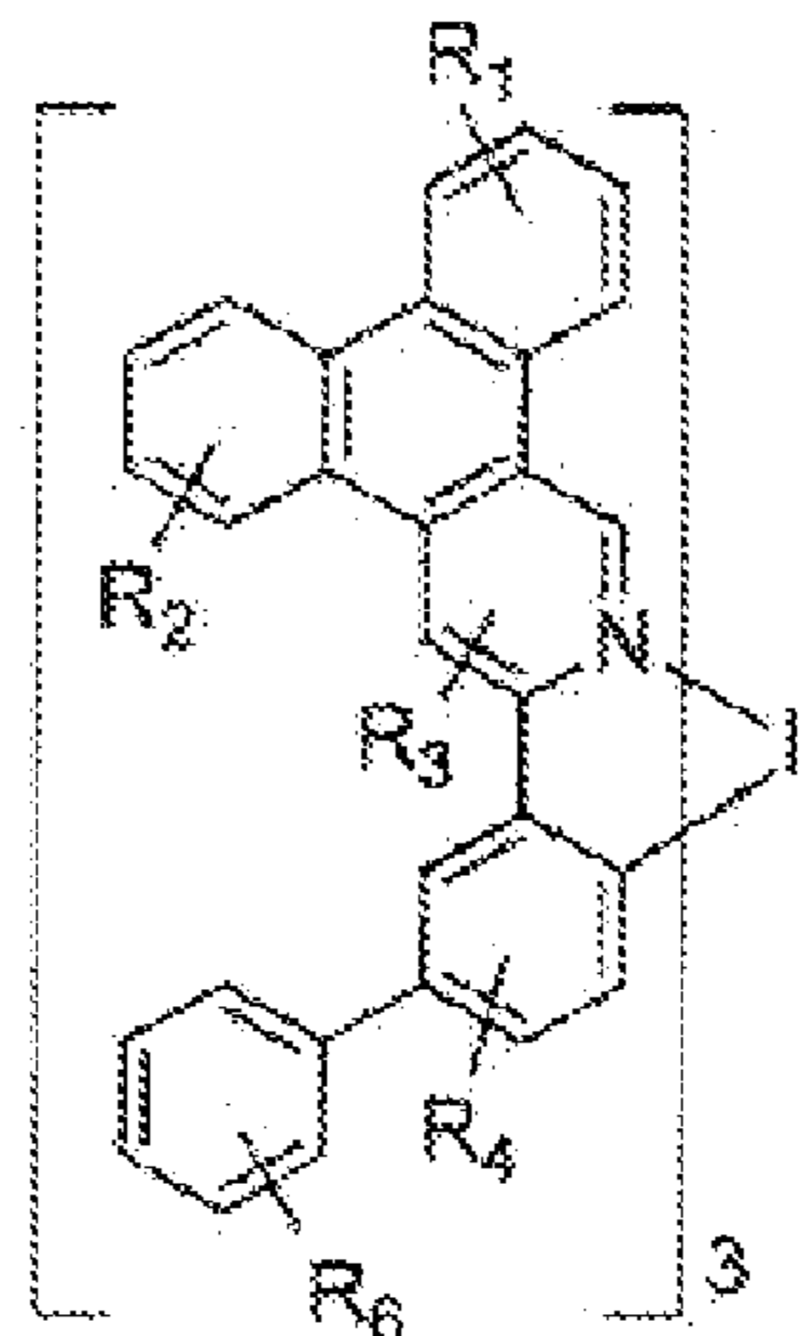
Compound 80
