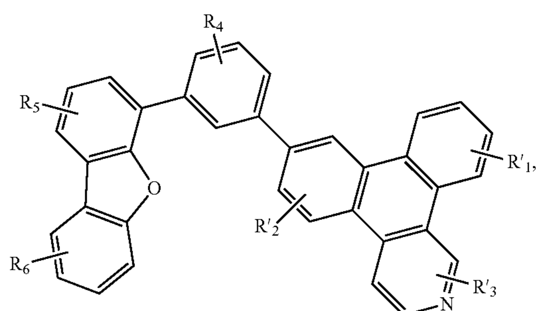
Compound 34G
