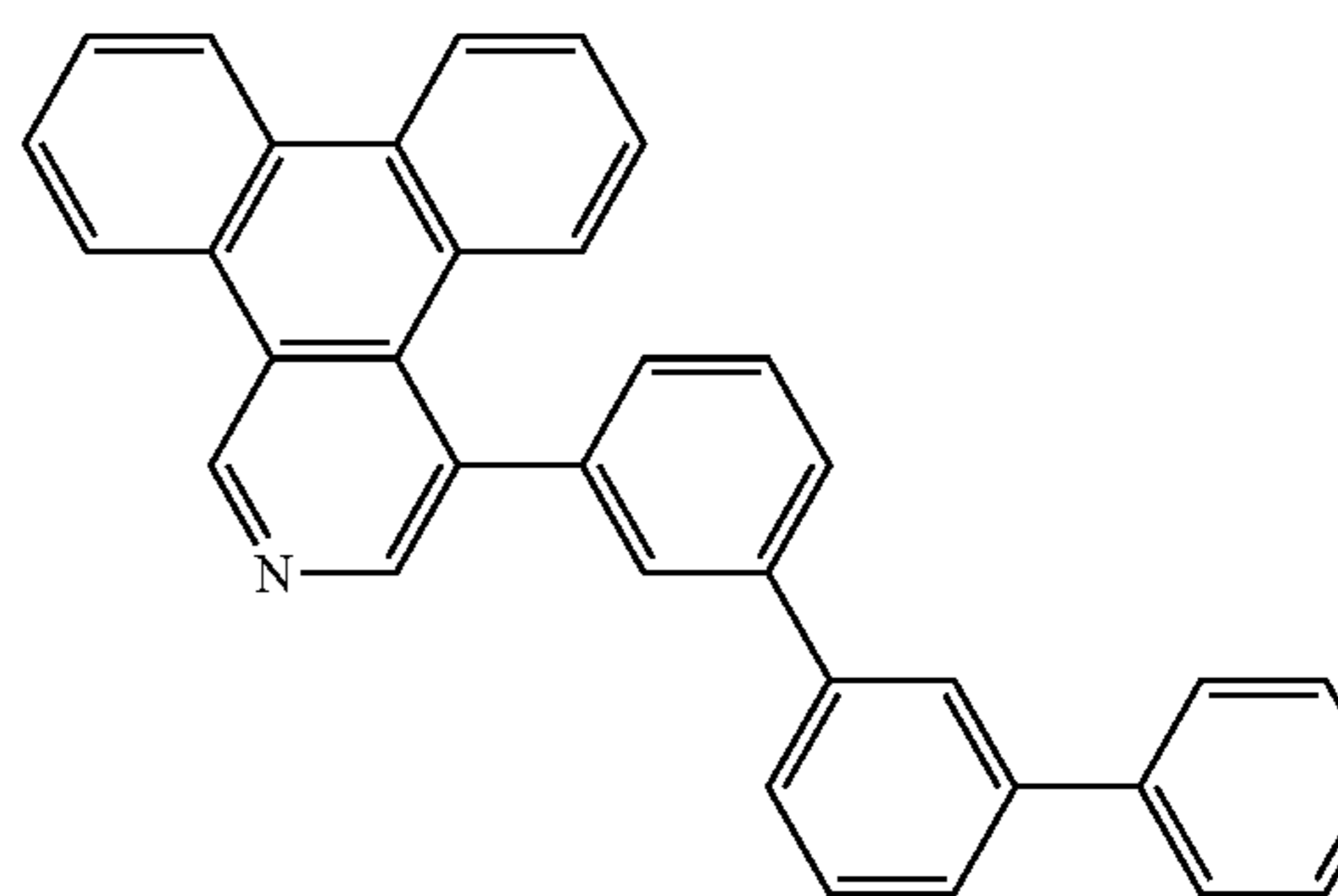
Compound 18
