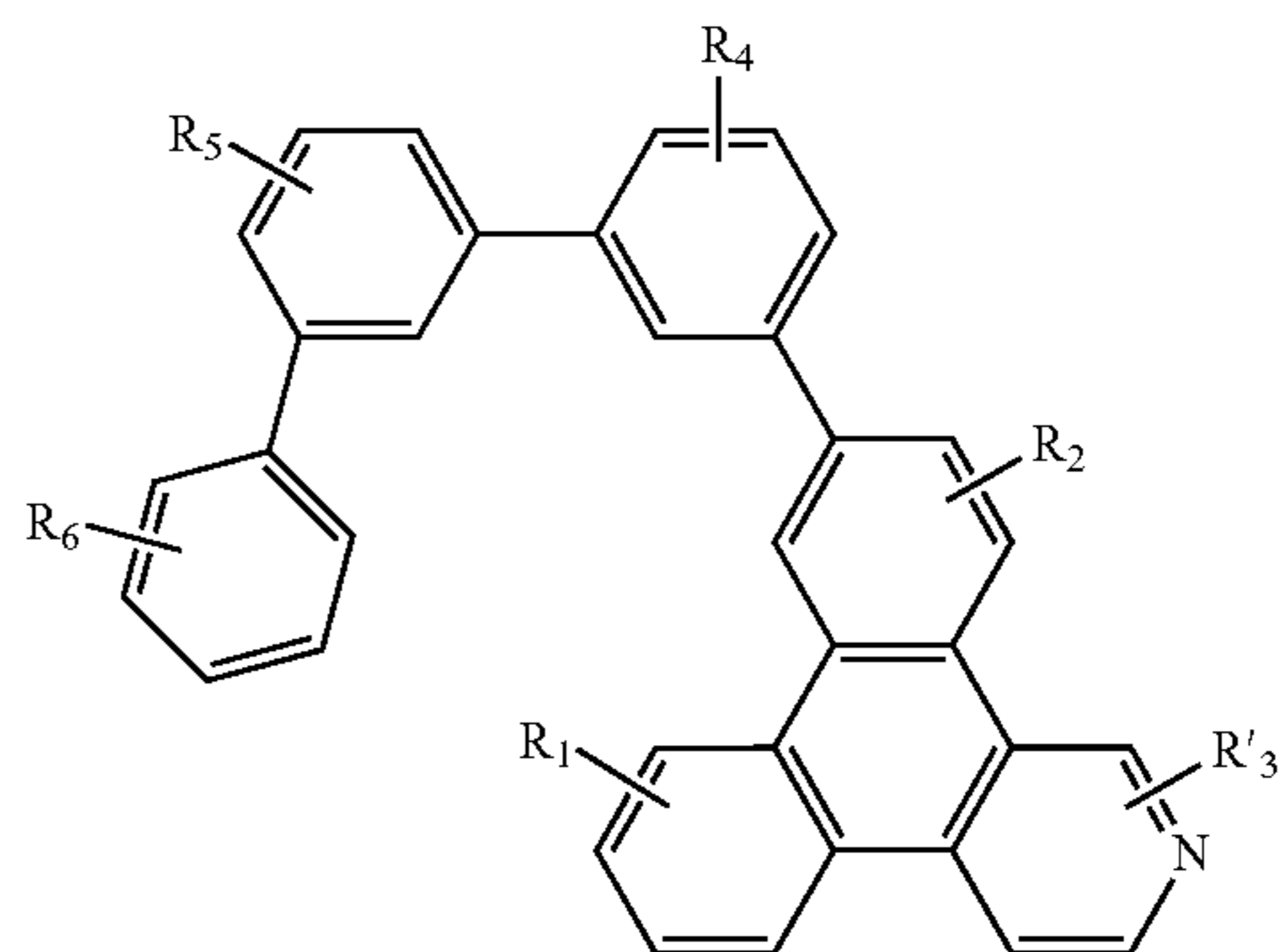
Compound 29G
