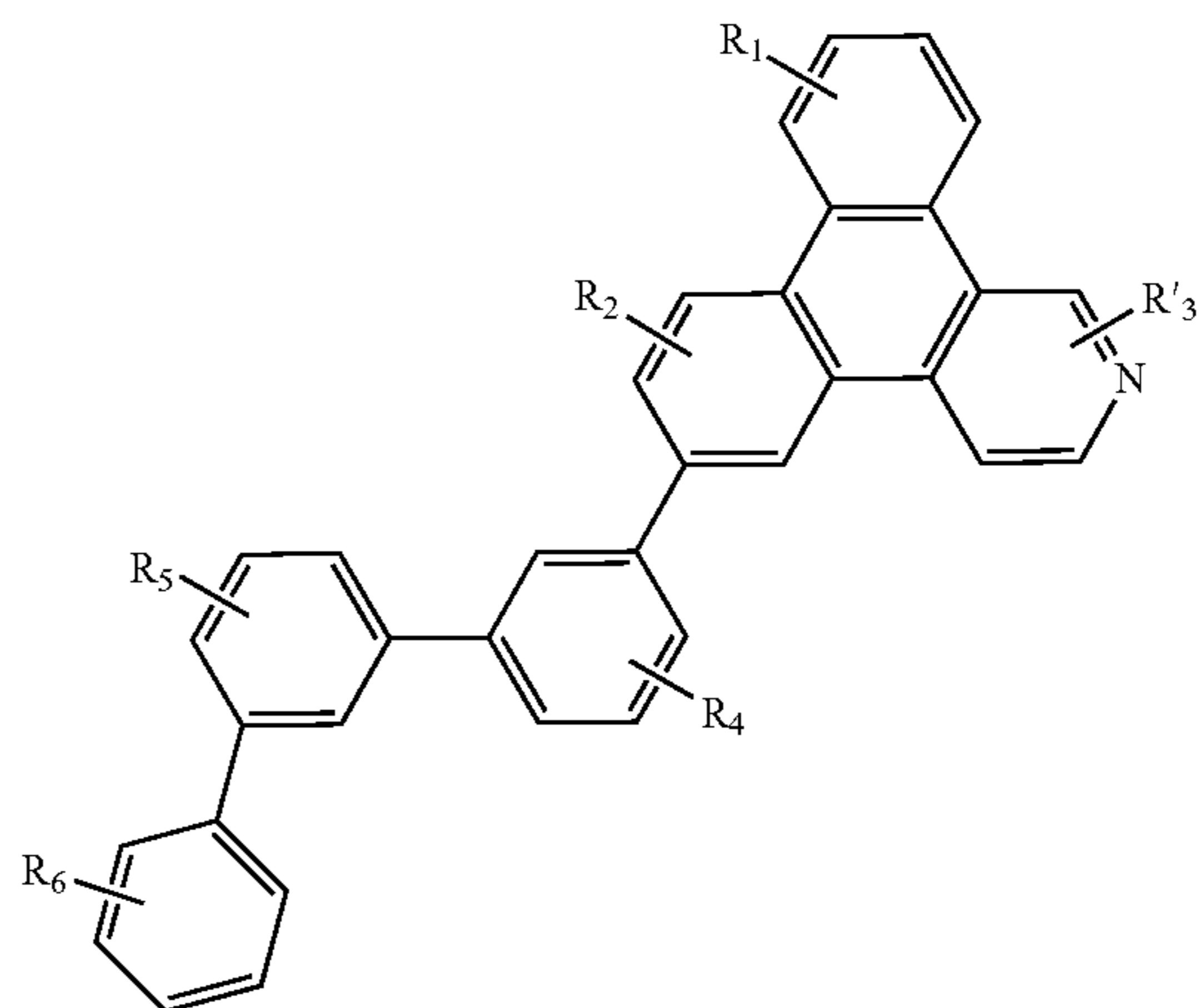
Compound 30G
