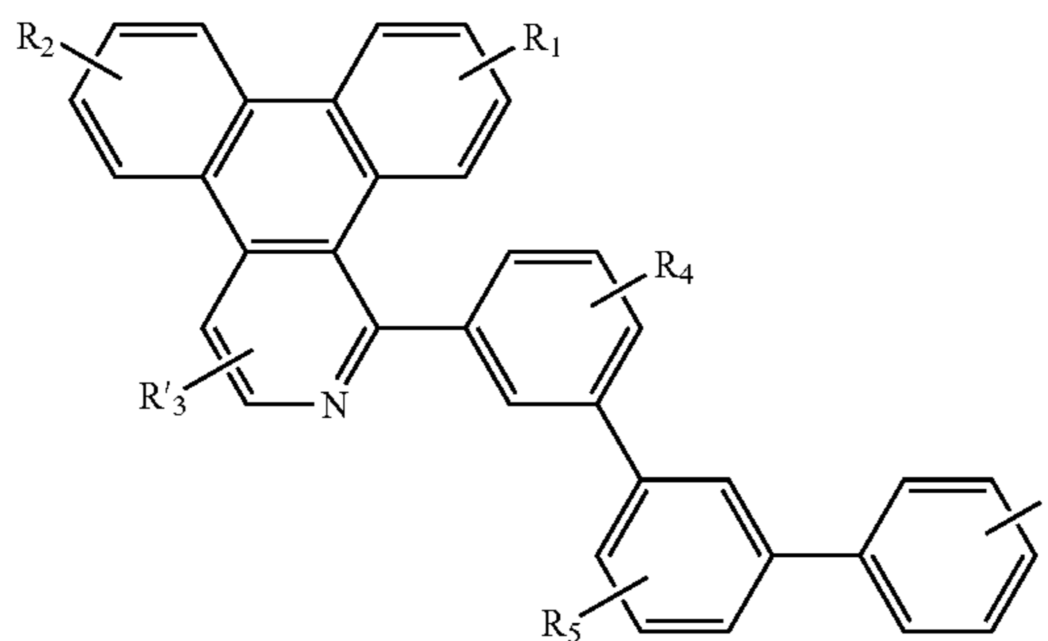
Compound 17G
