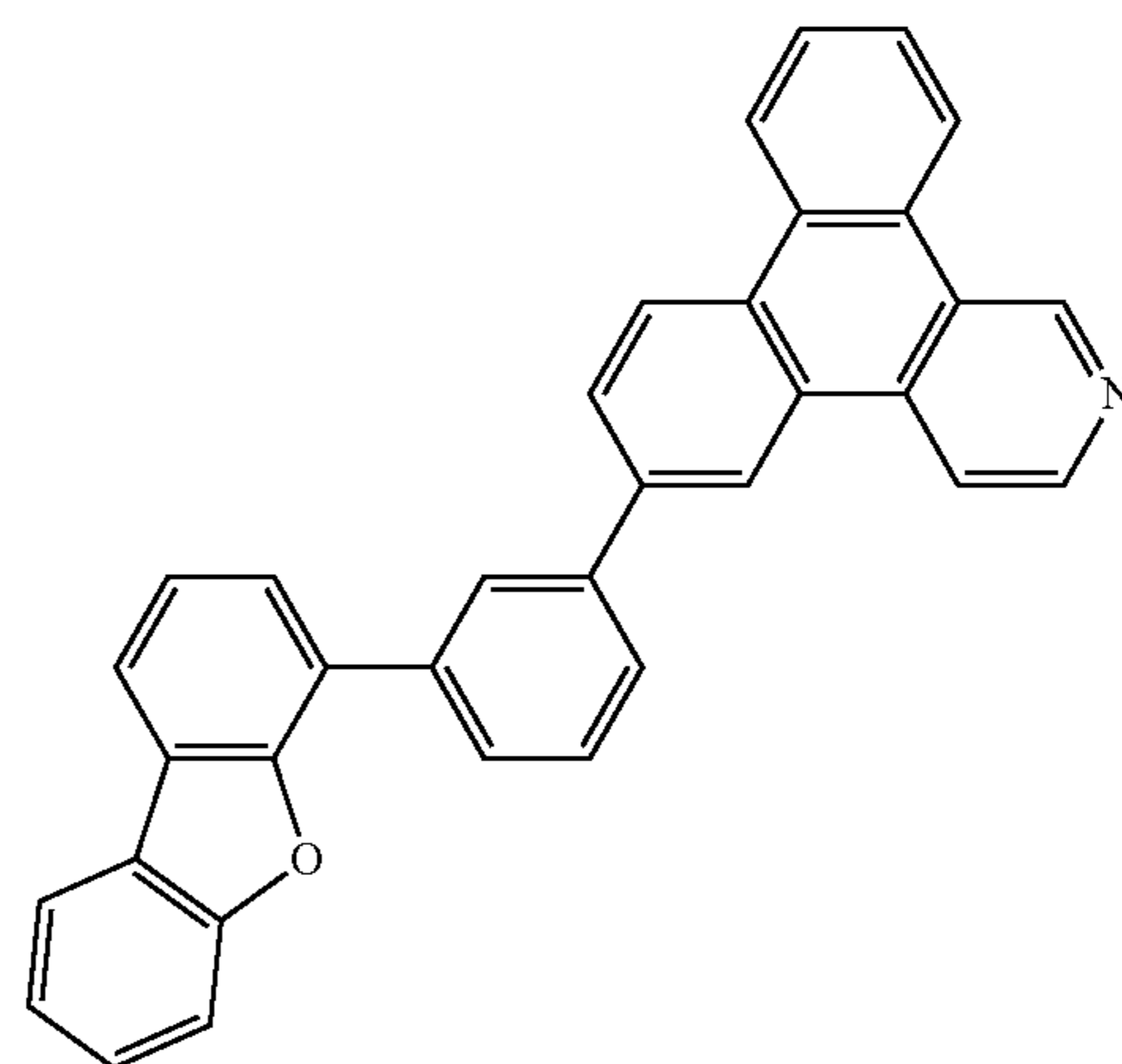
Compound 34
