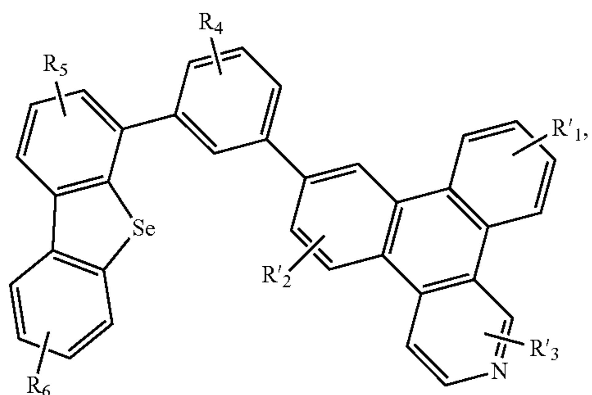
Compound 58G
