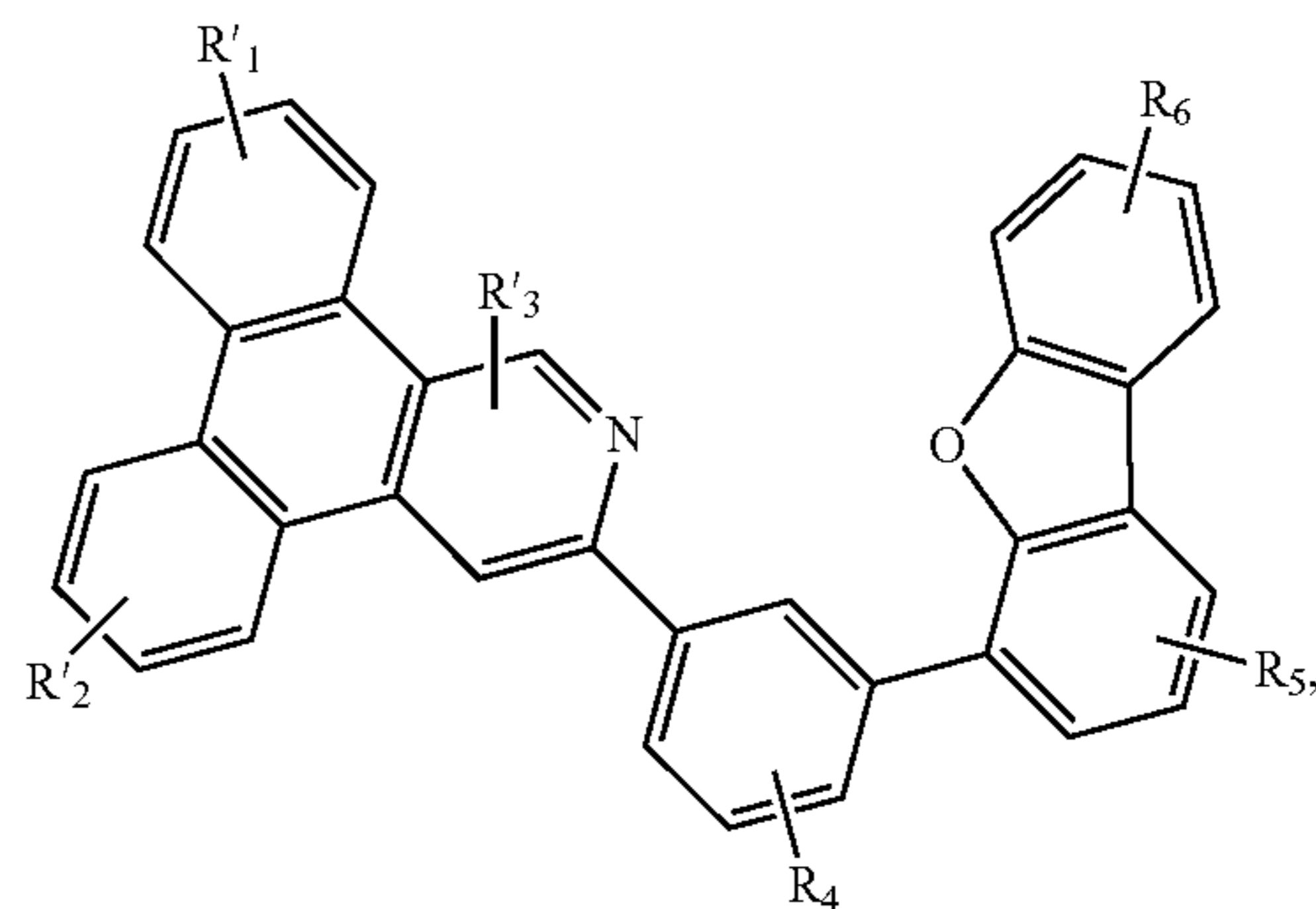
Compound 3G
