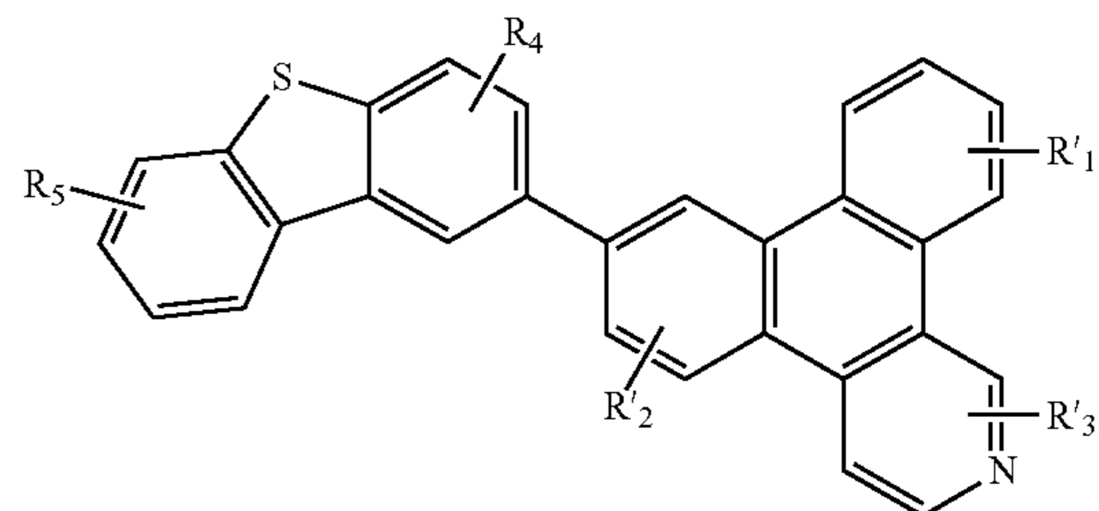
Compound 53G
