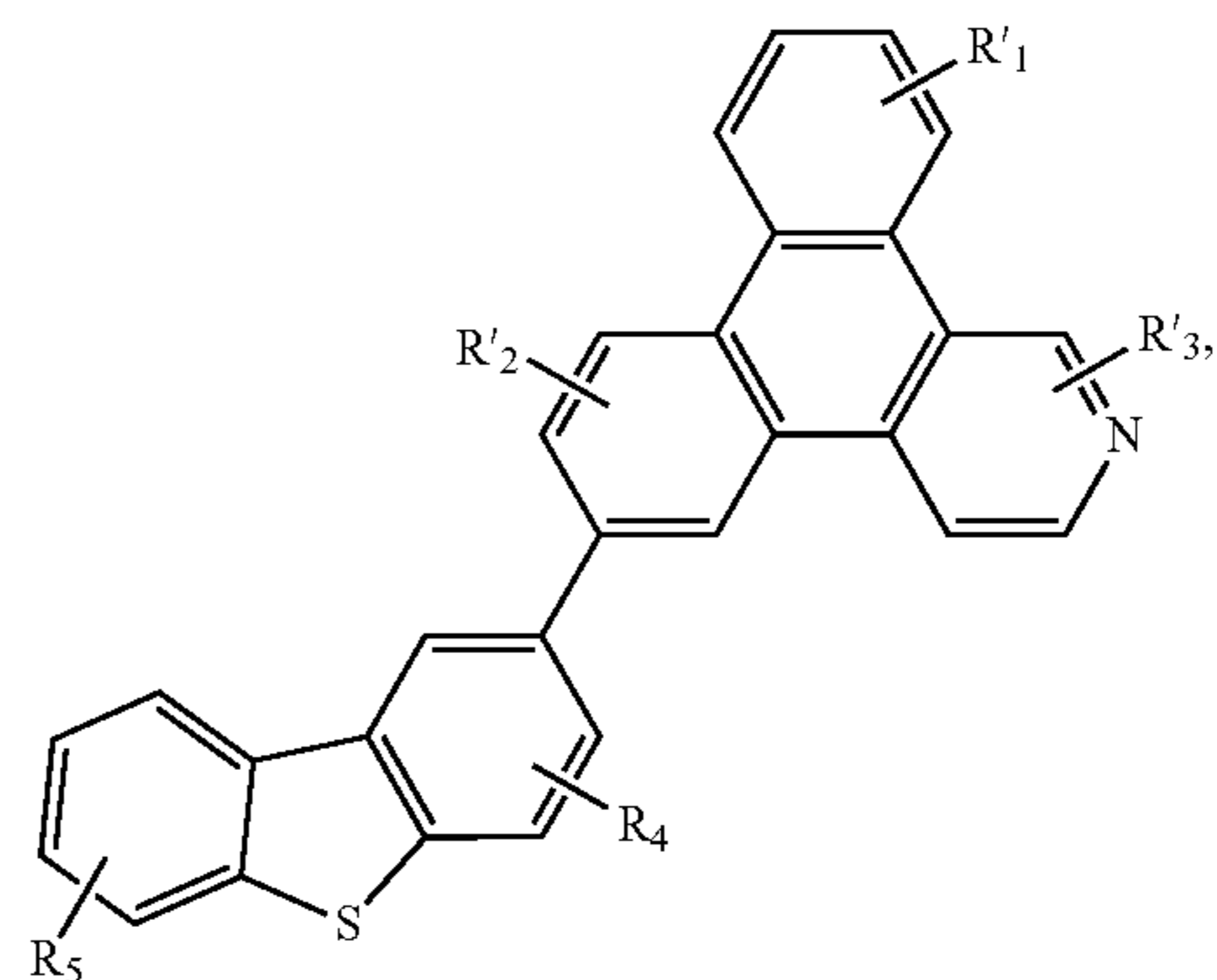
Compound 54G
