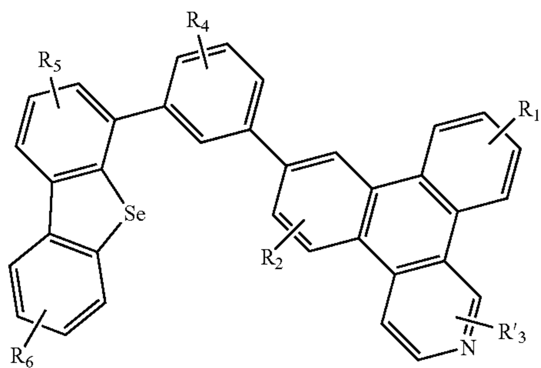
Compound 57G
