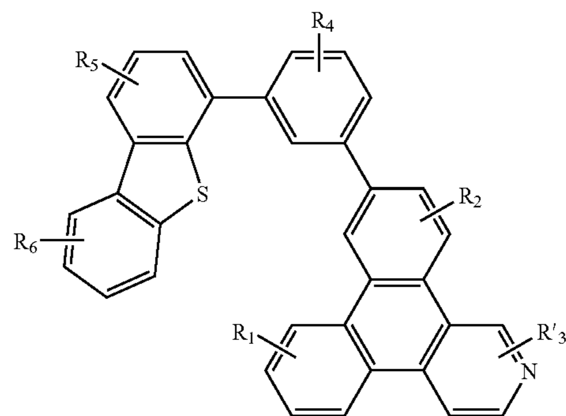
Compound 21G
