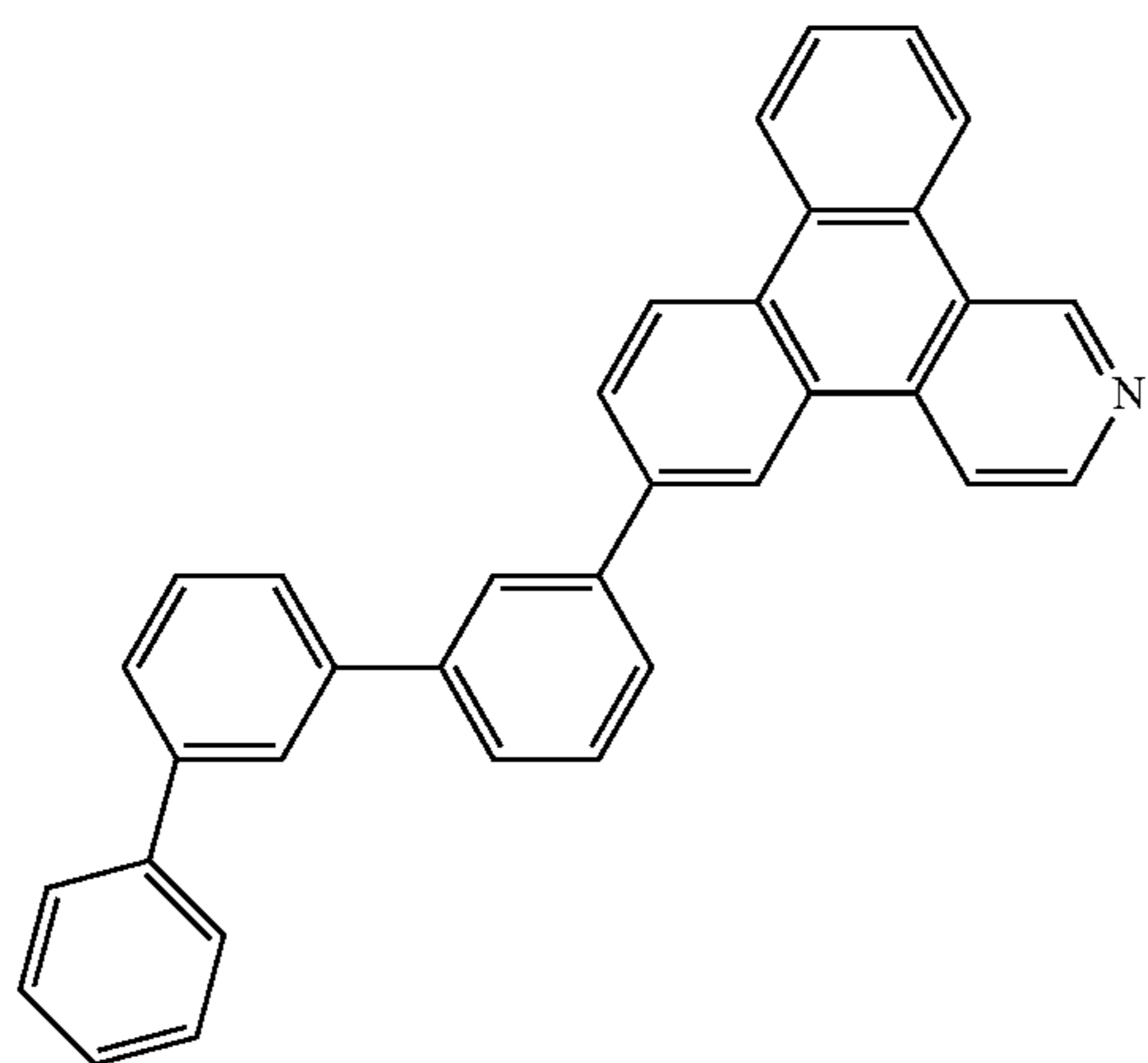
Compound 30
