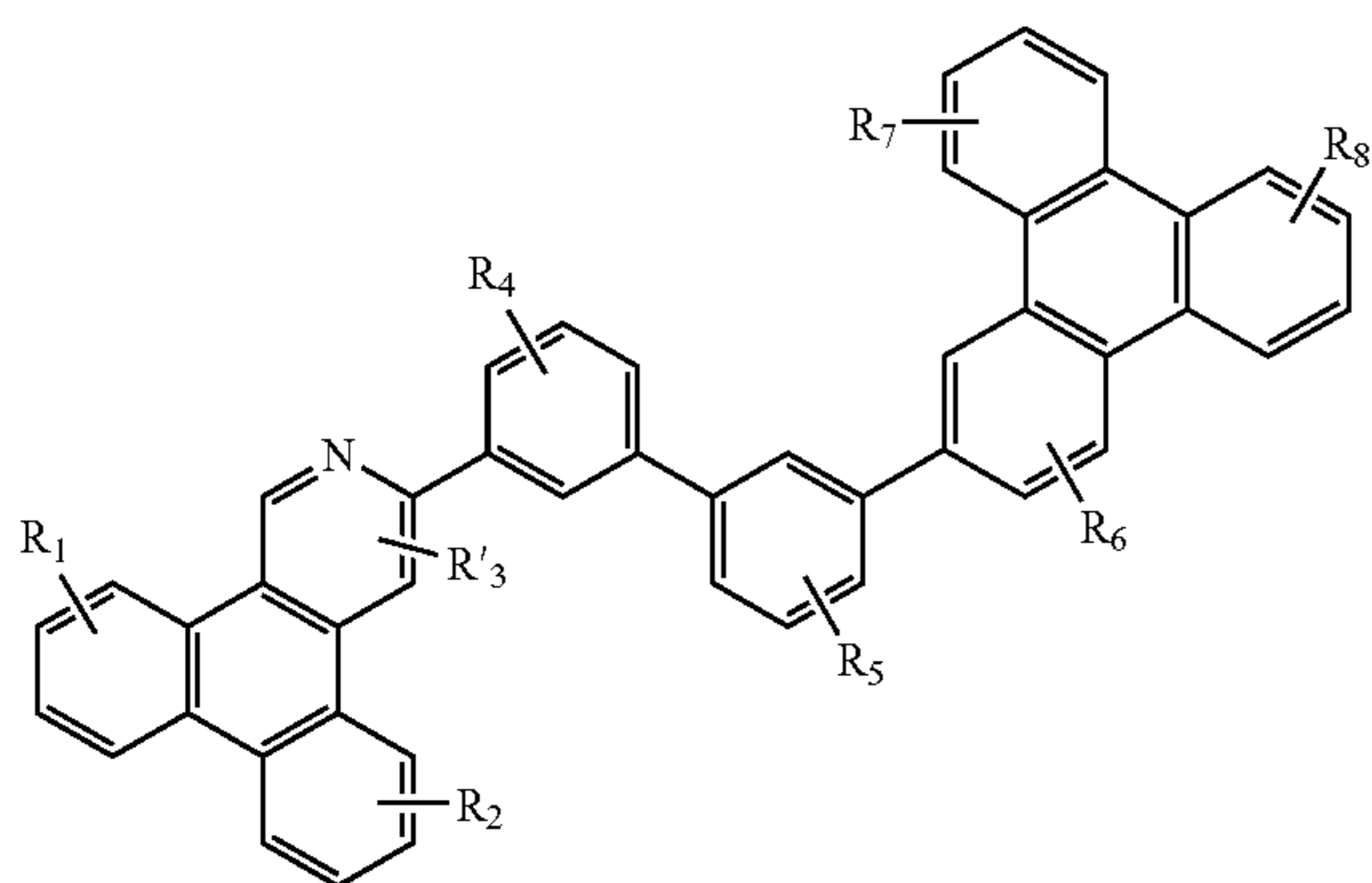
Compound 8G
