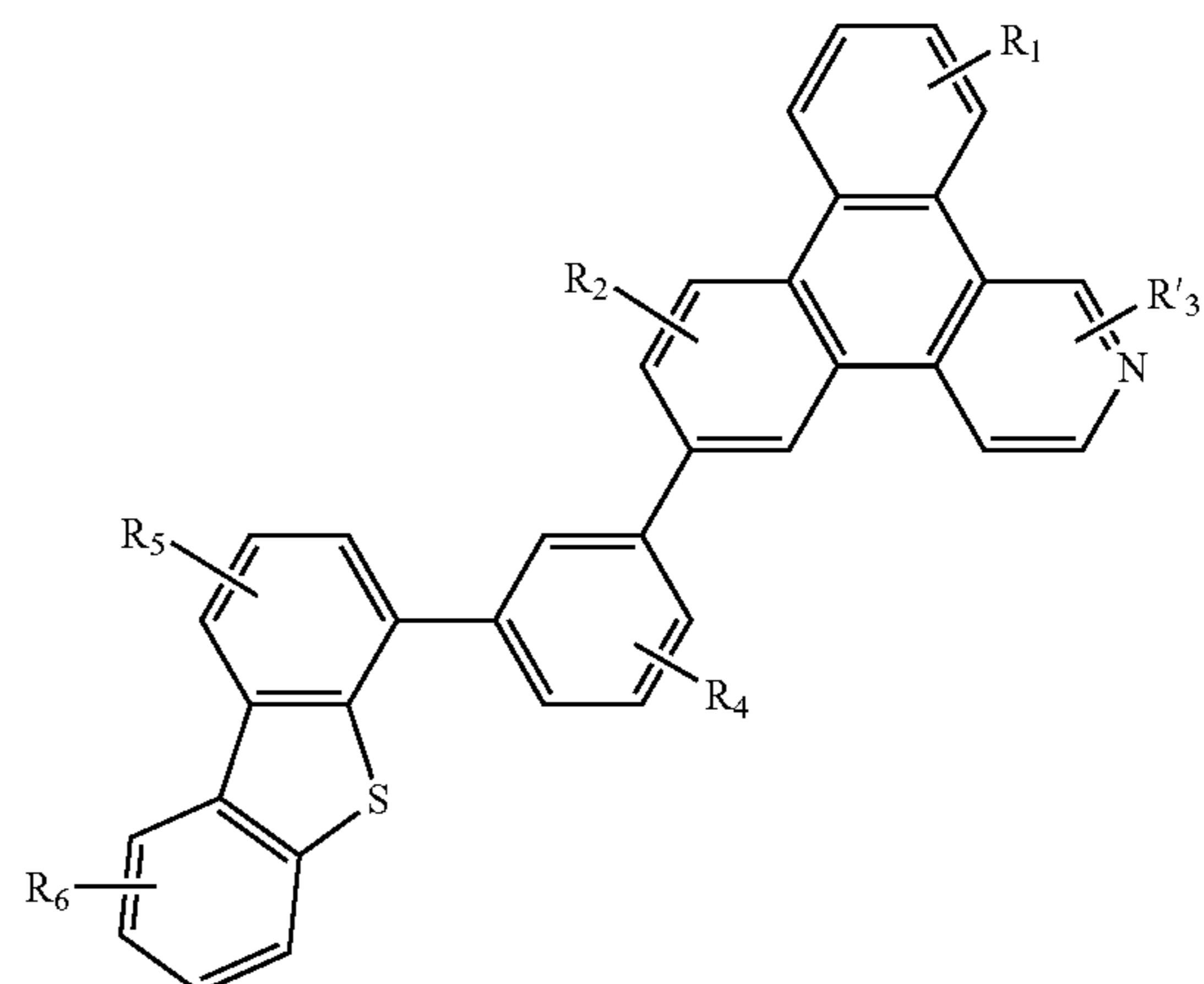
Compound 22G
