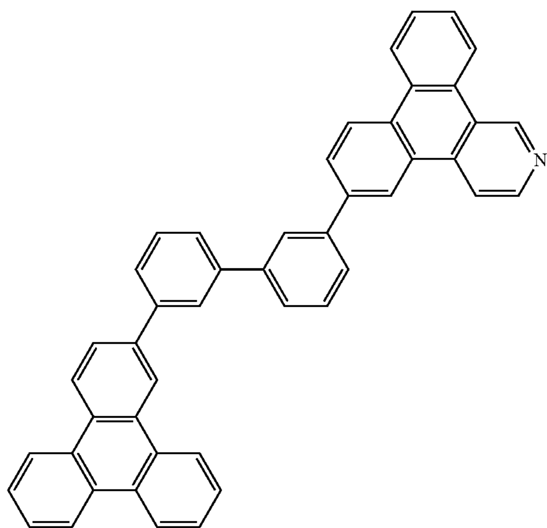
Compound 46
