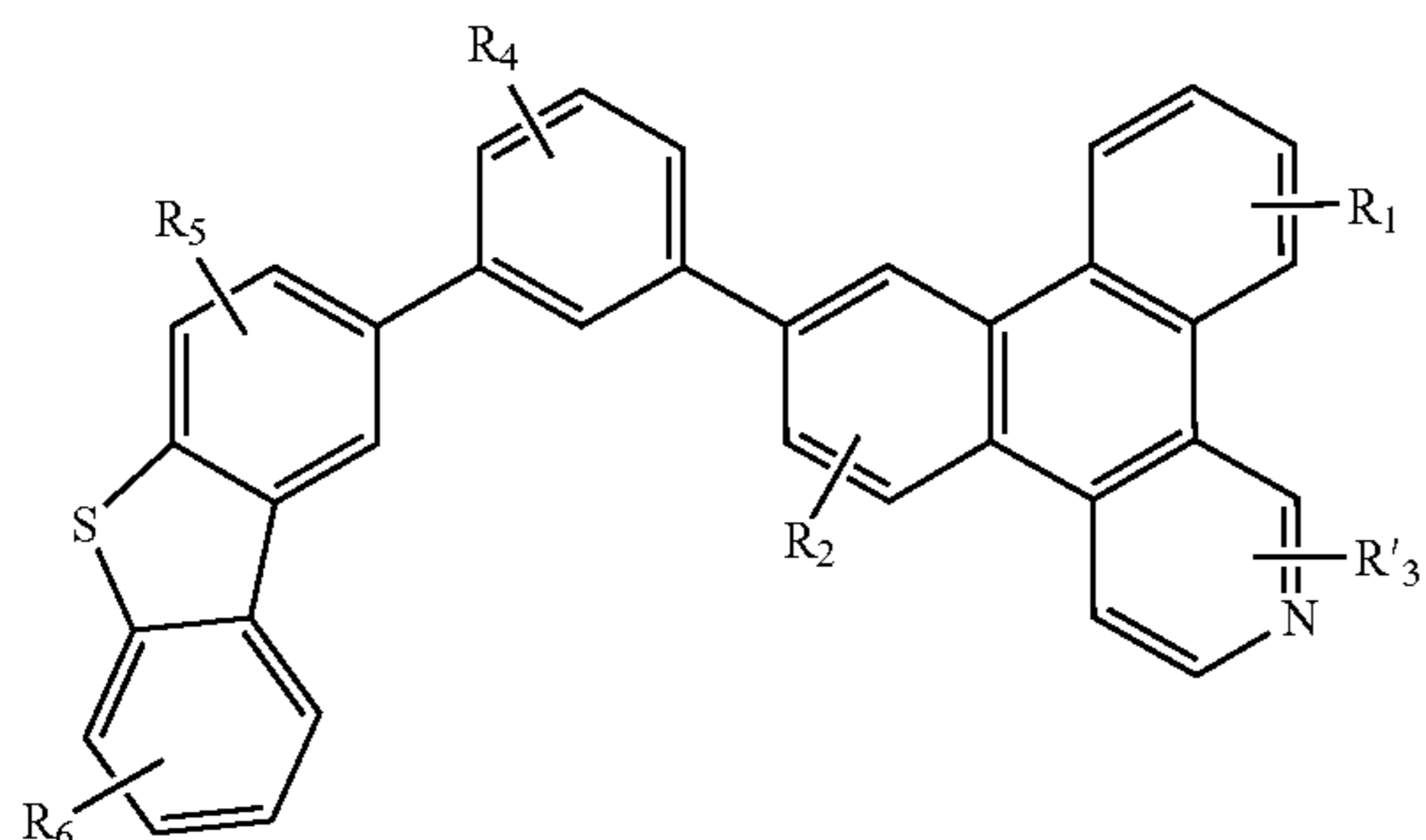
Compound 25G
