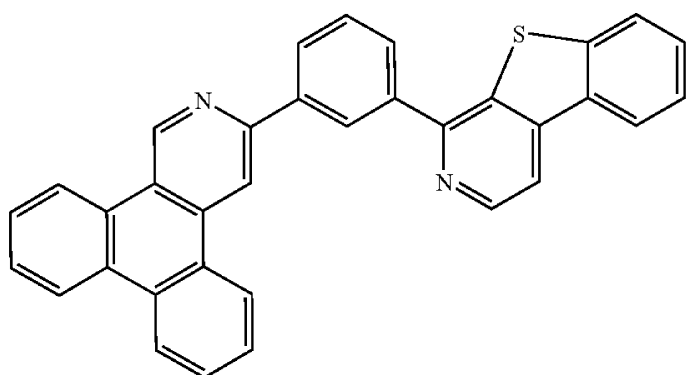
Compound 13
