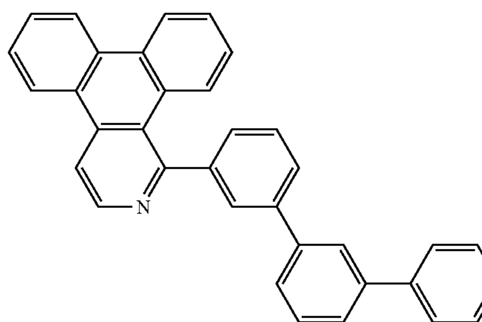
Compound 16
