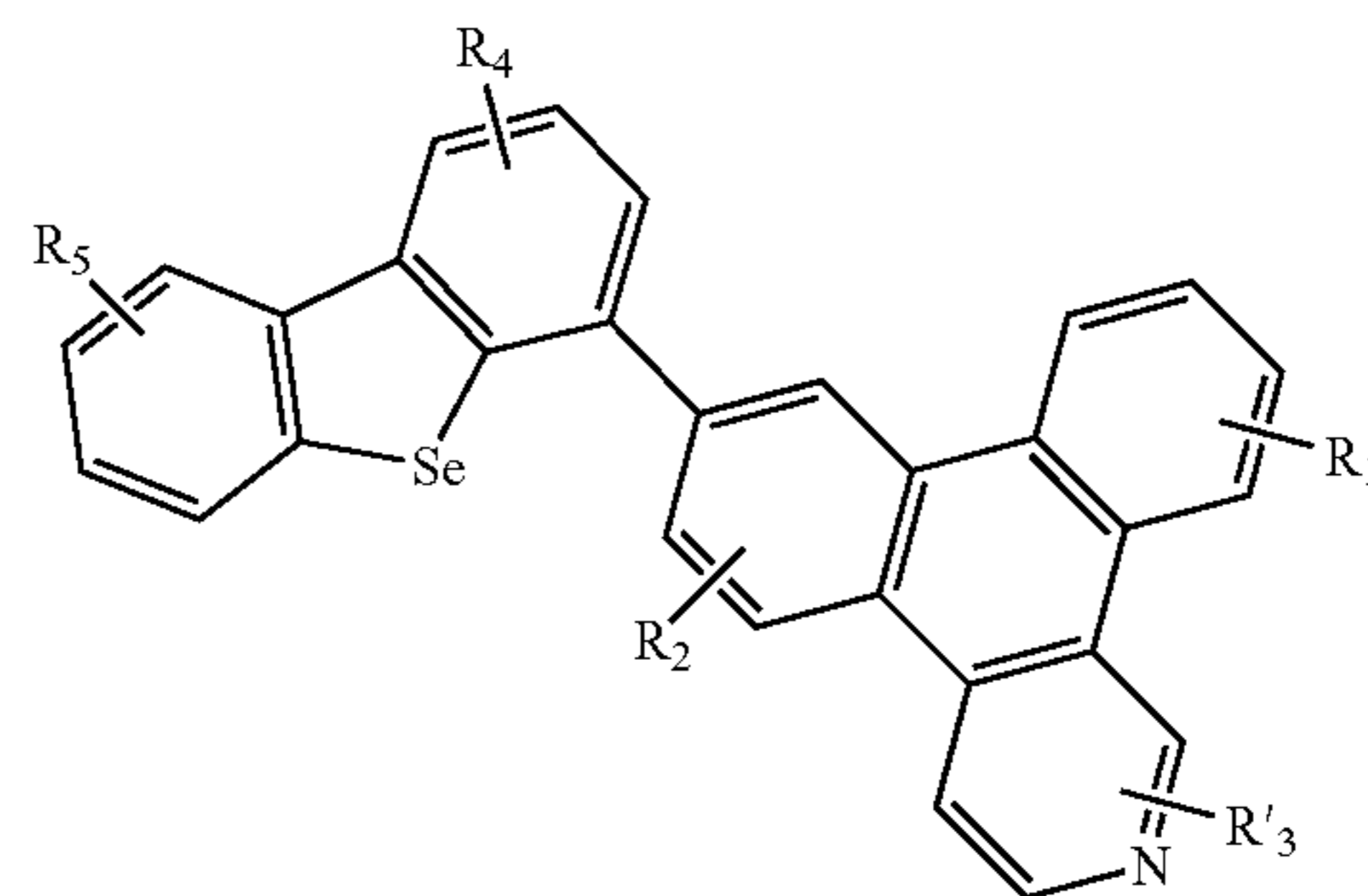
Compound 61G
