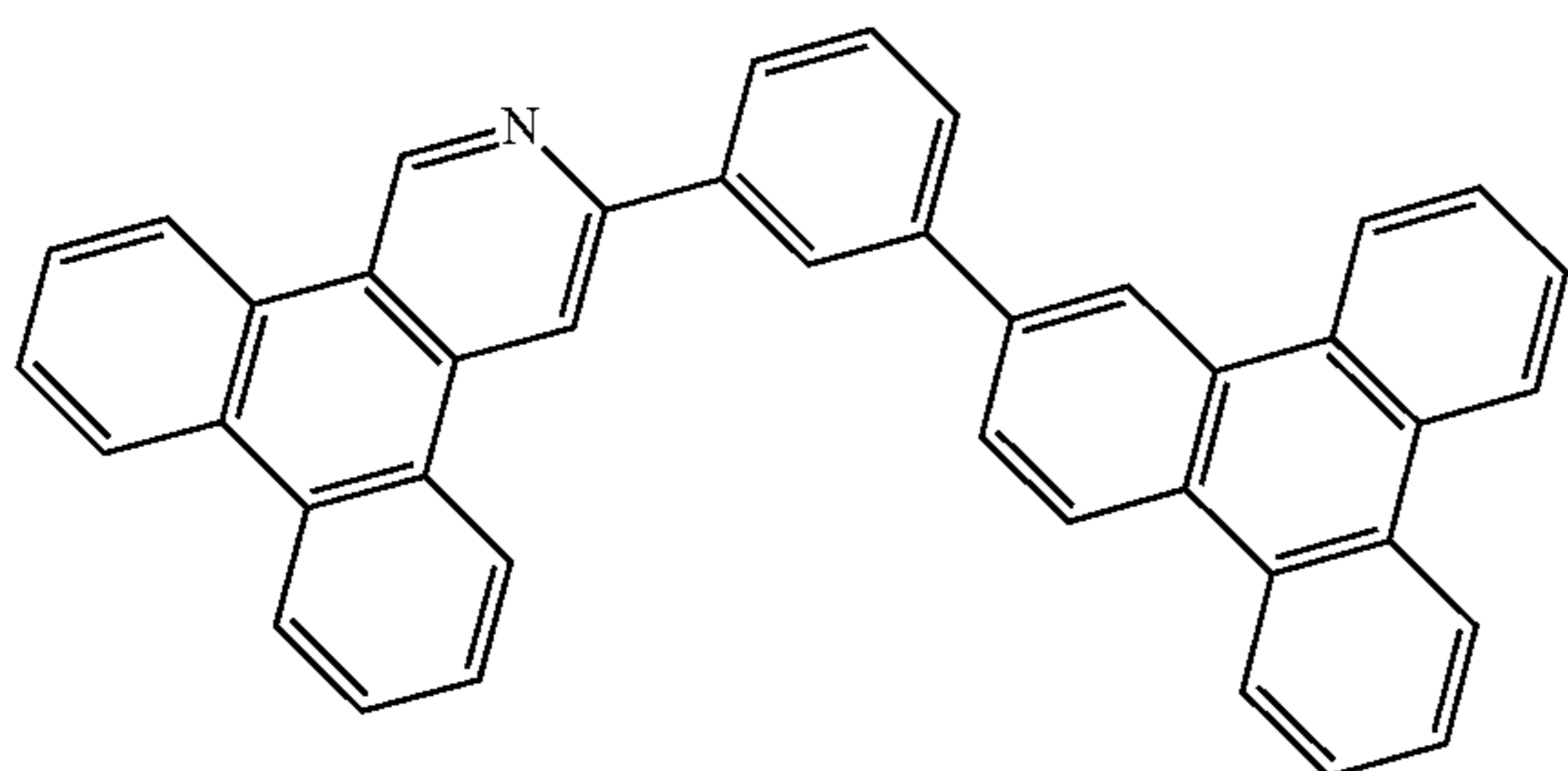
Compound 12
