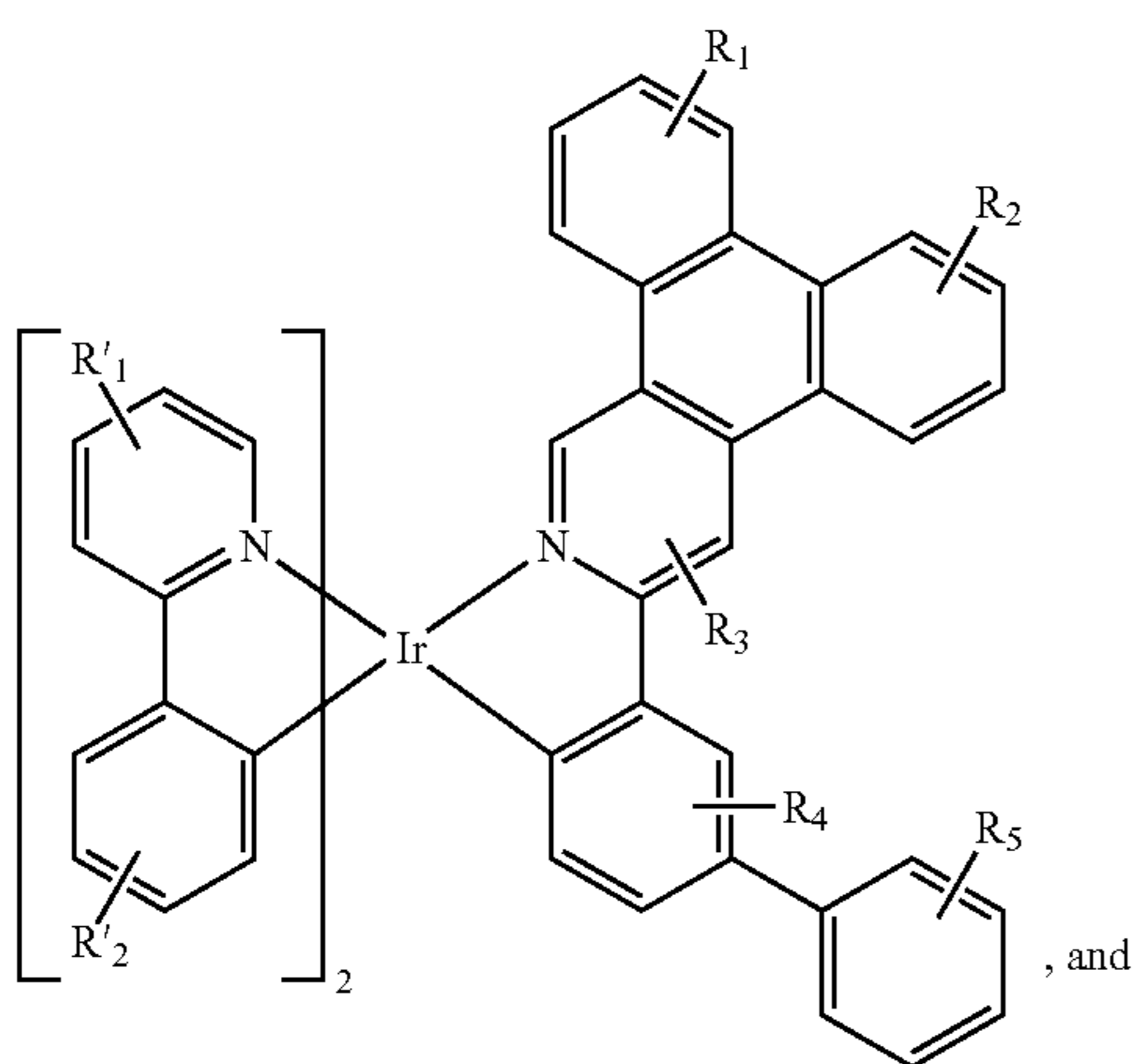
Compound 95
