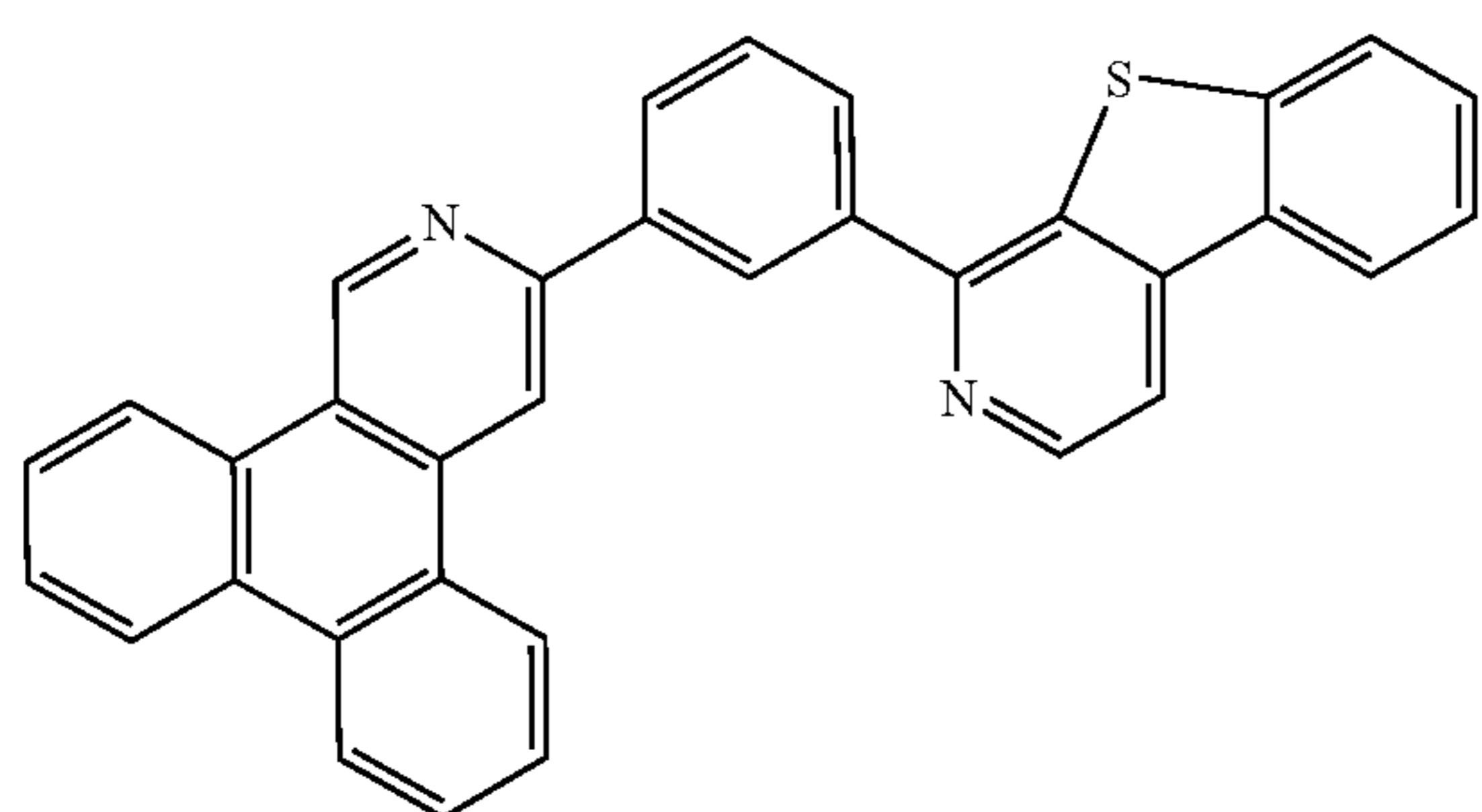
Compound 13
