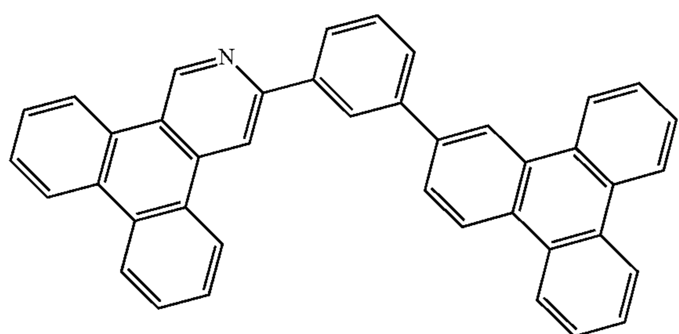
Compound 12
