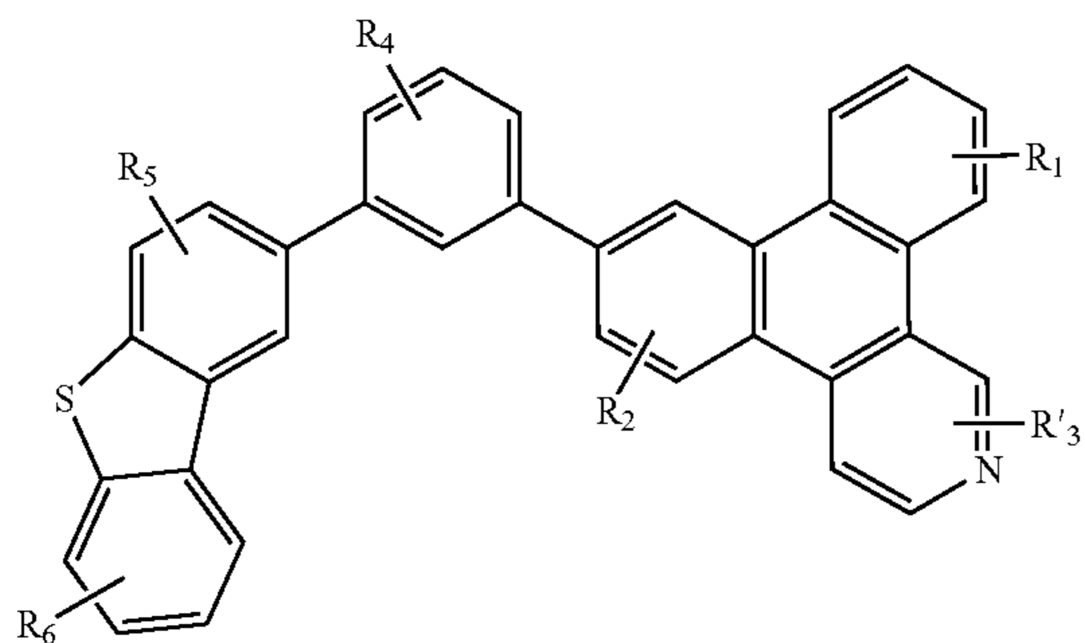
Compound 25G
