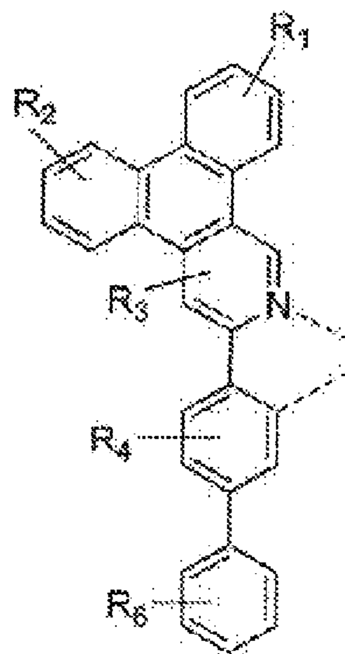
Compound 73G
