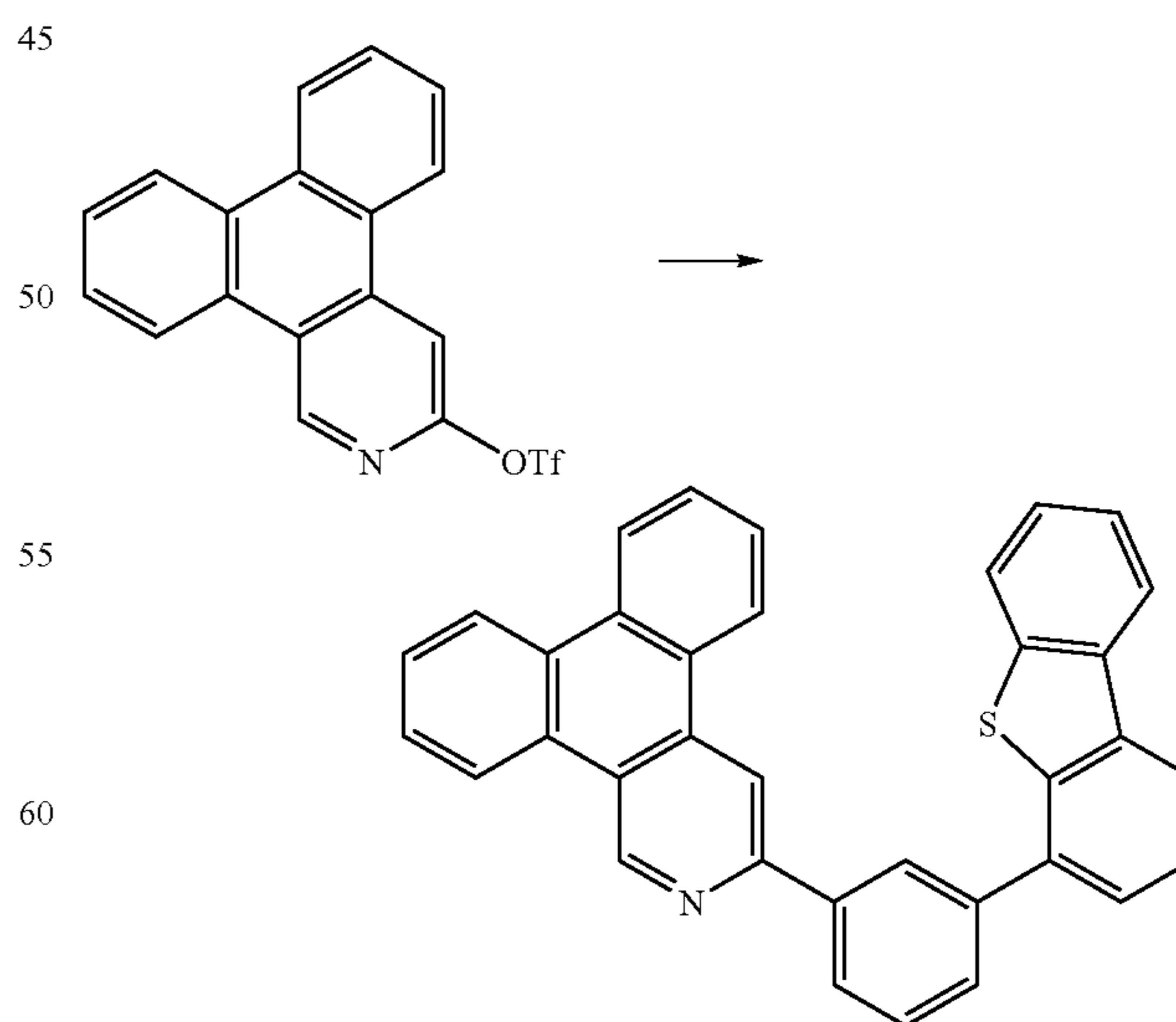
Compound 1
