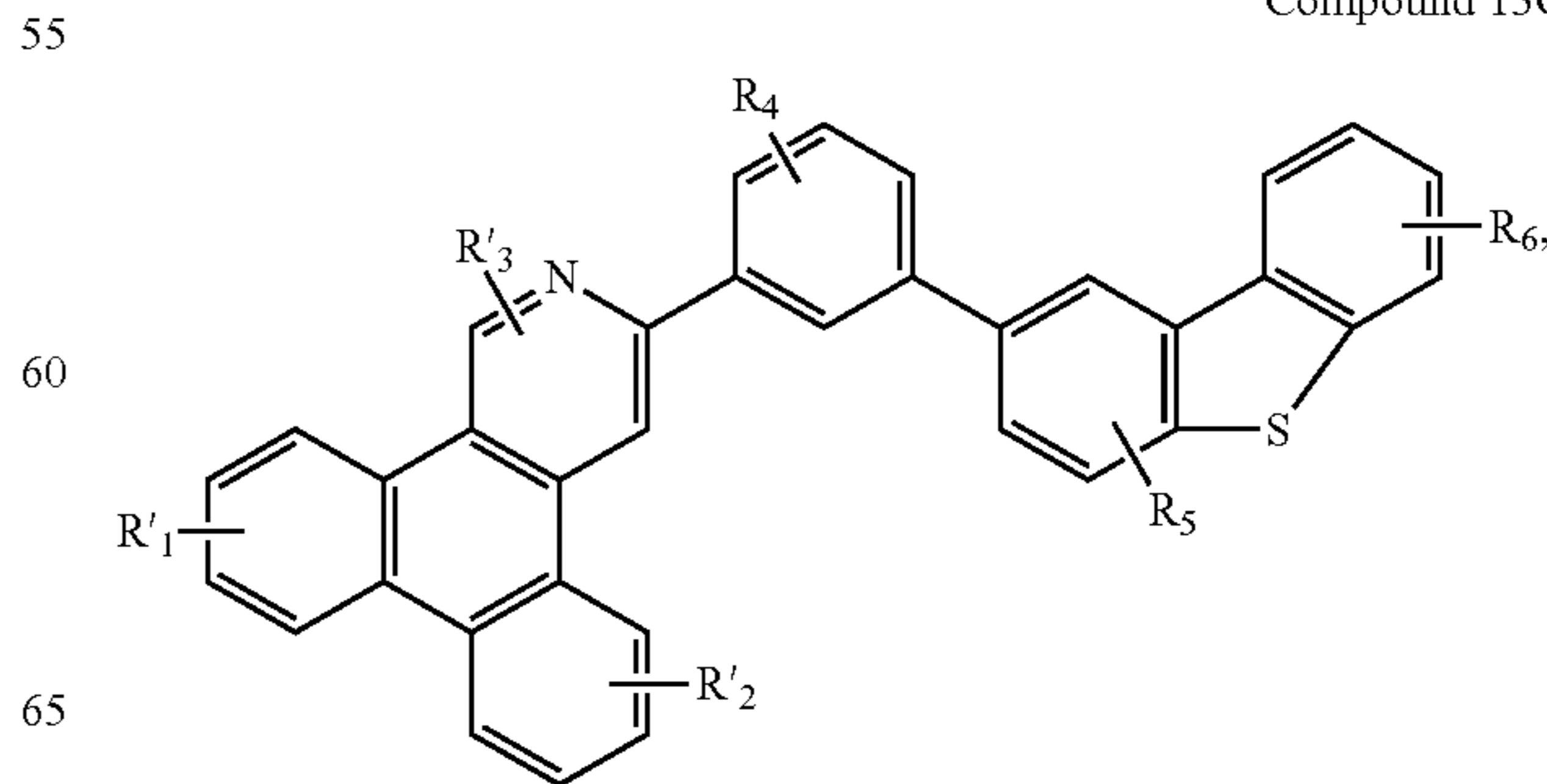
Compound 13G
