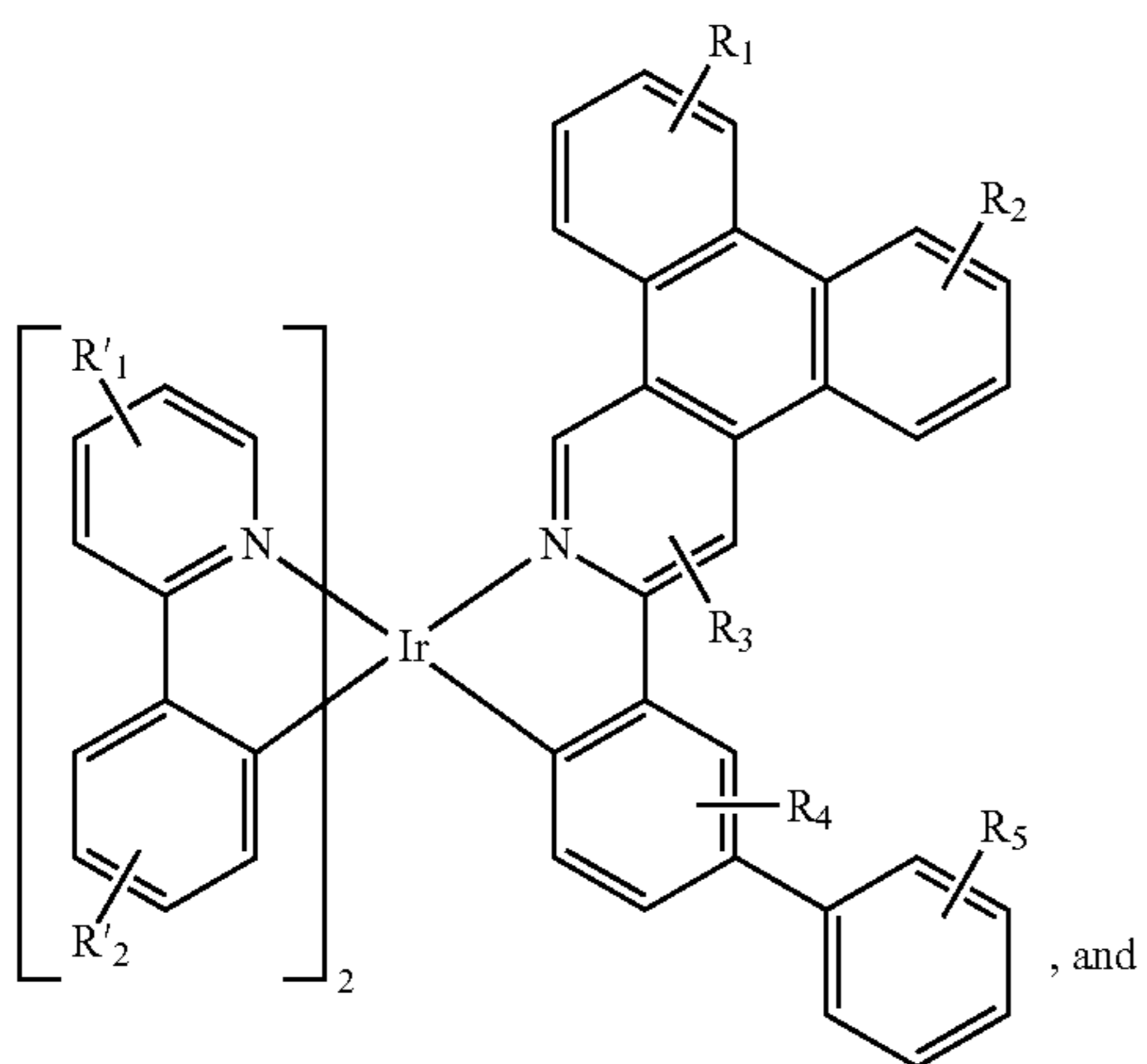
Compound 95
