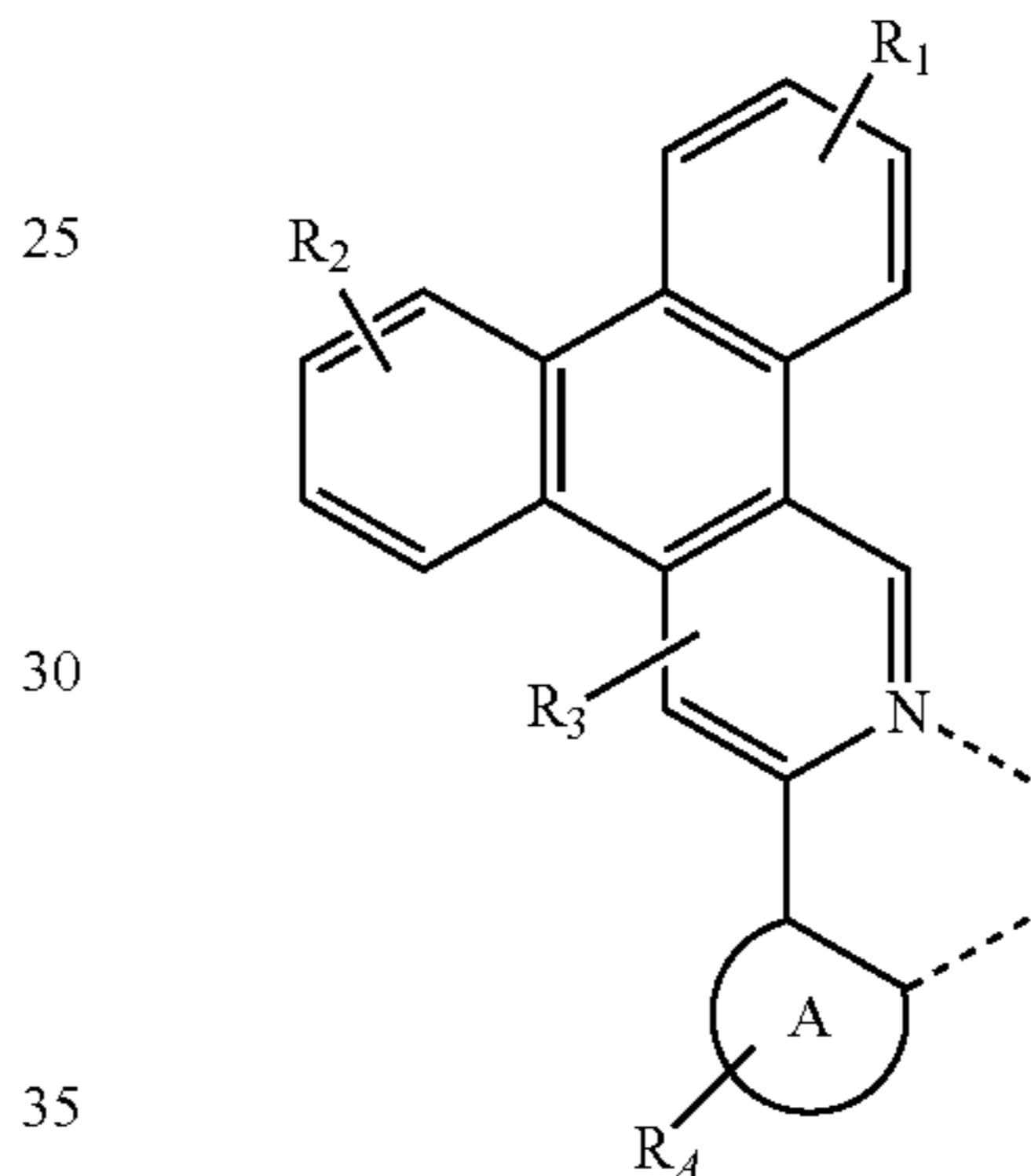
FORMULA I
