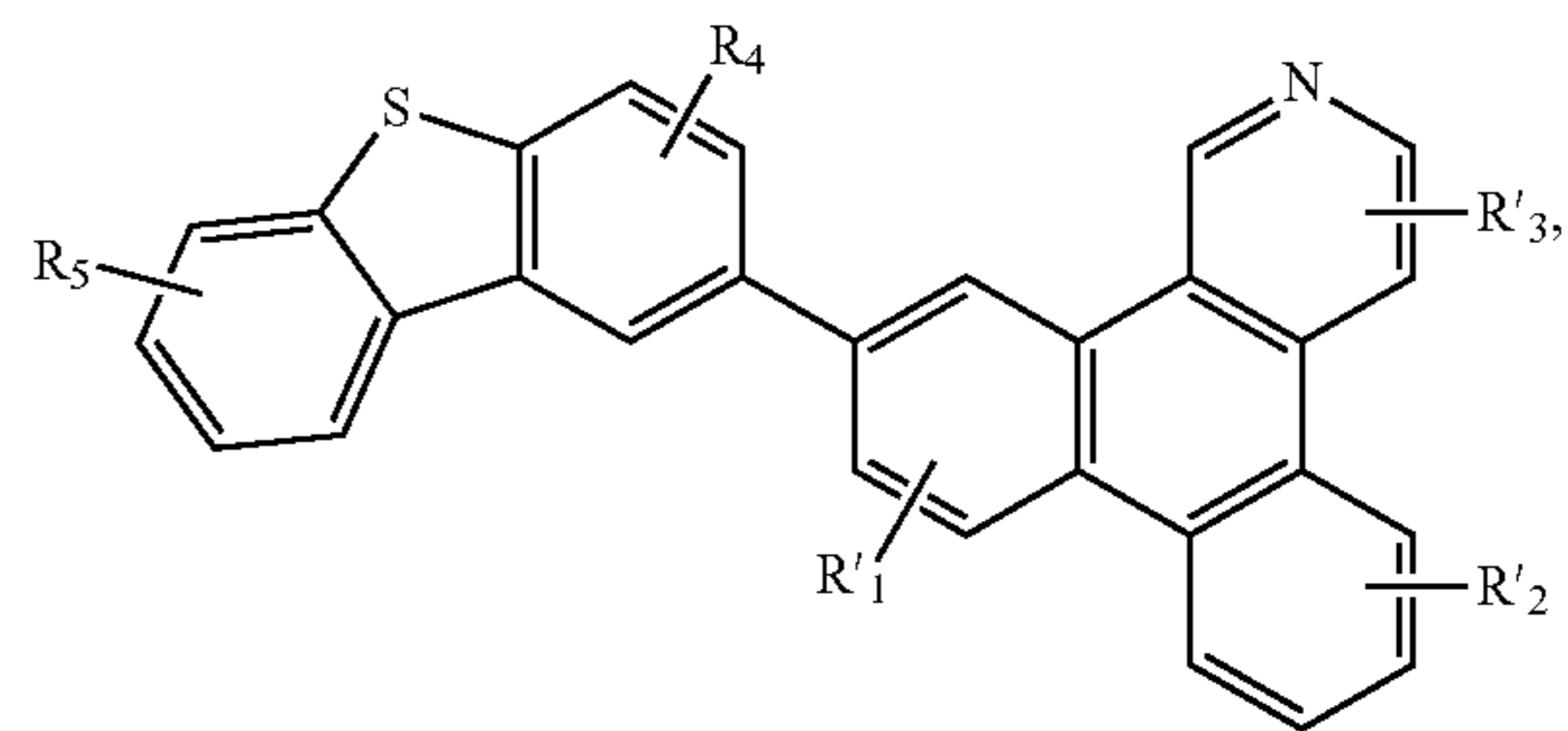
Compound 51G
