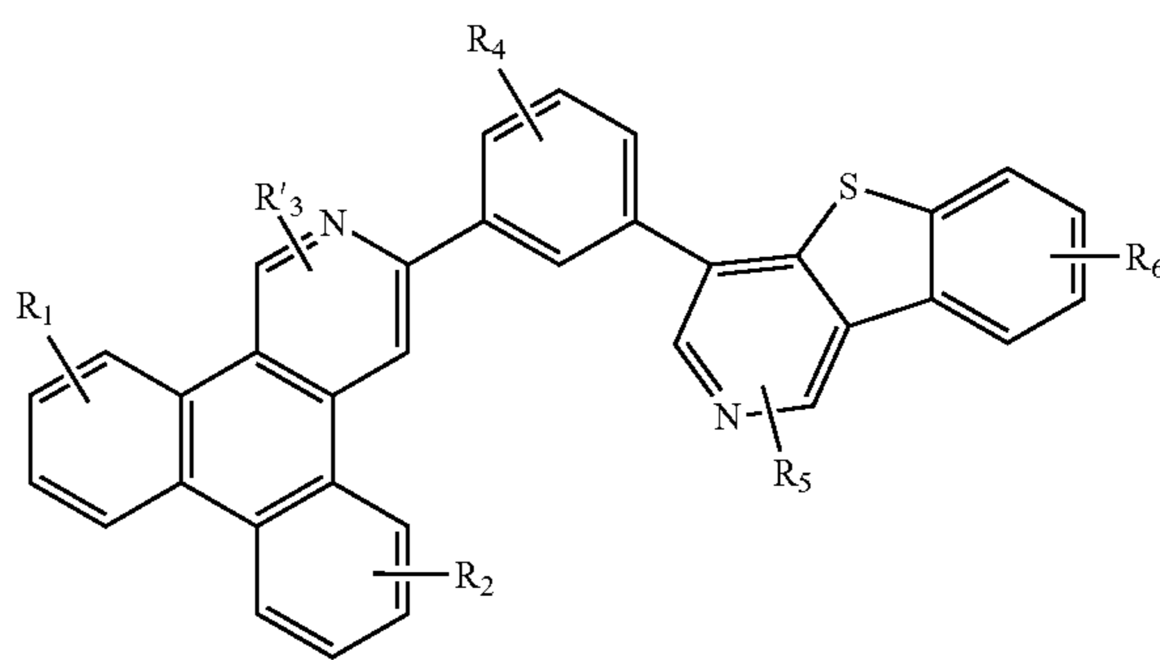
Compound 12G
