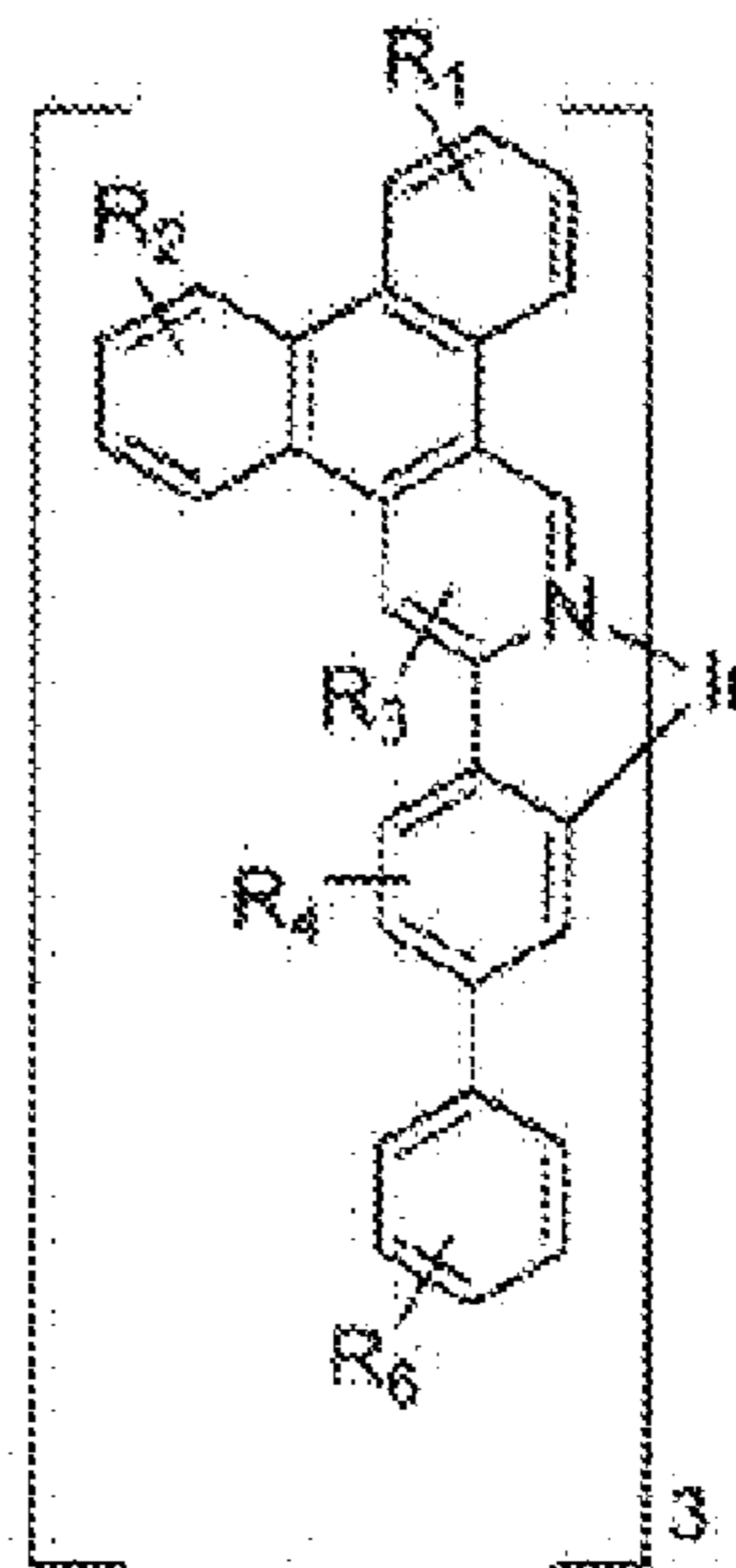
Compound 81
