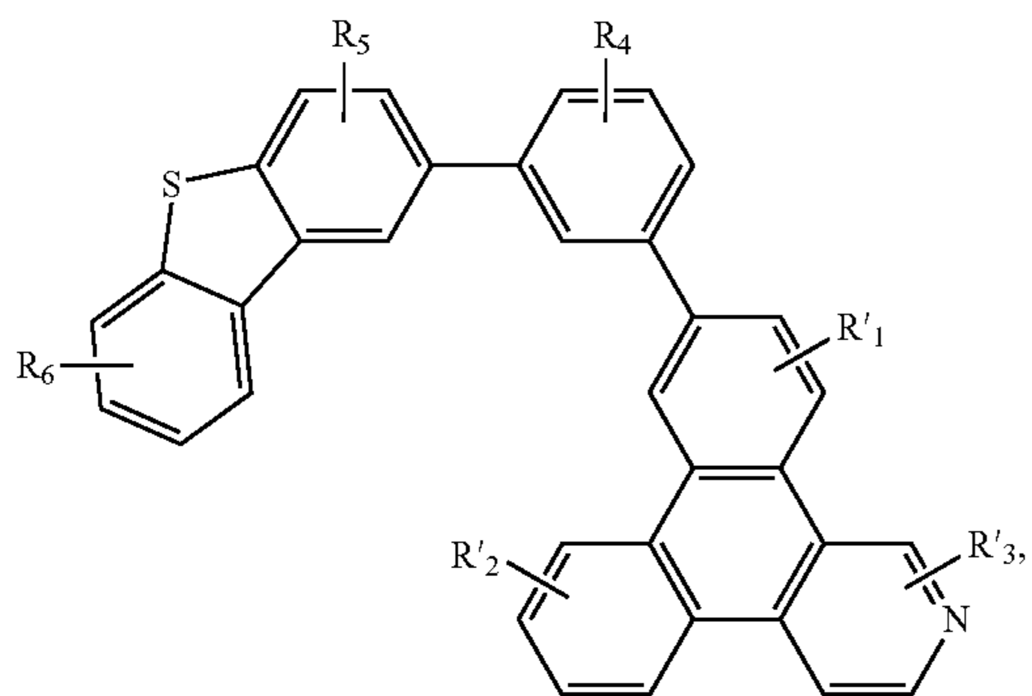
Compound 25G
