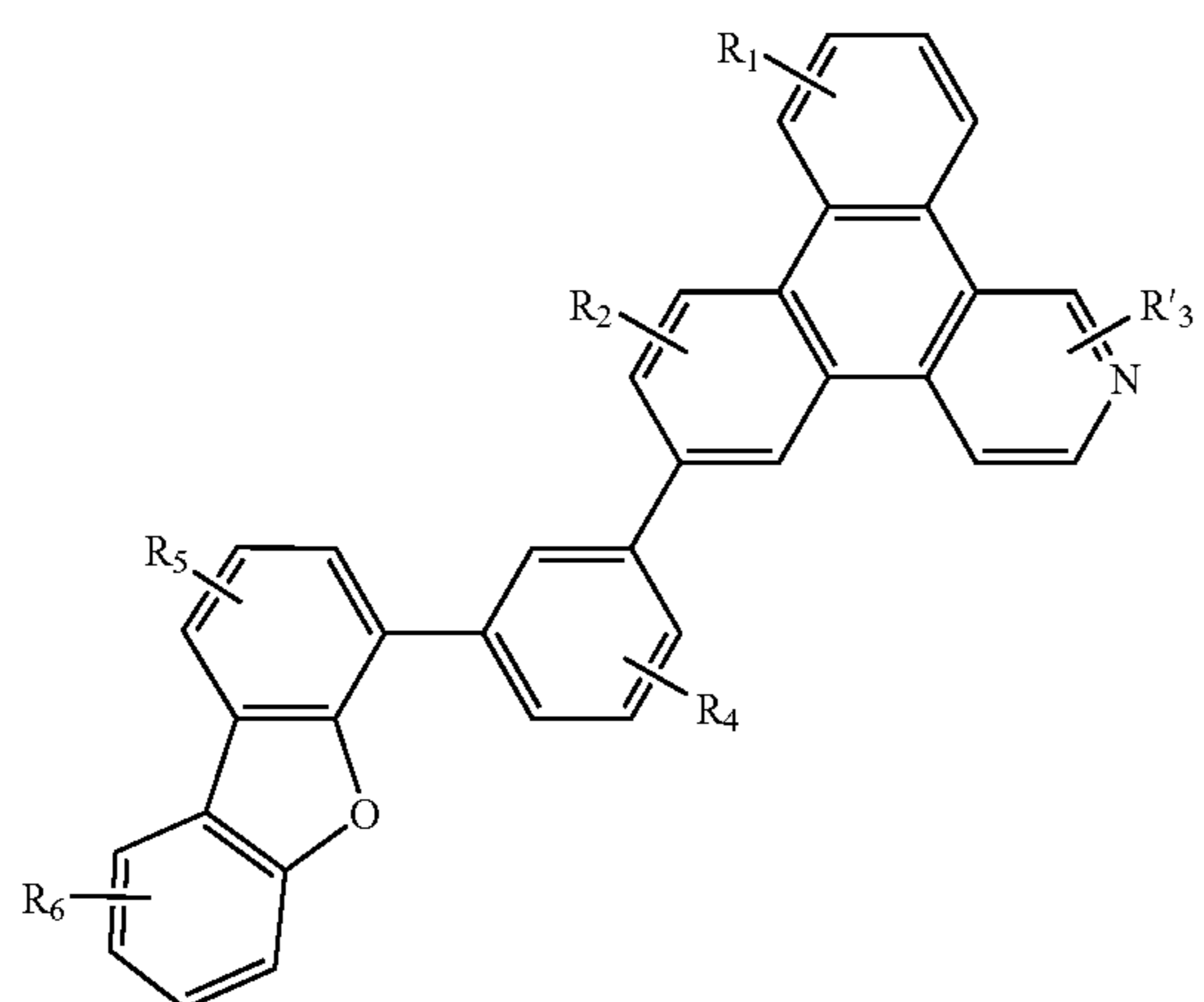
Compound 34G
