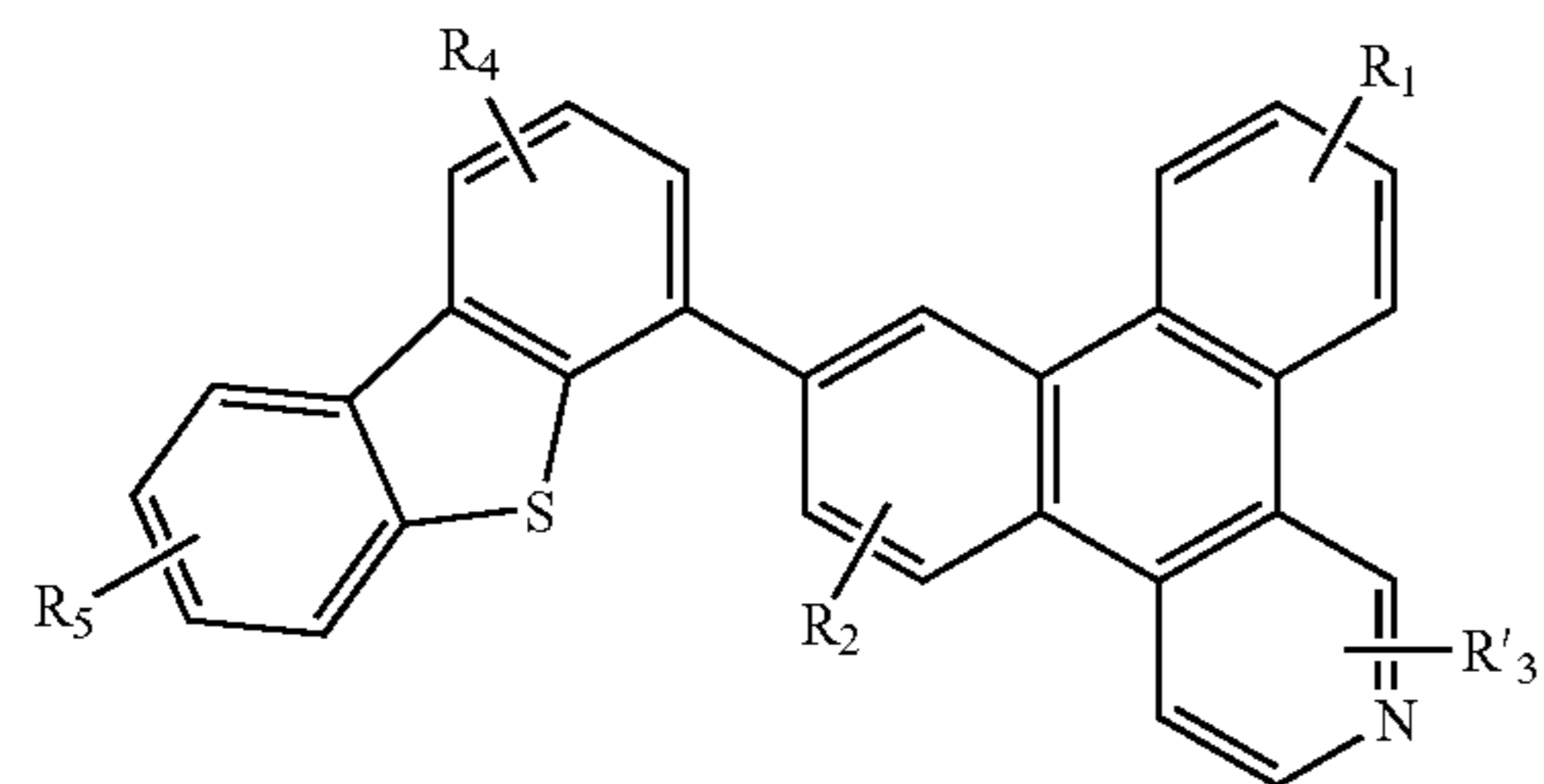
Compound 49G
