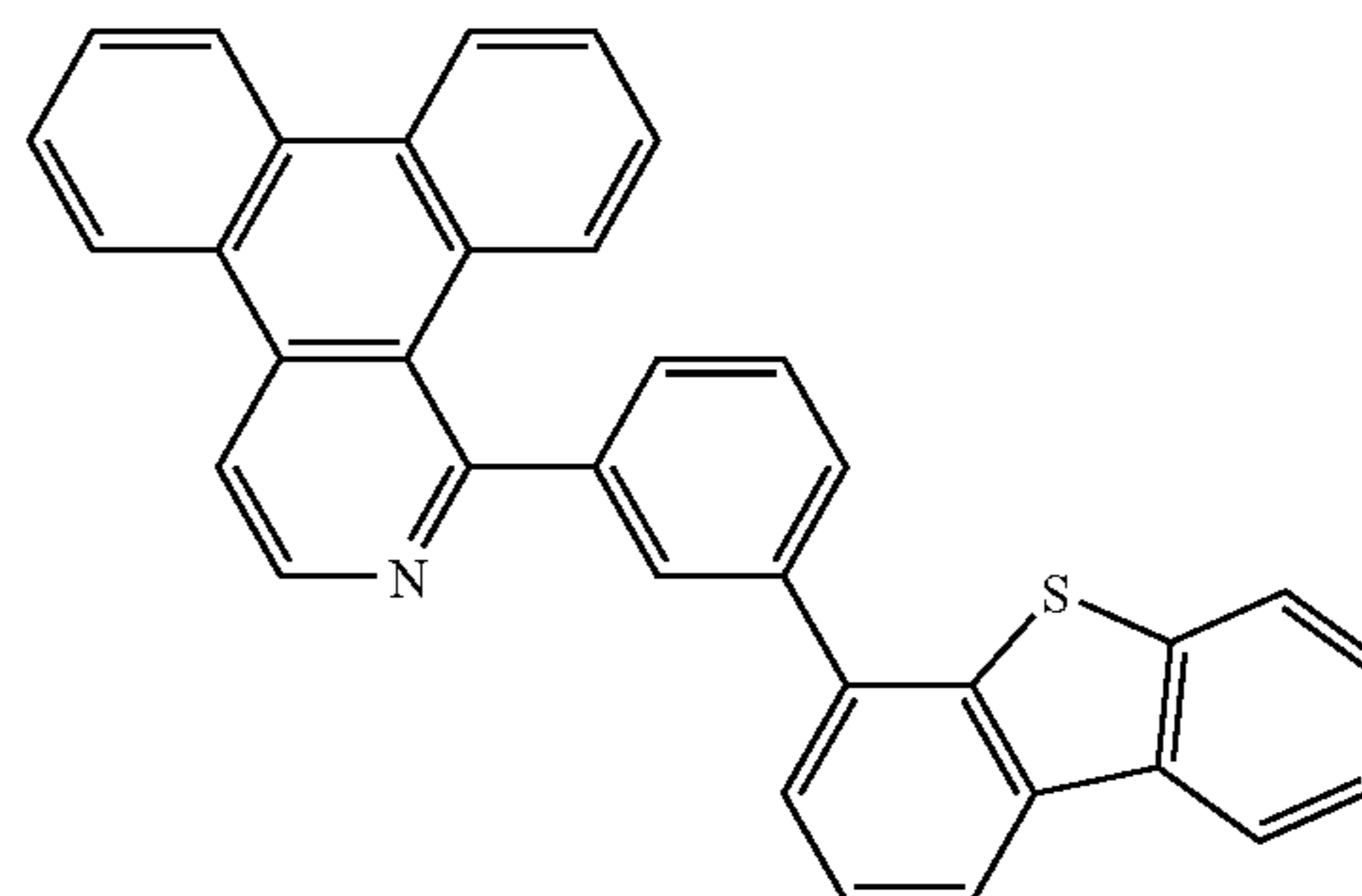
Compound 15
