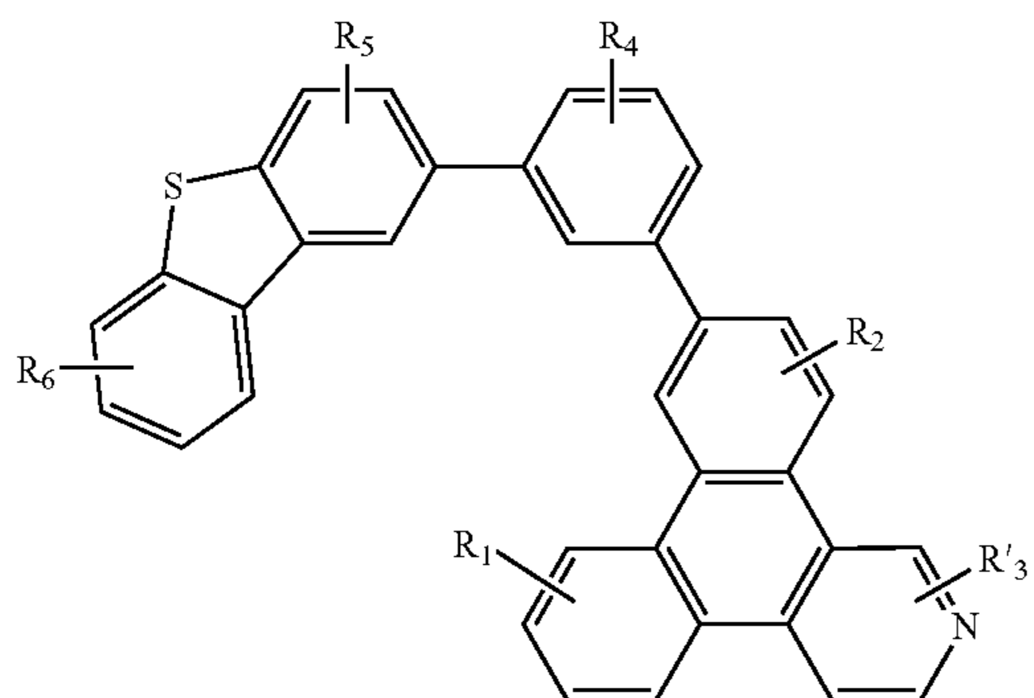
Compound 25G
