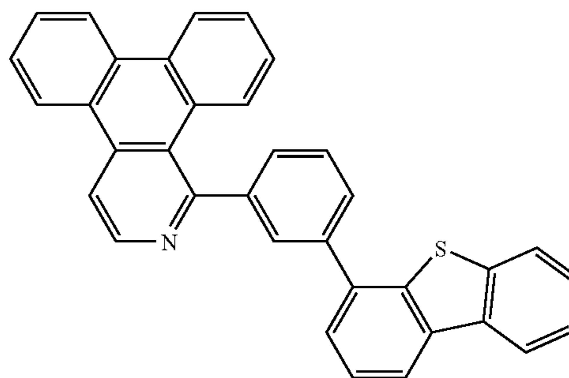
Compound 15
