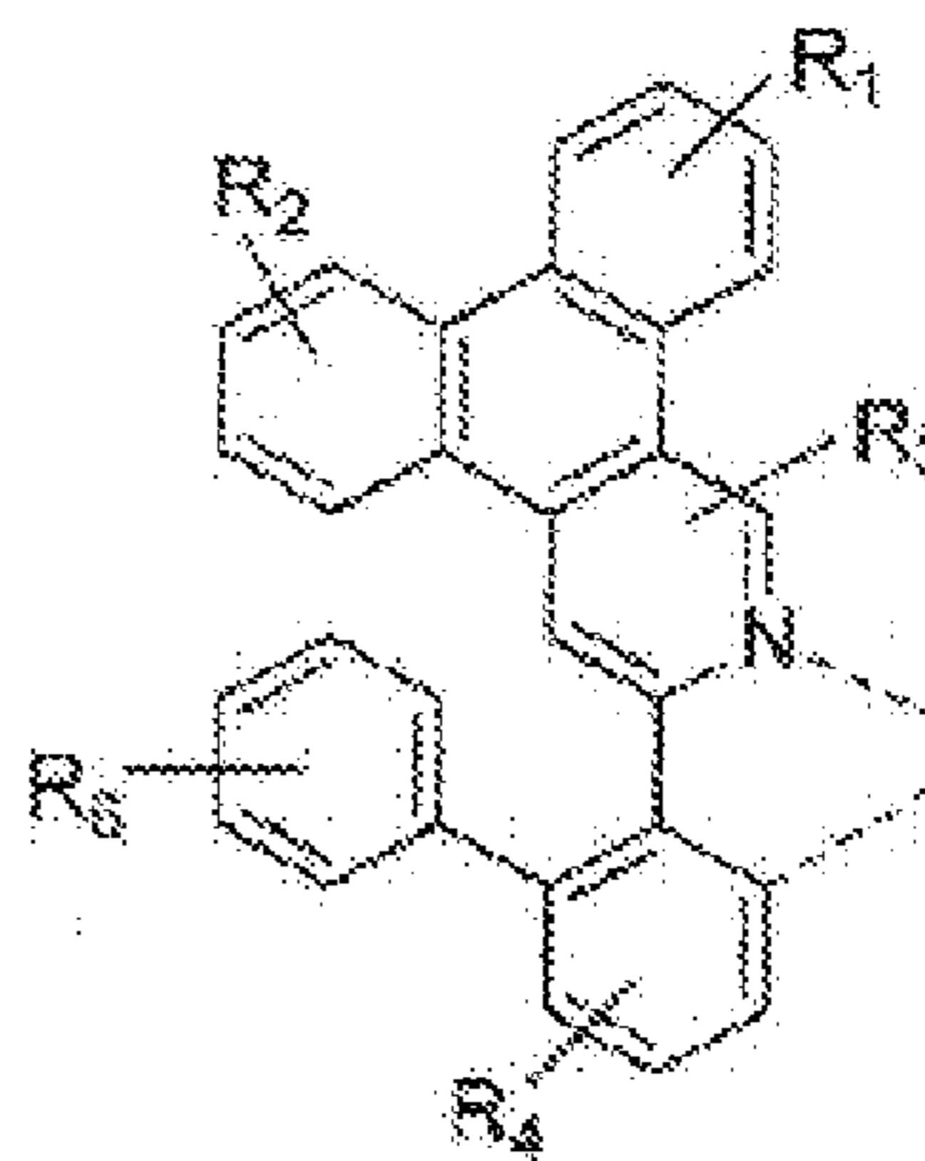
Compound 74G
