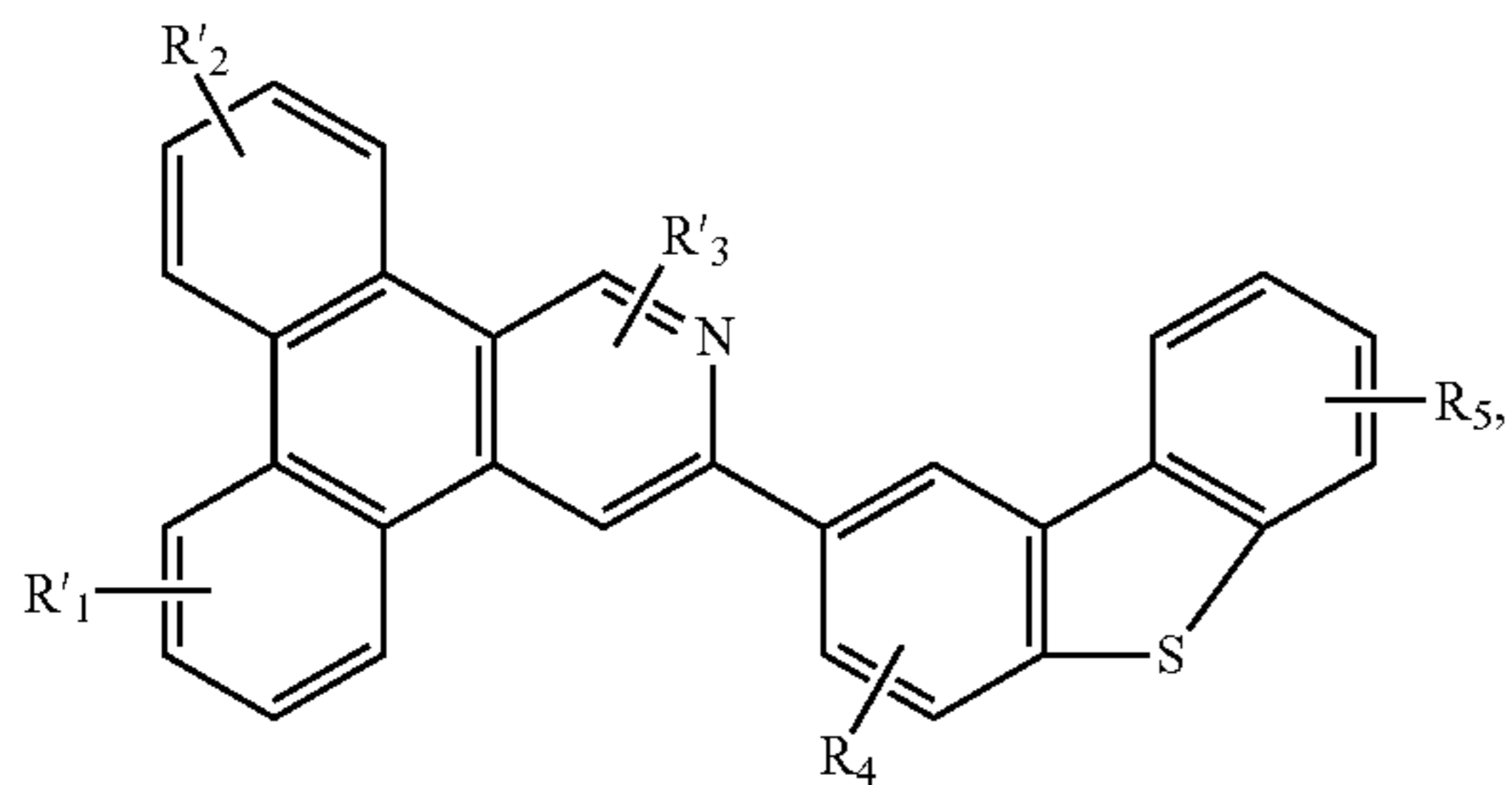
Compound 14G
