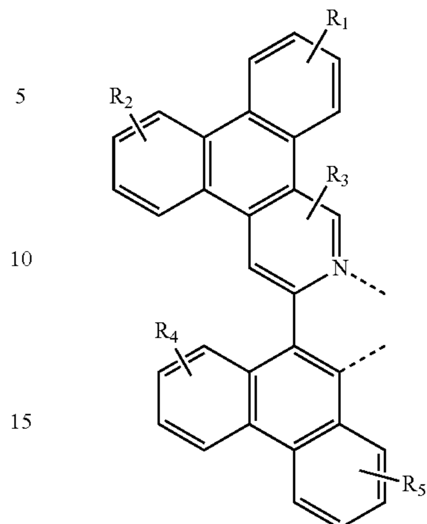
FORMULA II
