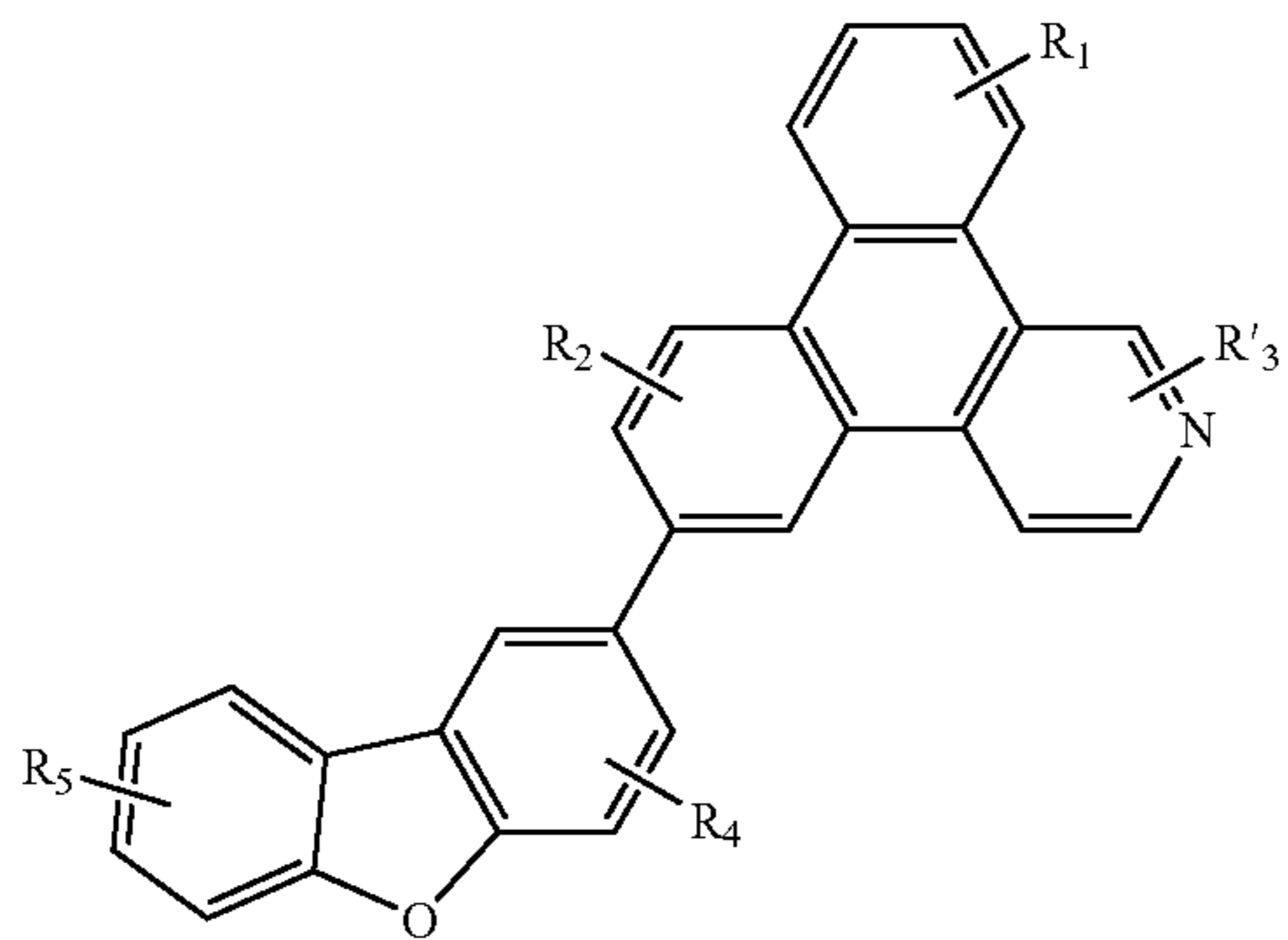
Compound 42G
