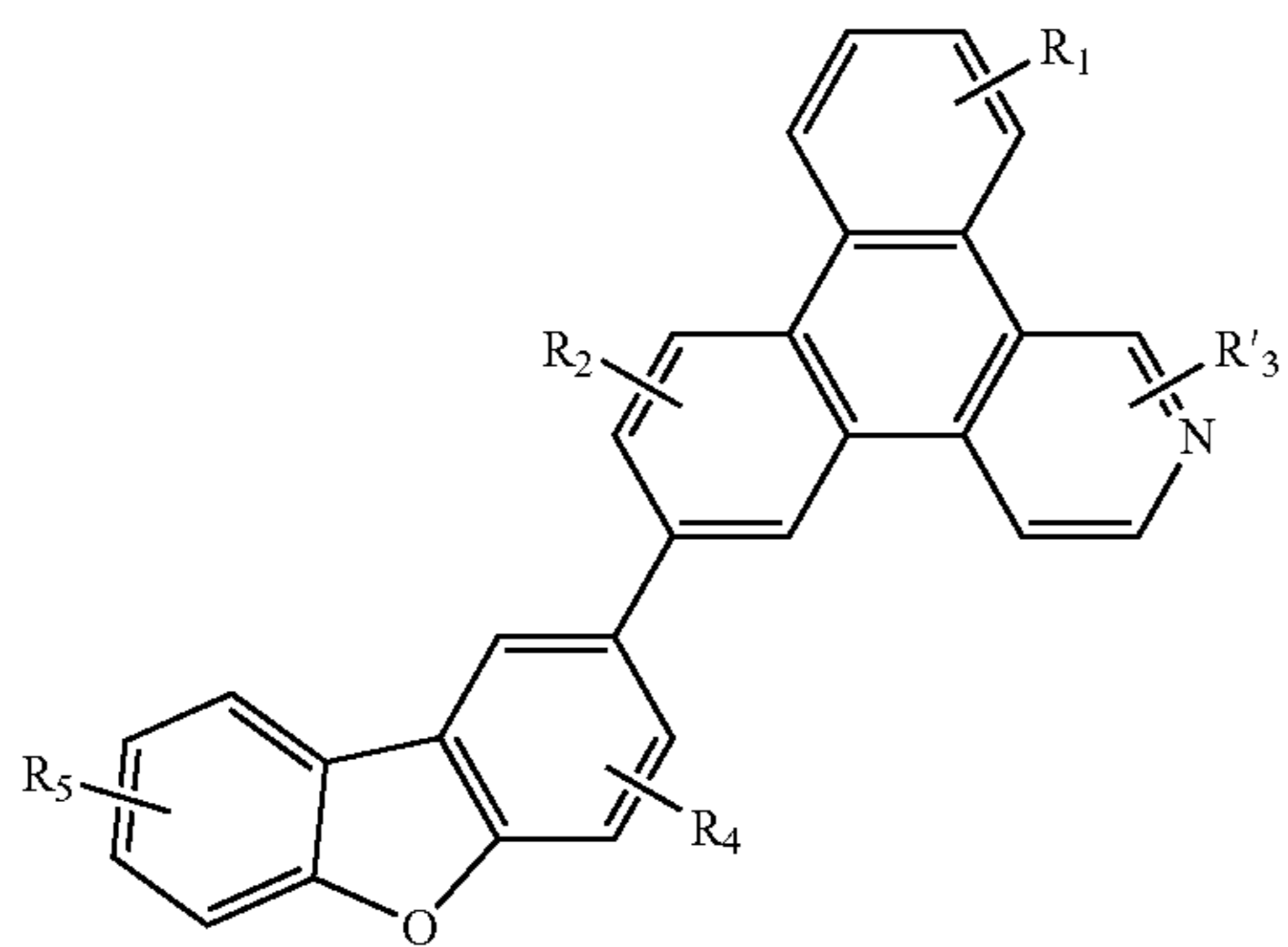
Compound 42G
