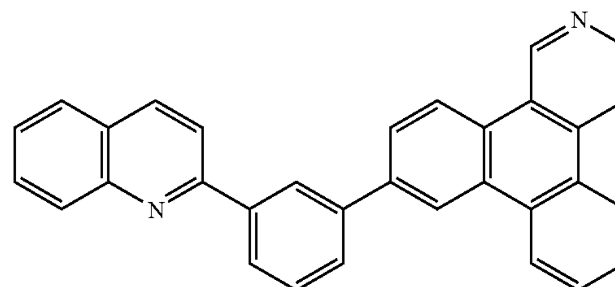
Compound 68
