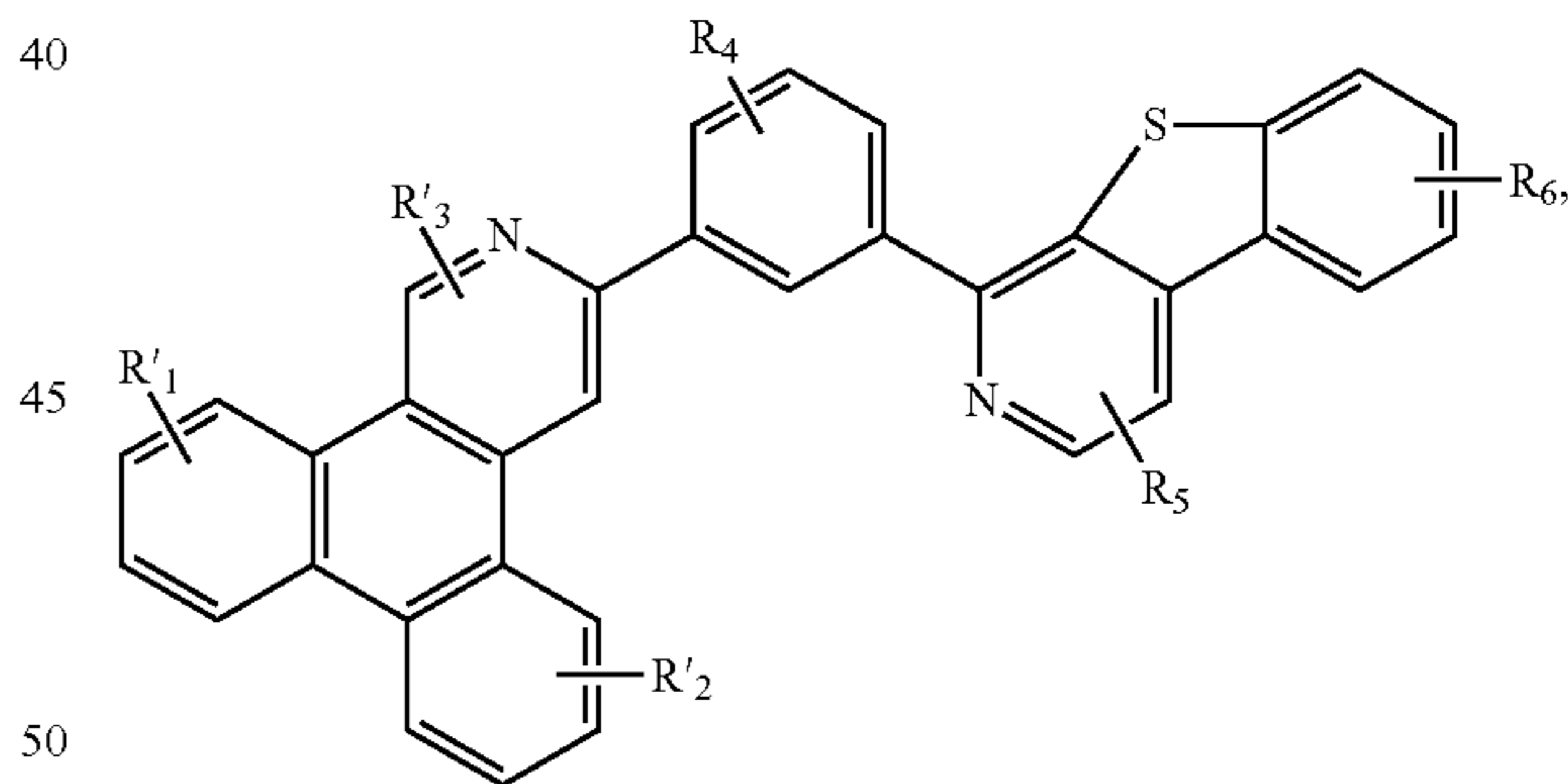
Compound 12G
