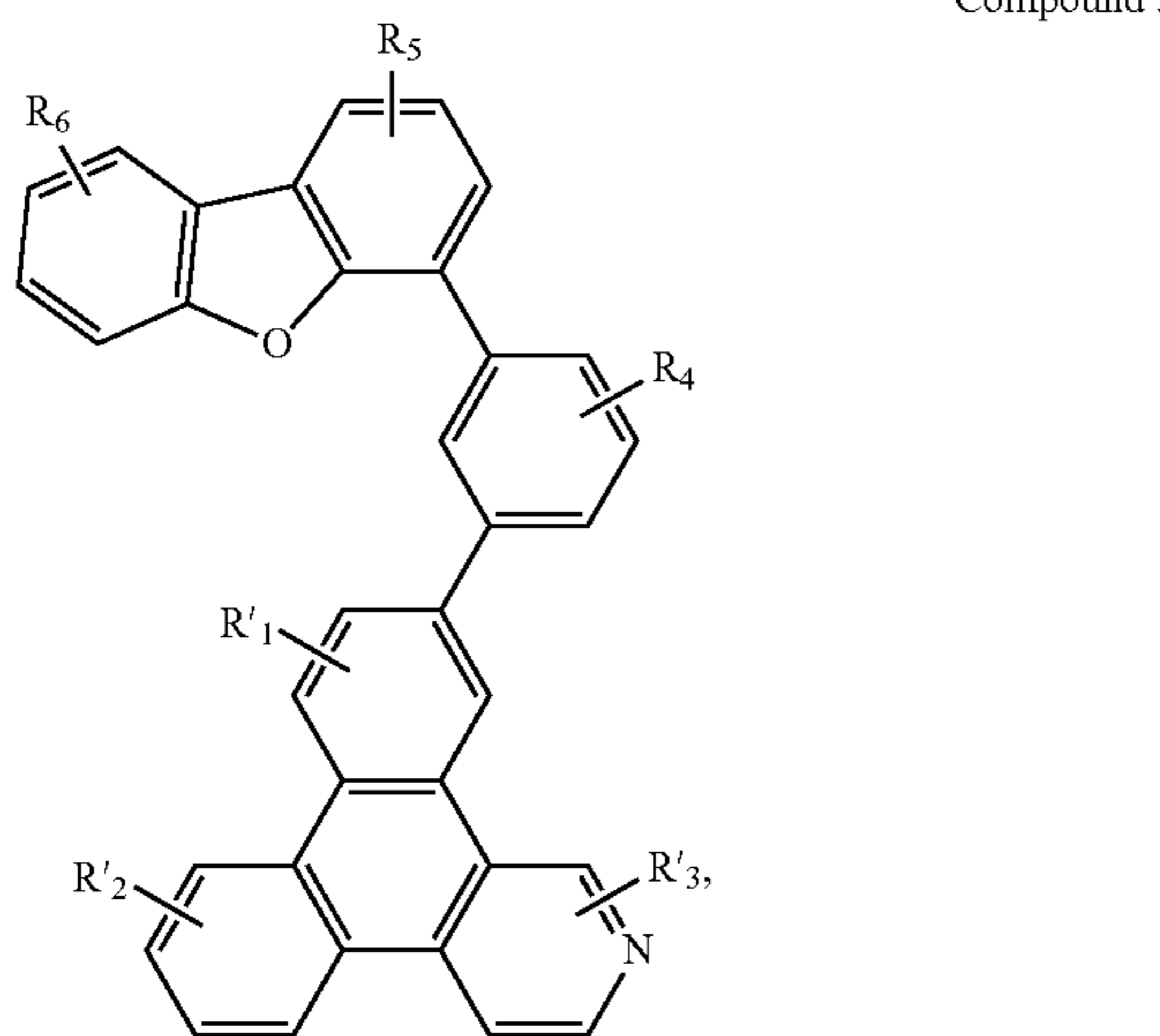
Compound 31G
