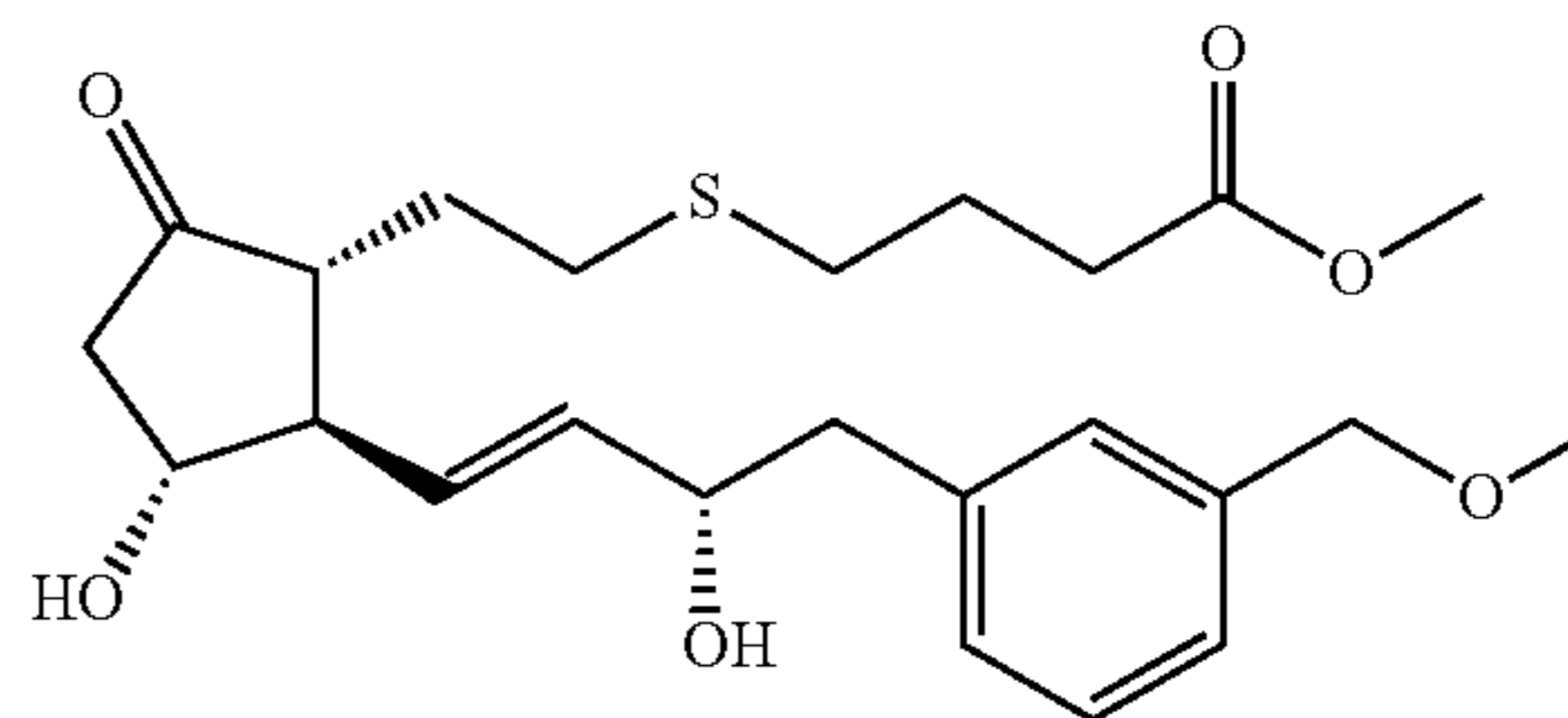
Compound 7
