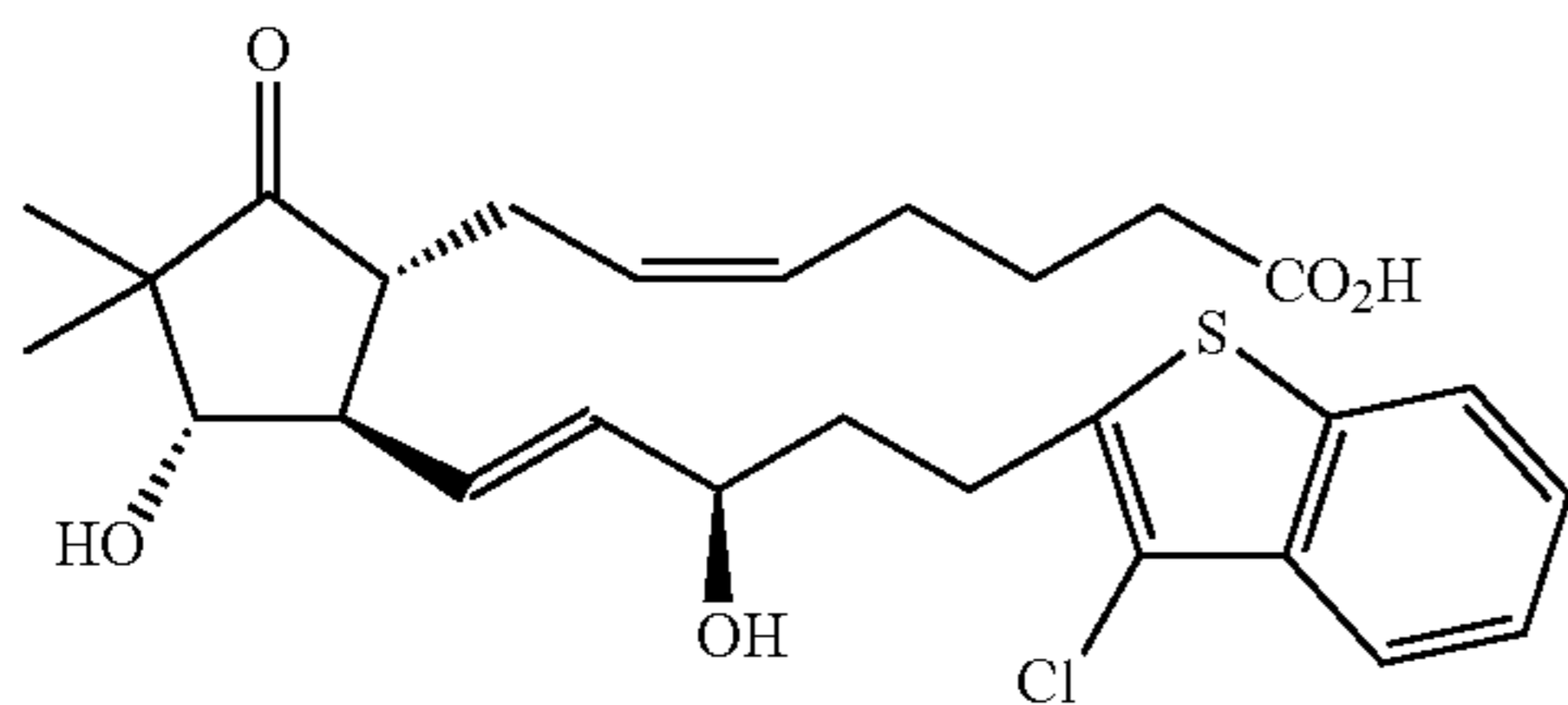
Compound 1
