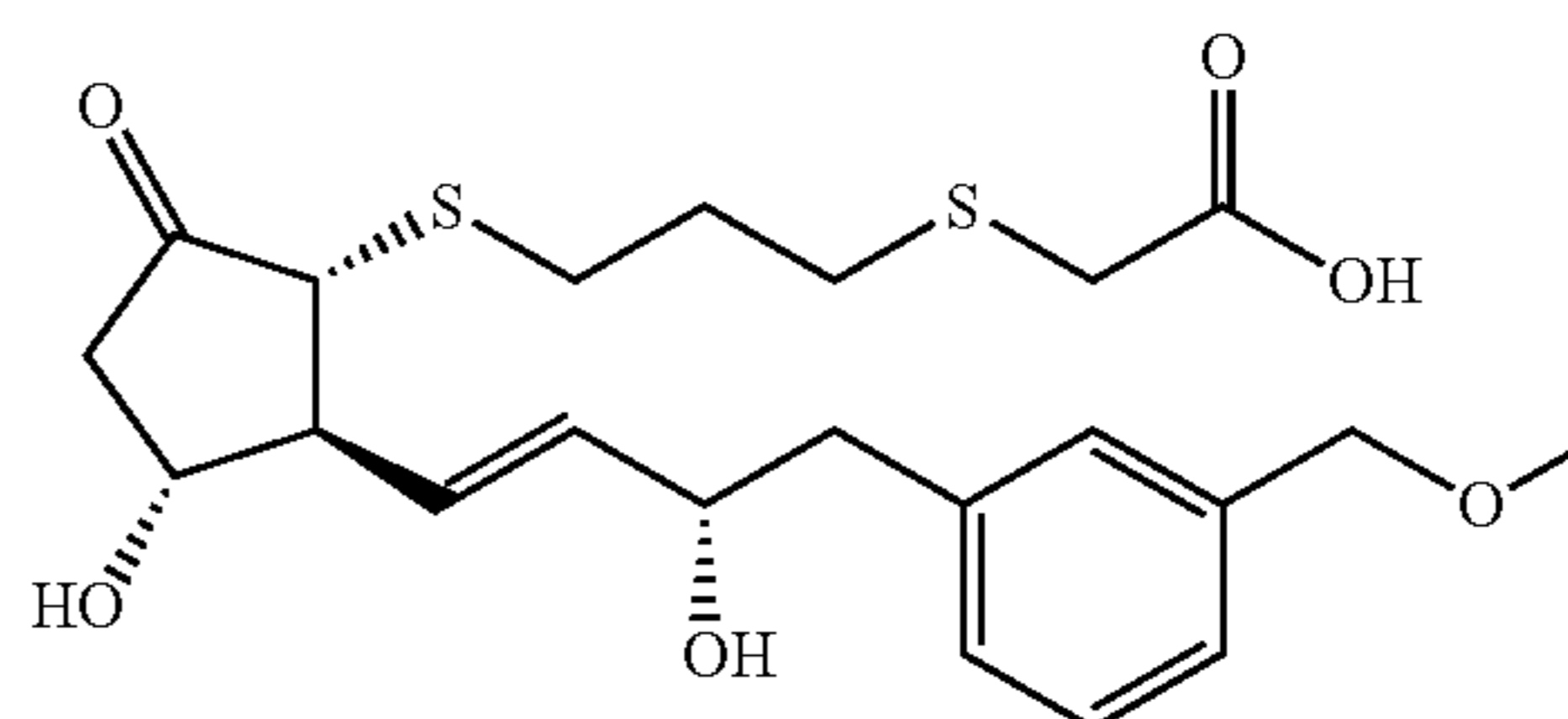
Compound 8
