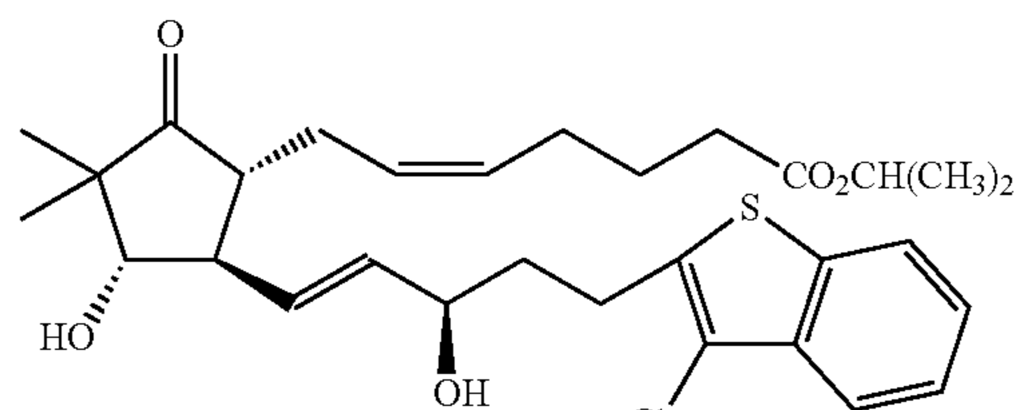
Compound 3
