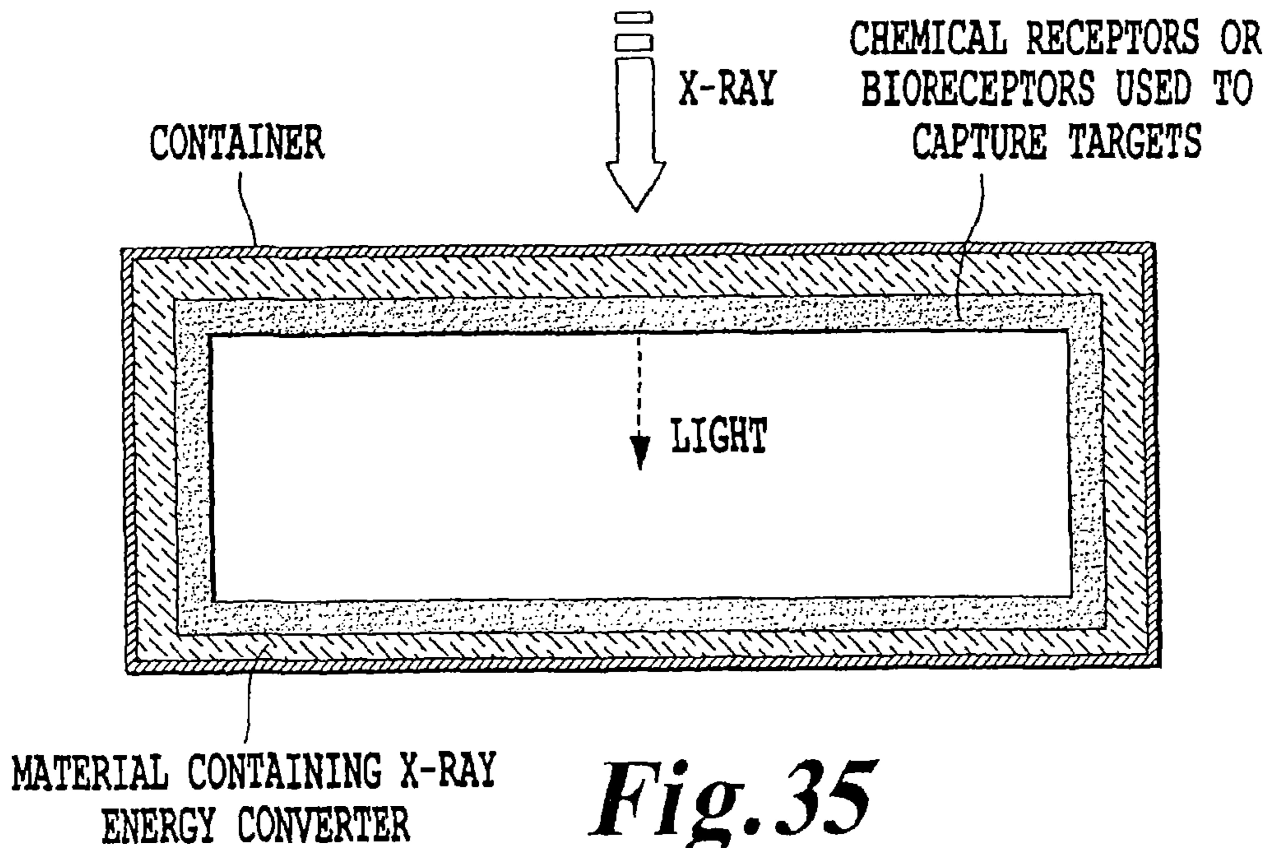
STERILIZATION SYSTEM 9 WITH CHEMICAL RECEPTORS OR BIORECEPTORS
