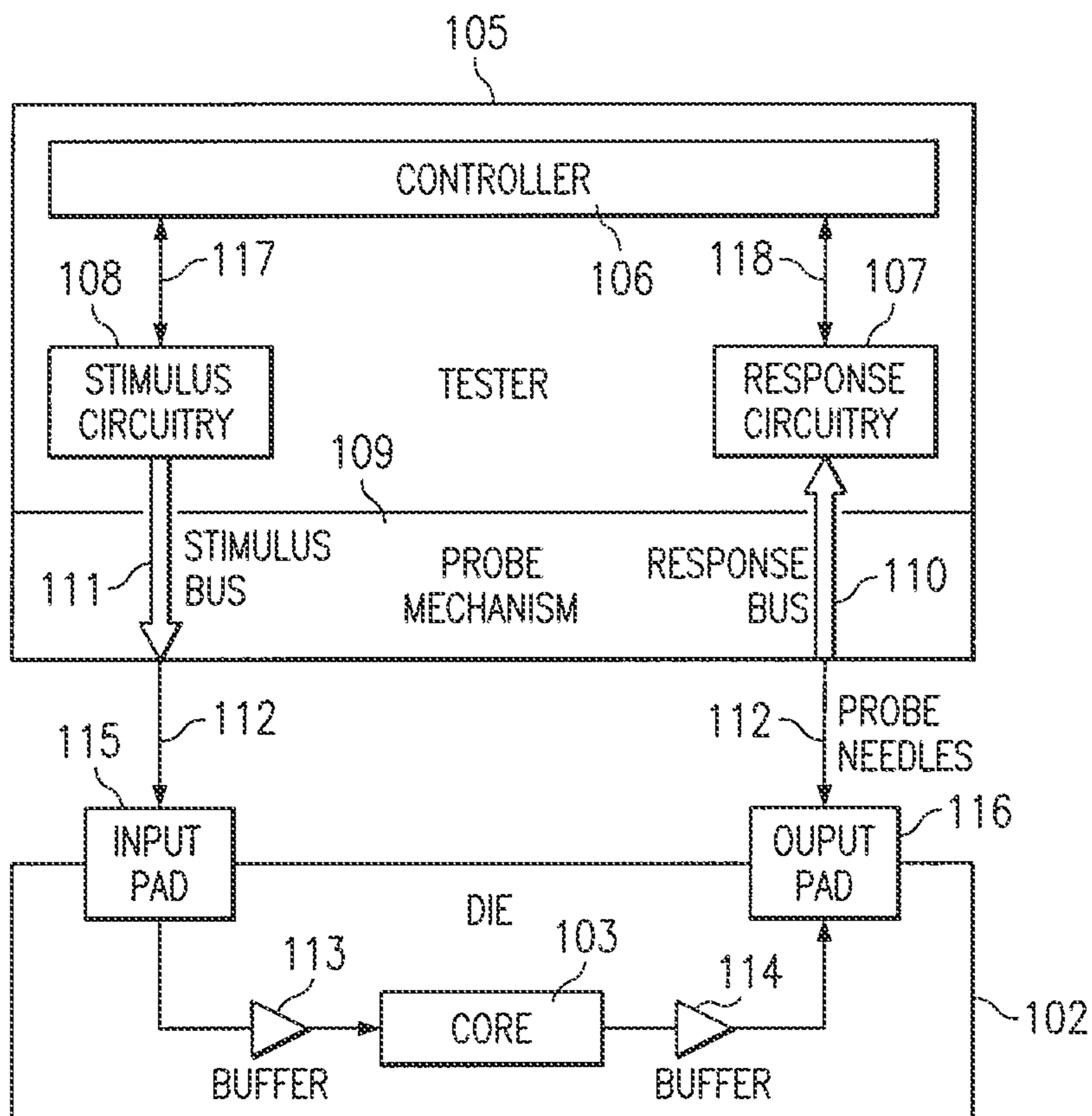
FIG. 1C (PRIOR ART)
