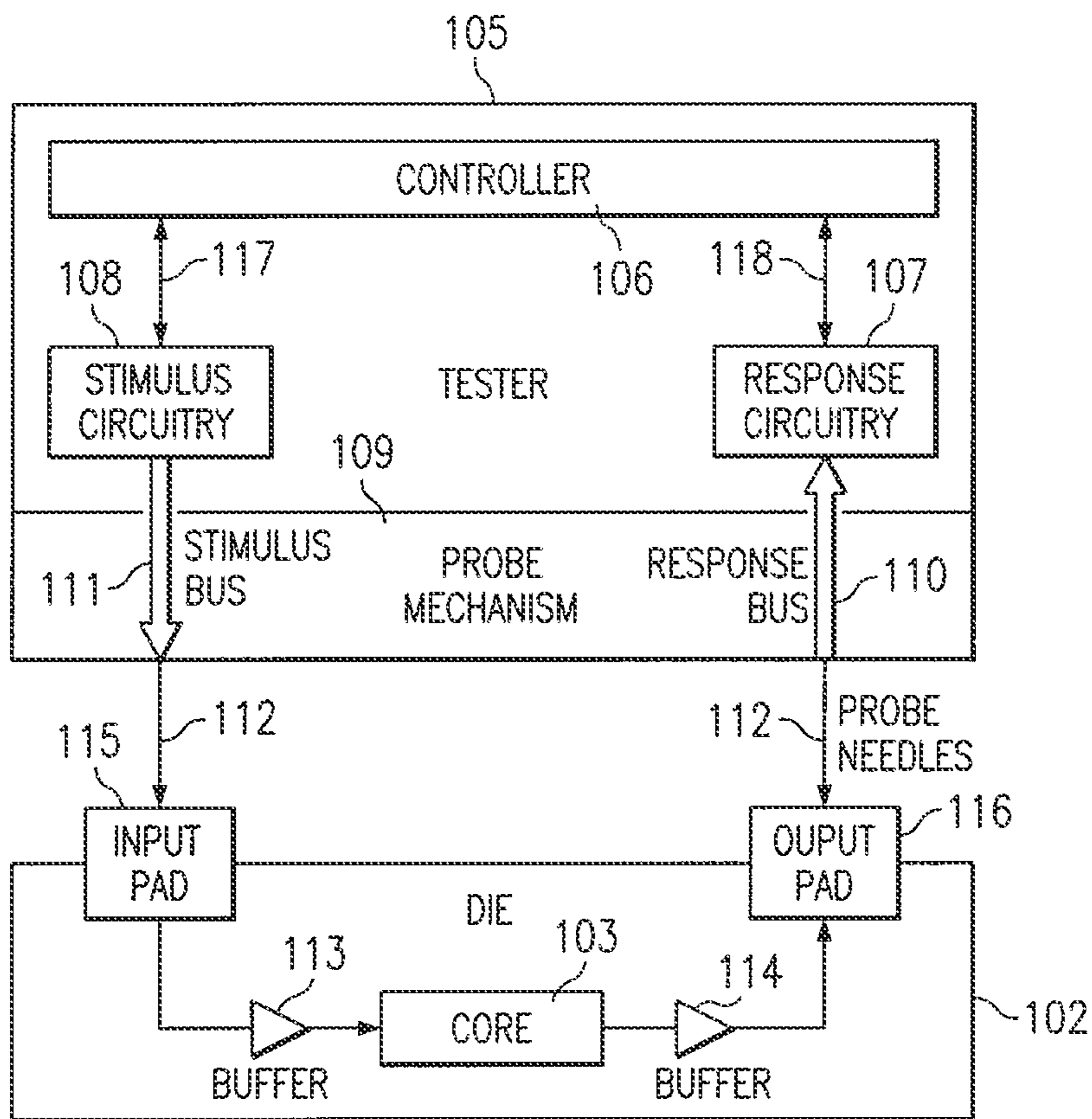
FIG. 1C (PRIOR ART)
