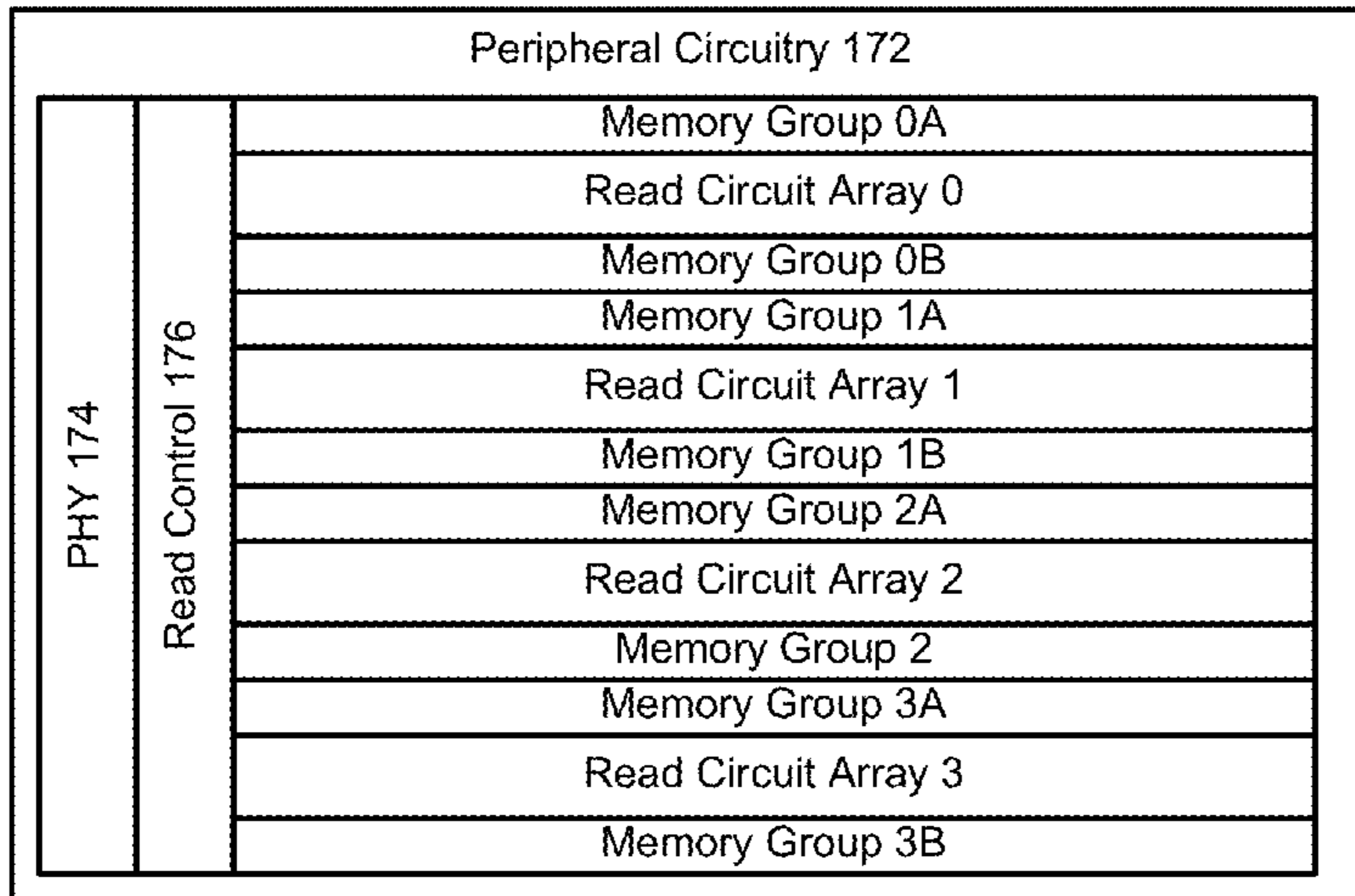
Preprocessor IC 170 (top view)
