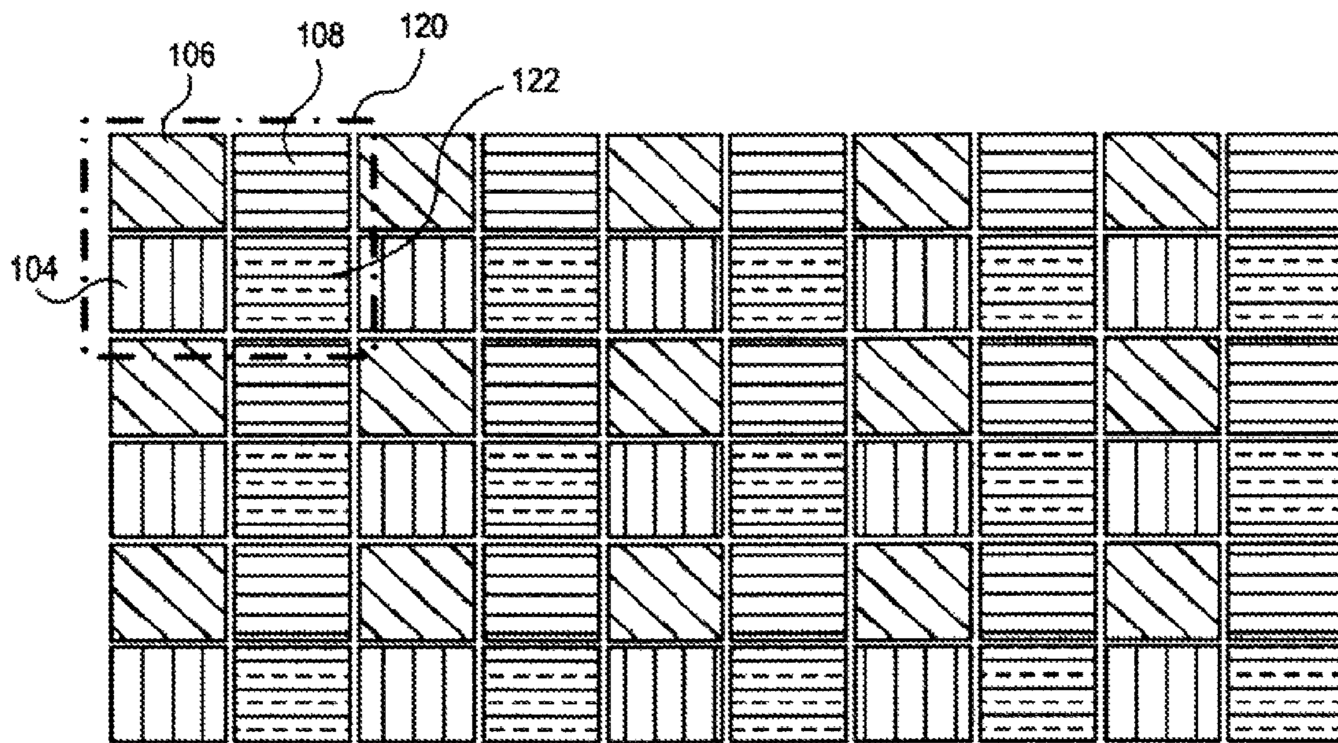
FIG. 9 (PRIOR ART)
