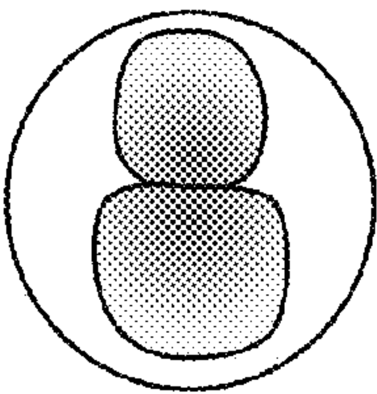
FIG. 74 symbol-radiation pattern #2
