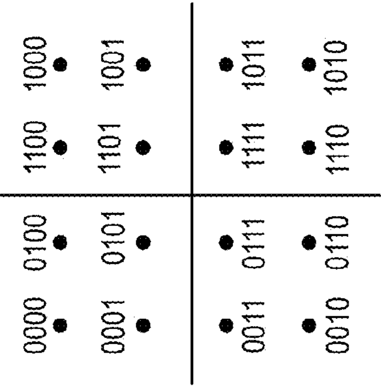
FIG. 101 constellation mapping 276
