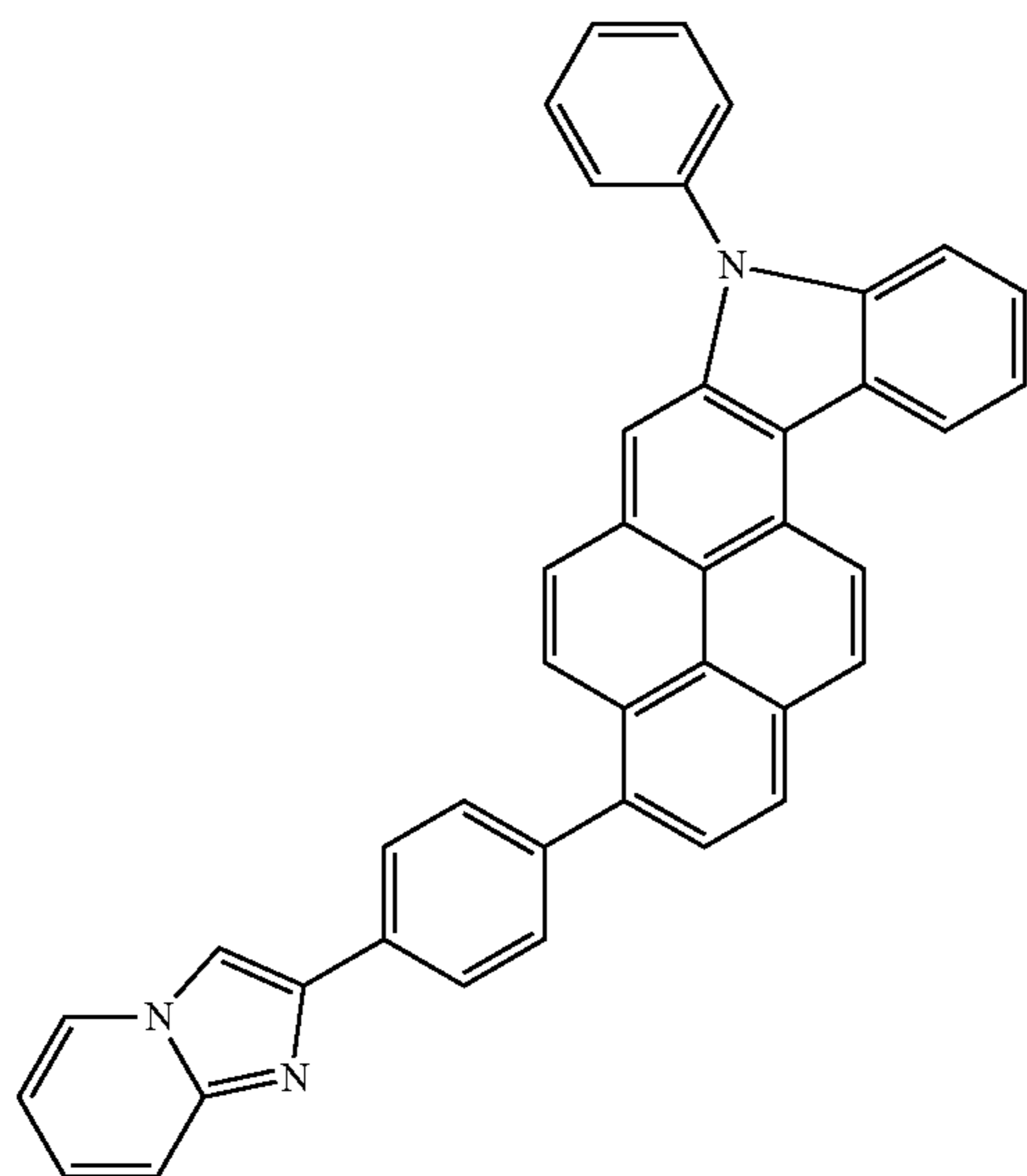
Compound 18
