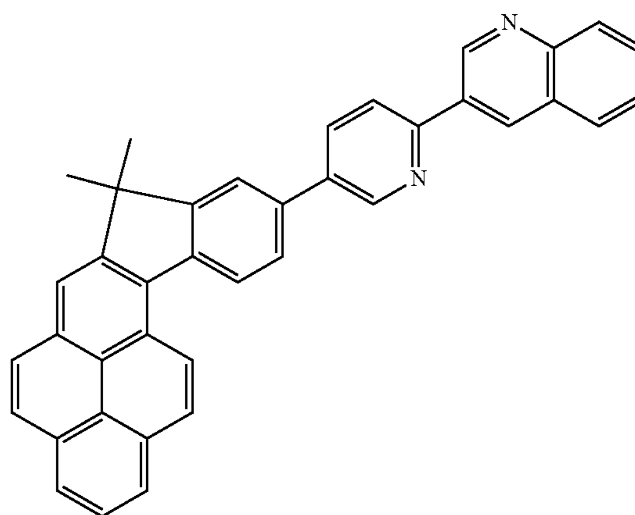
Compound 10
