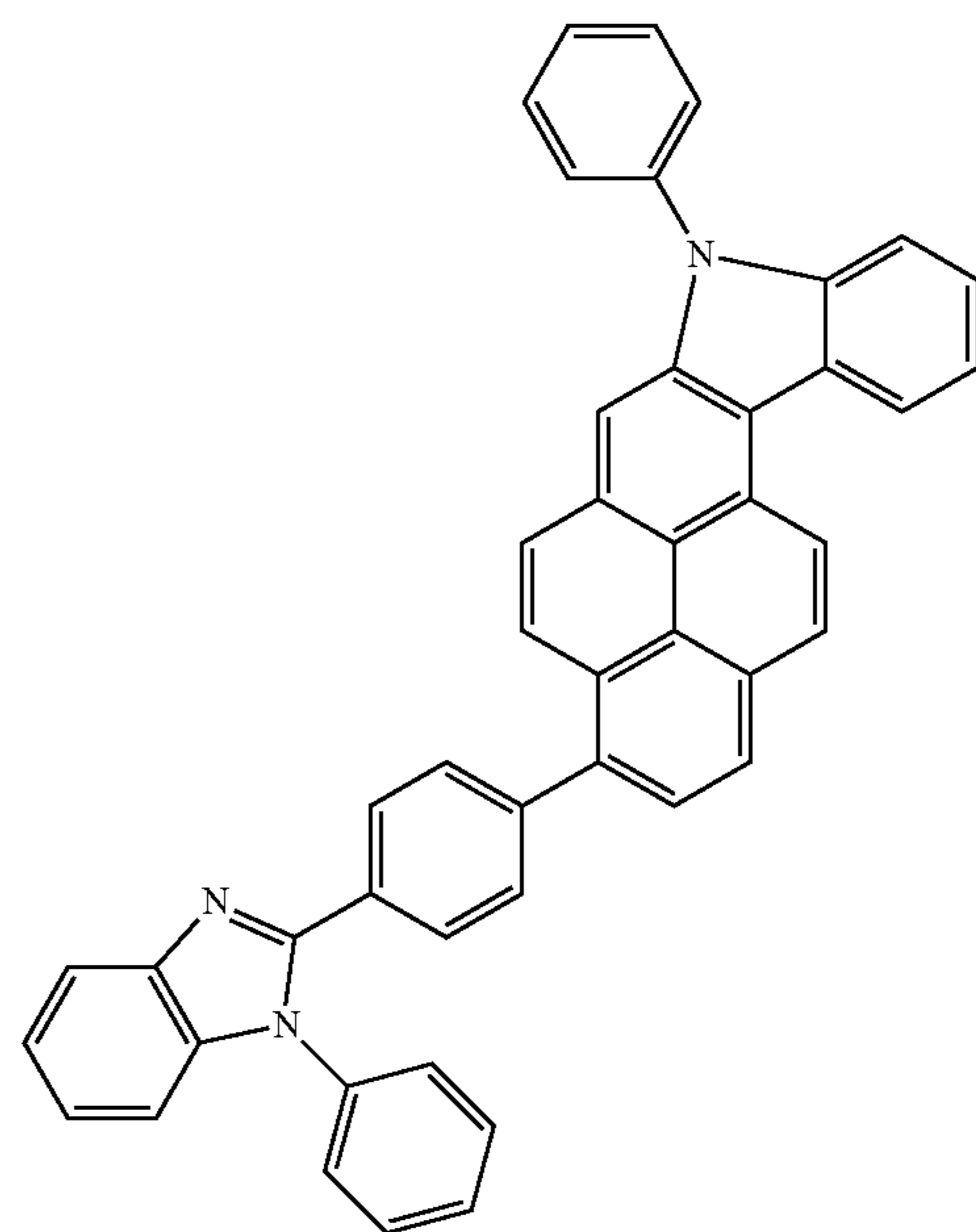
Compound 16
