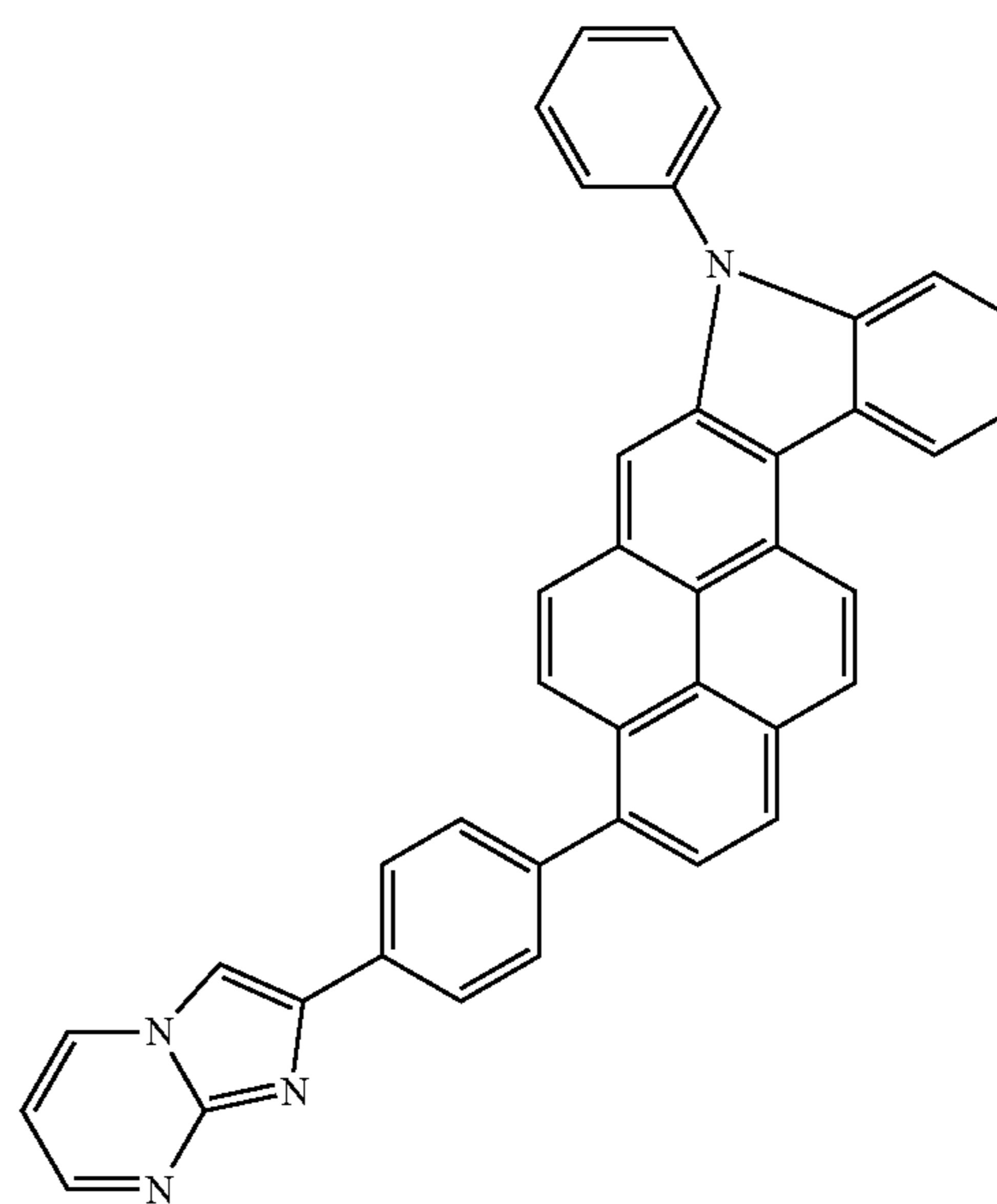
Compound 19
