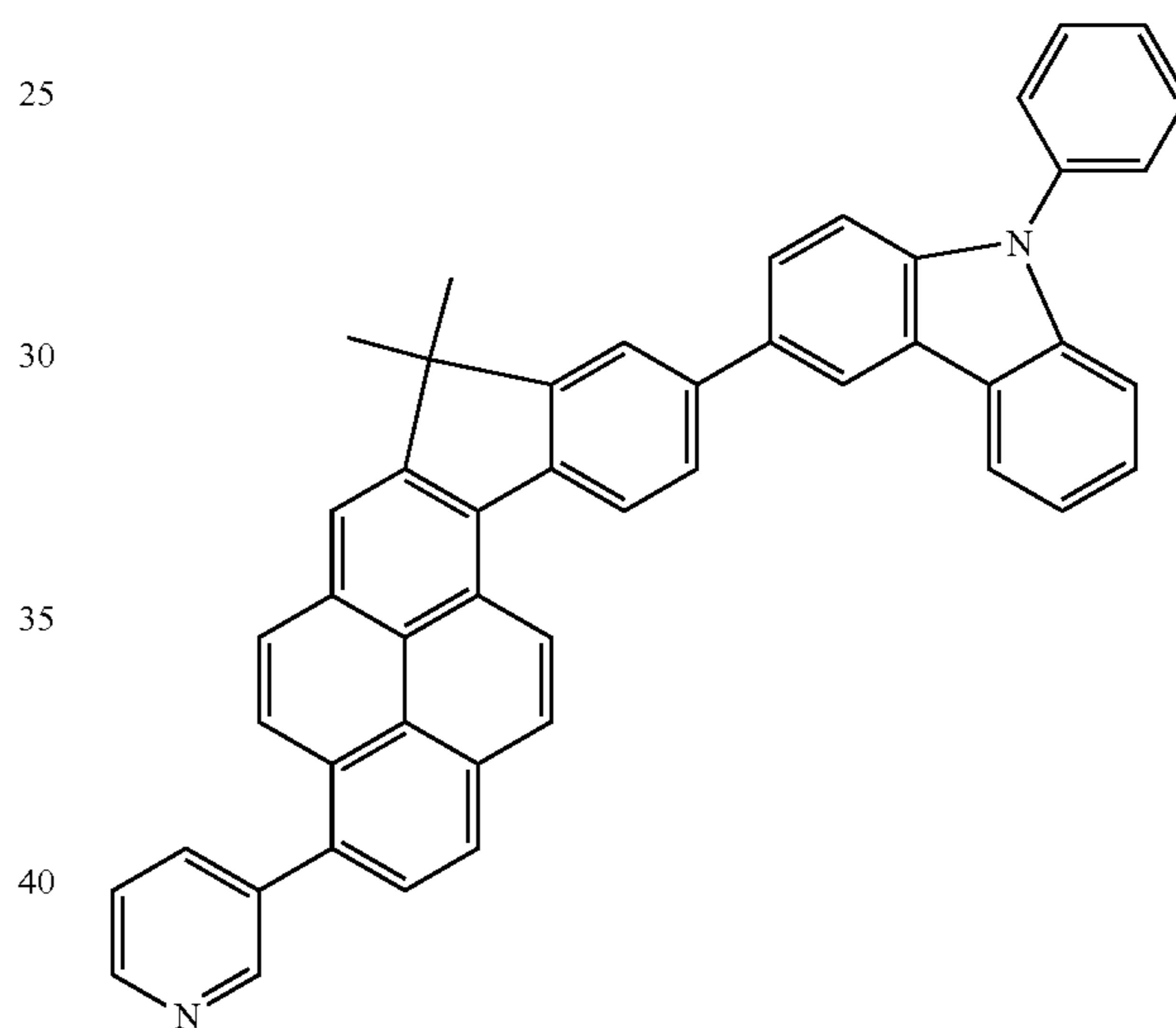
Compound 22
