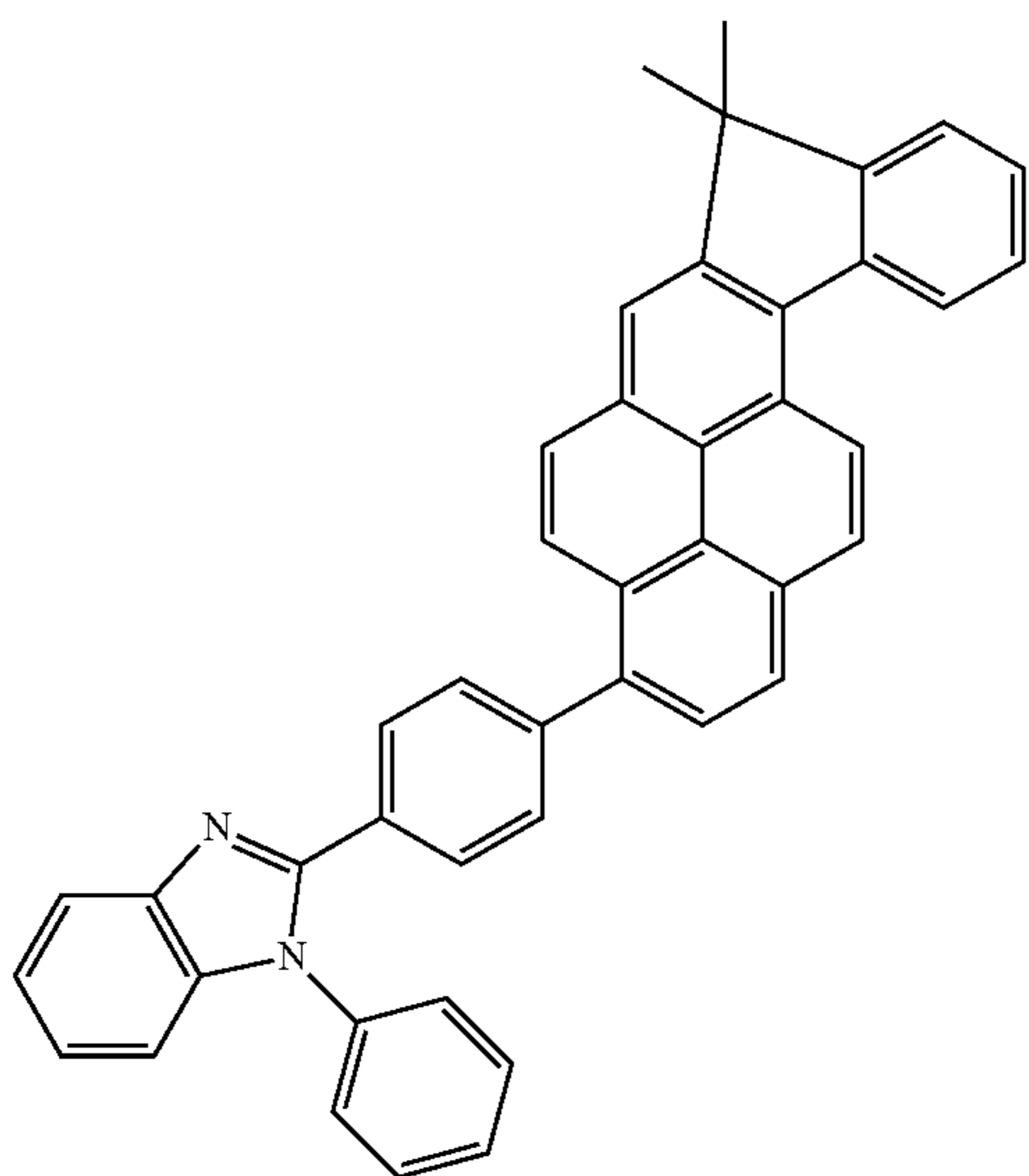
Compound 5
