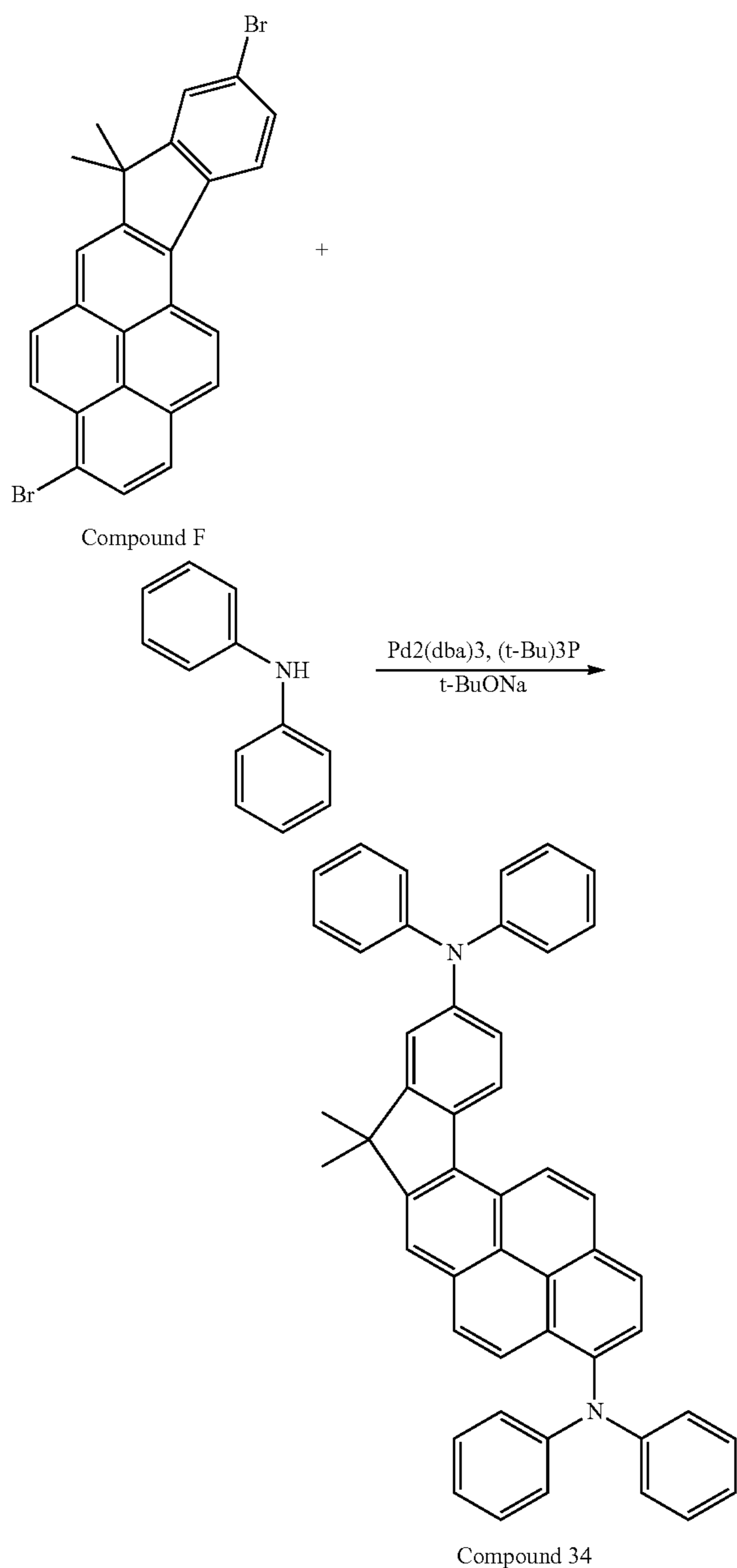
Reaction Scheme 7
