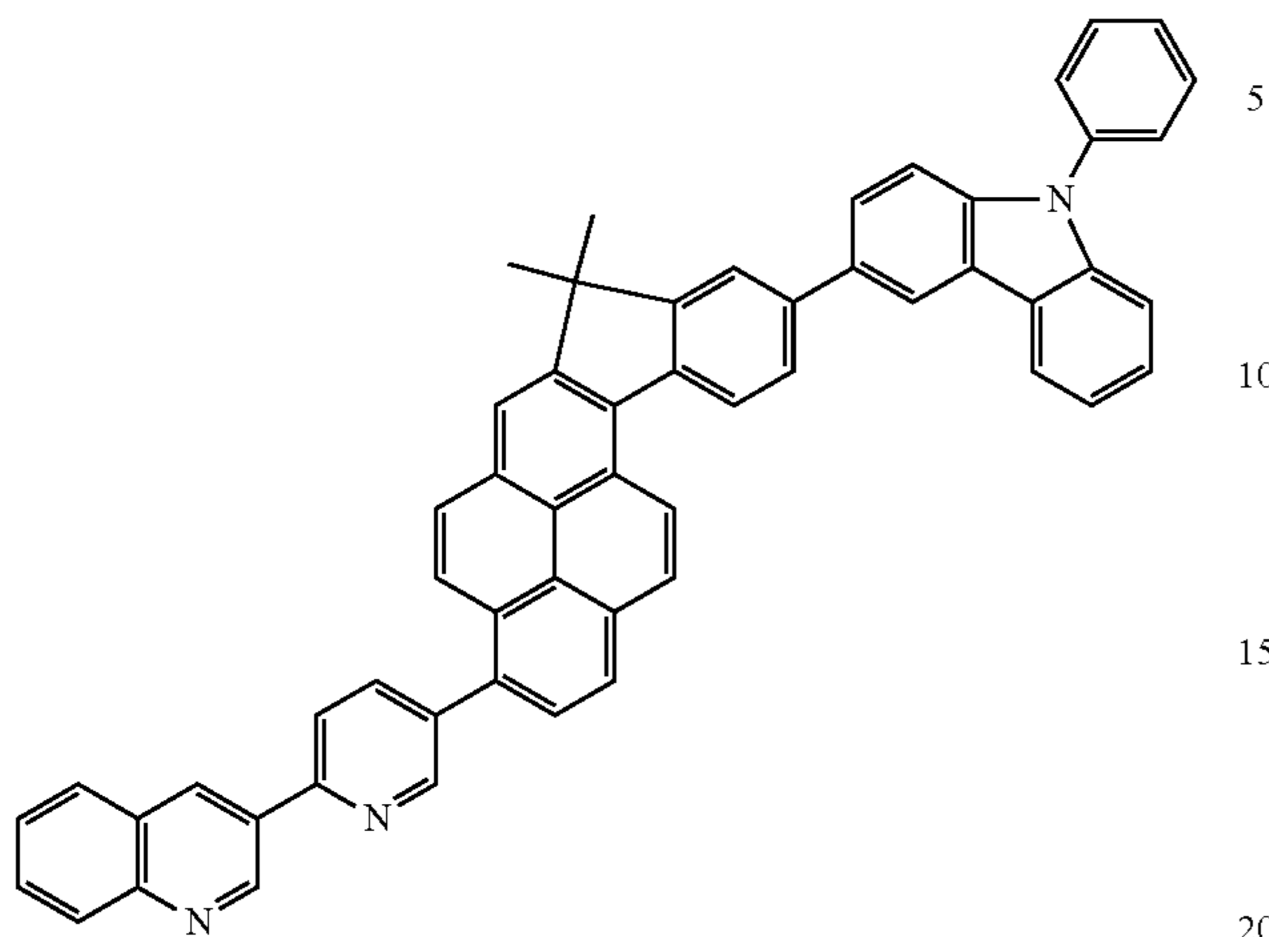
Compound 24
