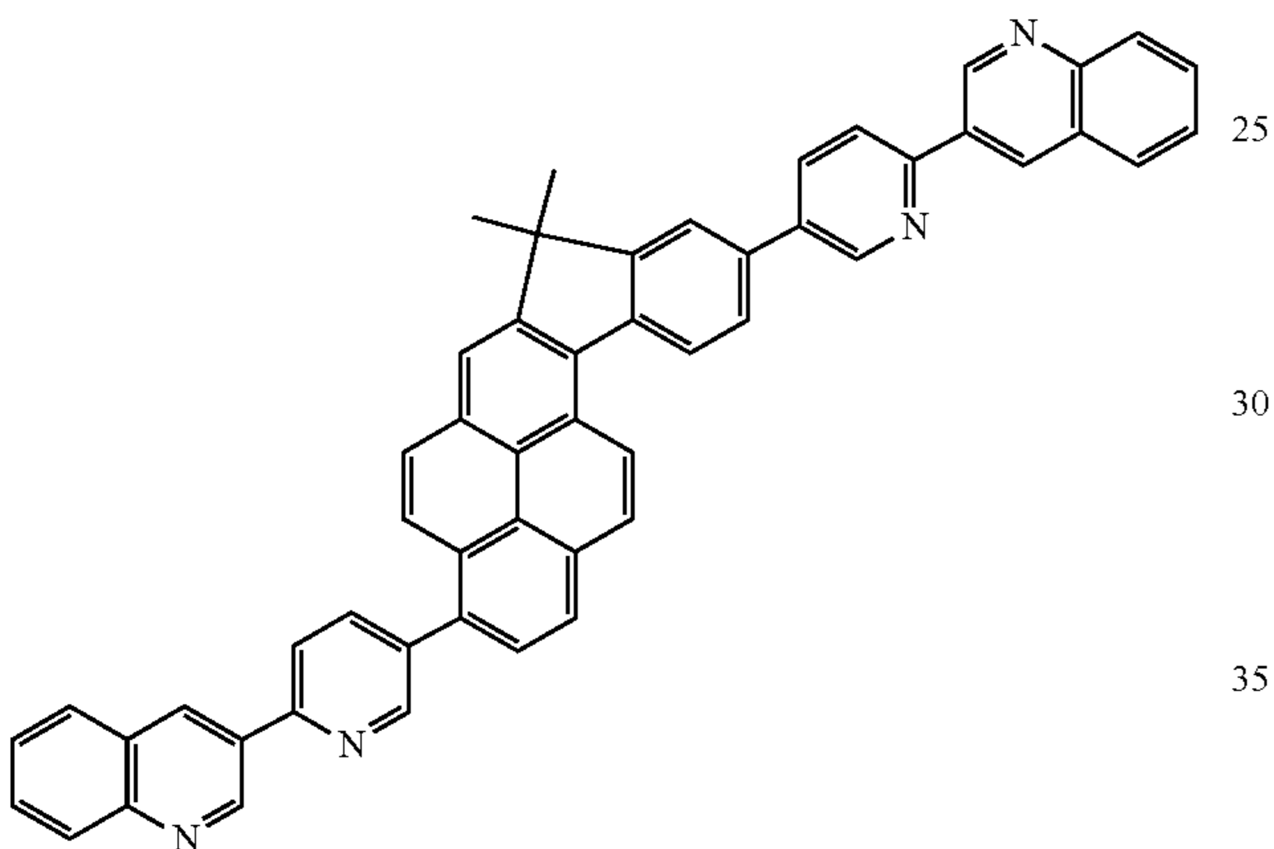
Compound 31
