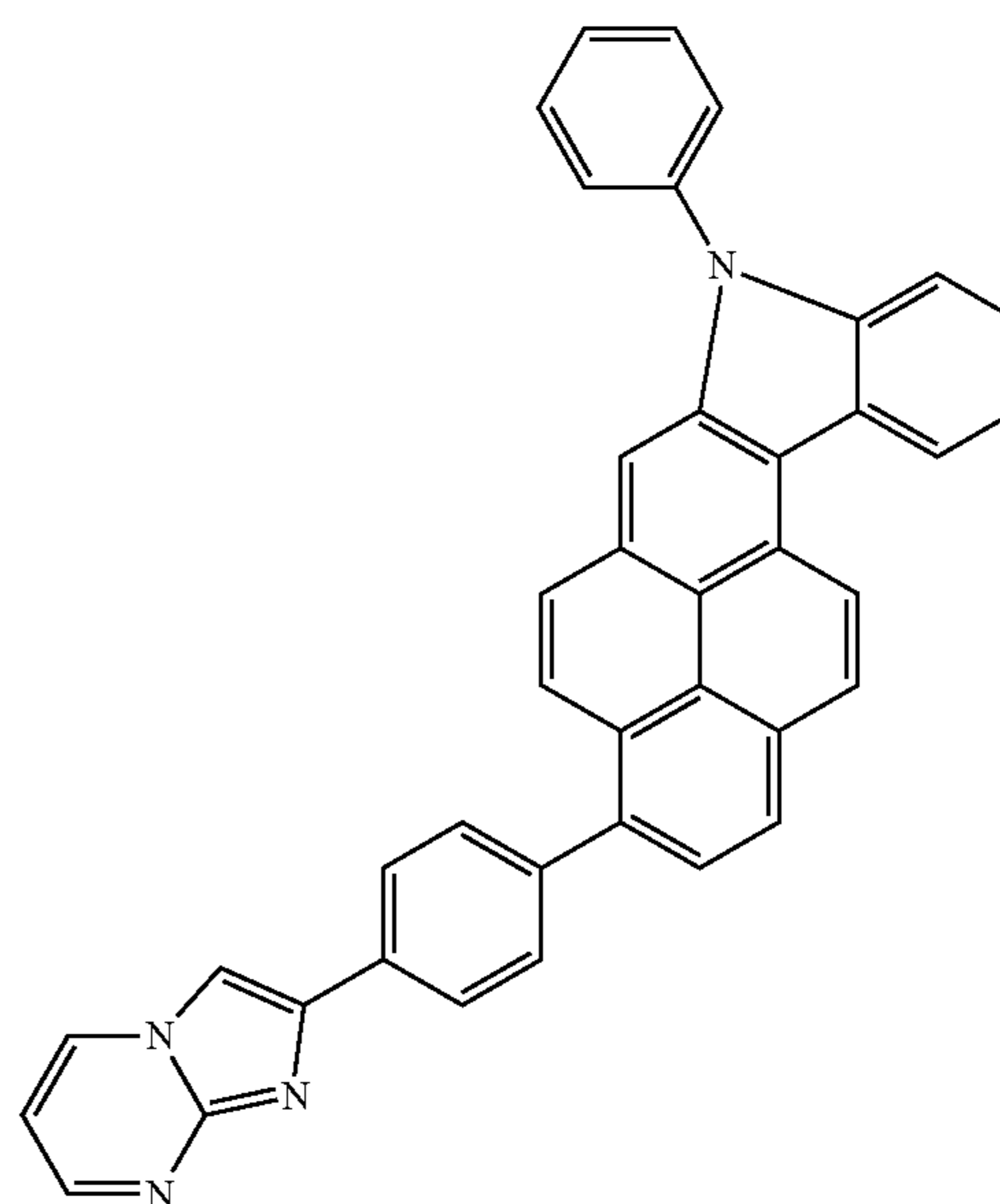
Compound 19
