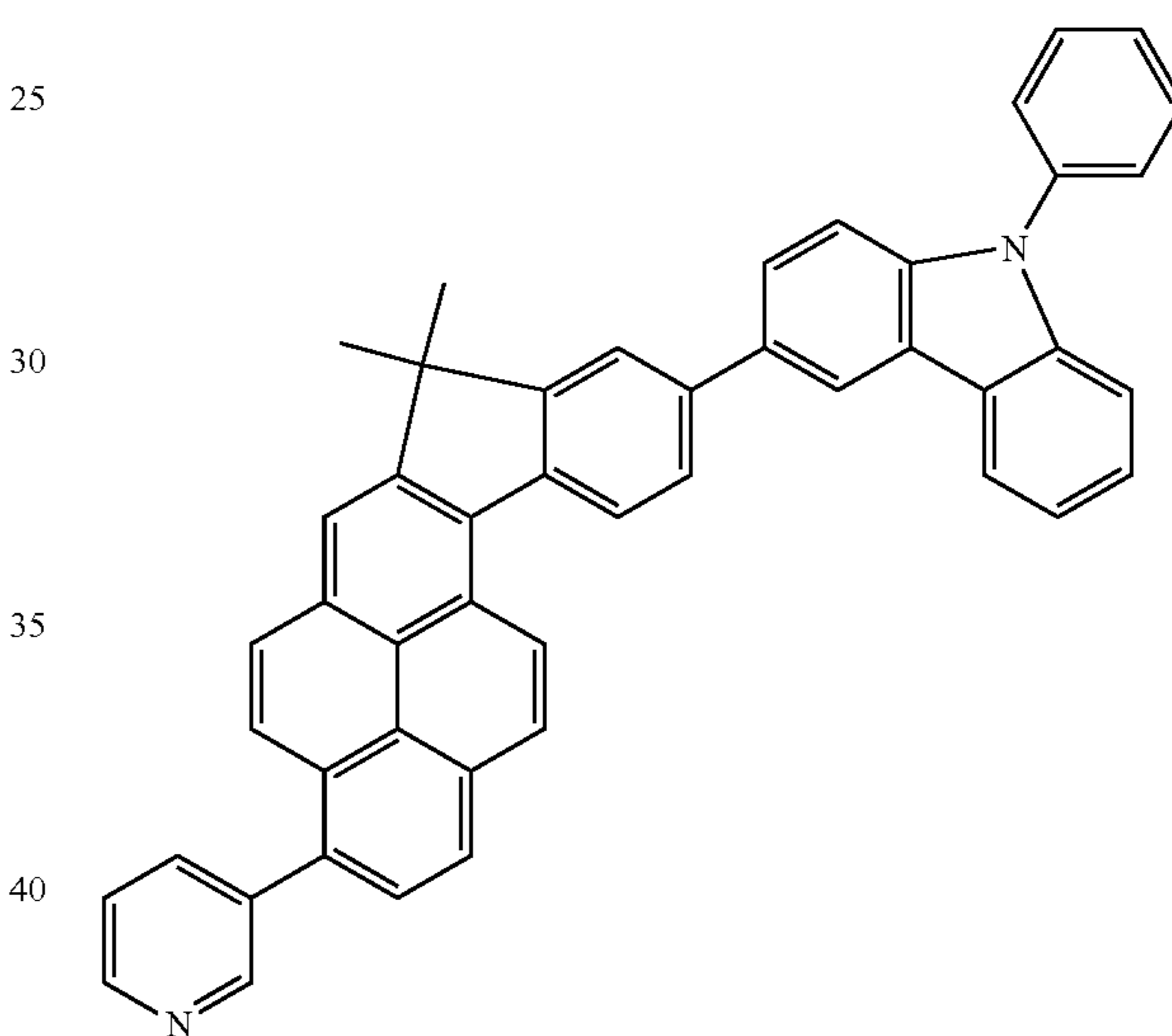
Compound 22
