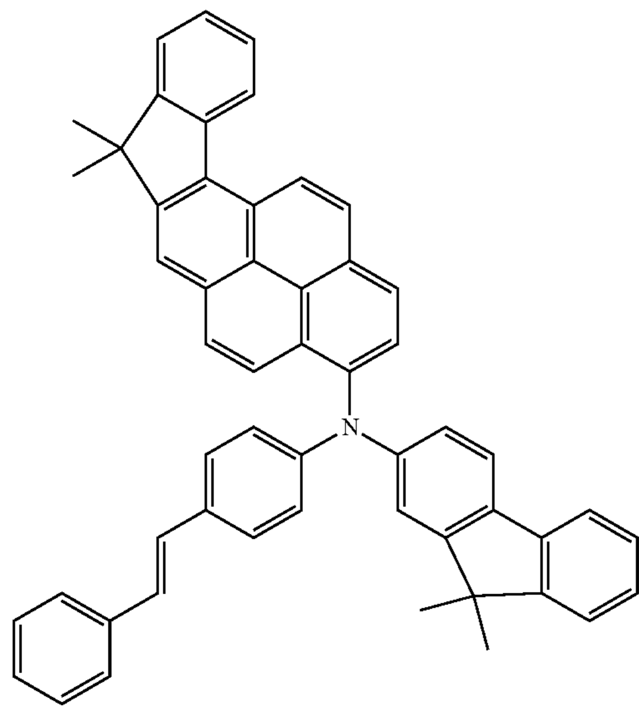
Compound 40
