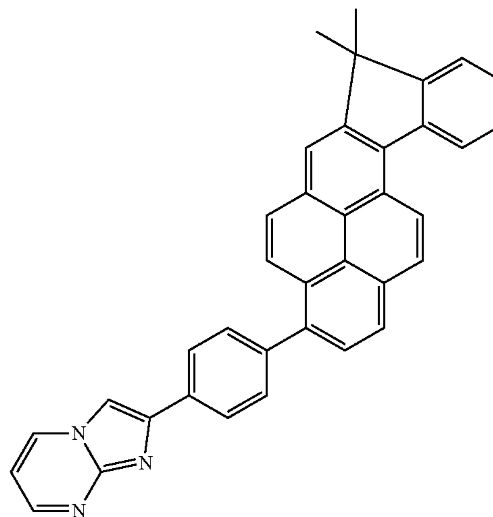
Compound 13
