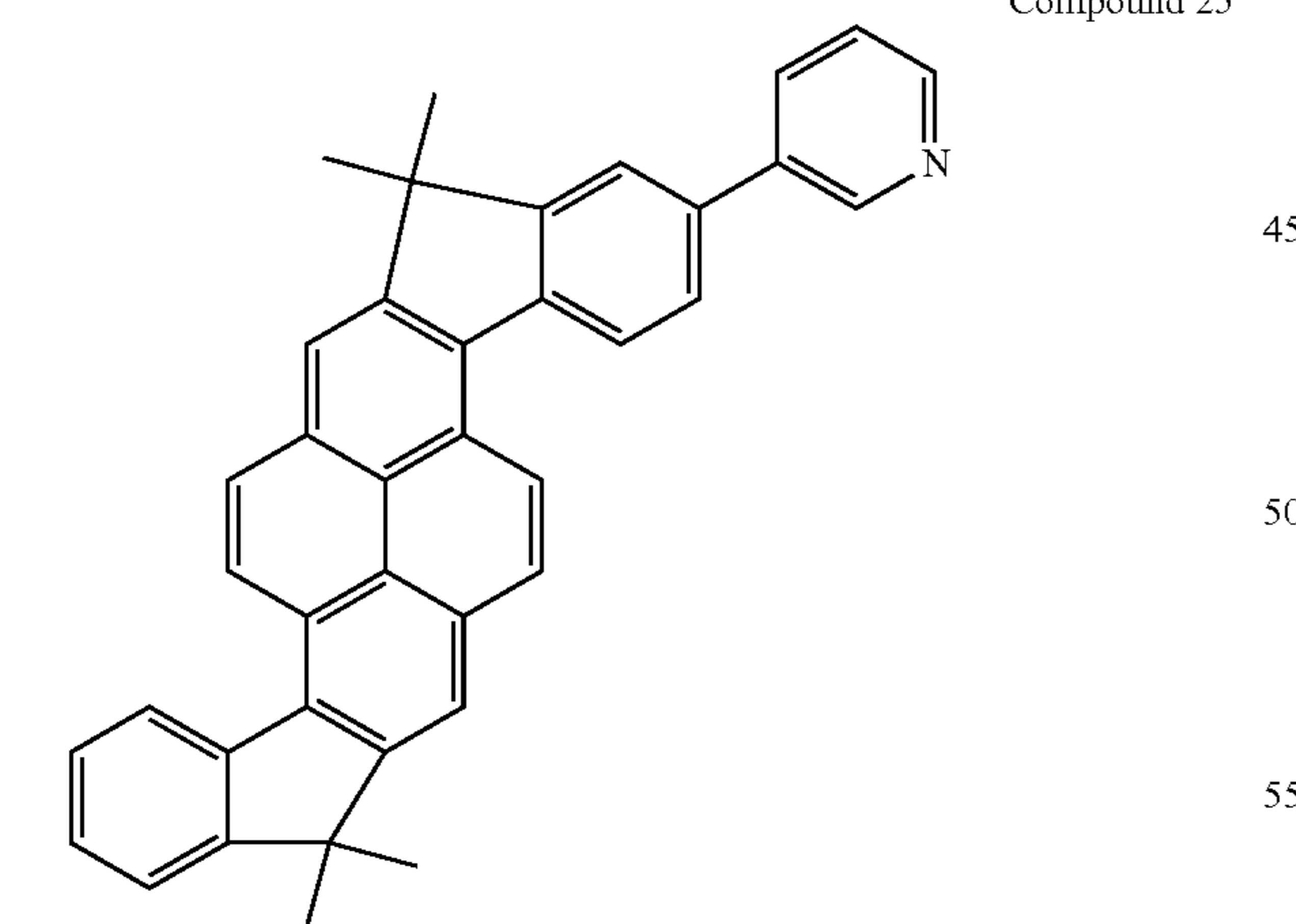
Compound 25
