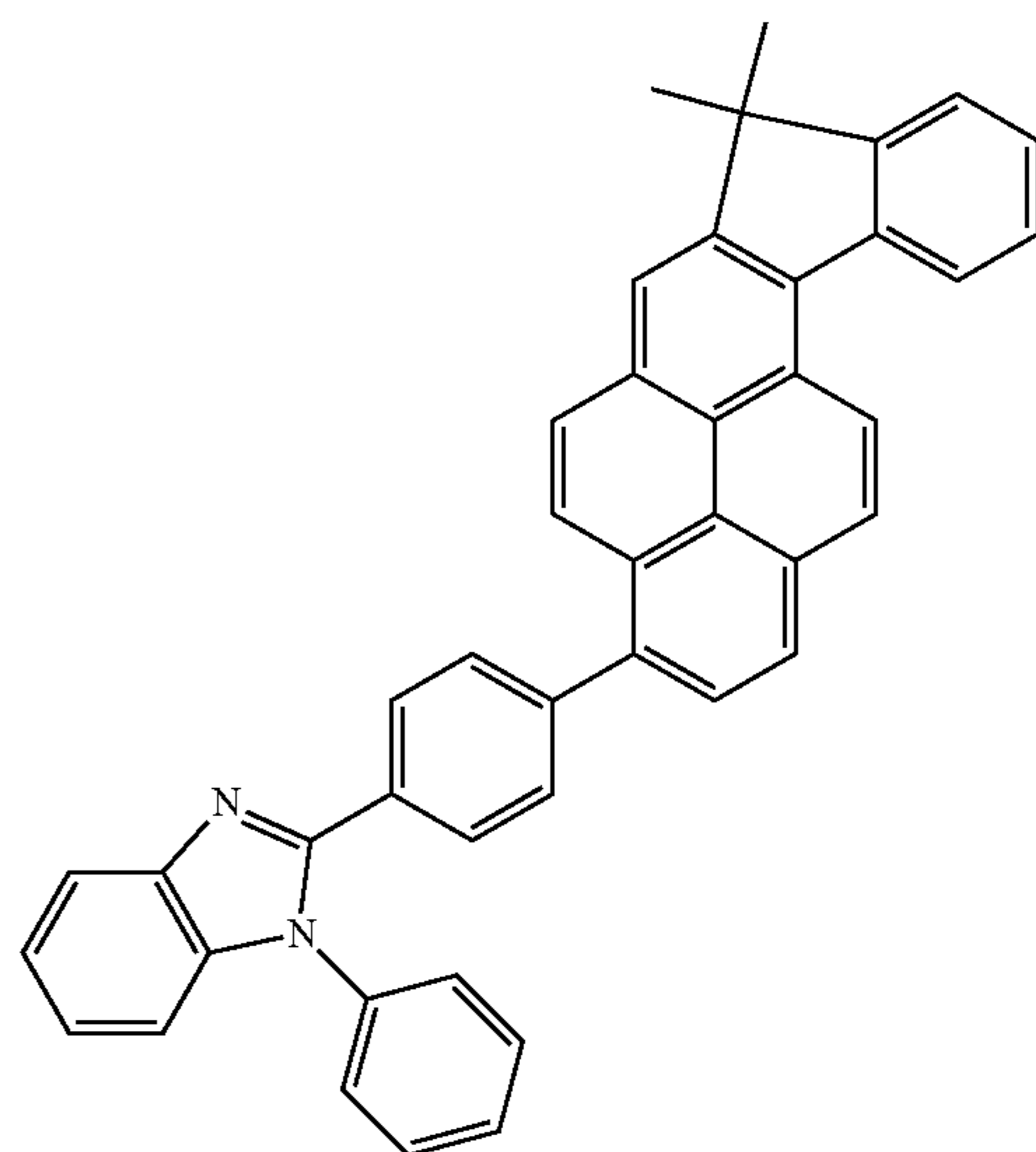
Compound 5
