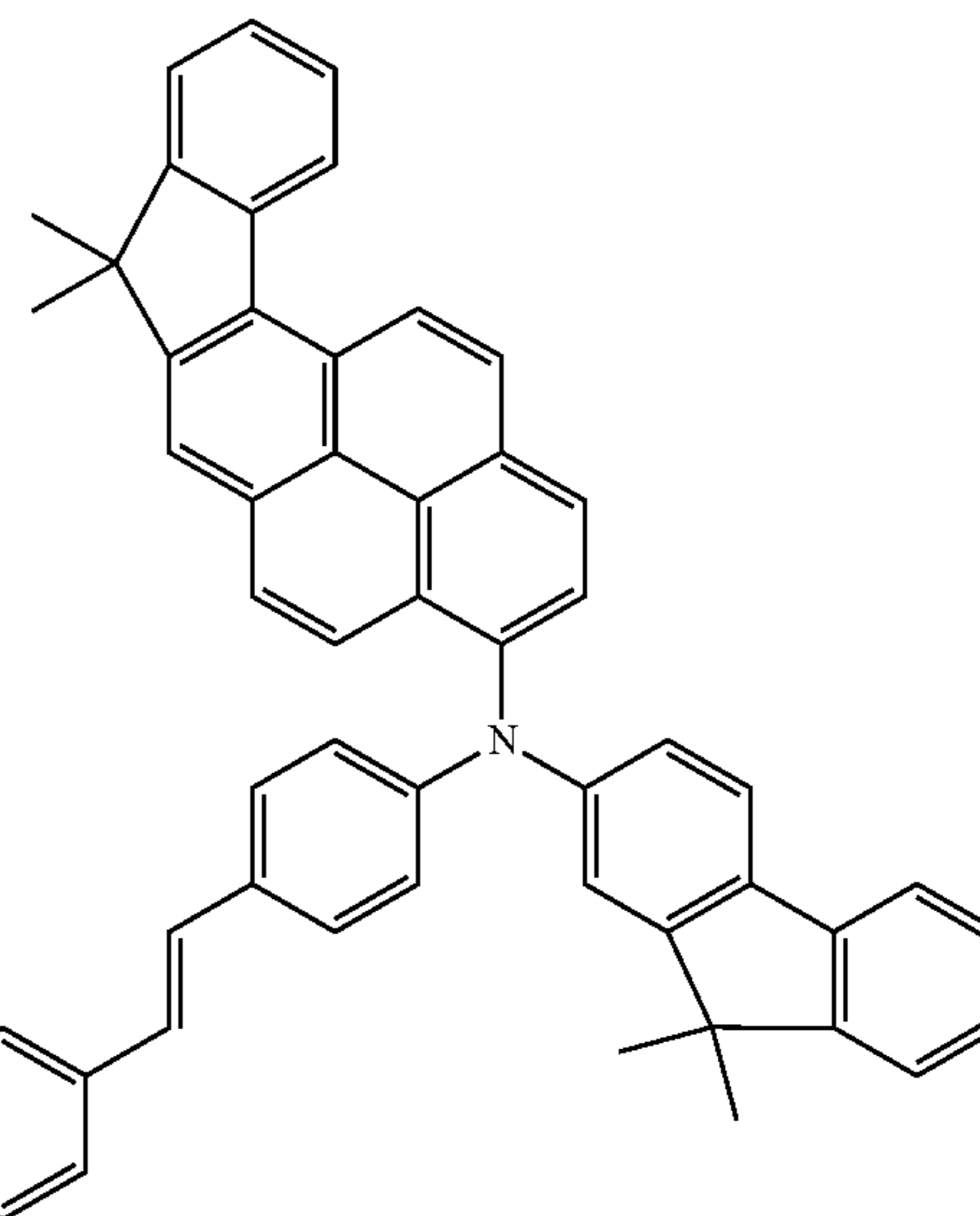
Compound 40
