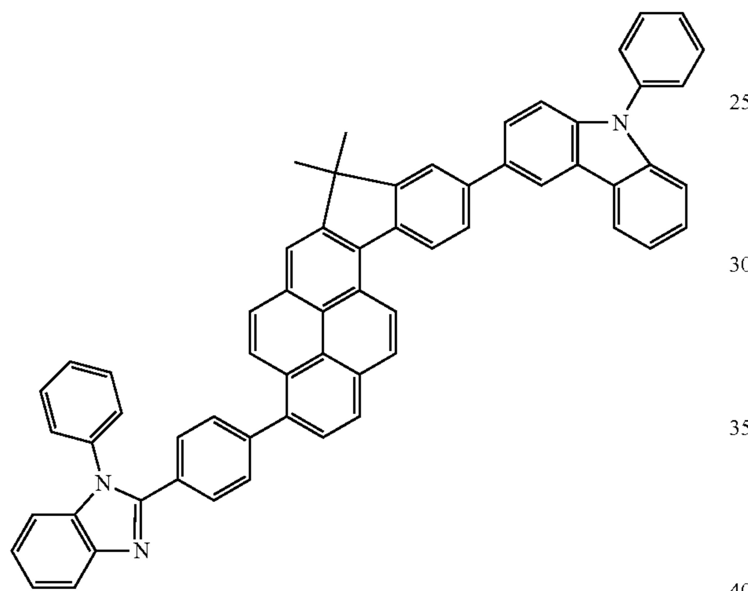
Compound 25
