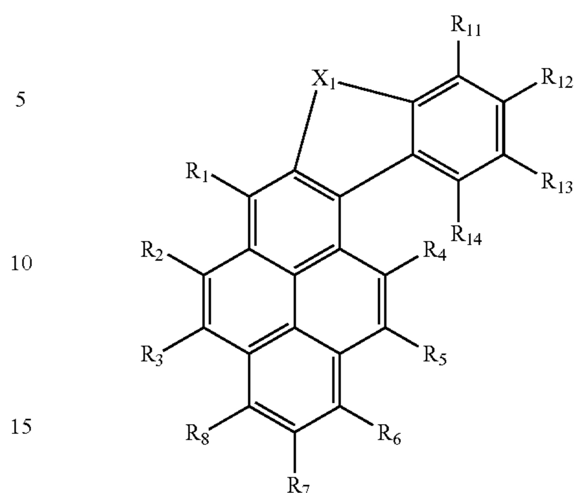
Compound 43
