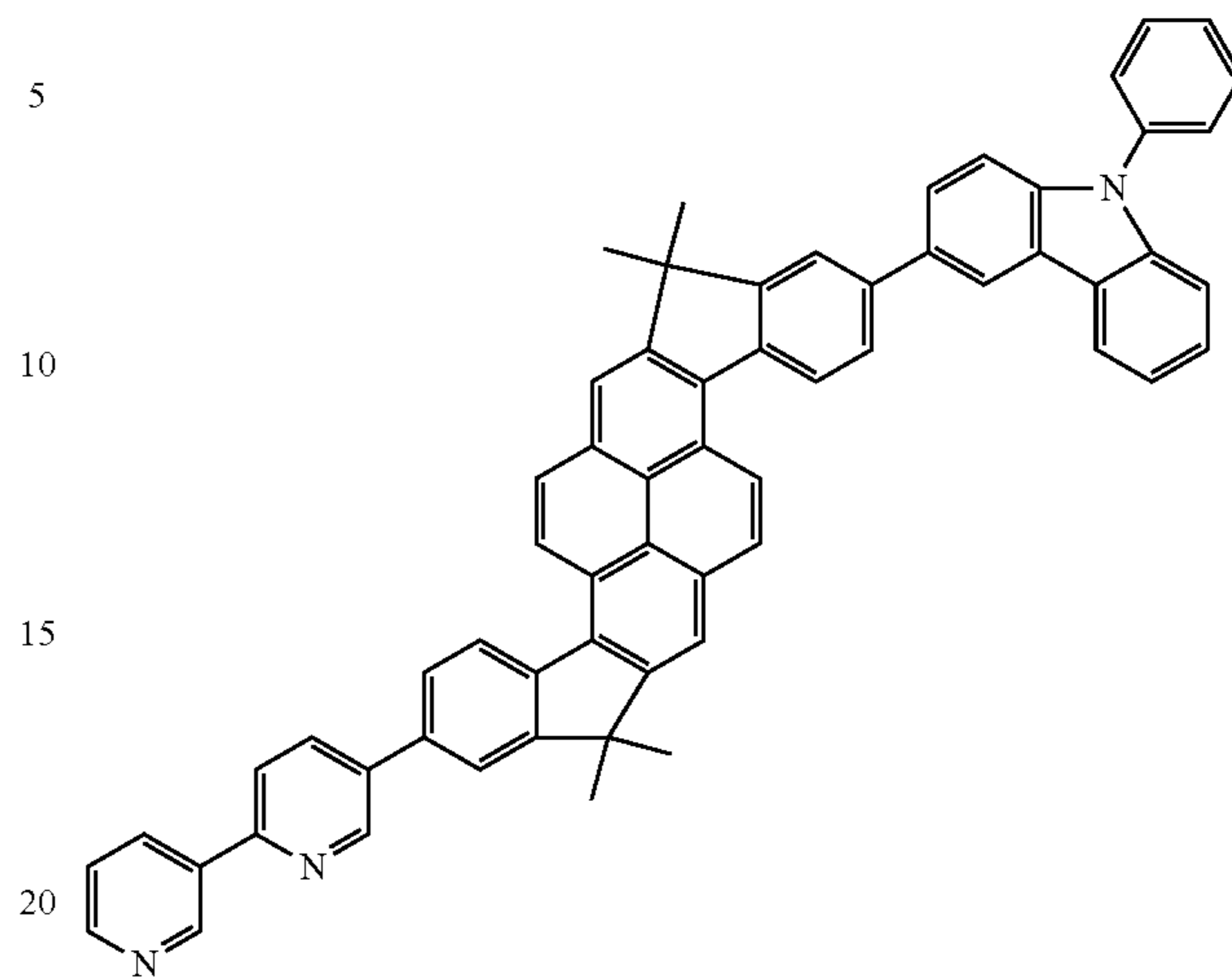
Compound 33
