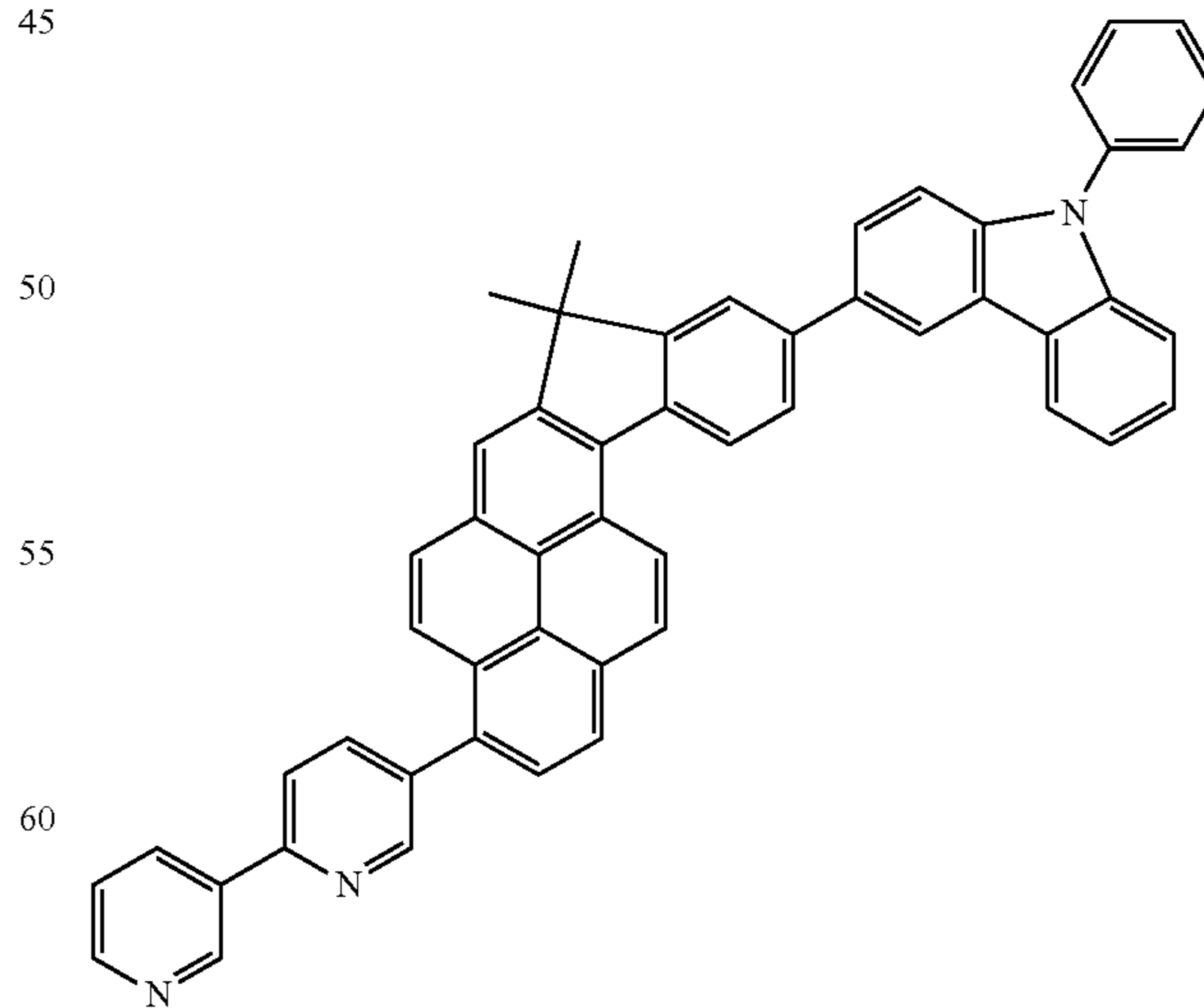
Compound 22
