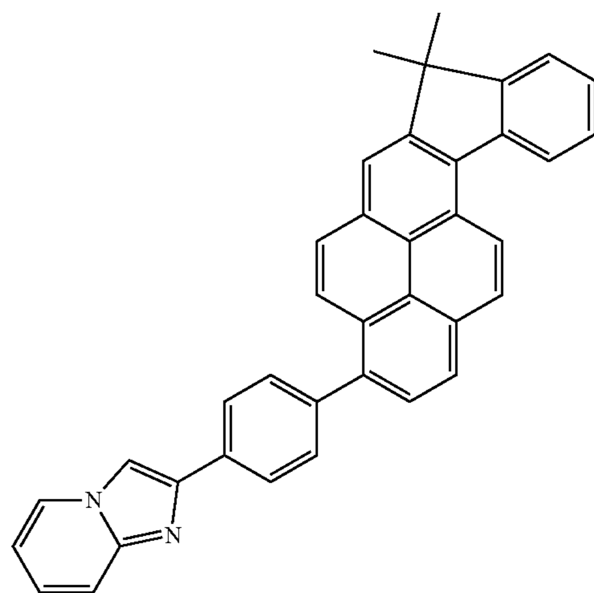
Compound 5
