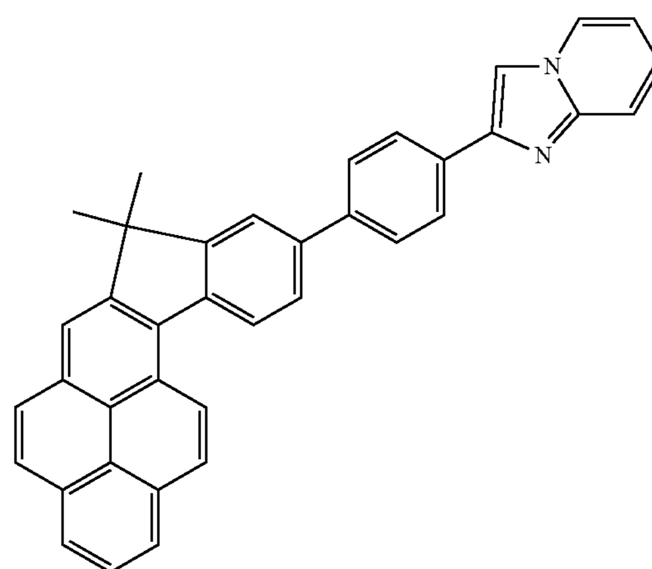
Compound 11
