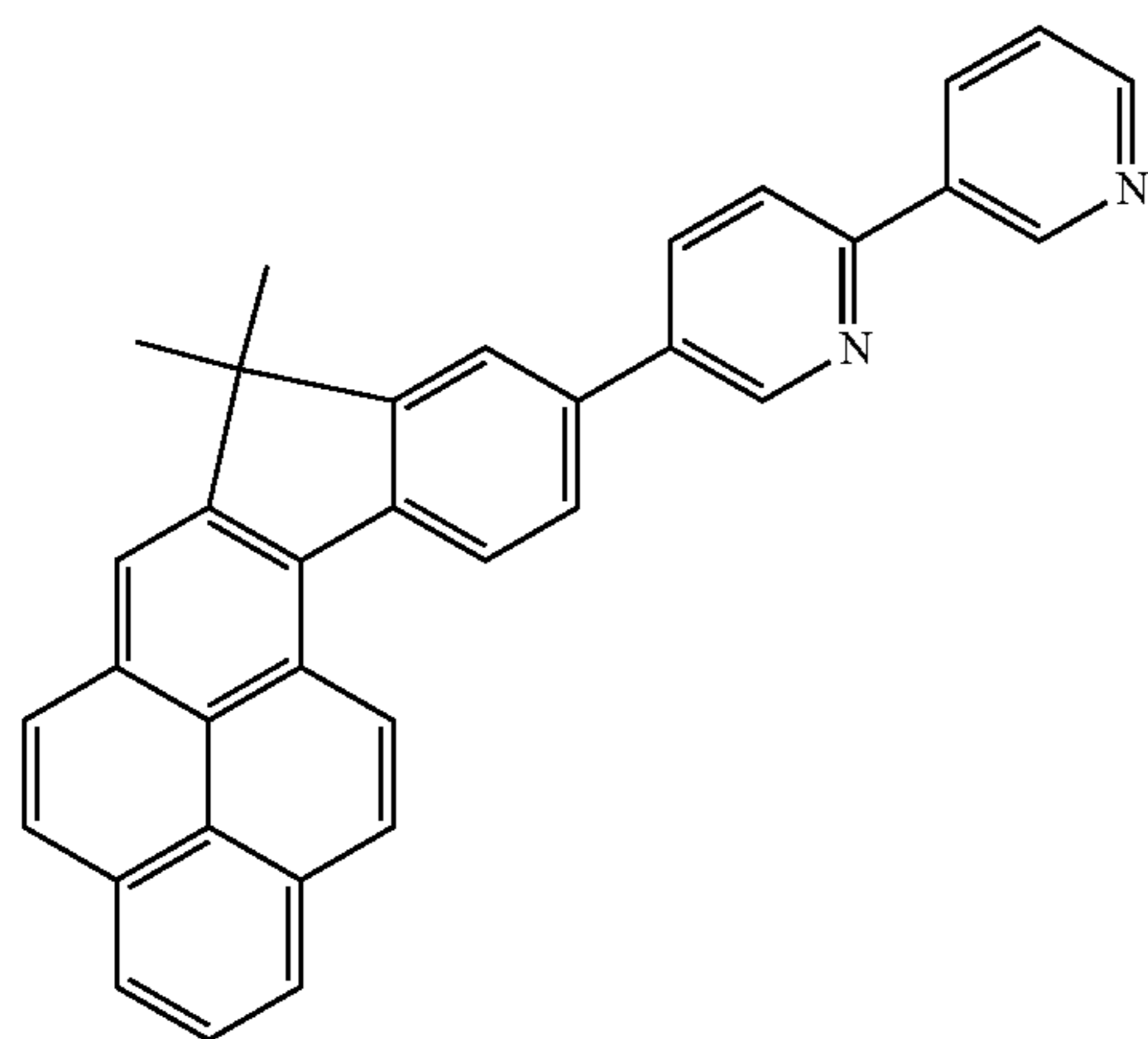
Compound 8
