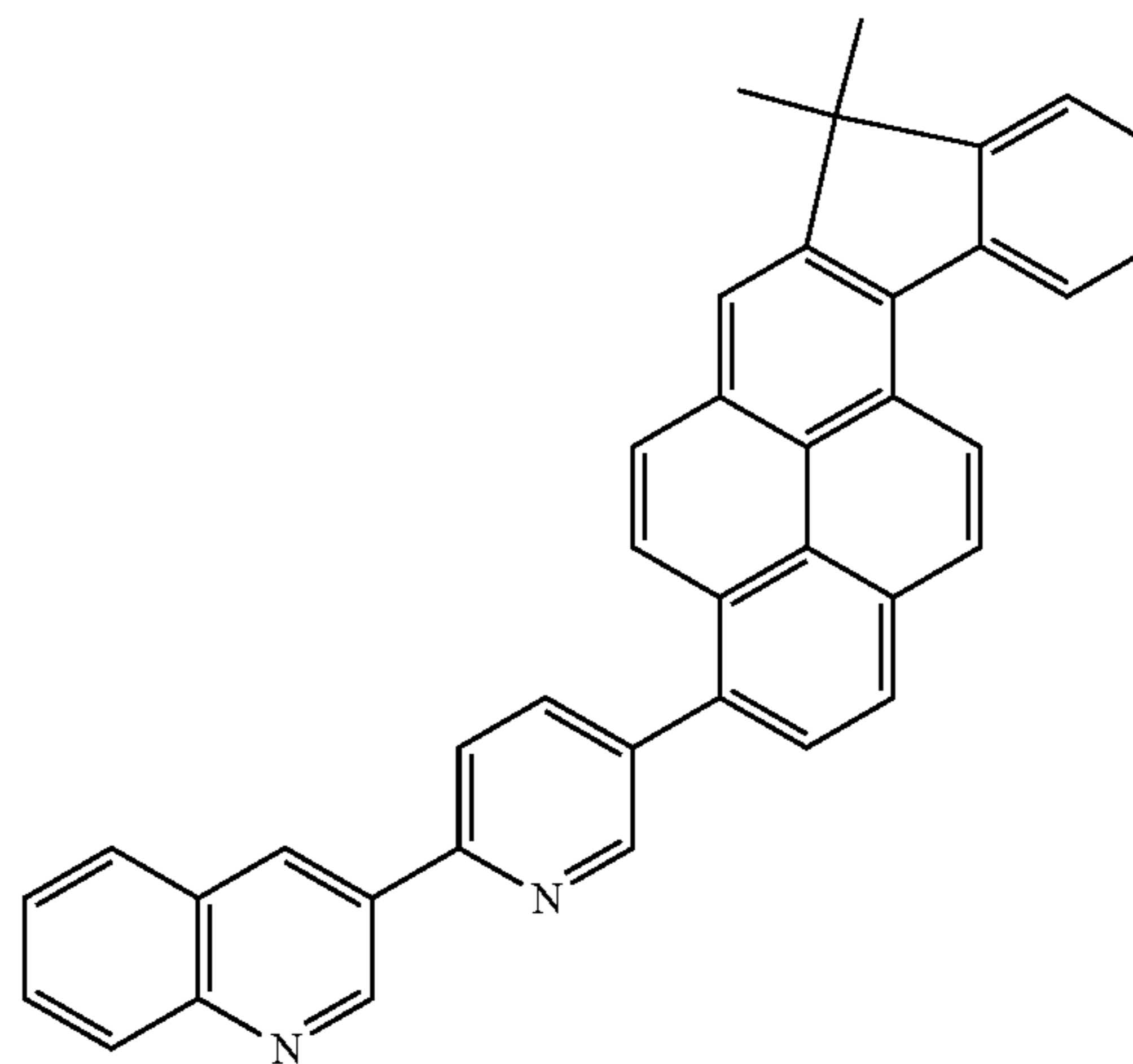
Compound 4
