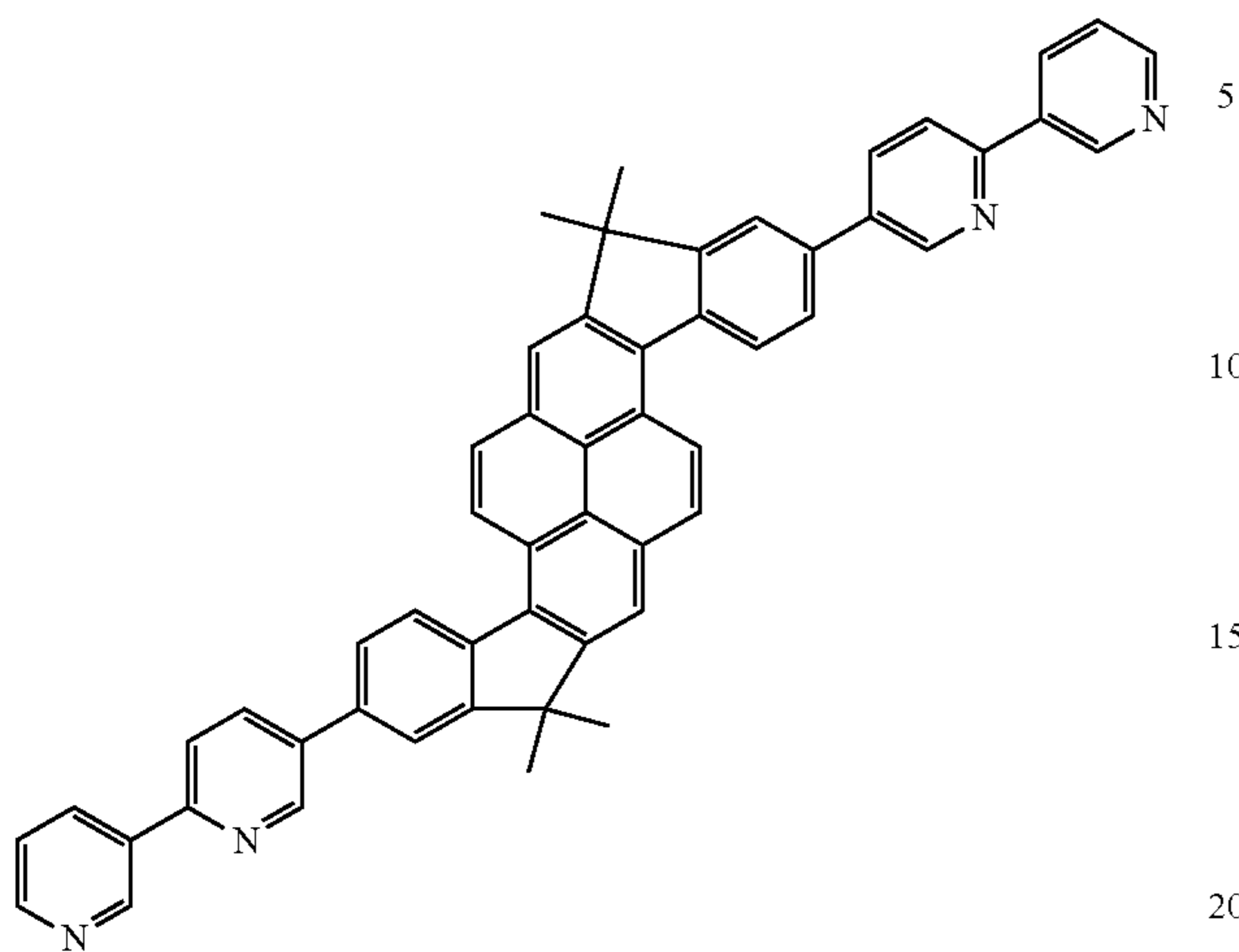
Compound 30
