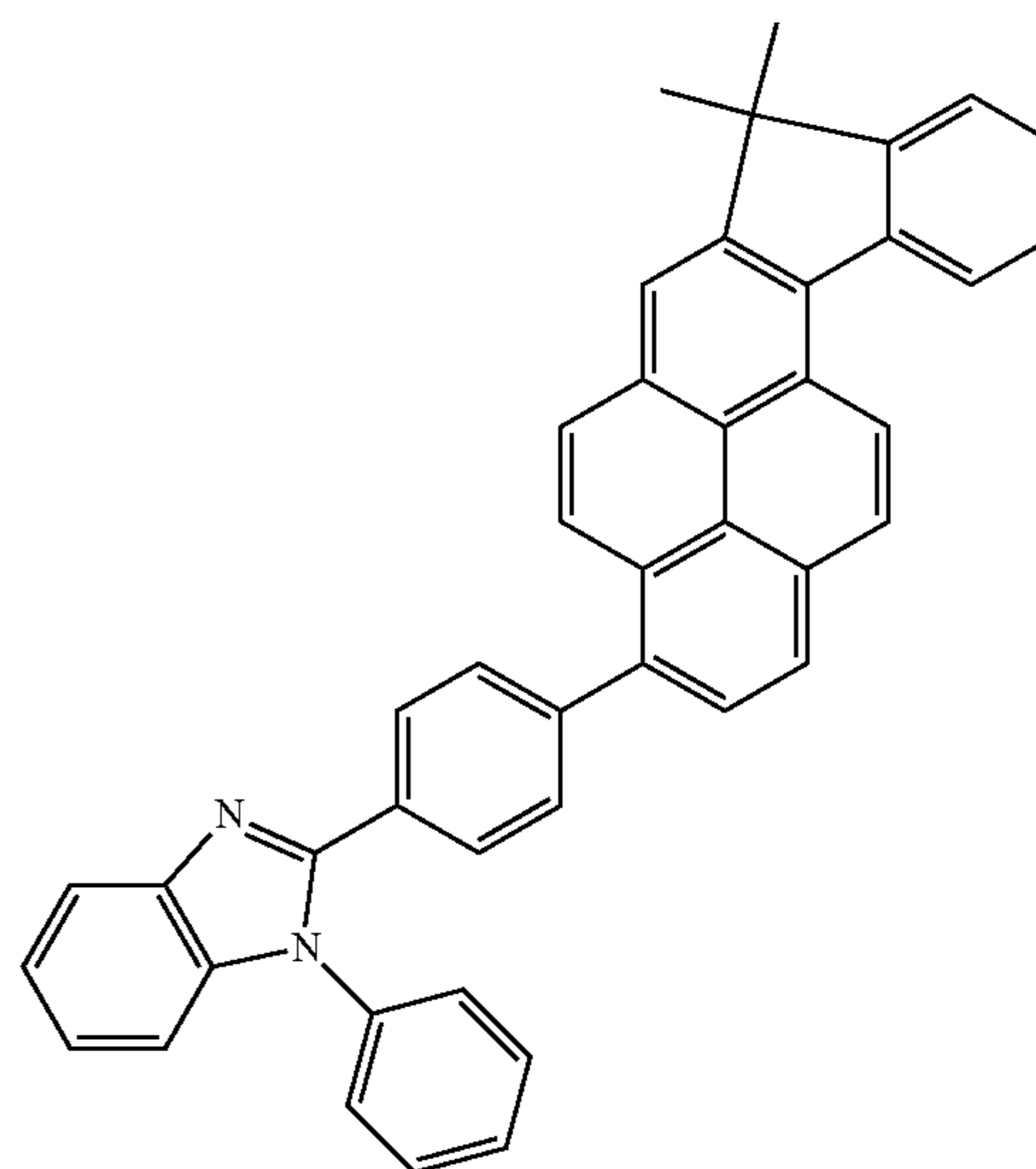
Compound 5
