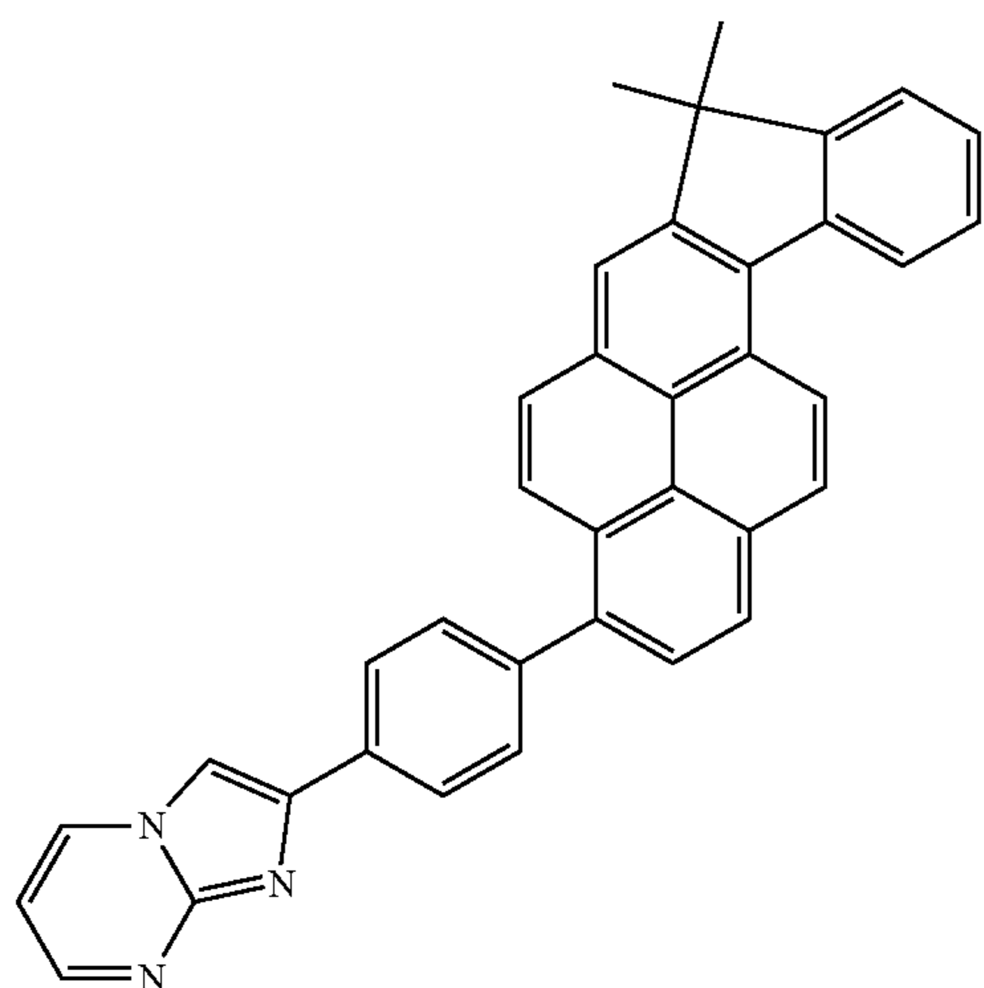
Compound 7
