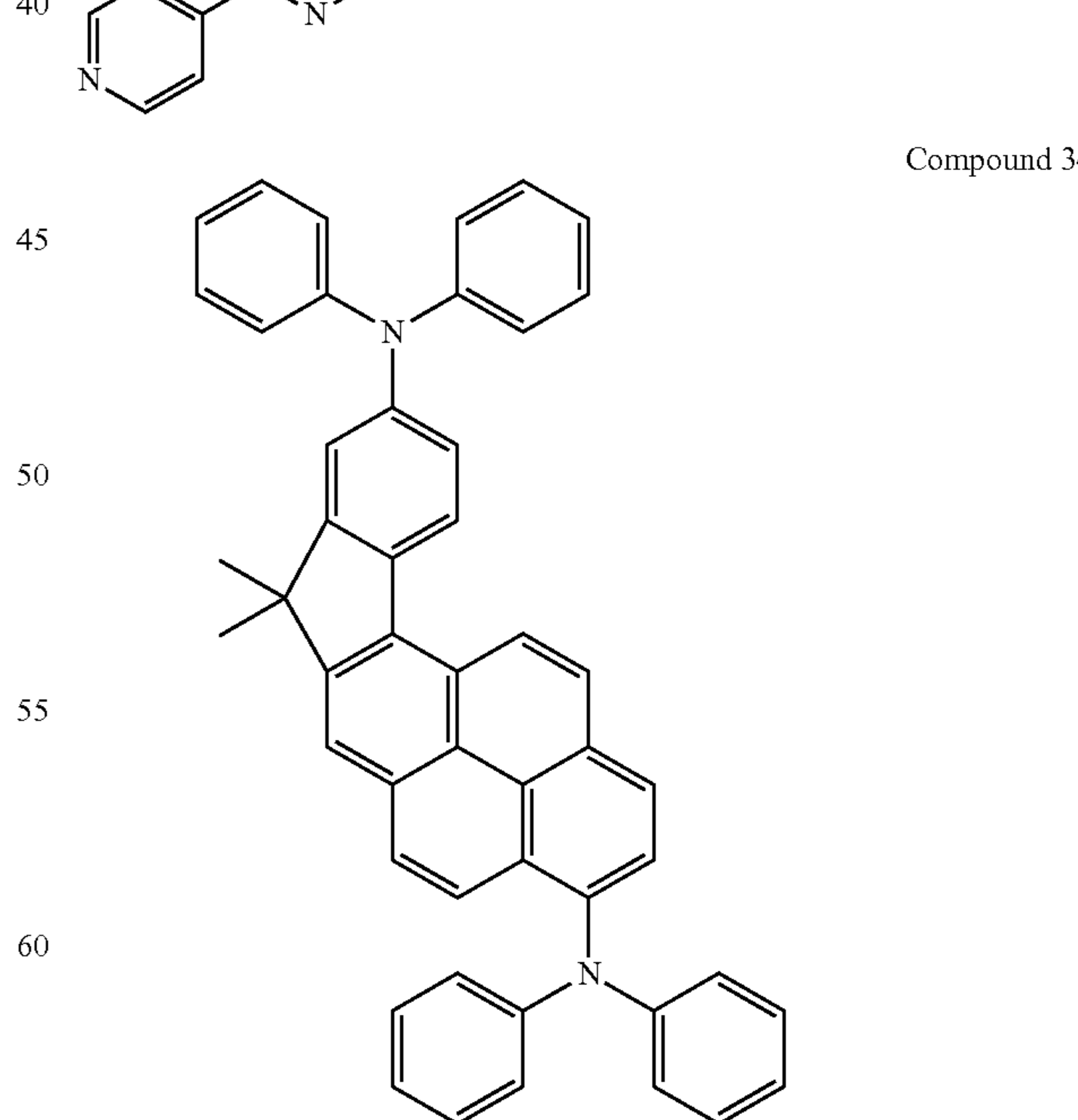
Compound 34
