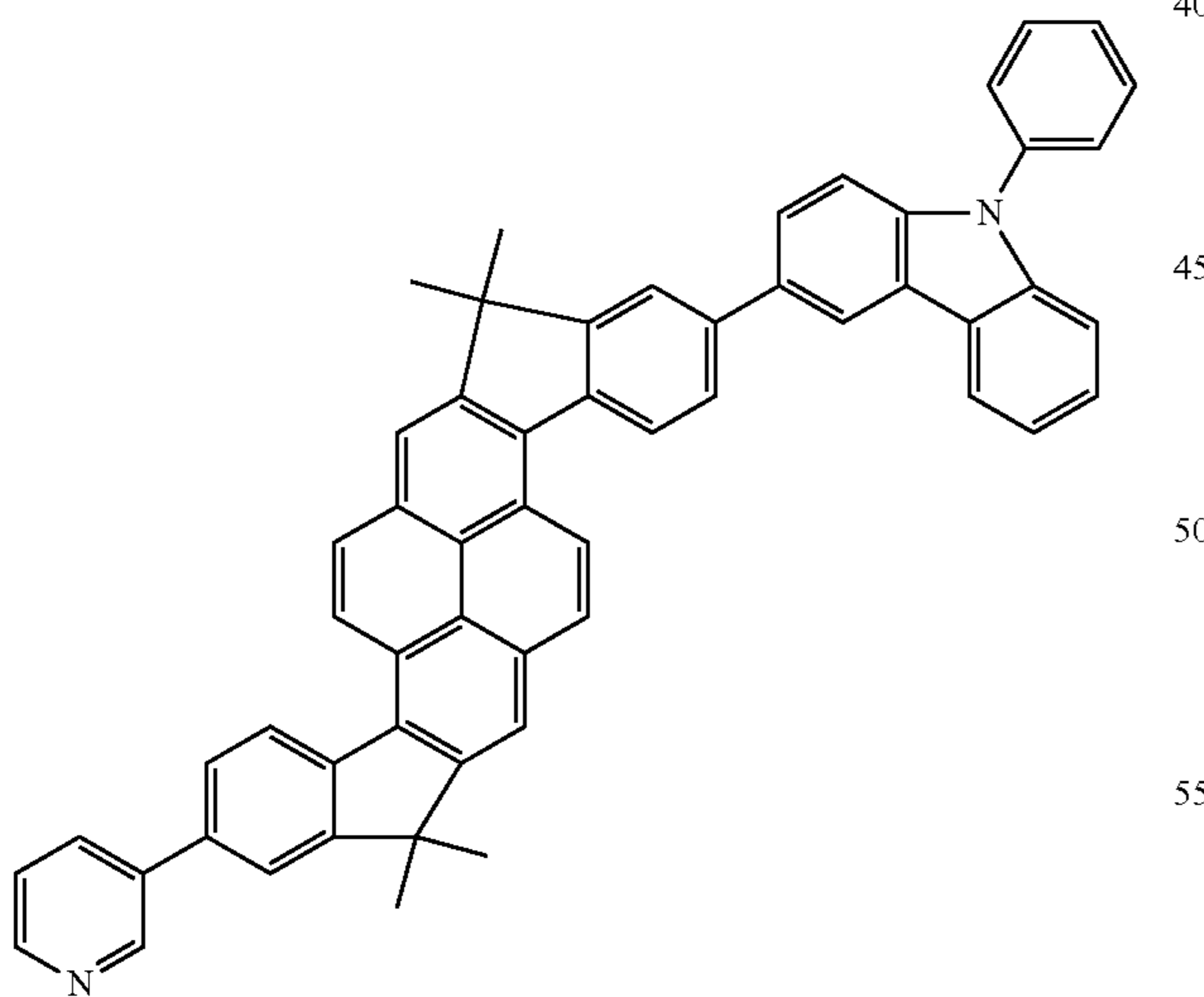
Compound 31
