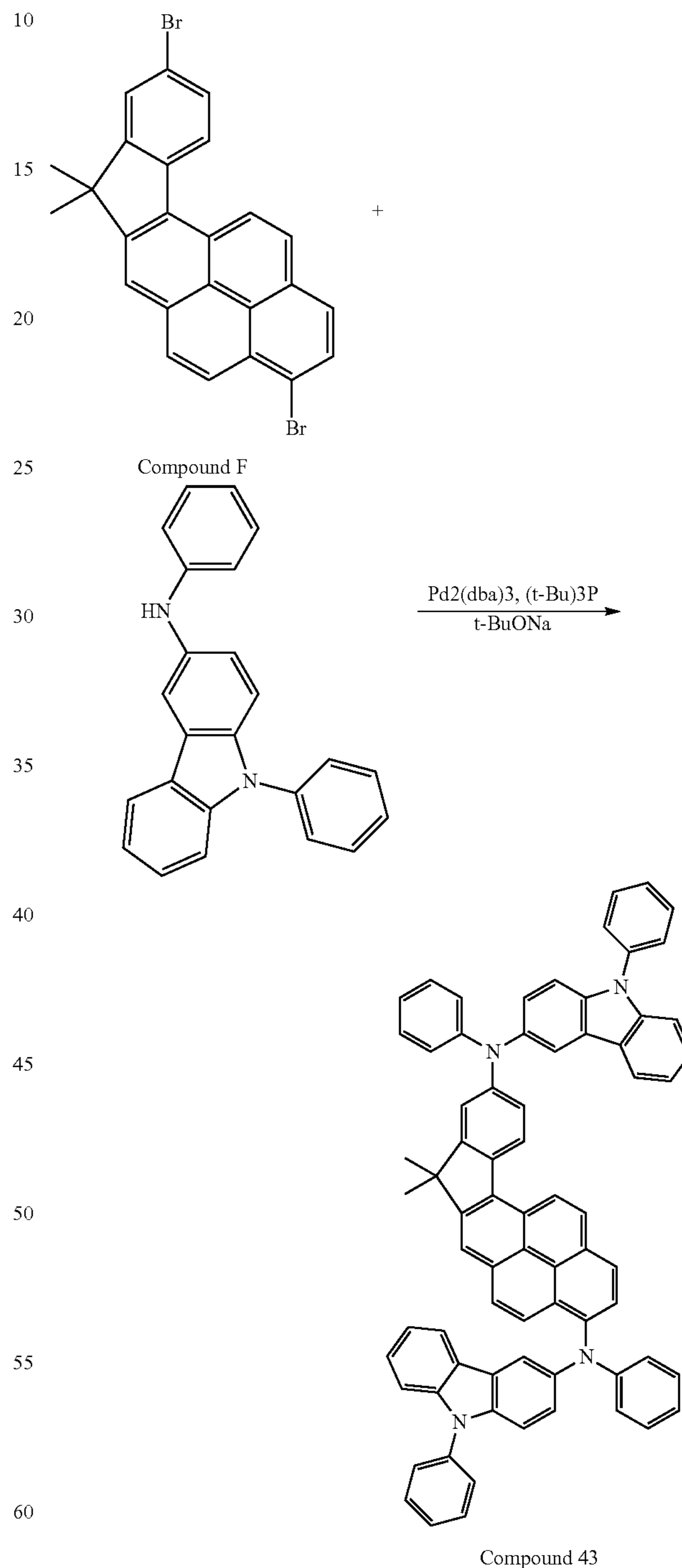
Reaction Scheme 8
