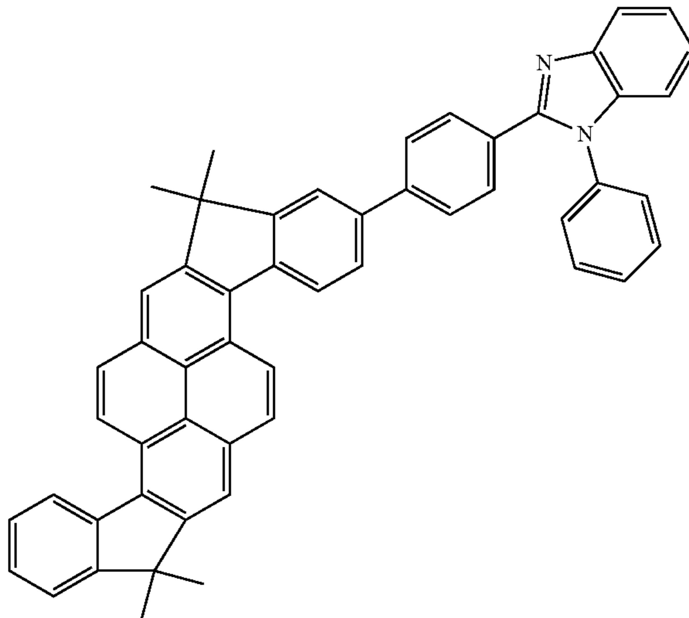
Compound 28
