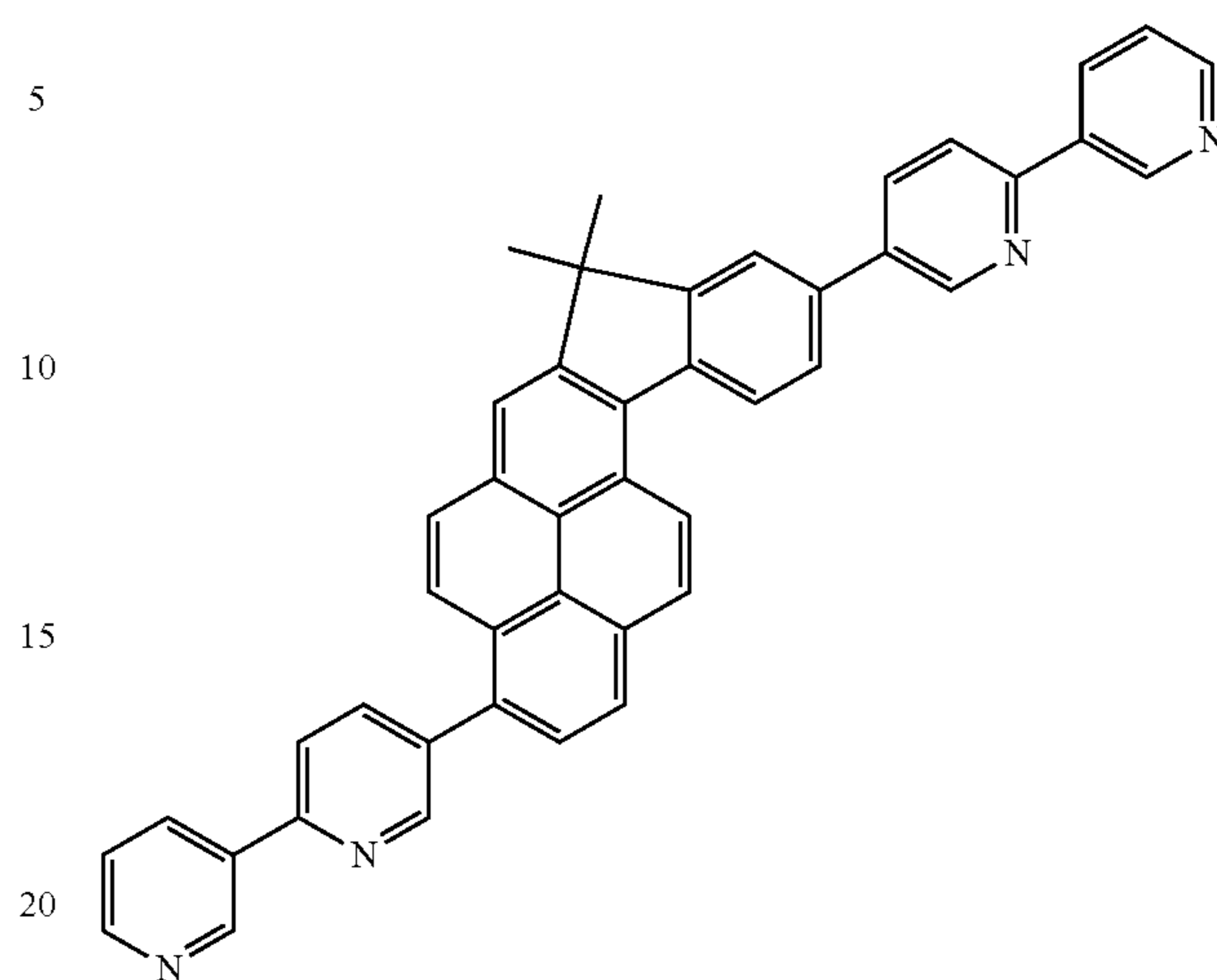
Compound 21
