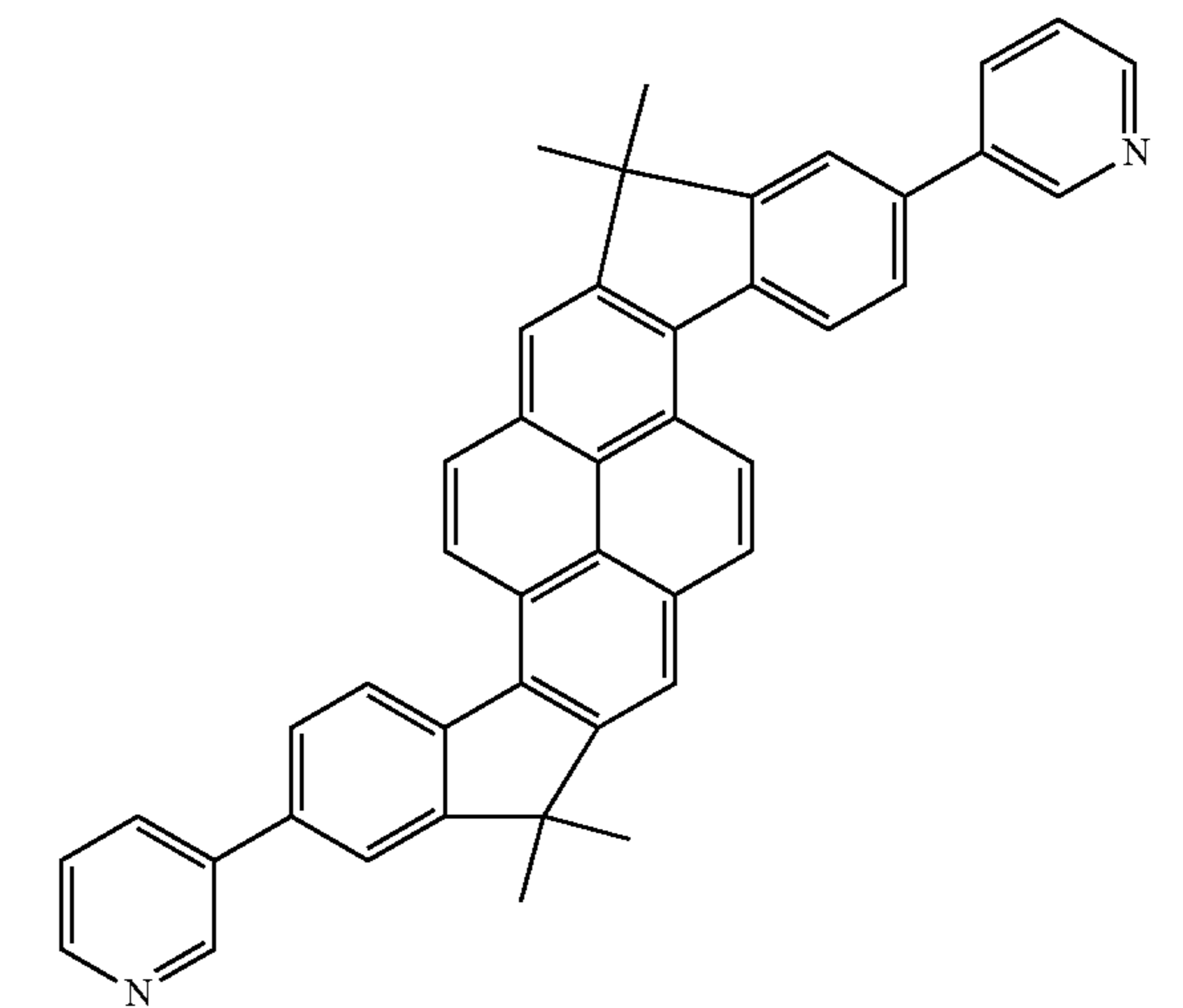
Compound 28
