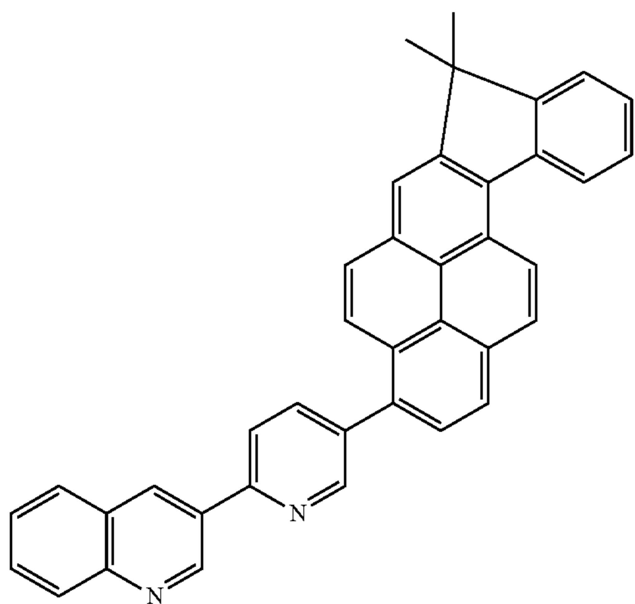
Compound 4
