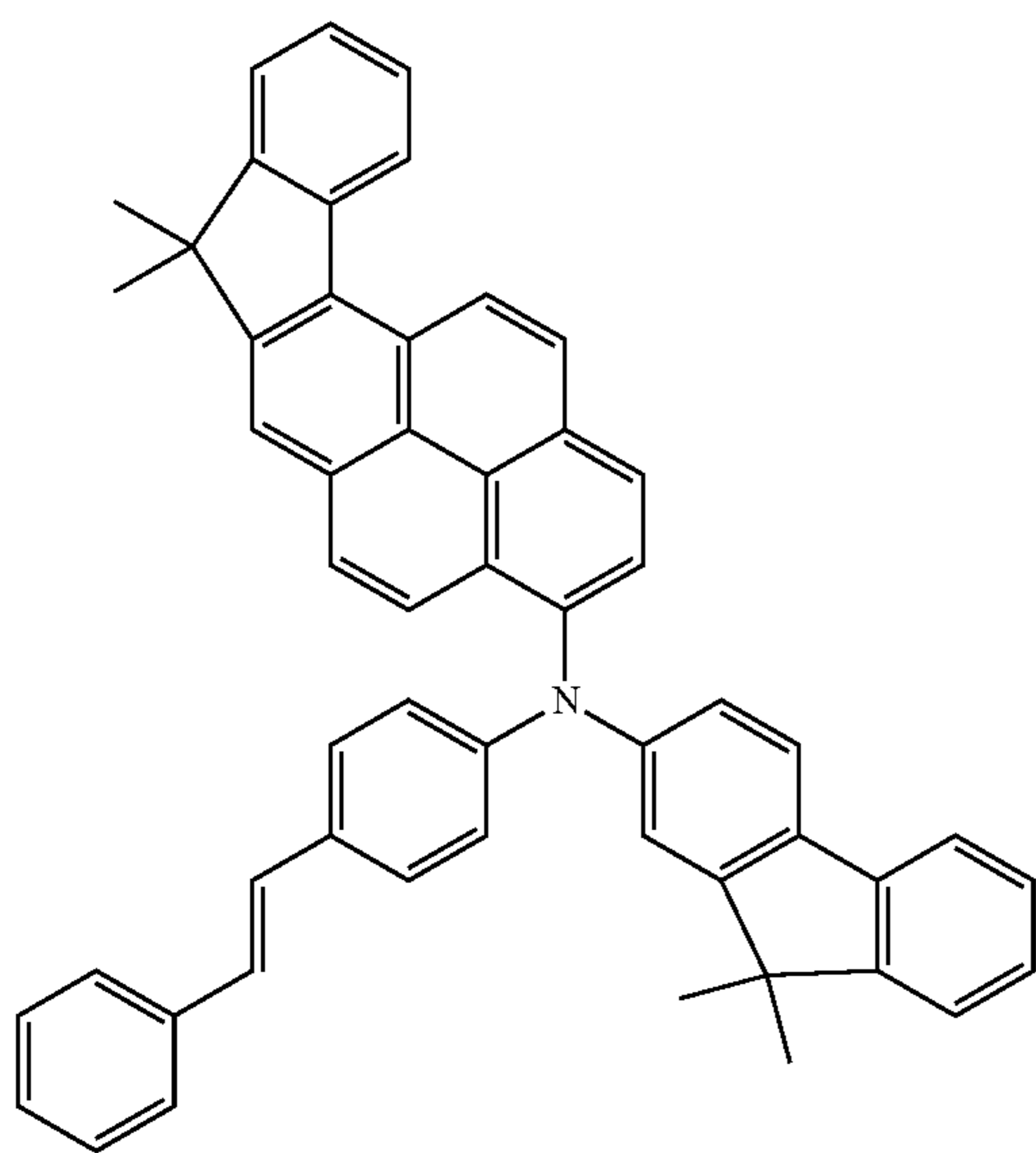
Compound 40
