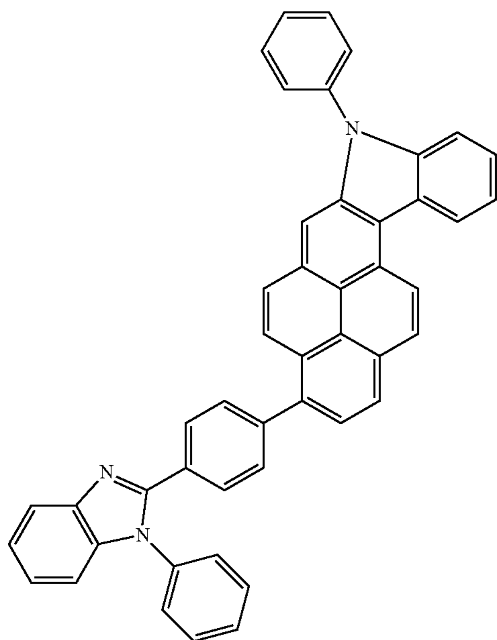
Compound 16
