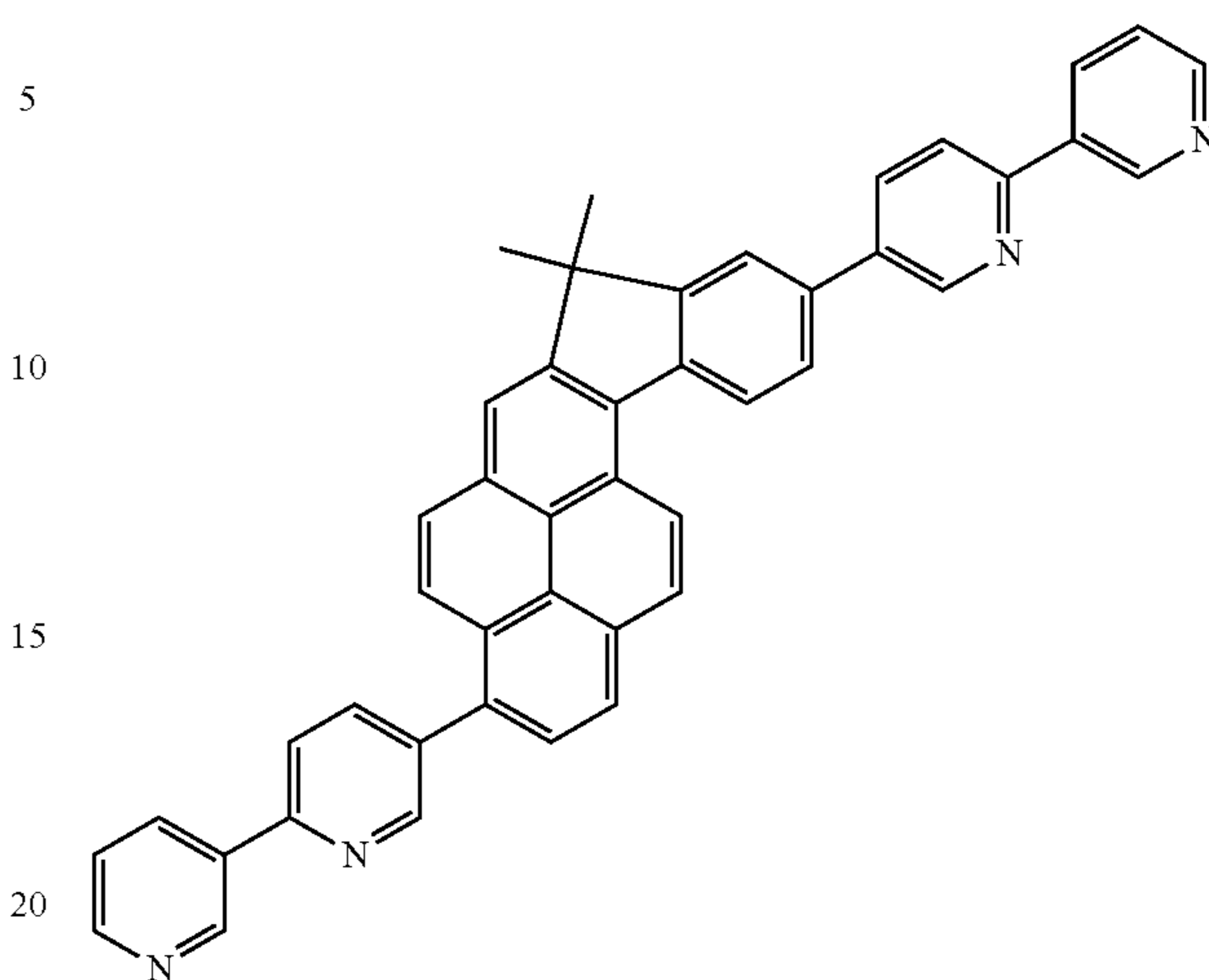
Compound 21
