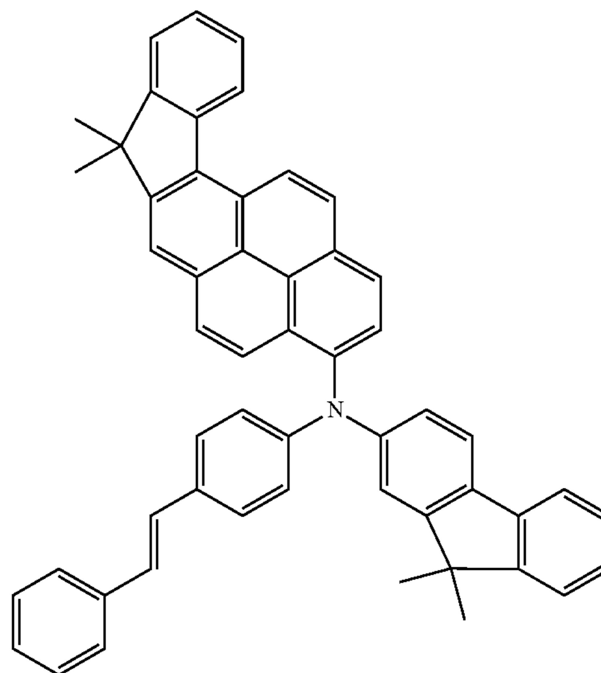
Compound 40
