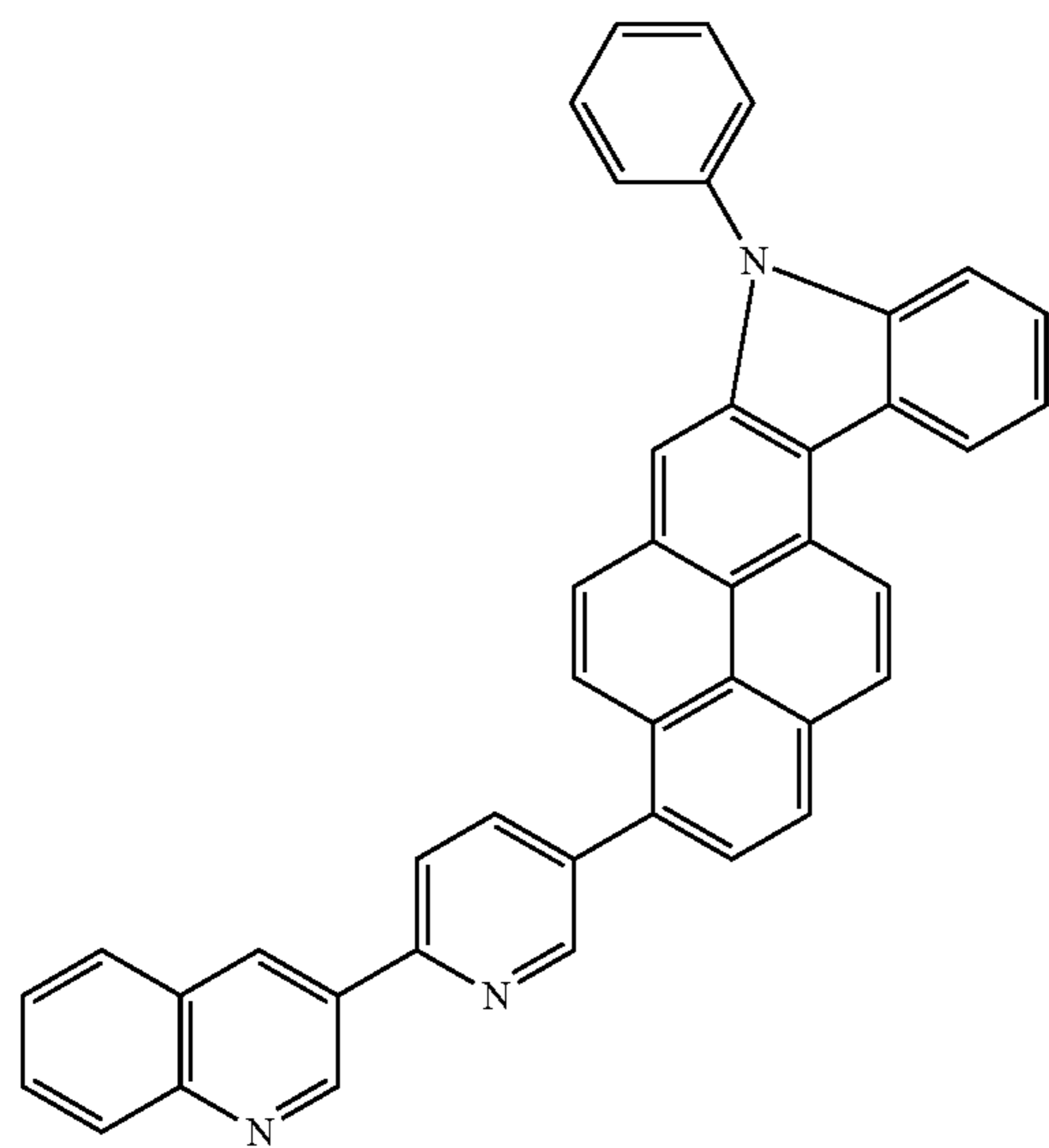
Compound 16
