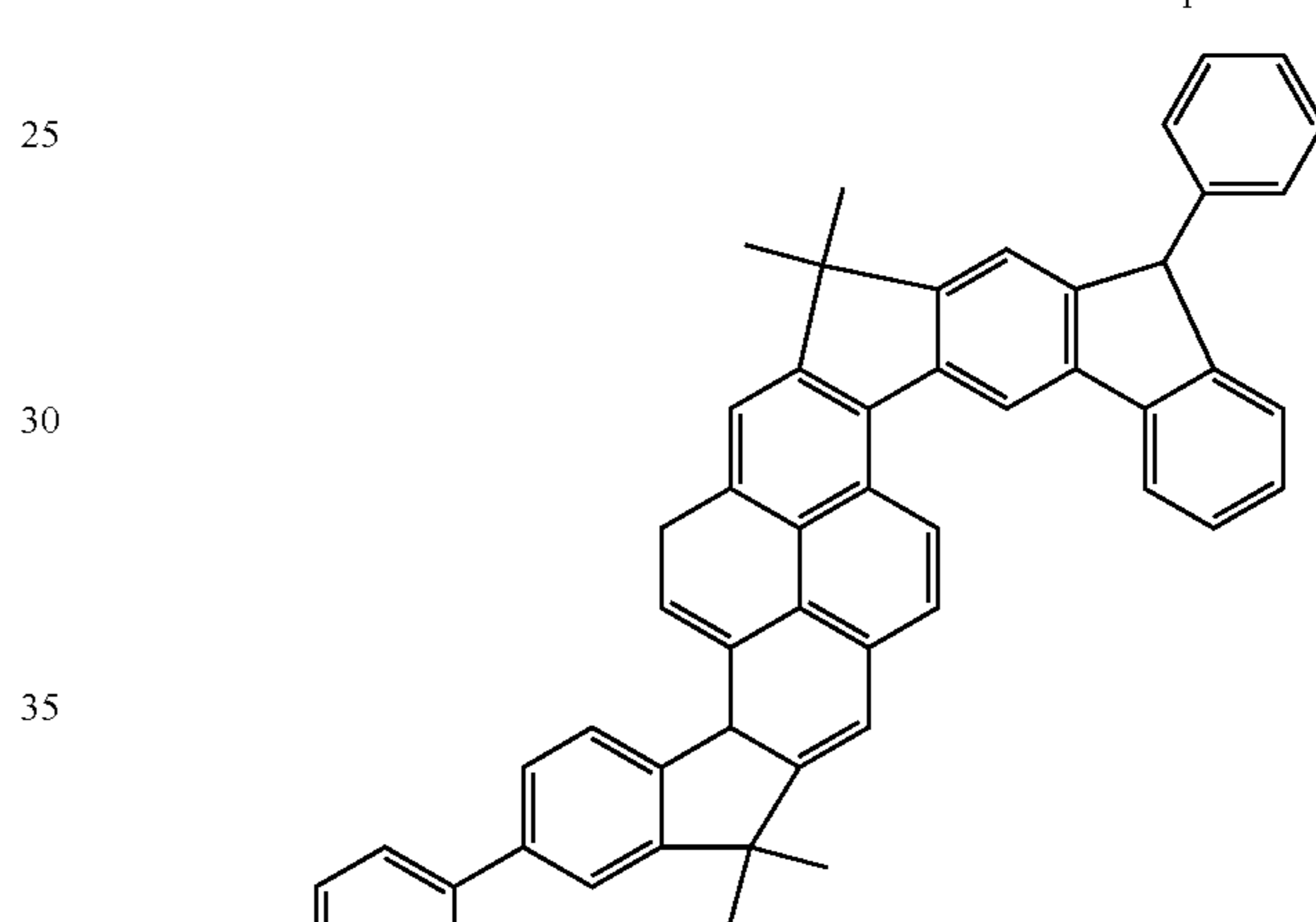
Compound 34
