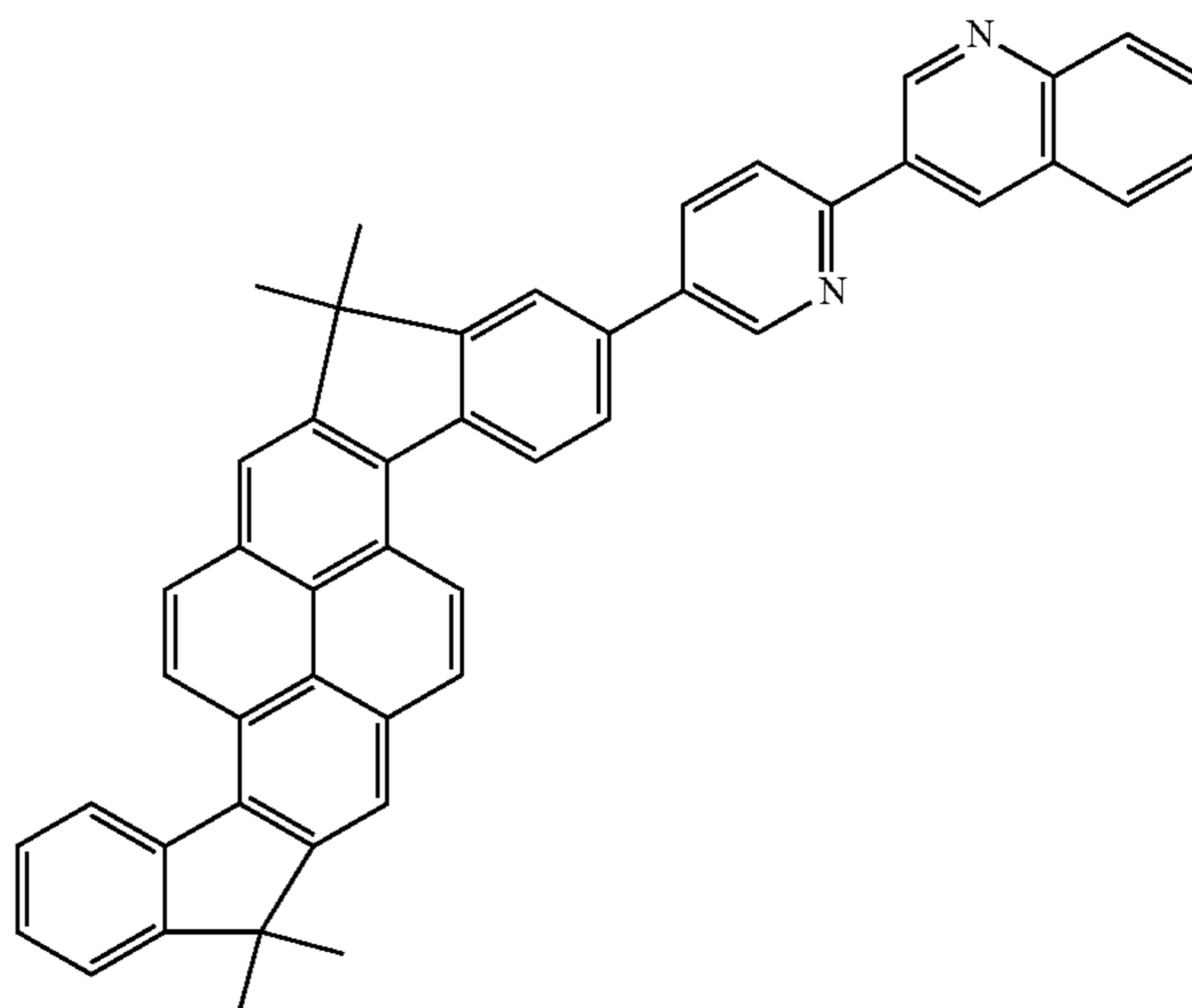
Compound 27
