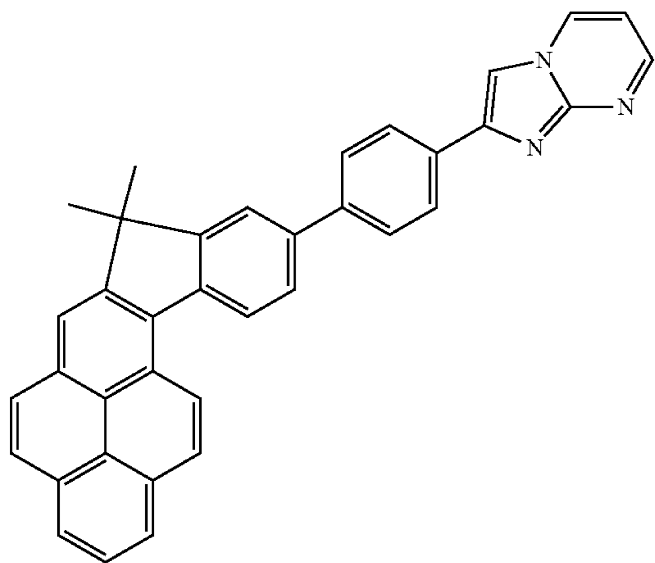
Compound 13
