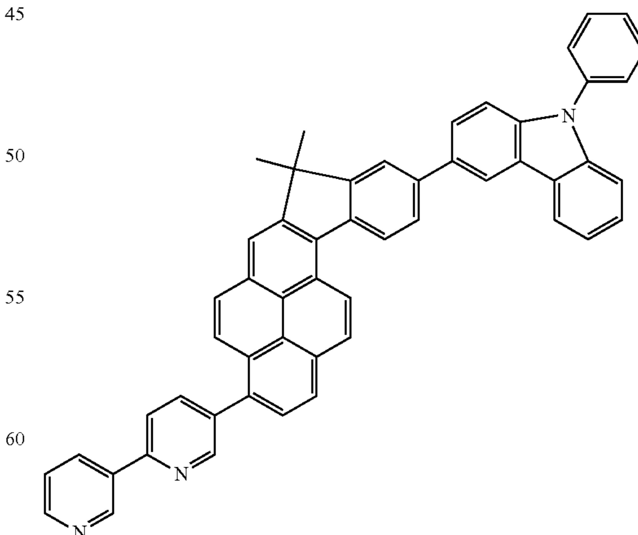
Compound 22
