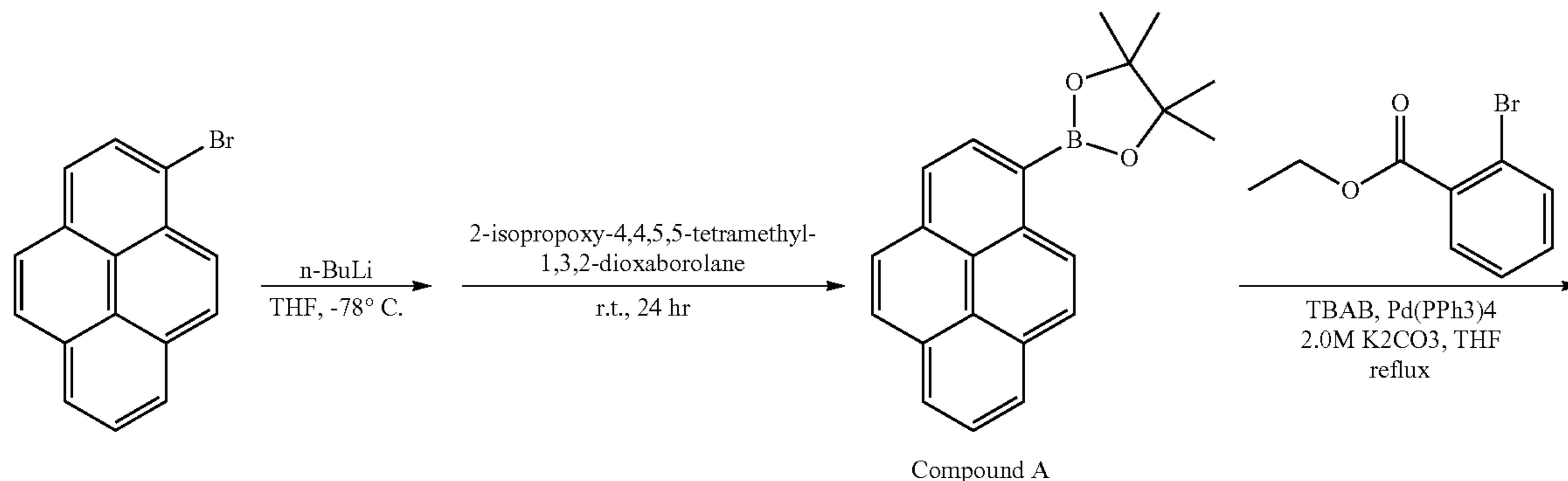
Reaction Scheme 2
