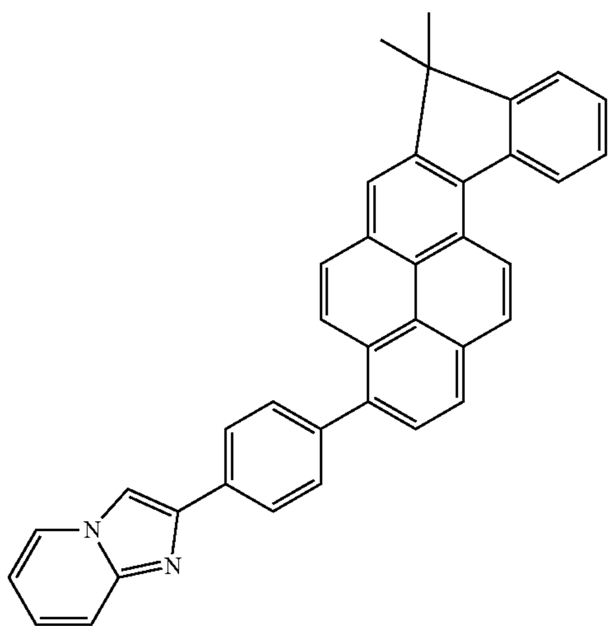
Compound 5
