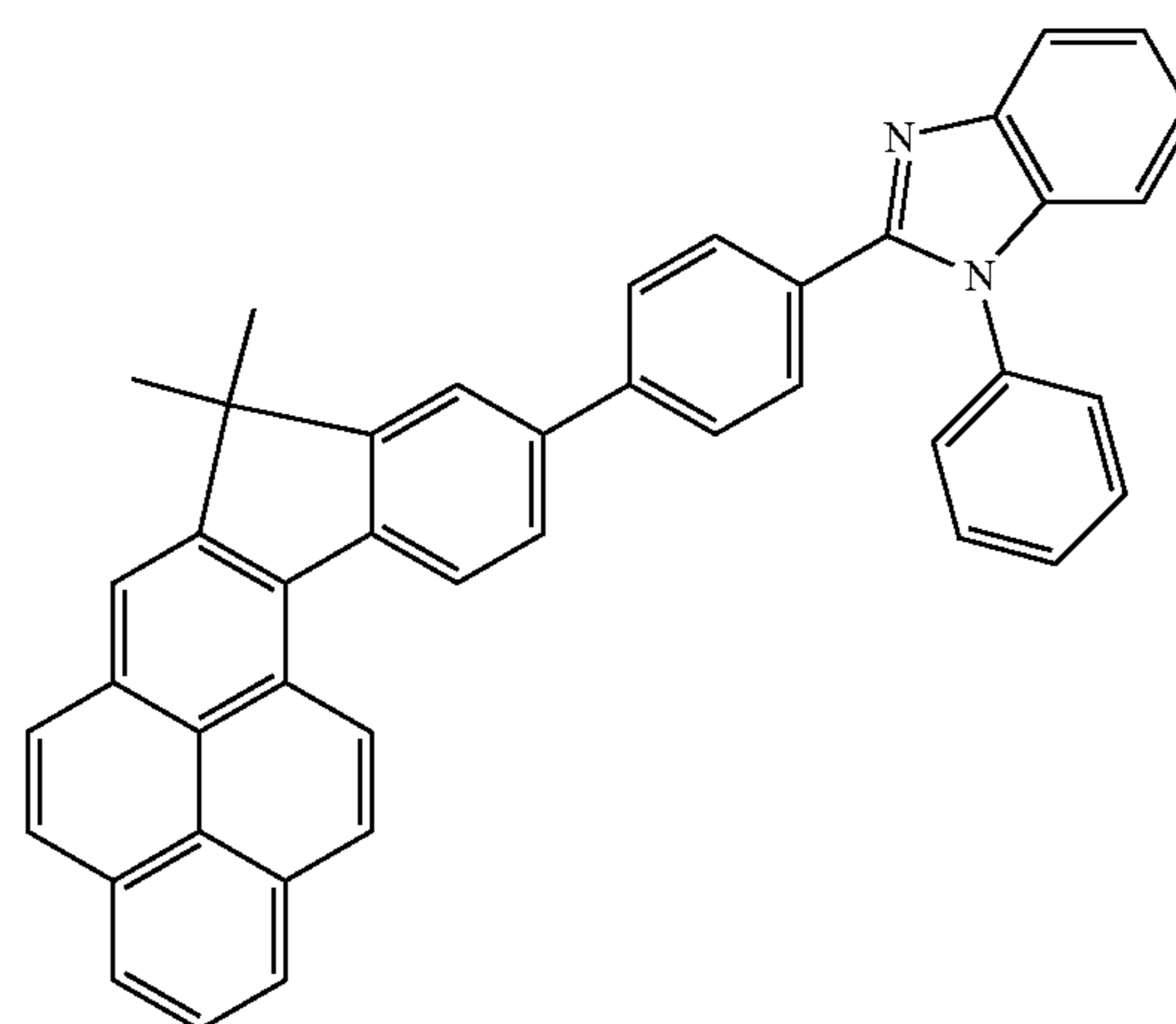
Compound 11
