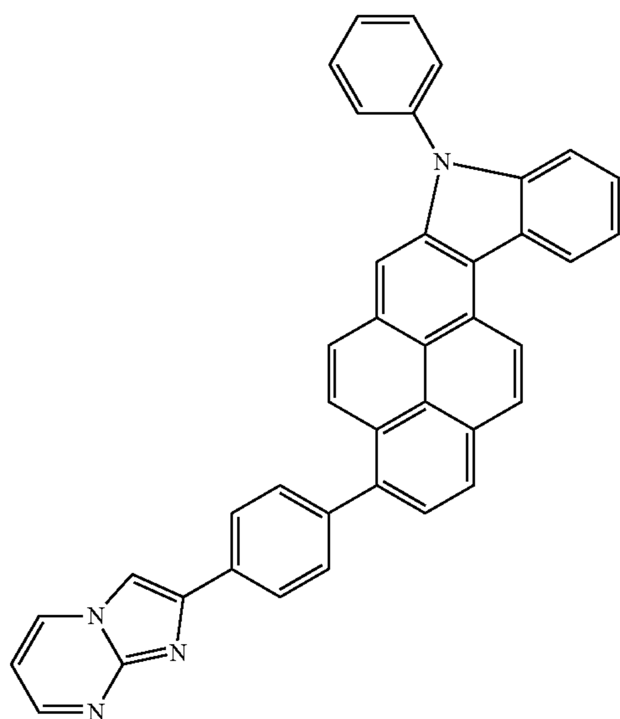
Compound 19
