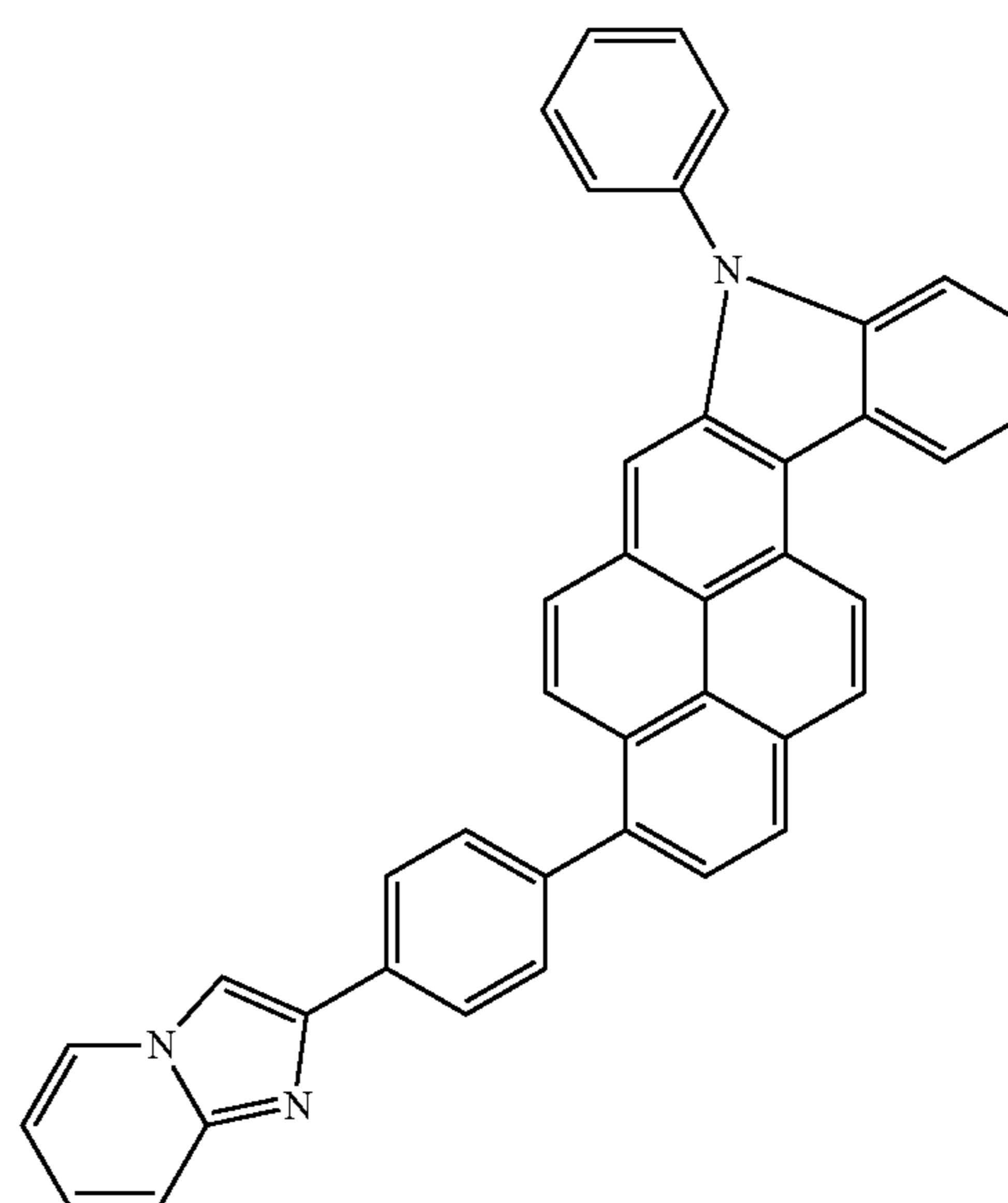
Compound 18
