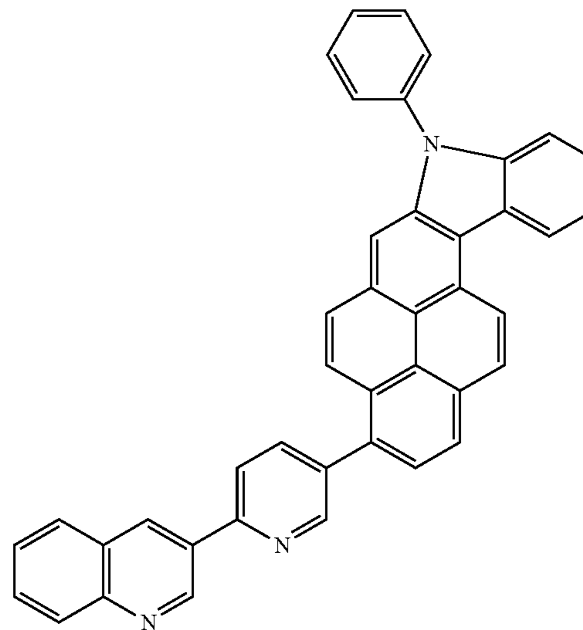
Compound 16
