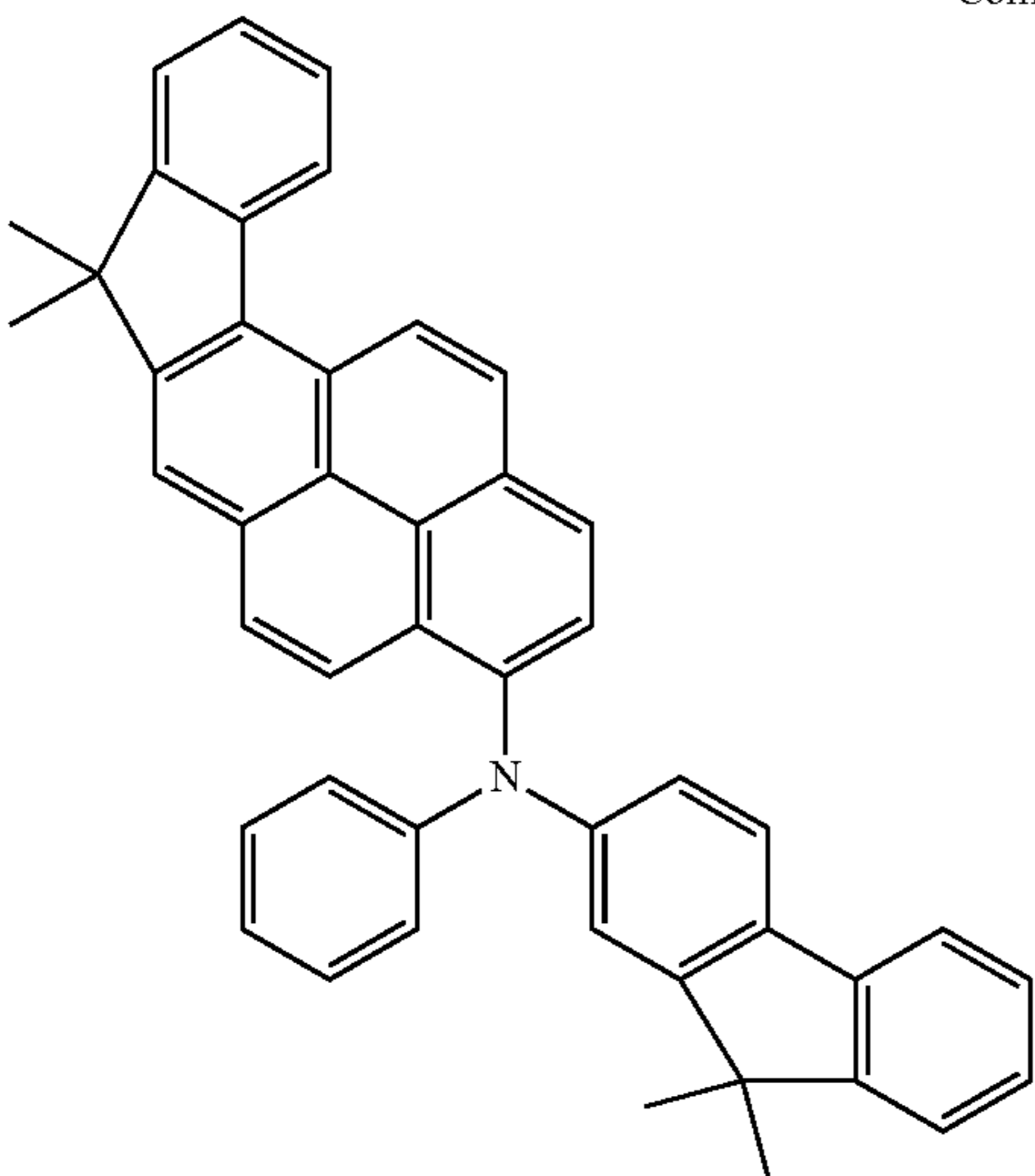
Compound 37
