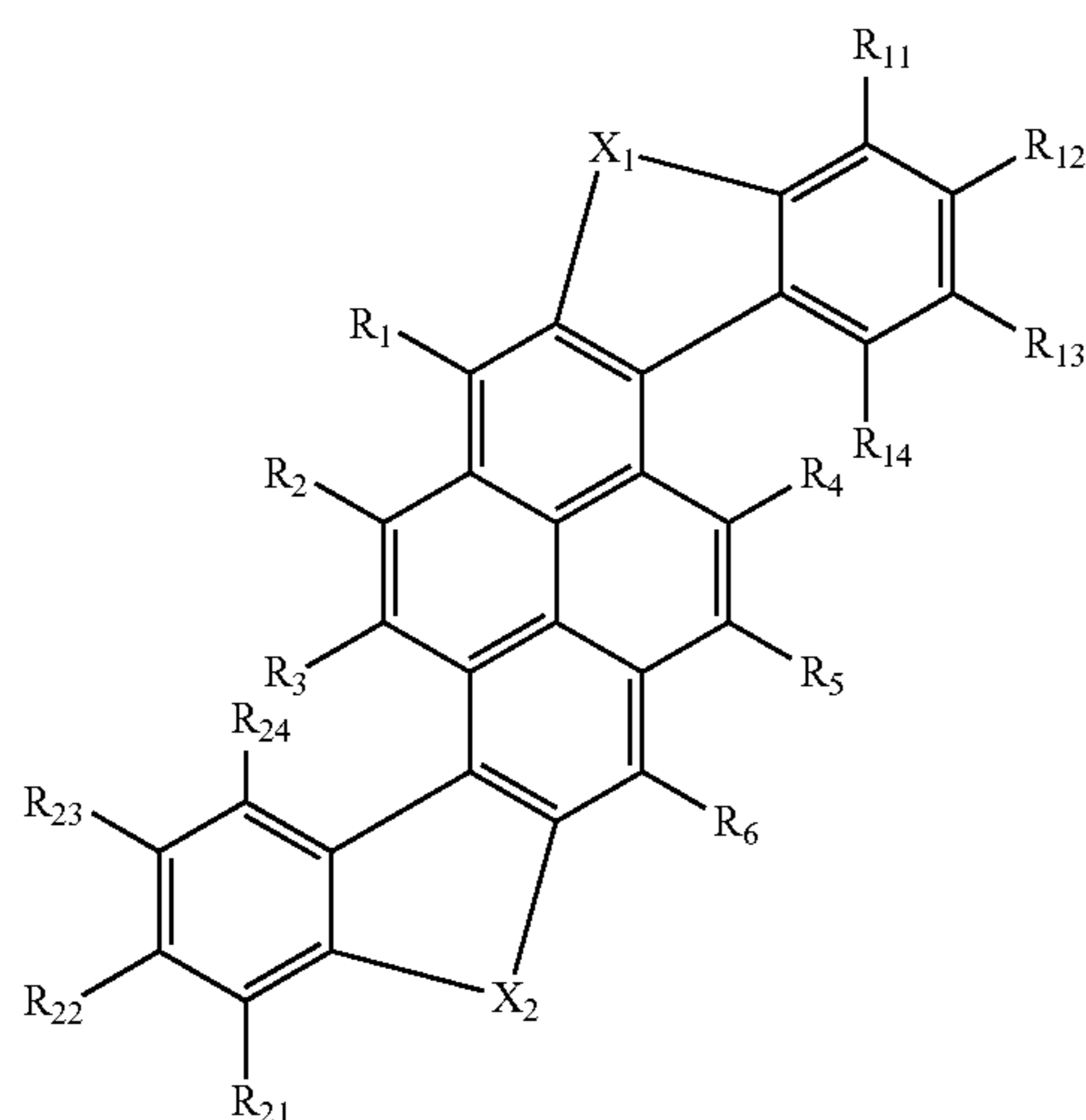
Formula 1A
