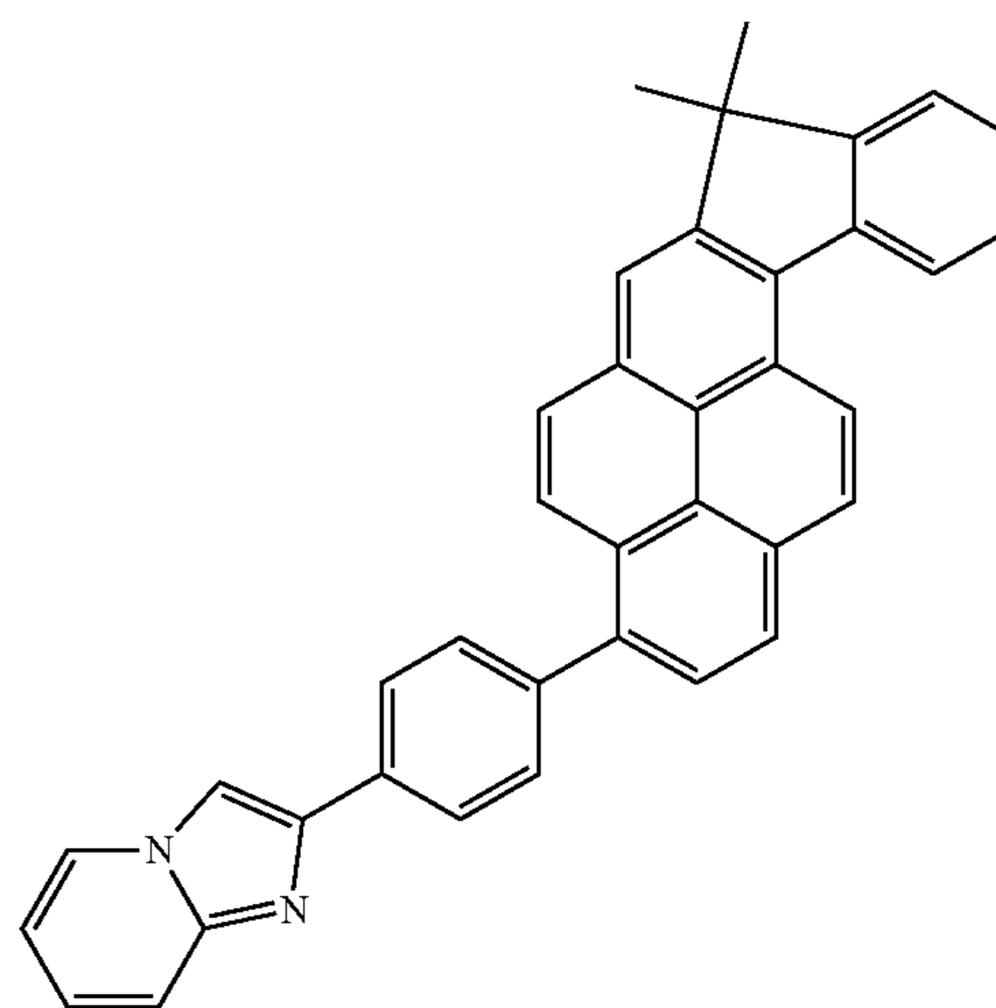
Compound 5
