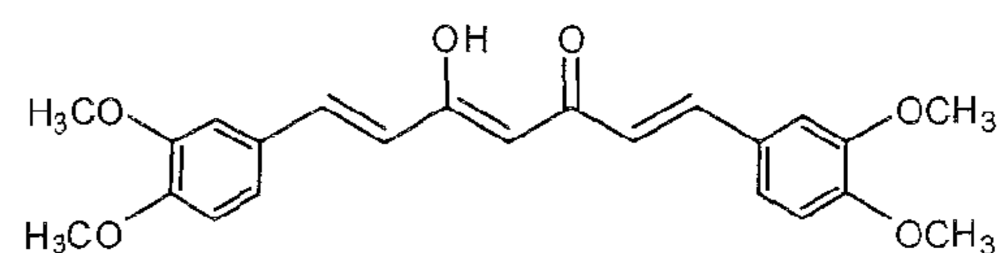
1,7-Bis-(3,4-dimethoxy-phenyl)-5-hydroxy-hepta-1,4,6-trien-3-one (dimethyl curcumin) (ASC-J9)
