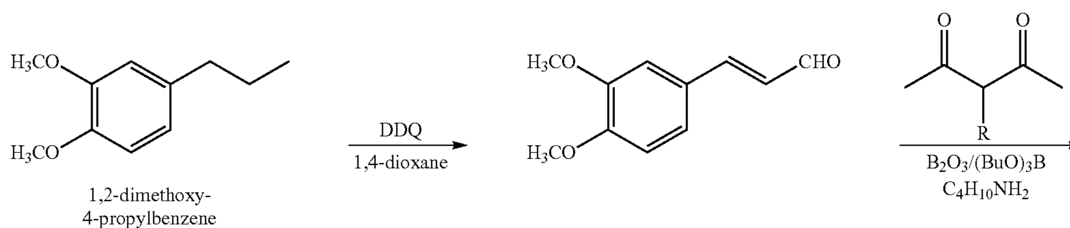
Scheme 20
