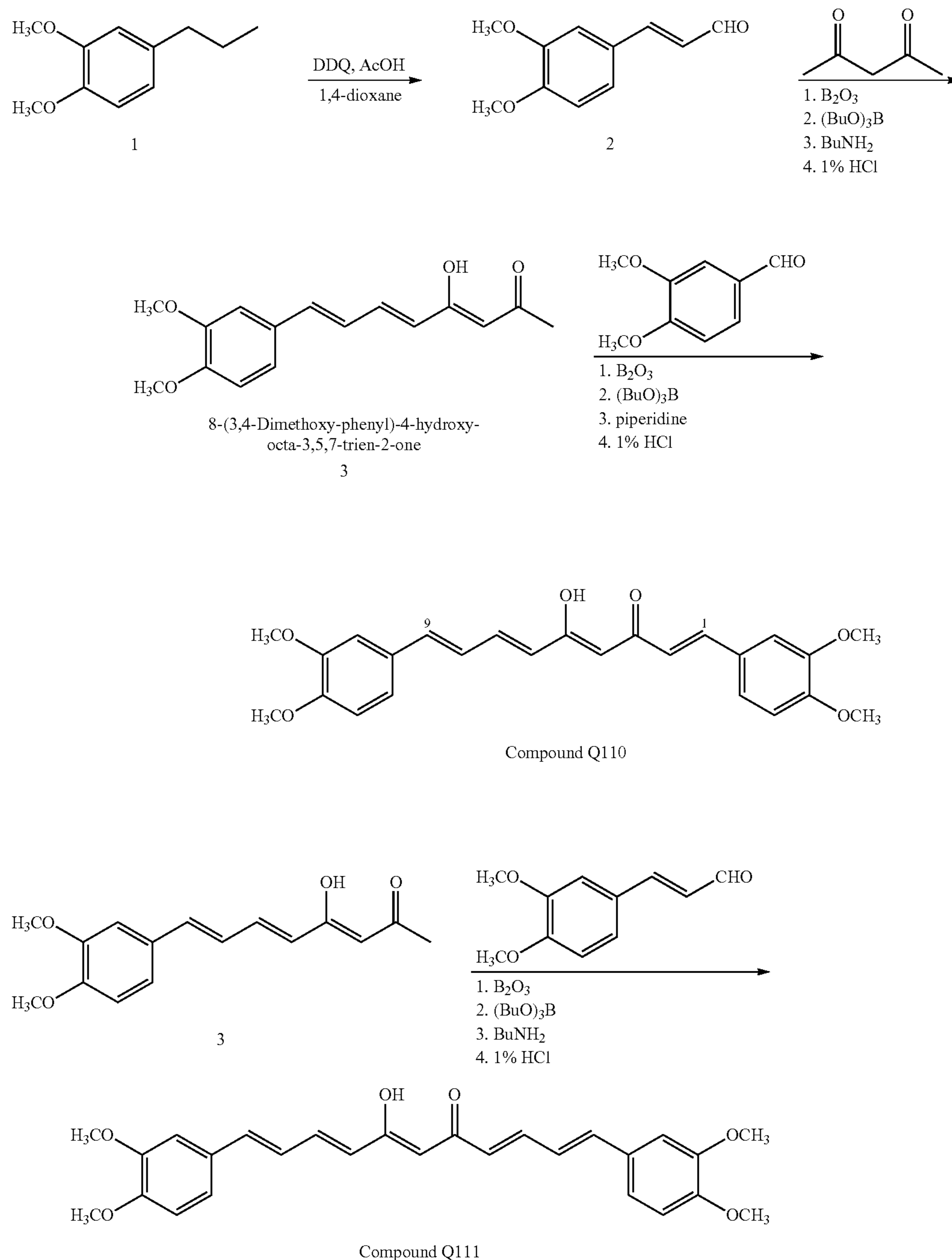
Scheme 13
