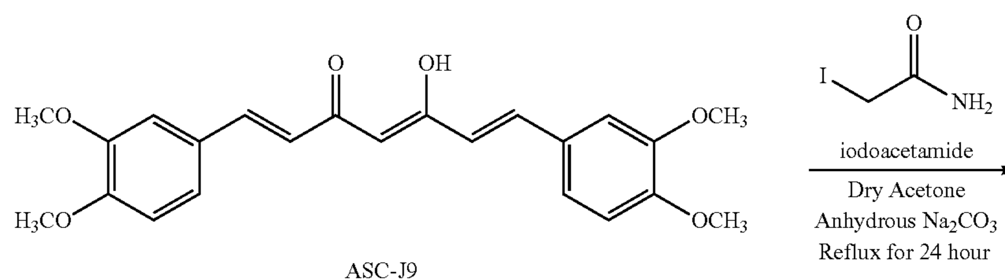
Scheme 7
