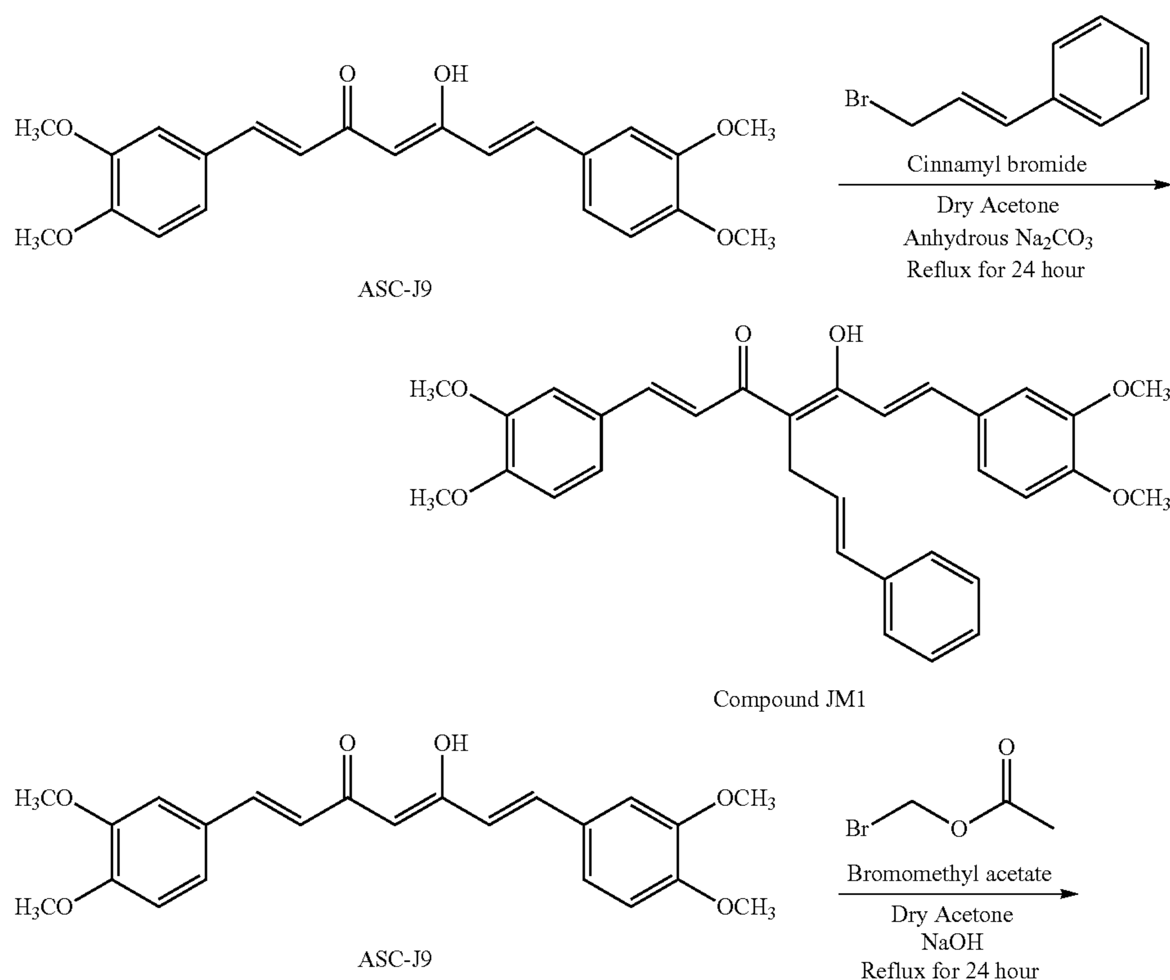
Scheme 9
