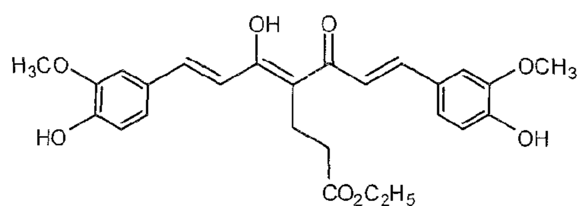
5-Hydroxy-7-(4-hydroxy-3-methoxy-phenyl)-4-[3-(4-hydroxy-3-methoxy-phenyl)-acryloyl]-hepta-4,6-dienoic acid ethyl ester (ASC-J15)
