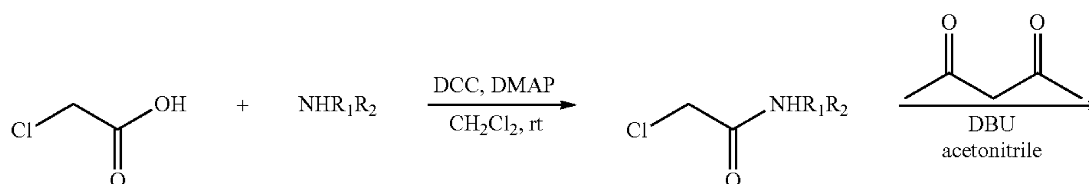
Scheme 15
