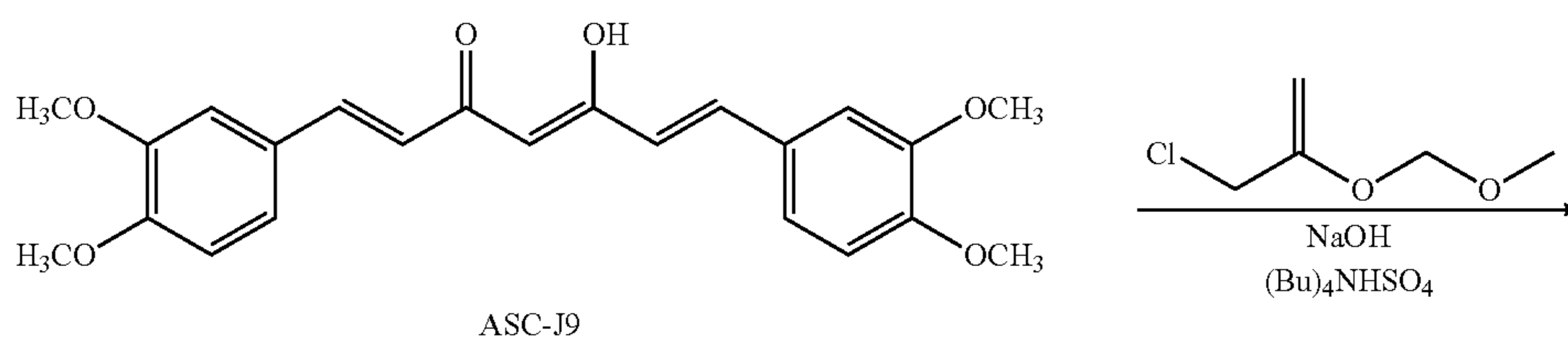
Scheme 6
