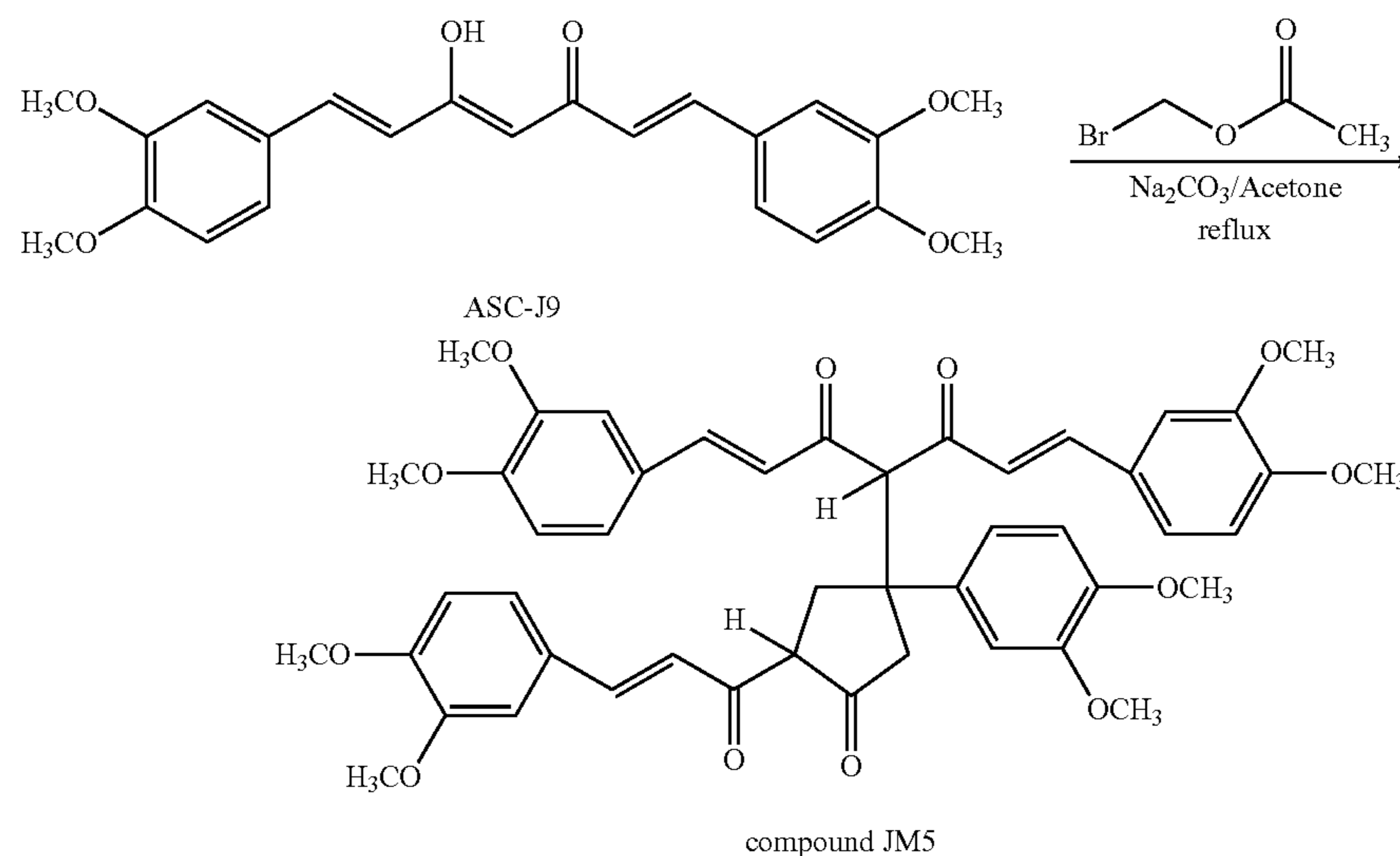
Scheme 12
