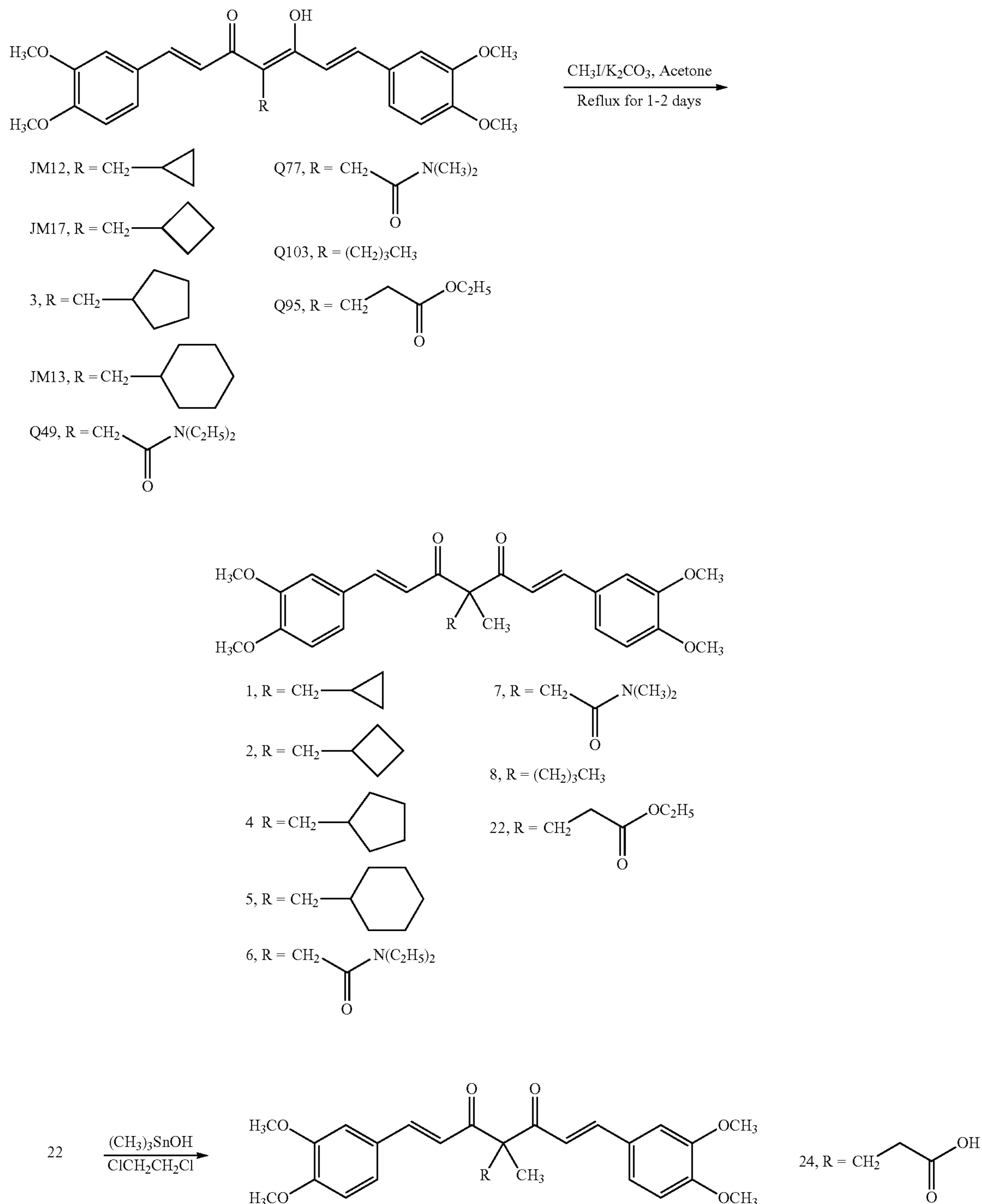
Scheme 14
