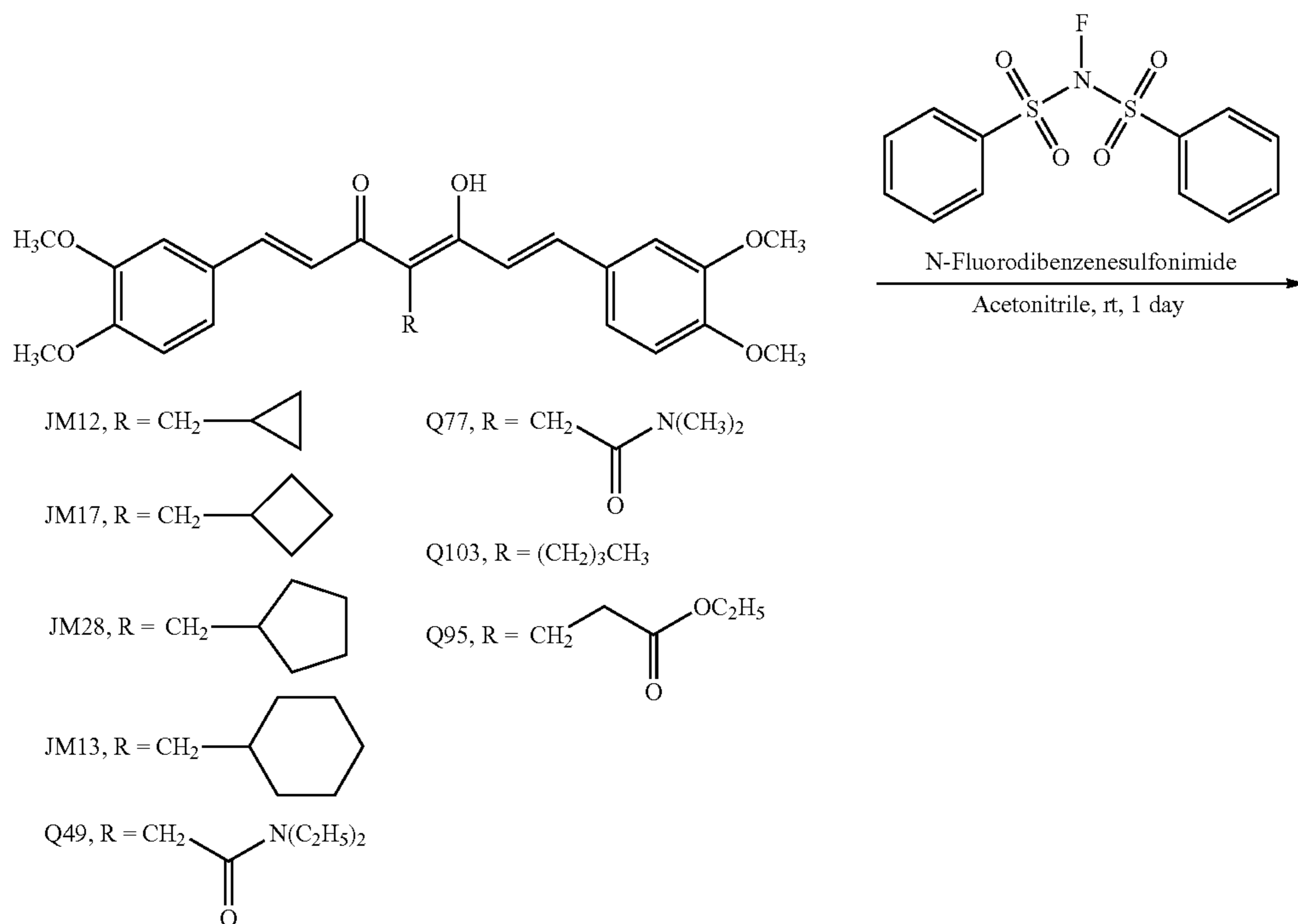
Scheme 16
