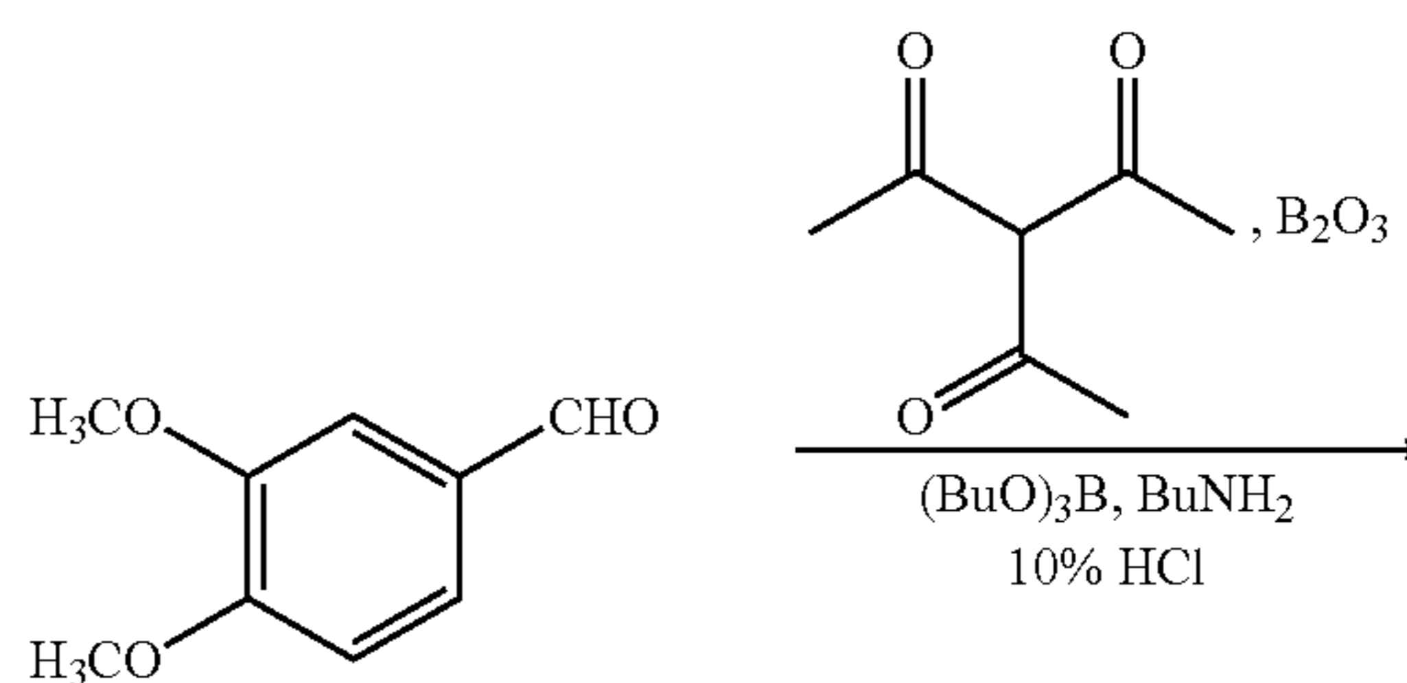
Scheme 11
