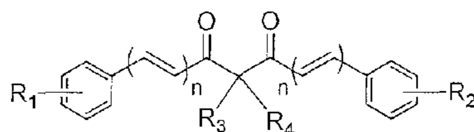
FIG. 10A. Summary of representative compounds including 4,4-disubstituted 1,7-bis-(3,4-dimethoxyphenyl)-hepta-1,6-diene-3,5-dione and 6,6-disubstituted 1,11-bis(substituted phenyl)-undeca-1,3,8,10-tetraene-5,7-dione scaffolds.
