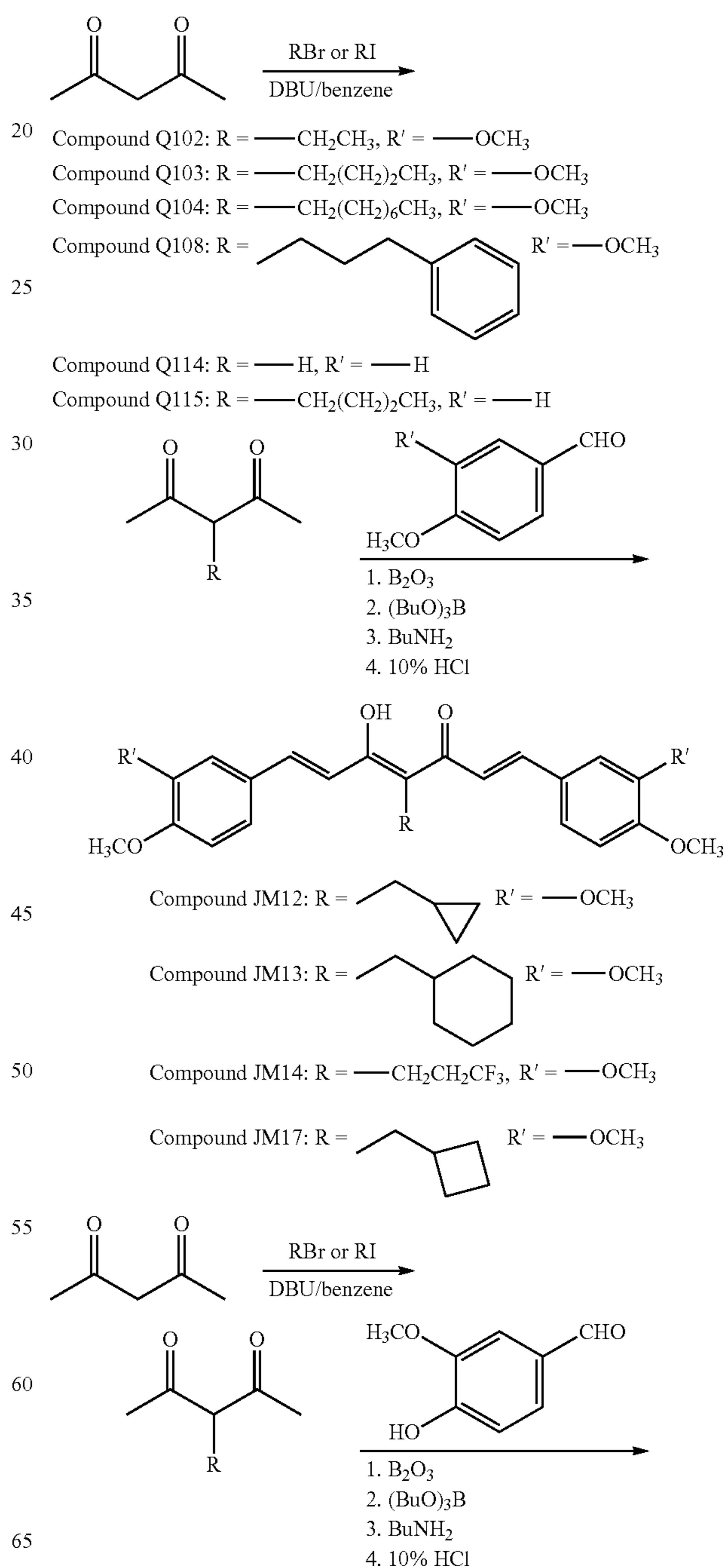
Scheme 10
