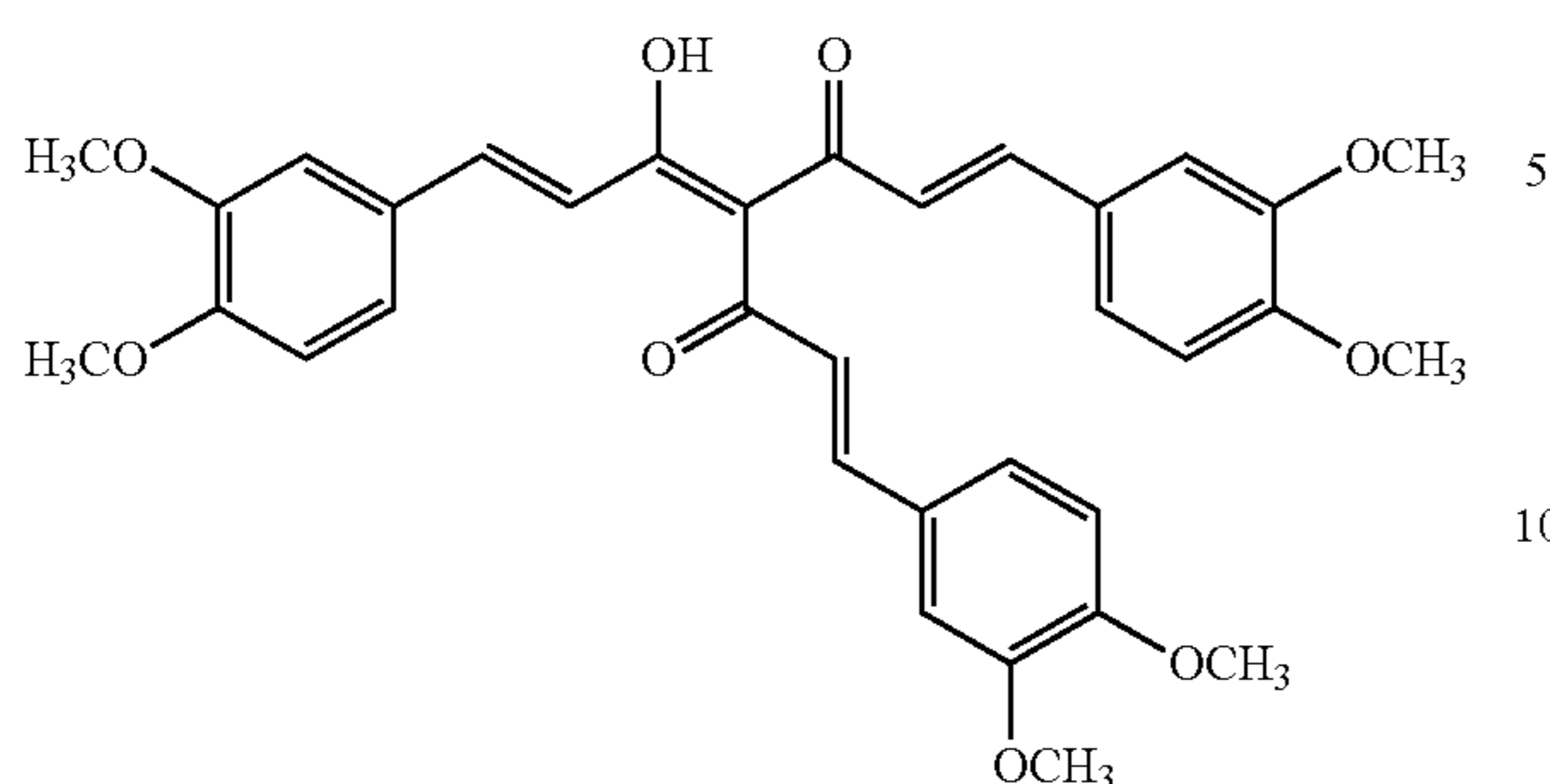
compound JM4
