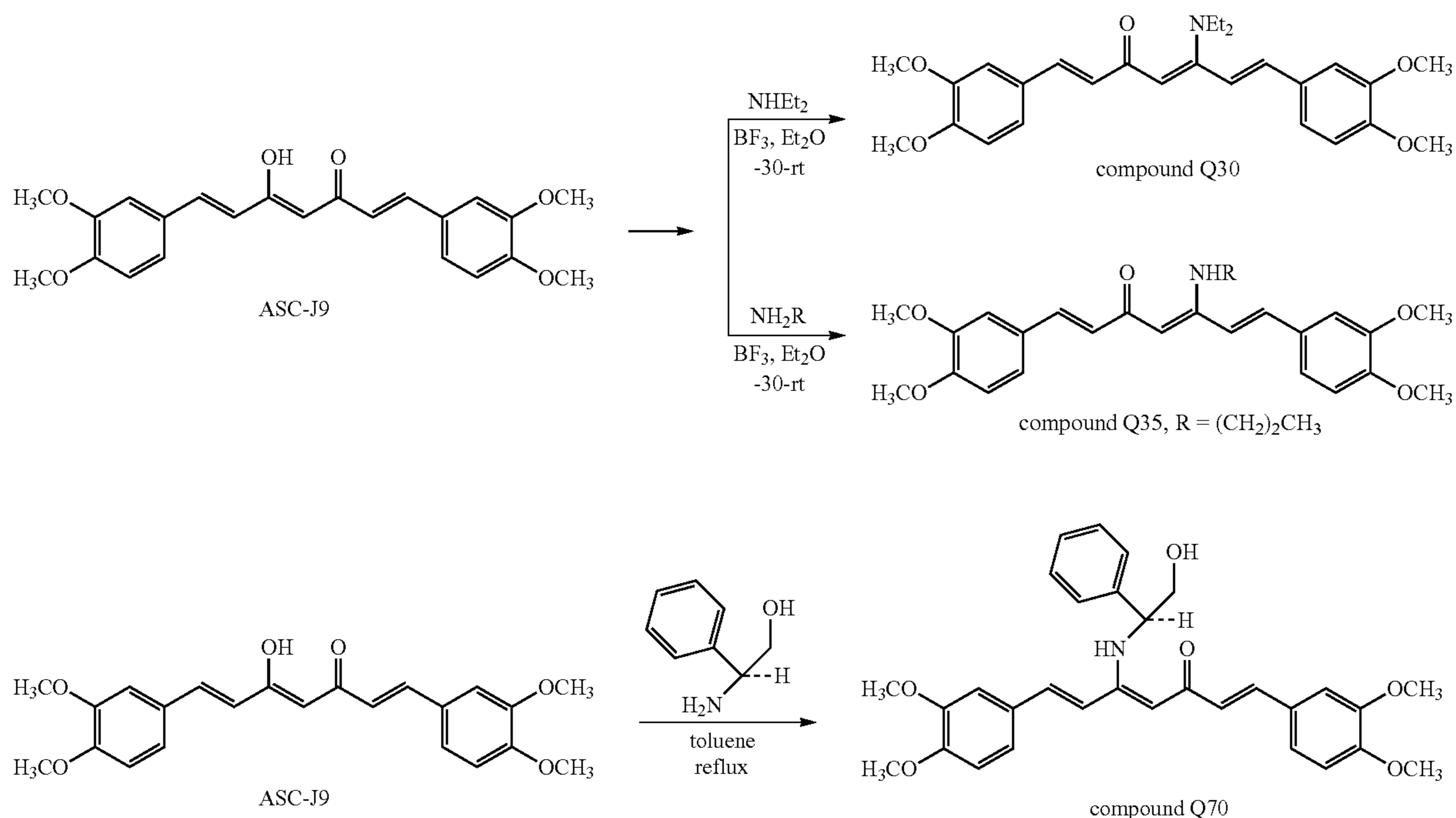
Scheme 5
