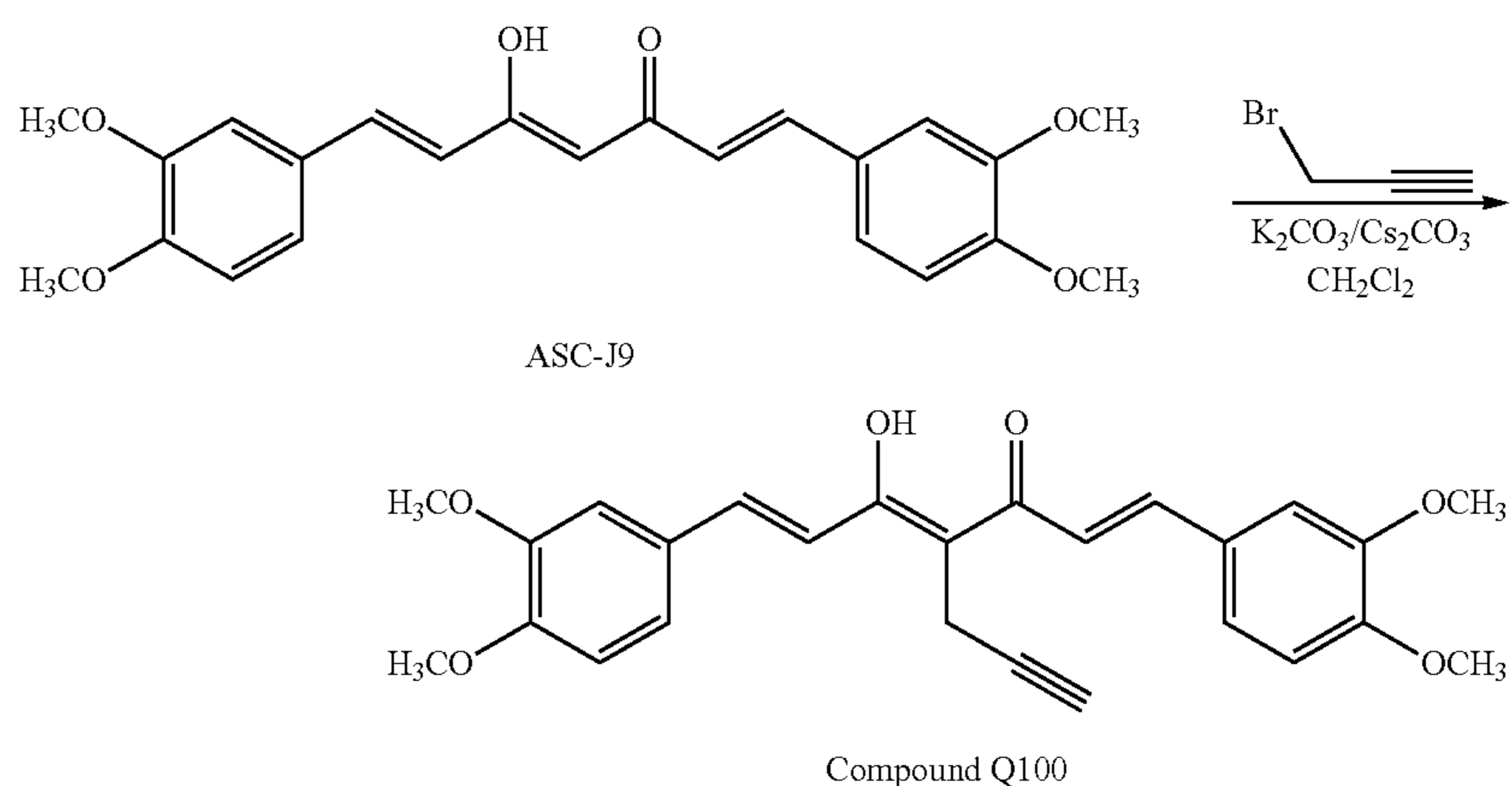
Scheme 8
