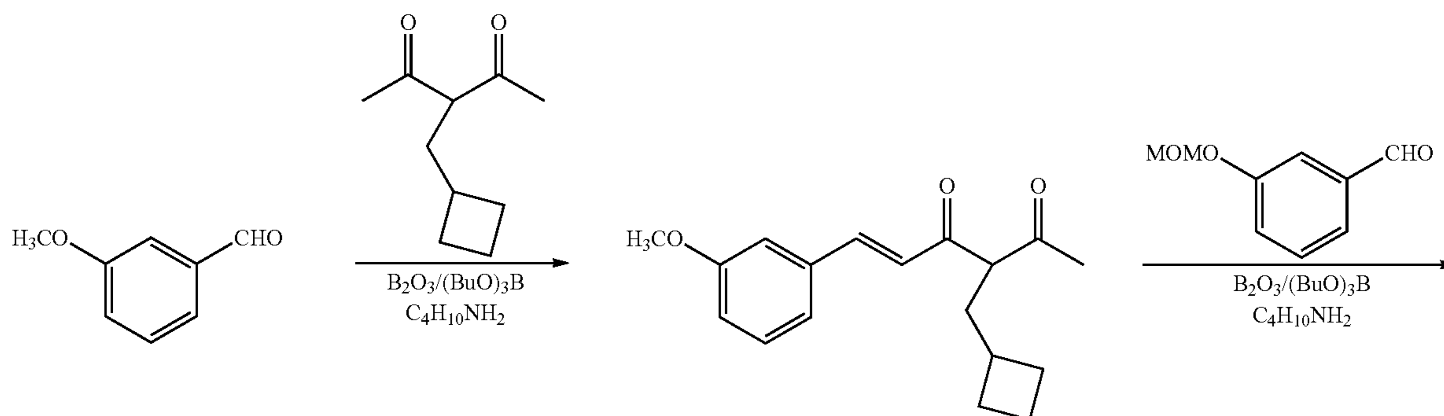
Scheme 19
