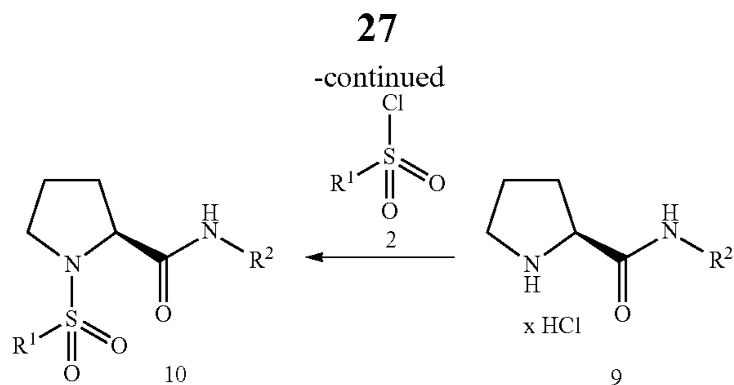
Scheme 2: Preparation of Compounds of Formula (I), Method B
