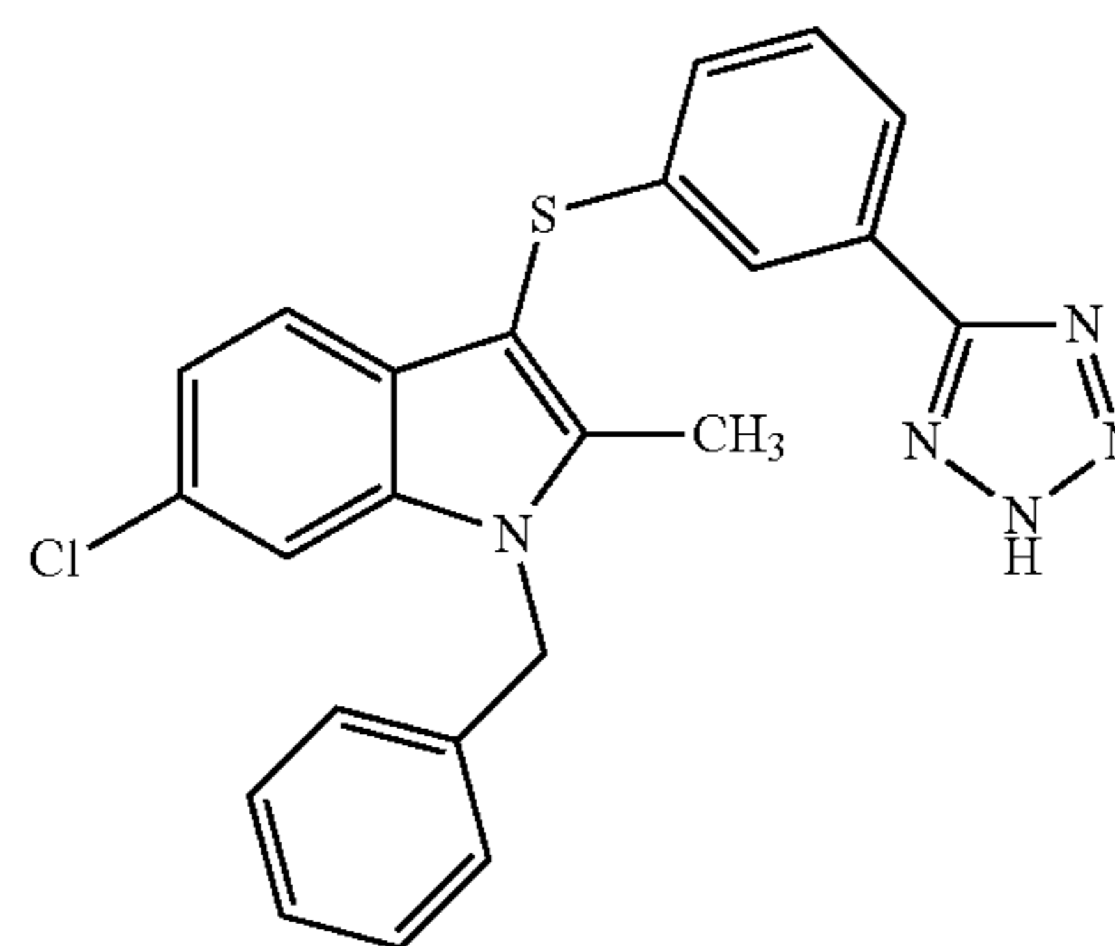
Step 3: 1-Benzyl-6-chloro-2-methyl-3-[3-(2H-tetrazol-5-yl)-phenylsulfanyl]-1H-indole
