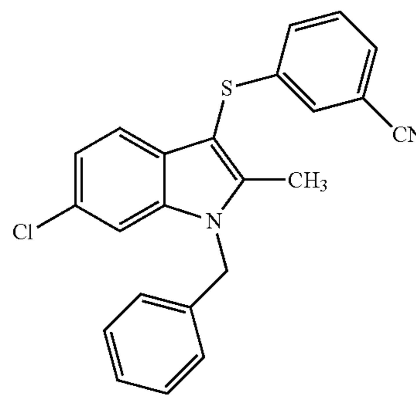
Step 2: 3-(1-Benzyl-6-chloro-2-methyl-1H-indol-3-ylsulfanyl)-benzonitrile
