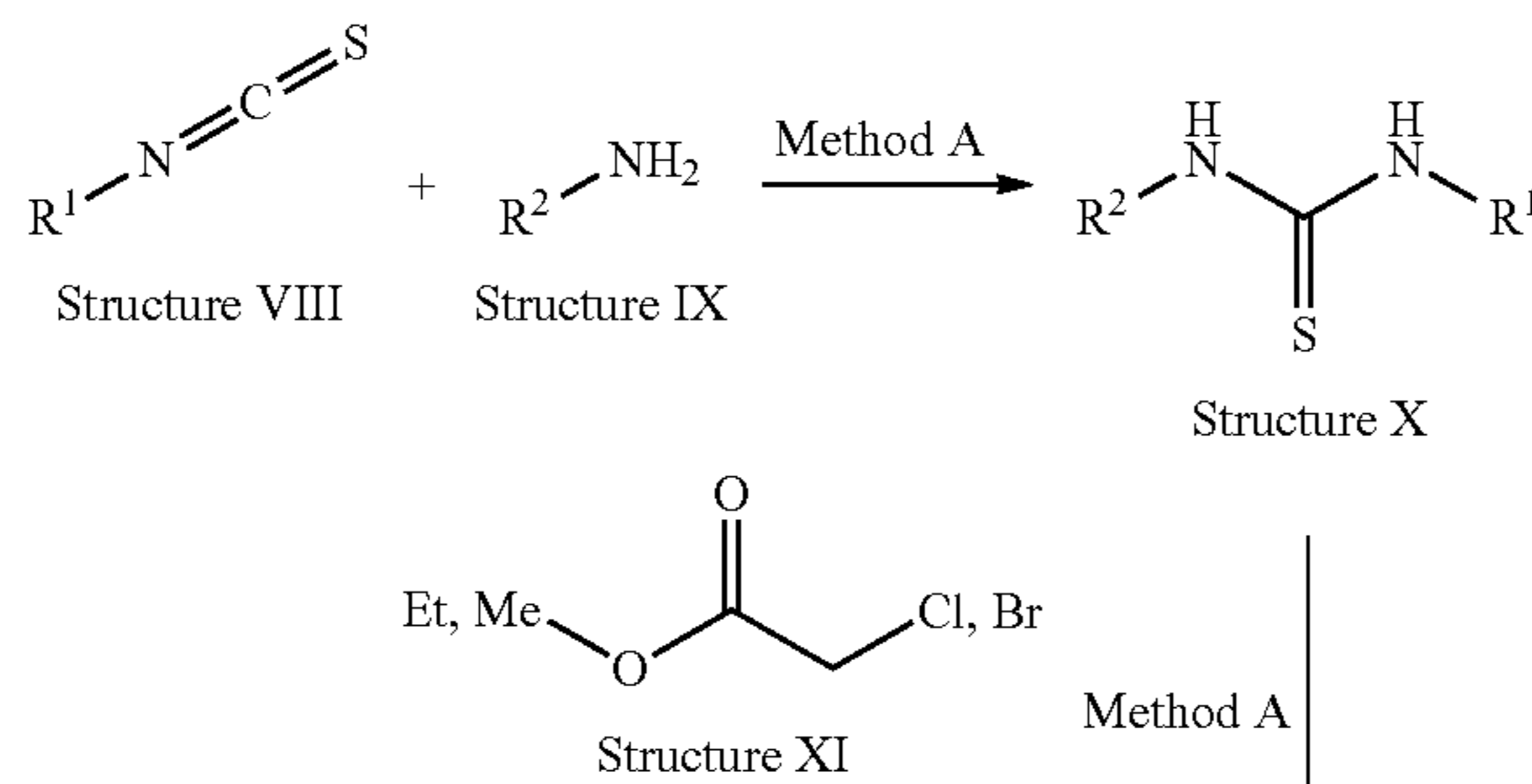
Scheme 1
