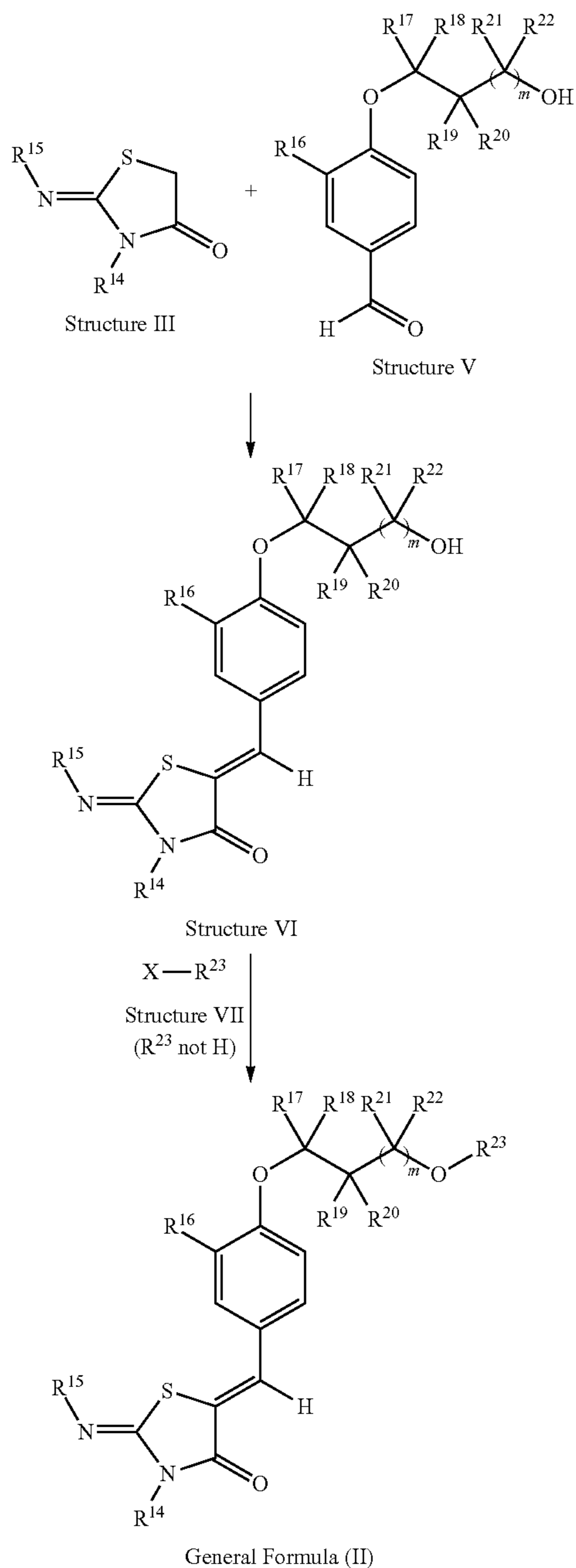
Scheme 3
