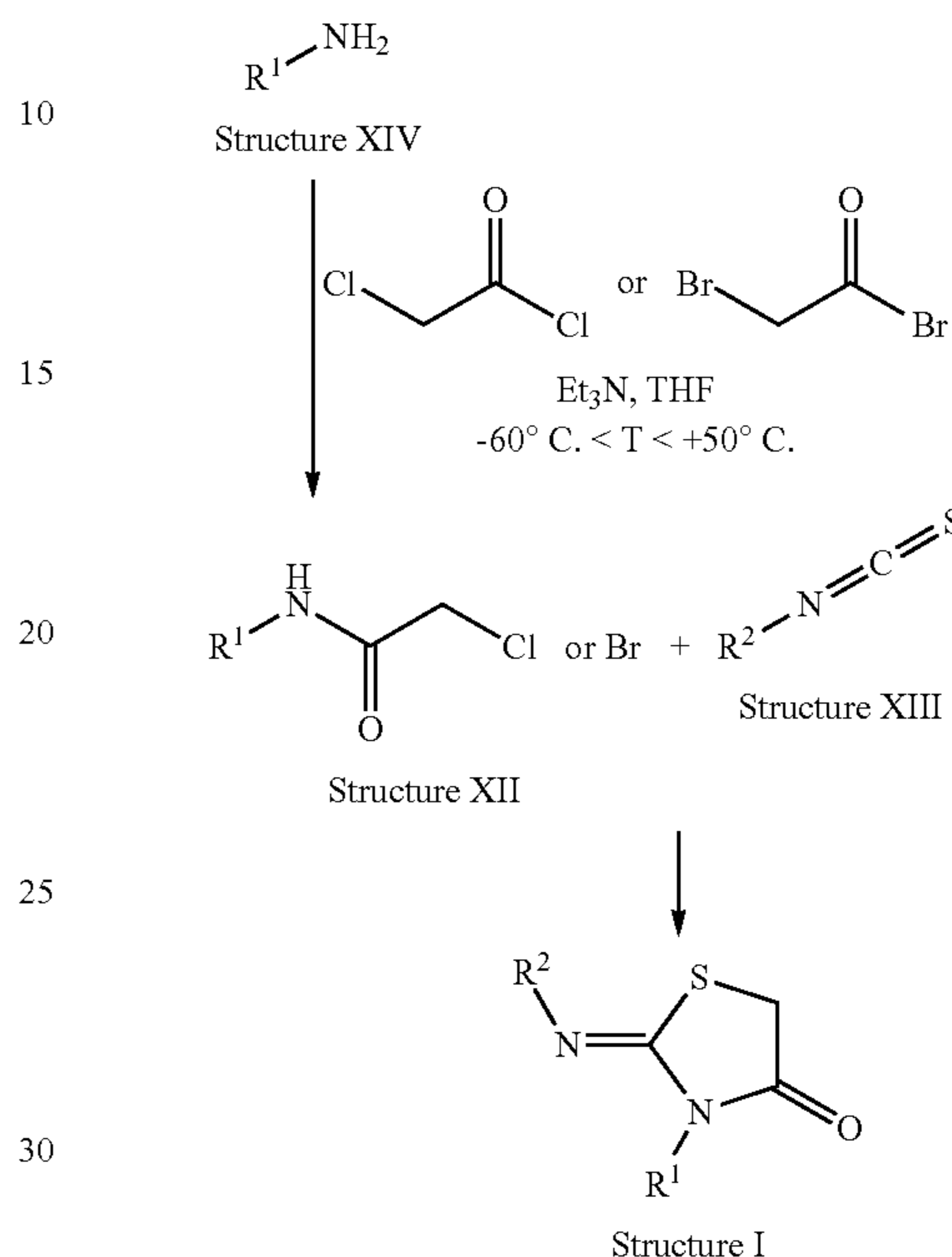
Scheme 4
