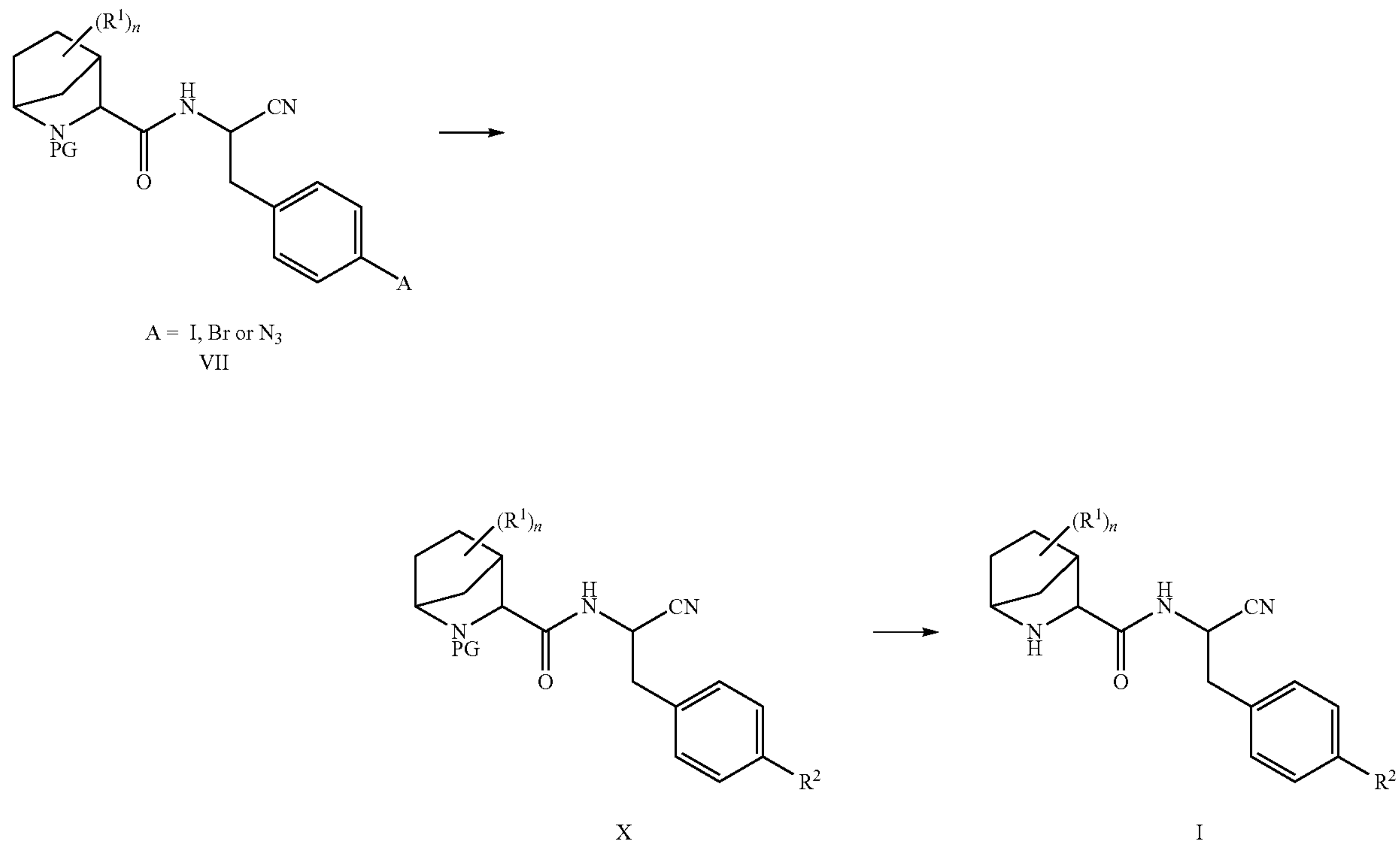
Scheme 2
