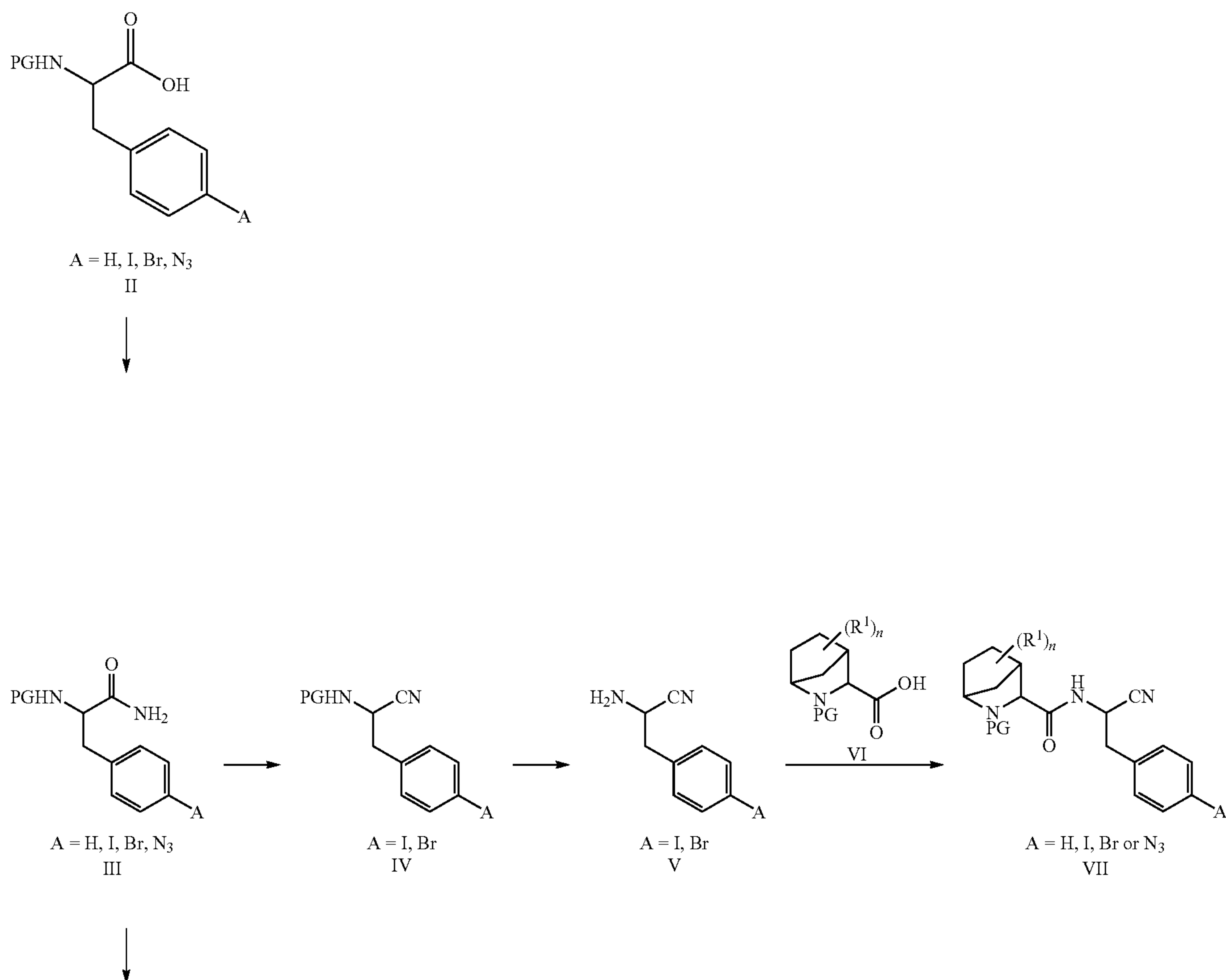
Scheme 1
