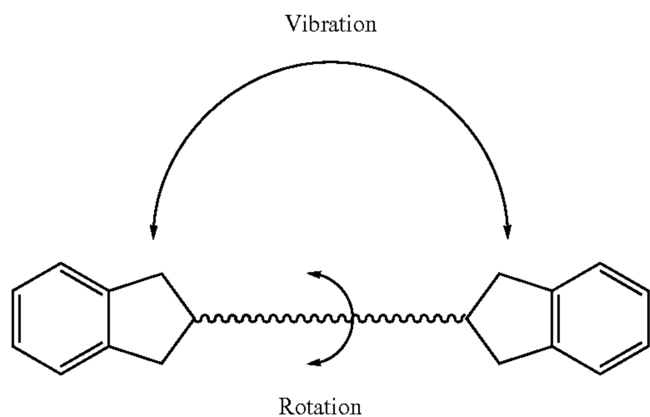
Scheme 1. 'Loose Belt Effect' through vibration and rotation around the middle conjugated double bonds
