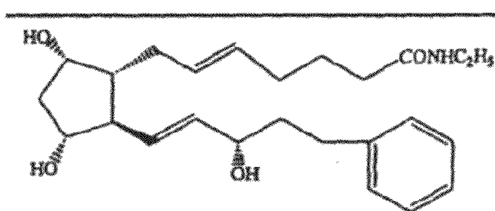
5,6-trans AGN 192024 isomer
