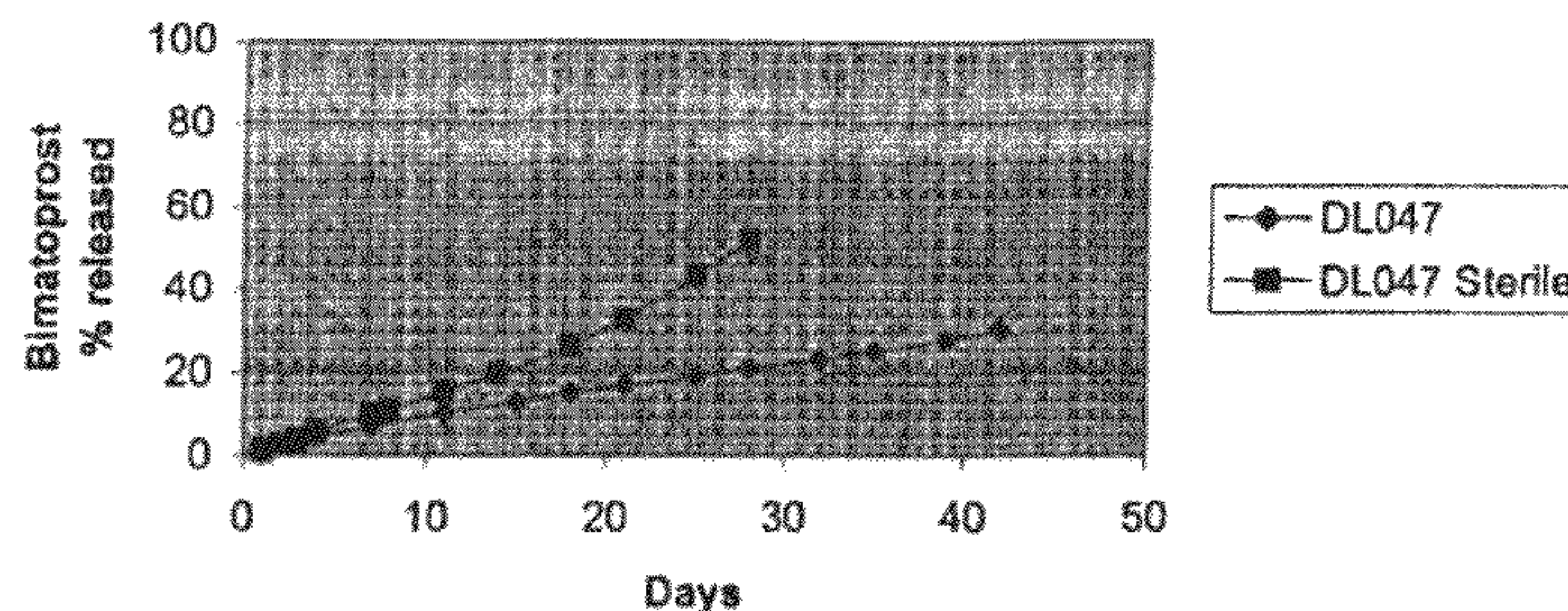
Bimatoprost release profile (Cumulative % released)
