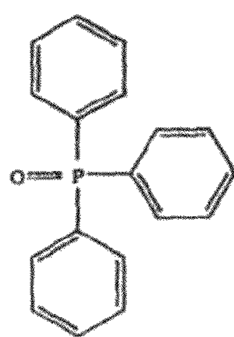
triphenylphosphine Oxide (TPPO)
