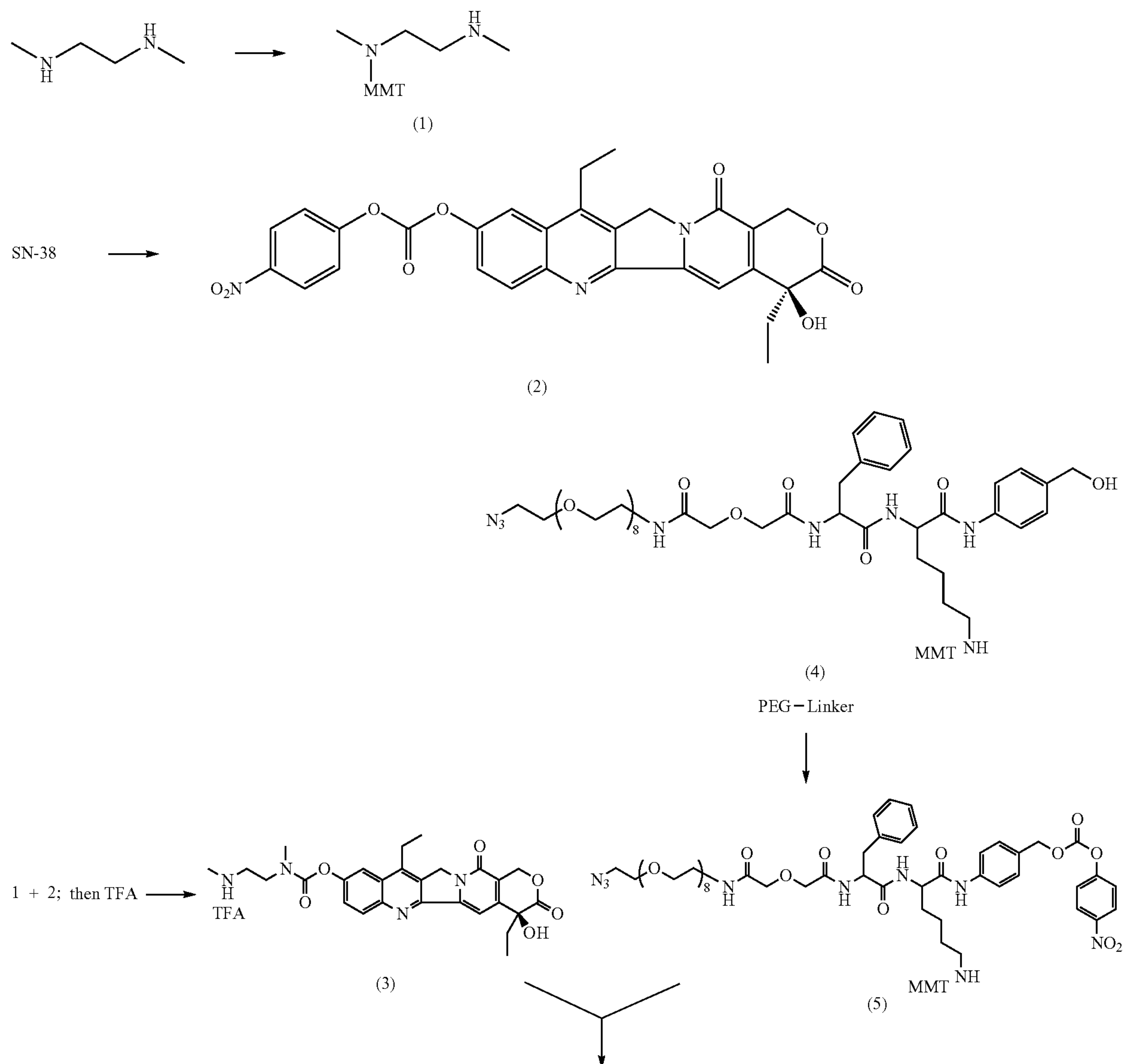
Scheme-4: Preparation of CL2E-SN-38
